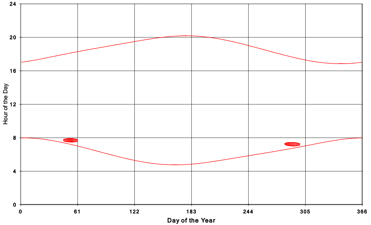
Goshen Wind Energy Centre Shadow Times on House 2160, All Windows from All Turbine
