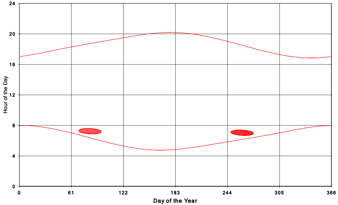
Jericho Wind Energy Centre Shadow Times on House 2114, All Windows from All Turbine
