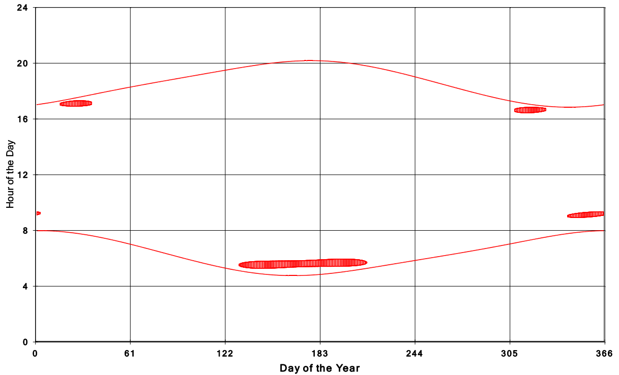
Jericho Wind Energy Centre Shadow Times on House 2115, All Windows from All Turbine
