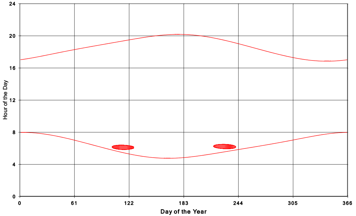
Goshen Wind Energy Centre Shadow Times on House 2131, All Windows from All Turbine
