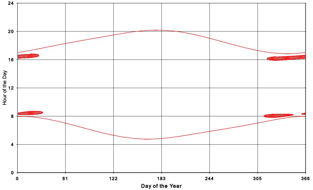
Goshen Wind Energy Centre Shadow Times on House 2080, All Windows from All Turbine
