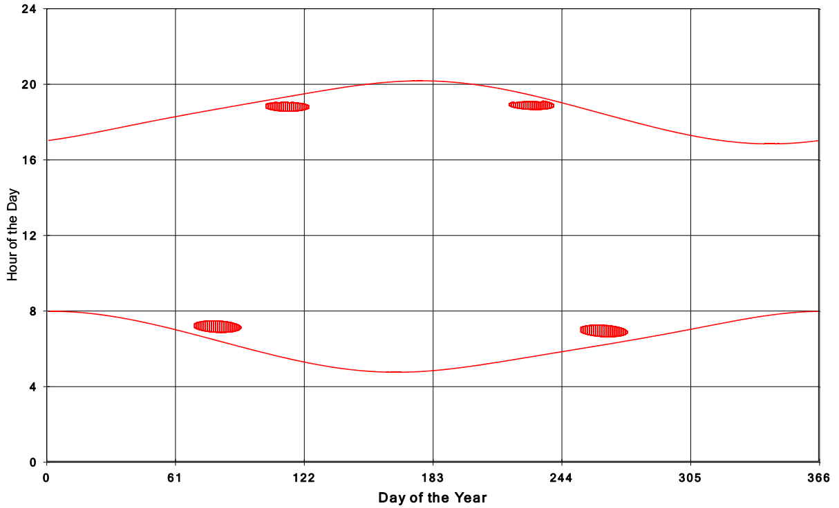
Goshen Wind Energy Centre Shadow Times on House 2138, All Windows from All Turbine
