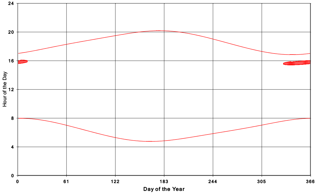
Goshen Wind Energy Centre Shadow Times on House 2178, All Windows from All Turbine
