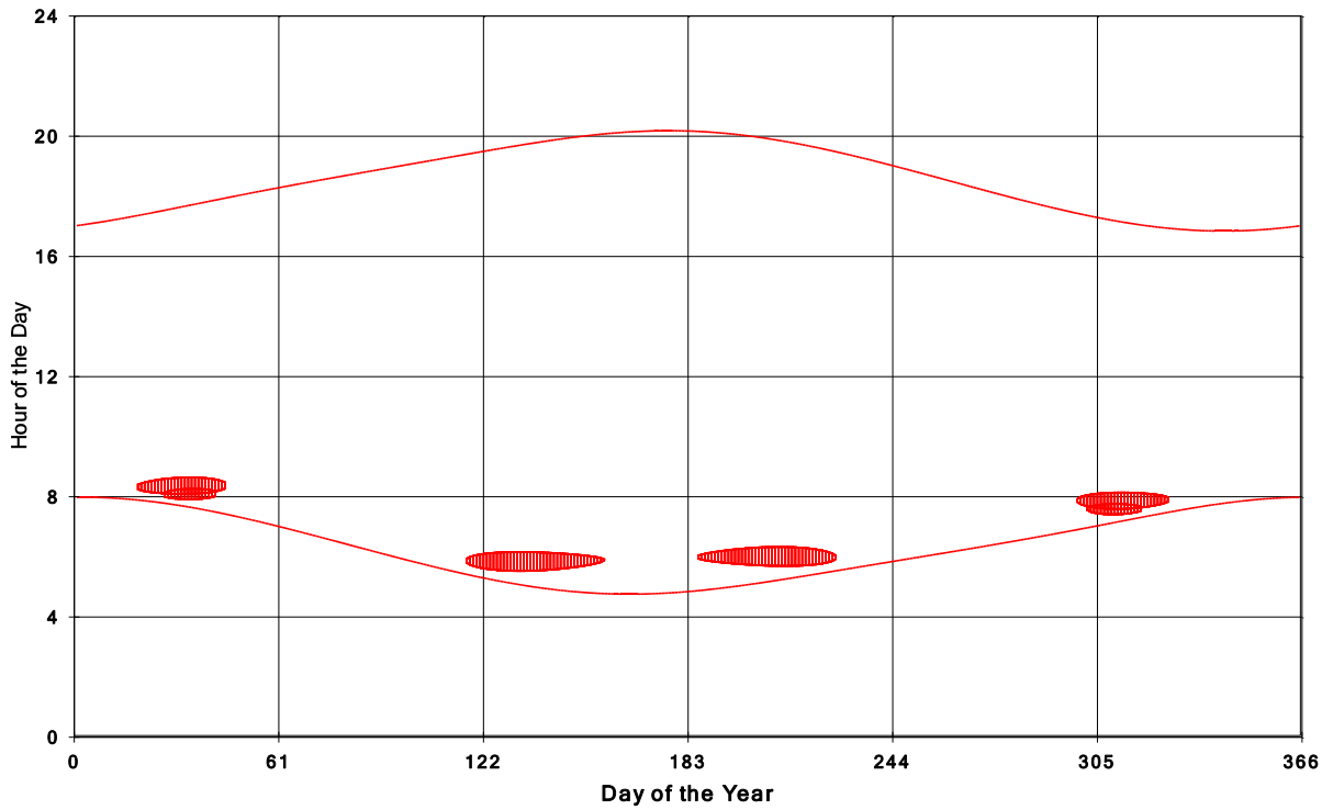
Goshen Wind Energy Centre Shadow Times on House 2081, All Windows from All Turbine
