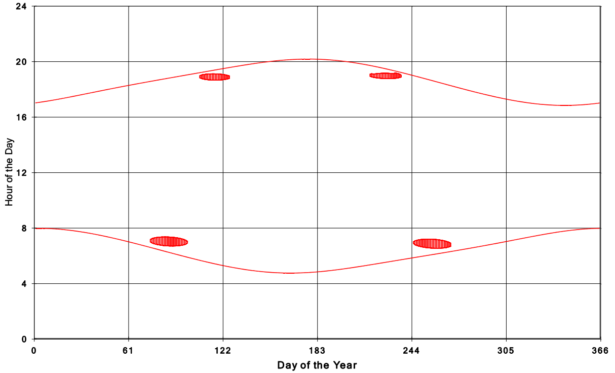
Goshen Wind Energy Centre Shadow Times on House 2139, All Windows from All Turbine
