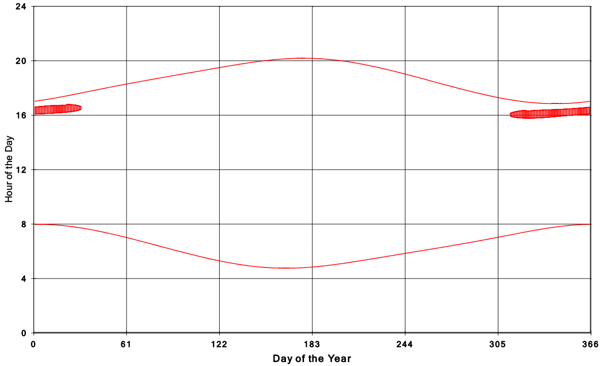
Goshen Wind Energy Centre Shadow Times on House 2203, All Windows from All Turbine
