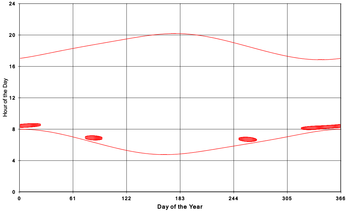
Goshen Wind Energy Centre Shadow Times on House 2148, All Windows from All Turbine
