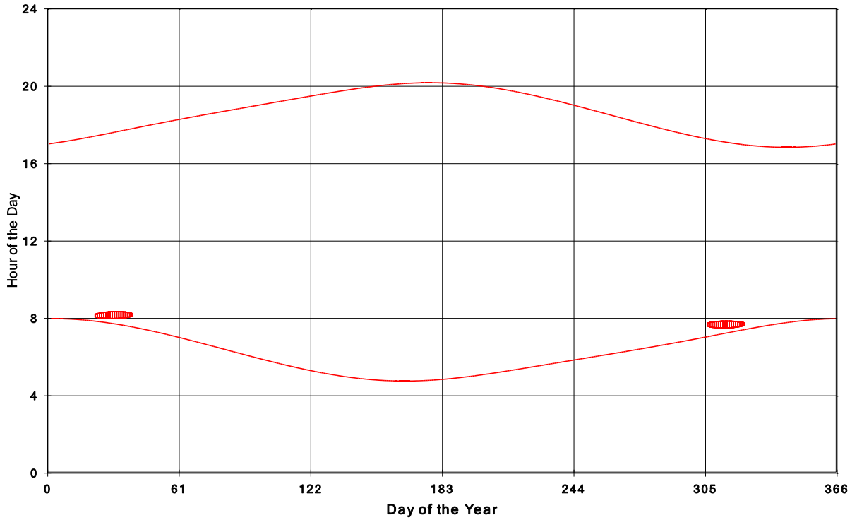
Goshen Wind Energy Centre Shadow Times on House 2174, All Windows from All Turbine
