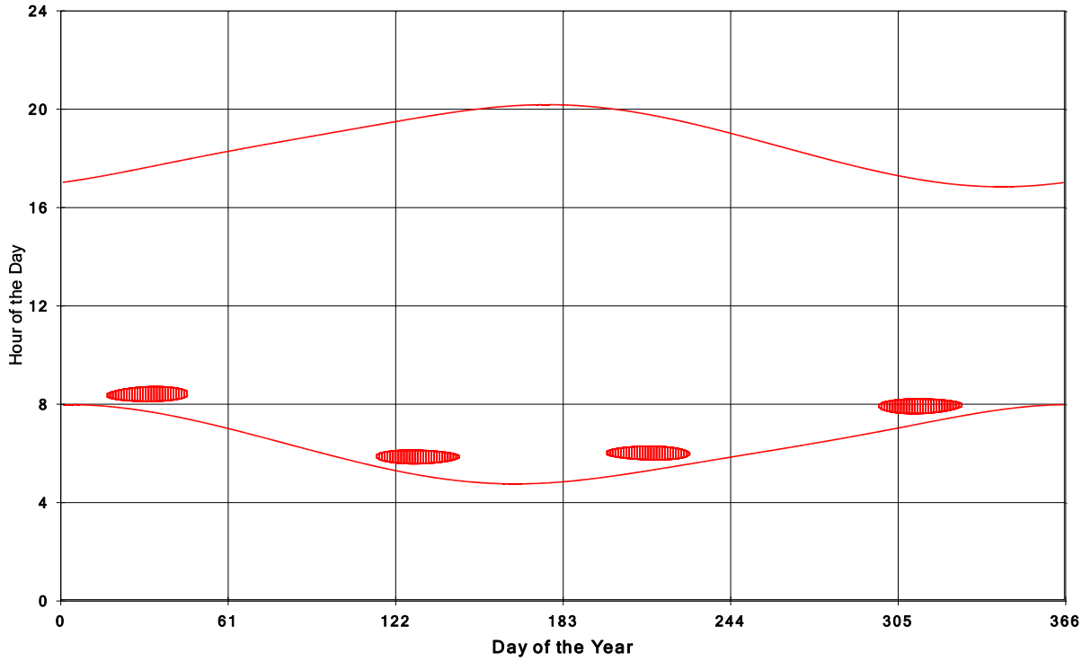
Goshen Wind Energy Centre Shadow Times on House 2116, All Windows from All Turbine
