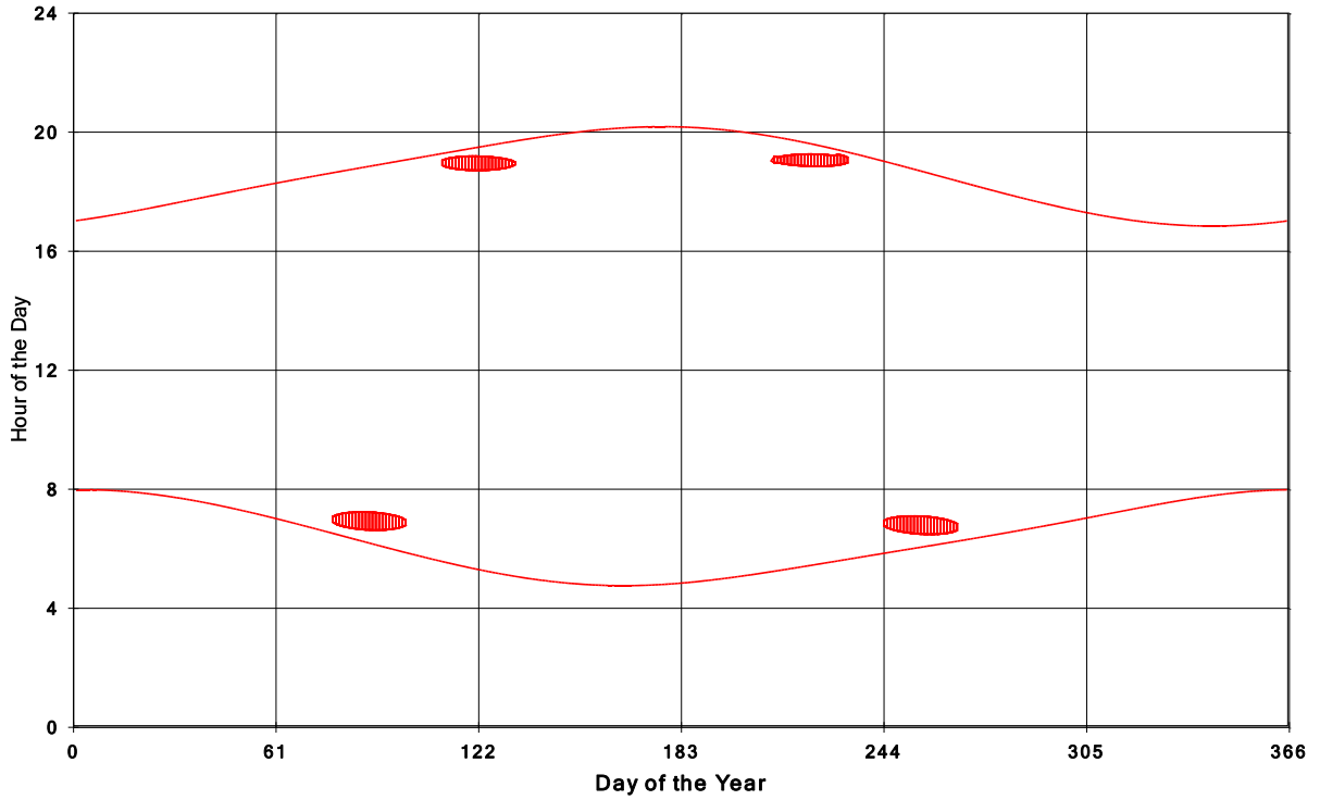
Goshen Wind Energy Centre Shadow Times on House 2137, All Windows from All Turbine
