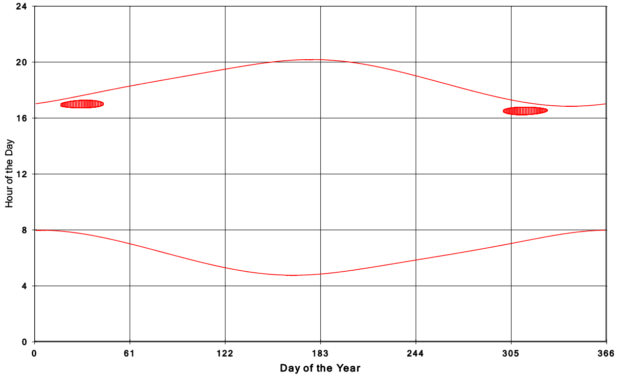
Goshen Wind Energy Centre Shadow Times on House 2135, All Windows from All Turbine
