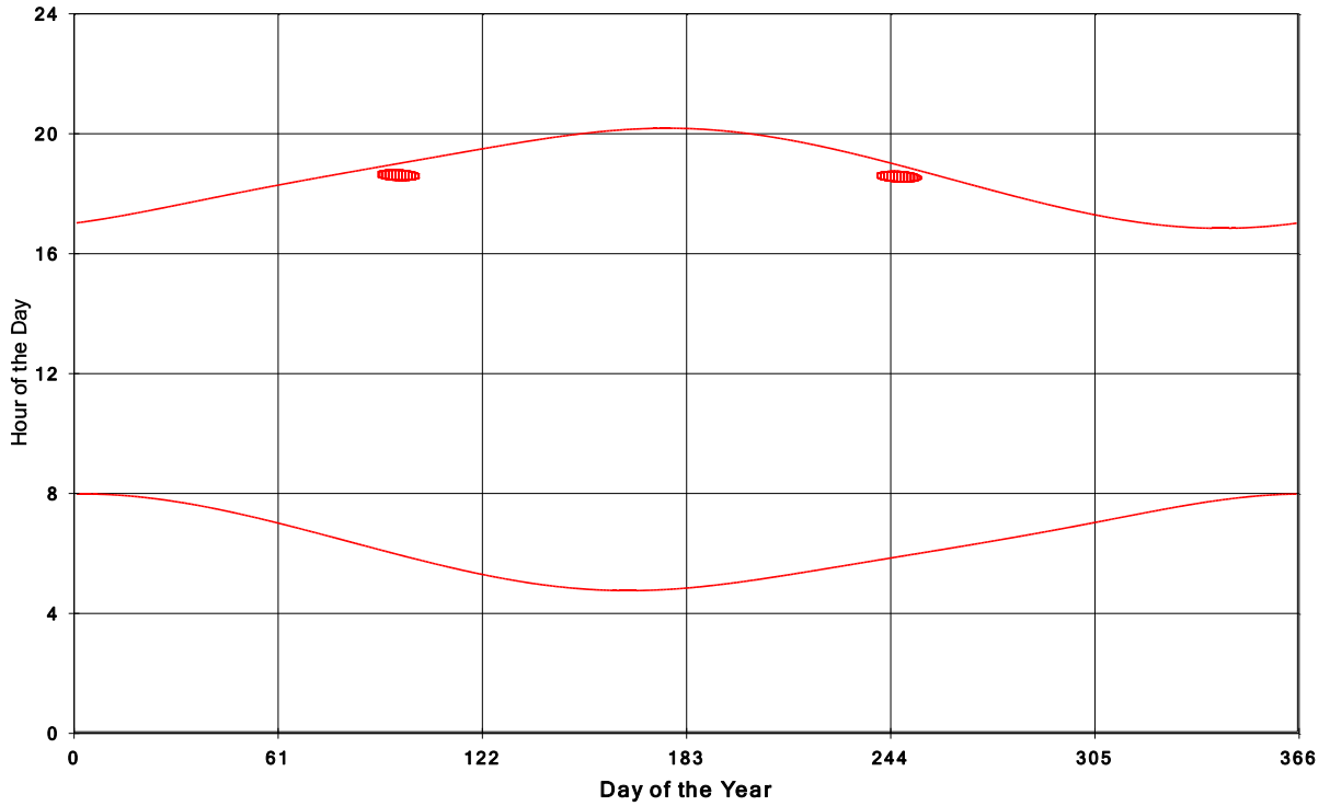
Goshen Wind Energy Centre Shadow Times on House 2185, All Windows from All Turbine
