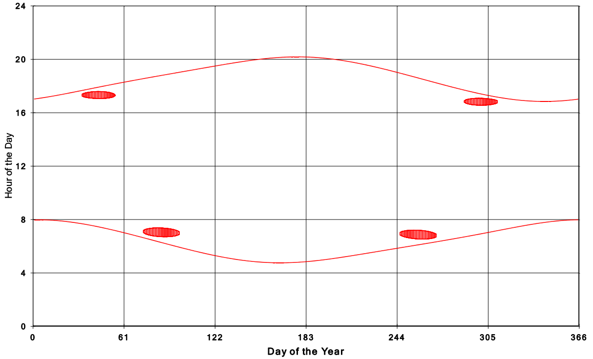
Goshen Wind Energy Centre Shadow Times on House 2191, All Windows from All Turbine
