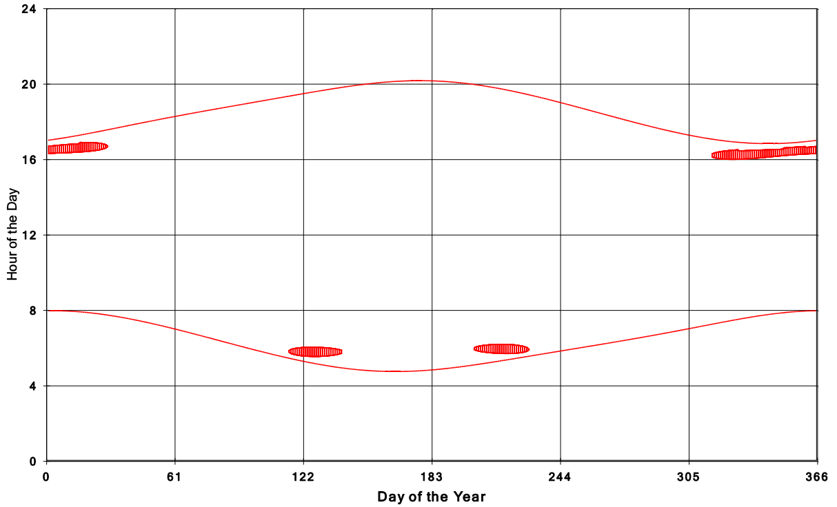
Goshen Wind Energy Centre Shadow Times on House 2153, All Windows from All Turbine
