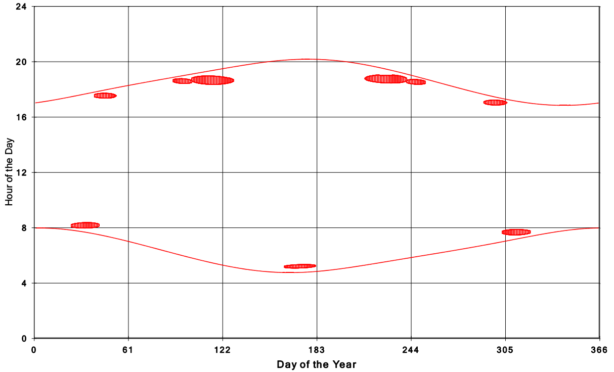
Goshen Wind Energy Centre Shadow Times on House 2194, All Windows from All Turbine
