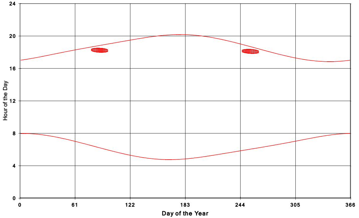
Goshen Wind Energy Centre Shadow Times on House 2202, All Windows from All Turbine
