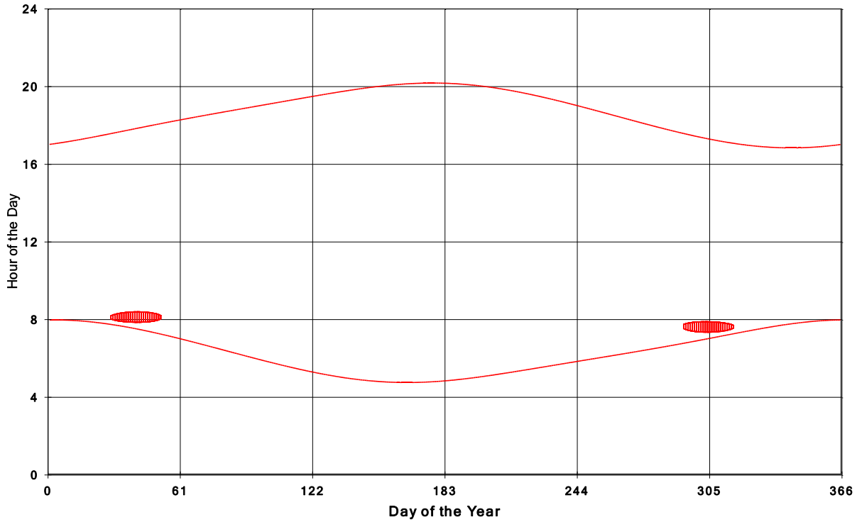
Goshen Wind Energy Centre Shadow Times on House 2162, All Windows from All Turbine
