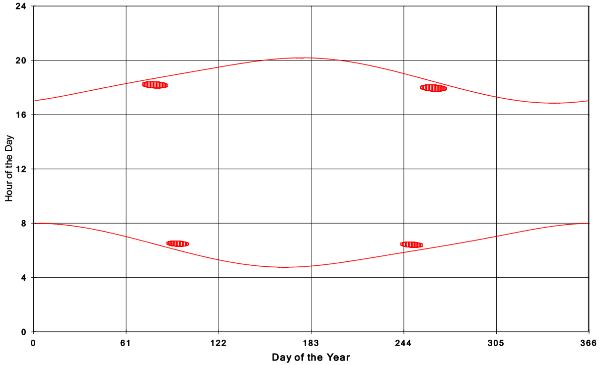
Goshen Wind Energy Centre Shadow Times on House 2152, All Windows from All Turbine
