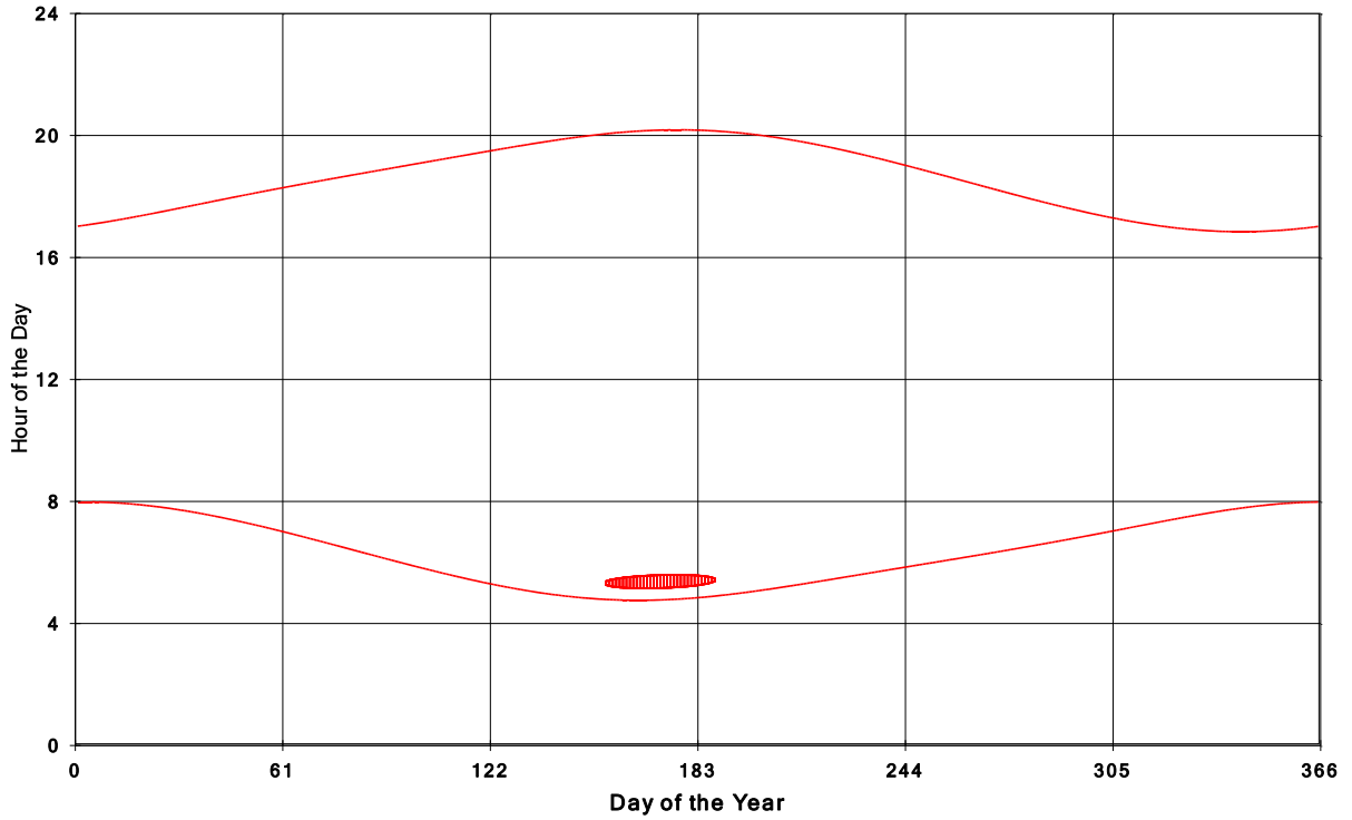
Goshen Wind Energy Centre Shadow Times on House 2087, All Windows from All Turbine
