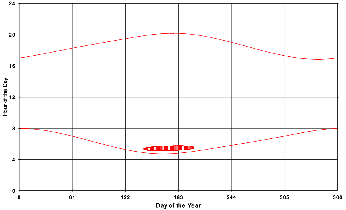
Goshen Wind Energy Centre Shadow Times on House 2101, All Windows from All Turbine
