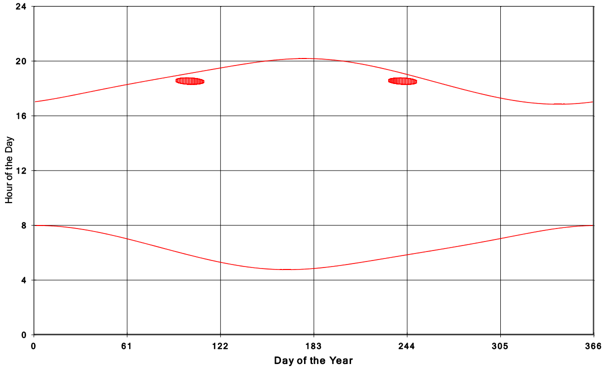
Goshen Wind Energy Centre Shadow Times on House 2168, All Windows from All Turbine
