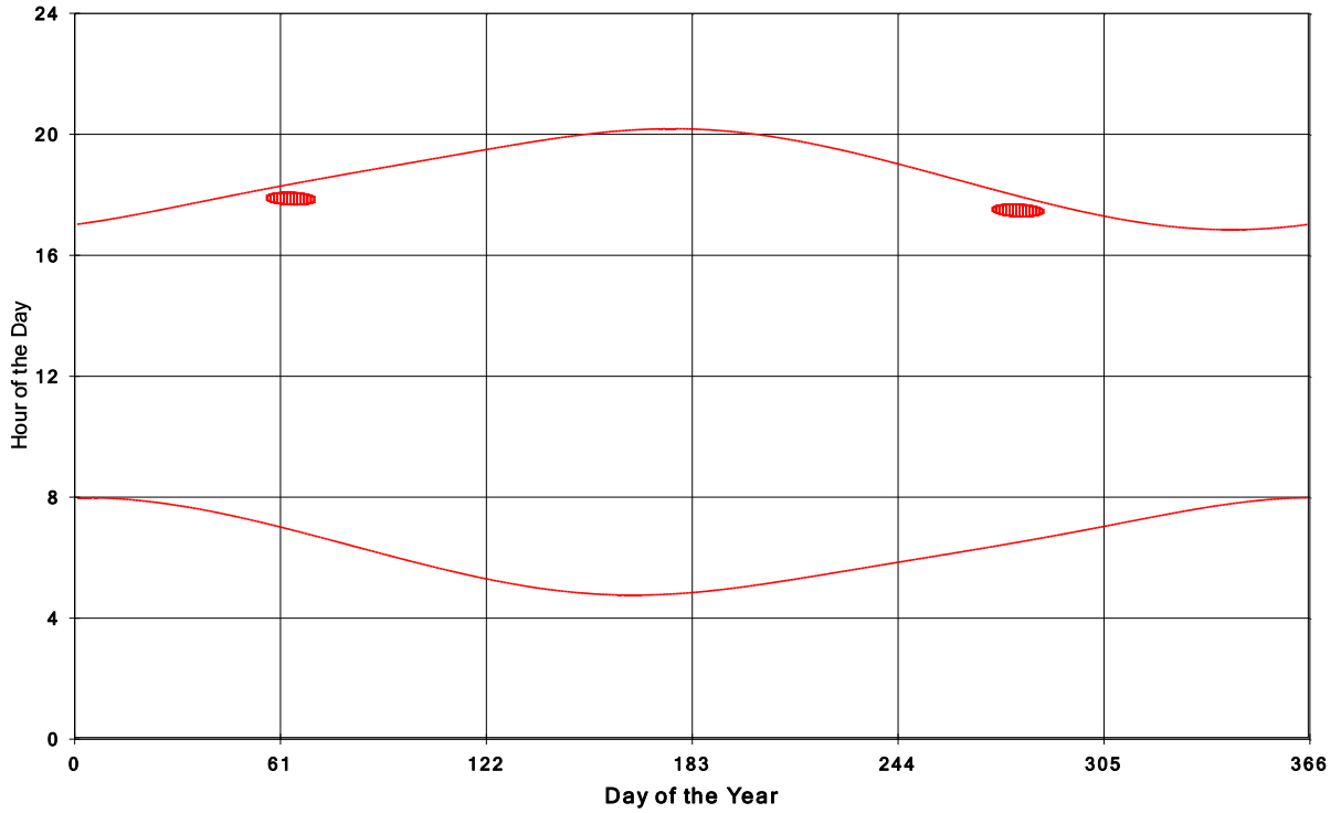
Goshen Wind Energy Centre Shadow Times on House 2167, All Windows from All Turbine
