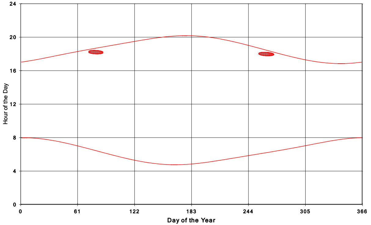
Goshen Wind Energy Centre Shadow Times on House 2090, All Windows from All Turbine
