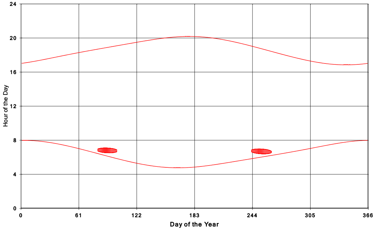
Goshen Wind Energy Centre Shadow Times on House 2117, All Windows from All Turbine
