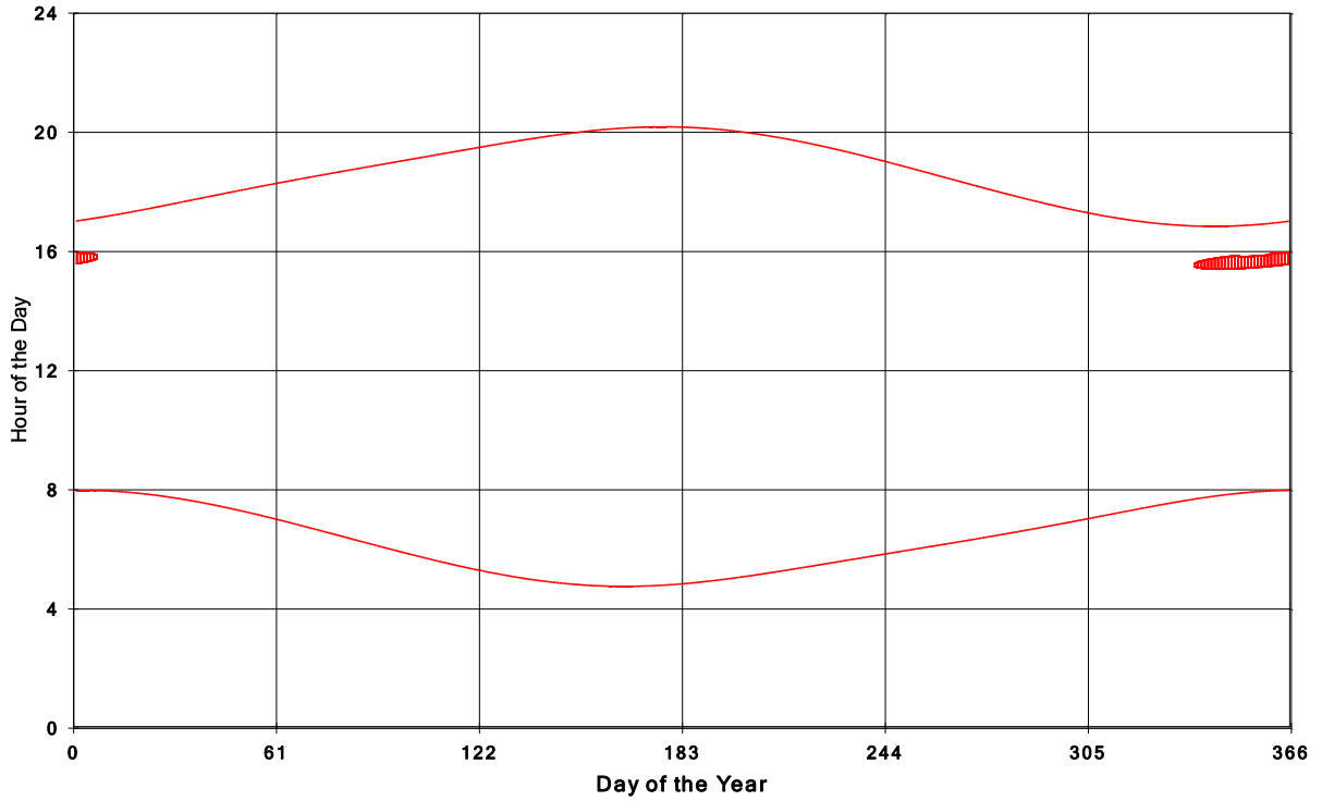
Goshen Wind Energy Centre Shadow Times on House 2177, All Windows from All Turbine
