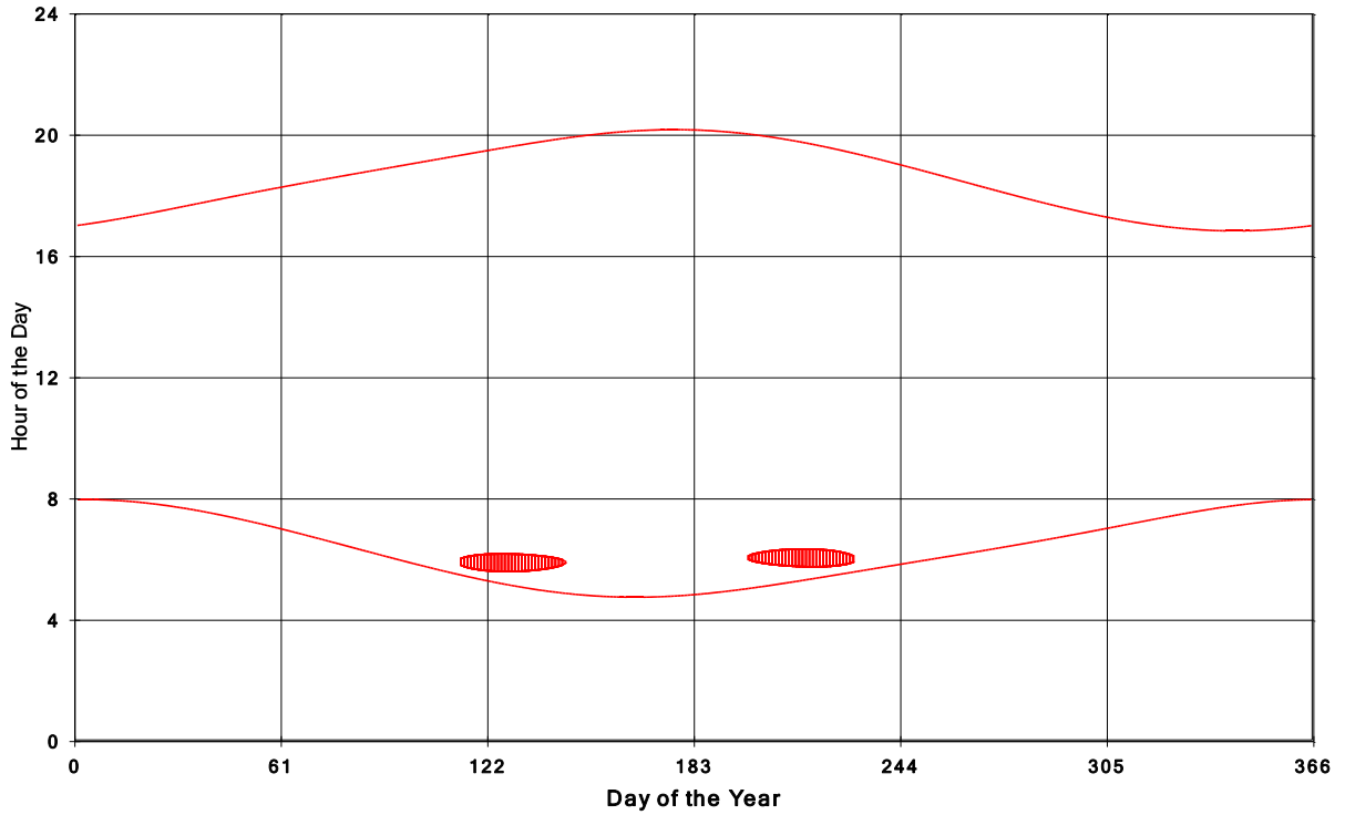
Goshen Wind Energy Centre Shadow Times on House 2107, All Windows from All Turbine
