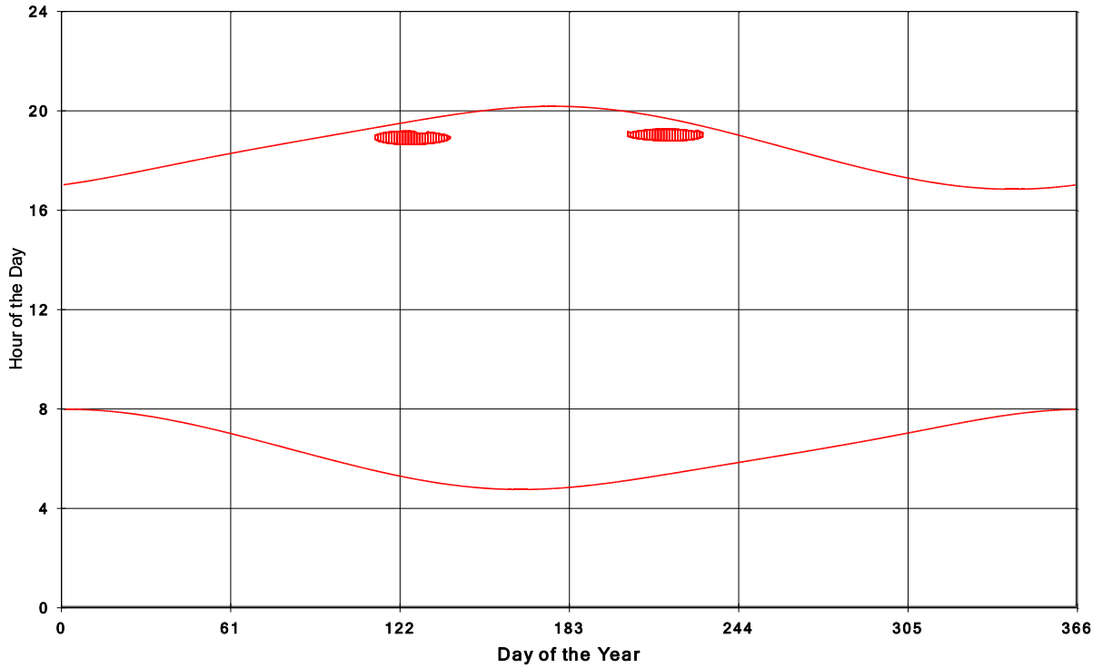
Goshen Wind Energy Centre Shadow Times on House 2201, All Windows from All Turbine
