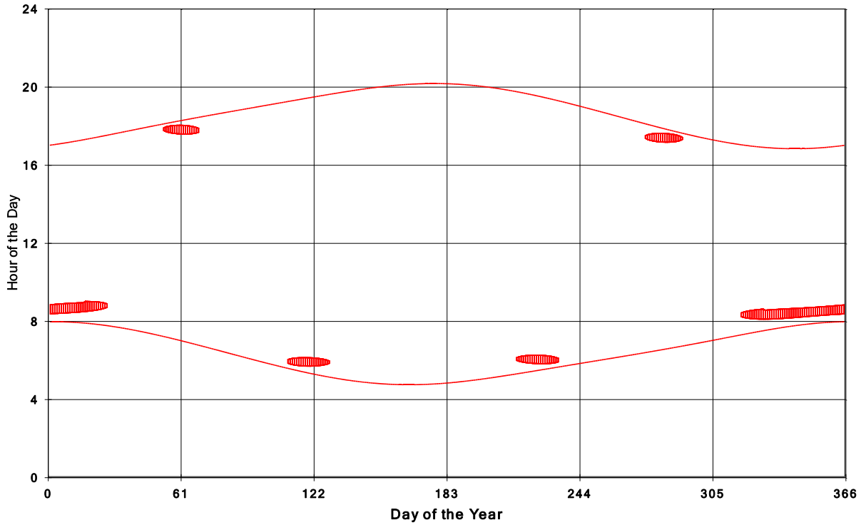
Goshen Wind Energy Centre Shadow Times on House 2136, All Windows from All Turbine
