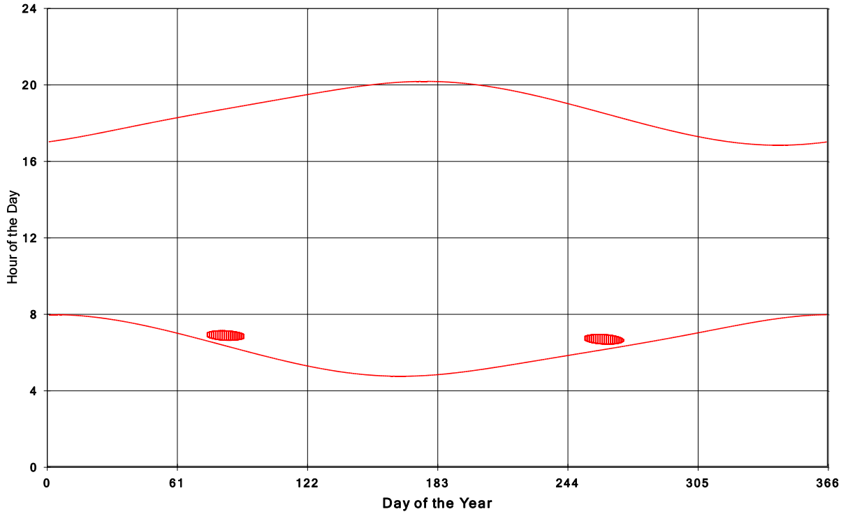
Goshen Wind Energy Centre Shadow Times on House 2159, All Windows from All Turbine
