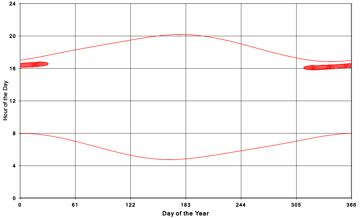
Goshen Wind Energy Centre Shadow Times on House 2204, All Windows from All Turbine
