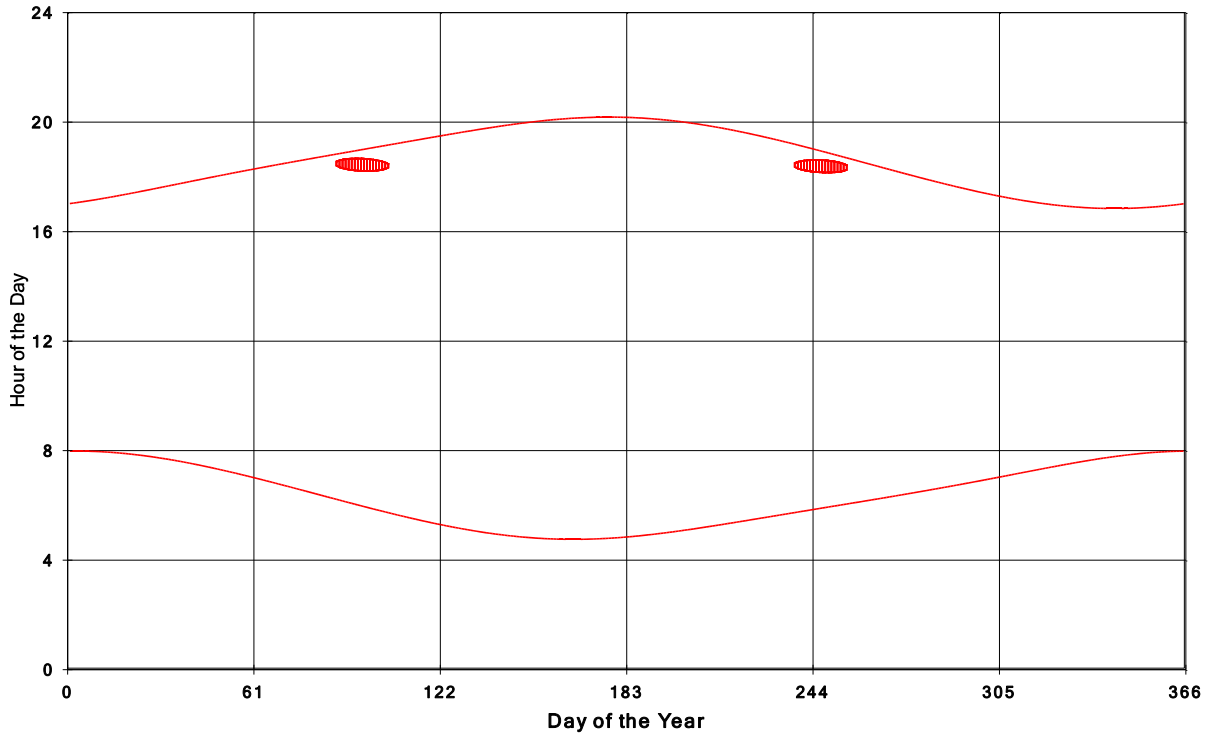
Goshen Wind Energy Centre Shadow Times on House 2170, All Windows from All Turbine
