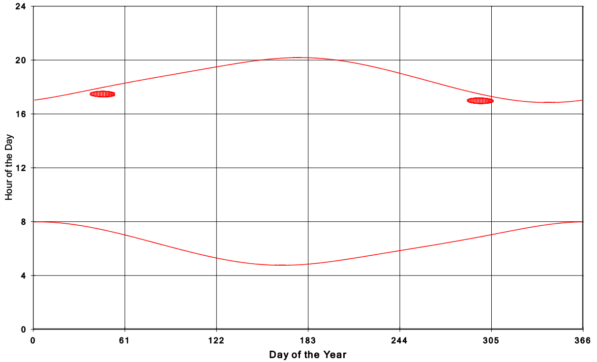
Goshen Wind Energy Centre Shadow Times on House 2206, All Windows from All Turbine
