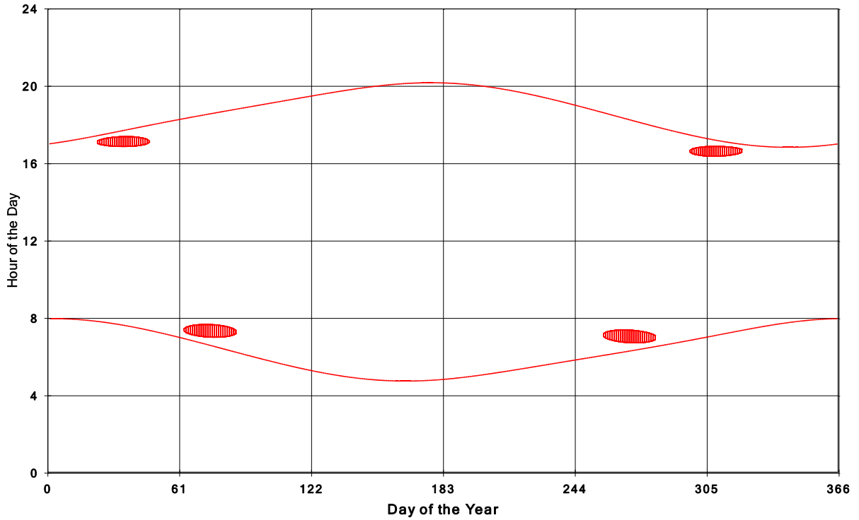
Goshen Wind Energy Centre Shadow Times on House 2192, All Windows from All Turbine
