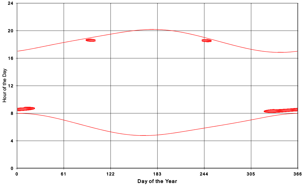
Goshen Wind Energy Centre Shadow Times on House 2057, All Windows from All Turbine
