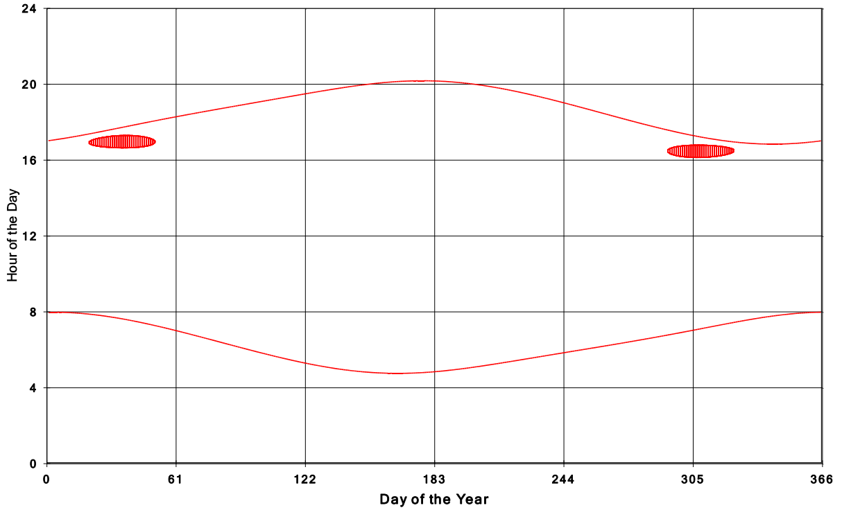
Goshen Wind Energy Centre Shadow Times on House 1904, All Windows from All Turbine
