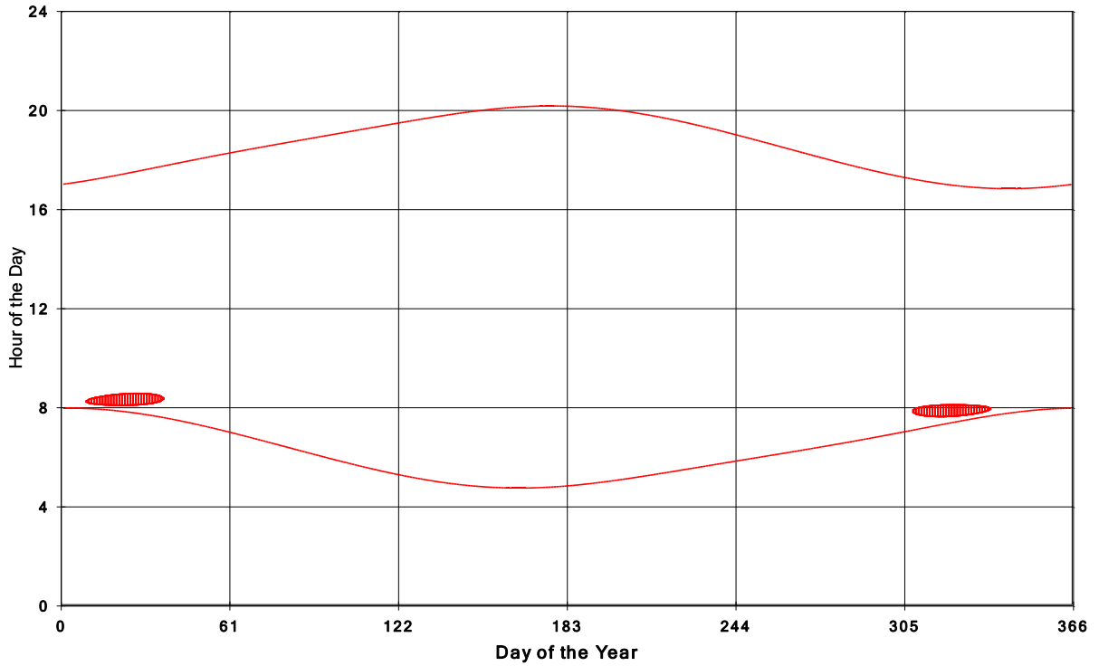
Goshen Wind Energy Centre Shadow Times on House 2044, All Windows from All Turbine
