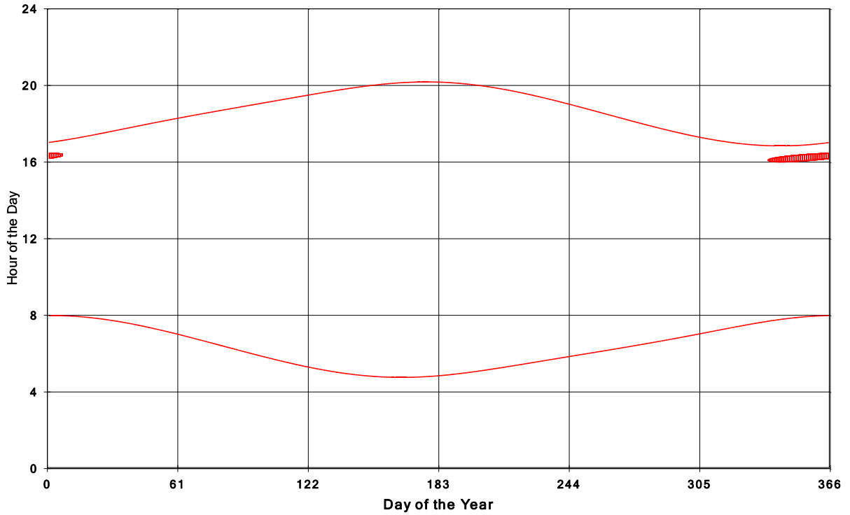
Goshen Wind Energy Centre Shadow Times on House 1902, All Windows from All Turbine
