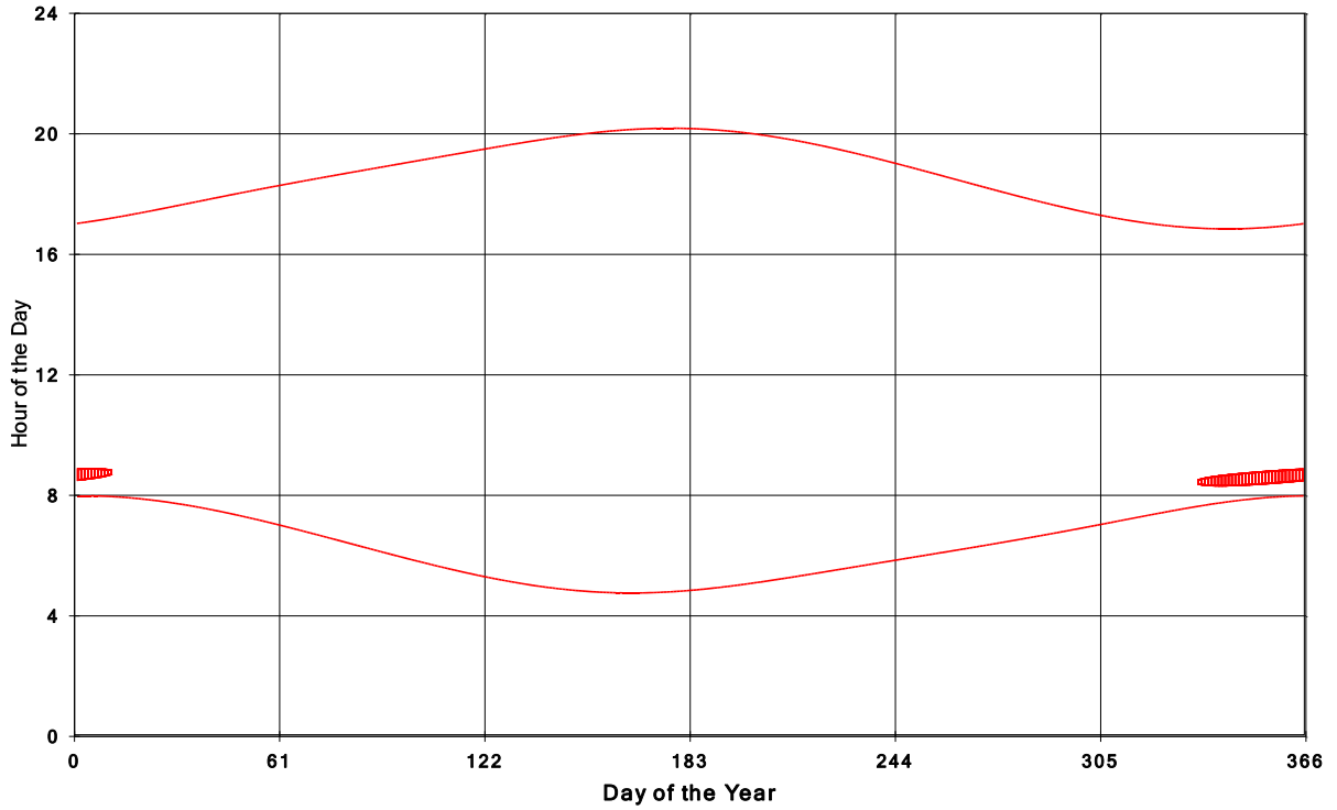
Goshen Wind Energy Centre Shadow Times on House 2016, All Windows from All Turbine
