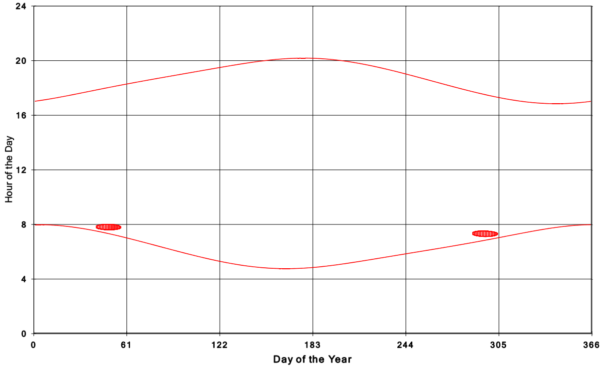
Goshen Wind Energy Centre Shadow Times on House 1974, All Windows from All Turbine
