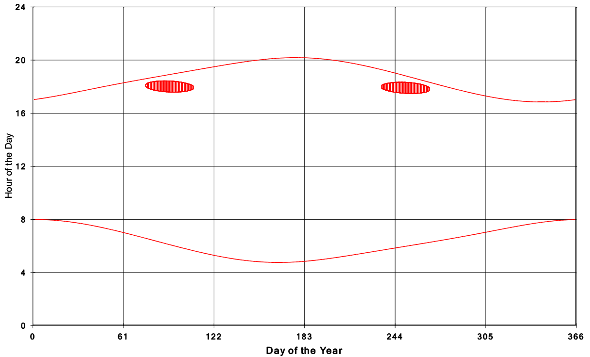
Goshen Wind Energy Centre Shadow Times on House 1990, All Windows from All Turbine
