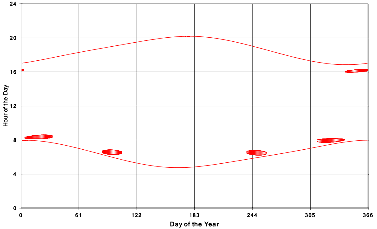
Goshen Wind Energy Centre Shadow Times on House 2008, All Windows from All Turbine
