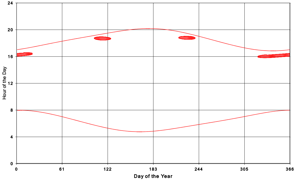
Goshen Wind Energy Centre Shadow Times on House 1978, All Windows from All Turbine
