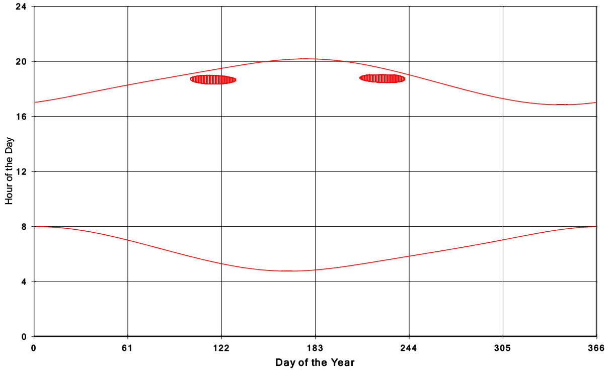
Goshen Wind Energy Centre Shadow Times on House 1983, All Windows from All Turbine
