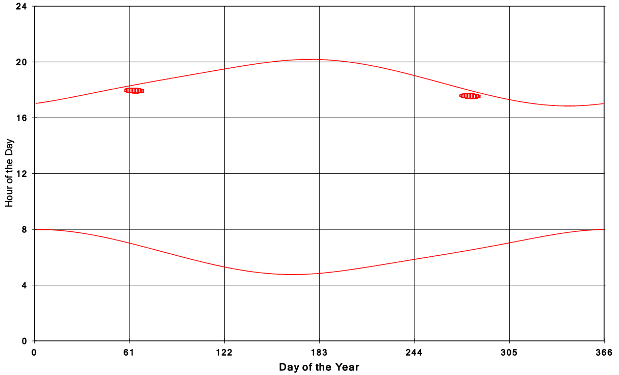
Goshen Wind Energy Centre Shadow Times on House 1948, All Windows from All Turbine
