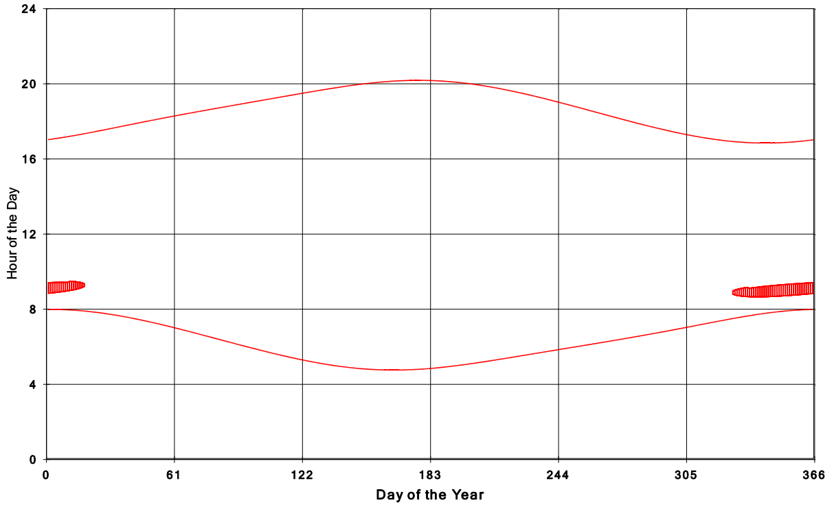
Goshen Wind Energy Centre Shadow Times on House 1985, All Windows from All Turbine
