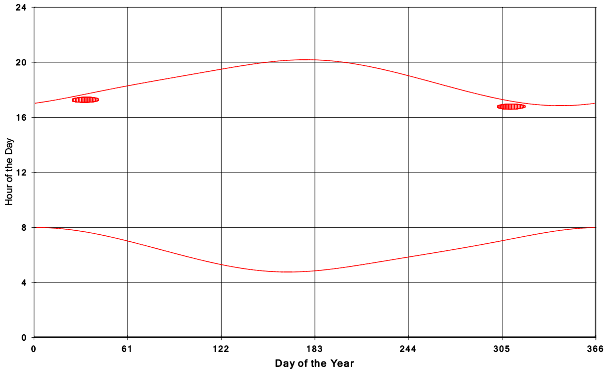
Goshen Wind Energy Centre Shadow Times on House 2052, All Windows from All Turbine
