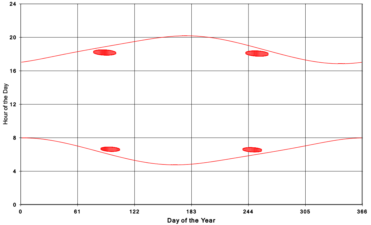
Goshen Wind Energy Centre Shadow Times on House 2001, All Windows from All Turbine
