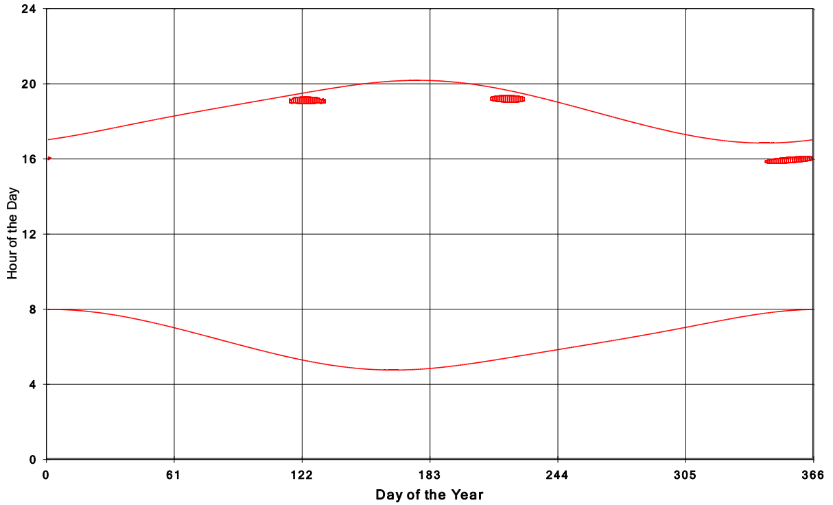
Goshen Wind Energy Centre Shadow Times on House 2063, All Windows from All Turbine
