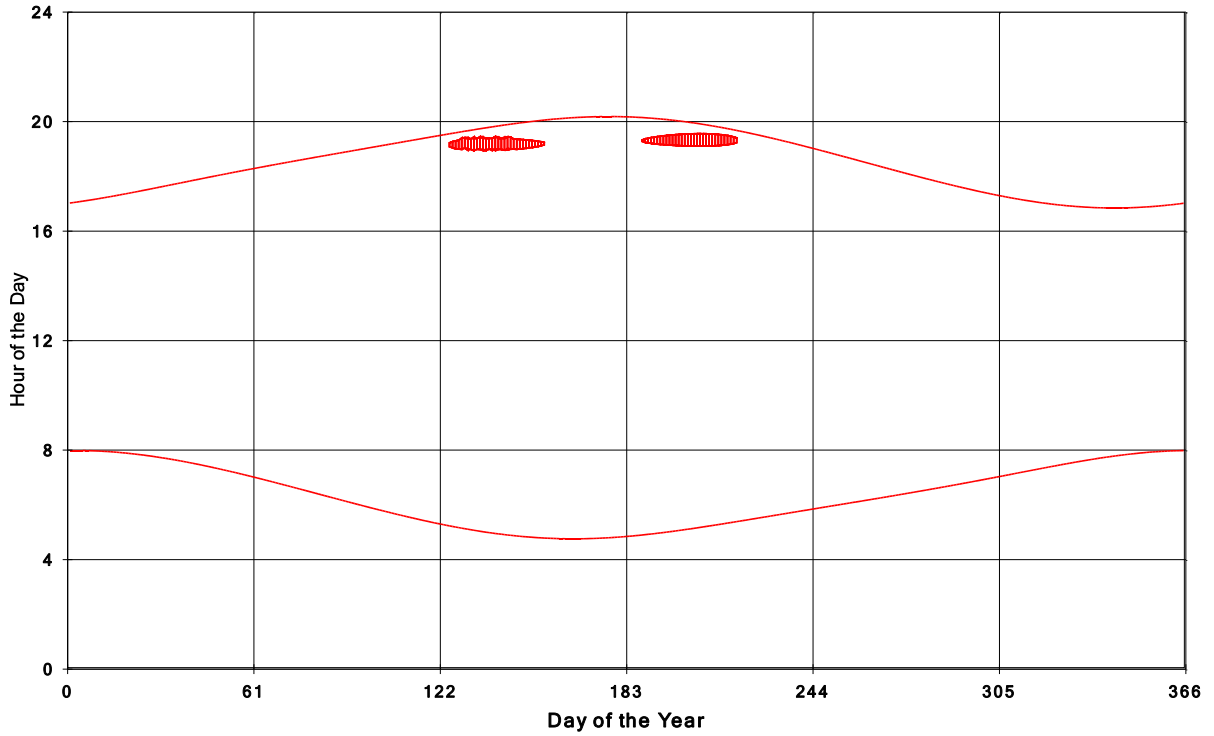
Goshen Wind Energy Centre Shadow Times on House 1891, All Windows from All Turbine
