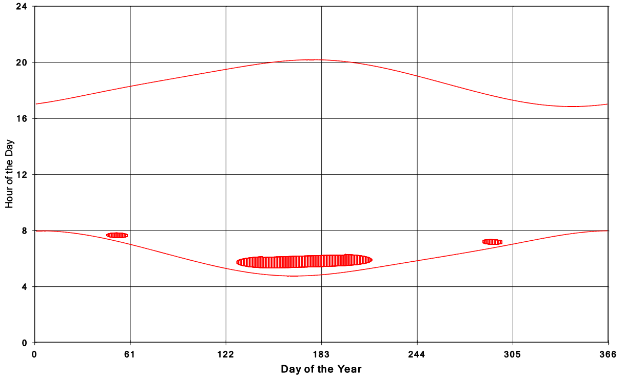
Goshen Wind Energy Centre Shadow Times on House 1884, All Windows from All Turbine
