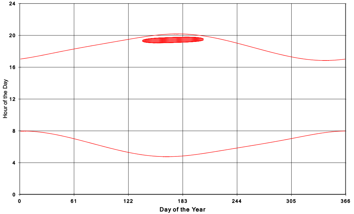
Goshen Wind Energy Centre Shadow Times on House 2002, All Windows from All Turbine
