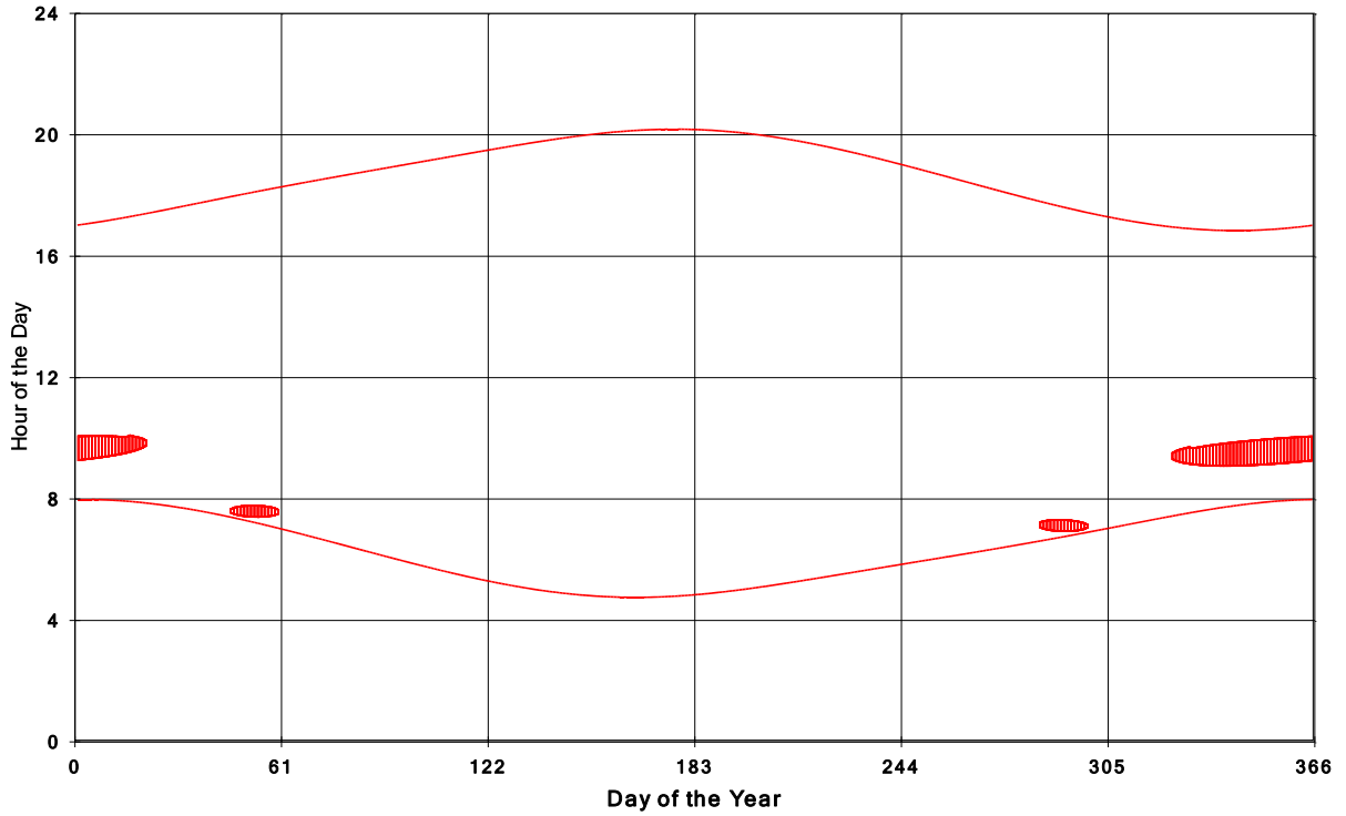
Goshen Wind Energy Centre Shadow Times on House 1875, All Windows from All Turbine
