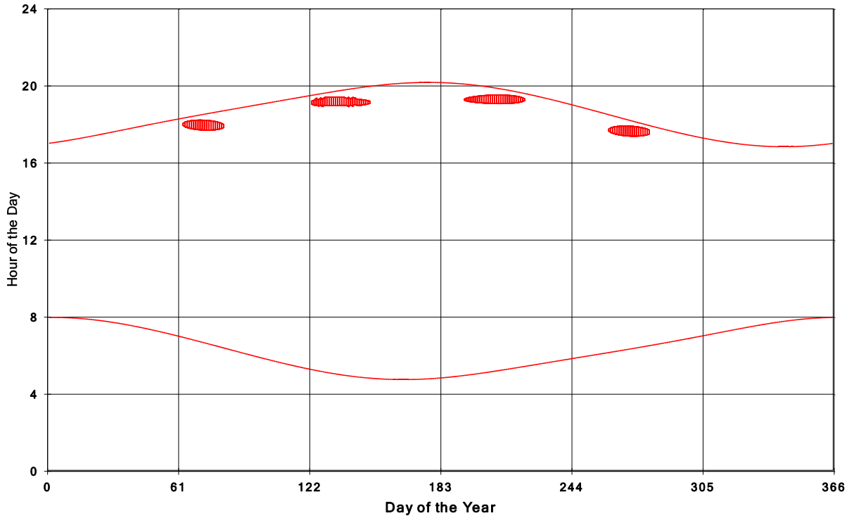
Goshen Wind Energy Centre Shadow Times on House 1913, All Windows from All Turbine
