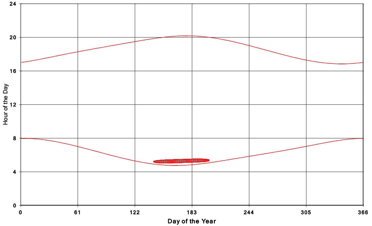
Goshen Wind Energy Centre Shadow Times on House 1969, All Windows from All Turbine
