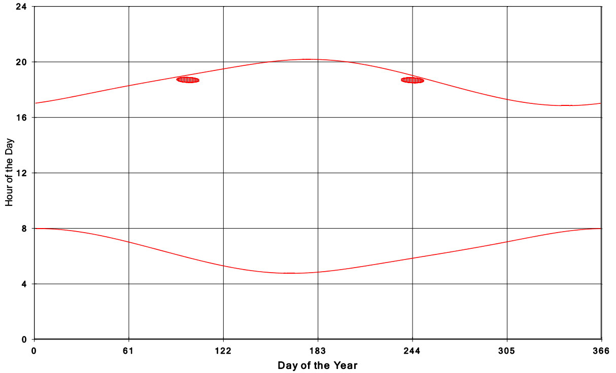
Goshen Wind Energy Centre Shadow Times on House 2054, All Windows from All Turbine
