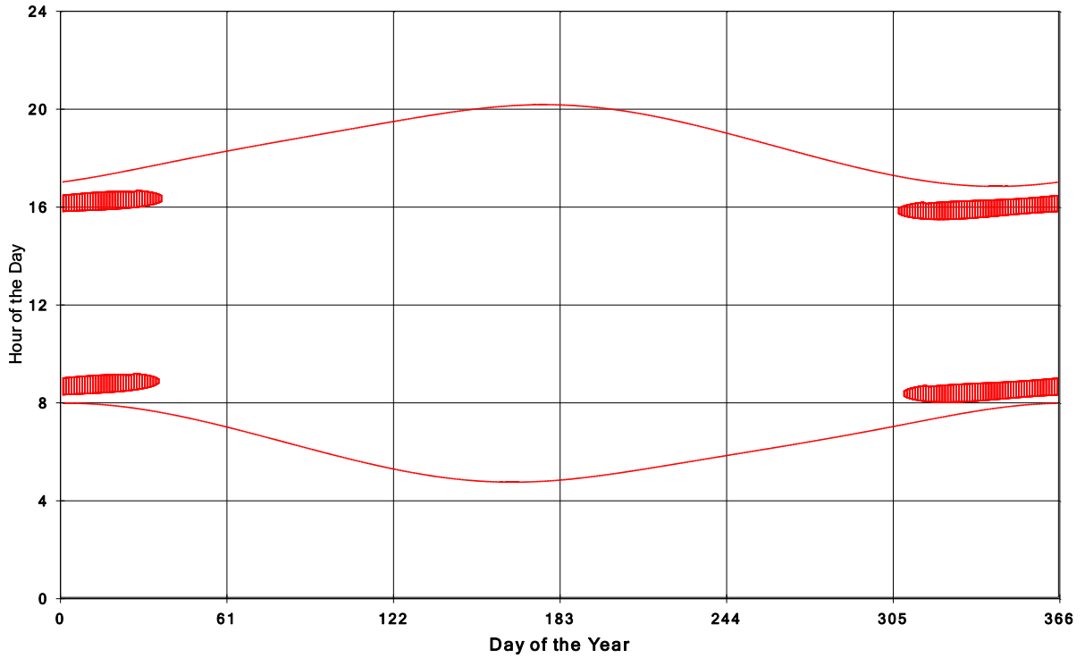
Goshen Wind Energy Centre Shadow Times on House 1879, All Windows from All Turbine
