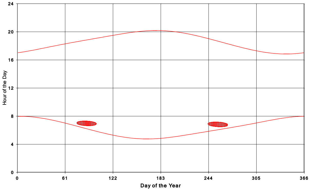
Goshen Wind Energy Centre Shadow Times on House 1910, All Windows from All Turbine
