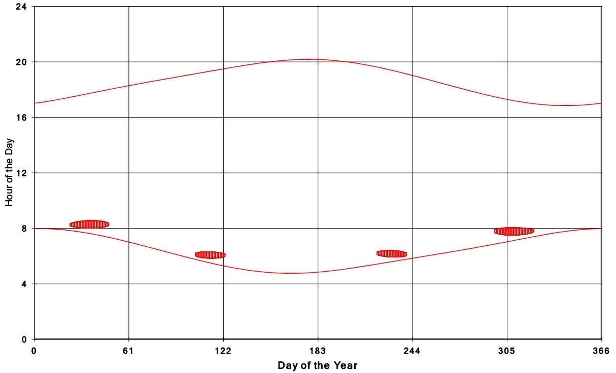
Goshen Wind Energy Centre Shadow Times on House 2075, All Windows from All Turbine
