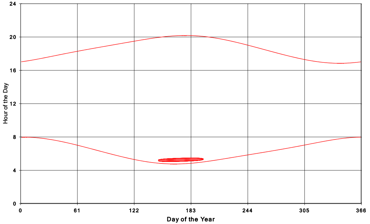
Goshen Wind Energy Centre Shadow Times on House 1994, All Windows from All Turbine
