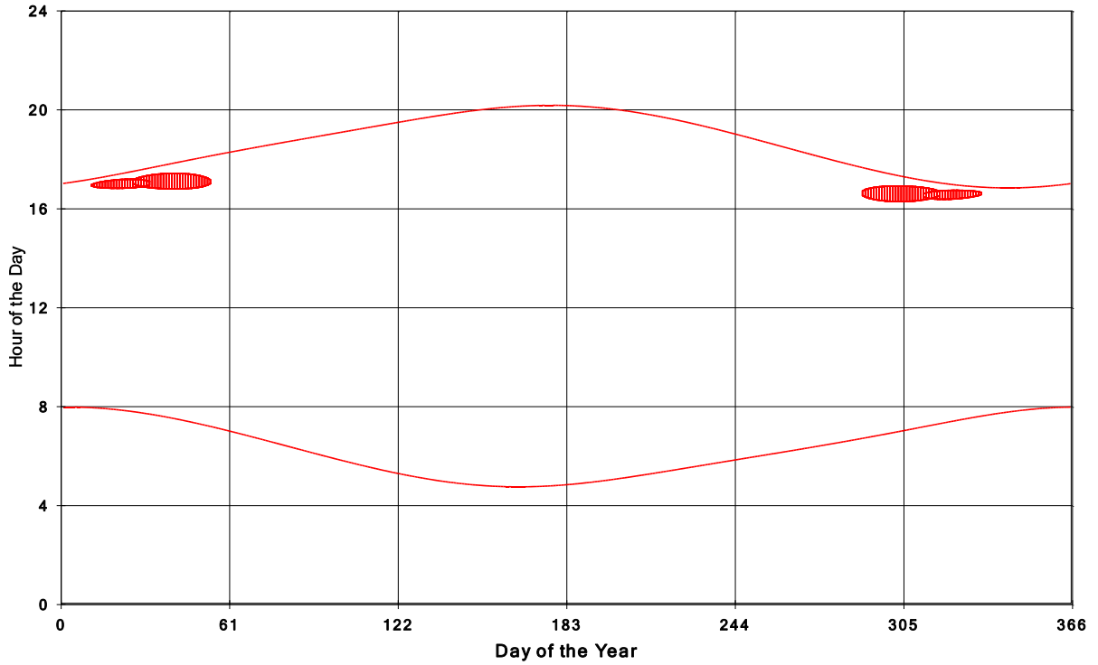
Goshen Wind Energy Centre Shadow Times on House 1893, All Windows from All Turbine
