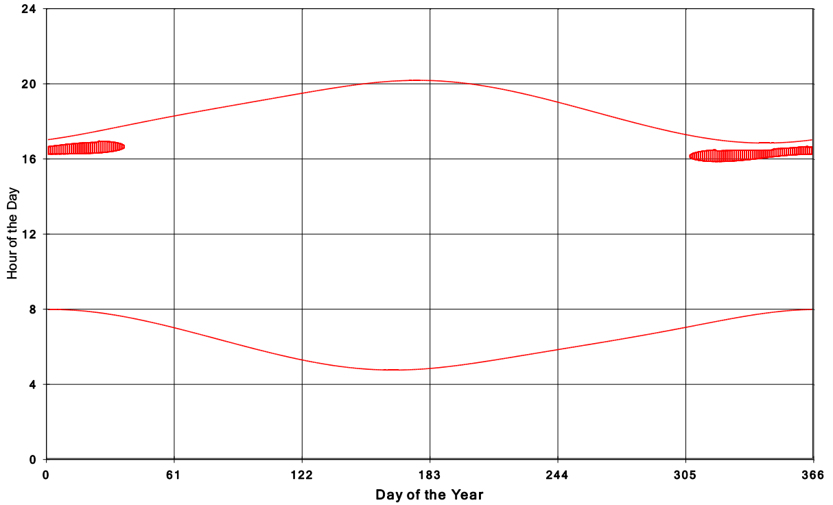
Goshen Wind Energy Centre Shadow Times on House 1894, All Windows from All Turbine
