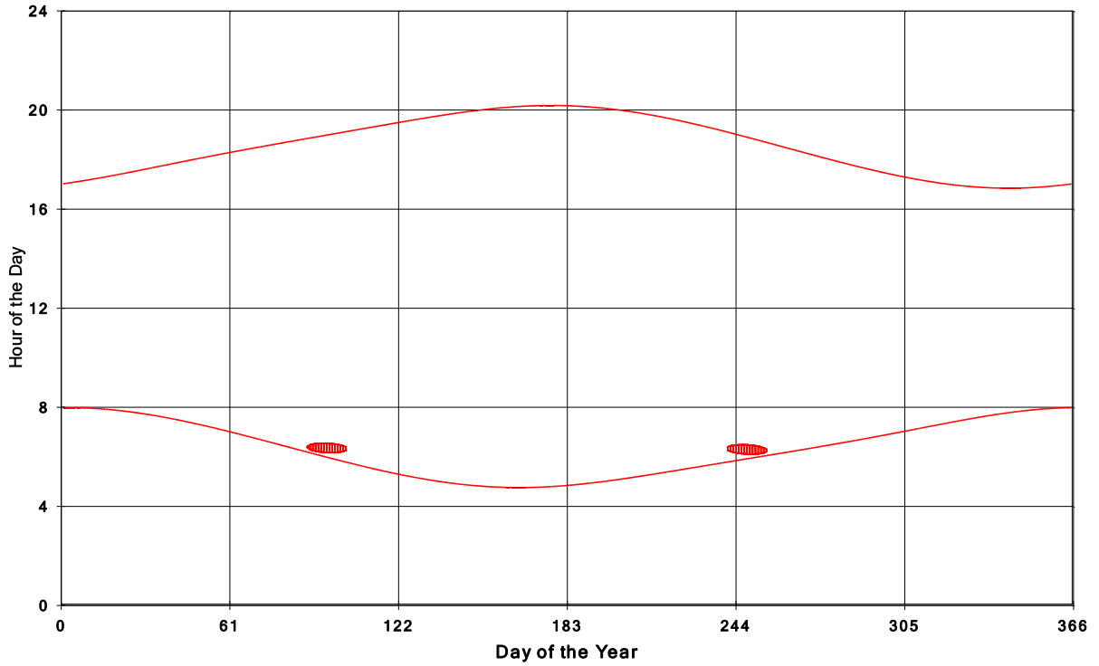
Goshen Wind Energy Centre Shadow Times on House 1981, All Windows from All Turbine
