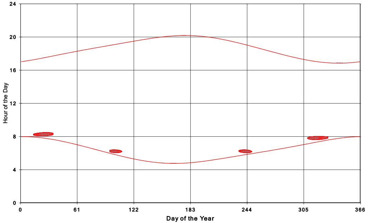
Goshen Wind Energy Centre Shadow Times on House 1975, All Windows from All Turbine
