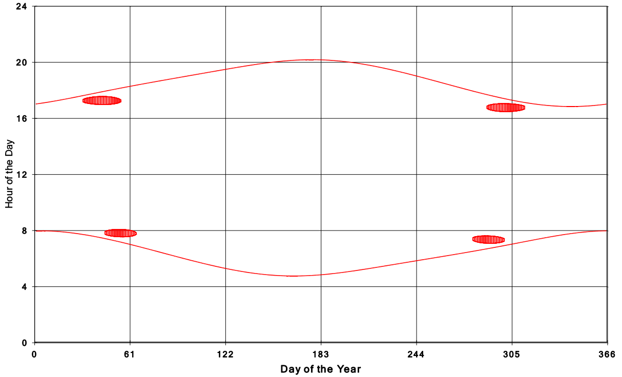
Goshen Wind Energy Centre Shadow Times on House 2058, All Windows from All Turbine
