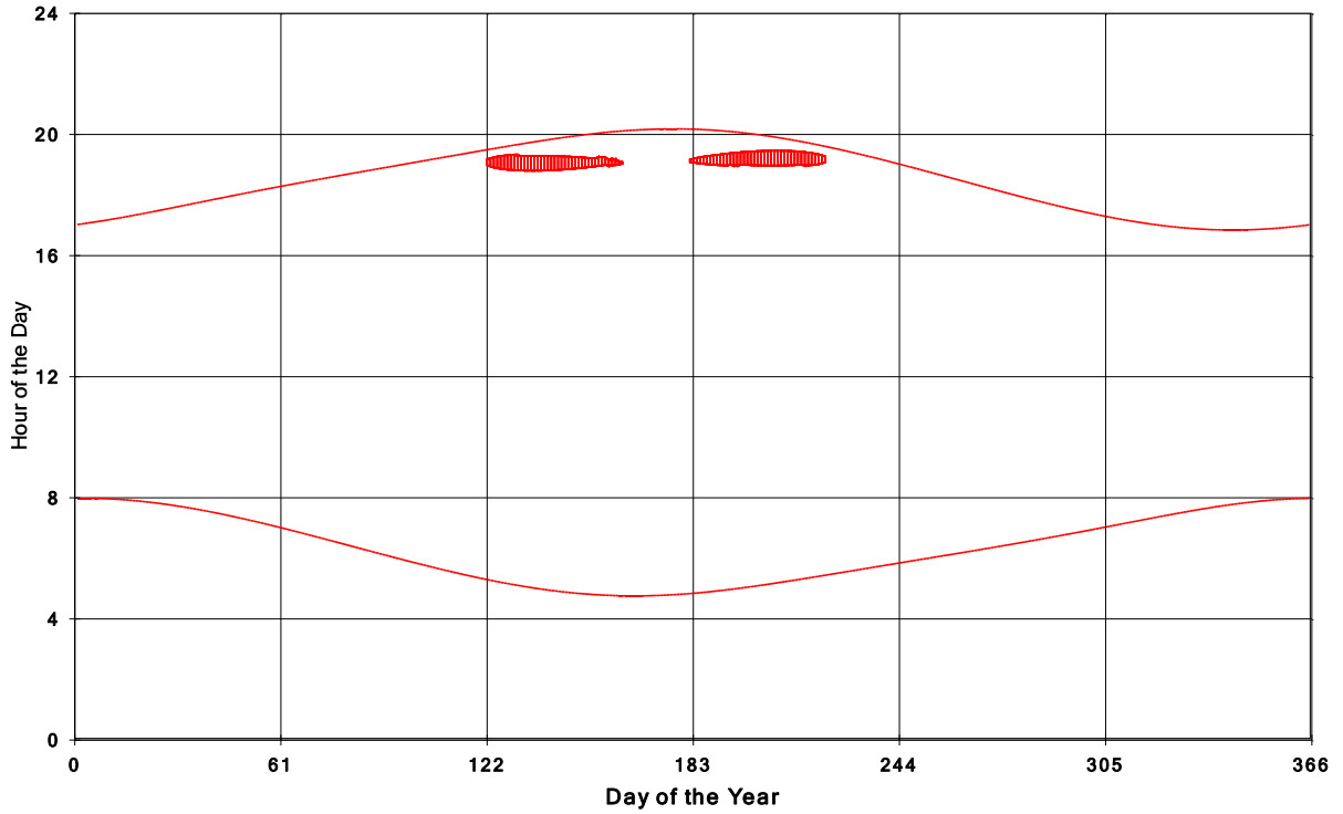
Goshen Wind Energy Centre Shadow Times on House 1897, All Windows from All Turbine
