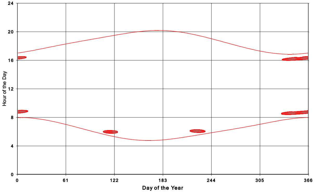
Jericho Wind Energy Centre Shadow Times on House 1909, All Windows from All Turbine
