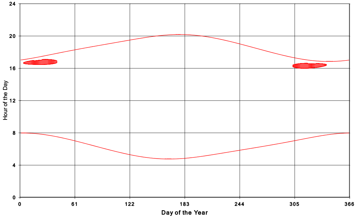
Goshen Wind Energy Centre Shadow Times on House 1892, All Windows from All Turbine
