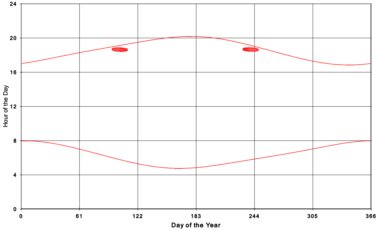
Goshen Wind Energy Centre Shadow Times on House 1986, All Windows from All Turbine
