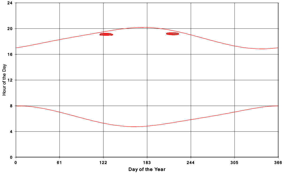
Goshen Wind Energy Centre Shadow Times on House 1901, All Windows from All Turbine
