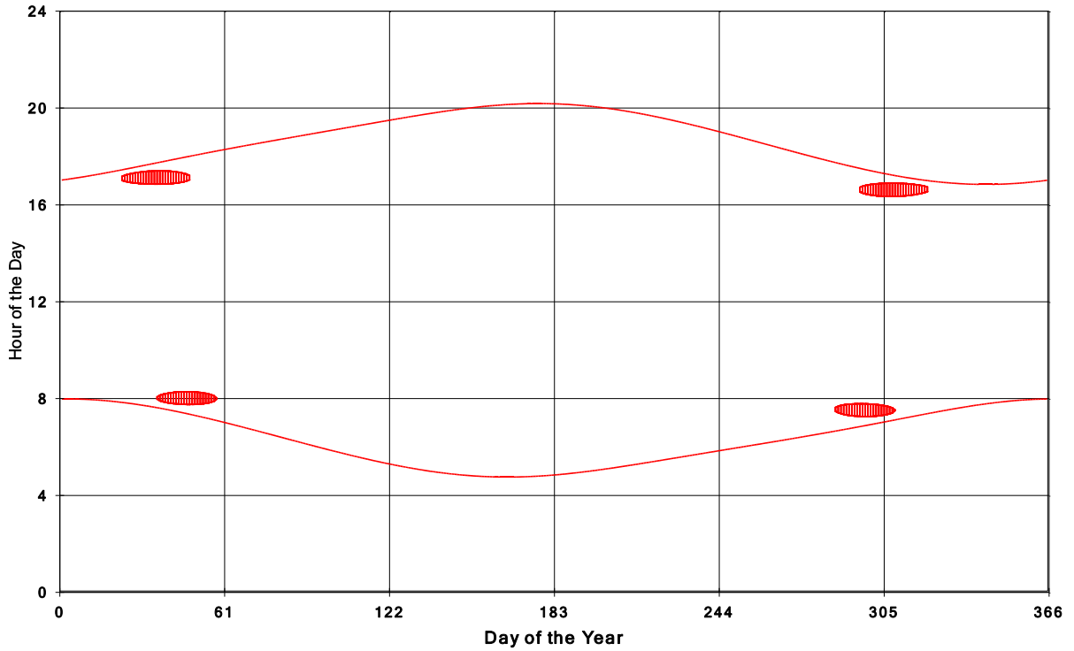
Goshen Wind Energy Centre Shadow Times on House 2059, All Windows from All Turbine
