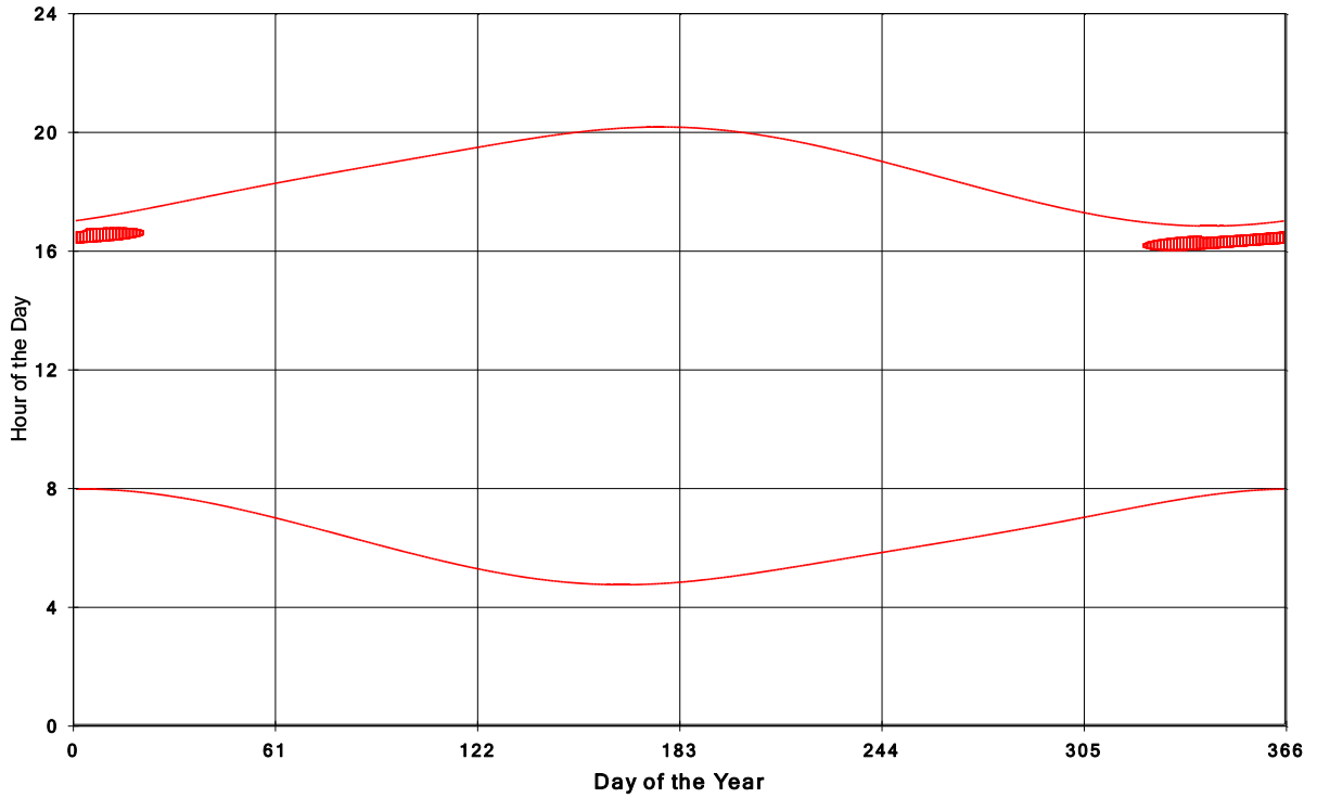
Goshen Wind Energy Centre Shadow Times on House 1898, All Windows from All Turbine
