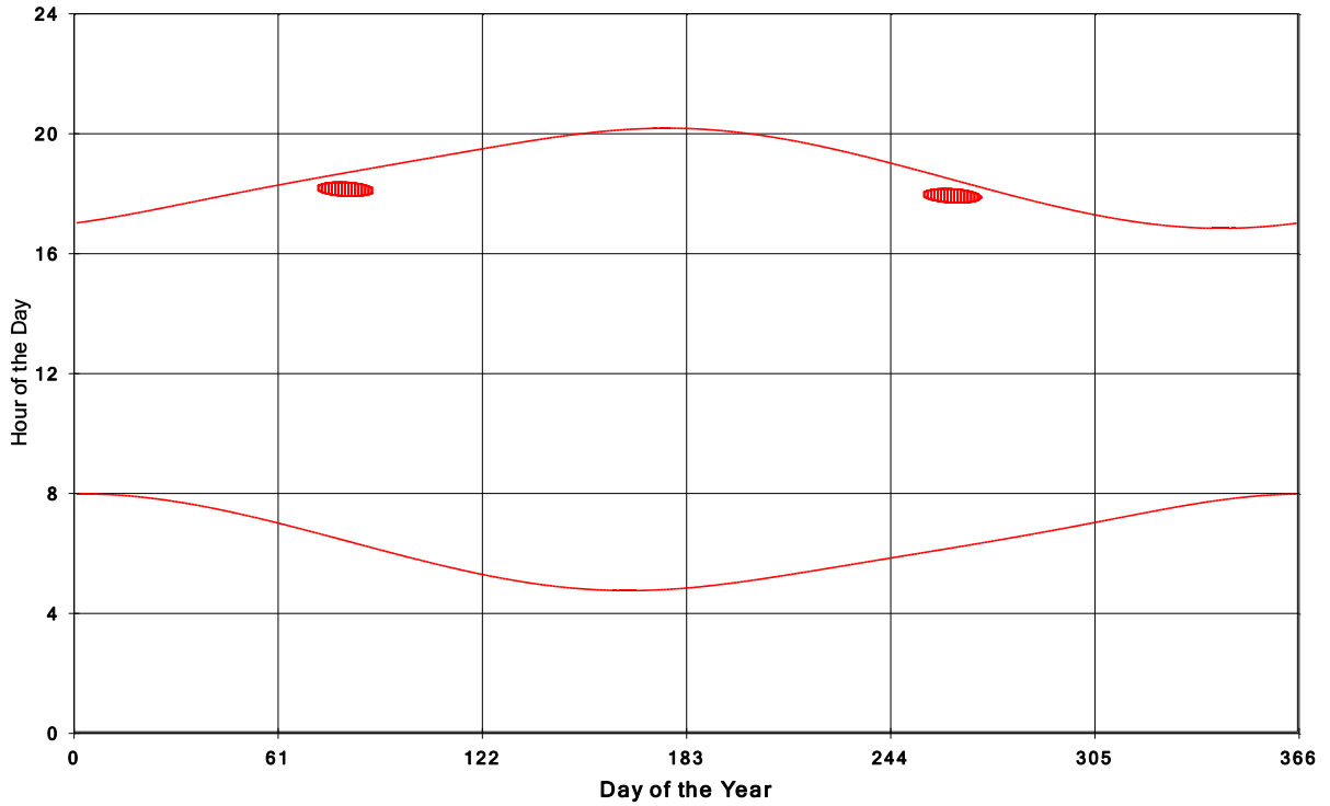
Goshen Wind Energy Centre Shadow Times on House 1979, All Windows from All Turbine
