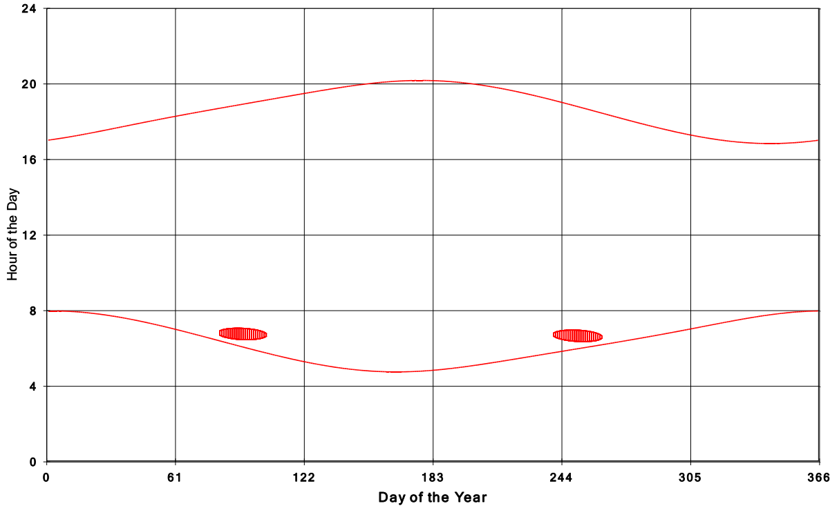
Goshen Wind Energy Centre Shadow Times on House 2072, All Windows from All Turbine
