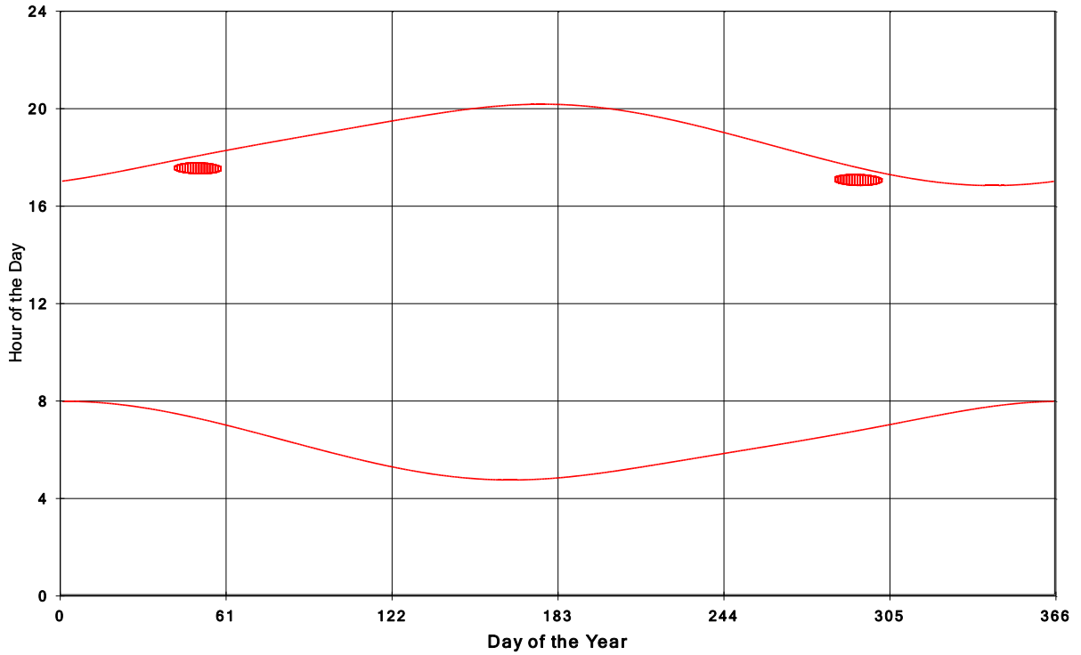
Goshen Wind Energy Centre Shadow Times on House 1947, All Windows from All Turbine
