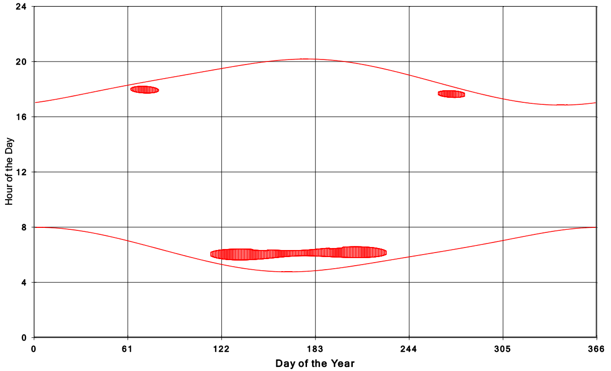
Goshen Wind Energy Centre Shadow Times on House 1886, All Windows from All Turbine
