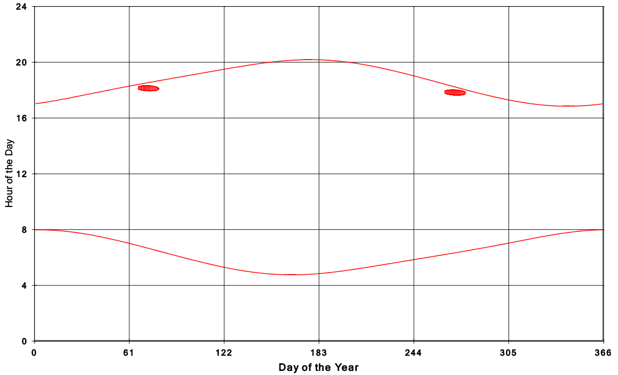
Goshen Wind Energy Centre Shadow Times on House 2061, All Windows from All Turbine
