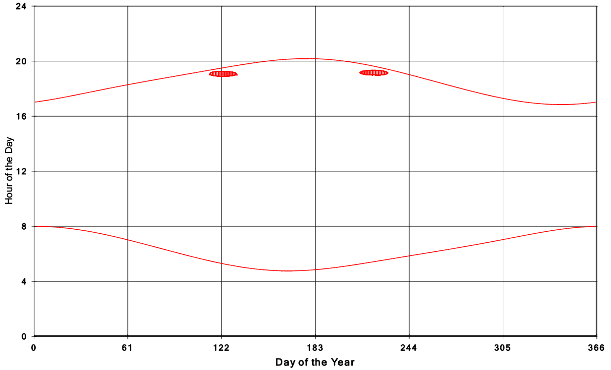
Goshen Wind Energy Centre Shadow Times on House 2062, All Windows from All Turbine
