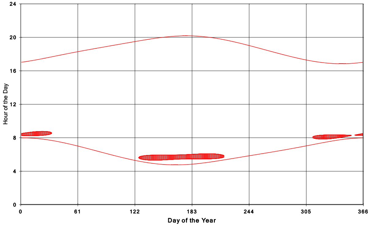
Goshen Wind Energy Centre Shadow Times on House 1905, All Windows from All Turbine
