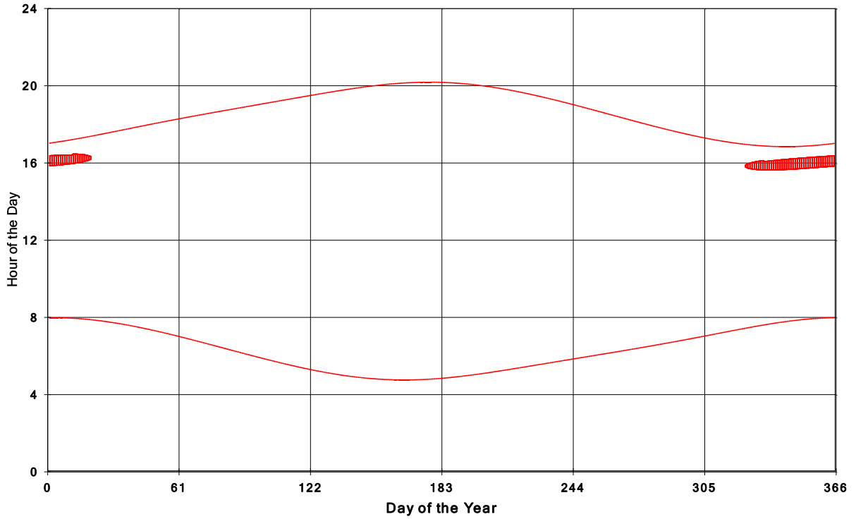
Goshen Wind Energy Centre Shadow Times on House 1984, All Windows from All Turbine
