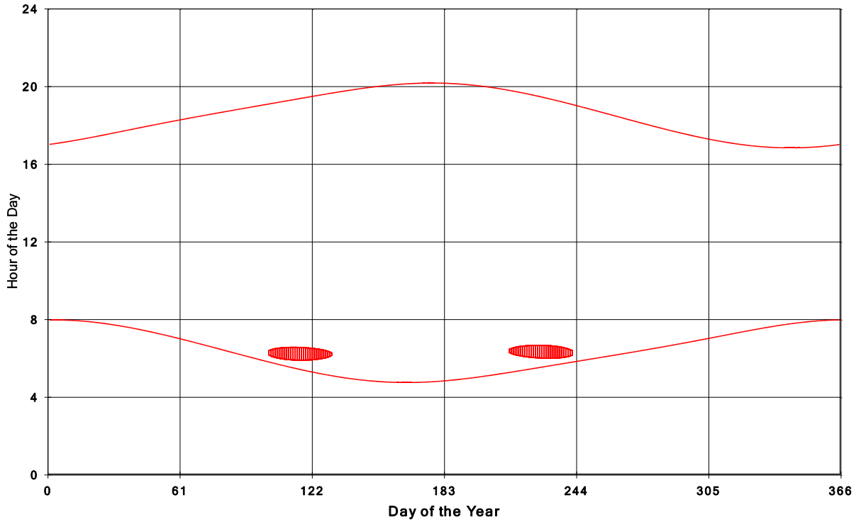
Goshen Wind Energy Centre Shadow Times on House 2005, All Windows from All Turbine
