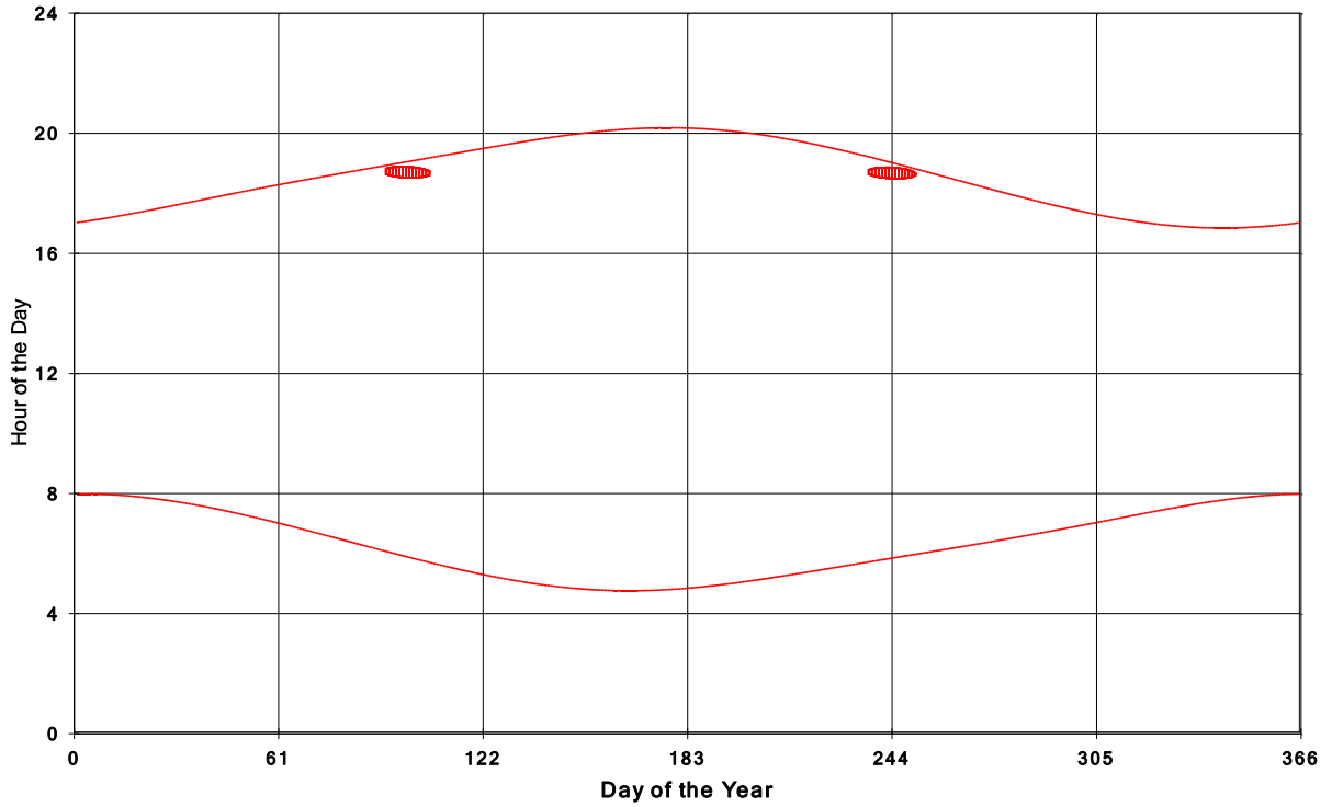
Goshen Wind Energy Centre Shadow Times on House 1906, All Windows from All Turbine
