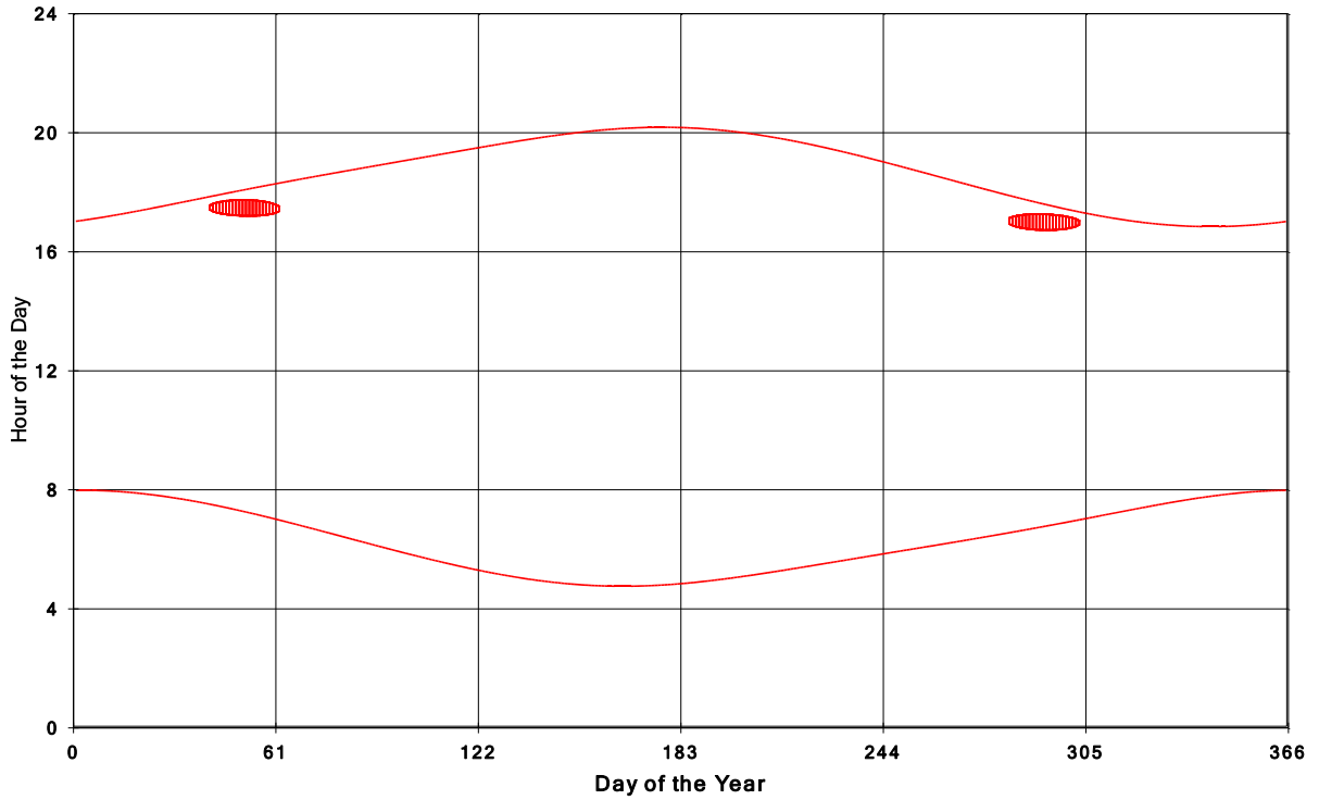
Goshen Wind Energy Centre Shadow Times on House 1959, All Windows from All Turbine
