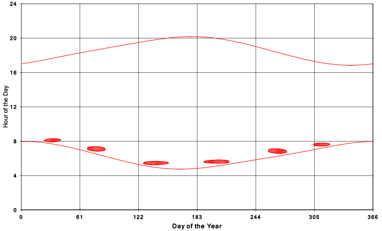
Goshen Wind Energy Centre Shadow Times on House 2012, All Windows from All Turbine
