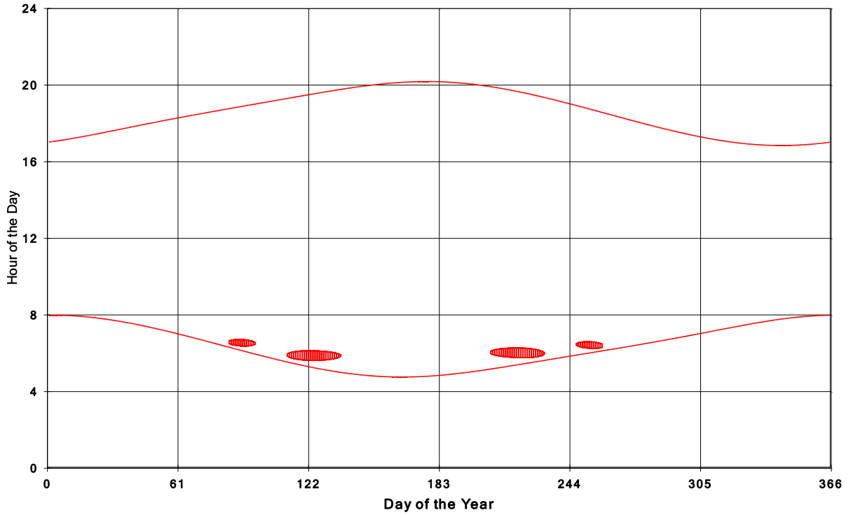
Goshen Wind Energy Centre Shadow Times on House 2000, All Windows from All Turbine
