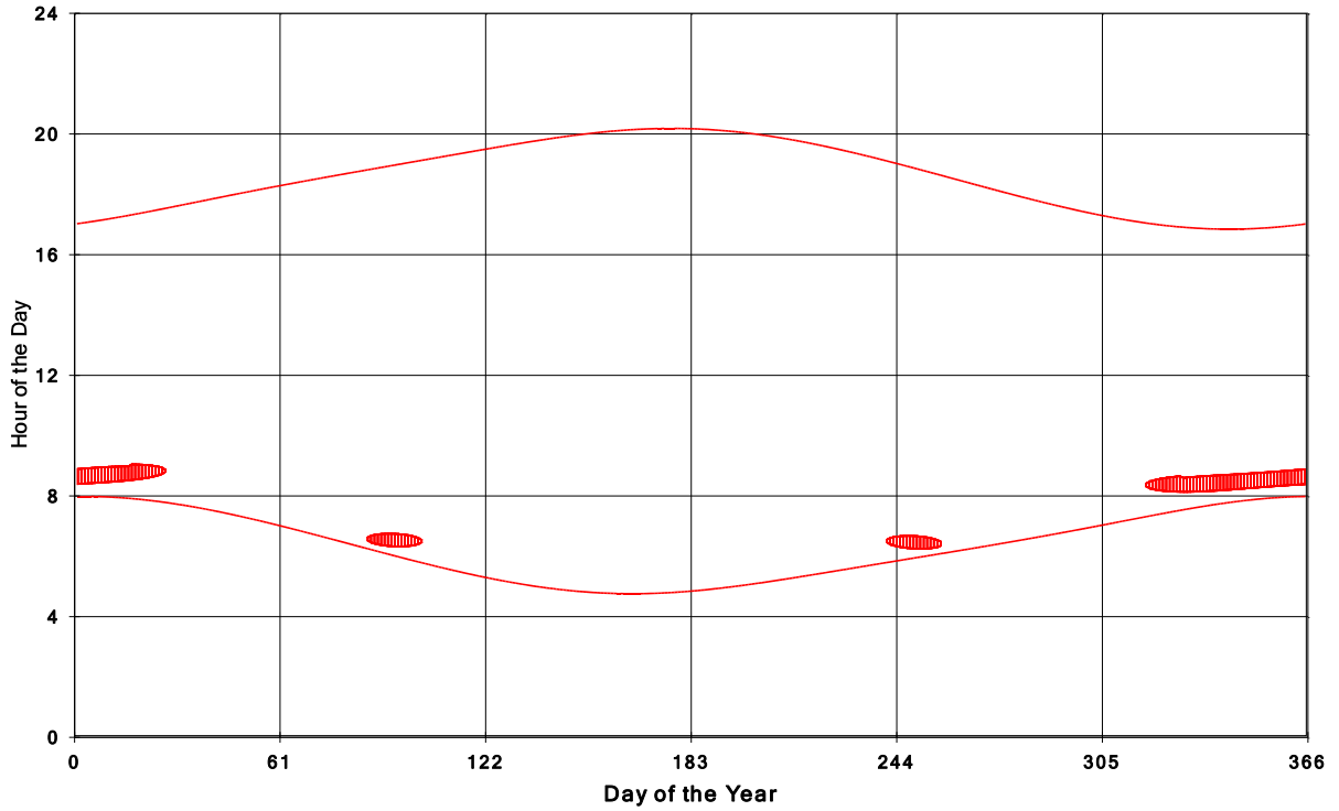
Goshen Wind Energy Centre Shadow Times on House 1912, All Windows from All Turbine
