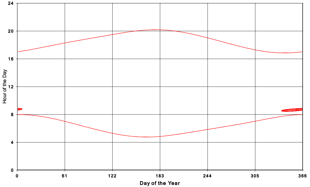
Goshen Wind Energy Centre Shadow Times on House 2017, All Windows from All Turbine
