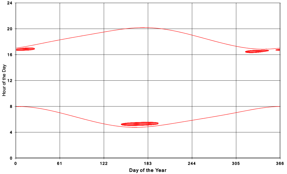
Jericho Wind Energy Centre Shadow Times on House 2045, All Windows from All Turbine
