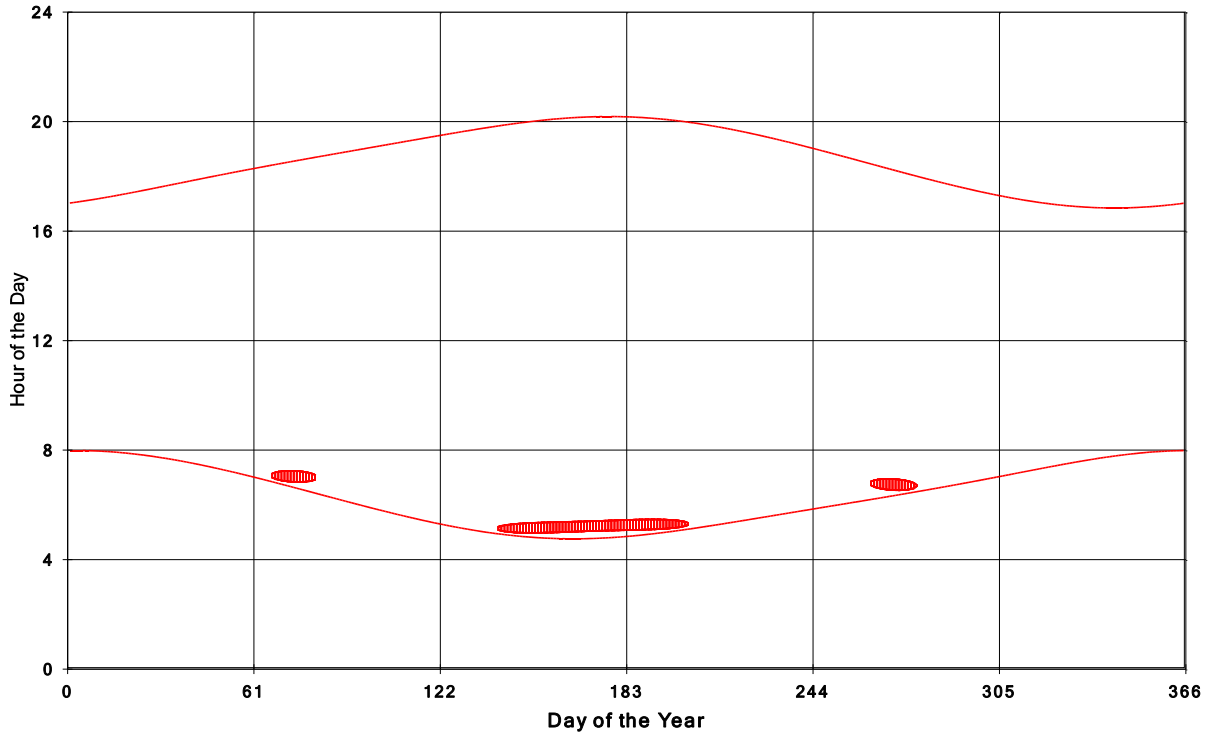
Goshen Wind Energy Centre Shadow Times on House 1880, All Windows from All Turbine
