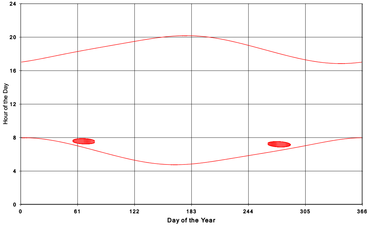
Goshen Wind Energy Centre Shadow Times on House 2027, All Windows from All Turbine
