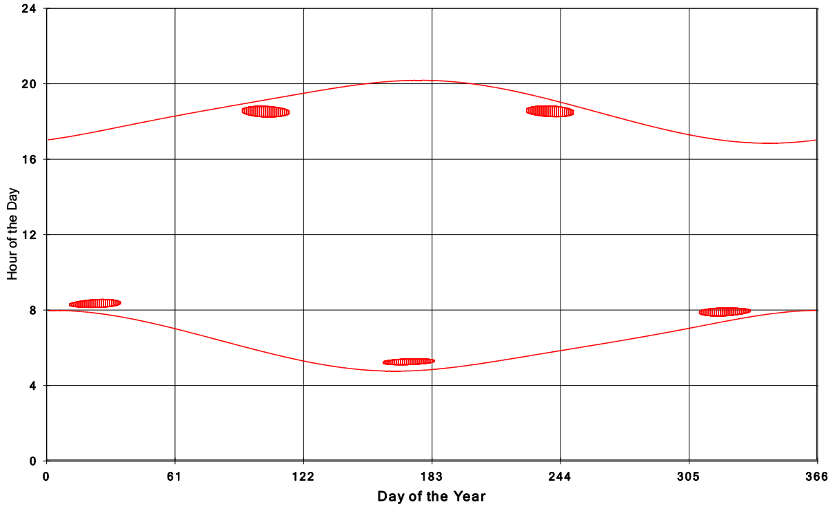
Goshen Wind Energy Centre Shadow Times on House 1887, All Windows from All Turbine
