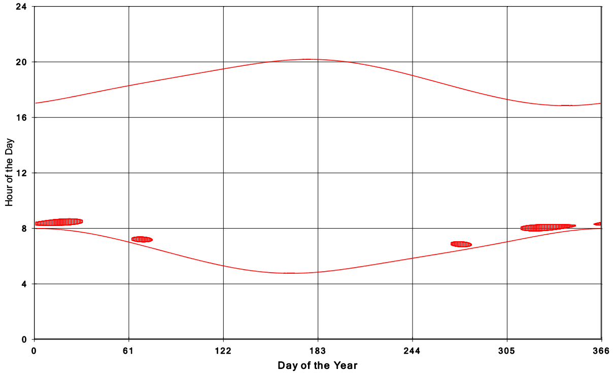
Goshen Wind Energy Centre Shadow Times on House 1908, All Windows from All Turbine
