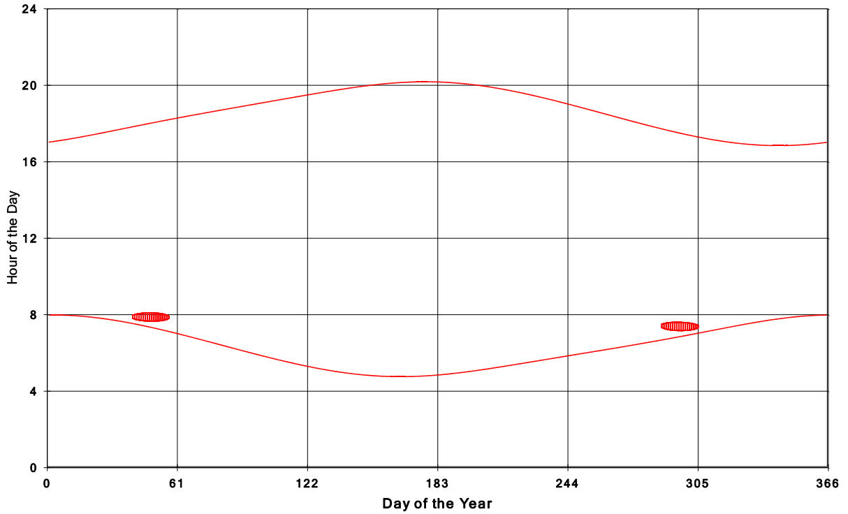
Goshen Wind Energy Centre Shadow Times on House 1996, All Windows from All Turbine
