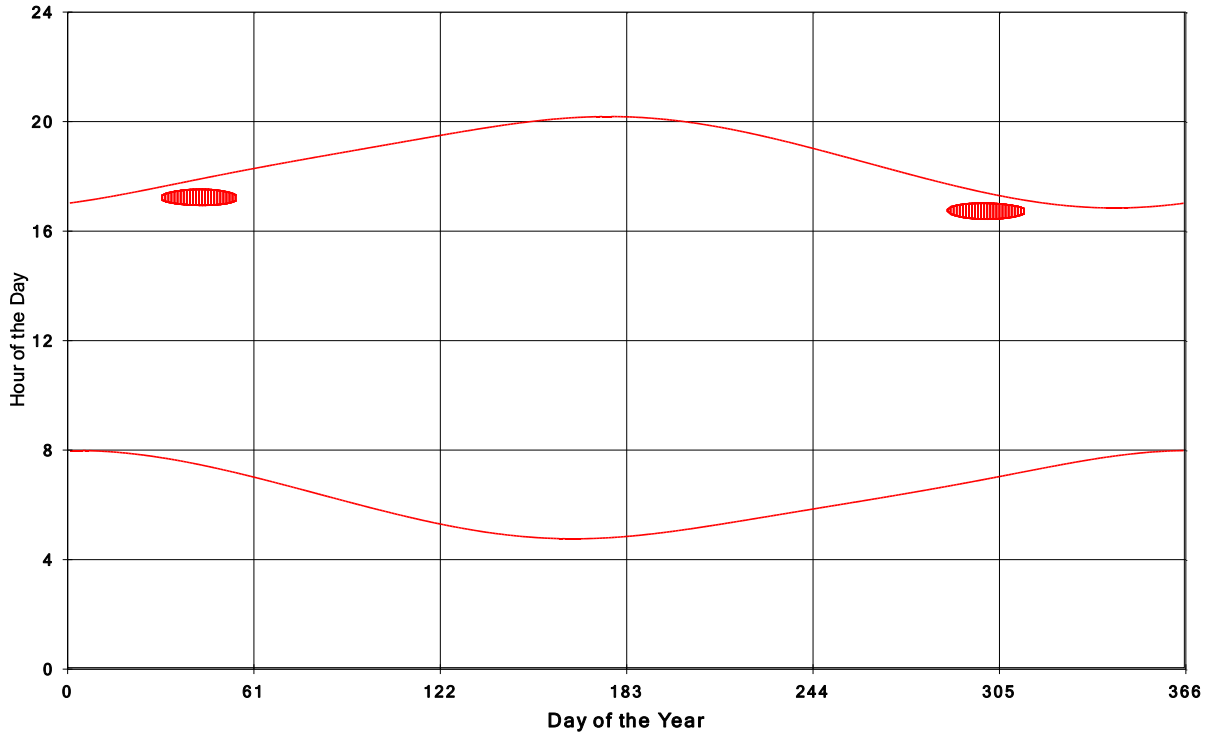
Goshen Wind Energy Centre Shadow Times on House 1946, All Windows from All Turbine
