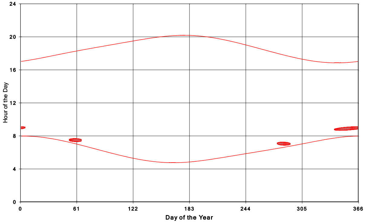
Goshen Wind Energy Centre Shadow Times on House 2015, All Windows from All Turbine
