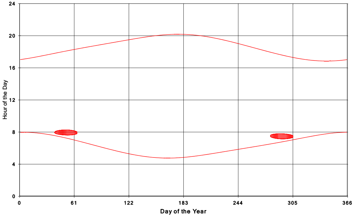
Jericho Wind Energy Centre Shadow Times on House 1988, All Windows from All Turbine
