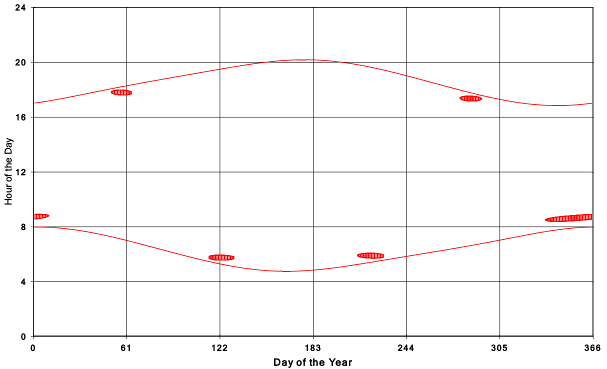
Jericho Wind Energy Centre Shadow Times on House 1883, All Windows from All Turbine
