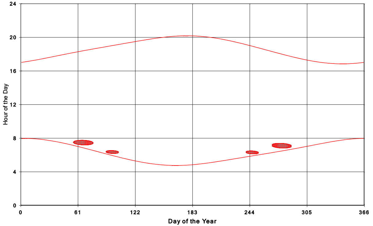
Goshen Wind Energy Centre Shadow Times on House 2014, All Windows from All Turbine
