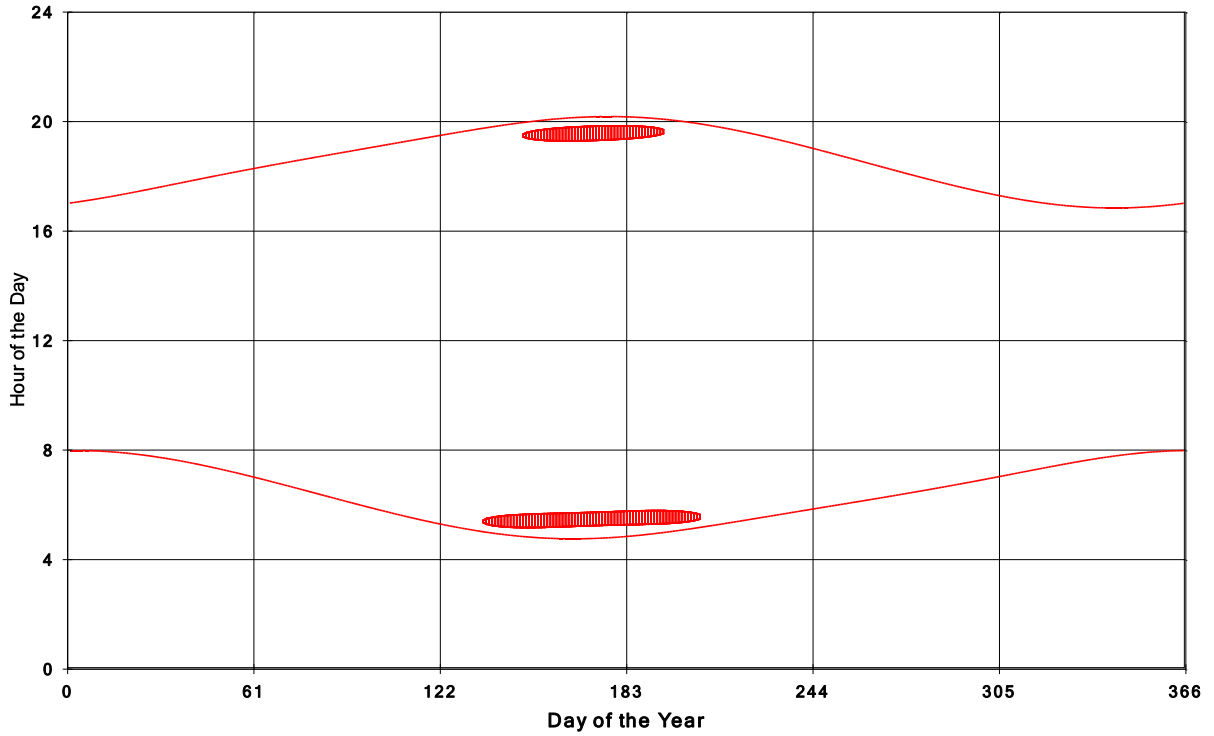
Goshen Wind Energy Centre Shadow Times on House 2060, All Windows from All Turbine
