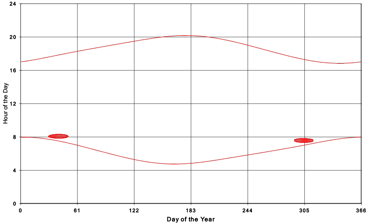
Goshen Wind Energy Centre Shadow Times on House 1967, All Windows from All Turbine
