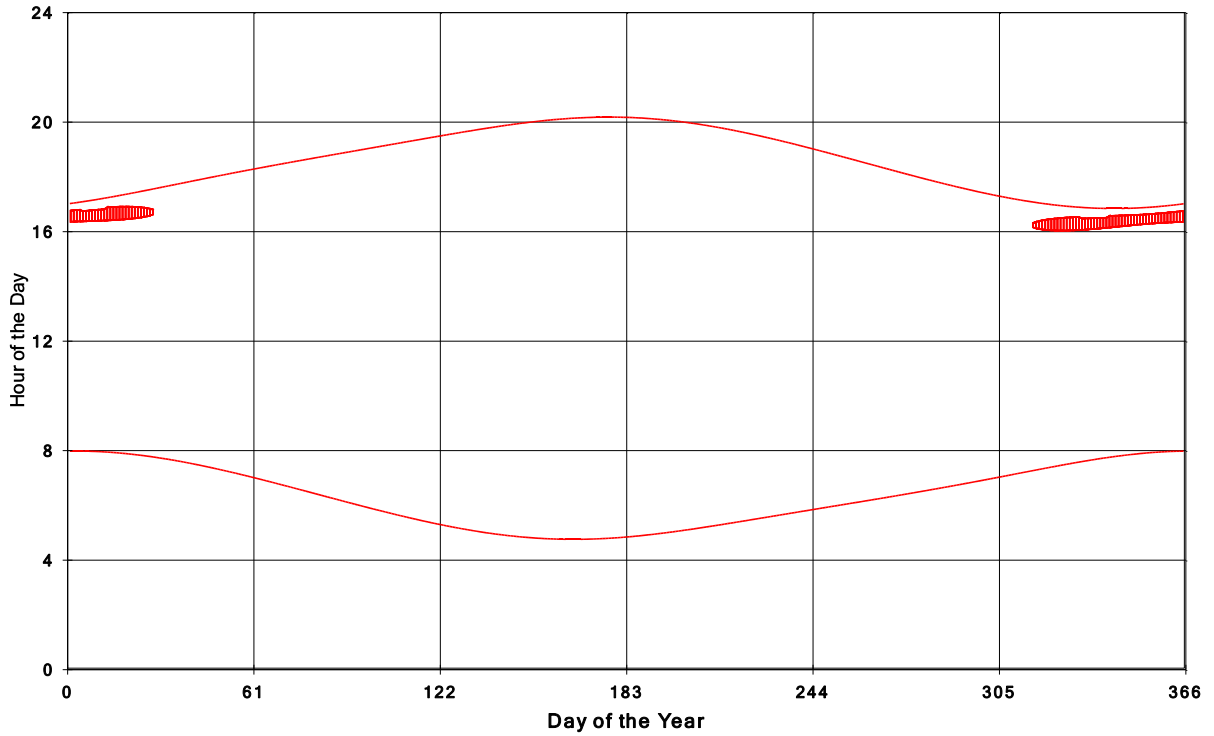
Goshen Wind Energy Centre Shadow Times on House 2009, All Windows from All Turbine
