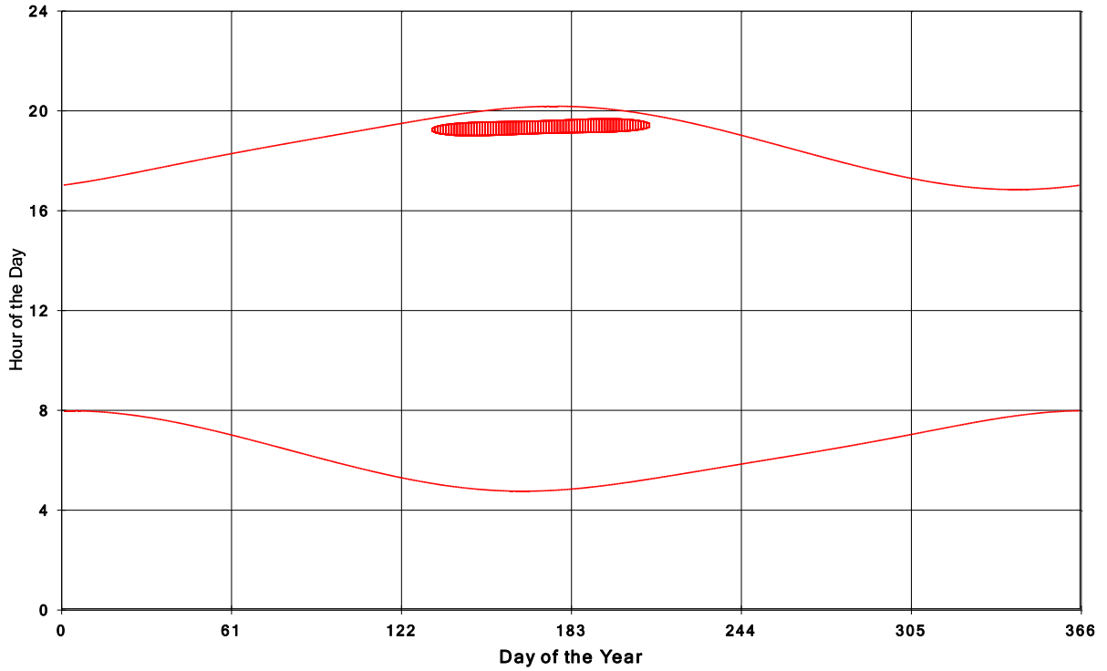
Goshen Wind Energy Centre Shadow Times on House 1895, All Windows from All Turbine
