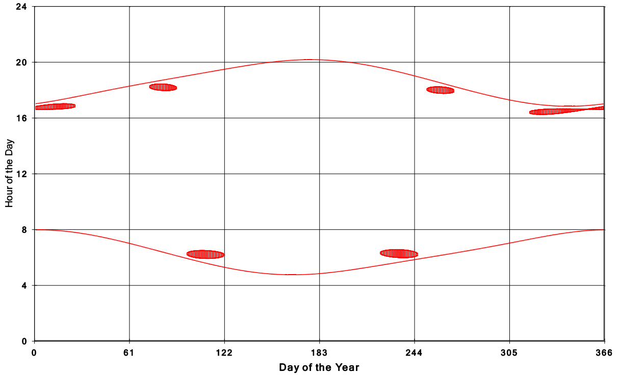
Goshen Wind Energy Centre Shadow Times on House 1987, All Windows from All Turbine
