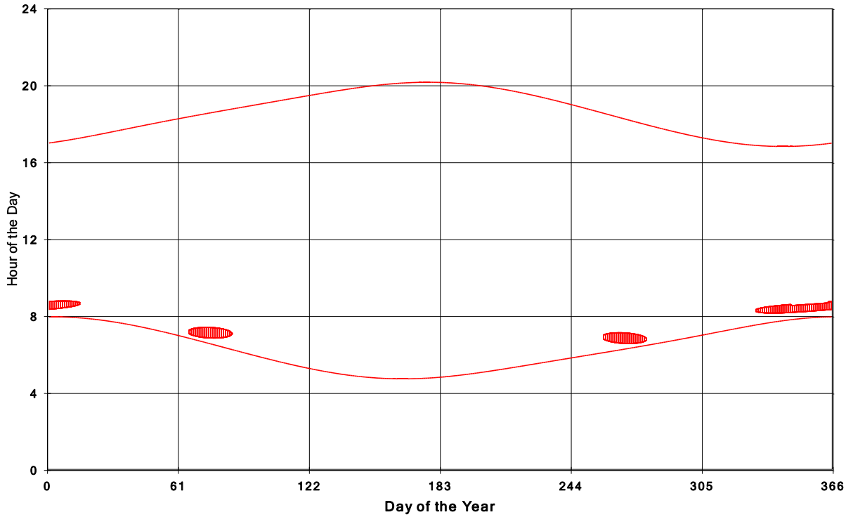
Goshen Wind Energy Centre Shadow Times on House 1705, All Windows from All Turbine
