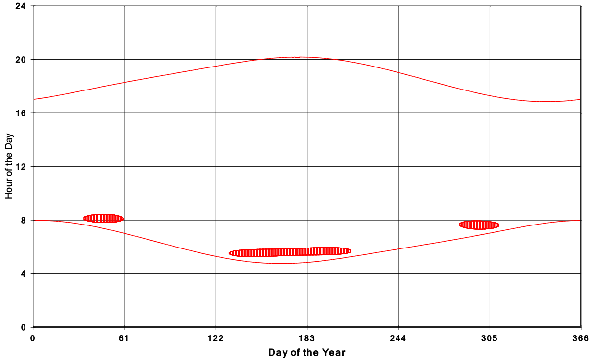
Goshen Wind Energy Centre Shadow Times on House 1722, All Windows from All Turbine
