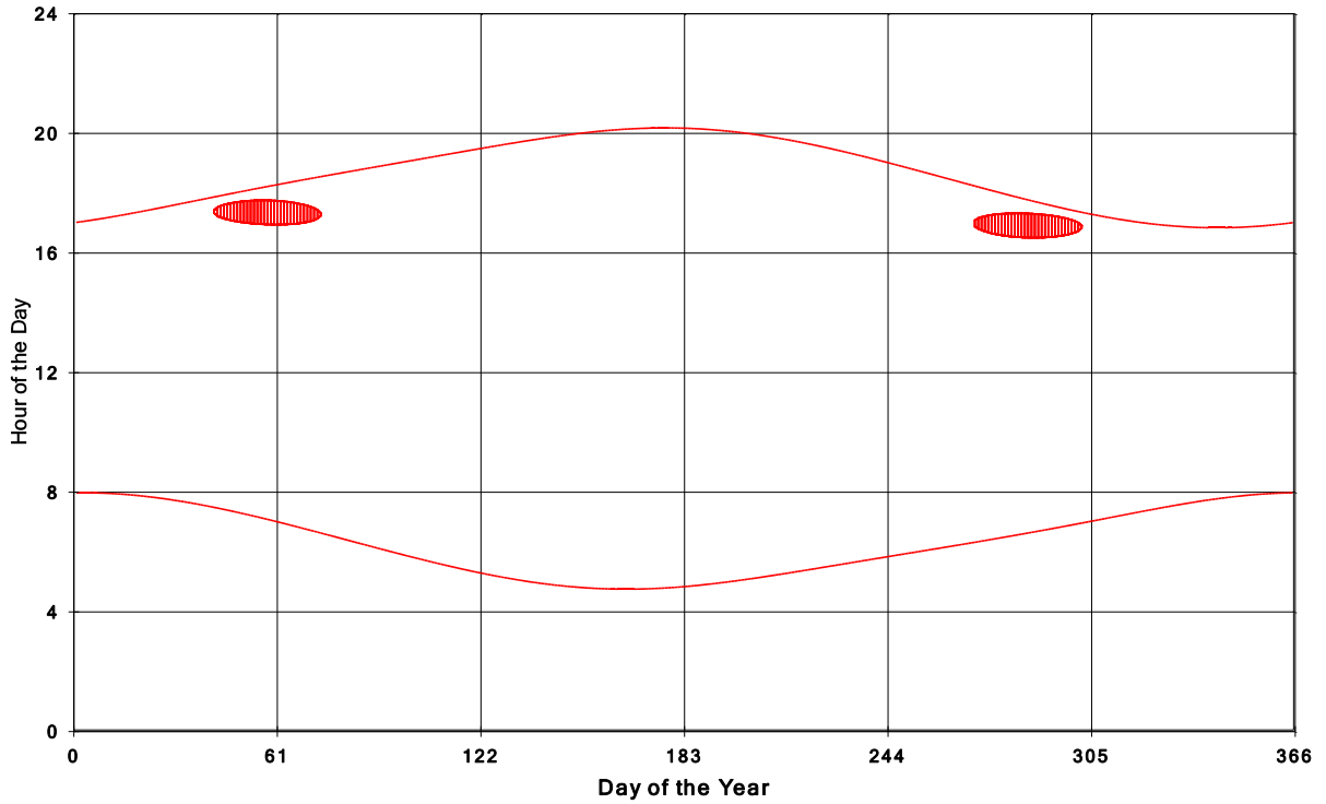
Goshen Wind Energy Centre Shadow Times on House 1840, All Windows from All Turbine
