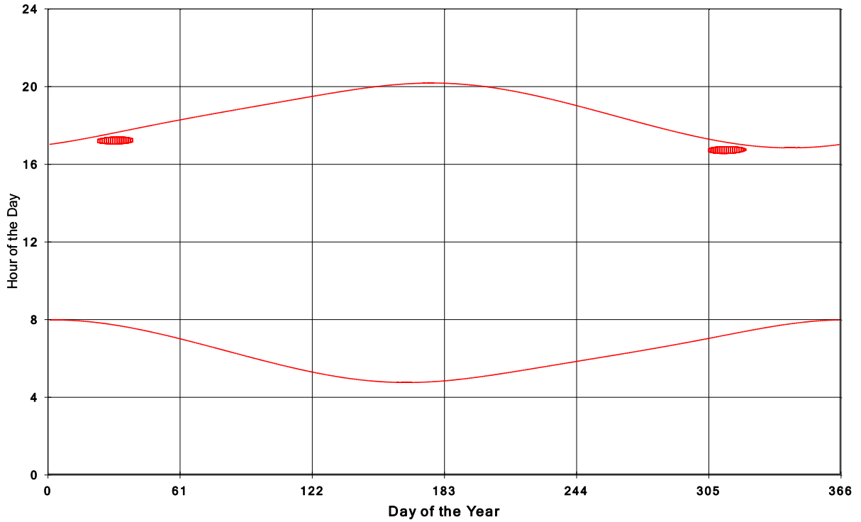
Goshen Wind Energy Centre Shadow Times on House 1765, All Windows from All Turbine
