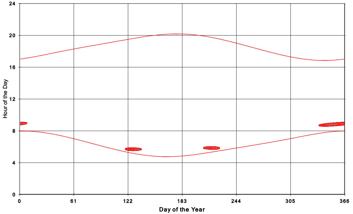
Goshen Wind Energy Centre Shadow Times on House 1700, All Windows from All Turbine
