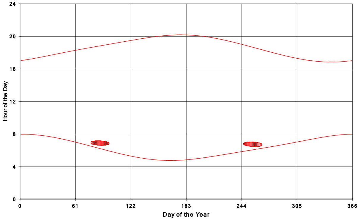
Goshen Wind Energy Centre Shadow Times on House 1701, All Windows from All Turbine
