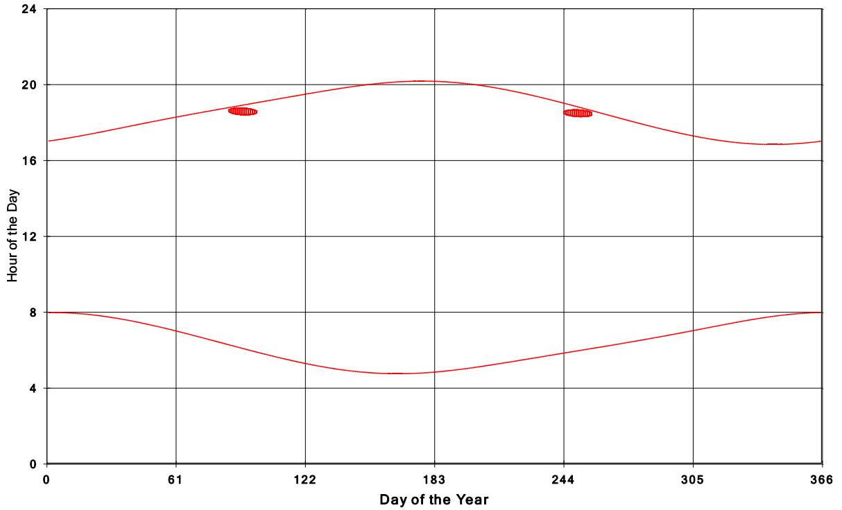
Goshen Wind Energy Centre Shadow Times on House 1762, All Windows from All Turbine
