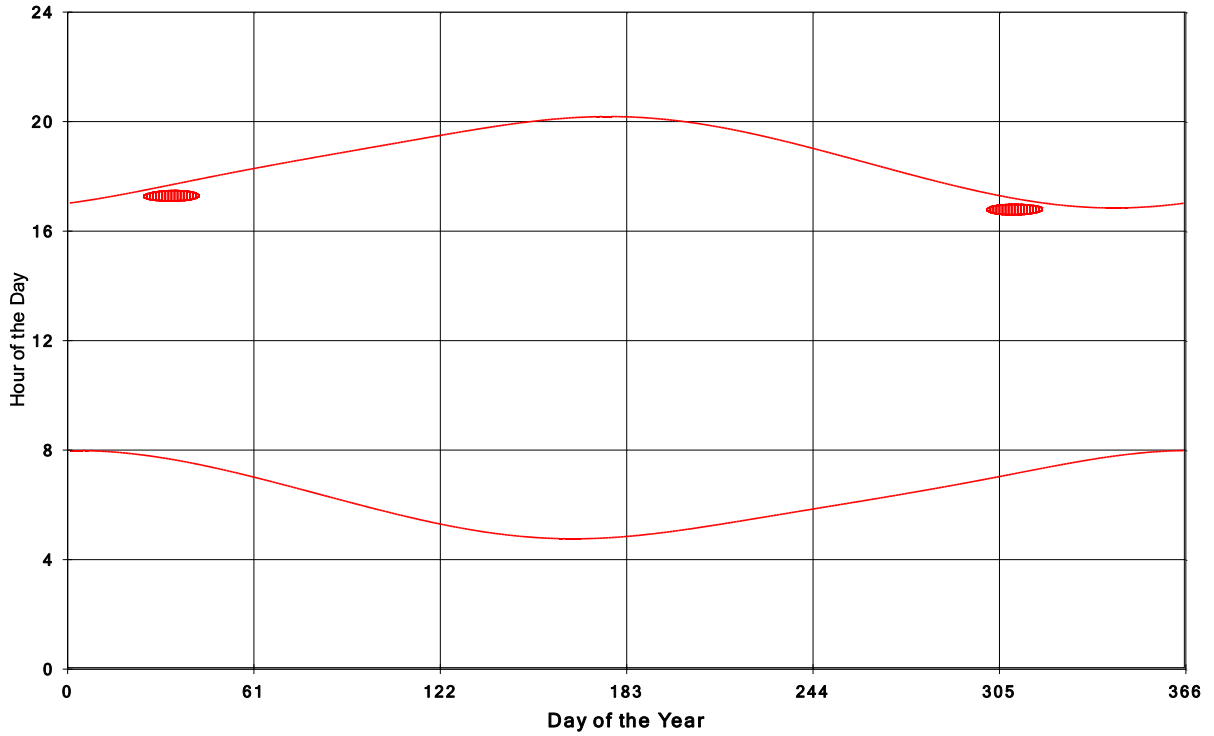
Goshen Wind Energy Centre Shadow Times on House 1761, All Windows from All Turbine
