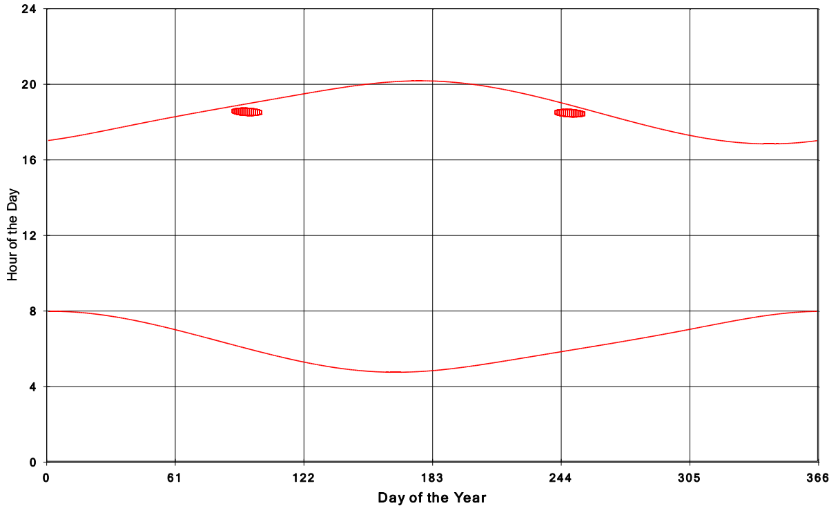
Goshen Wind Energy Centre Shadow Times on House 1750, All Windows from All Turbine
