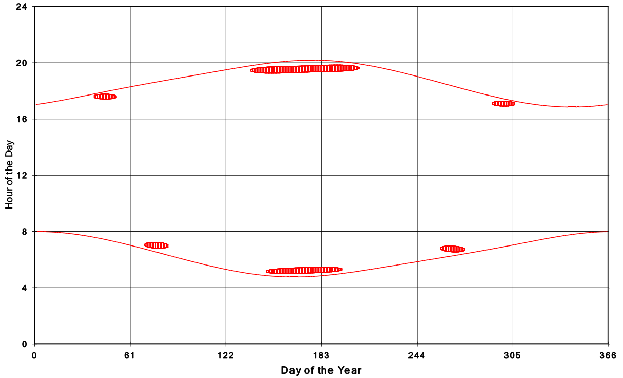
Goshen Wind Energy Centre Shadow Times on House 1854, All Windows from All Turbine
