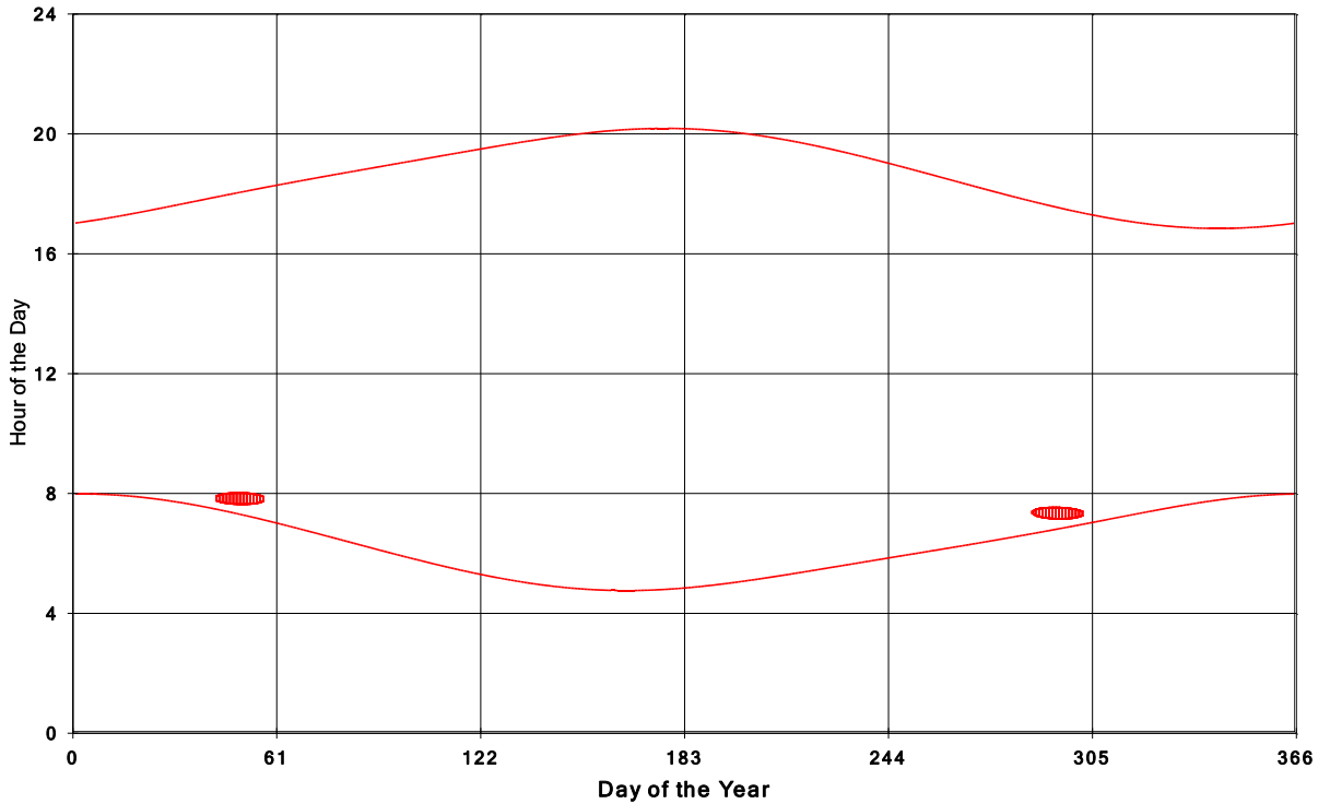
Jericho Wind Energy Centre Shadow Times on House 1813, All Windows from All Turbine
