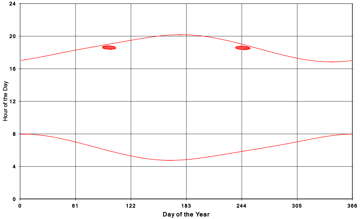
Goshen Wind Energy Centre Shadow Times on House 1751, All Windows from All Turbine
