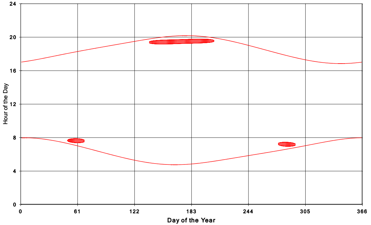
Goshen Wind Energy Centre Shadow Times on House 1693, All Windows from All Turbine
