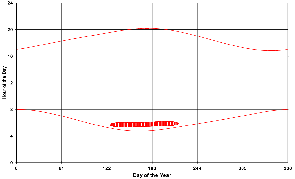
Goshen Wind Energy Centre Shadow Times on House 1820, All Windows from All Turbine
