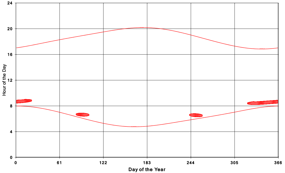
Goshen Wind Energy Centre Shadow Times on House 1717, All Windows from All Turbine
