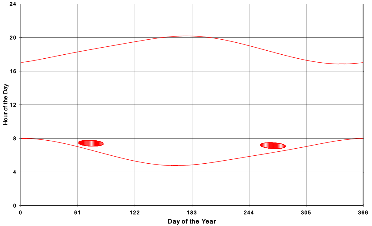
Goshen Wind Energy Centre Shadow Times on House 1737, All Windows from All Turbine
