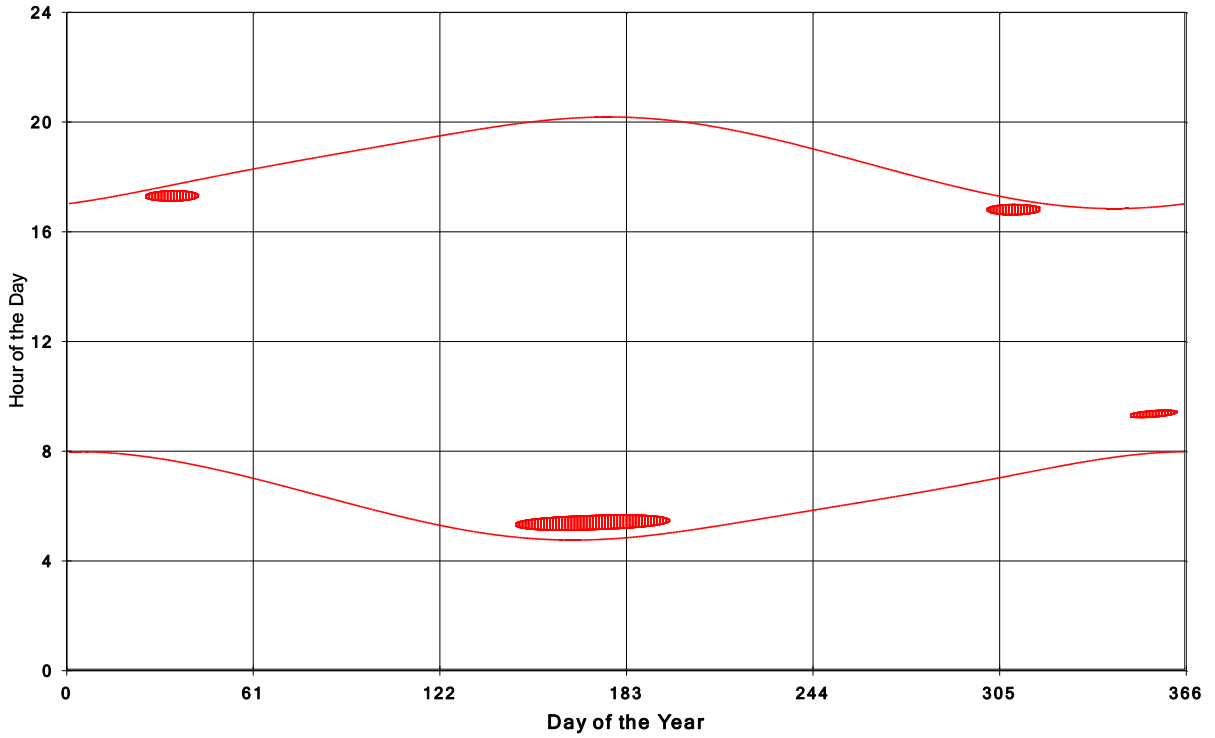
Jericho Wind Energy Centre Shadow Times on House 1816, All Windows from All Turbine
