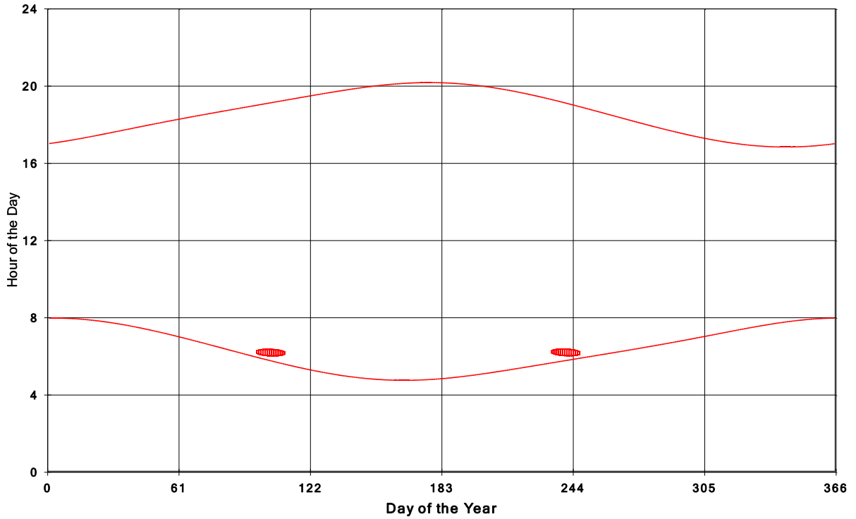
Goshen Wind Energy Centre Shadow Times on House 1783, All Windows from All Turbine
