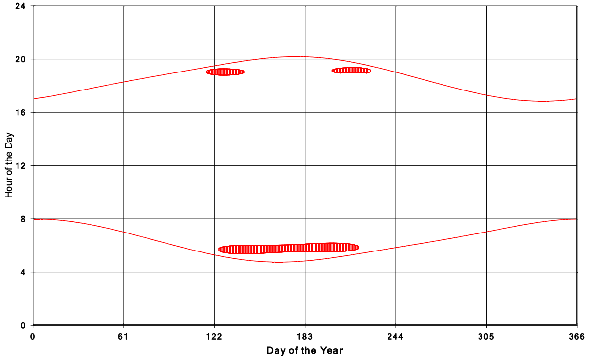
Goshen Wind Energy Centre Shadow Times on House 1785, All Windows from All Turbine
