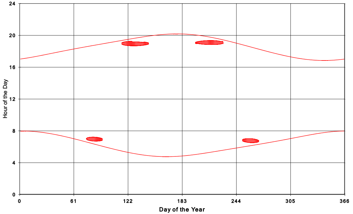
Goshen Wind Energy Centre Shadow Times on House 1843, All Windows from All Turbine
