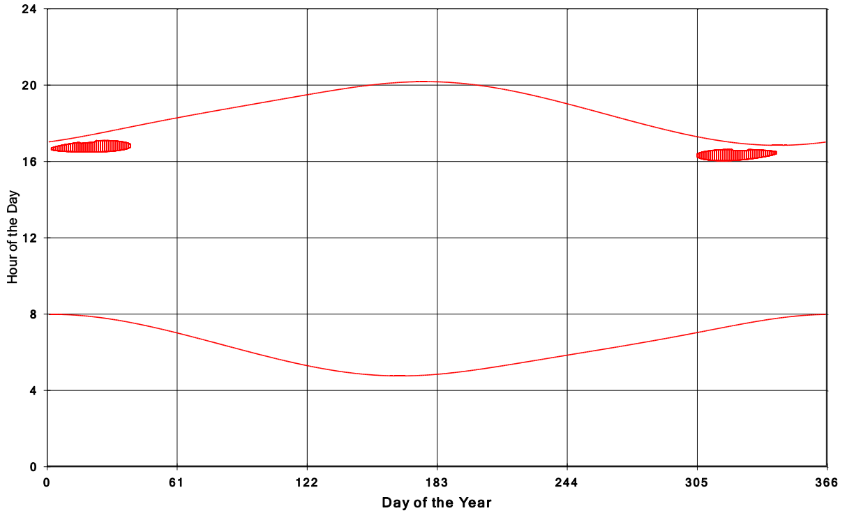
Goshen Wind Energy Centre Shadow Times on House 1694, All Windows from All Turbine
