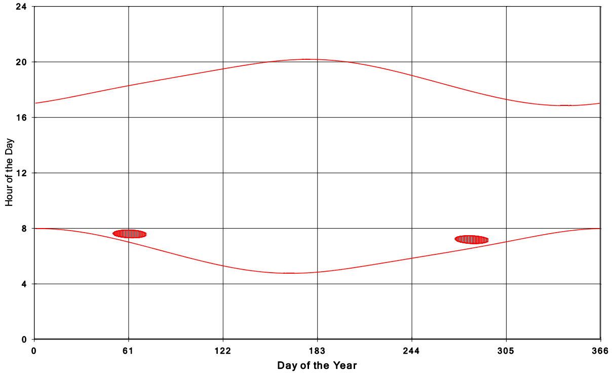
Goshen Wind Energy Centre Shadow Times on House 1699, All Windows from All Turbine
