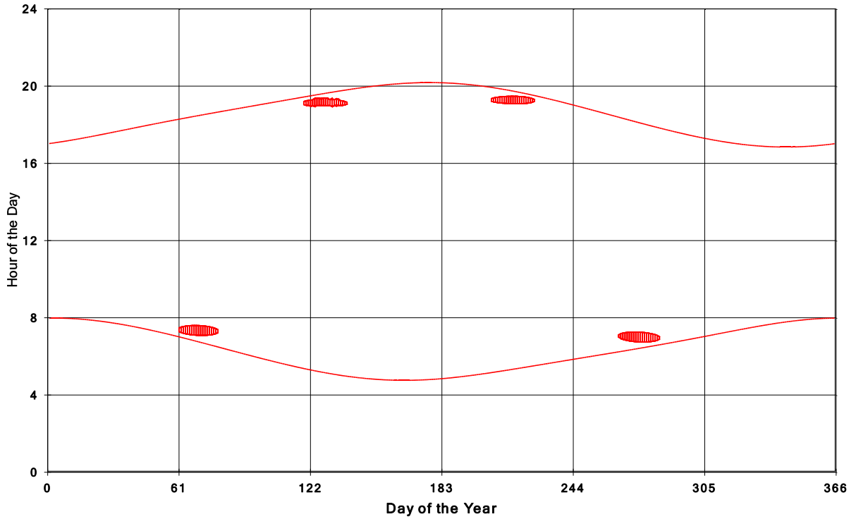
Goshen Wind Energy Centre Shadow Times on House 1860, All Windows from All Turbine
