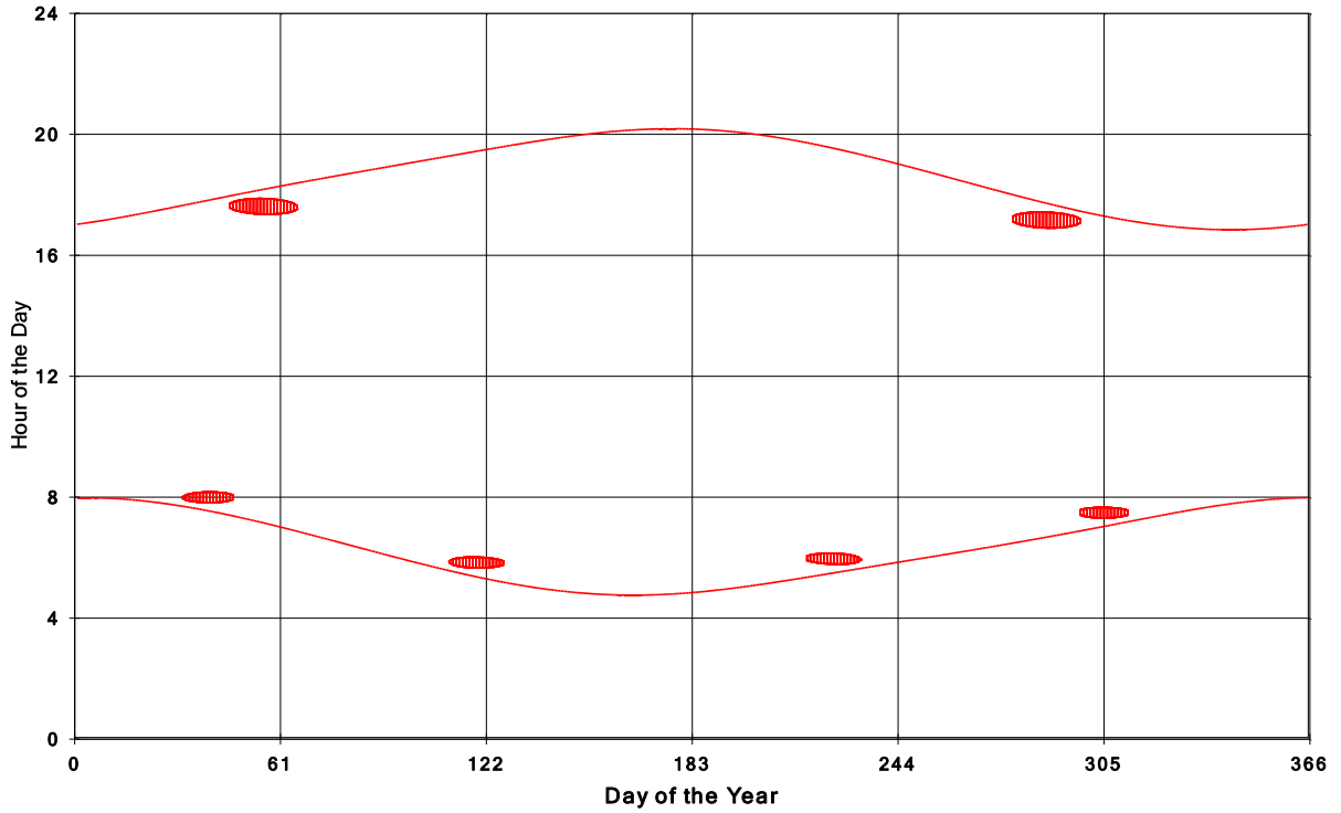
Goshen Wind Energy Centre Shadow Times on House 1707, All Windows from All Turbine
