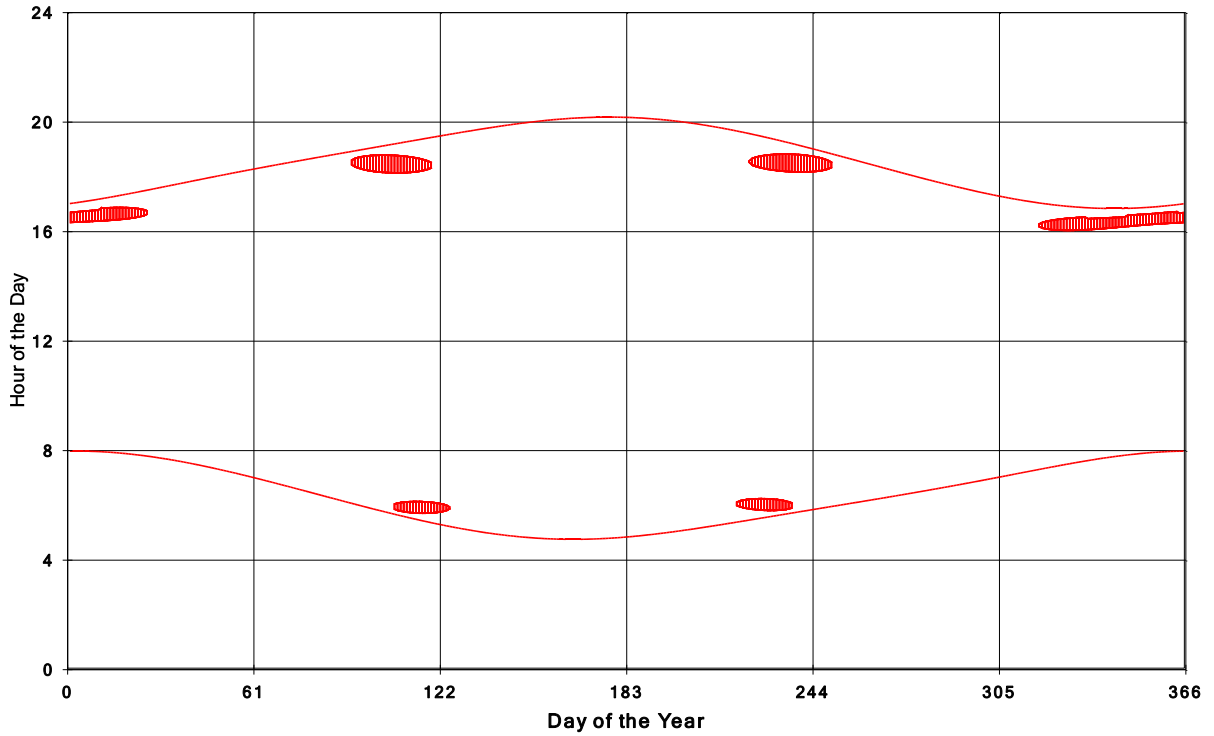
Goshen Wind Energy Centre Shadow Times on House 1852, All Windows from All Turbine
