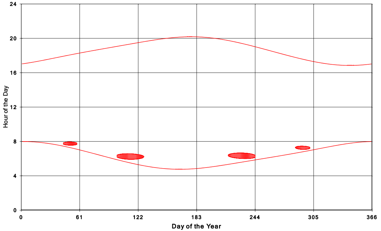
Goshen Wind Energy Centre Shadow Times on House 1862, All Windows from All Turbine
