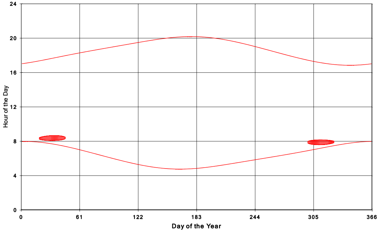
Goshen Wind Energy Centre Shadow Times on House 1788, All Windows from All Turbine
