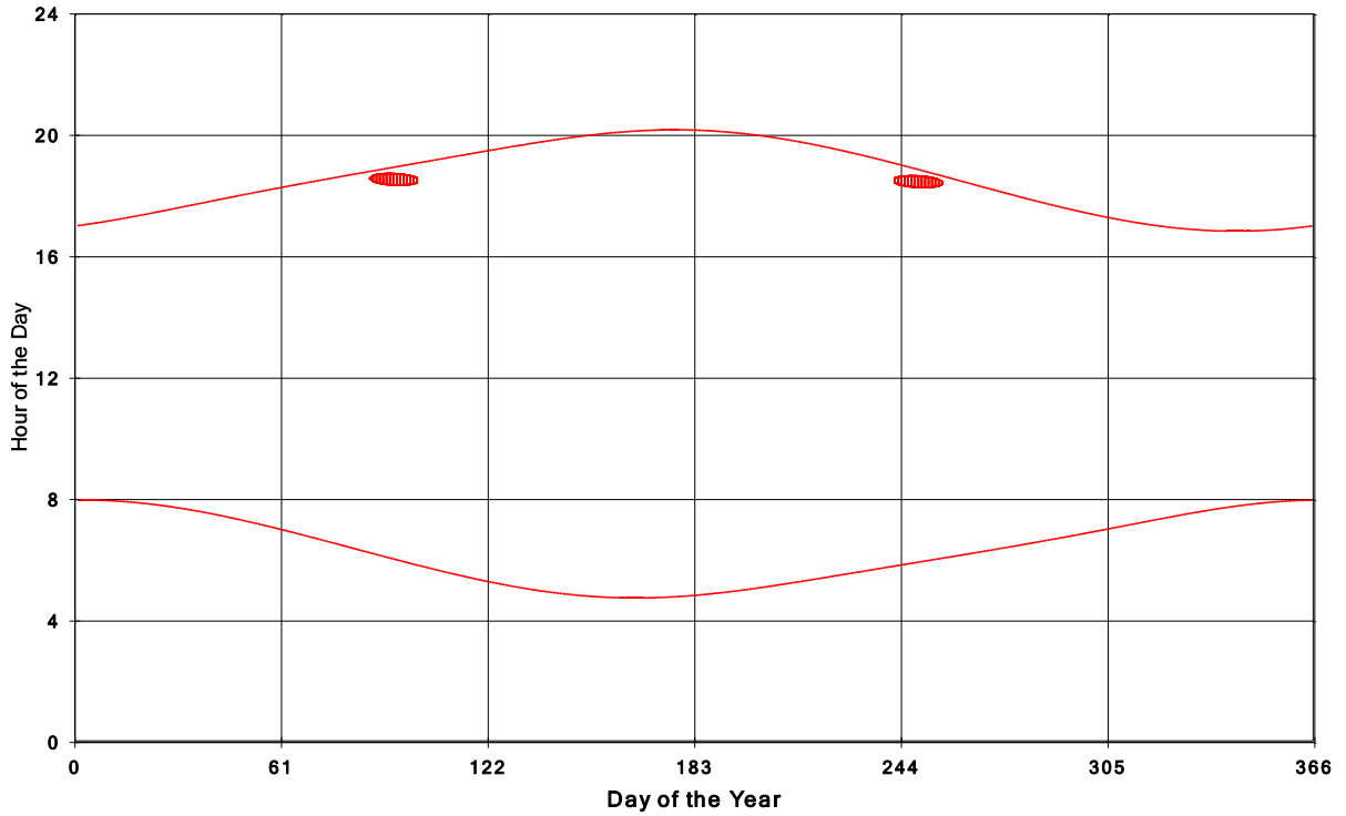
Goshen Wind Energy Centre Shadow Times on House 1752, All Windows from All Turbine
