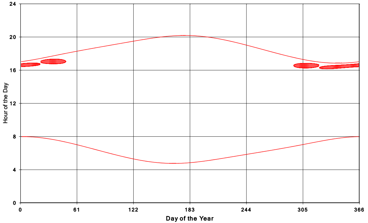
Goshen Wind Energy Centre Shadow Times on House 1797, All Windows from All Turbine
