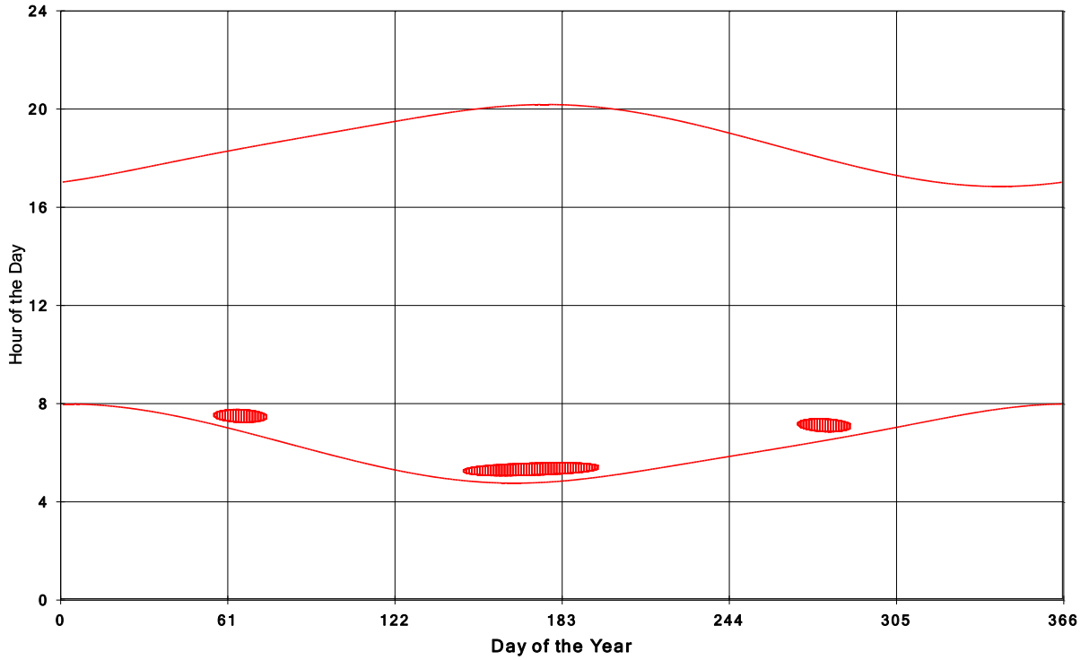
Goshen Wind Energy Centre Shadow Times on House 1716, All Windows from All Turbine
