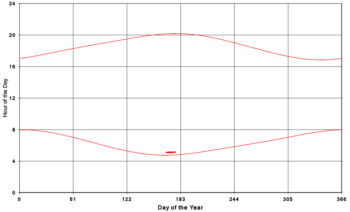
Goshen Wind Energy Centre Shadow Times on House 1702, All Windows from All Turbine
