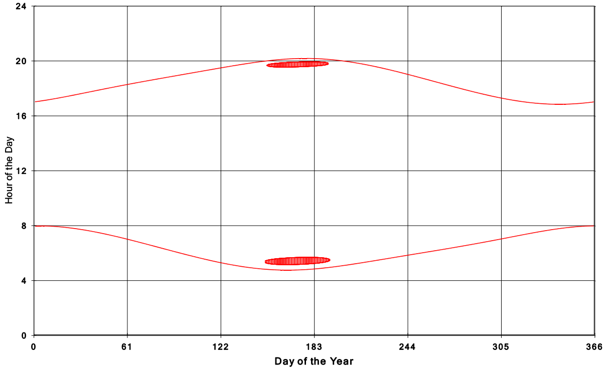
Goshen Wind Energy Centre Shadow Times on House 1845, All Windows from All Turbine
