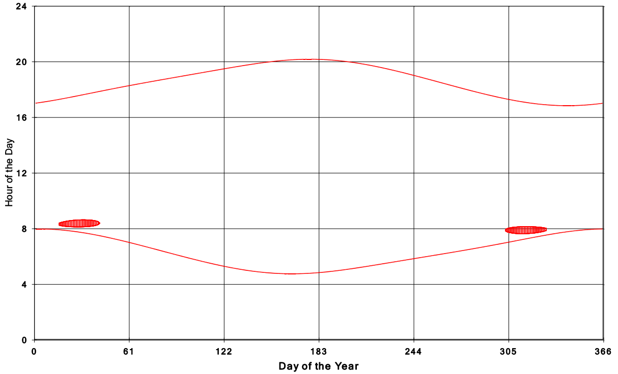
Goshen Wind Energy Centre Shadow Times on House 1822, All Windows from All Turbine
