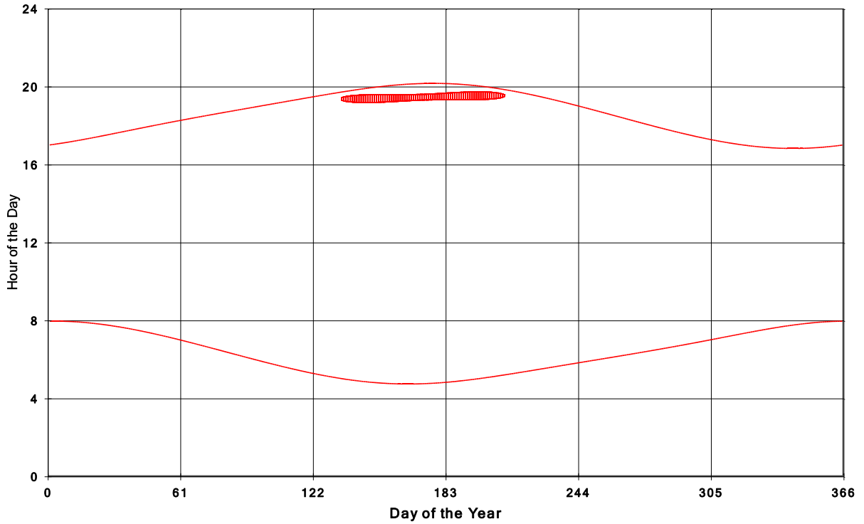
Goshen Wind Energy Centre Shadow Times on House 1791, All Windows from All Turbine
