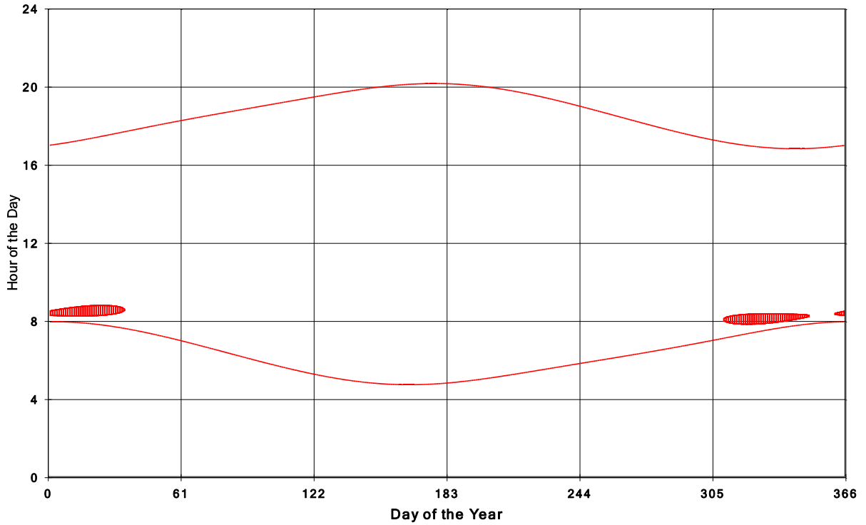
Goshen Wind Energy Centre Shadow Times on House 1821, All Windows from All Turbine
