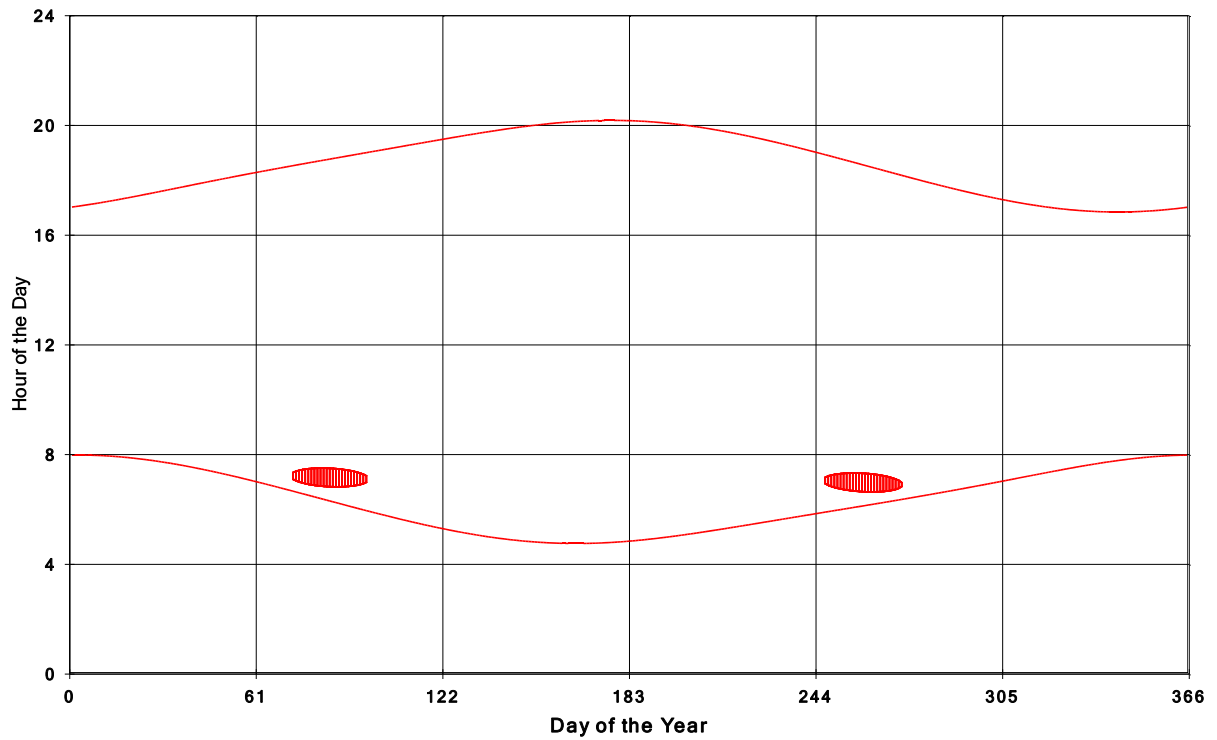
Jericho Wind Energy Centre Shadow Times on House 1815, All Windows from All Turbine:
