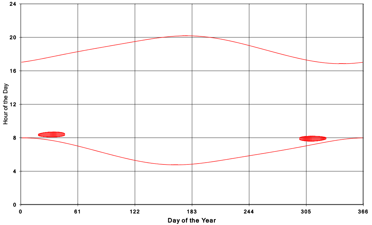
Goshen Wind Energy Centre Shadow Times on House 1789, All Windows from All Turbine
