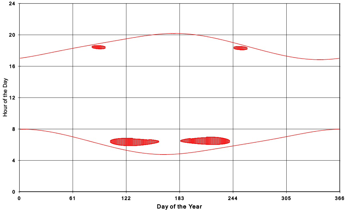
Goshen Wind Energy Centre Shadow Times on House 1709, All Windows from All Turbine
