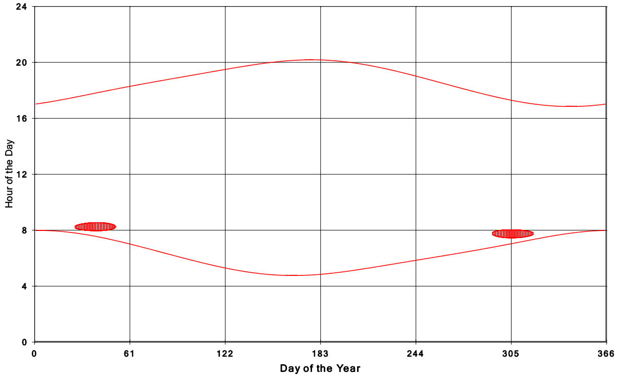
Goshen Wind Energy Centre Shadow Times on House 1735, All Windows from All Turbine
