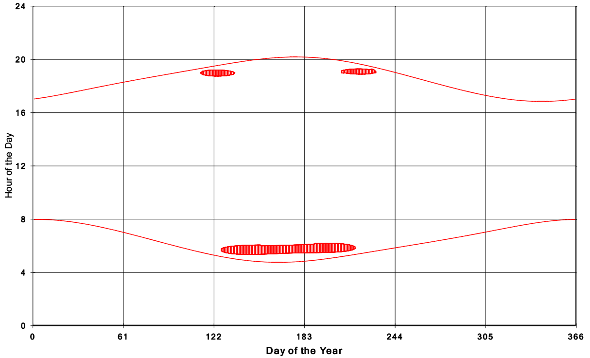
Goshen Wind Energy Centre Shadow Times on House 1786, All Windows from All Turbine
