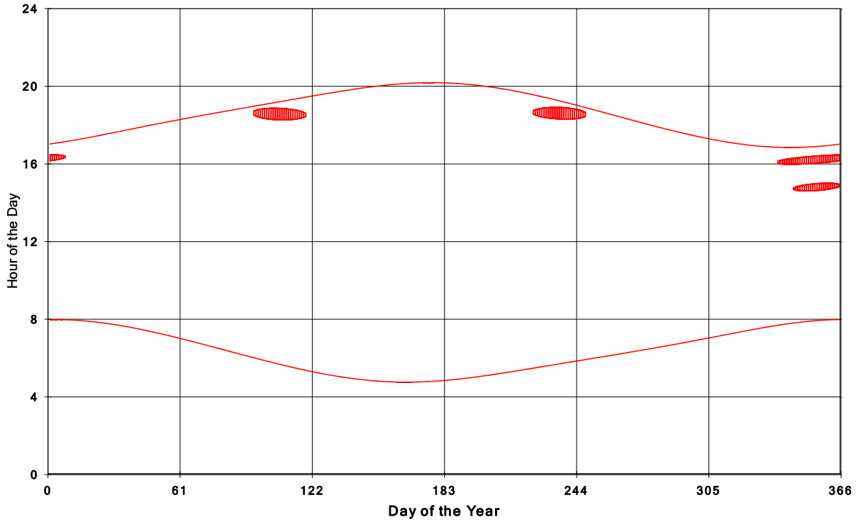
Goshen Wind Energy Centre Shadow Times on House 1866, All Windows from All Turbine
