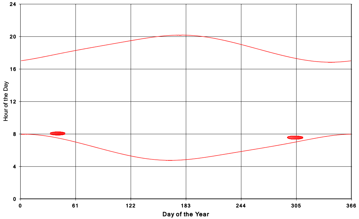
Jericho Wind Energy Centre Shadow Times on House 1814, All Windows from All Turbine:
