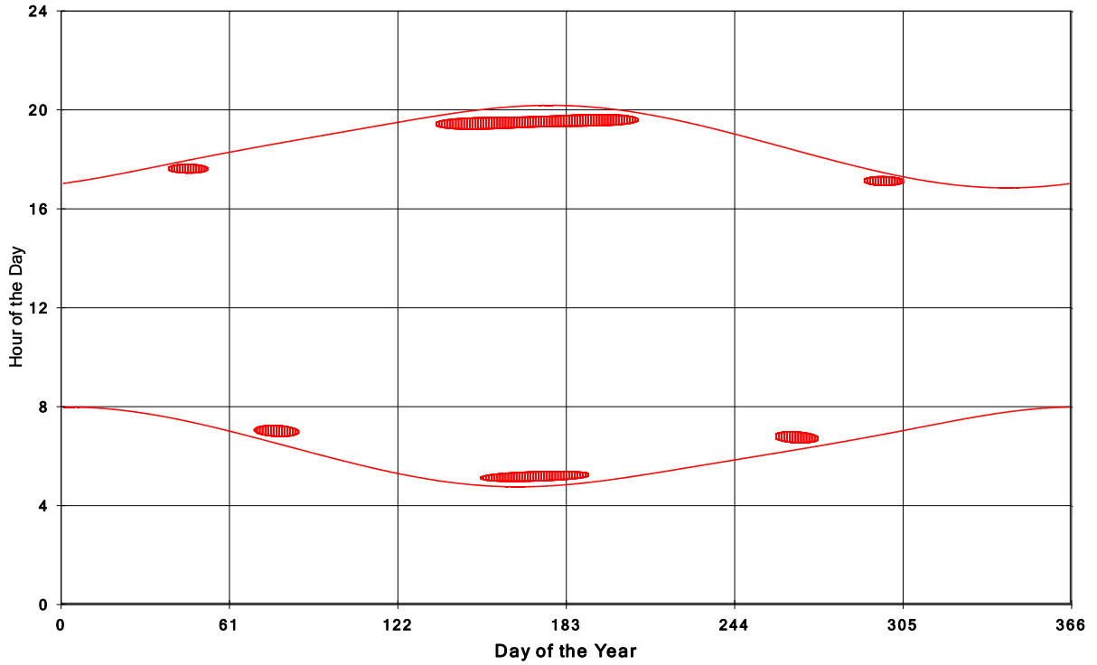
Goshen Wind Energy Centre Shadow Times on House 1859, All Windows from All Turbine
