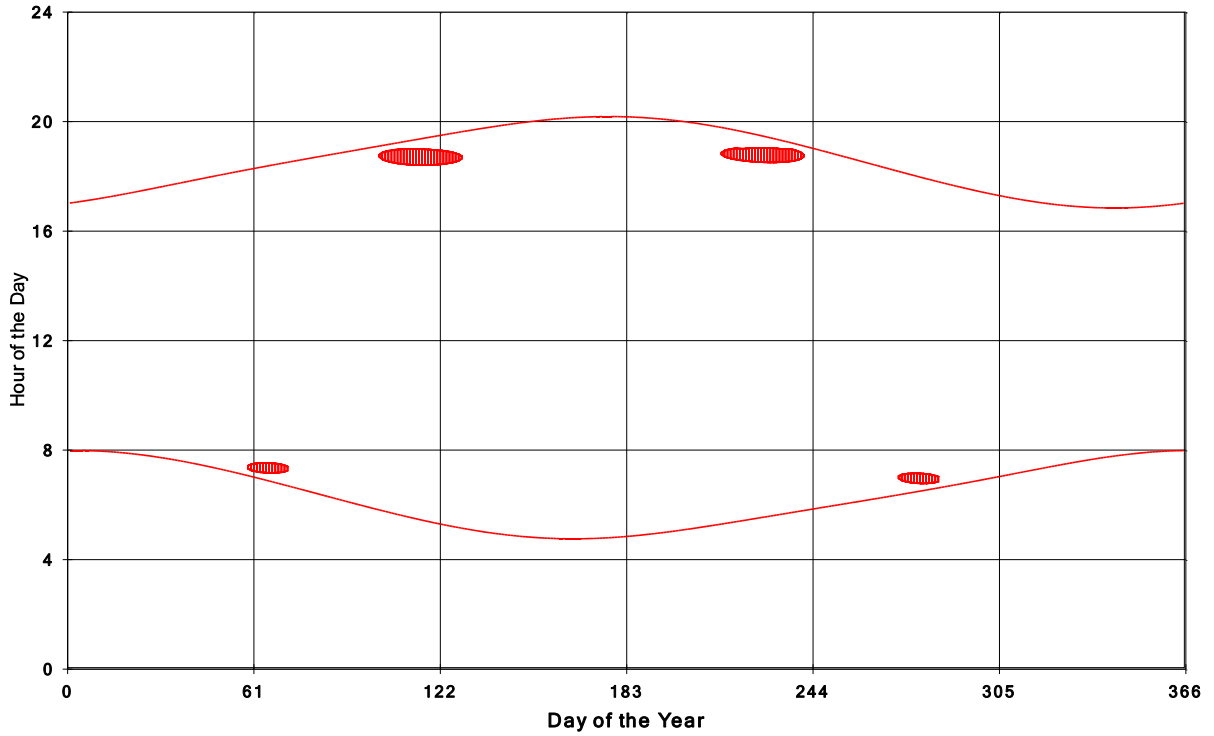
Goshen Wind Energy Centre Shadow Times on House 1841, All Windows from All Turbine
