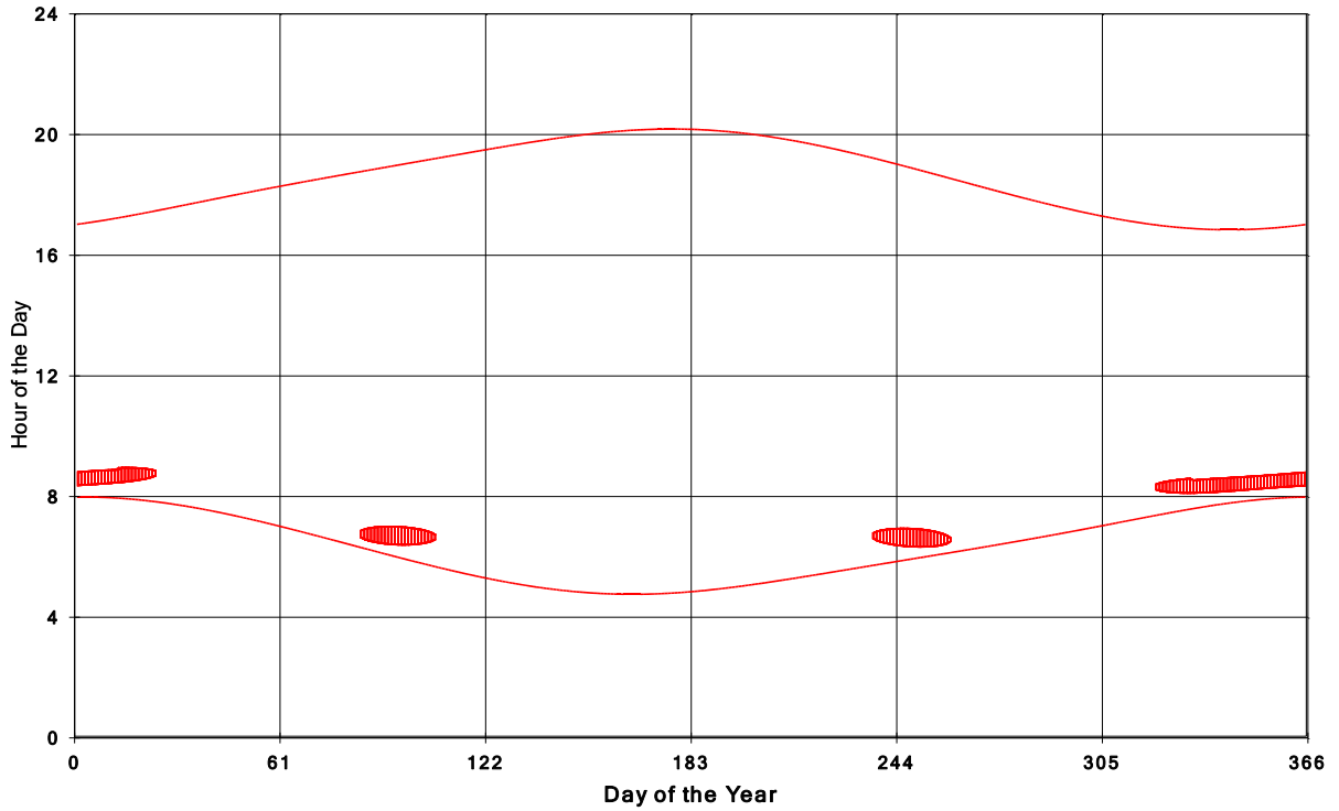
Goshen Wind Energy Centre Shadow Times on House 1779, All Windows from All Turbine
