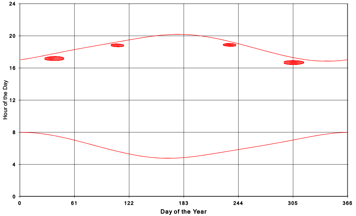
Goshen Wind Energy Centre Shadow Times on House 1867, All Windows from All Turbine
