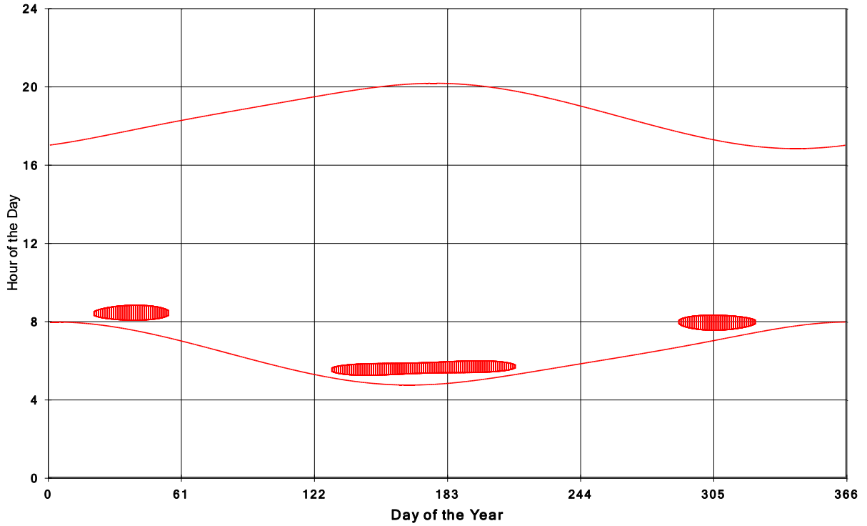
Goshen Wind Energy Centre Shadow Times on House 1776, All Windows from All Turbine
