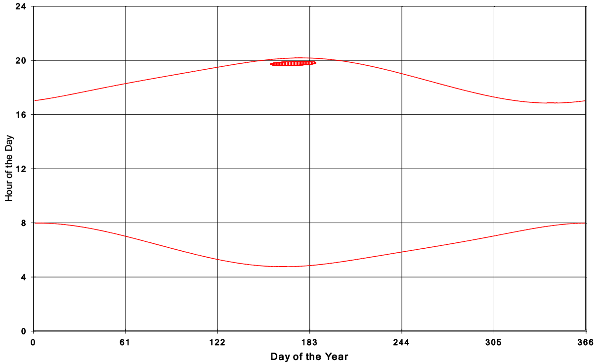
Goshen Wind Energy Centre Shadow Times on House 1793, All Windows from All Turbine
