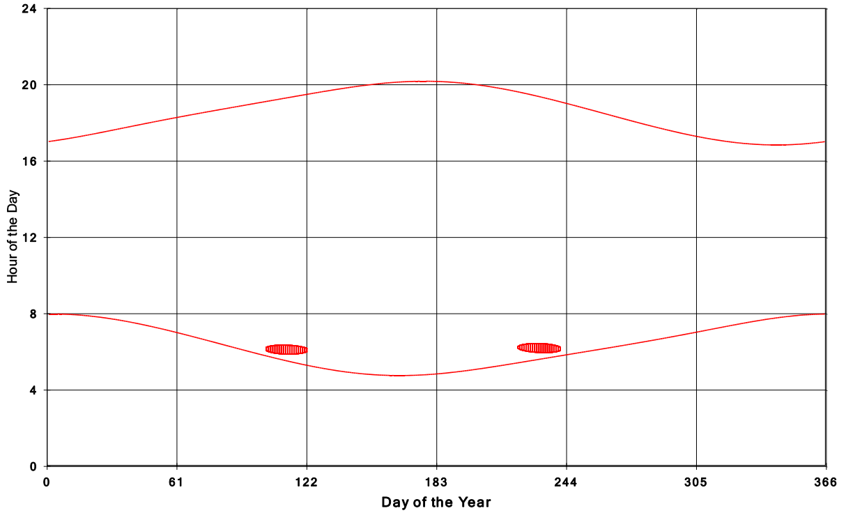
Goshen Wind Energy Centre Shadow Times on House 1811, All Windows from All Turbine
