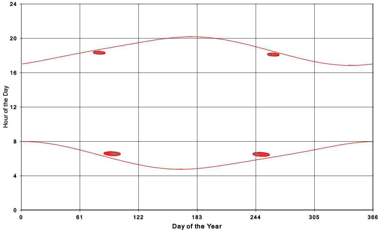
Goshen Wind Energy Centre Shadow Times on House 1837, All Windows from All Turbine
