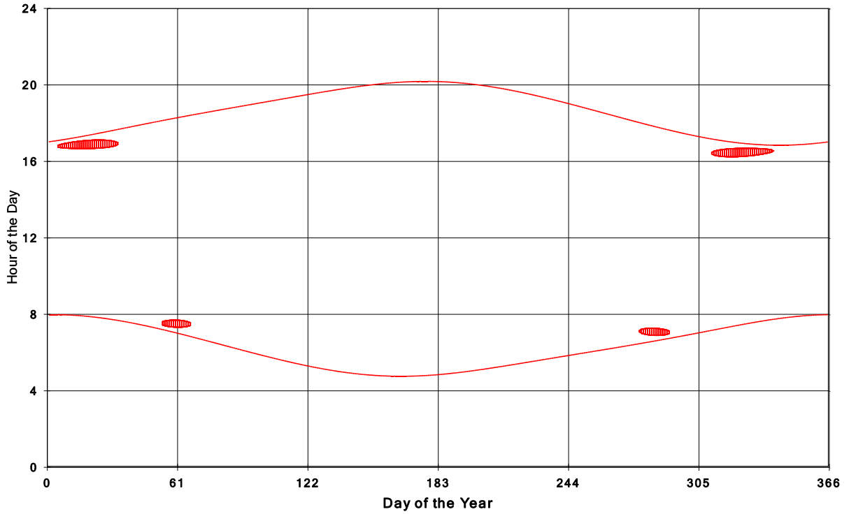
Goshen Wind Energy Centre Shadow Times on House 1839, All Windows from All Turbine
