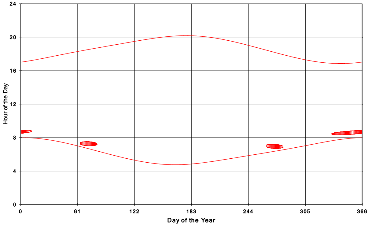
Goshen Wind Energy Centre Shadow Times on House 1780, All Windows from All Turbine
