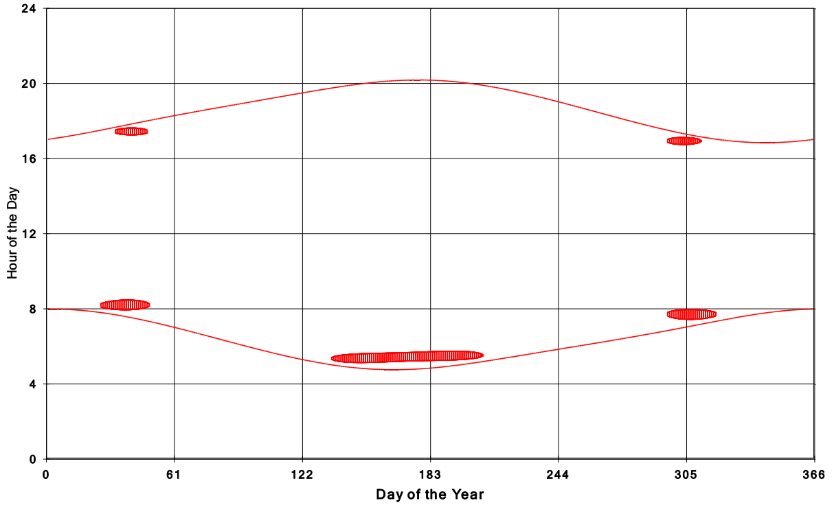
Goshen Wind Energy Centre Shadow Times on House 1861, All Windows from All Turbine
