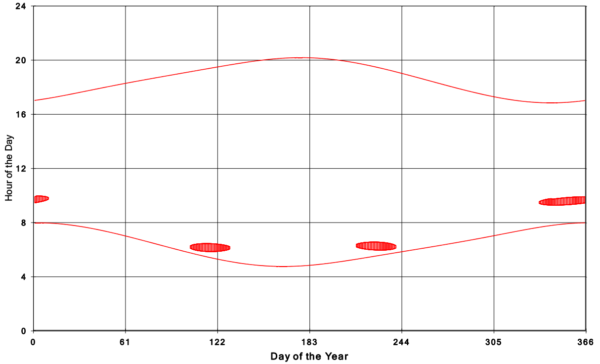
Goshen Wind Energy Centre Shadow Times on House 1764, All Windows from All Turbine
