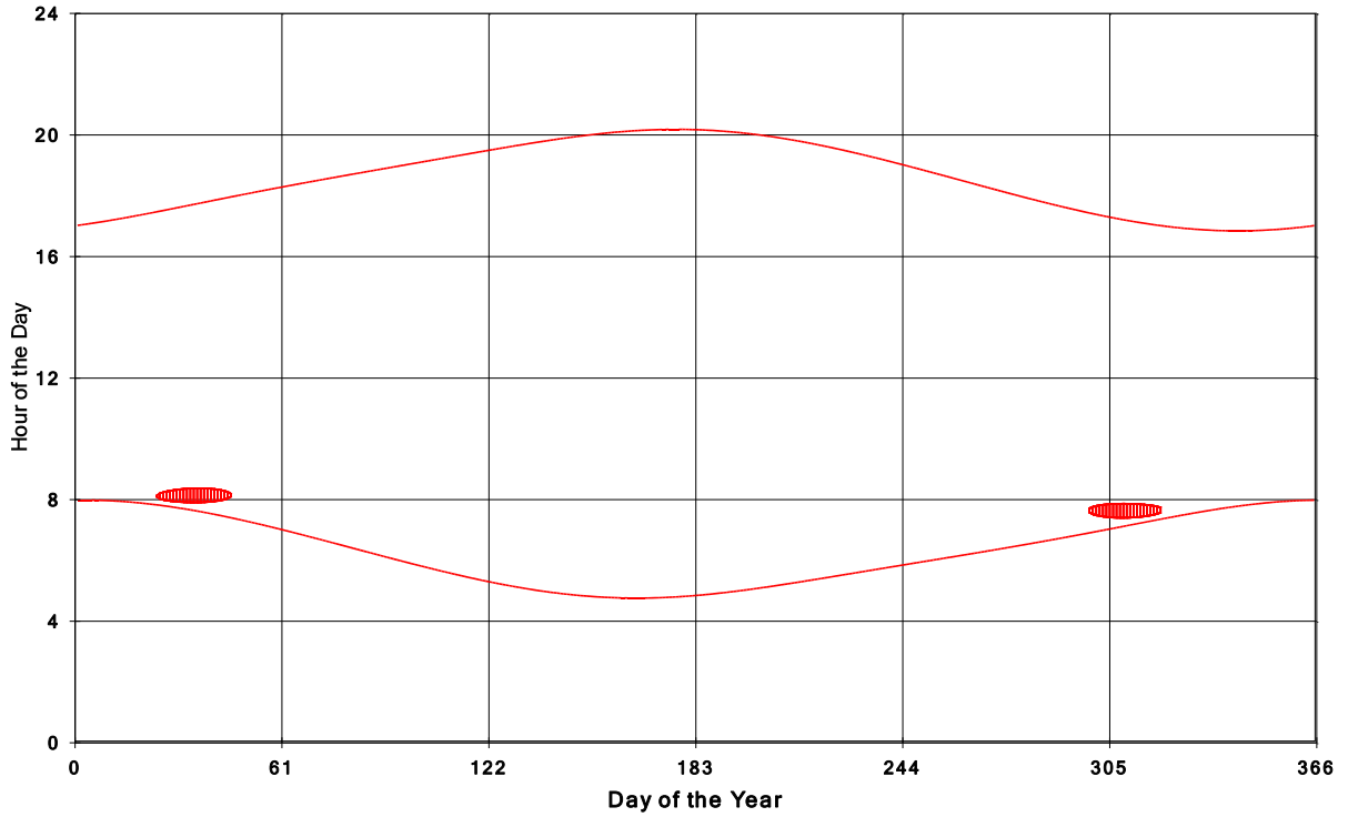
Goshen Wind Energy Centre Shadow Times on House 1853, All Windows from All Turbine
