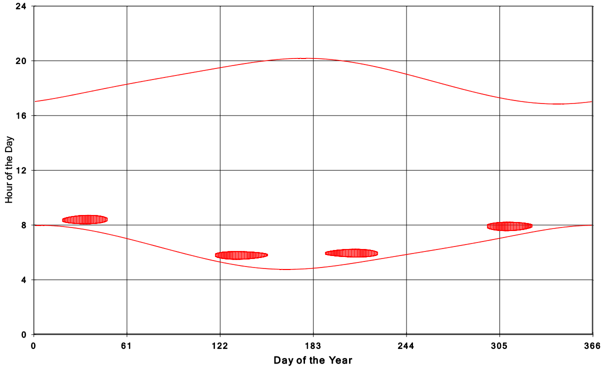
Goshen Wind Energy Centre Shadow Times on House 1818, All Windows from All Turbine
