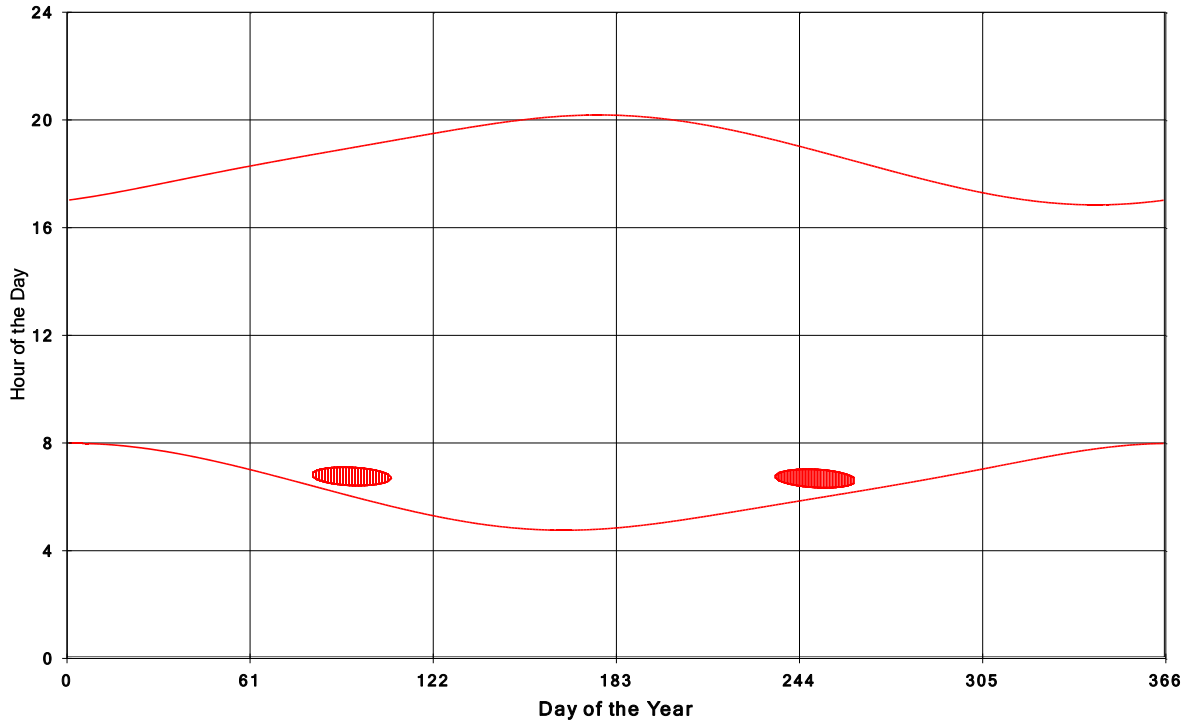
Jericho Wind Energy Centre Shadow Times on House 1755, All Windows from All Turbine:
