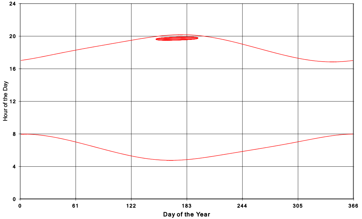
Goshen Wind Energy Centre Shadow Times on House 1794, All Windows from All Turbine
