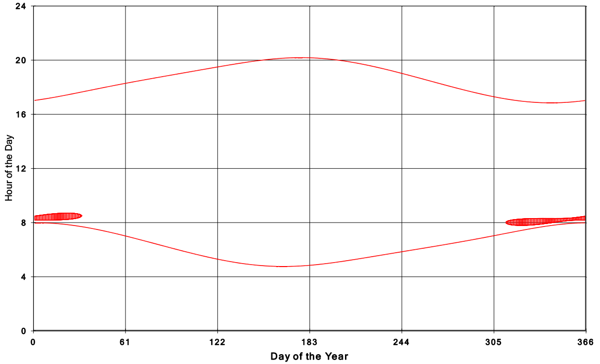
Goshen Wind Energy Centre Shadow Times on House 1748, All Windows from All Turbine
