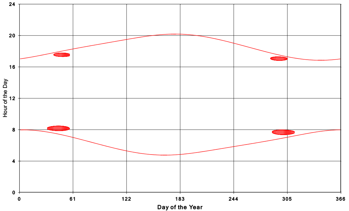
Goshen Wind Energy Centre Shadow Times on House 1817, All Windows from All Turbine
