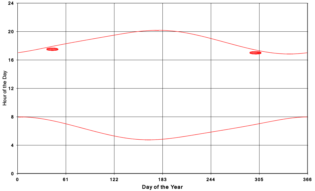
Goshen Wind Energy Centre Shadow Times on House 1803, All Windows from All Turbine
