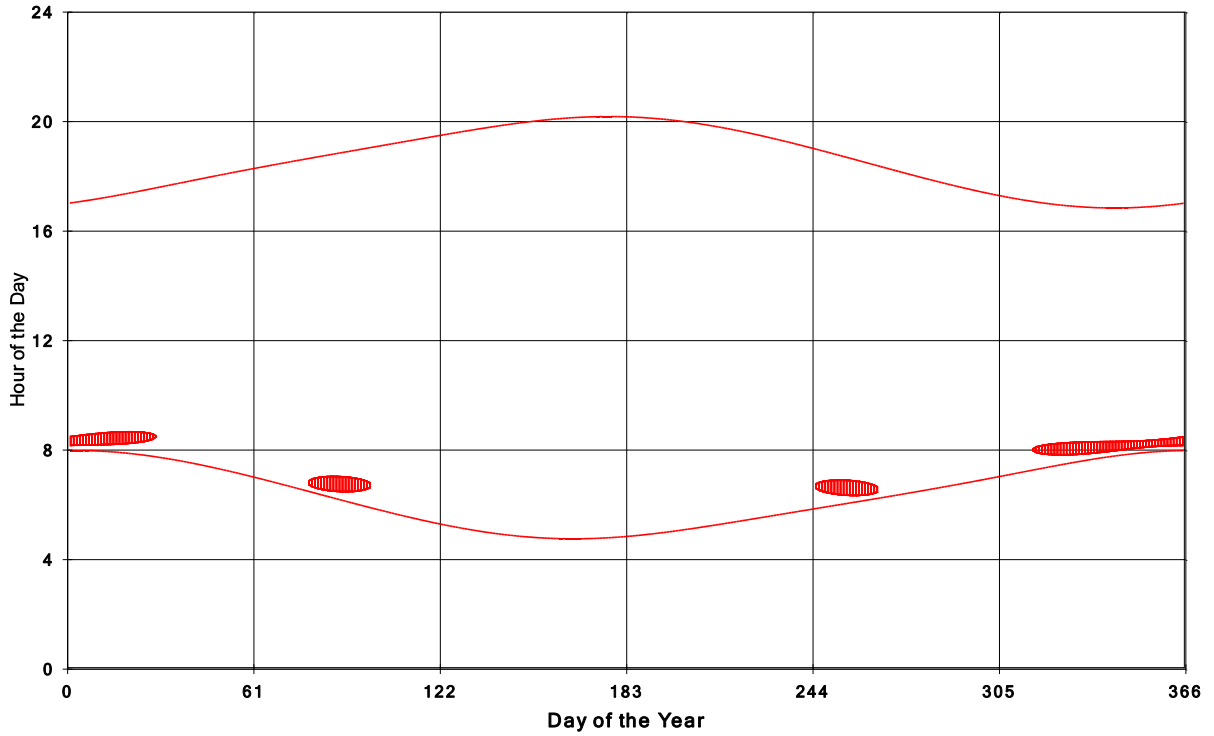
Goshen Wind Energy Centre Shadow Times on House 1557, All Windows from All Turbine
