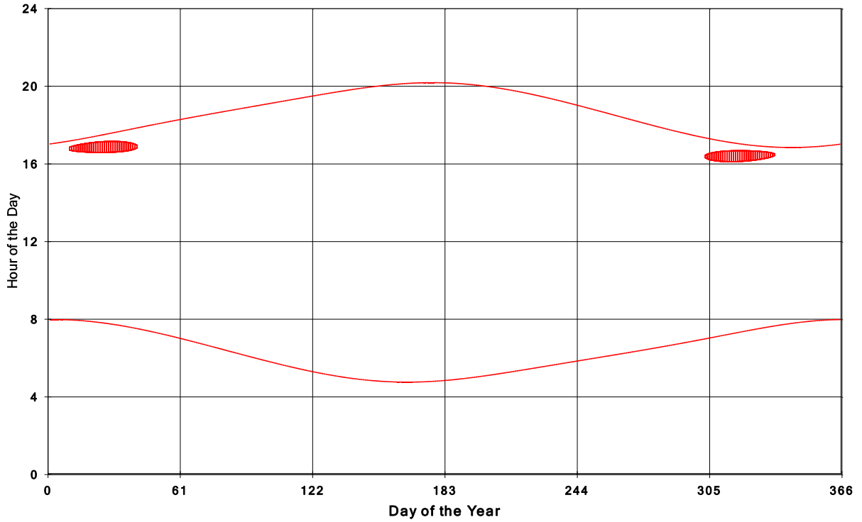
Goshen Wind Energy Centre Shadow Times on House 1569, All Windows from All Turbine
