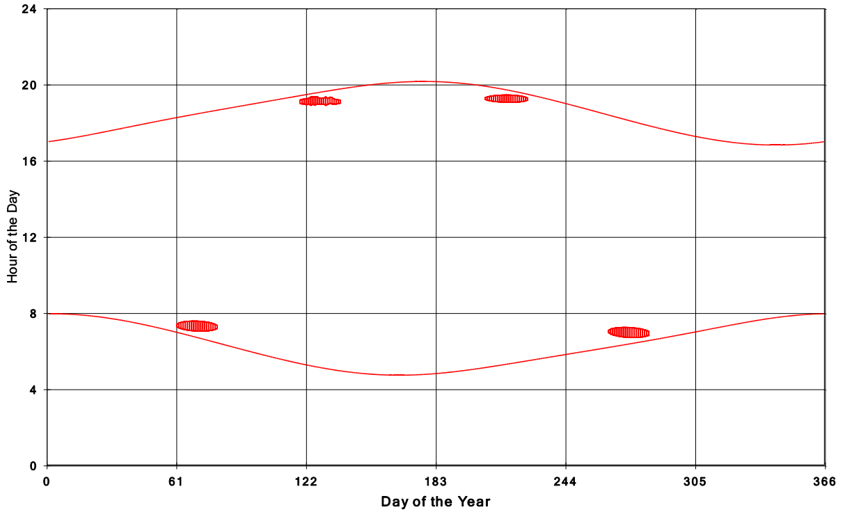
Goshen Wind Energy Centre Shadow Times on House 1570, All Windows from All Turbine
