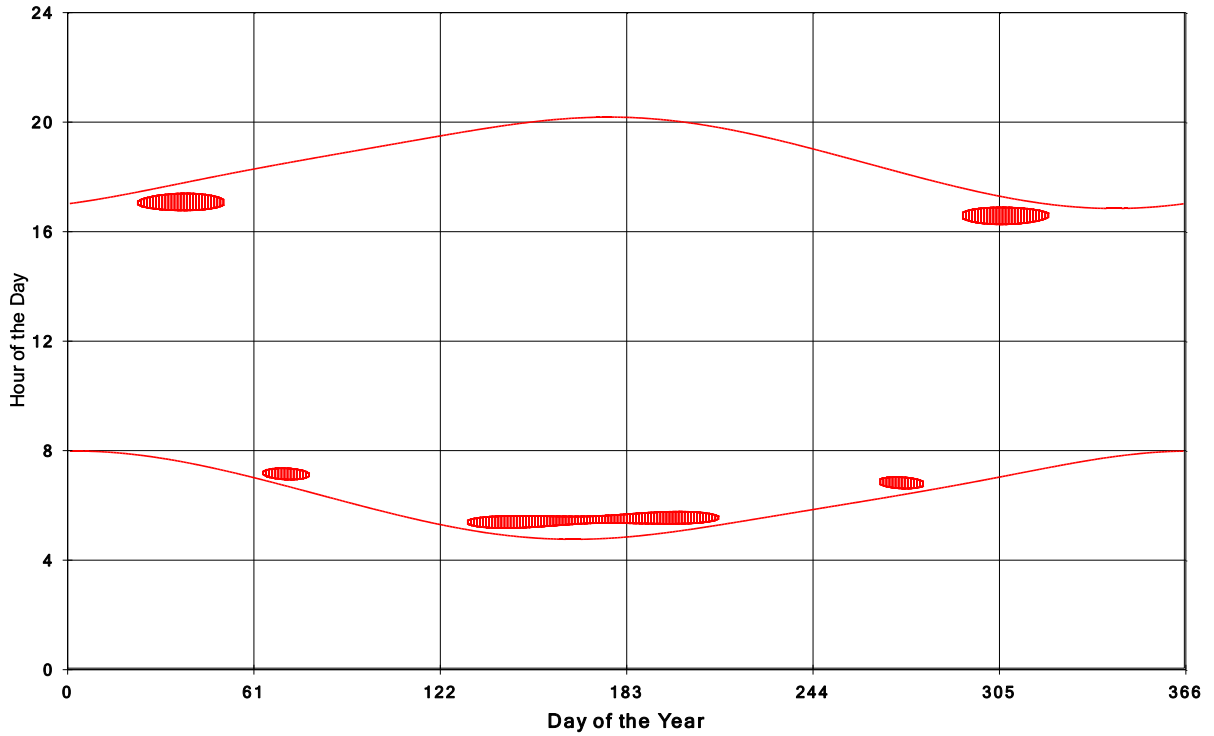
Goshen Wind Energy Centre Shadow Times on House 1556, All Windows from All Turbine
