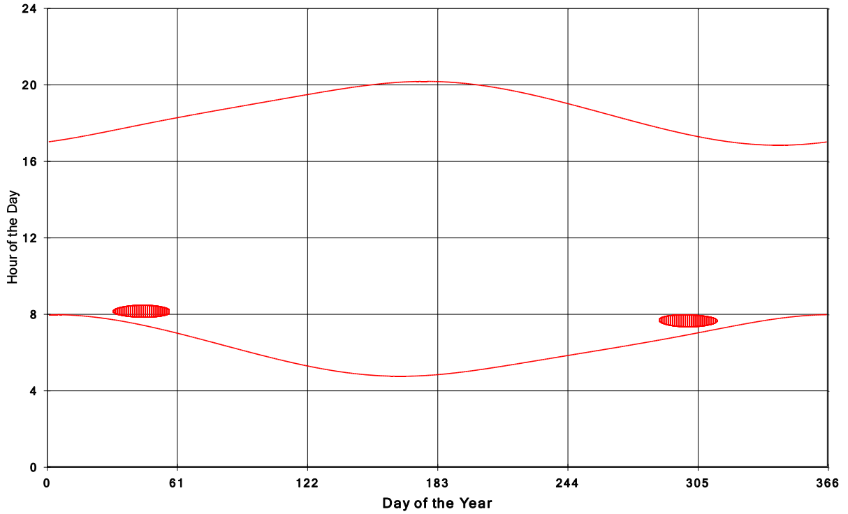
Goshen Wind Energy Centre Shadow Times on House 1588, All Windows from All Turbine
