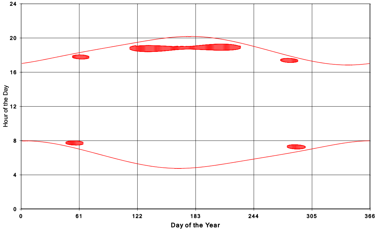
Goshen Wind Energy Centre Shadow Times on House 1426, All Windows from All Turbine
