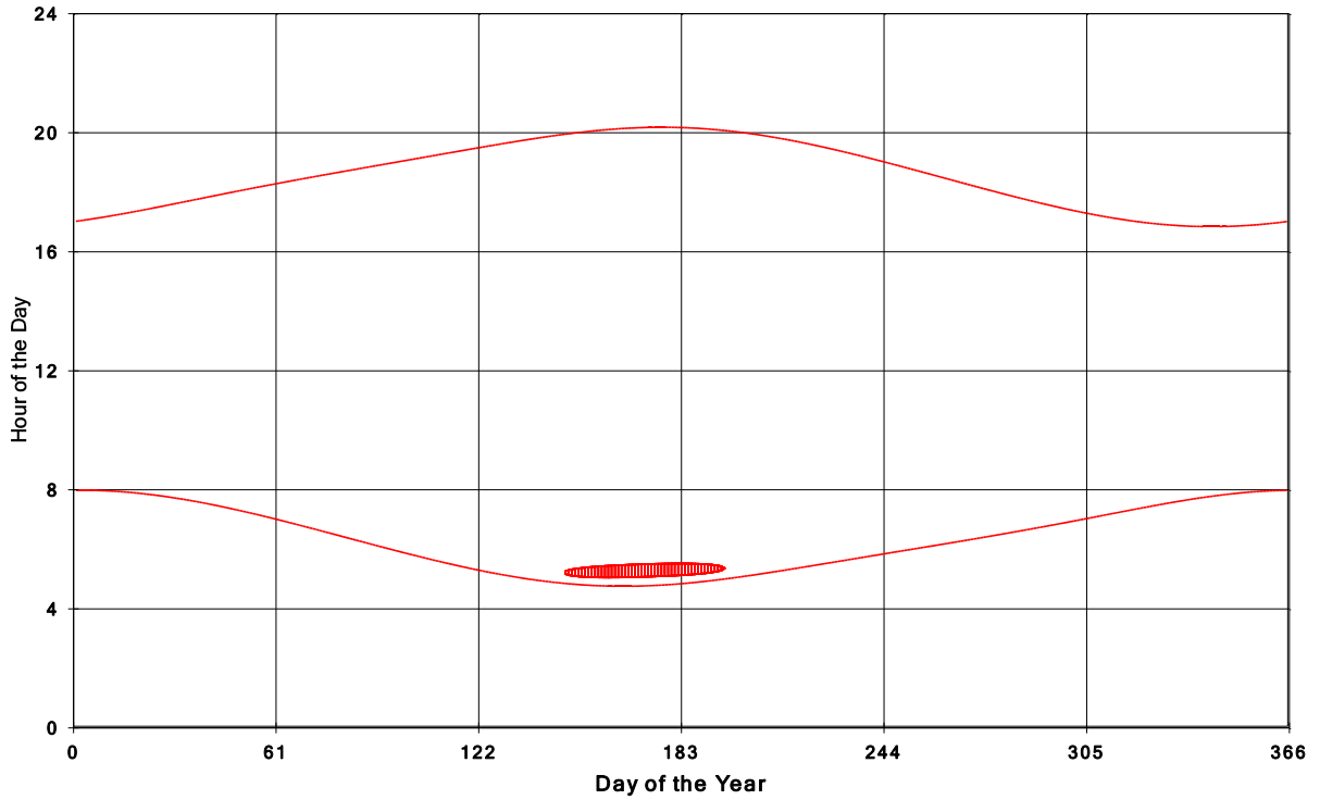
Goshen Wind Energy Centre Shadow Times on House 1399, All Windows from All Turbine
