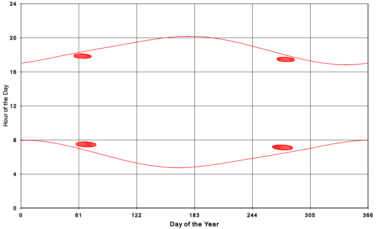
Goshen Wind Energy Centre Shadow Times on House 1445, All Windows from All Turbine
