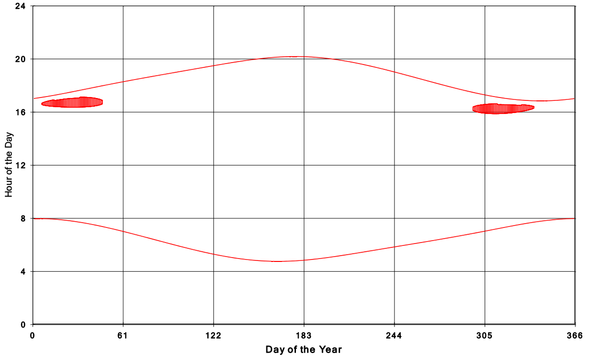
Goshen Wind Energy Centre Shadow Times on House 1402, All Windows from All Turbine
