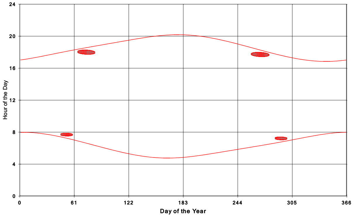
Goshen Wind Energy Centre Shadow Times on House 1456, All Windows from All Turbine
