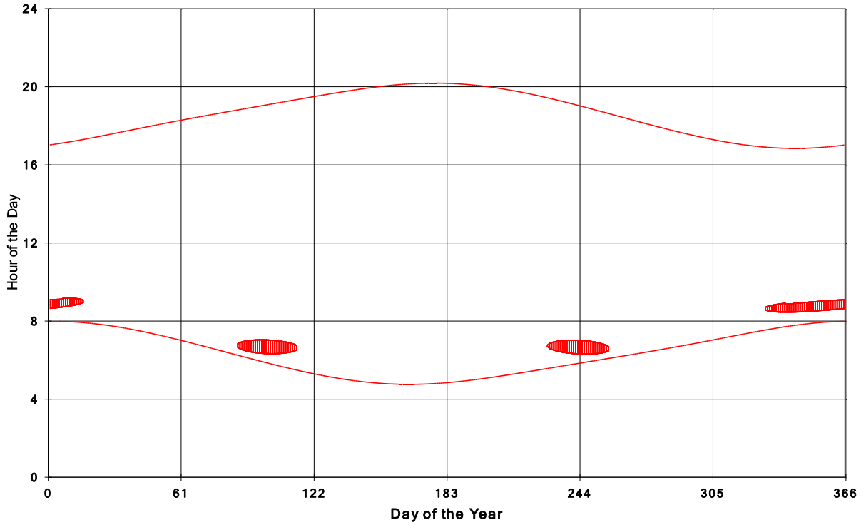
Goshen Wind Energy Centre Shadow Times on House 1500, All Windows from All Turbine
