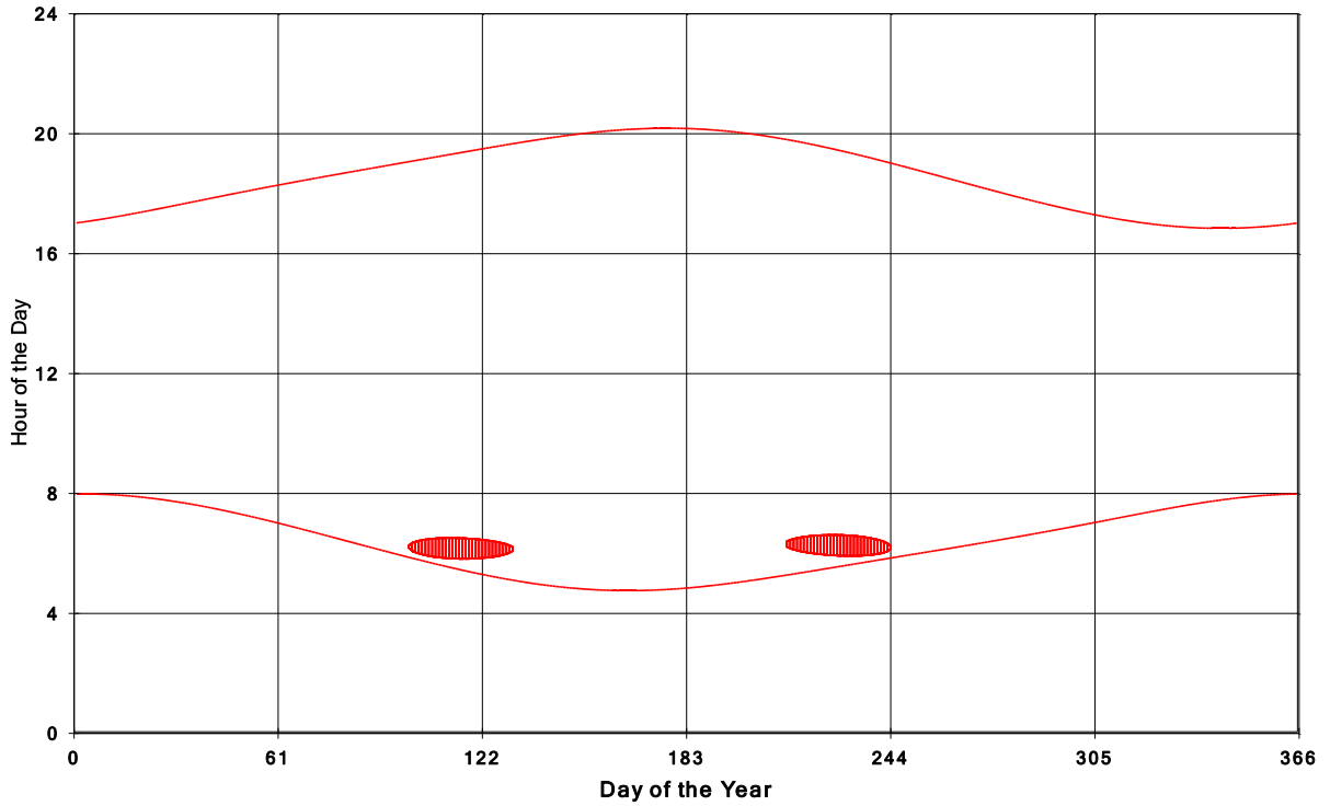
Goshen Wind Energy Centre Shadow Times on House 1330, All Windows from All Turbine
