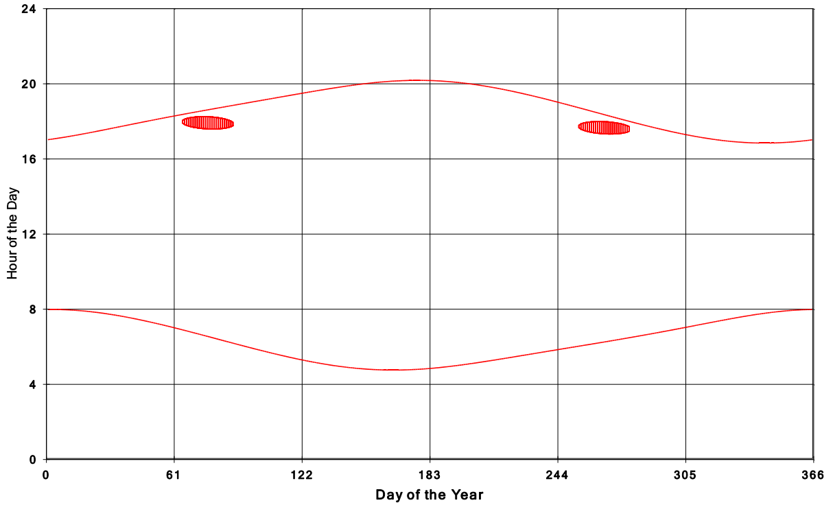
Goshen Wind Energy Centre Shadow Times on House 1453, All Windows from All Turbine
