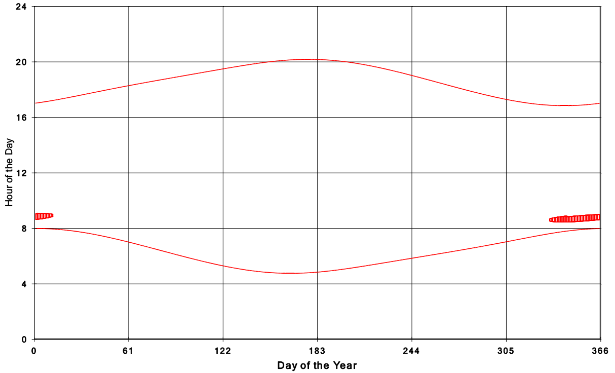
Goshen Wind Energy Centre Shadow Times on House 1430, All Windows from All Turbine
