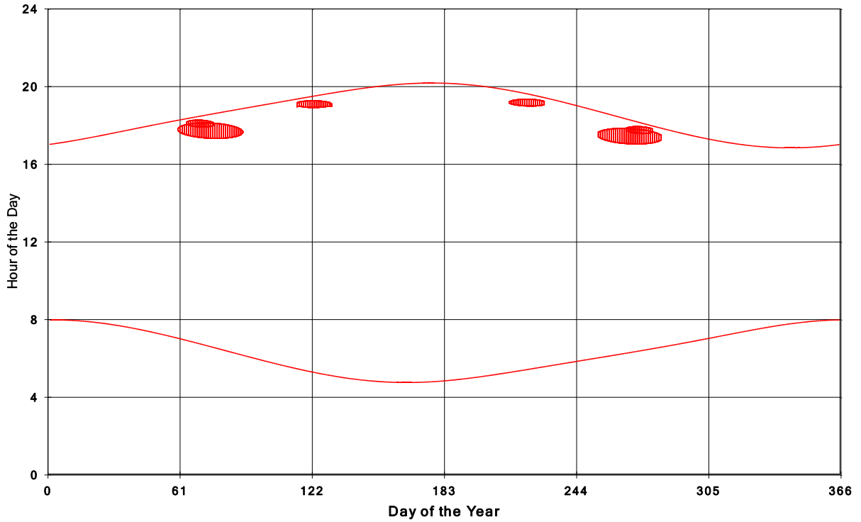
Goshen Wind Energy Centre Shadow Times on House 1442, All Windows from All Turbine
