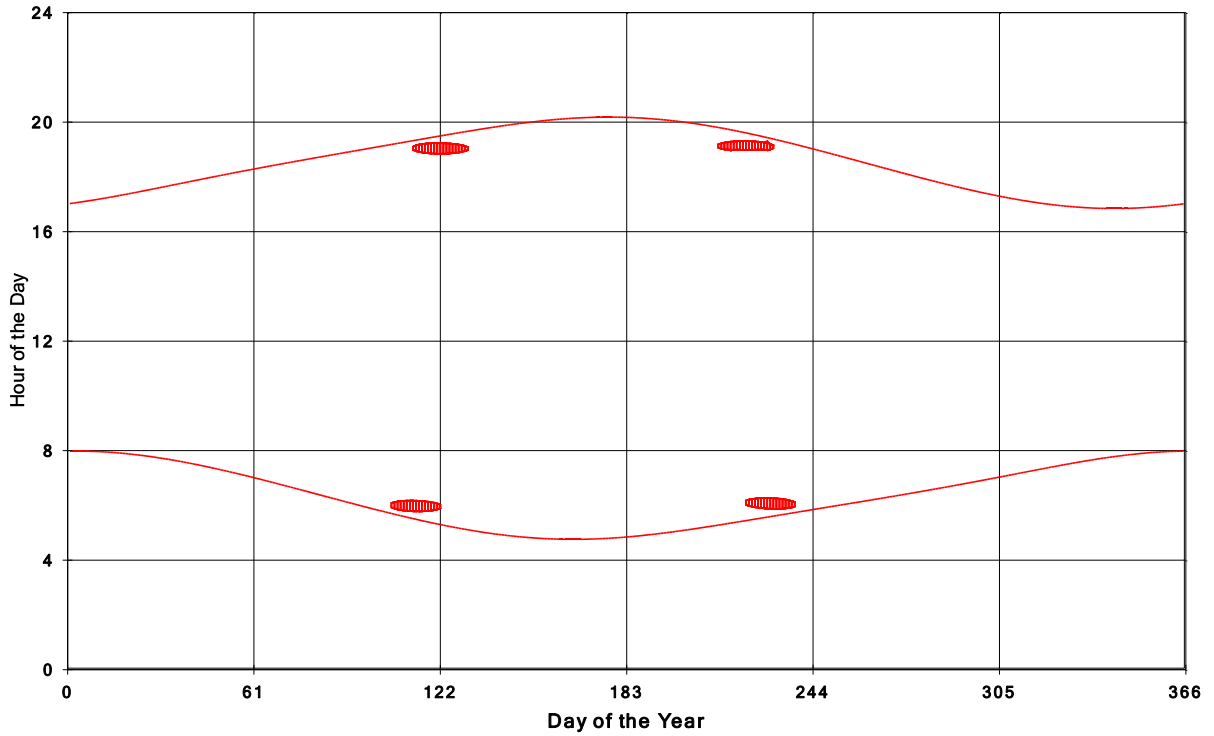
Goshen Wind Energy Centre Shadow Times on House 1346, All Windows from All Turbine
