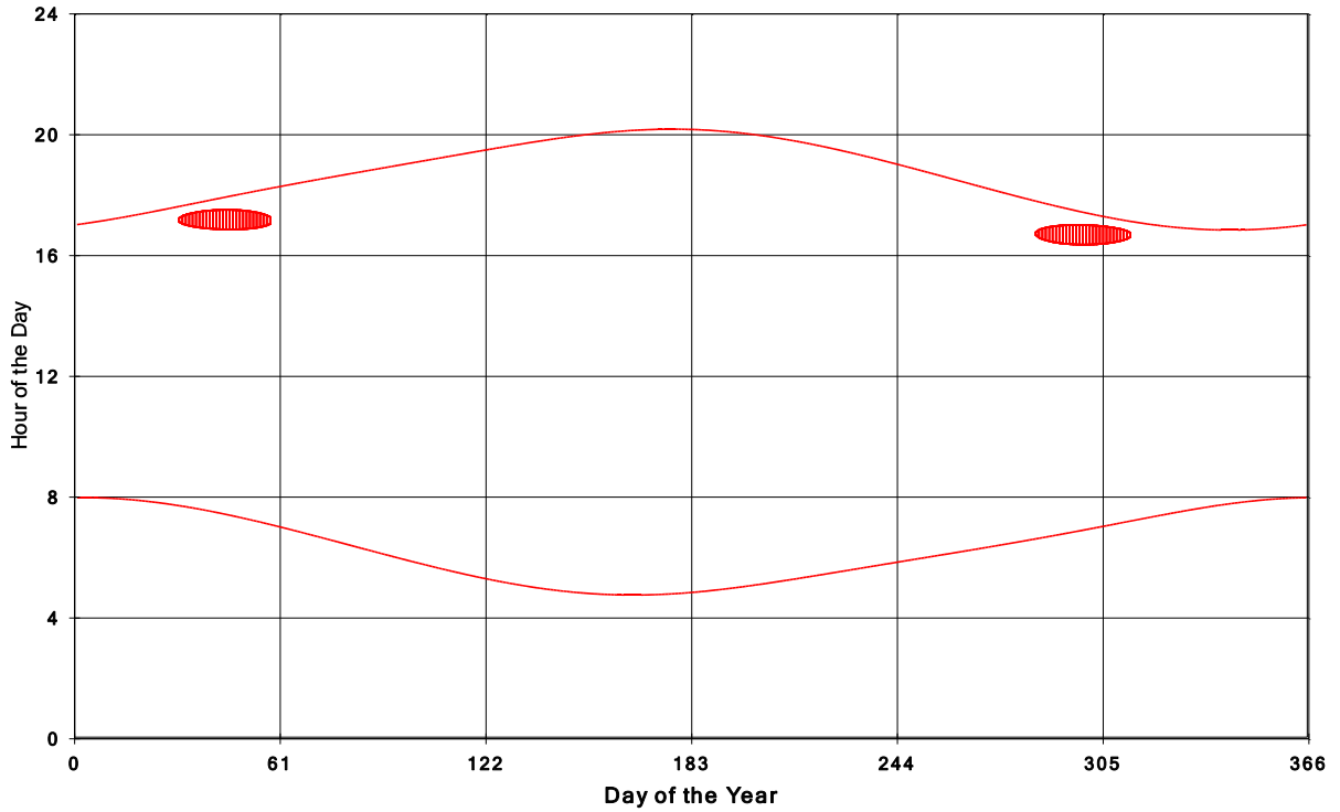
Goshen Wind Energy Centre Shadow Times on House 1336, All Windows from All Turbine
