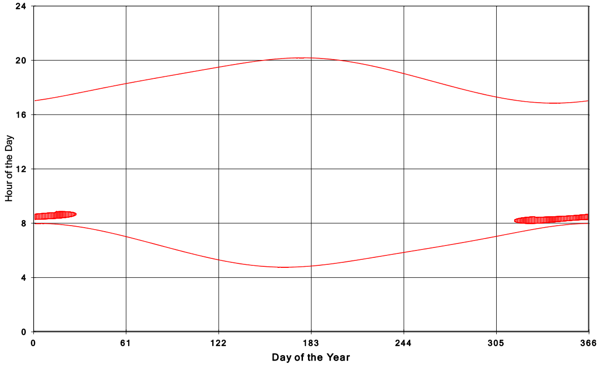
Goshen Wind Energy Centre Shadow Times on House 1452, All Windows from All Turbine
