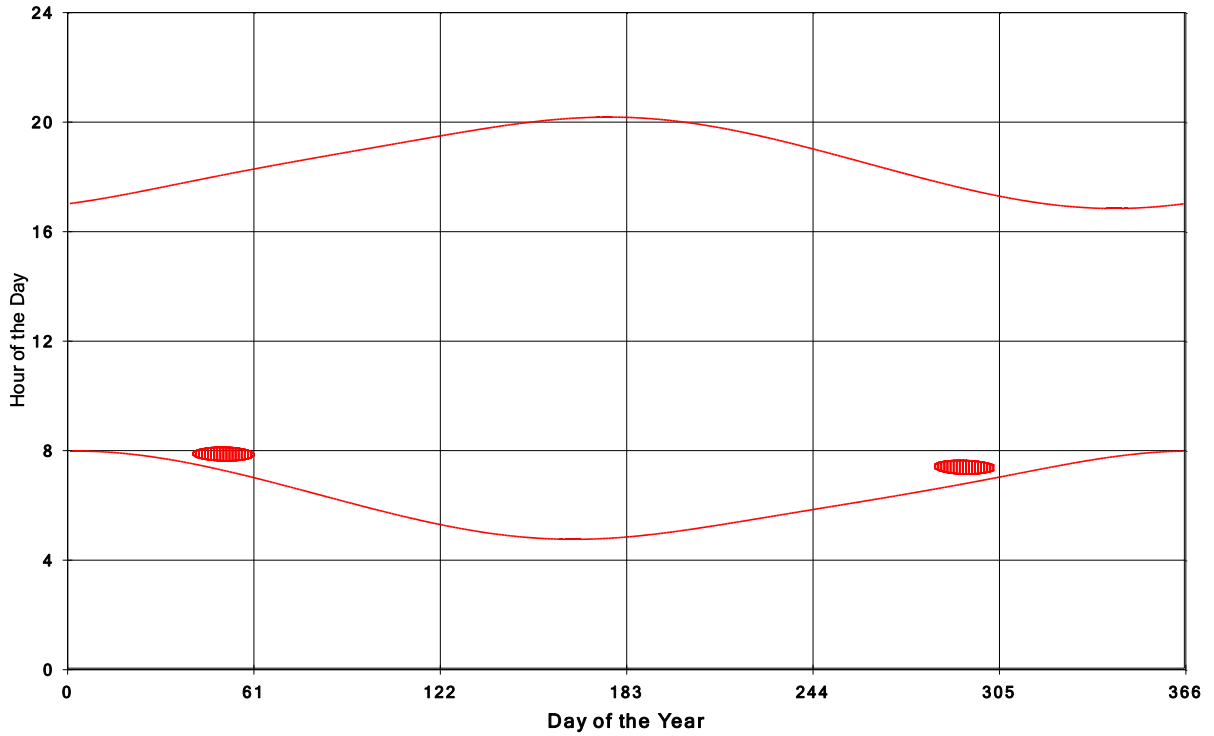
Goshen Wind Energy Centre Shadow Times on House 1446, All Windows from All Turbine
