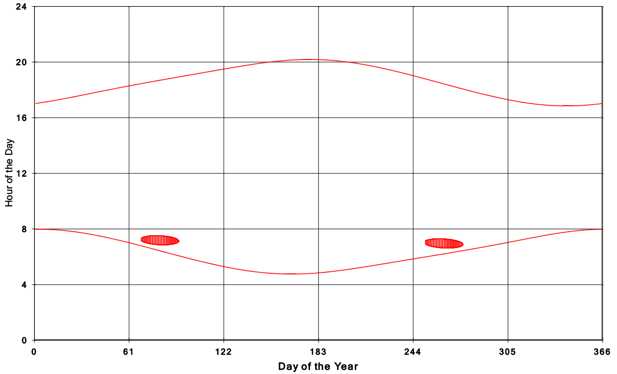
Goshen Wind Energy Centre Shadow Times on House 1342, All Windows from All Turbine
