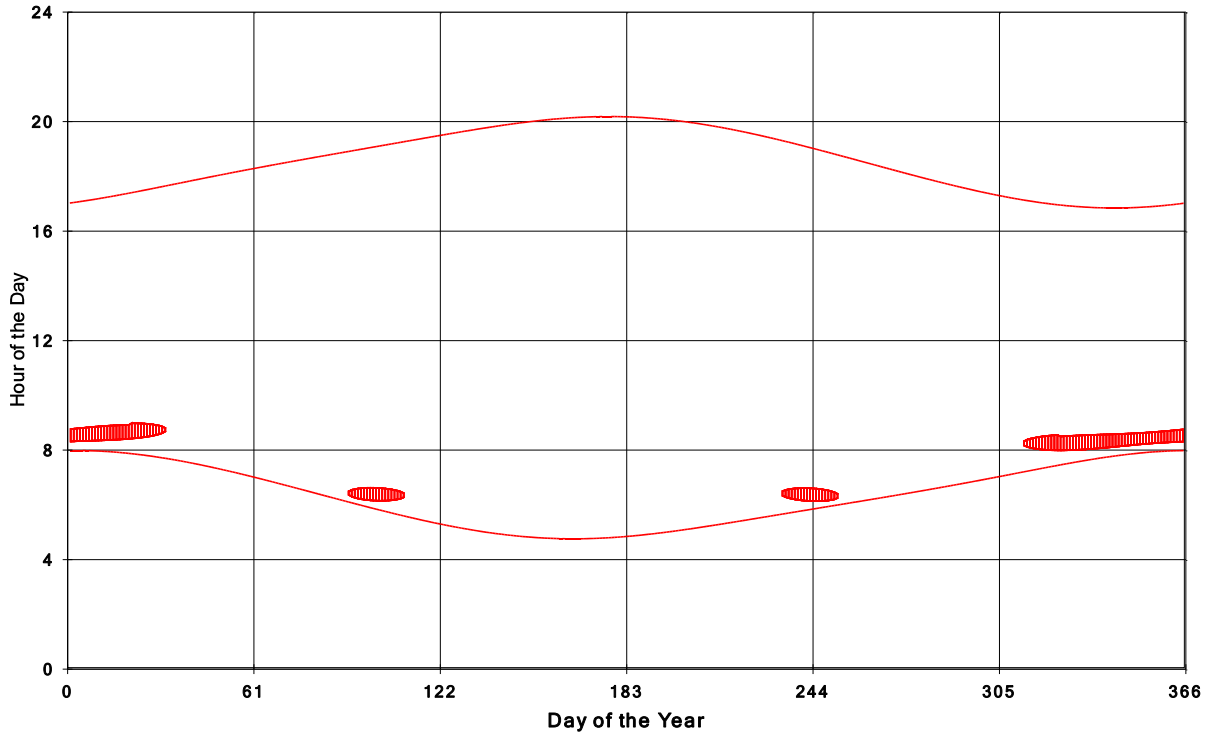
Goshen Wind Energy Centre Shadow Times on House 1459, All Windows from All Turbine
