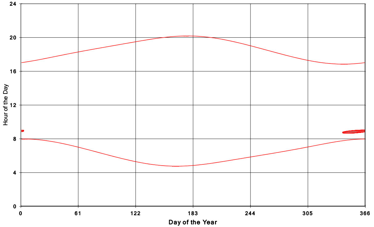
Goshen Wind Energy Centre Shadow Times on House 1419, All Windows from All Turbine
