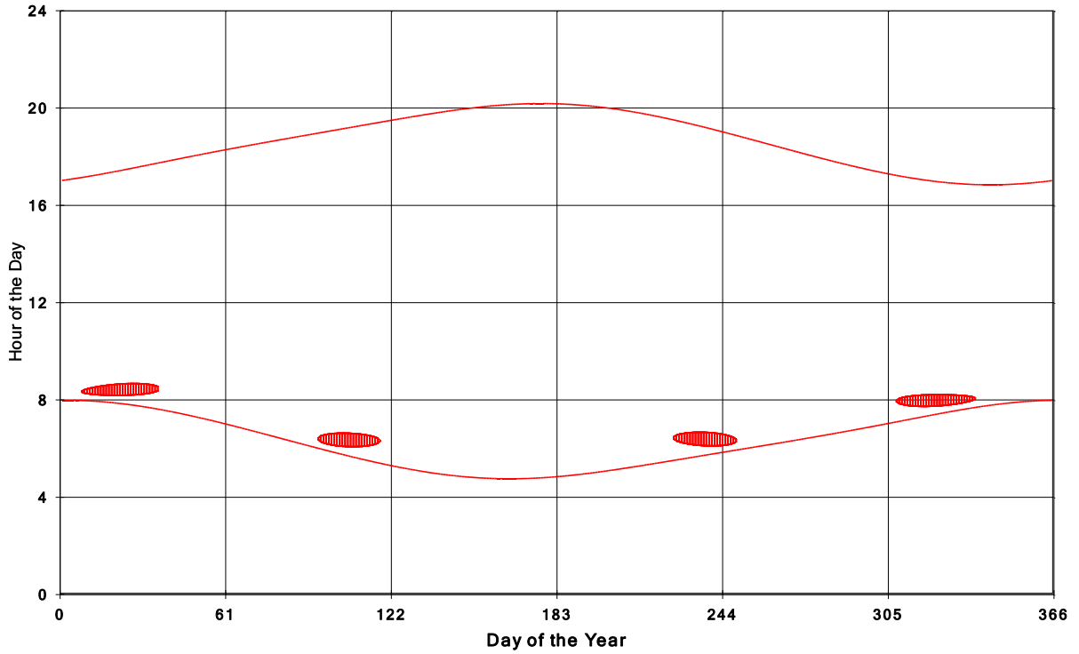
Goshen Wind Energy Centre Shadow Times on House 1450, All Windows from All Turbine
