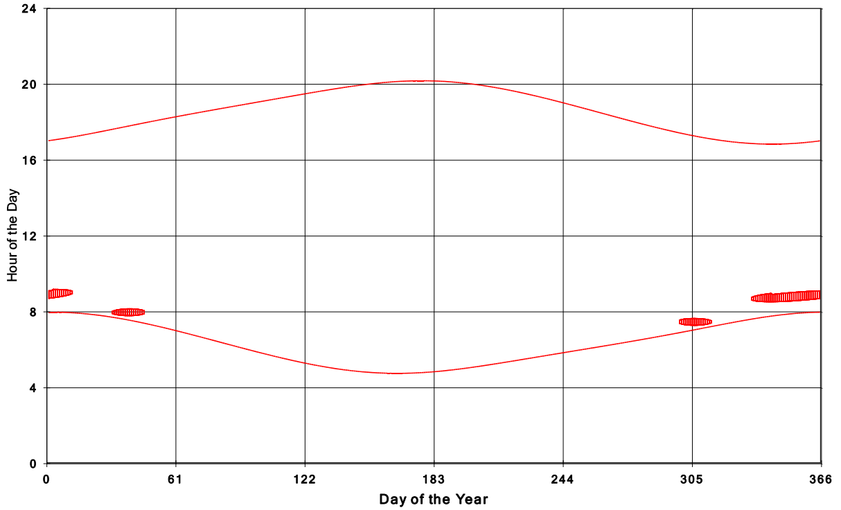
Goshen Wind Energy Centre Shadow Times on House 1482, All Windows from All Turbine
