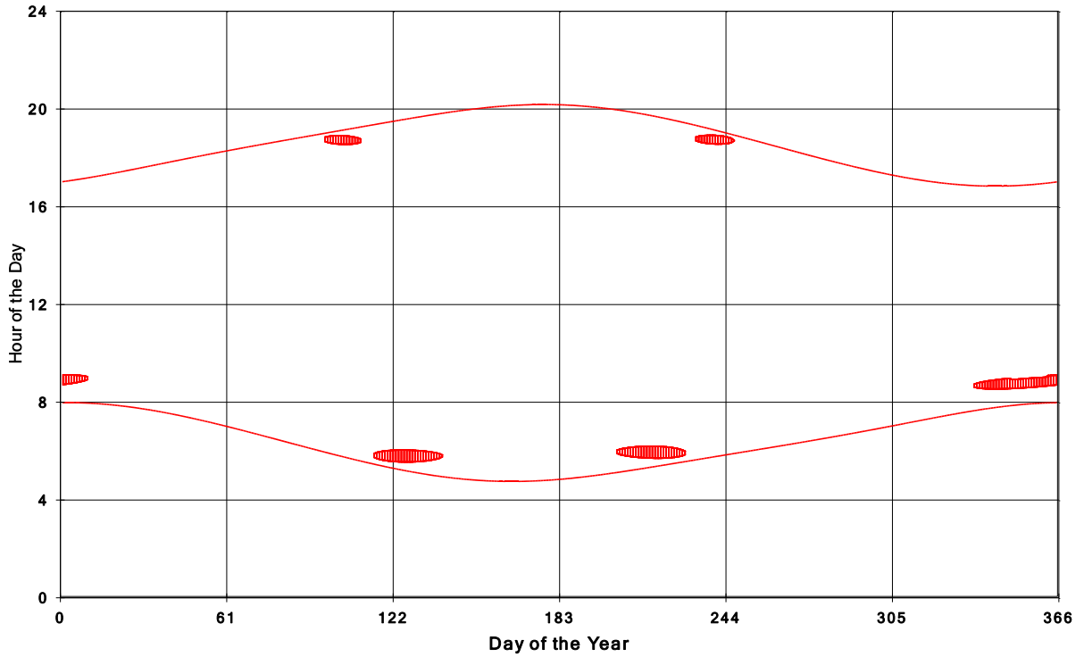
Goshen Wind Energy Centre Shadow Times on House 1507, All Windows from All Turbine
