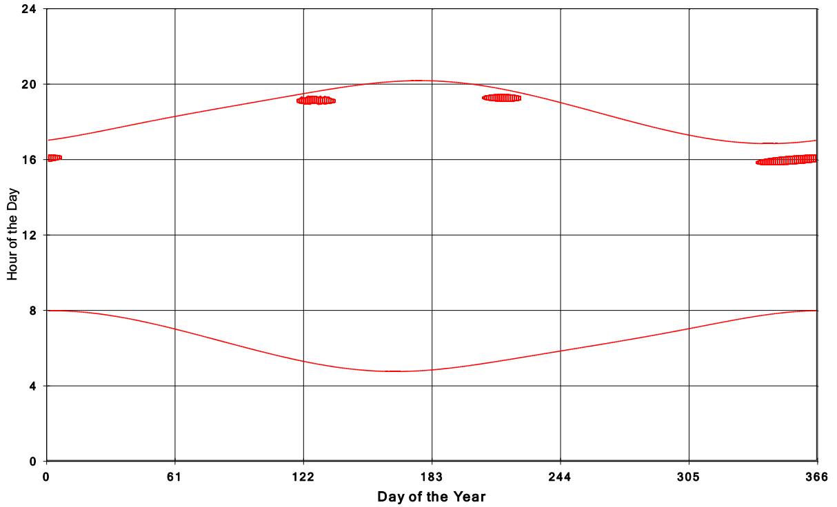
Goshen Wind Energy Centre Shadow Times on House 1492, All Windows from All Turbine
