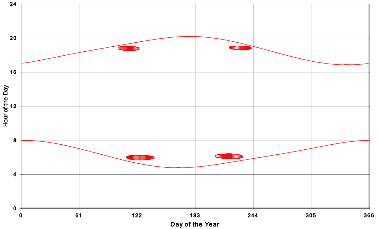
Goshen Wind Energy Centre Shadow Times on House 1444, All Windows from All Turbine
