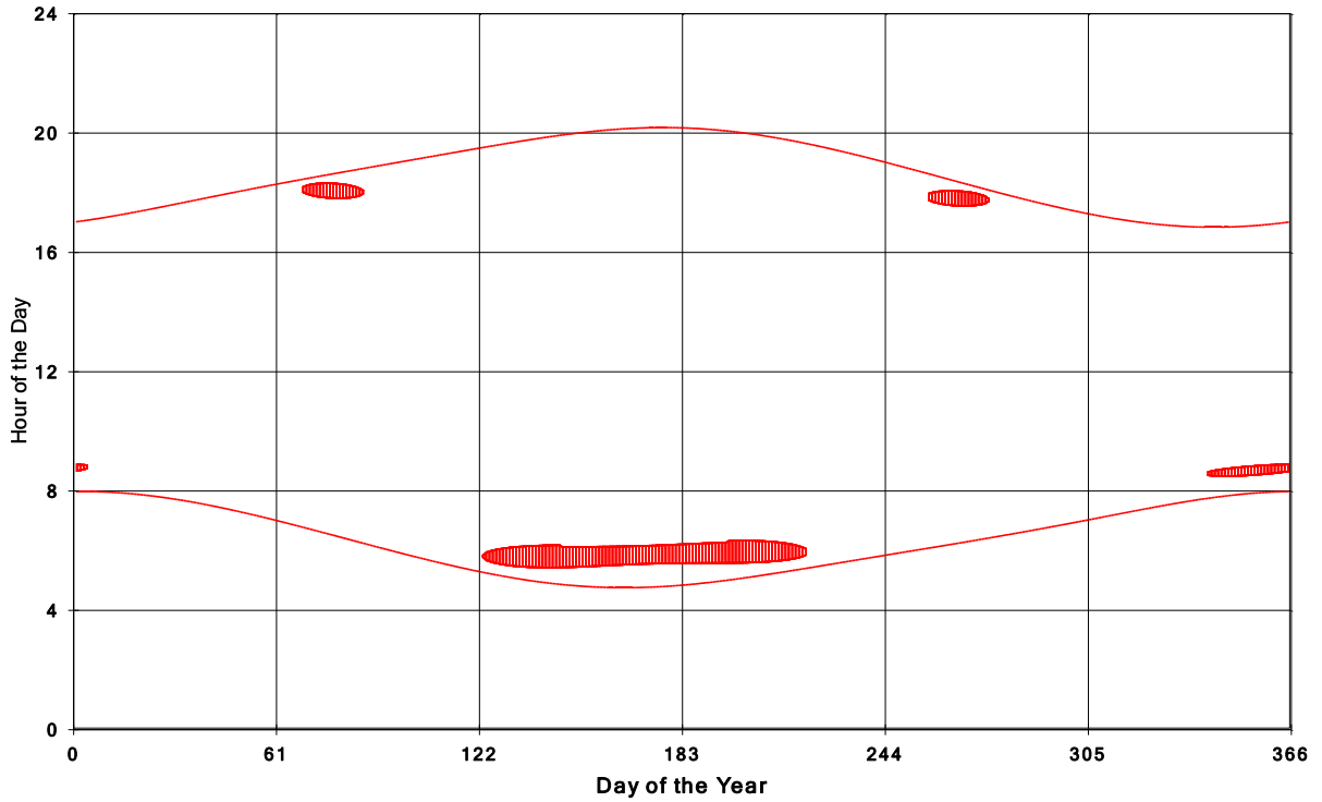
Goshen Wind Energy Centre Shadow Times on House 1364, All Windows from All Turbine
