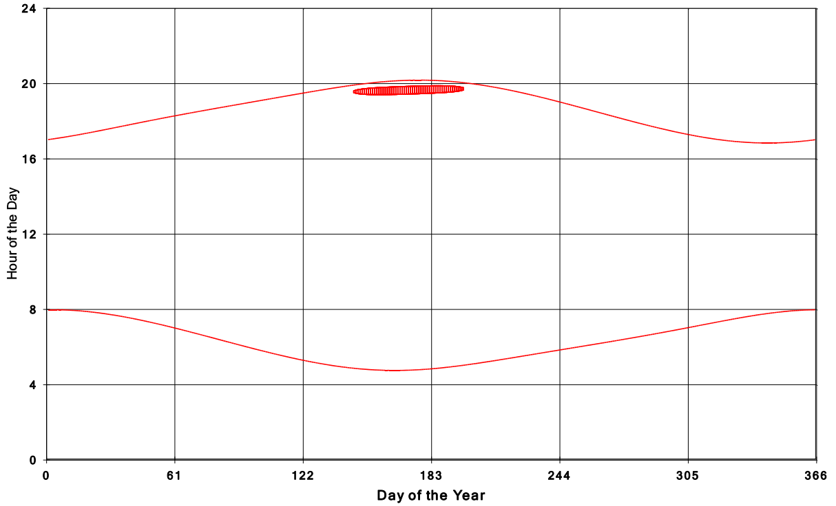
Goshen Wind Energy Centre Shadow Times on House 1341, All Windows from All Turbine
