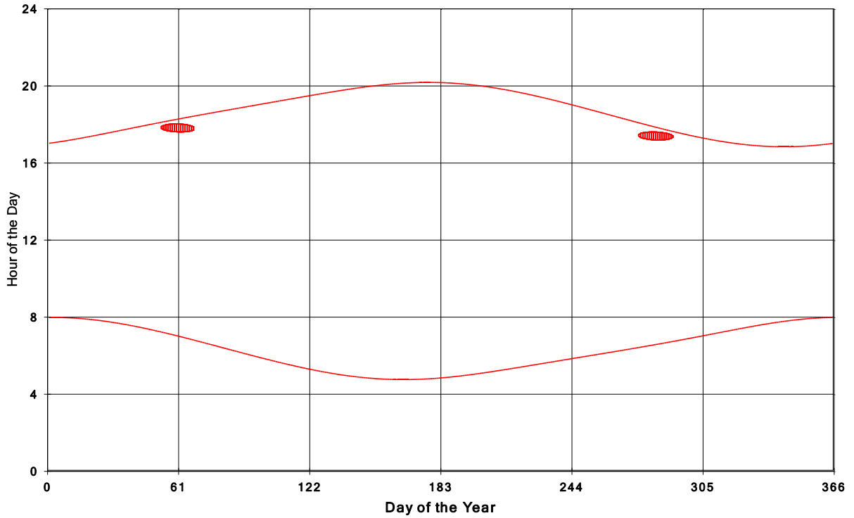
Goshen Wind Energy Centre Shadow Times on House 1483, All Windows from All Turbine
