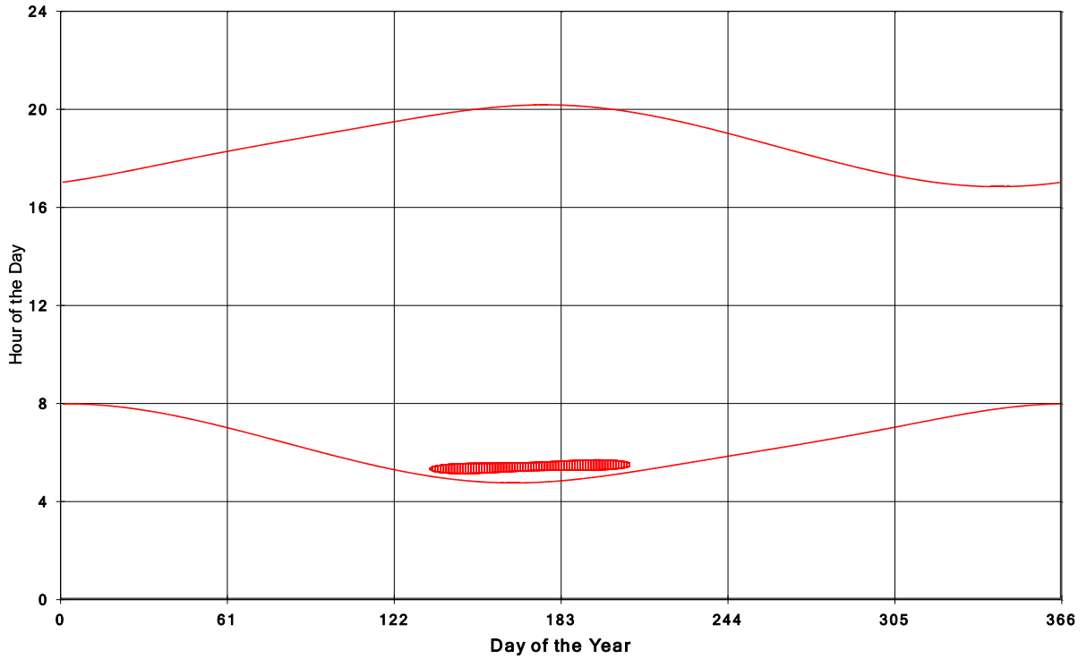
Goshen Wind Energy Centre Shadow Times on House 1458, All Windows from All Turbine
