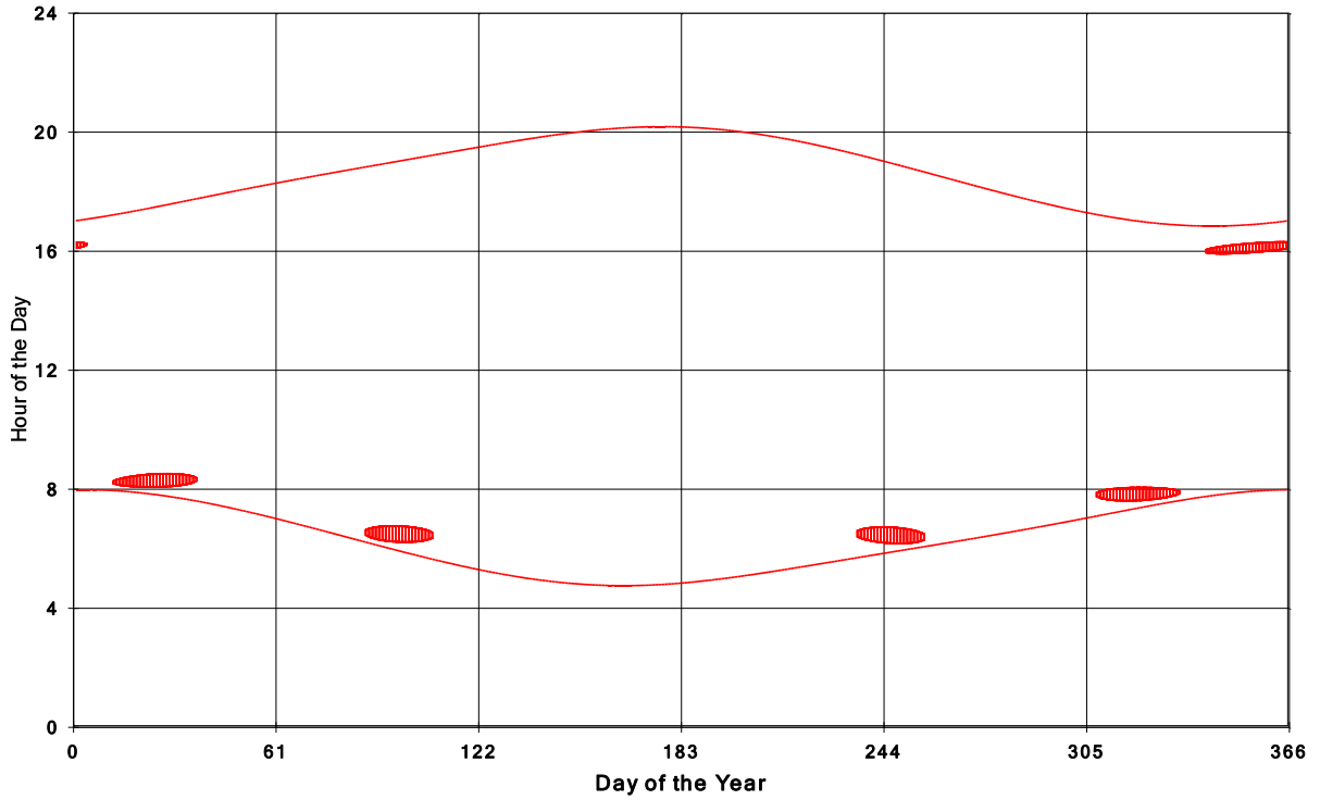
Goshen Wind Energy Centre Shadow Times on House 1370, All Windows from All Turbine
