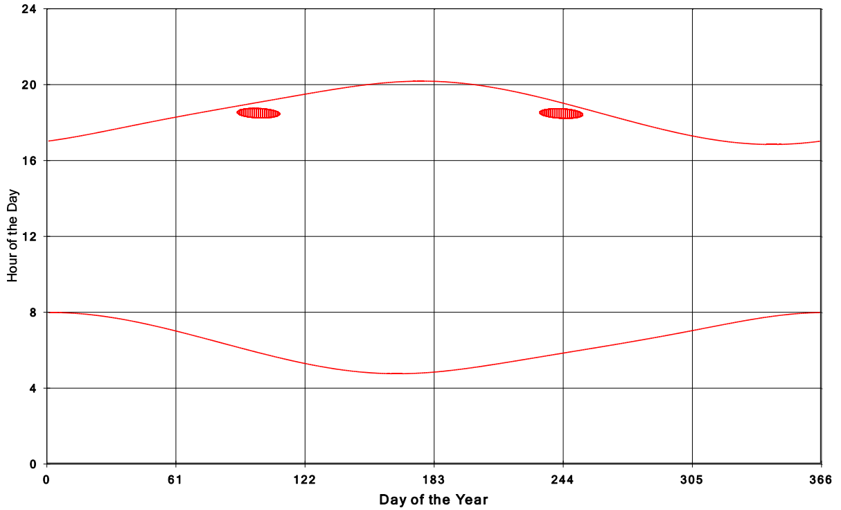
Goshen Wind Energy Centre Shadow Times on House 1349, All Windows from All Turbine
