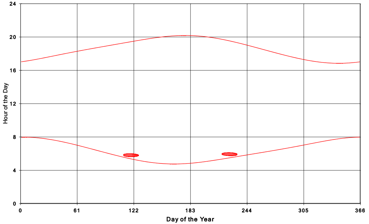
Goshen Wind Energy Centre Shadow Times on House 1344, All Windows from All Turbine
