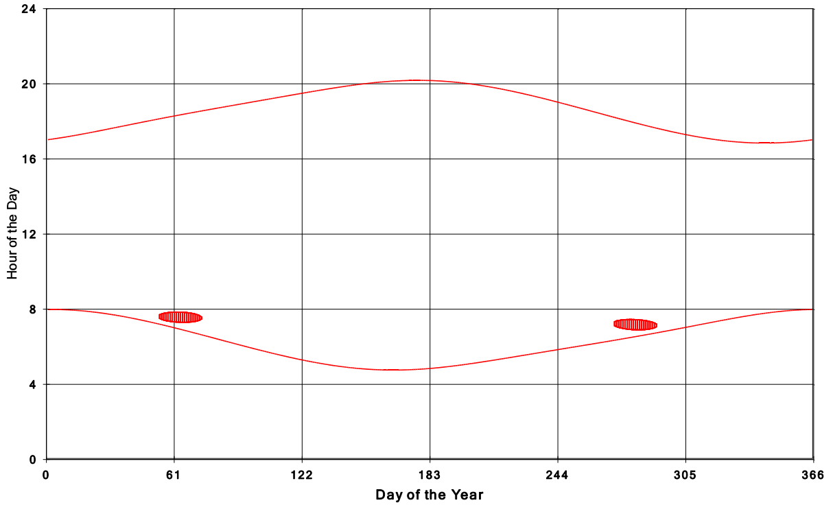
Goshen Wind Energy Centre Shadow Times on House 1503, All Windows from All Turbine
