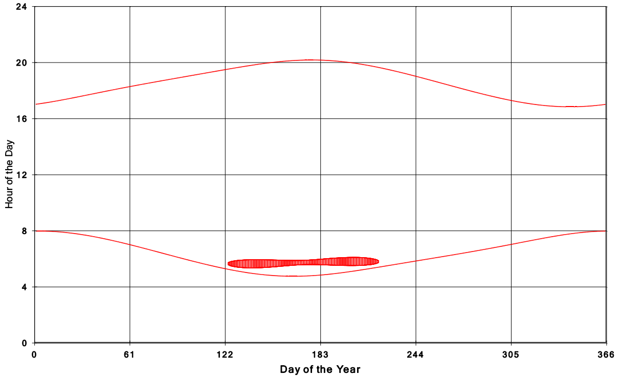
Goshen Wind Energy Centre Shadow Times on House 1499, All Windows from All Turbine
