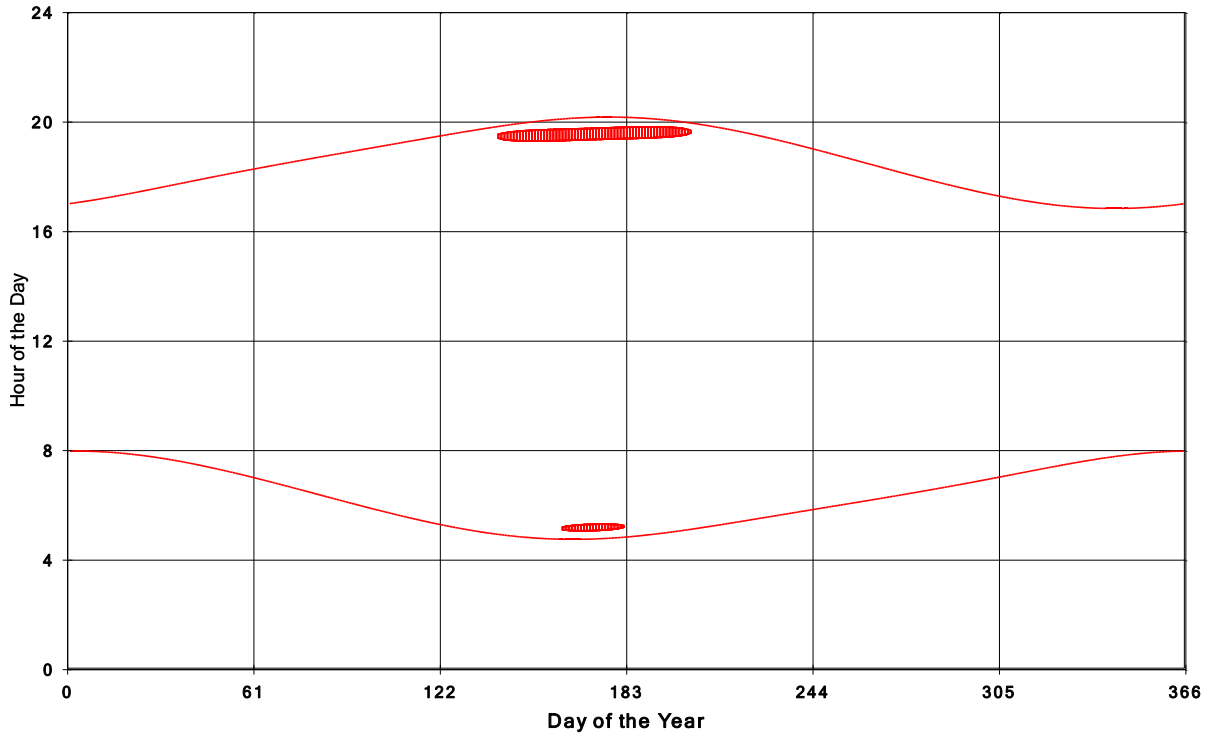
Goshen Wind Energy Centre Shadow Times on House 1340, All Windows from All Turbine
