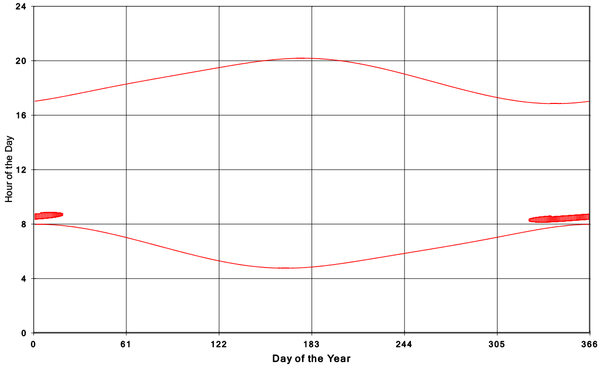
Goshen Wind Energy Centre Shadow Times on House 1418, All Windows from All Turbine
