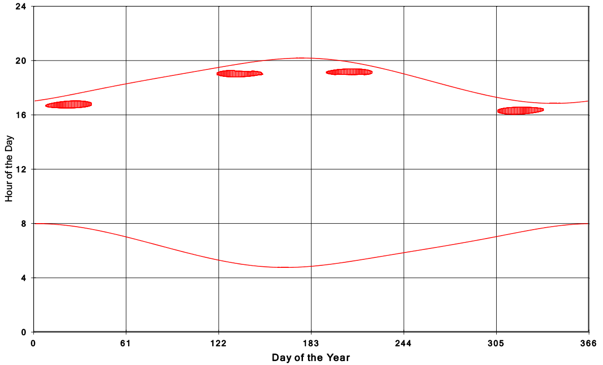
Goshen Wind Energy Centre Shadow Times on House 1427, All Windows from All Turbine
