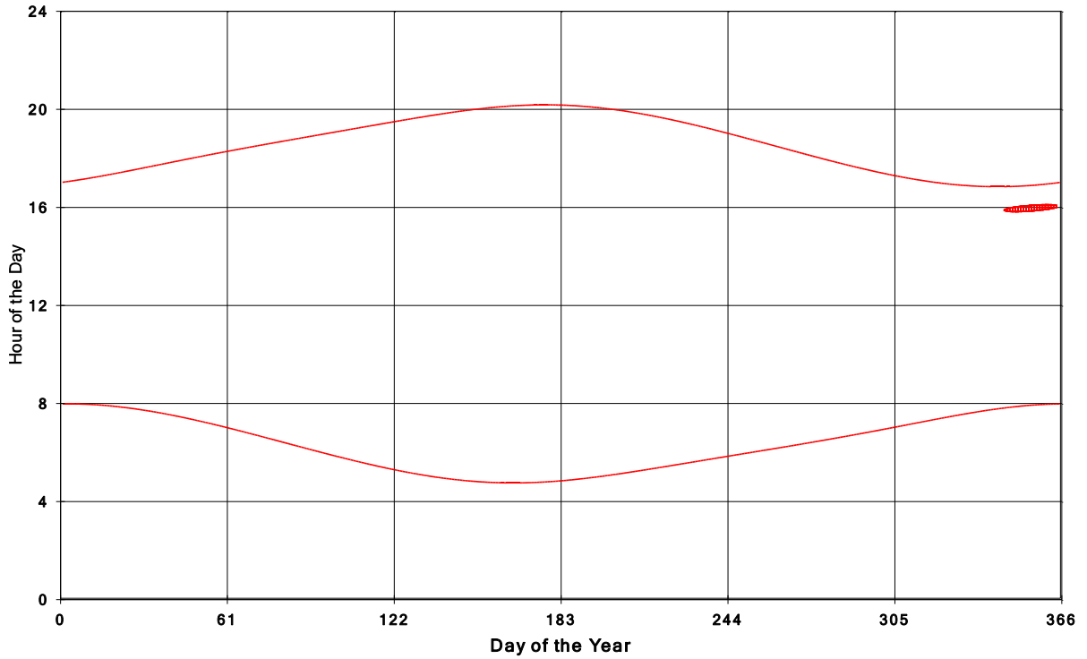
Goshen Wind Energy Centre Shadow Times on House 1407, All Windows from All Turbine
