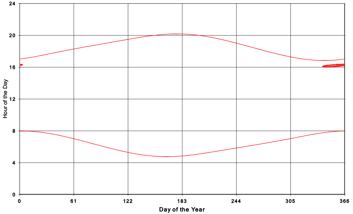
Goshen Wind Energy Centre Shadow Times on House 1411, All Windows from All Turbine
