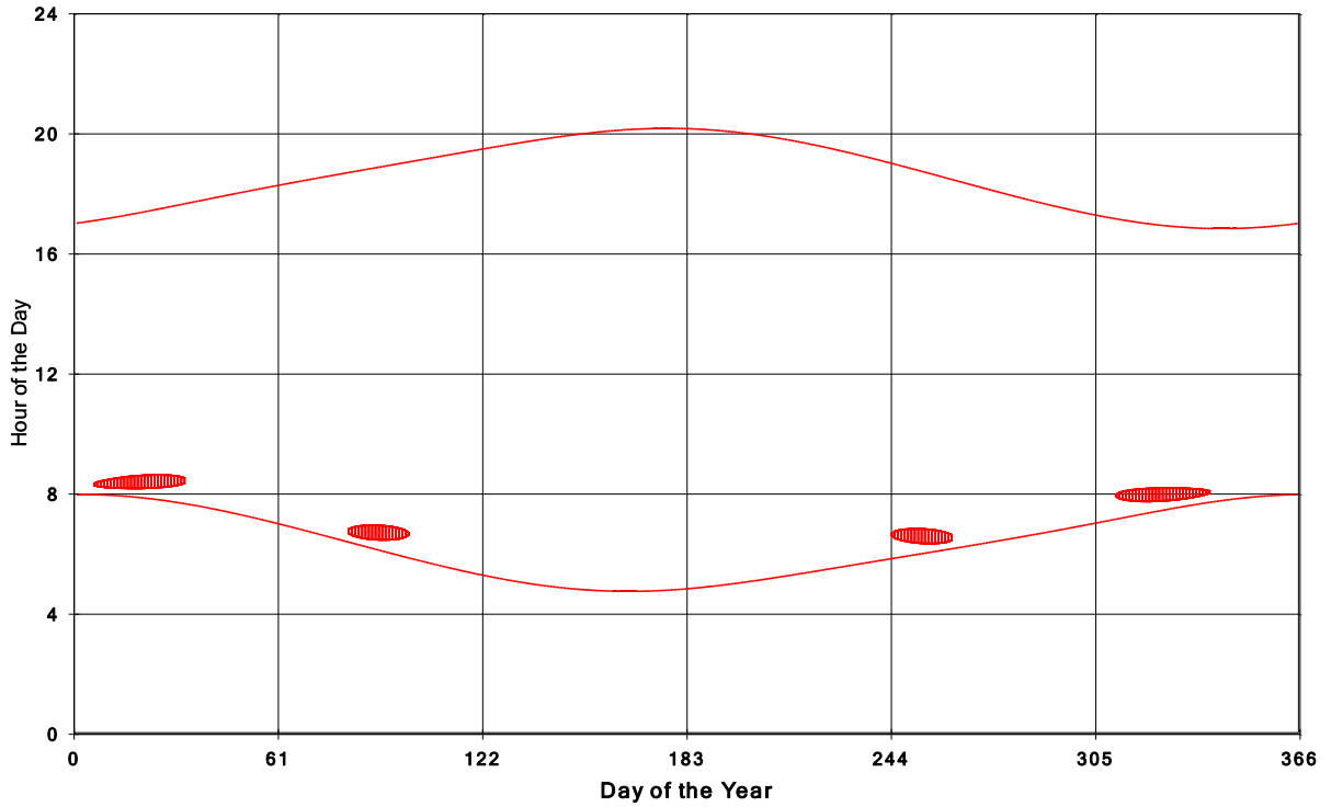
Goshen Wind Energy Centre Shadow Times on House 1501, All Windows from All Turbine
