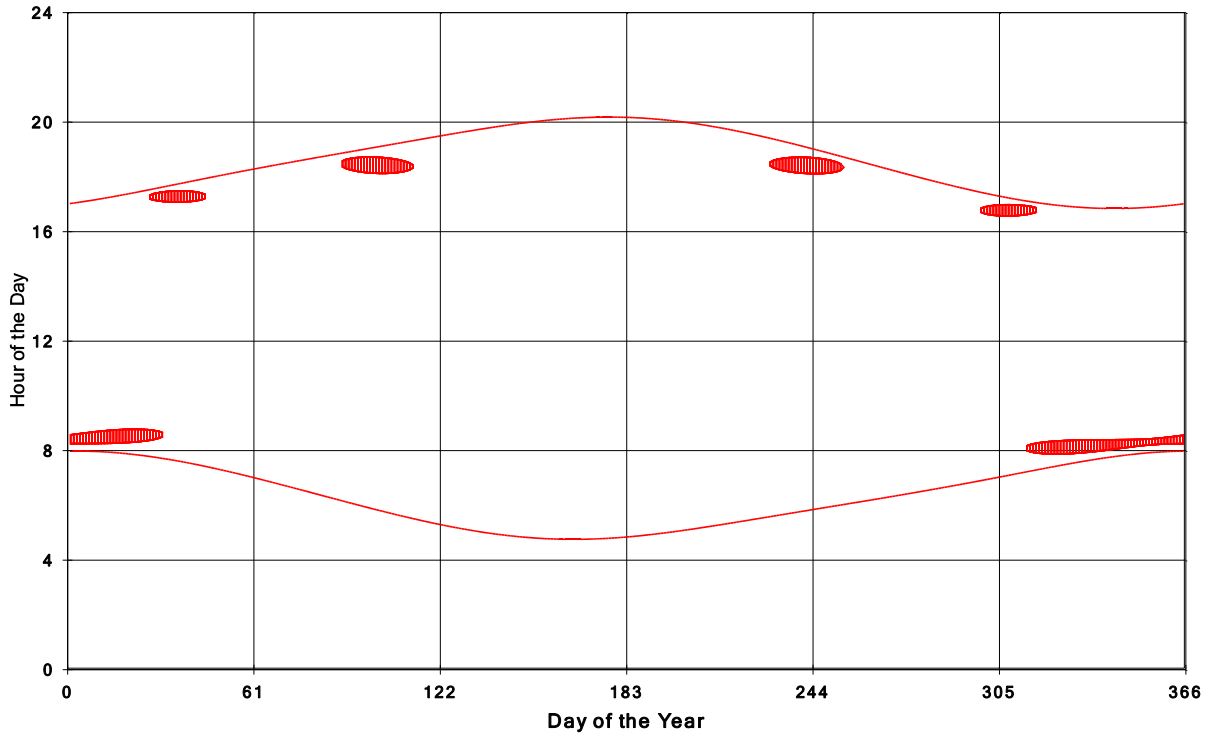
Goshen Wind Energy Centre Shadow Times on House 1338, All Windows from All Turbine
