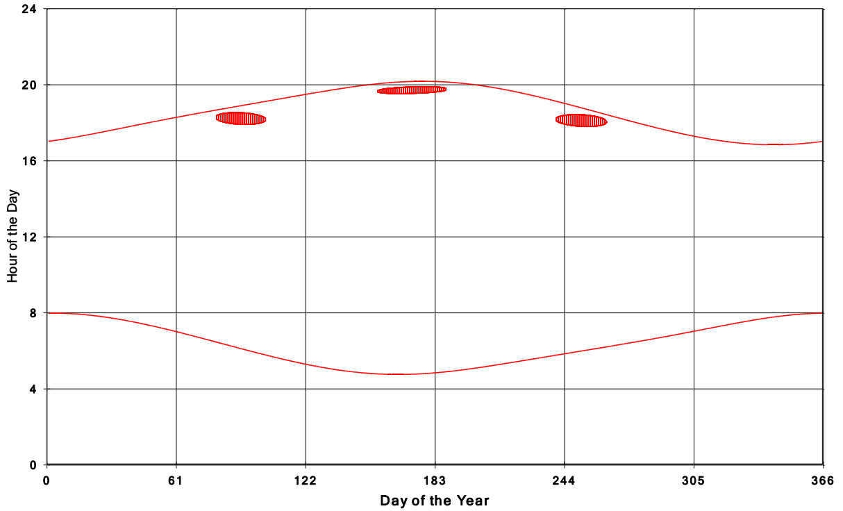
Goshen Wind Energy Centre Shadow Times on House 1449, All Windows from All Turbine
