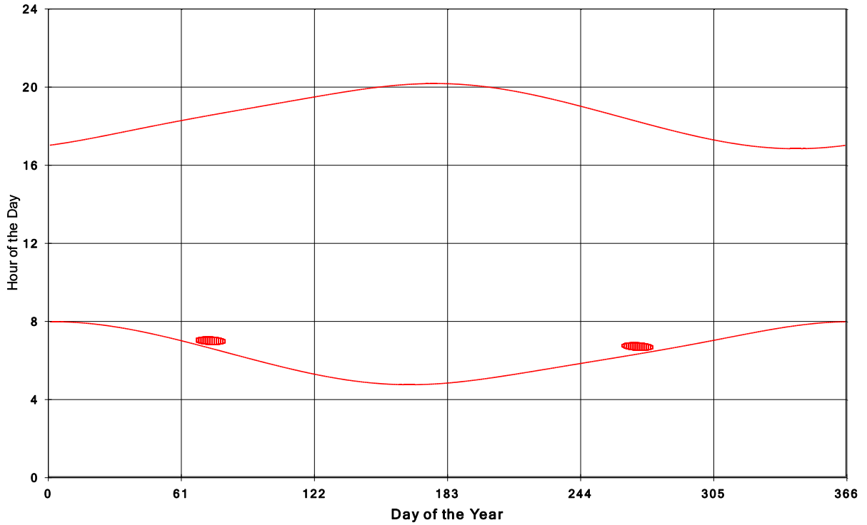
Goshen Wind Energy Centre Shadow Times on House 1333, All Windows from All Turbine
