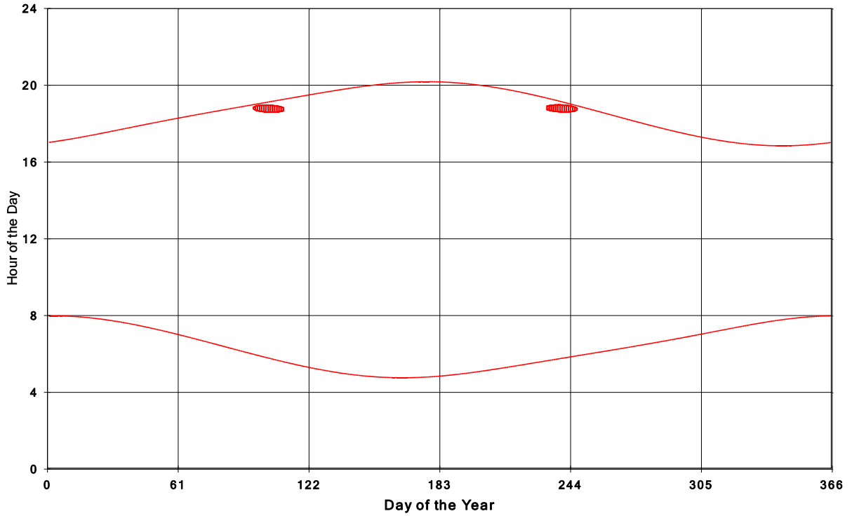
Goshen Wind Energy Centre Shadow Times on House 1362, All Windows from All Turbine
