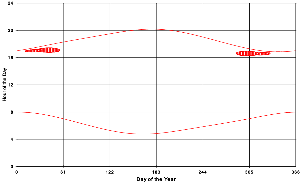
Goshen Wind Energy Centre Shadow Times on House 1355, All Windows from All Turbine
