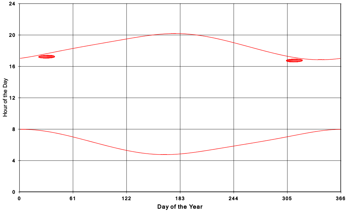
Goshen Wind Energy Centre Shadow Times on House 1488, All Windows from All Turbine
