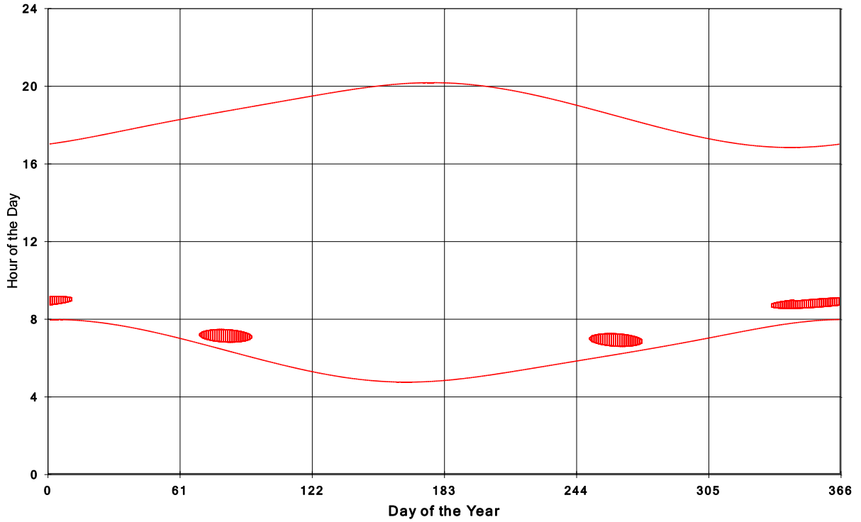
Goshen Wind Energy Centre Shadow Times on House 1504, All Windows from All Turbine
