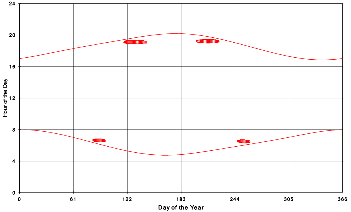
Goshen Wind Energy Centre Shadow Times on House 1493, All Windows from All Turbine
