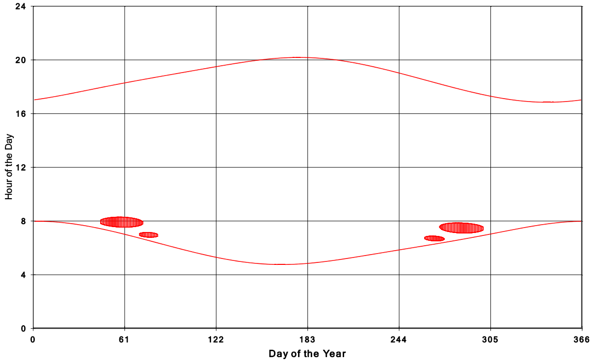
Goshen Wind Energy Centre Shadow Times on House 1360, All Windows from All Turbine
