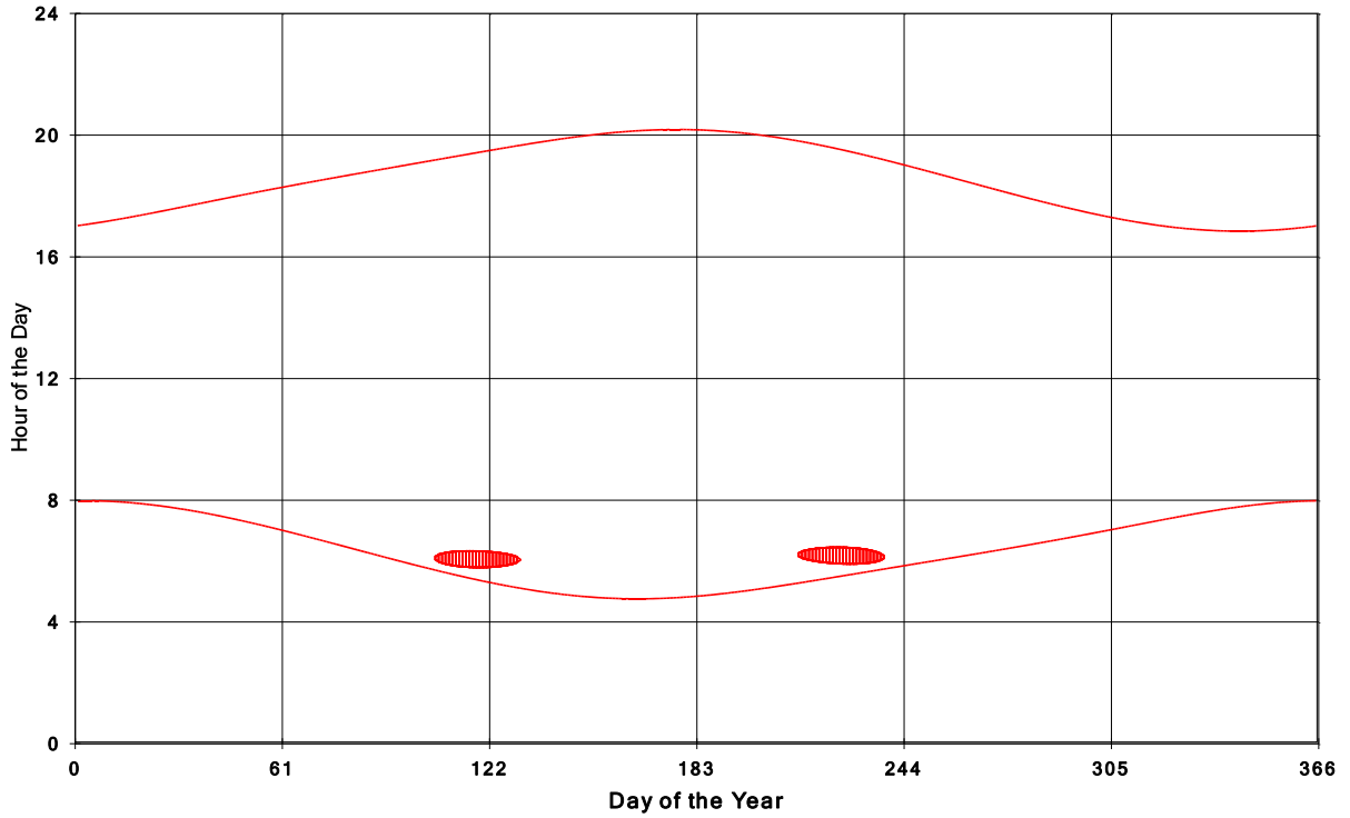
Goshen Wind Energy Centre Shadow Times on House 1432, All Windows from All Turbine
