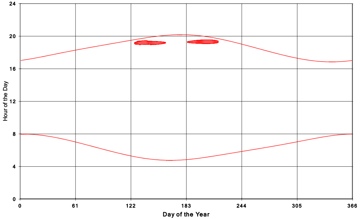
Goshen Wind Energy Centre Shadow Times on House 1356, All Windows from All Turbine
