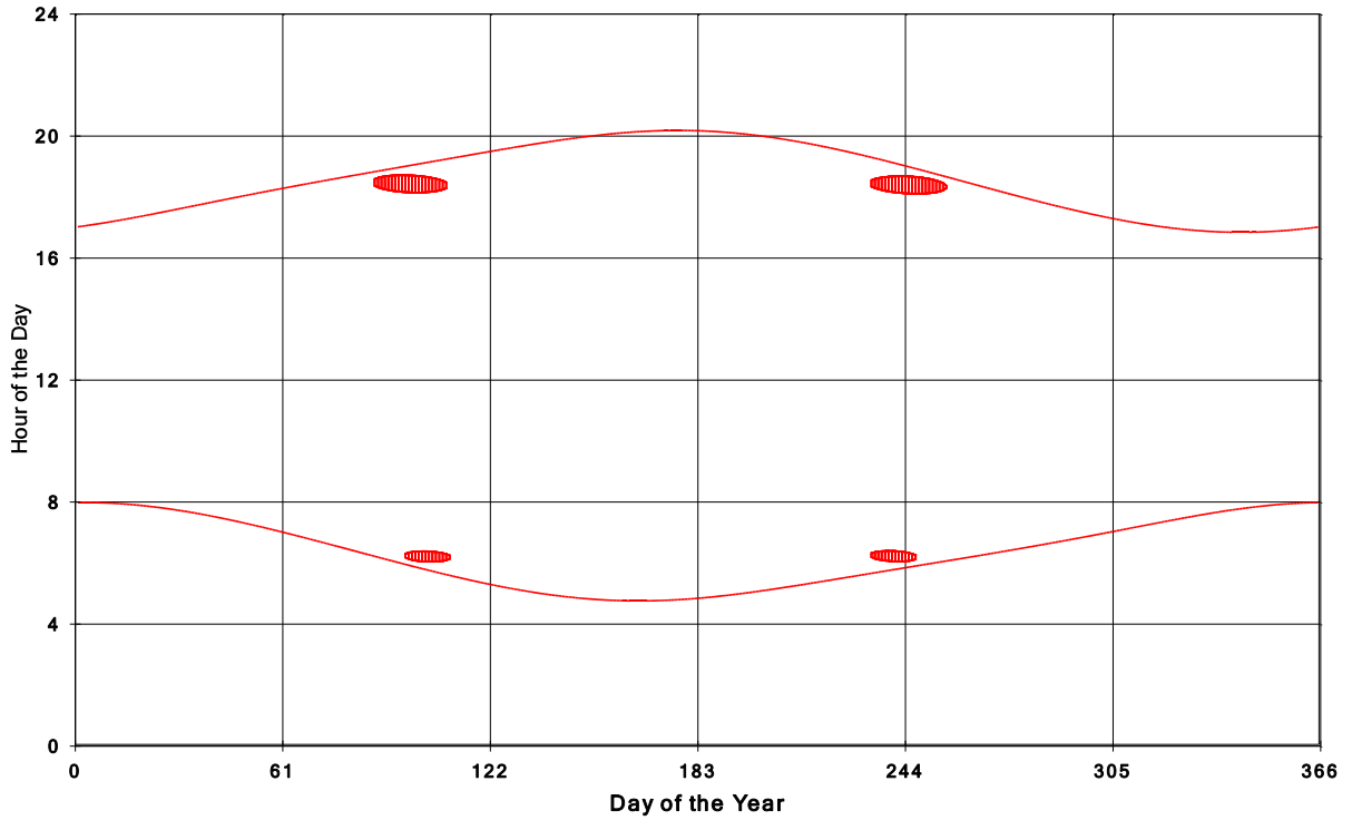
Goshen Wind Energy Centre Shadow Times on House 1368, All Windows from All Turbine
