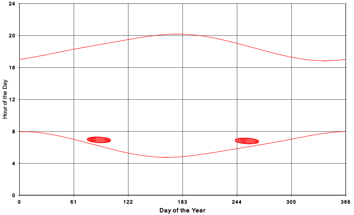
Jericho Wind Energy Centre Shadow Times on House 1484, All Windows from All Turbine
