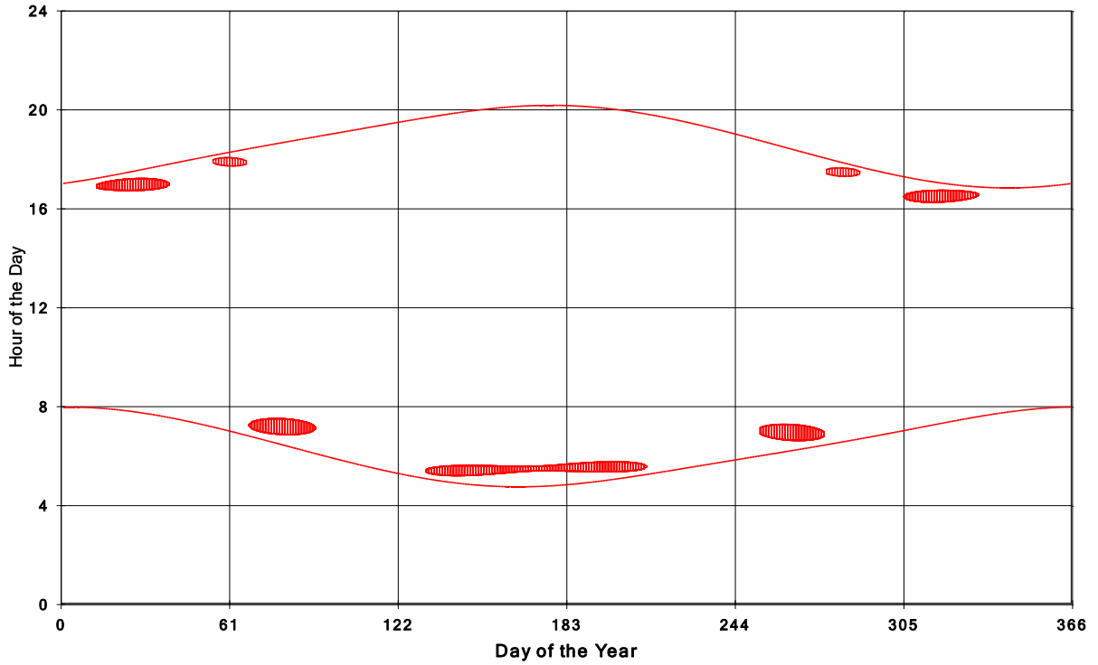
Goshen Wind Energy Centre Shadow Times on House 1489, All Windows from All Turbine
