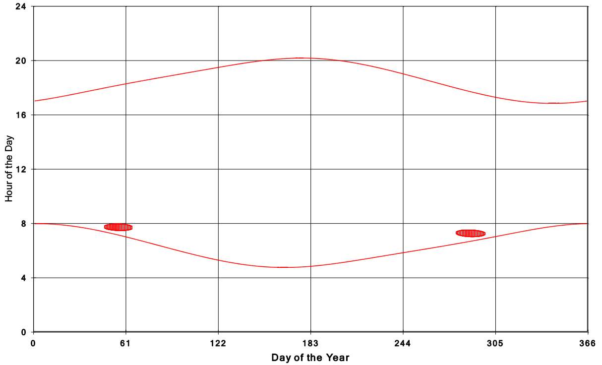
Goshen Wind Energy Centre Shadow Times on House 1420, All Windows from All Turbine
