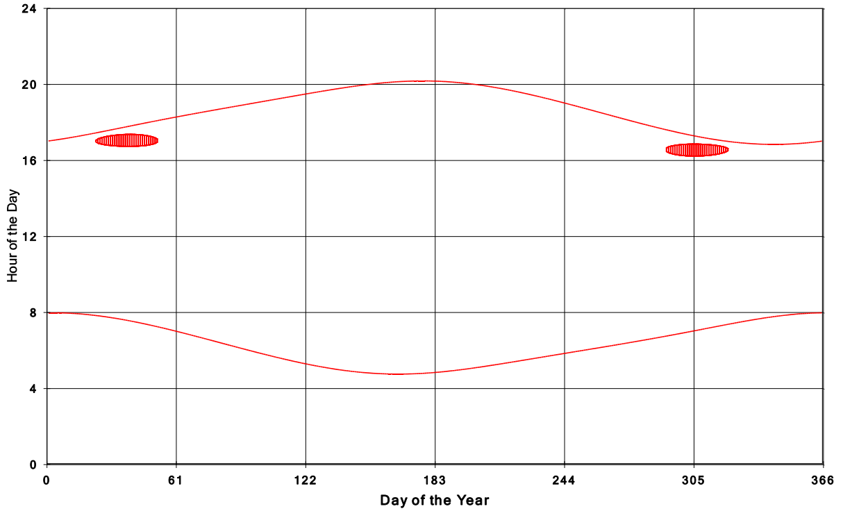
Goshen Wind Energy Centre Shadow Times on House 1337, All Windows from All Turbine
