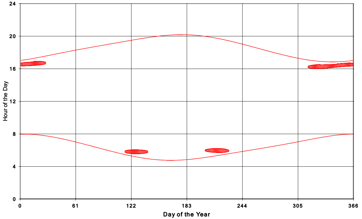
Goshen Wind Energy Centre Shadow Times on House 1366, All Windows from All Turbine
