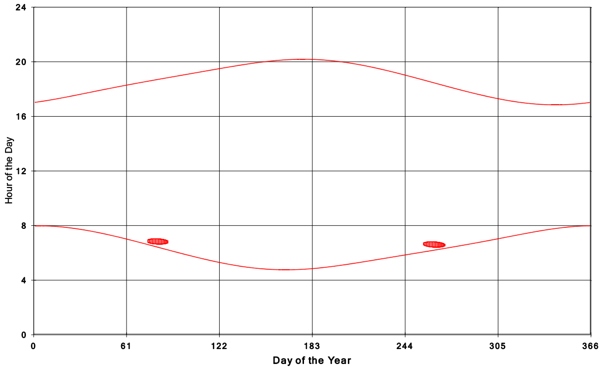
Goshen Wind Energy Centre Shadow Times on House 1485, All Windows from All Turbine
