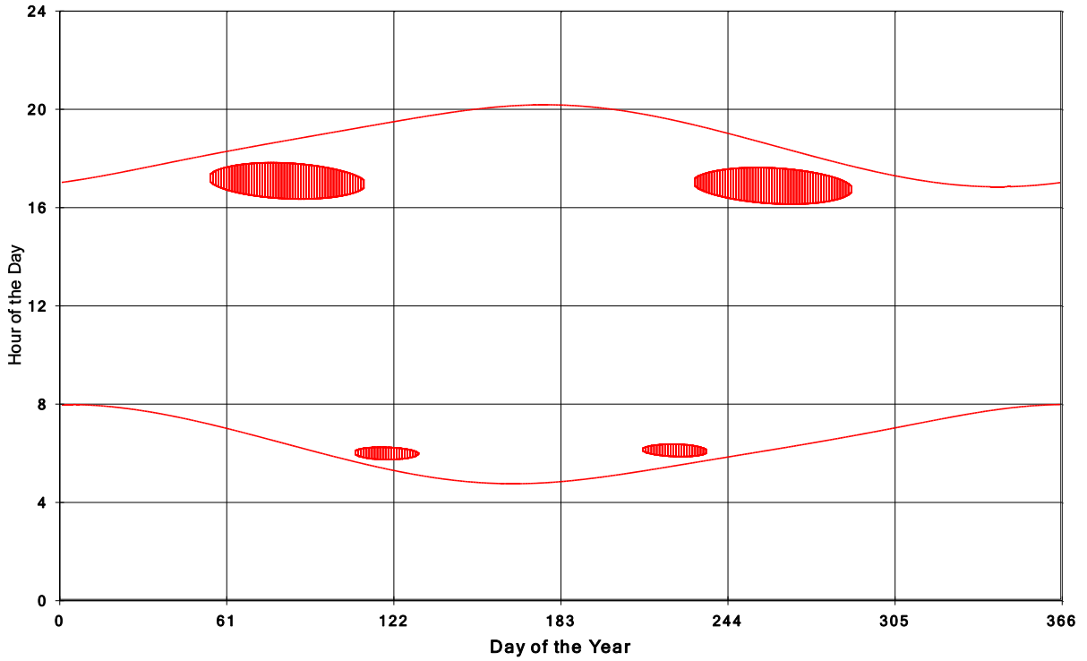
Jericho Wind Energy Centre Shadow Times on House 1455, All Windows from All Turbine
