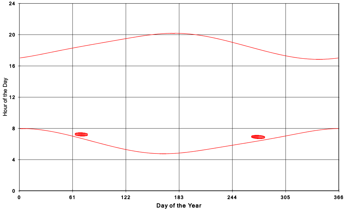
Goshen Wind Energy Centre Shadow Times on House 1448, All Windows from All Turbine
