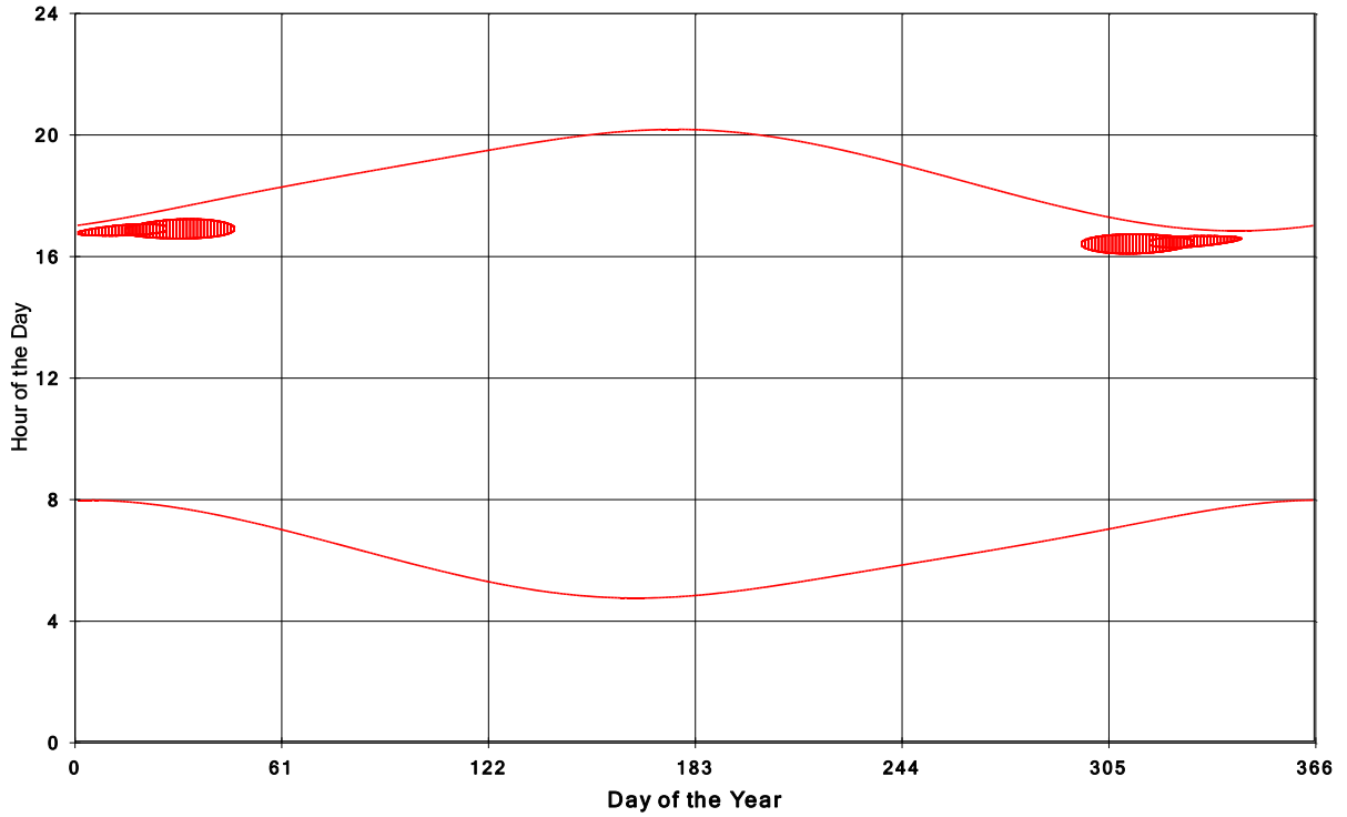
Goshen Wind Energy Centre Shadow Times on House 1354, All Windows from All Turbine
