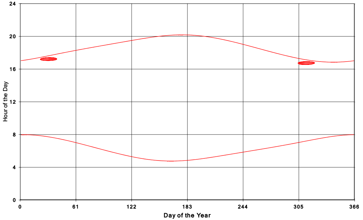
Goshen Wind Energy Centre Shadow Times on House 1439, All Windows from All Turbine
