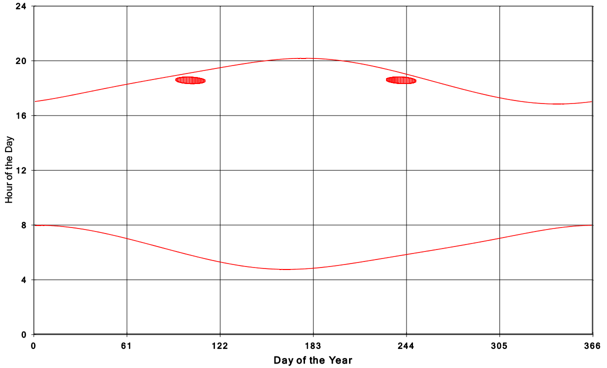
Goshen Wind Energy Centre Shadow Times on House 1348, All Windows from All Turbine
