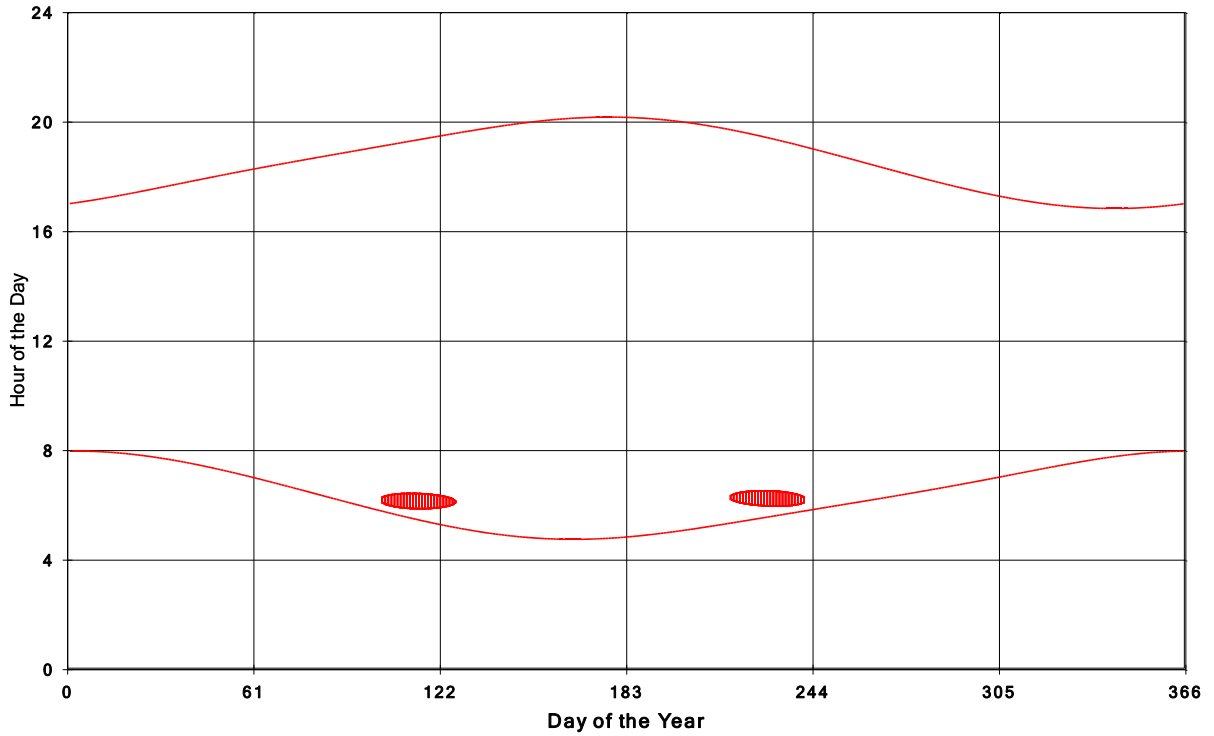
Goshen Wind Energy Centre Shadow Times on House 1433, All Windows from All Turbine
