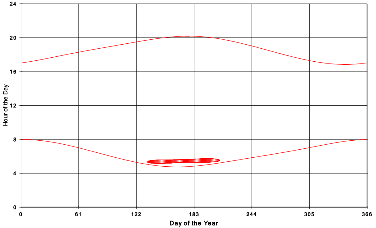
Goshen Wind Energy Centre Shadow Times on House 1502, All Windows from All Turbine
