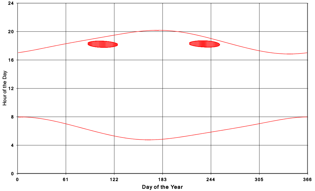
Goshen Wind Energy Centre Shadow Times on House 1335, All Windows from All Turbine
