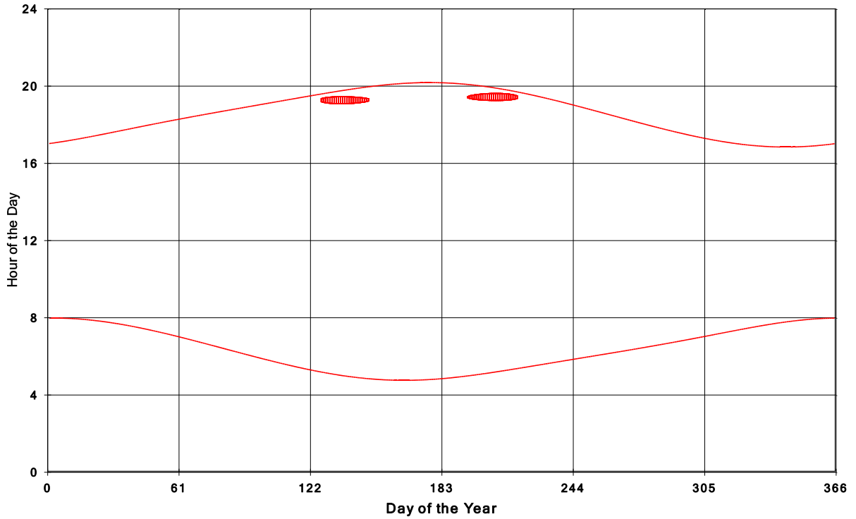
Goshen Wind Energy Centre Shadow Times on House 1170, All Windows from All Turbine
