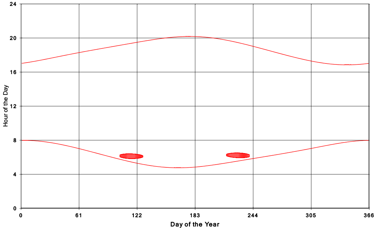
Goshen Wind Energy Centre Shadow Times on House 1288, All Windows from All Turbine
