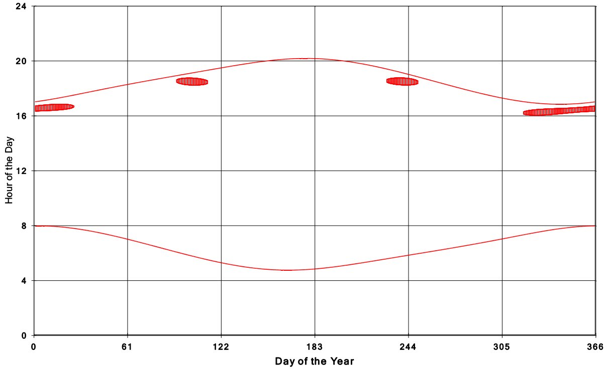
Goshen Wind Energy Centre Shadow Times on House 1274, All Windows from All Turbine
