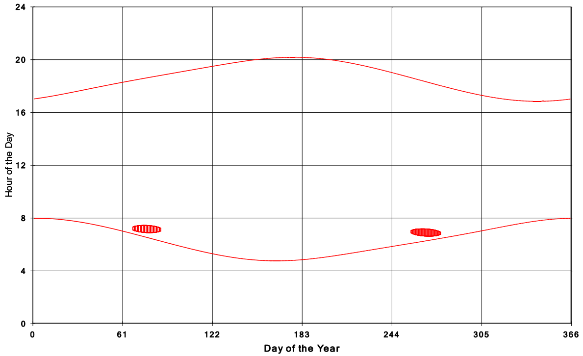
Jericho Wind Energy Centre Shadow Times on House 1249, All Windows from All Turbine:
