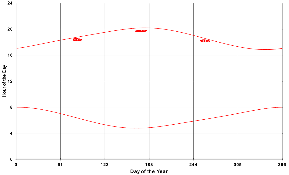
Goshen Wind Energy Centre Shadow Times on House 1212, All Windows from All Turbine
