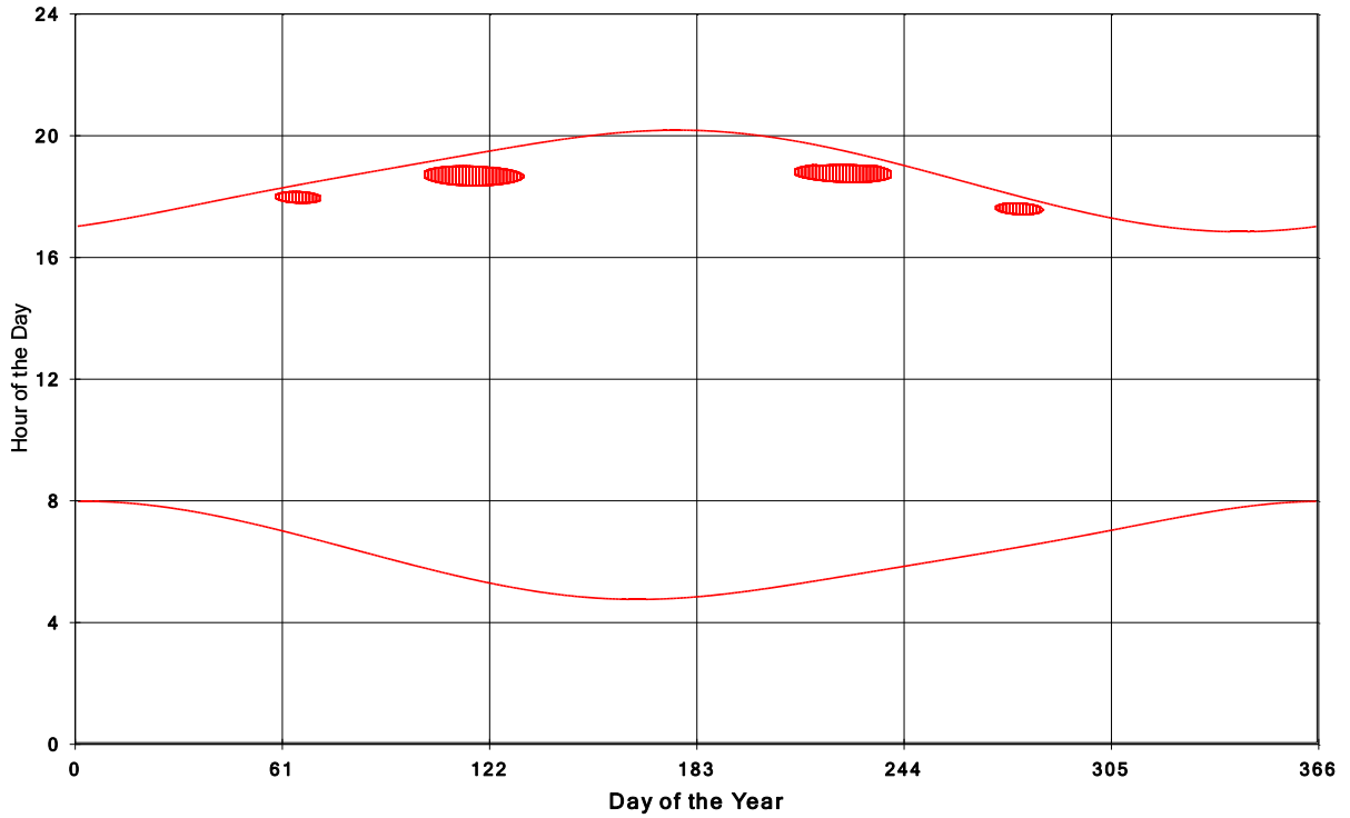
Goshen Wind Energy Centre Shadow Times on House 1318, All Windows from All Turbine
