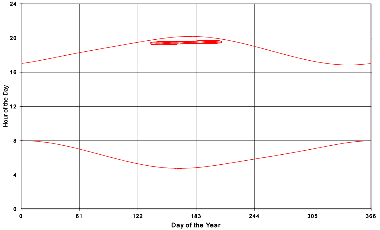
Goshen Wind Energy Centre Shadow Times on House 1173, All Windows from All Turbine
