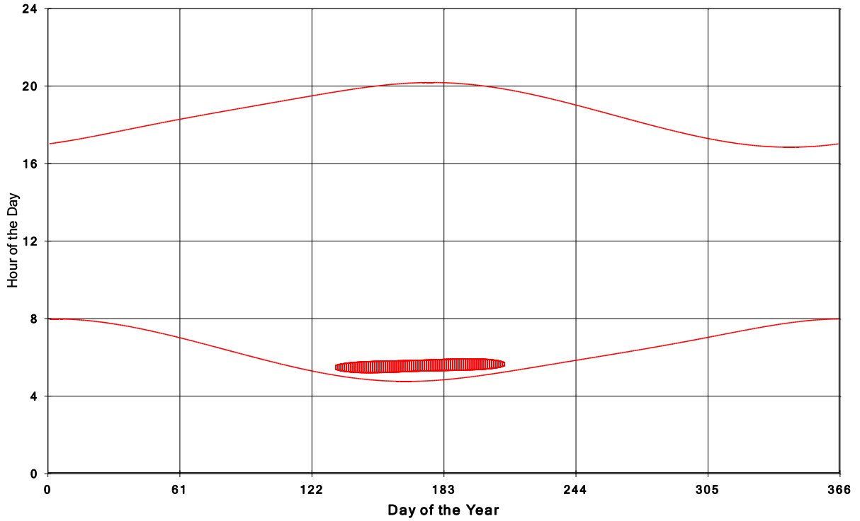
Goshen Wind Energy Centre Shadow Times on House 1224, All Windows from All Turbine
