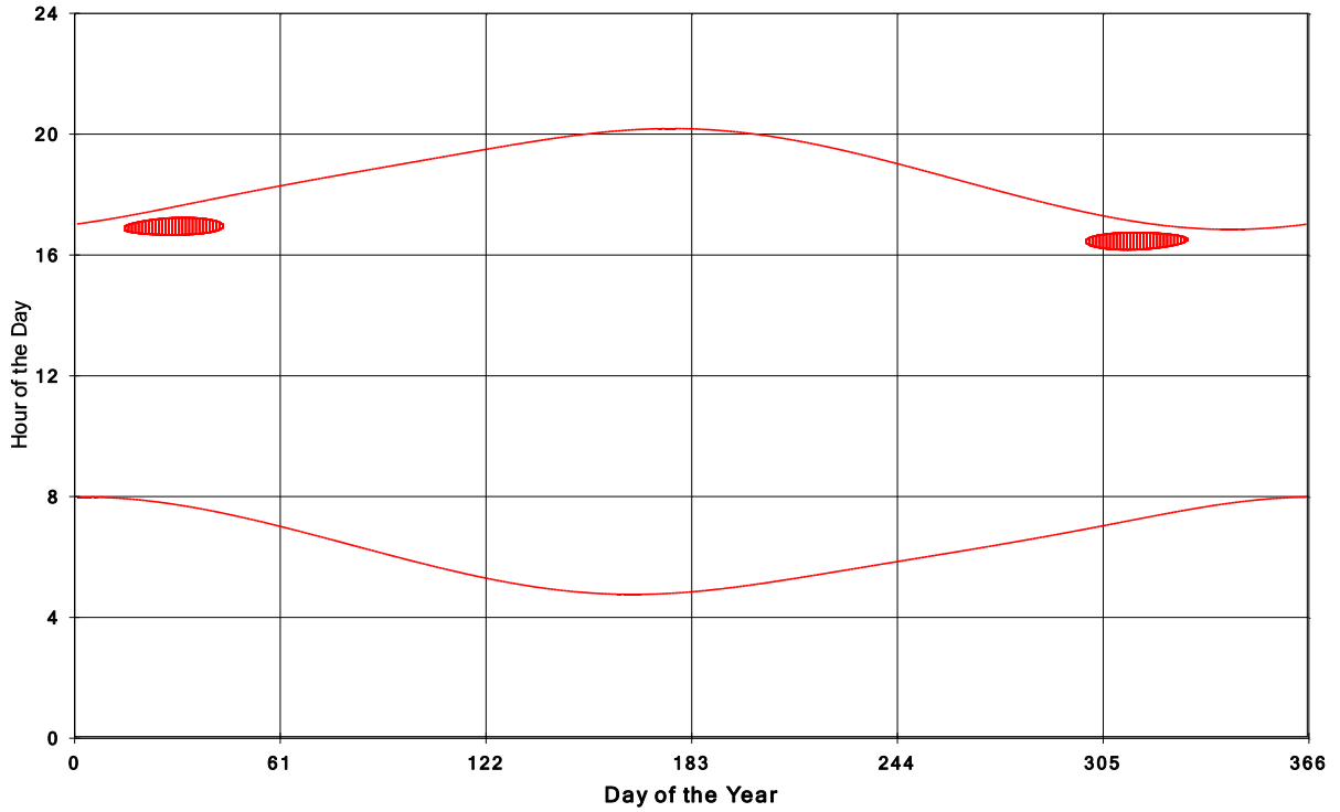
Goshen Wind Energy Centre Shadow Times on House 1323, All Windows from All Turbine
