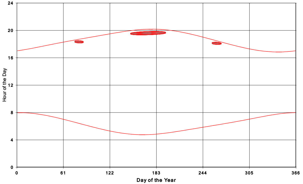
Goshen Wind Energy Centre Shadow Times on House 1213, All Windows from All Turbine
