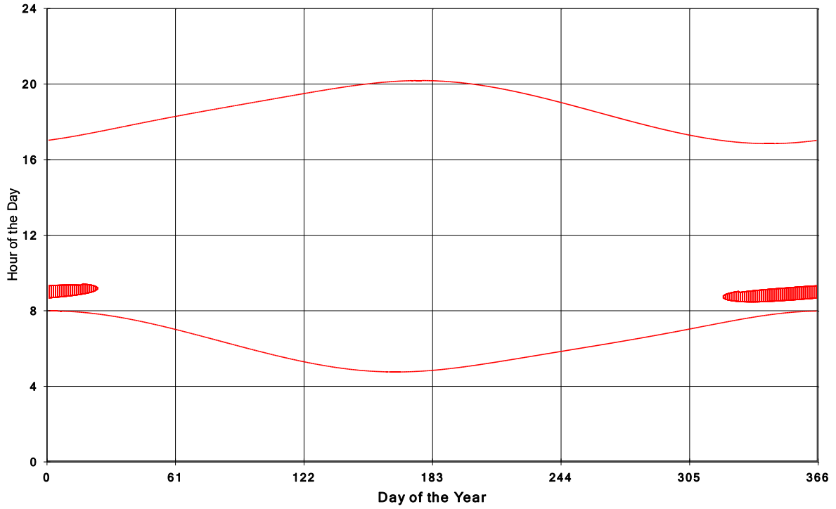
Jericho Wind Energy Centre Shadow Times on House 1248, All Windows from All Turbine
