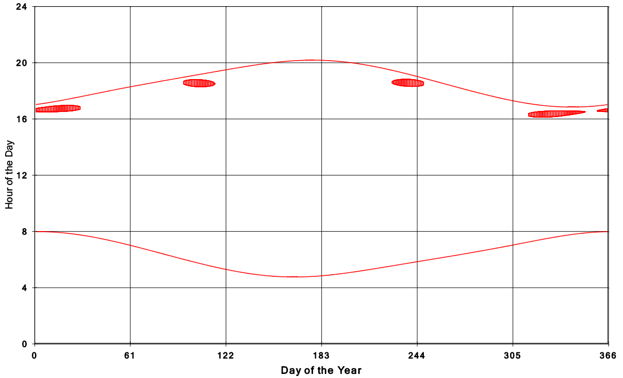
Goshen Wind Energy Centre Shadow Times on House 1273, All Windows from All Turbine
