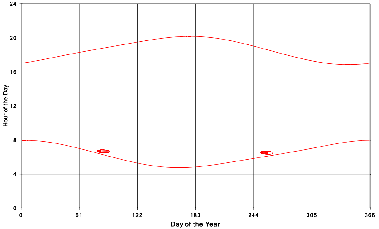
Goshen Wind Energy Centre Shadow Times on House 1202, All Windows from All Turbine
