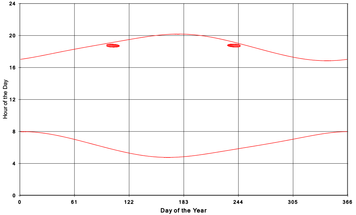
Goshen Wind Energy Centre Shadow Times on House 1317, All Windows from All Turbine
