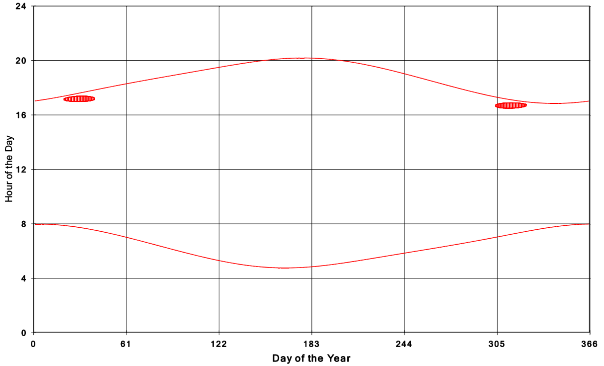
Goshen Wind Energy Centre Shadow Times on House 1206, All Windows from All Turbine
