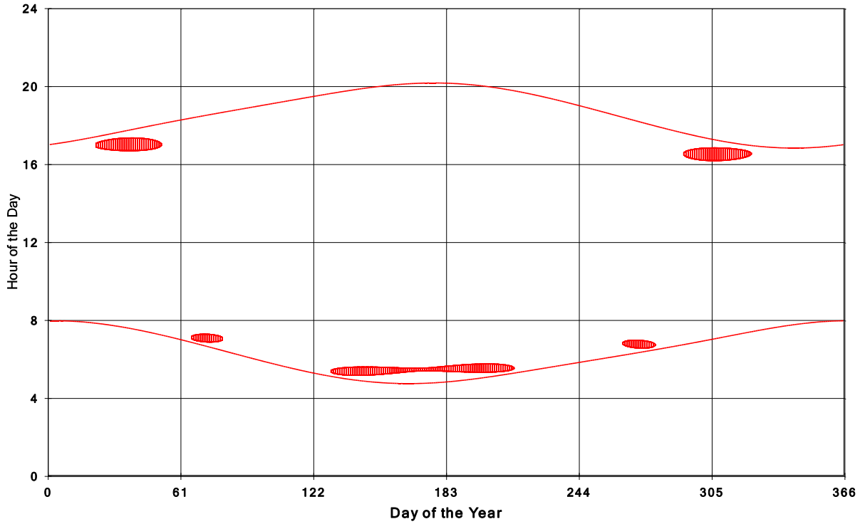
Goshen Wind Energy Centre Shadow Times on House 1308, All Windows from All Turbine
