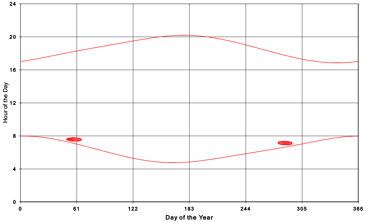
Goshen Wind Energy Centre Shadow Times on House 1178, All Windows from All Turbine
