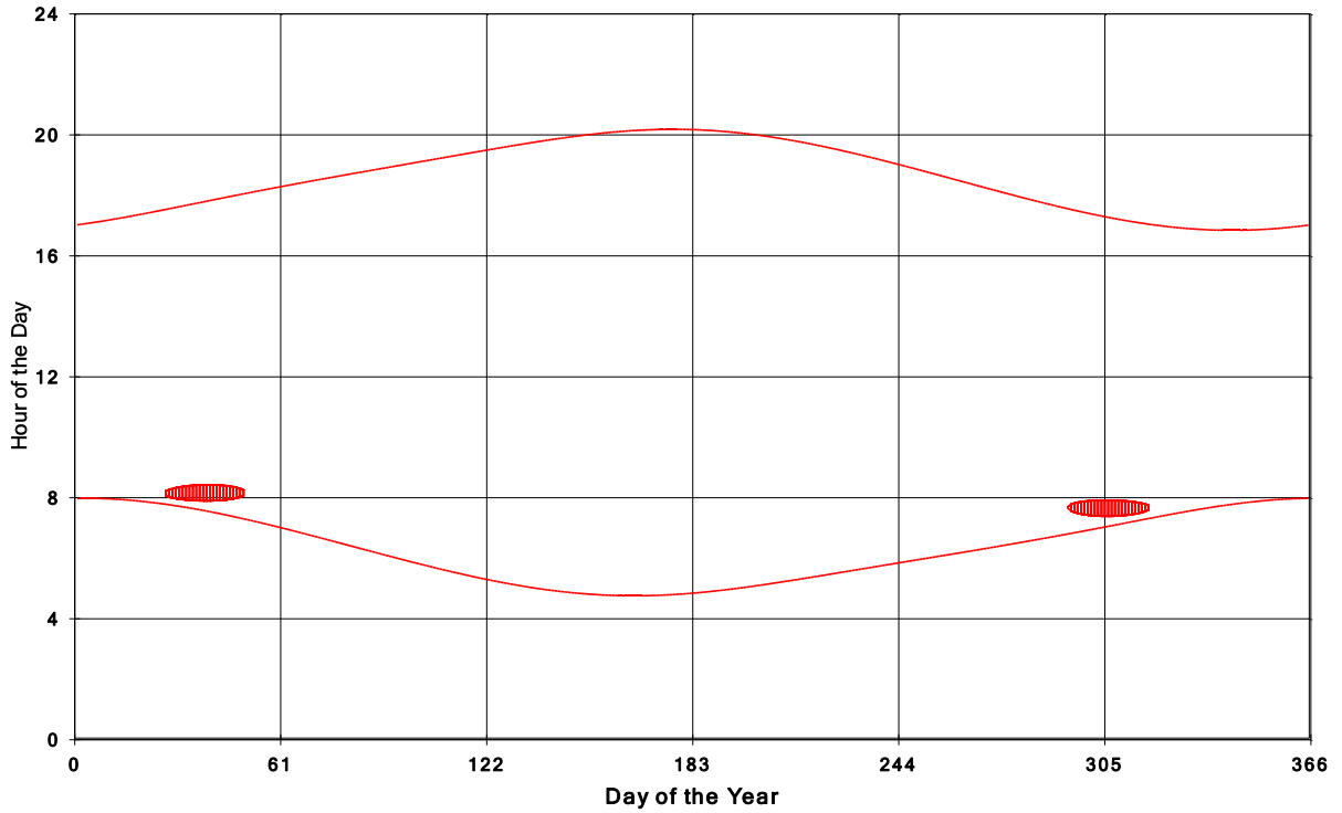
Goshen Wind Energy Centre Shadow Times on House 1326, All Windows from All Turbine
