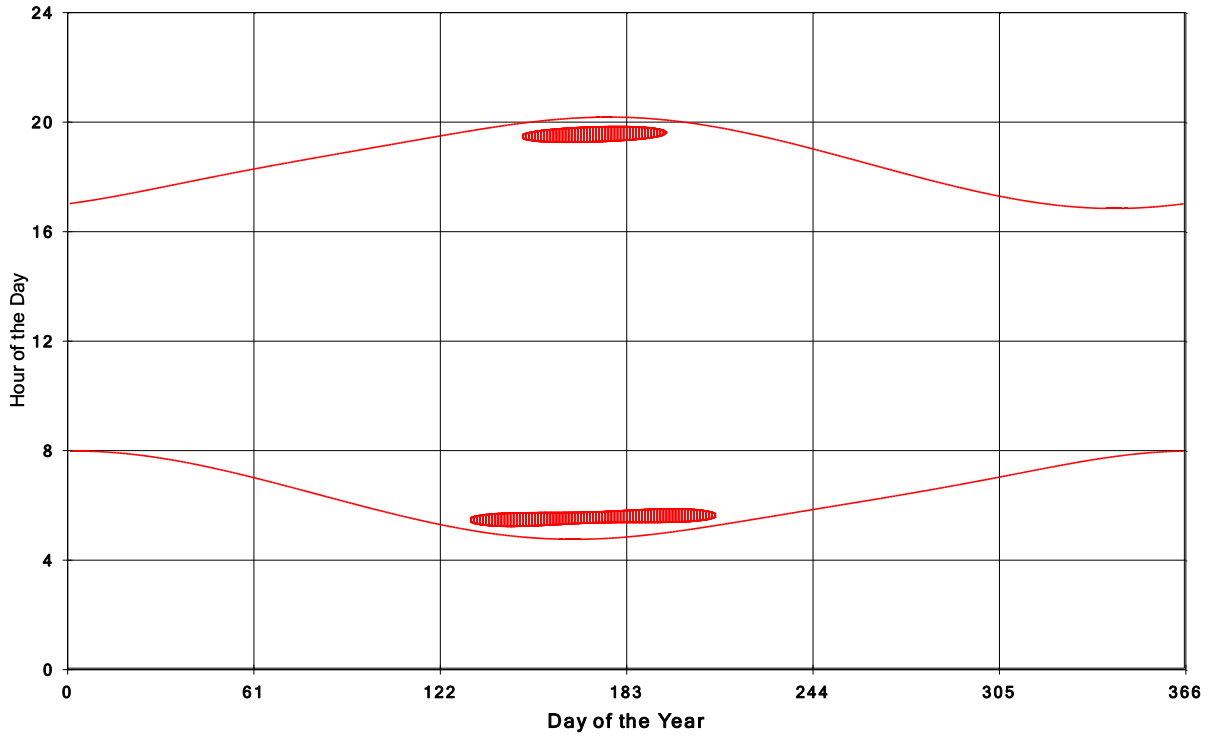
Goshen Wind Energy Centre Shadow Times on House 1214, All Windows from All Turbine
