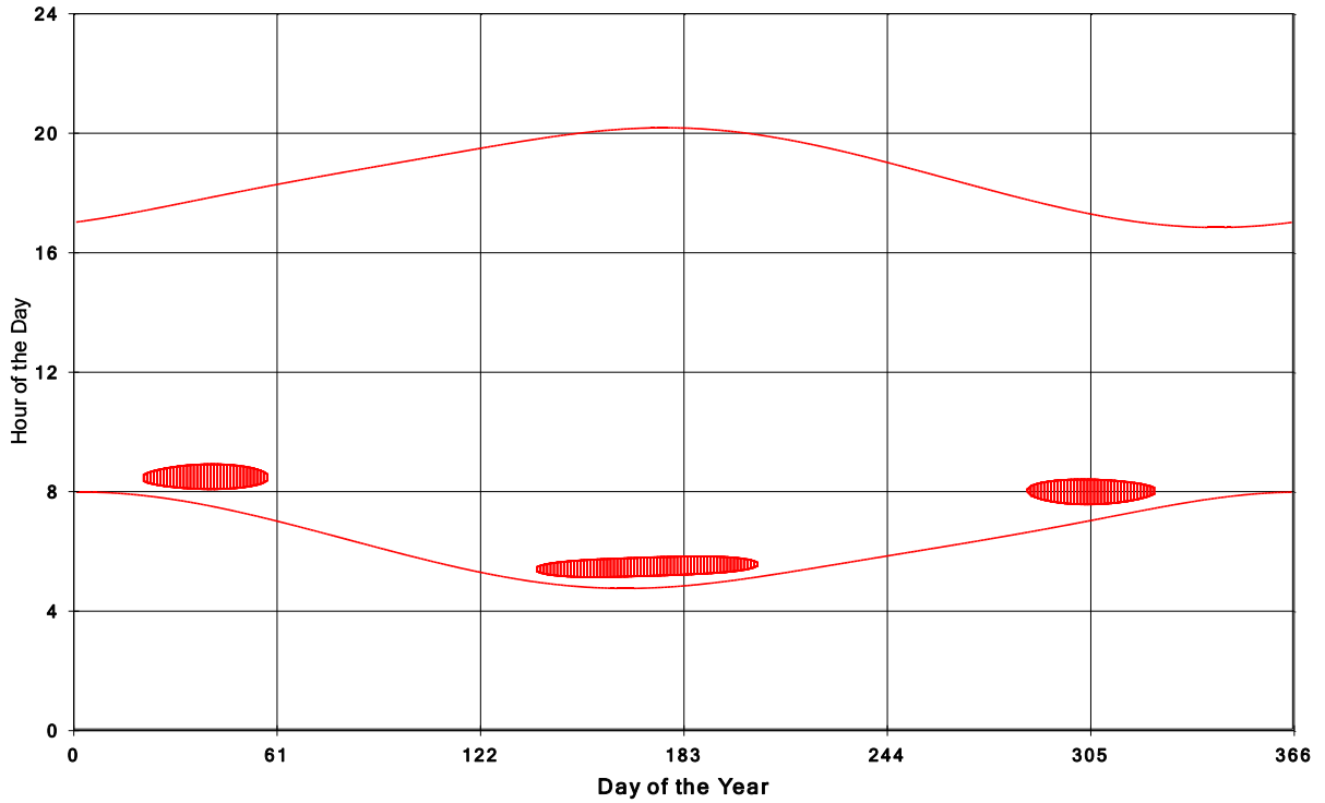
Goshen Wind Energy Centre Shadow Times on House 1225, All Windows from All Turbine
