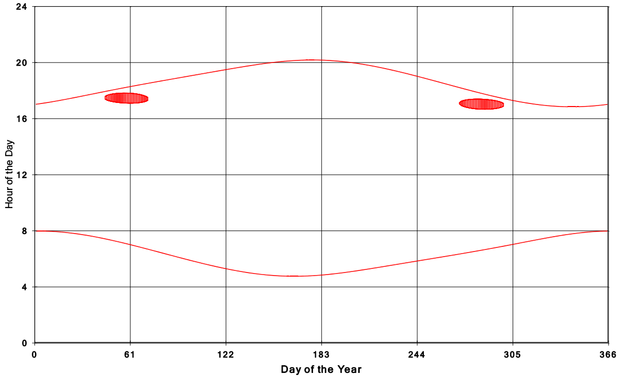
Goshen Wind Energy Centre Shadow Times on House 1293, All Windows from All Turbine
