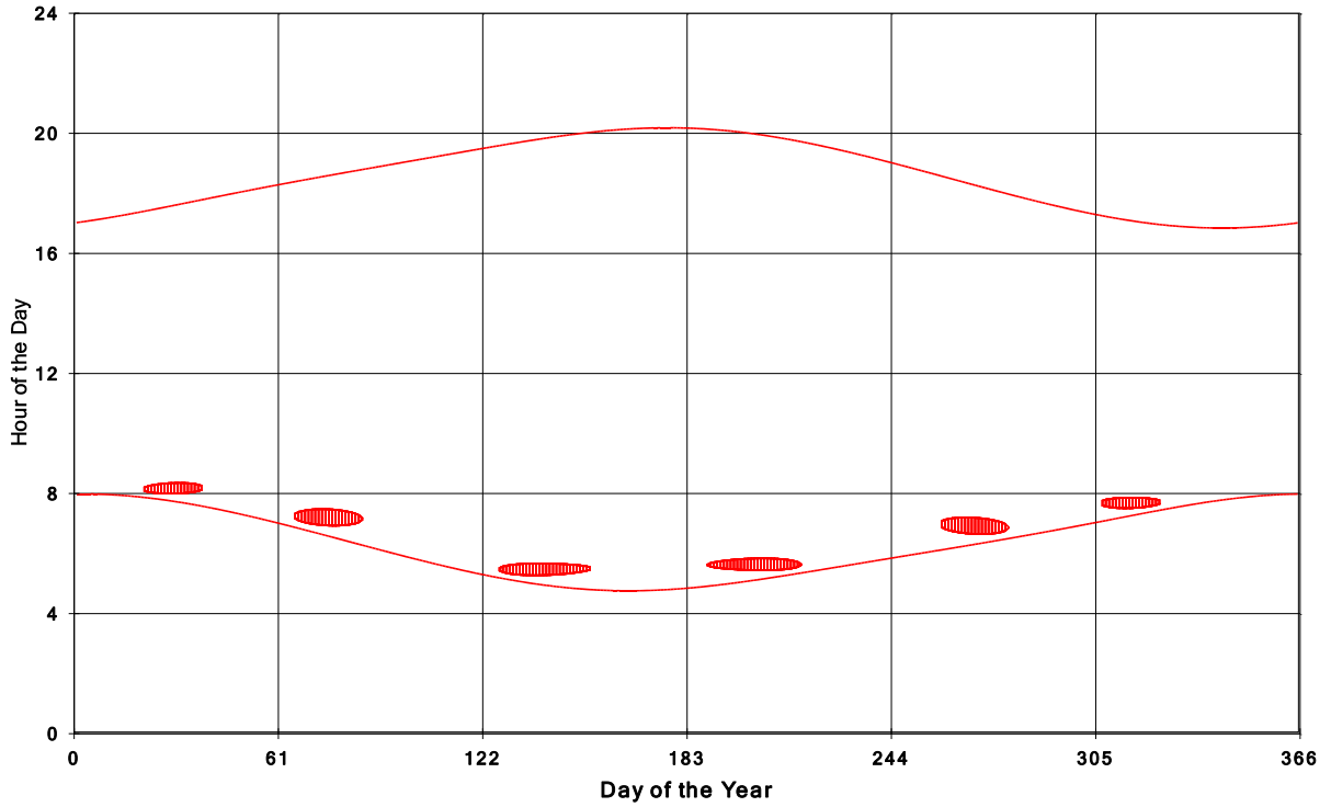
Goshen Wind Energy Centre Shadow Times on House 1176, All Windows from All Turbine
