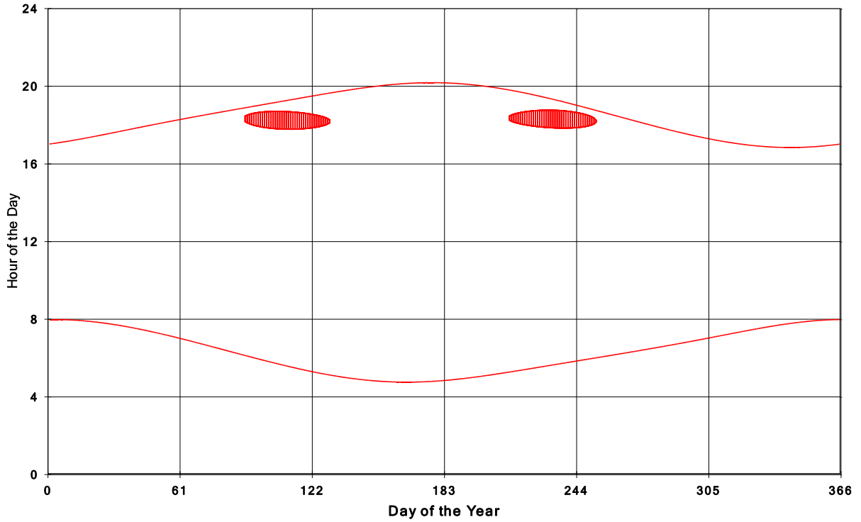
Goshen Wind Energy Centre Shadow Times on House 1166, All Windows from All Turbine
