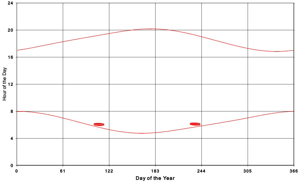
Goshen Wind Energy Centre Shadow Times on House 1227, All Windows from All Turbine
