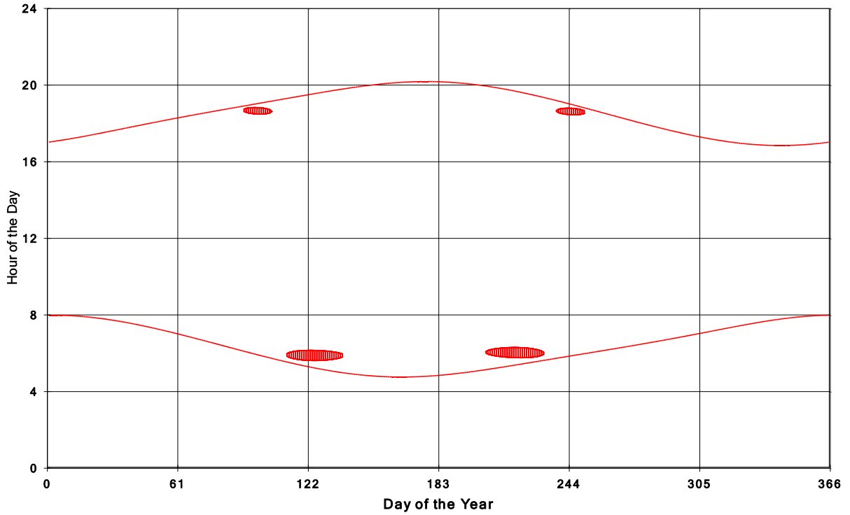
Goshen Wind Energy Centre Shadow Times on House 1235, All Windows from All Turbine
