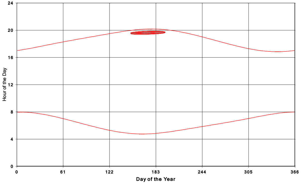
Goshen Wind Energy Centre Shadow Times on House 1255, All Windows from All Turbine
