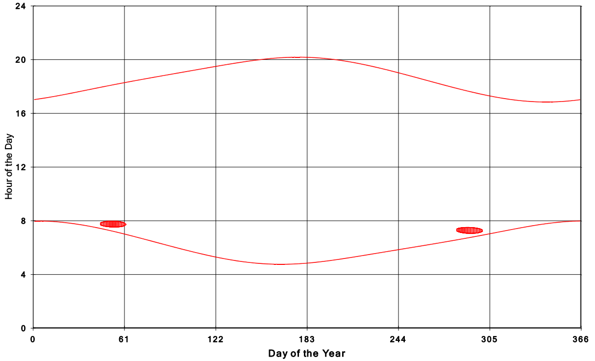
Goshen Wind Energy Centre Shadow Times on House 1287, All Windows from All Turbine
