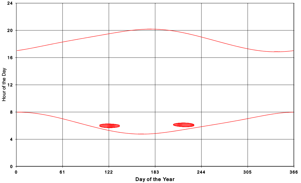
Goshen Wind Energy Centre Shadow Times on House 1251, All Windows from All Turbine
