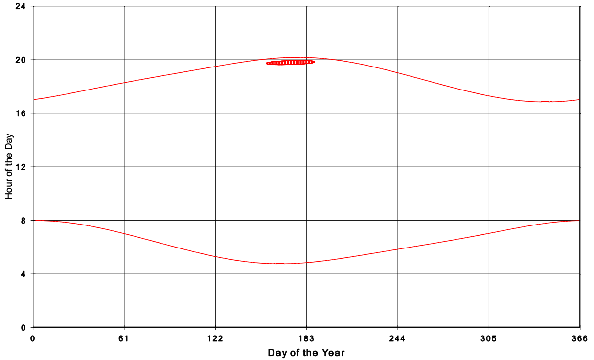
Goshen Wind Energy Centre Shadow Times on House 1286, All Windows from All Turbine
