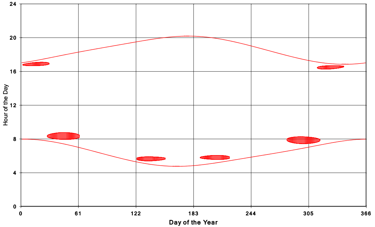
Goshen Wind Energy Centre Shadow Times on House 1210, All Windows from All Turbine
