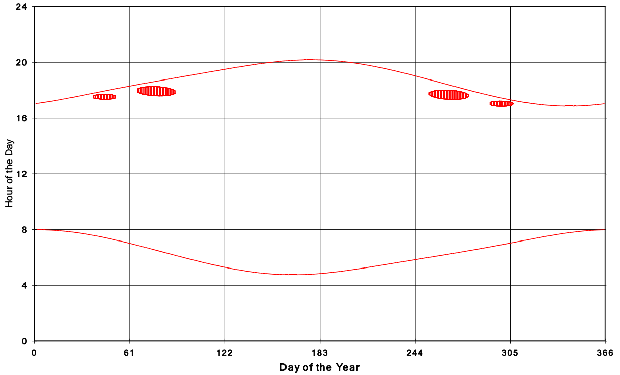
Goshen Wind Energy Centre Shadow Times on House 1320, All Windows from All Turbine
