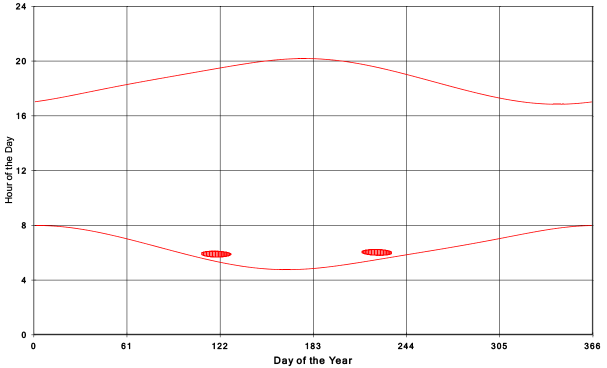
Goshen Wind Energy Centre Shadow Times on House 1261, All Windows from All Turbine
