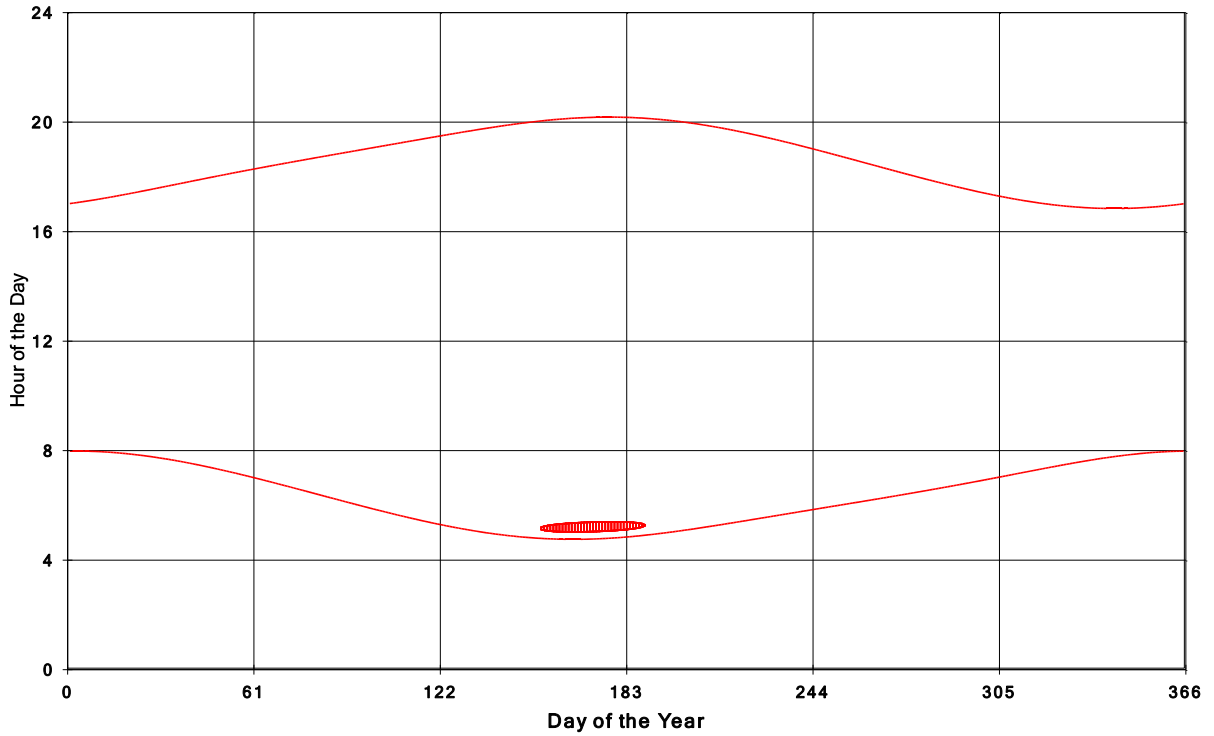
Goshen Wind Energy Centre Shadow Times on House 1290, All Windows from All Turbine
