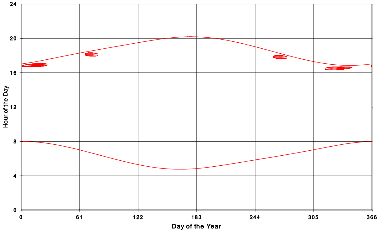
Goshen Wind Energy Centre Shadow Times on House 1216, All Windows from All Turbine
