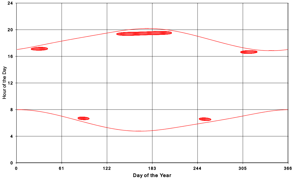
Goshen Wind Energy Centre Shadow Times on House 1295, All Windows from All Turbine
