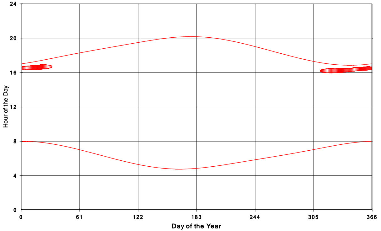
Goshen Wind Energy Centre Shadow Times on House 1321, All Windows from All Turbine
