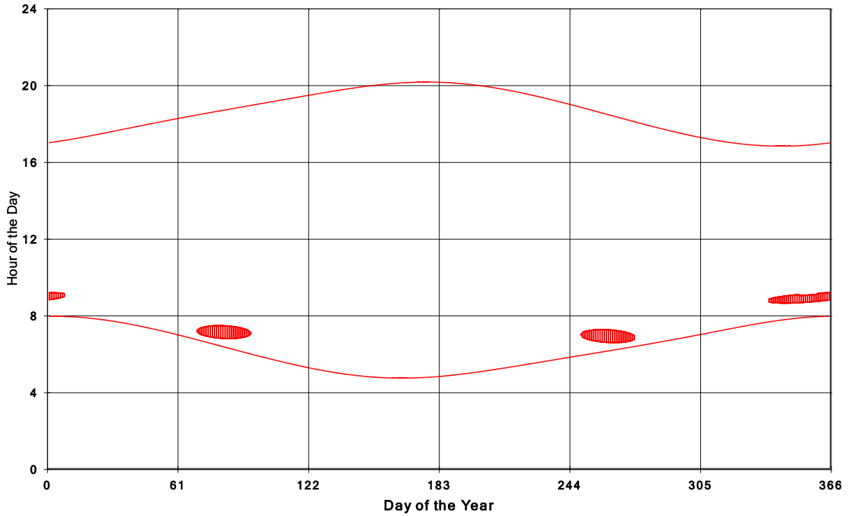
Goshen Wind Energy Centre Shadow Times on House 1234, All Windows from All Turbine
