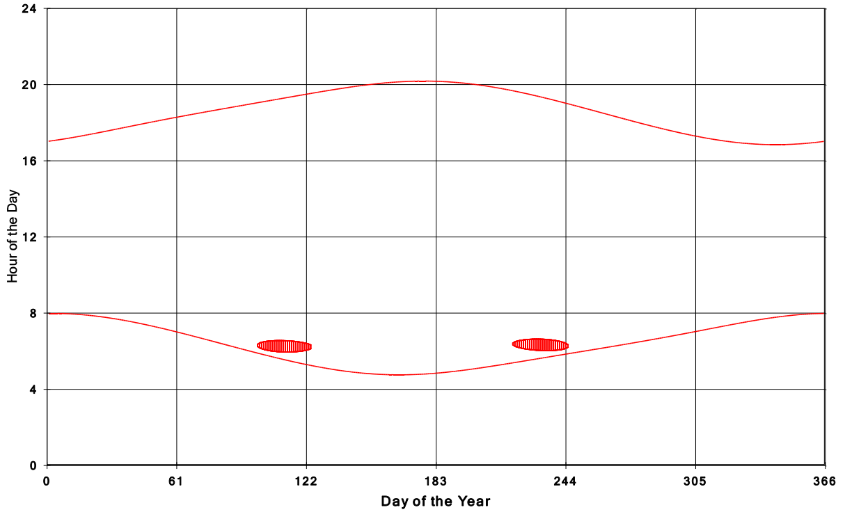
Goshen Wind Energy Centre Shadow Times on House 1289, All Windows from All Turbine
