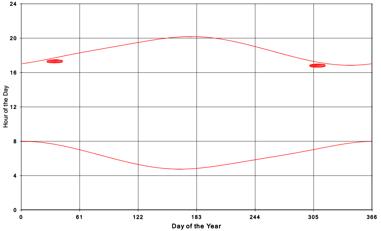
Goshen Wind Energy Centre Shadow Times on House 1215, All Windows from All Turbine
