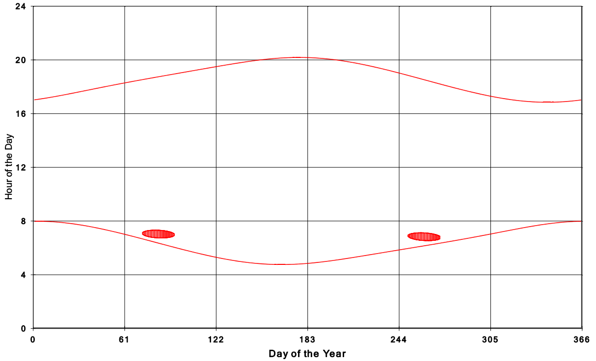
Goshen Wind Energy Centre Shadow Times on House 1267, All Windows from All Turbine
