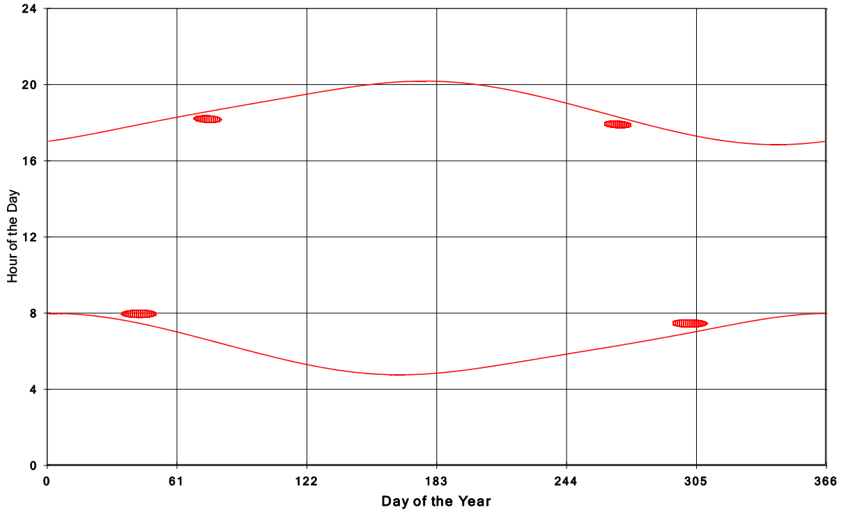
Goshen Wind Energy Centre Shadow Times on House 1194, All Windows from All Turbine
