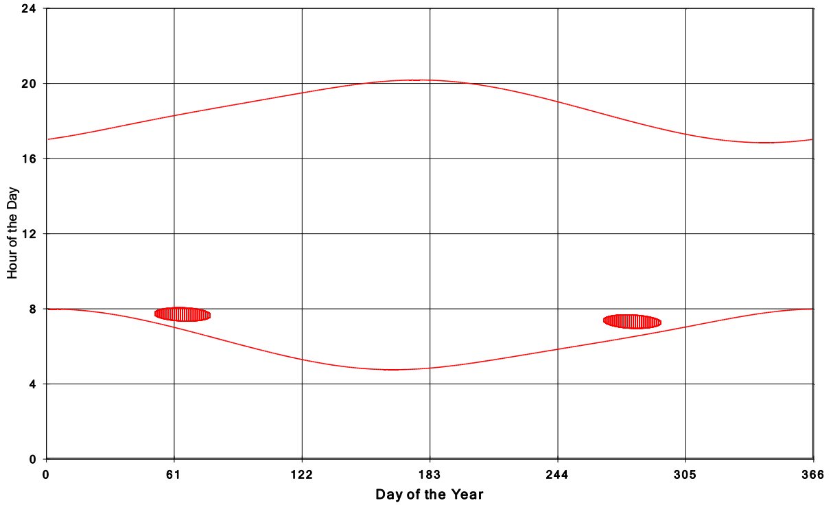
Goshen Wind Energy Centre Shadow Times on House 1211, All Windows from All Turbine
