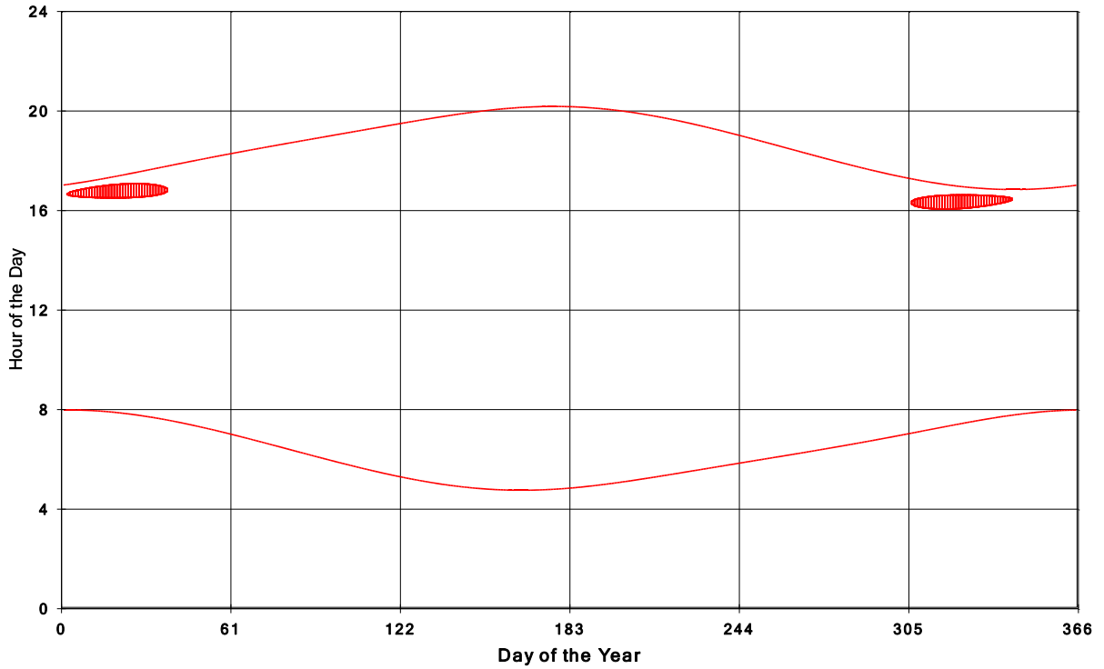
Goshen Wind Energy Centre Shadow Times on House 1322, All Windows from All Turbine
