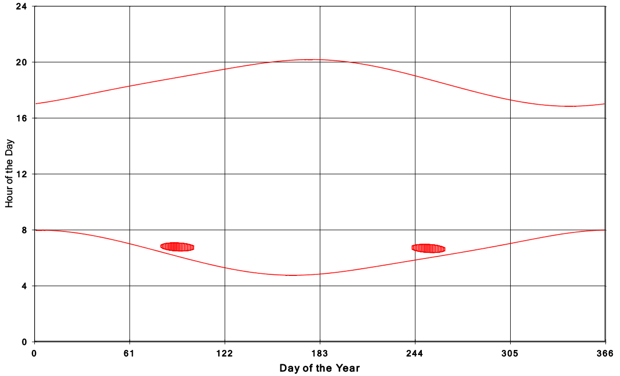
Goshen Wind Energy Centre Shadow Times on House 1268, All Windows from All Turbine
