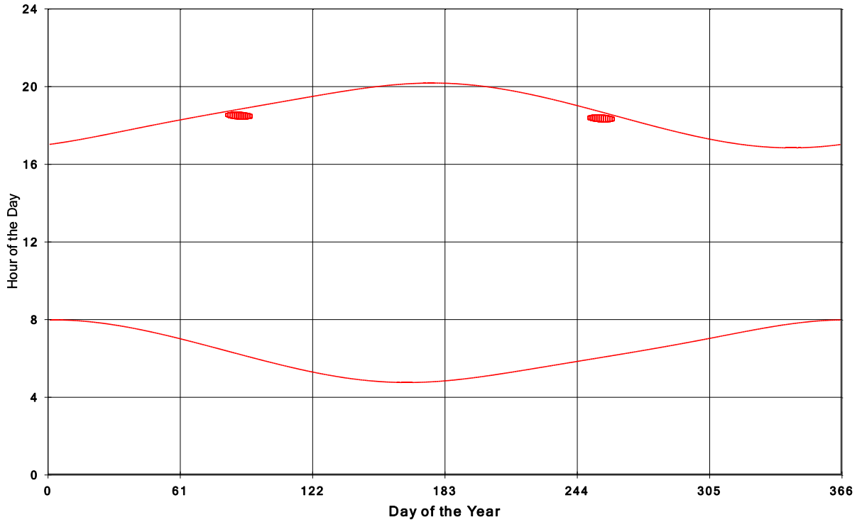
Goshen Wind Energy Centre Shadow Times on House 1207, All Windows from All Turbine
