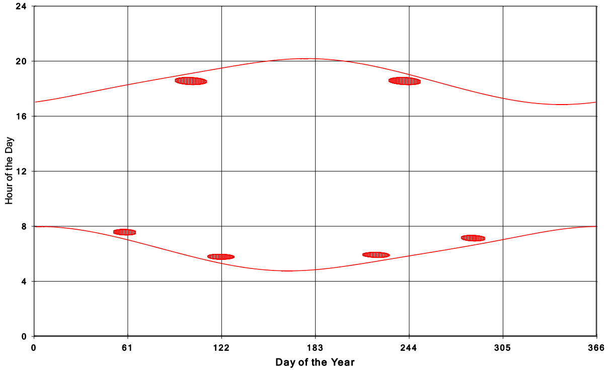
Goshen Wind Energy Centre Shadow Times on House 1294, All Windows from All Turbine
