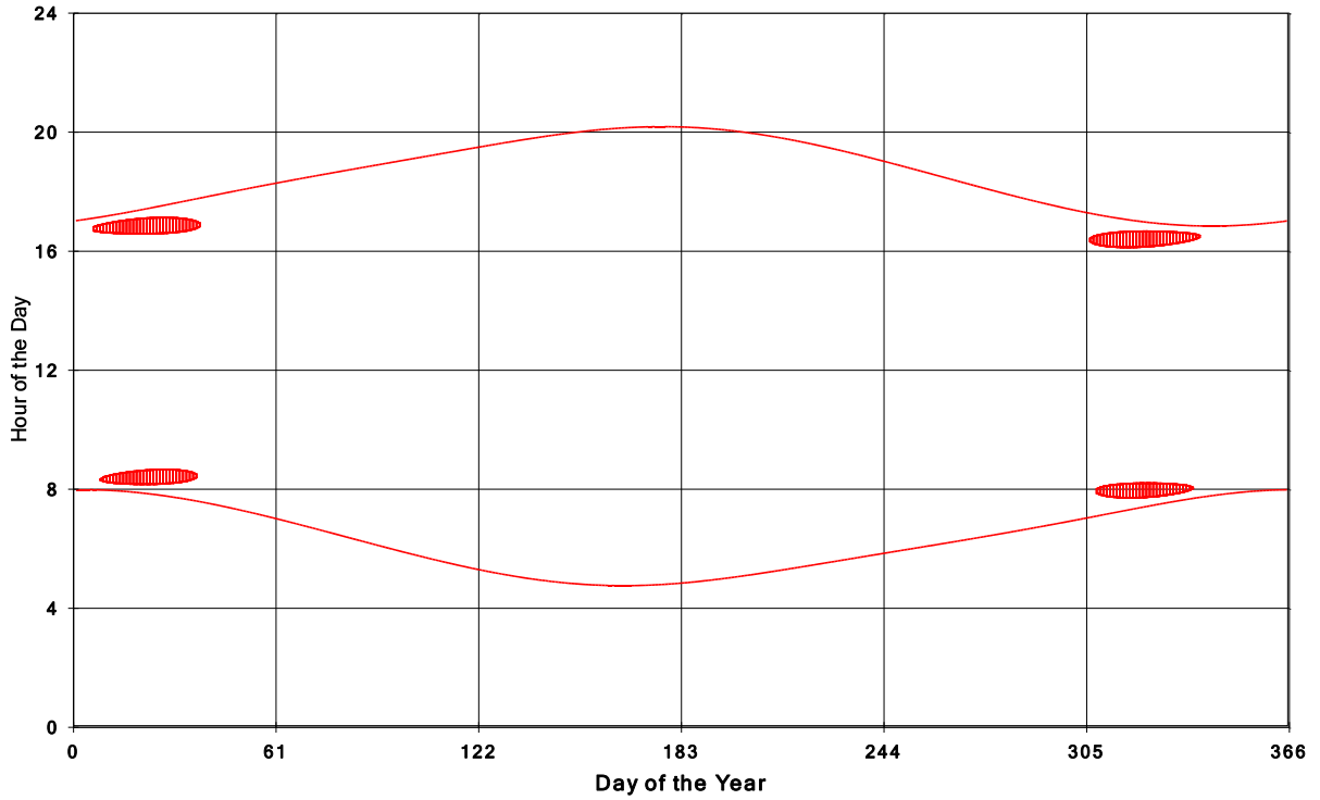
Goshen Wind Energy Centre Shadow Times on House 1229, All Windows from All Turbine
