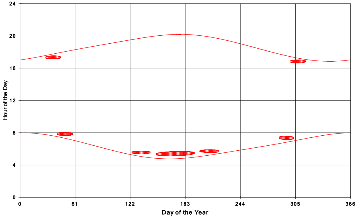
Goshen Wind Energy Centre Shadow Times on House 1311, All Windows from All Turbine
