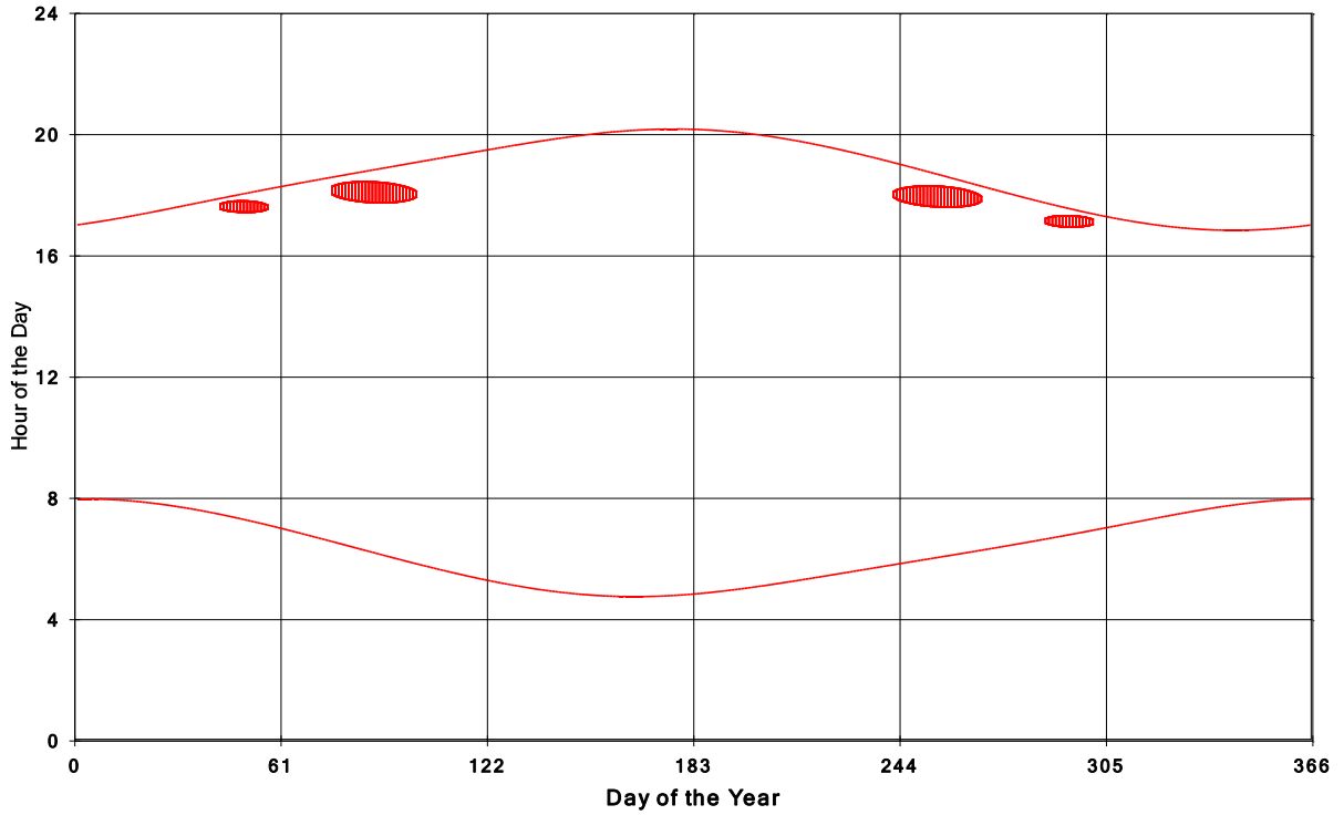
Goshen Wind Energy Centre Shadow Times on House 1319, All Windows from All Turbine
