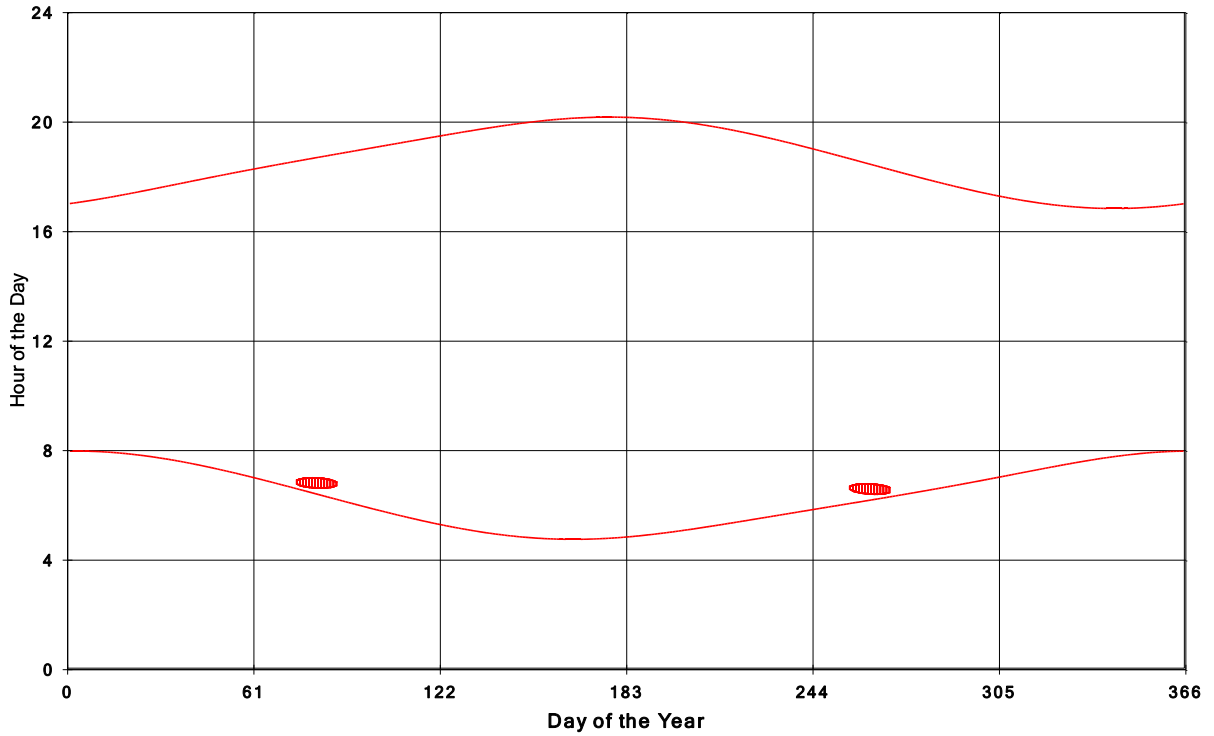
Goshen Wind Energy Centre Shadow Times on House 1199, All Windows from All Turbine
