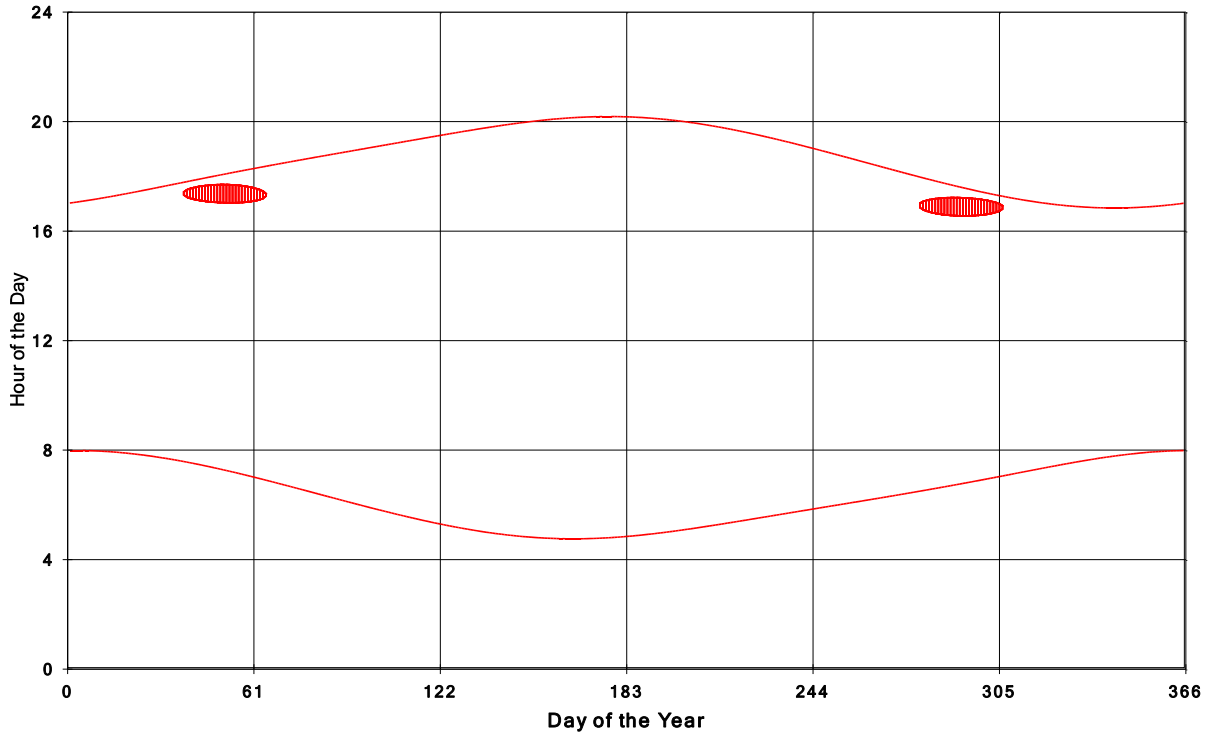
Goshen Wind Energy Centre Shadow Times on House 1217, All Windows from All Turbine
