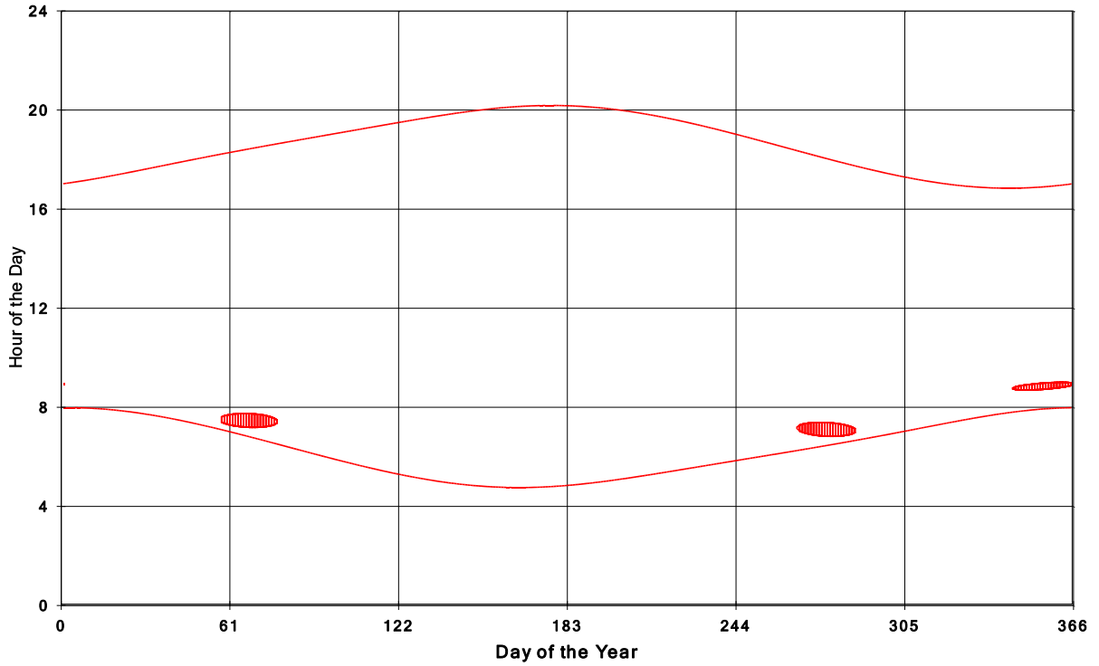
Goshen Wind Energy Centre Shadow Times on House 1233, All Windows from All Turbine
