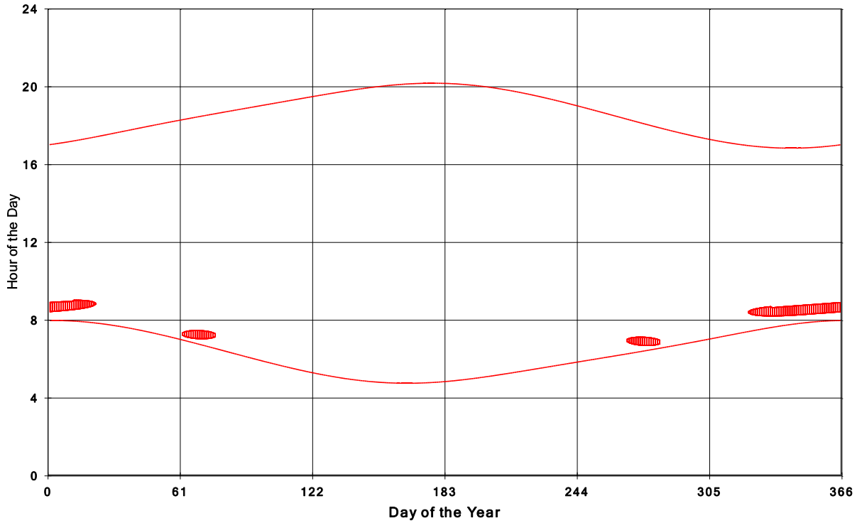
Goshen Wind Energy Centre Shadow Times on House 1180, All Windows from All Turbine
