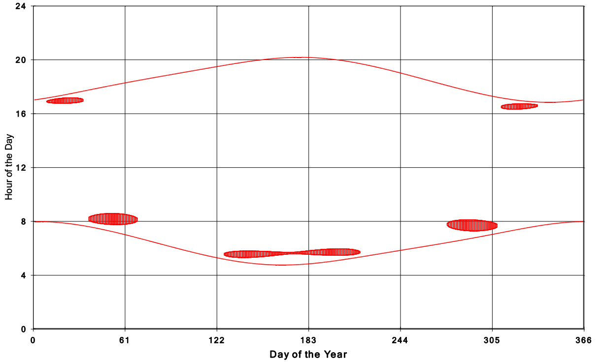
Goshen Wind Energy Centre Shadow Times on House 1209, All Windows from All Turbine
