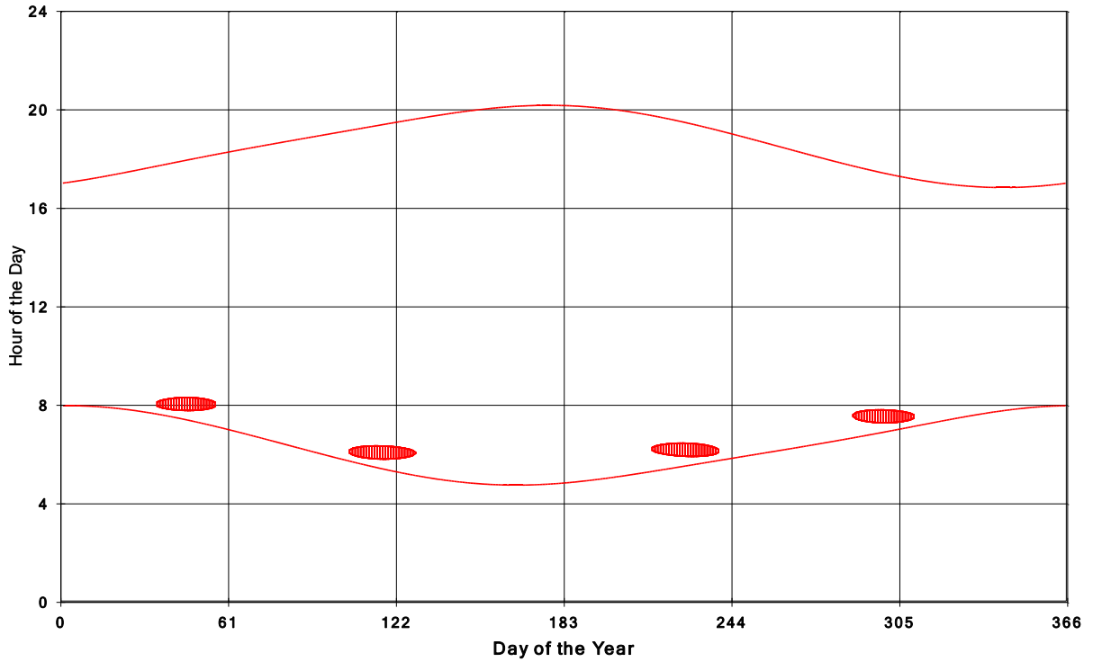
Goshen Wind Energy Centre Shadow Times on House 1230, All Windows from All Turbine
