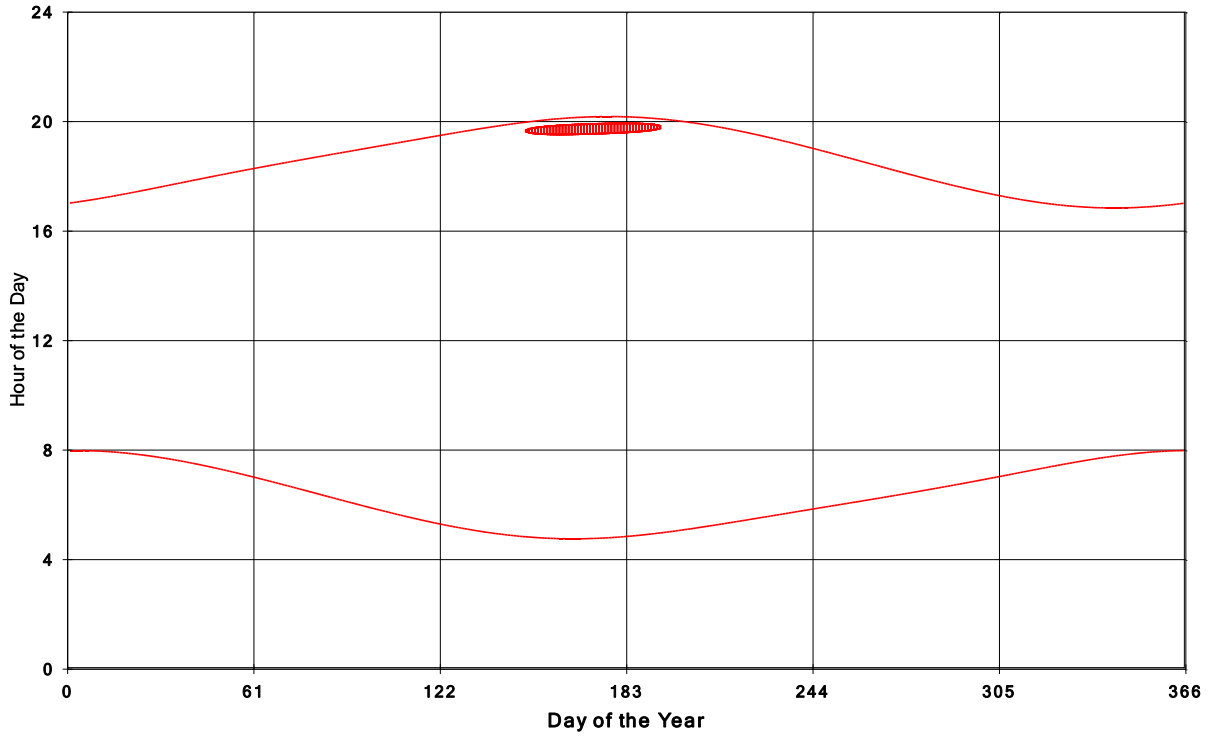
Goshen Wind Energy Centre Shadow Times on House 1285, All Windows from All Turbine
