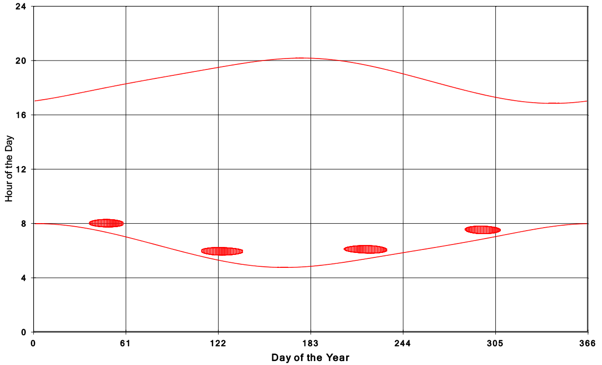
Goshen Wind Energy Centre Shadow Times on House 1232, All Windows from All Turbine
