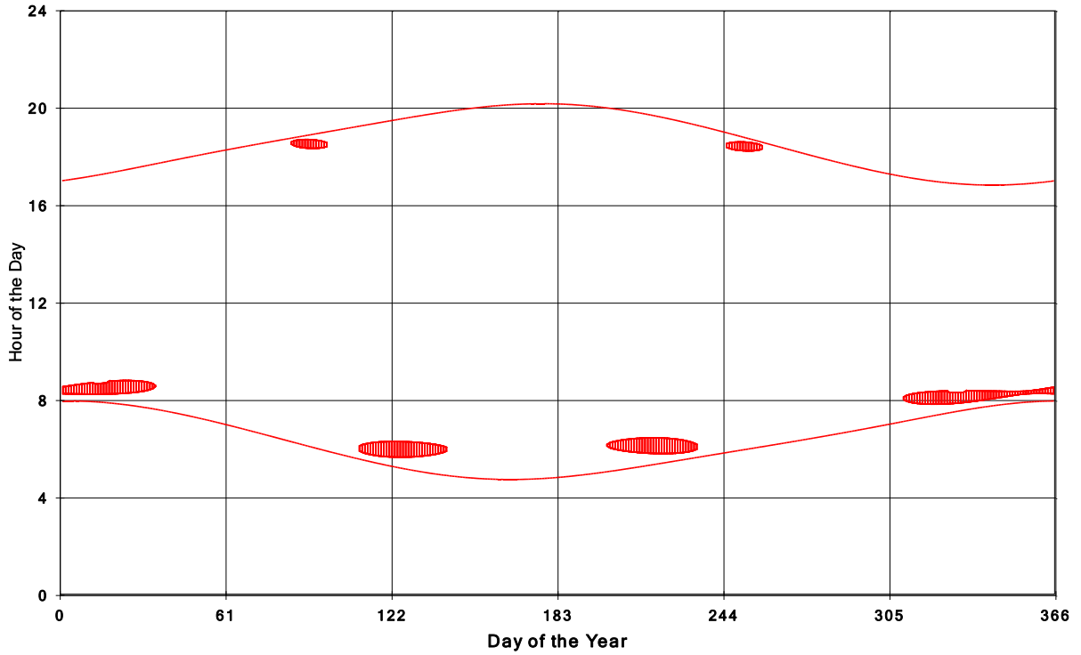
Goshen Wind Energy Centre Shadow Times on House 1325, All Windows from All Turbine
