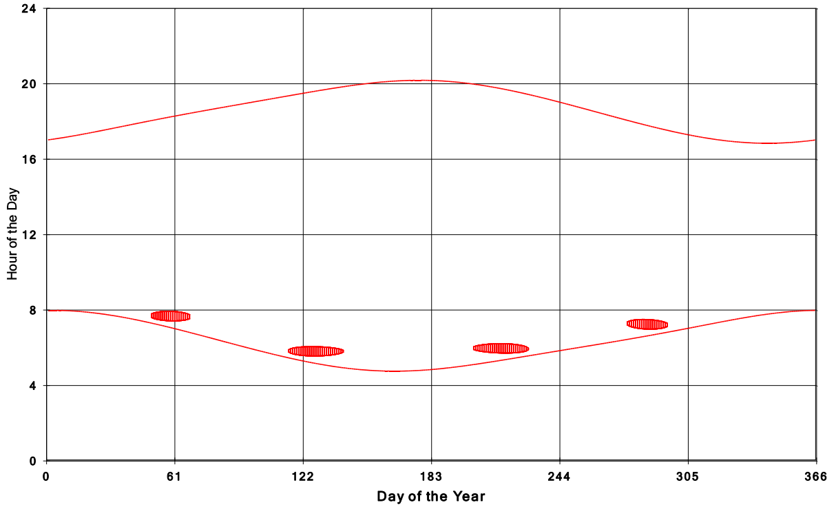
Goshen Wind Energy Centre Shadow Times on House 1231, All Windows from All Turbine
