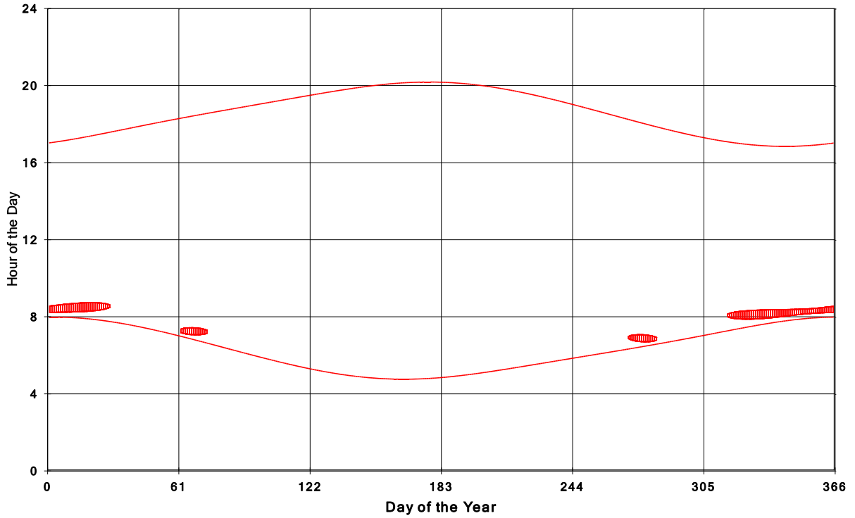
Goshen Wind Energy Centre Shadow Times on House 1179, All Windows from All Turbine
