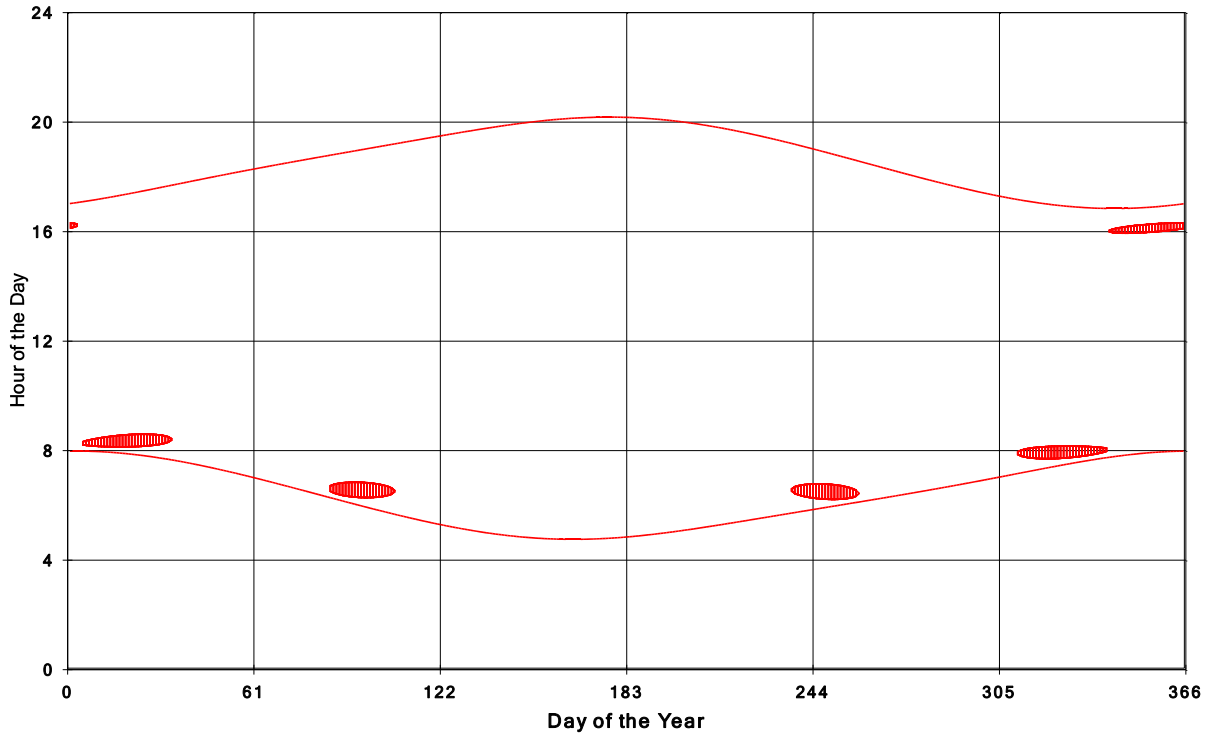
Goshen Wind Energy Centre Shadow Times on House 1309, All Windows from All Turbine
