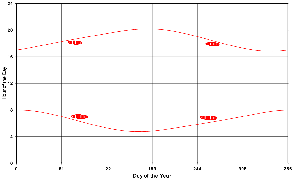
Goshen Wind Energy Centre Shadow Times on House 1265, All Windows from All Turbine
