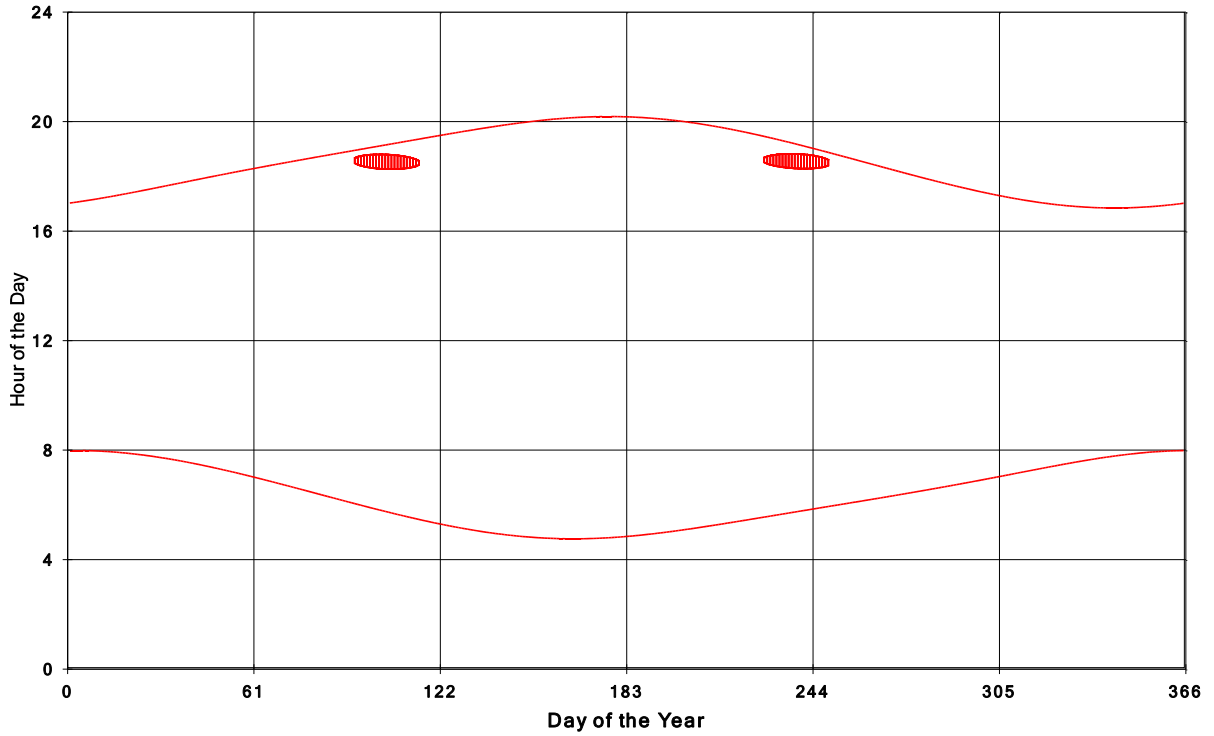
Goshen Wind Energy Centre Shadow Times on House 1019, All Windows from All Turbine
