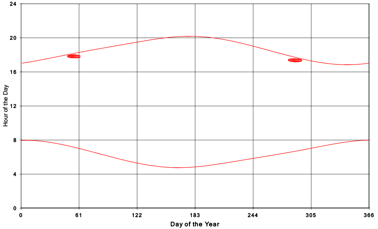
Goshen Wind Energy Centre Shadow Times on House 997, All Windows from All Turbine:
