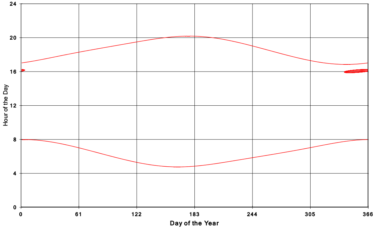
Goshen Wind Energy Centre Shadow Times on House 1133, All Windows from All Turbine
