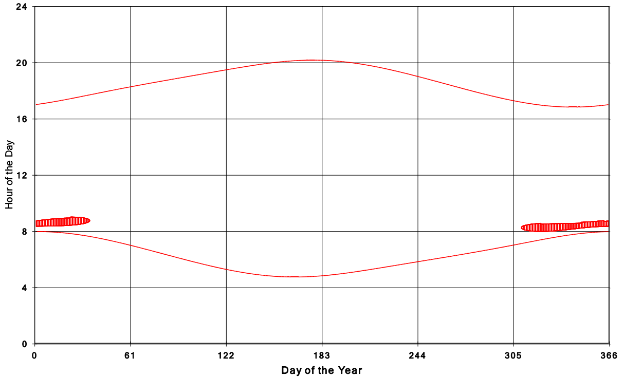
Goshen Wind Energy Centre Shadow Times on House 1055, All Windows from All Turbine
