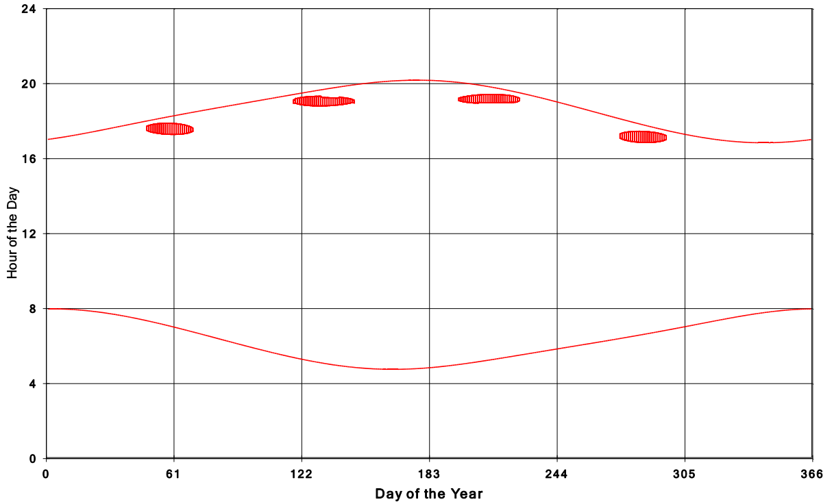
Goshen Wind Energy Centre Shadow Times on House 1162, All Windows from All Turbine
