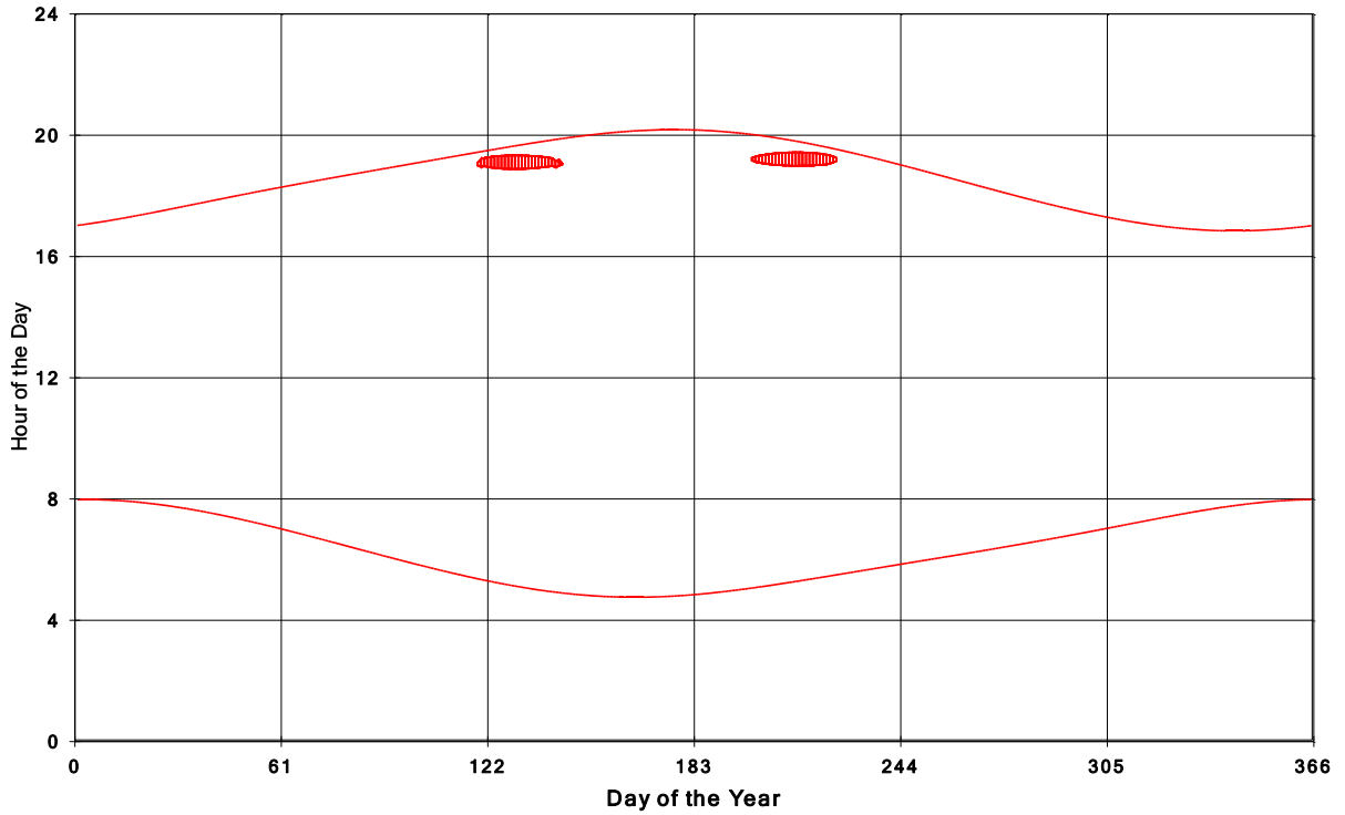
Goshen Wind Energy Centre Shadow Times on House 1037, All Windows from All Turbine
