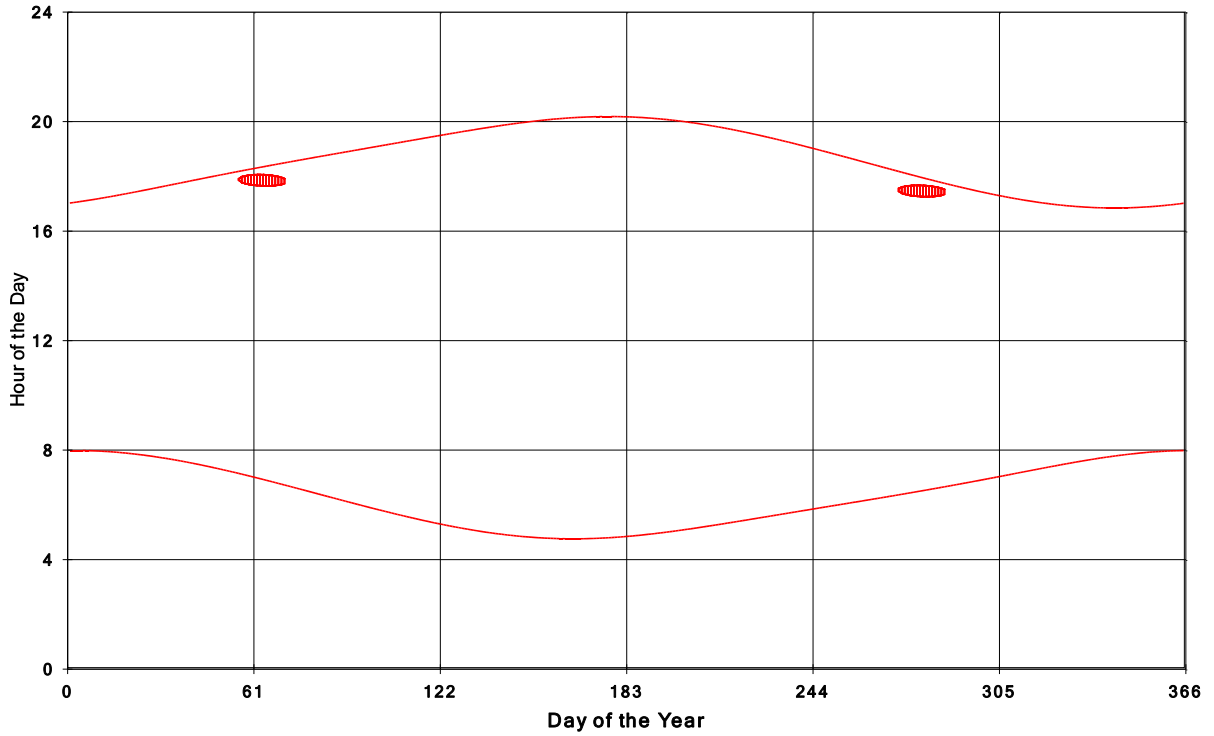
Goshen Wind Energy Centre Shadow Times on House 1011, All Windows from All Turbine
