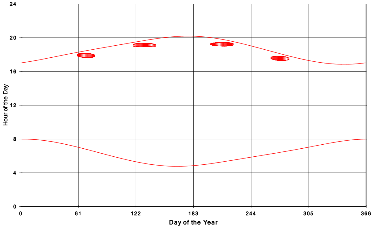
Goshen Wind Energy Centre Shadow Times on House 1061, All Windows from All Turbine
