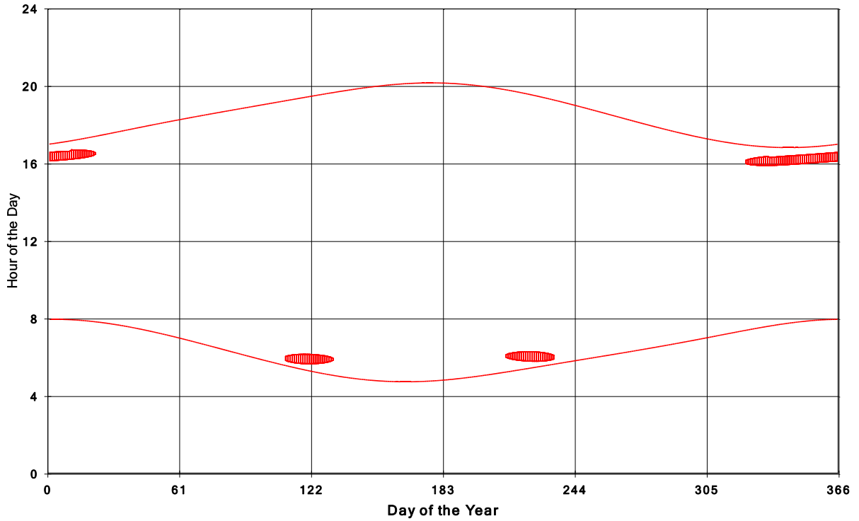
Goshen Wind Energy Centre Shadow Times on House 998, All Windows from All Turbine:
