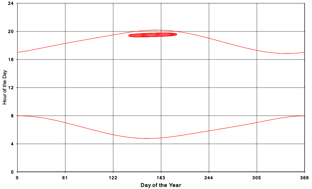
Goshen Wind Energy Centre Shadow Times on House 1020, All Windows from All Turbine
