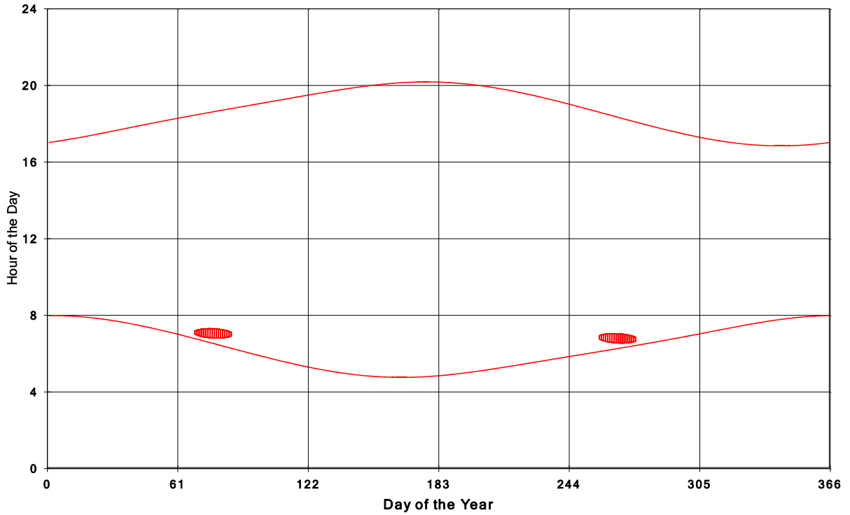
Goshen Wind Energy Centre Shadow Times on House 1006, All Windows from All Turbine
