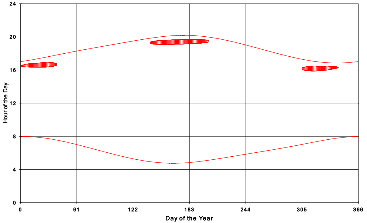
Goshen Wind Energy Centre Shadow Times on House 1145, All Windows from All Turbine
