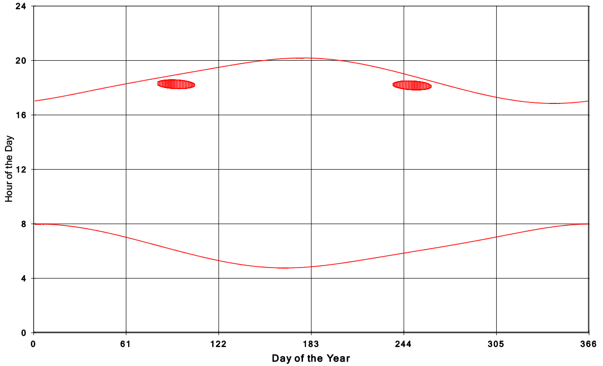
Goshen Wind Energy Centre Shadow Times on House 1030, All Windows from All Turbine
