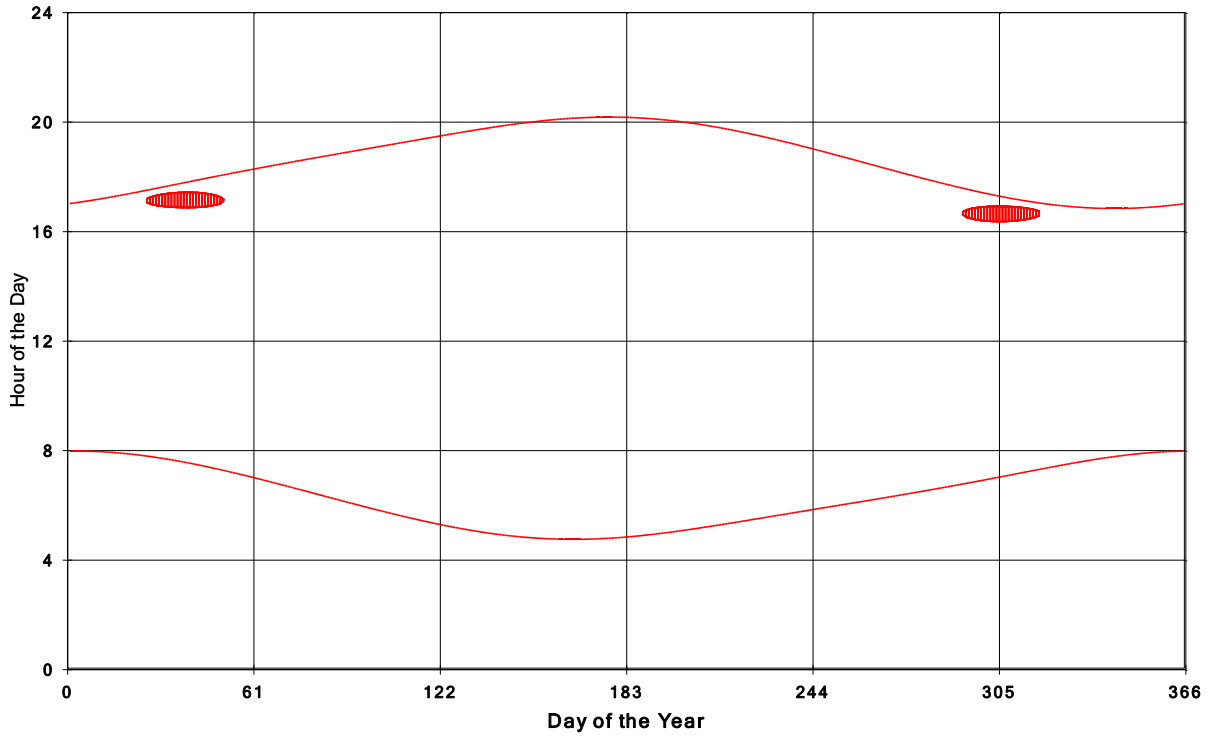
Goshen Wind Energy Centre Shadow Times on House 1094, All Windows from All Turbine
