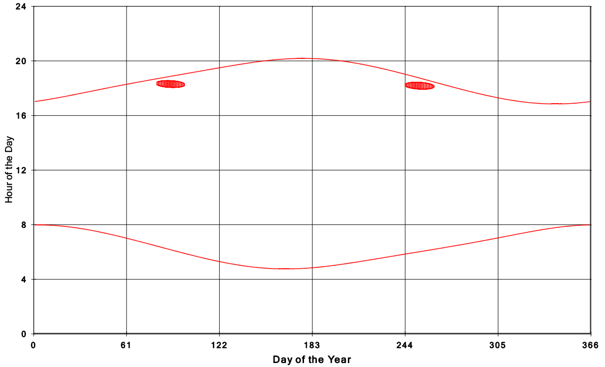
Goshen Wind Energy Centre Shadow Times on House 1043, All Windows from All Turbine
