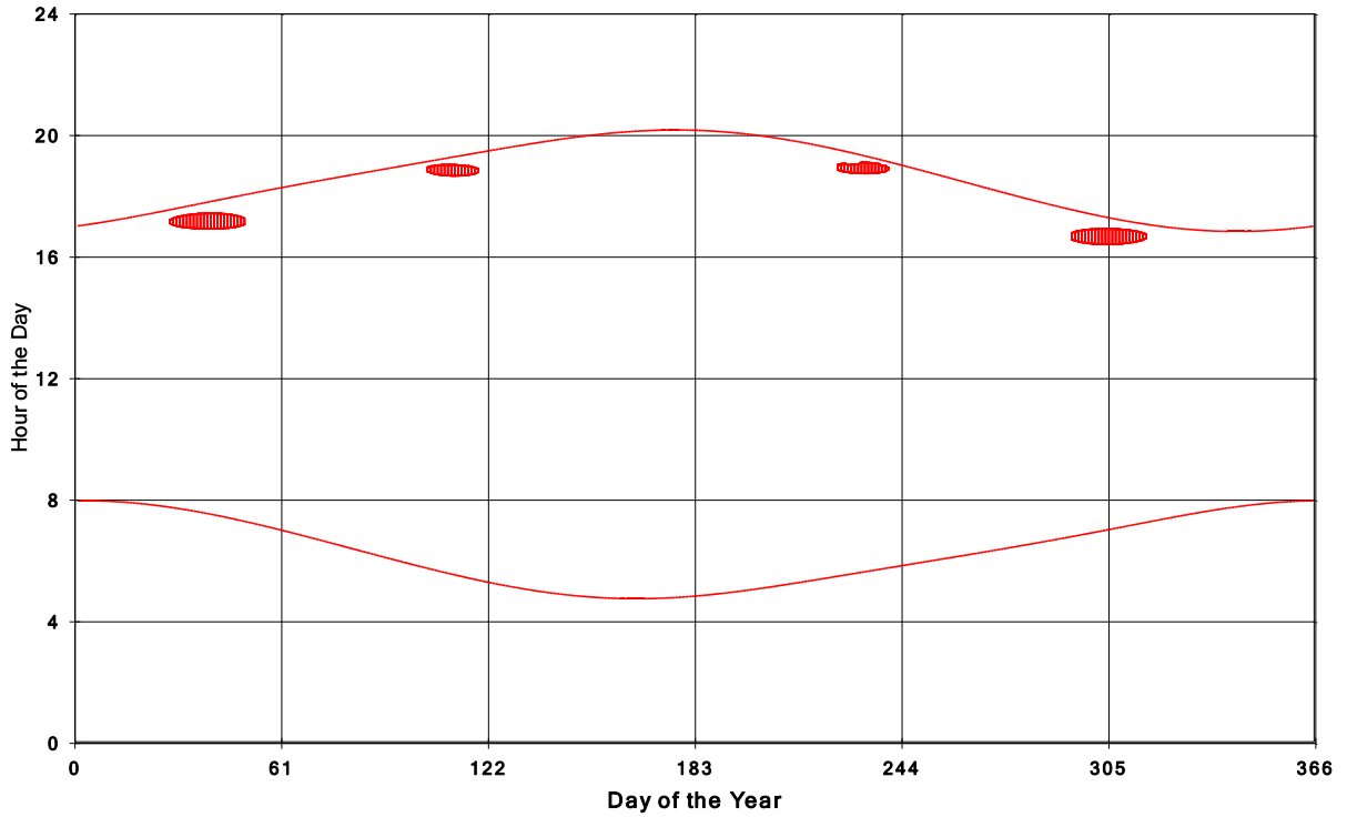
Goshen Wind Energy Centre Shadow Times on House 1018, All Windows from All Turbine
