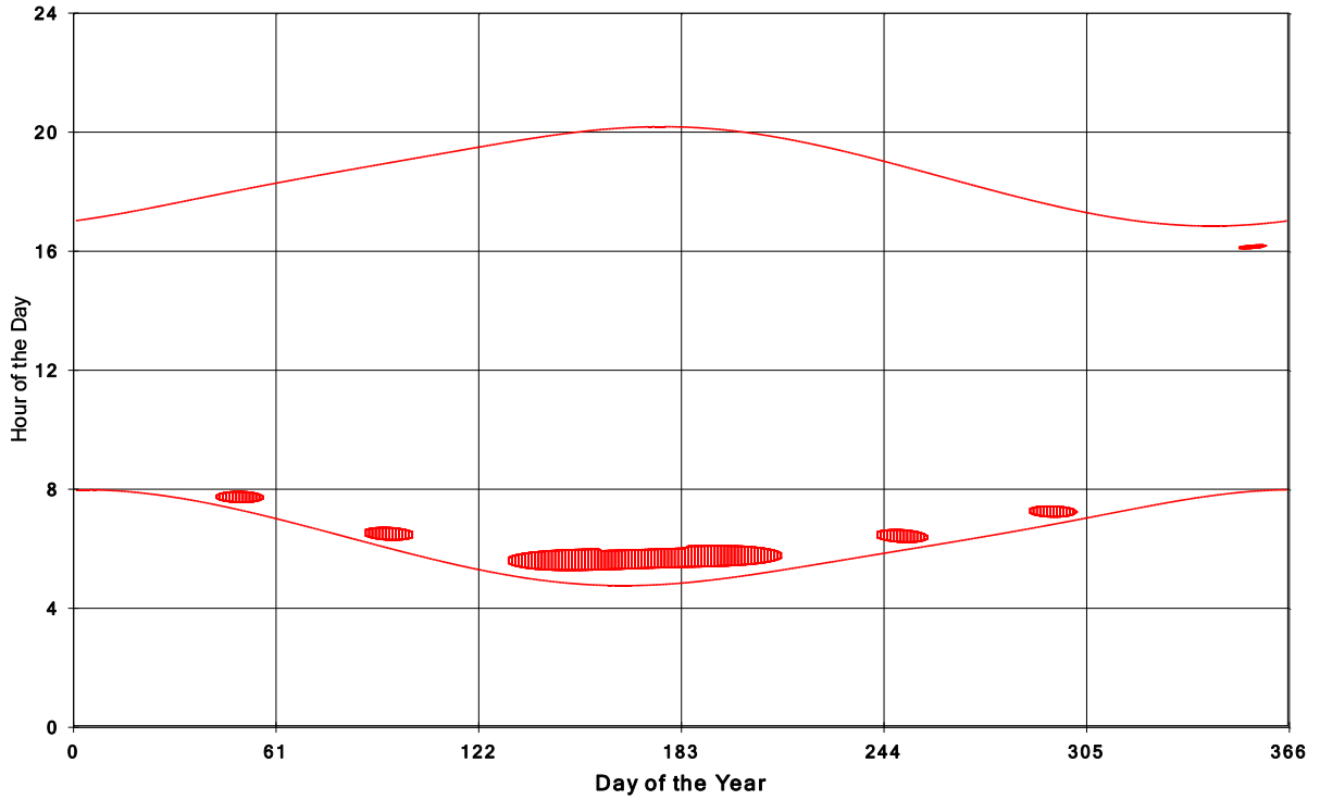
Goshen Wind Energy Centre Shadow Times on House 1163, All Windows from All Turbine
