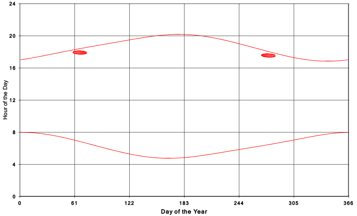
Goshen Wind Energy Centre Shadow Times on House 1012, All Windows from All Turbine
