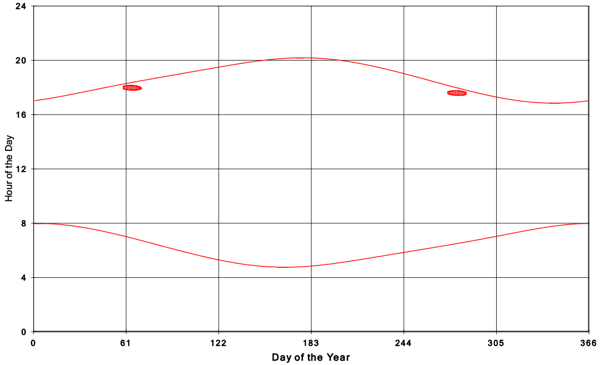
Goshen Wind Energy Centre Shadow Times on House 1097, All Windows from All Turbine
