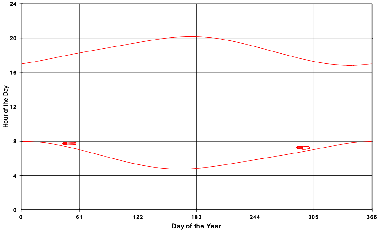
Goshen Wind Energy Centre Shadow Times on House 1026, All Windows from All Turbine
