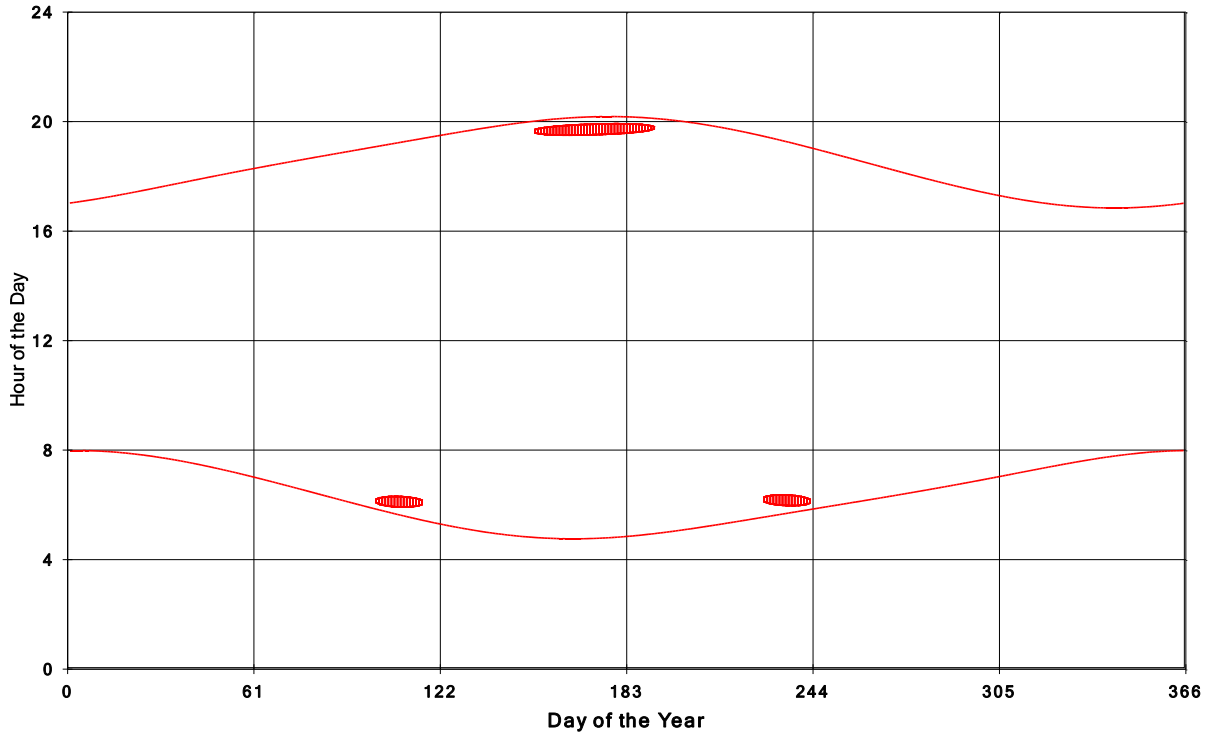
Goshen Wind Energy Centre Shadow Times on House 1158, All Windows from All Turbine
