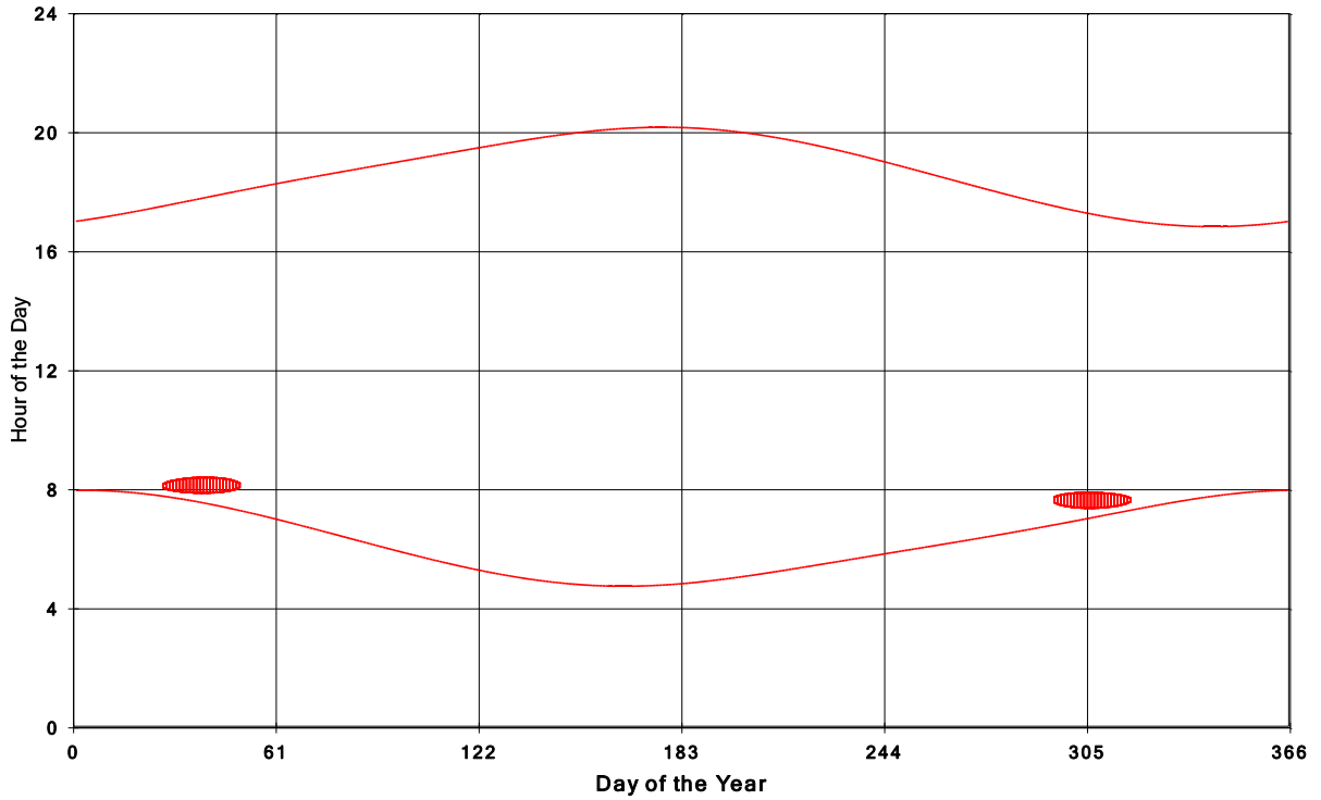
Goshen Wind Energy Centre Shadow Times on House 1008, All Windows from All Turbine
