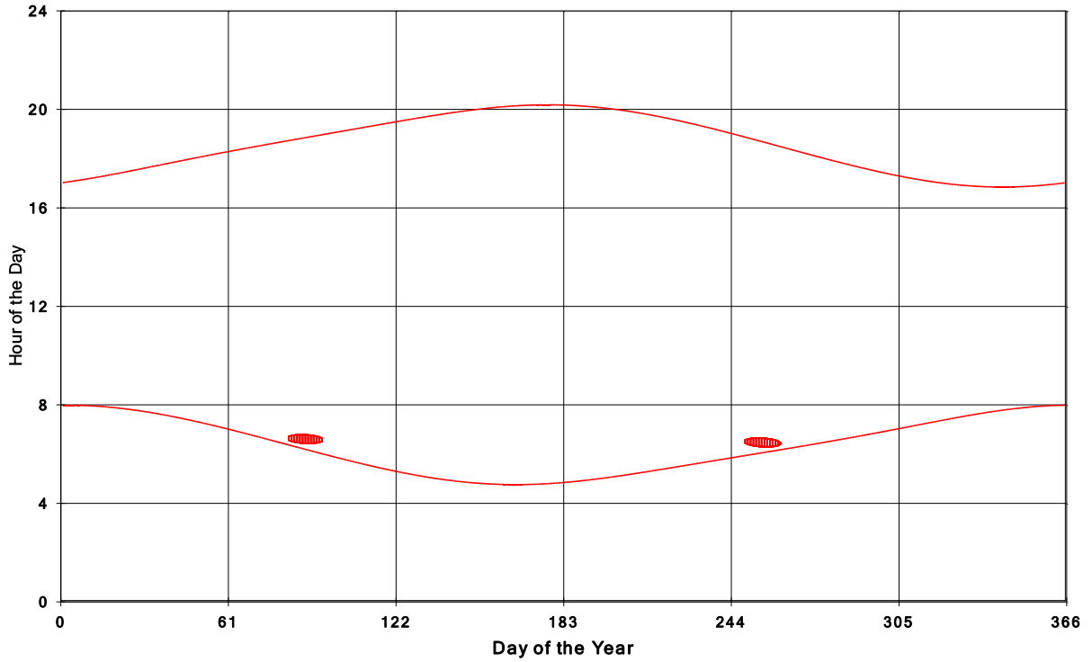
Goshen Wind Energy Centre Shadow Times on House 1137, All Windows from All Turbine
