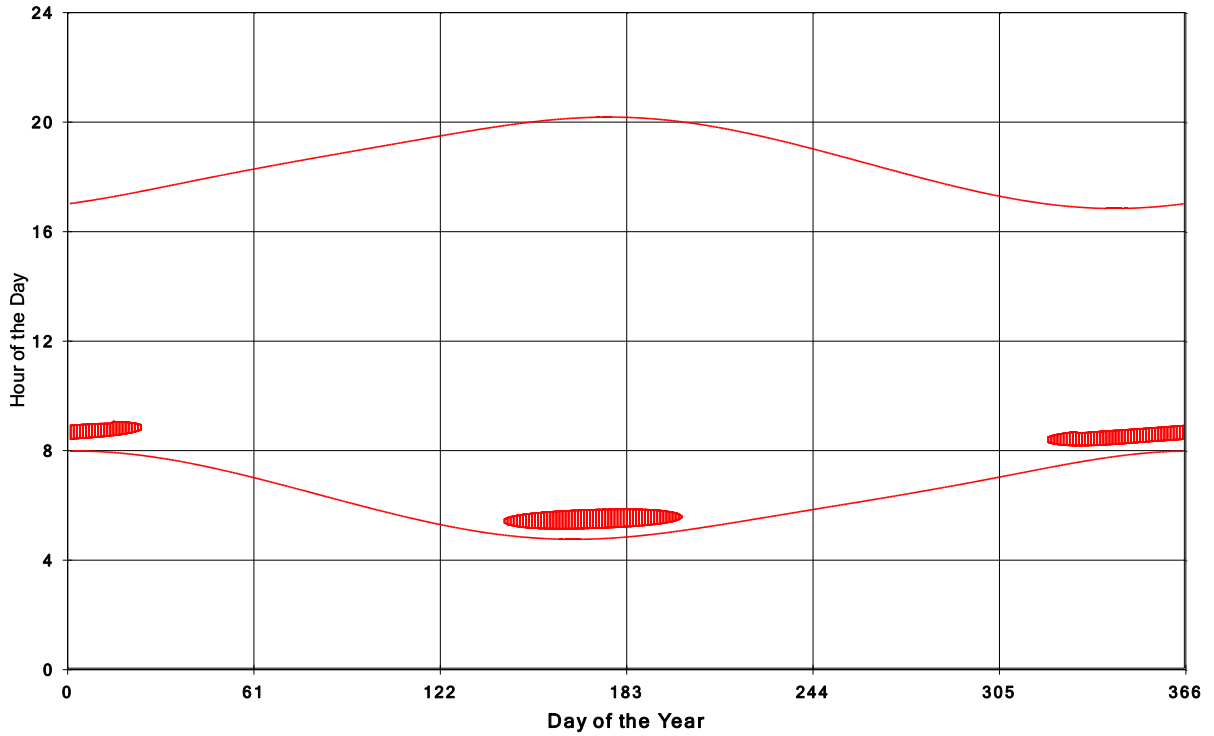
Goshen Wind Energy Centre Shadow Times on House 1049, All Windows from All Turbine
