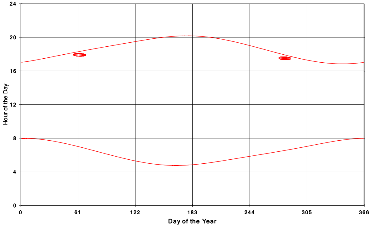
Goshen Wind Energy Centre Shadow Times on House 1095, All Windows from All Turbine
