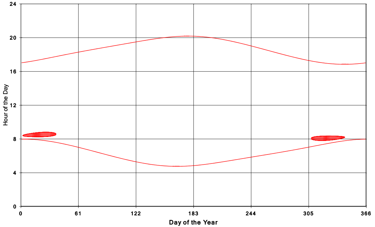
Goshen Wind Energy Centre Shadow Times on House 1149, All Windows from All Turbine
