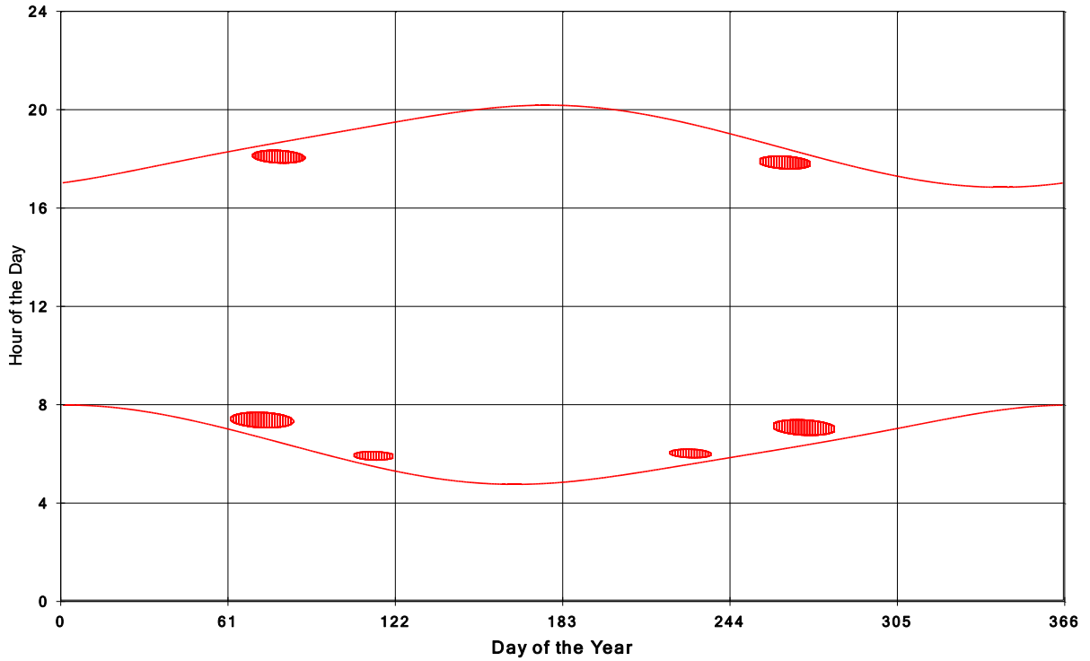
Goshen Wind Energy Centre Shadow Times on House 1165, All Windows from All Turbine
