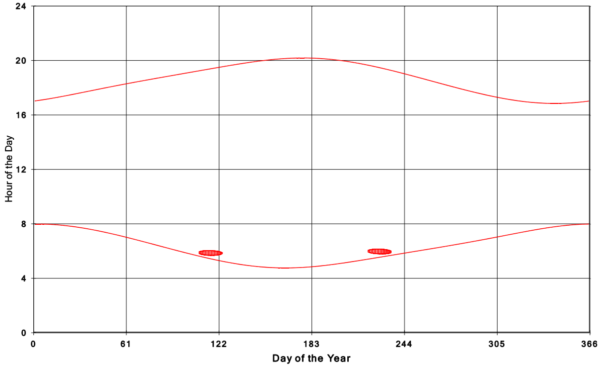
Goshen Wind Energy Centre Shadow Times on House 1033, All Windows from All Turbine
