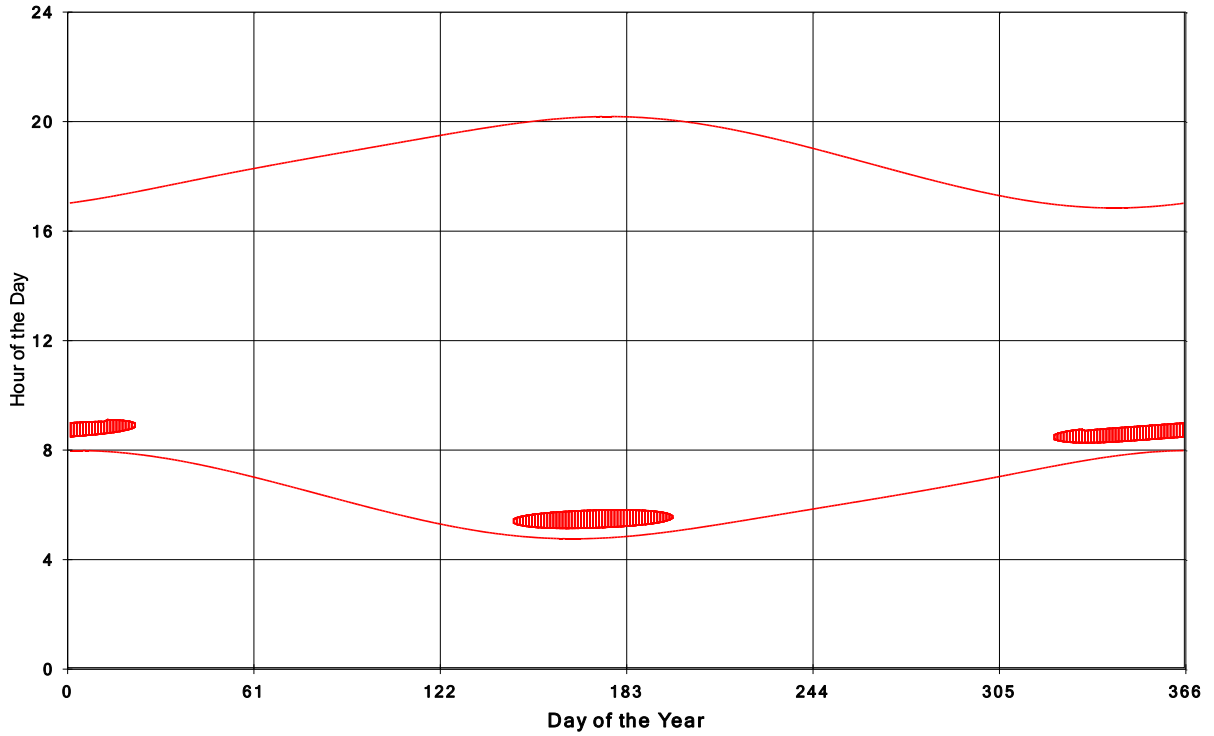
Goshen Wind Energy Centre Shadow Times on House 1050, All Windows from All Turbine
