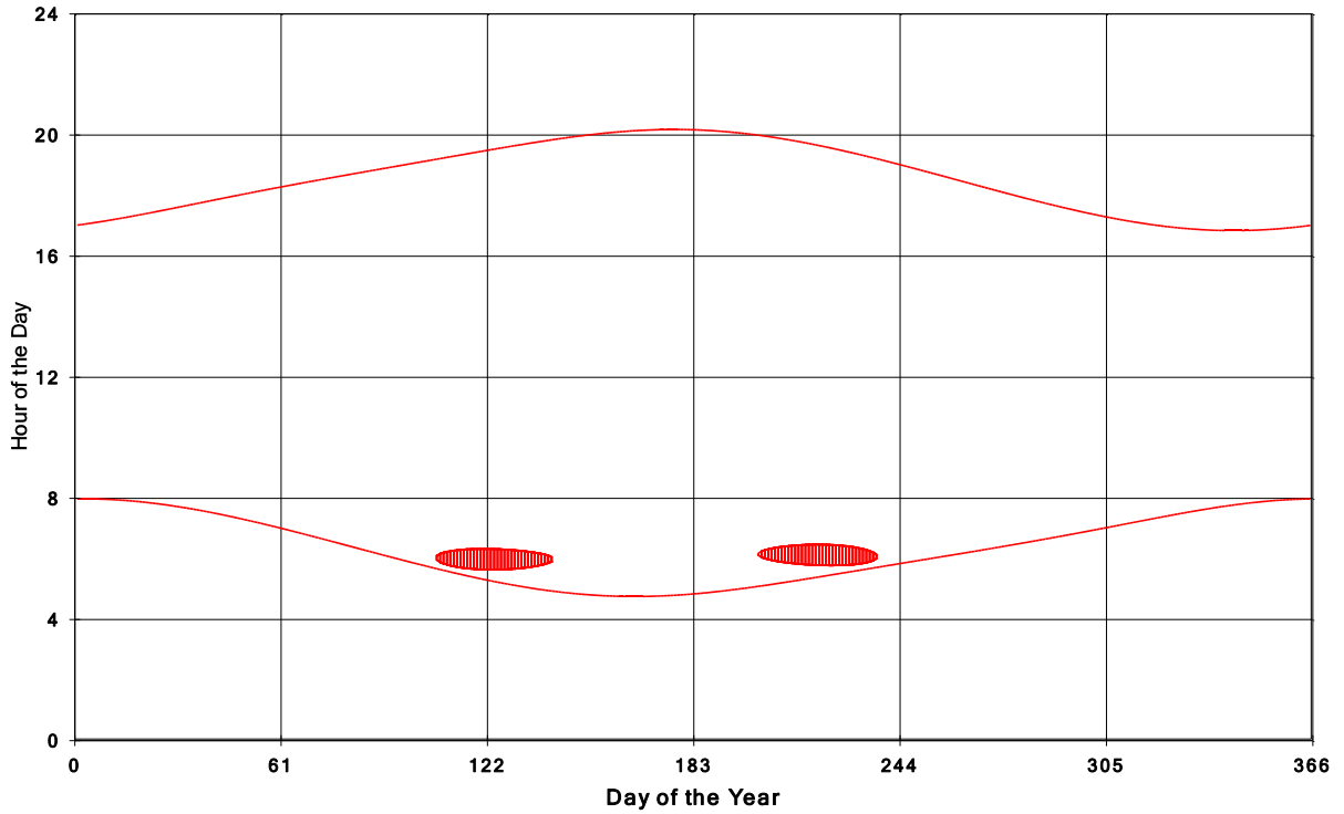
Goshen Wind Energy Centre Shadow Times on House 1024, All Windows from All Turbine
