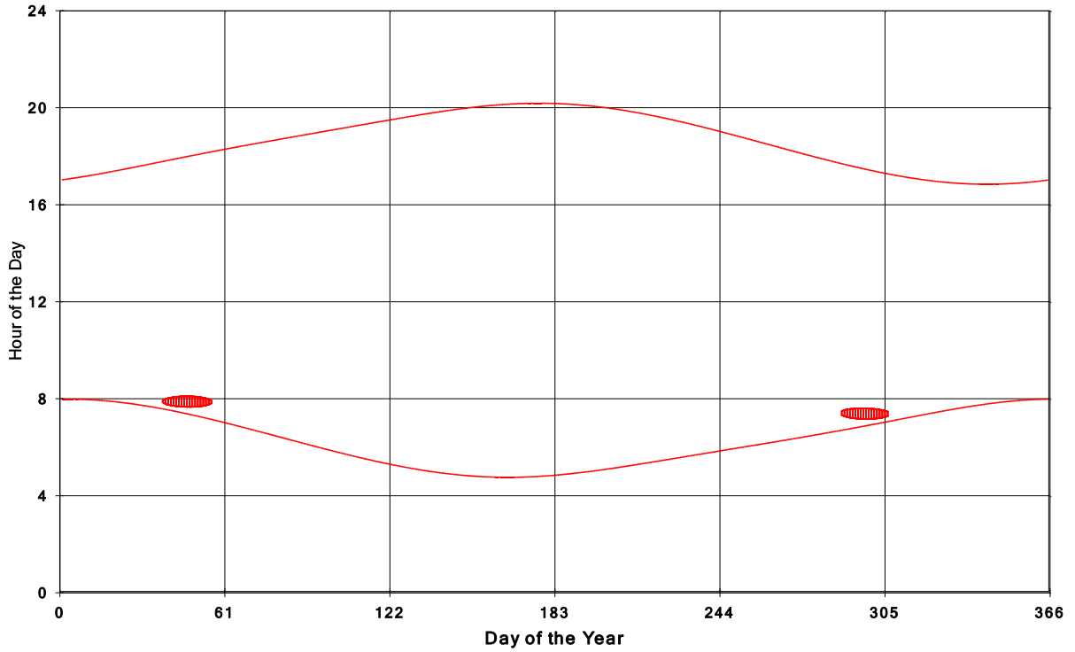
Goshen Wind Energy Centre Shadow Times on House 1007, All Windows from All Turbine
