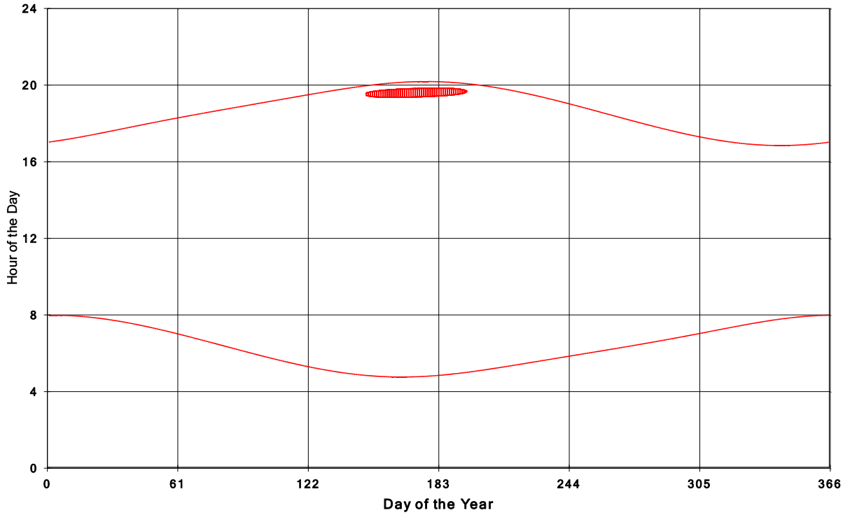
Goshen Wind Energy Centre Shadow Times on House 1057, All Windows from All Turbine
