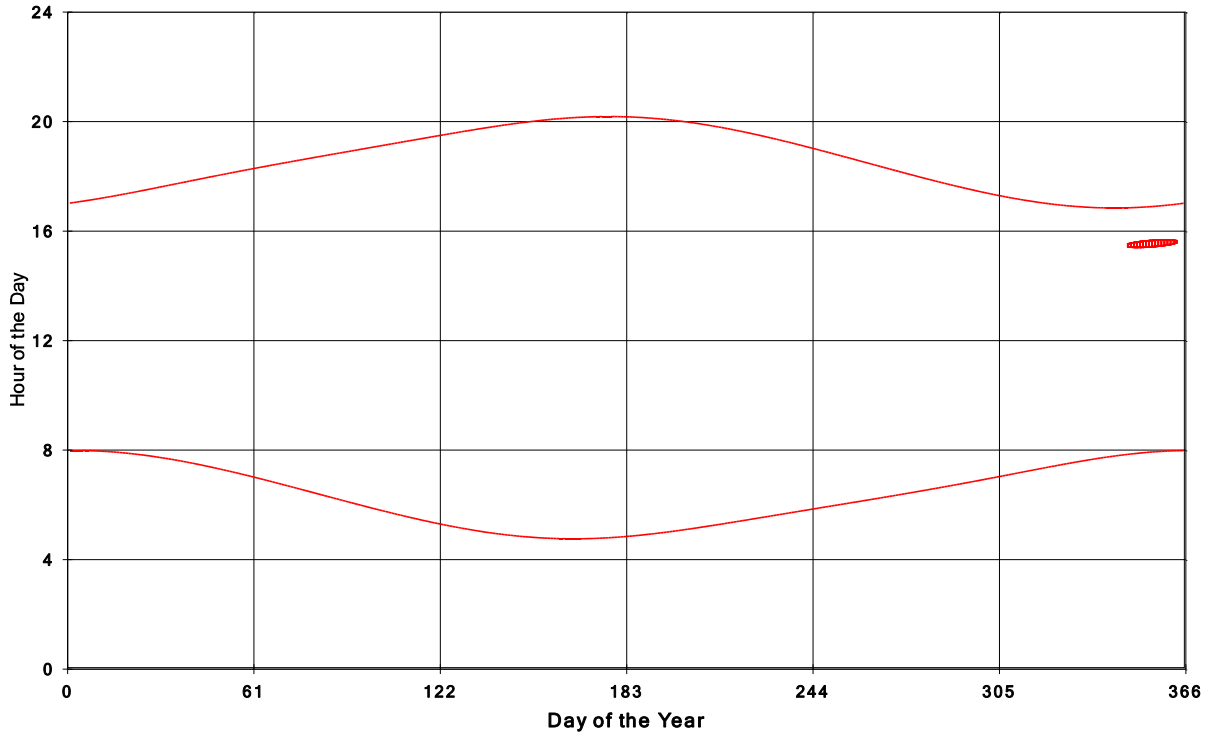
Goshen Wind Energy Centre Shadow Times on House 1028, All Windows from All Turbine
