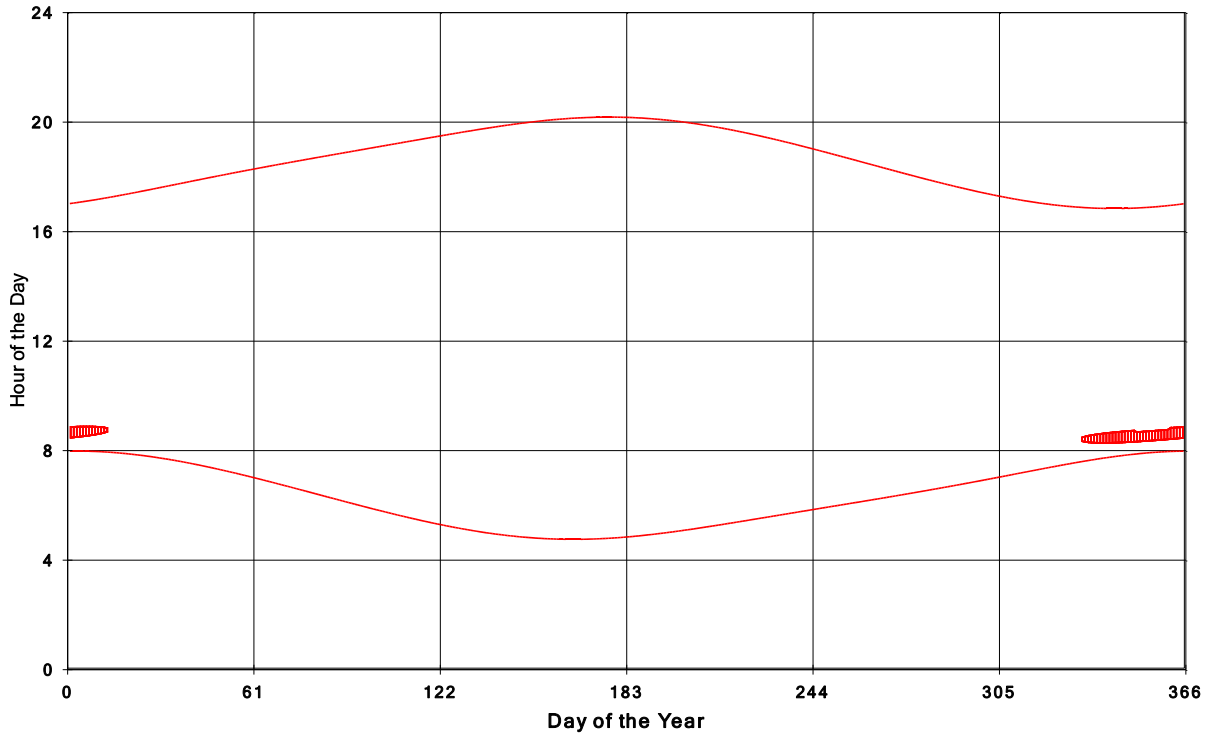
Goshen Wind Energy Centre Shadow Times on House 1119, All Windows from All Turbine
