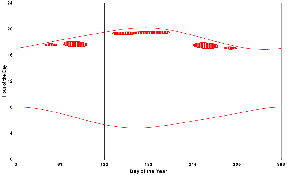
Goshen Wind Energy Centre Shadow Times on House 1015, All Windows from All Turbine
