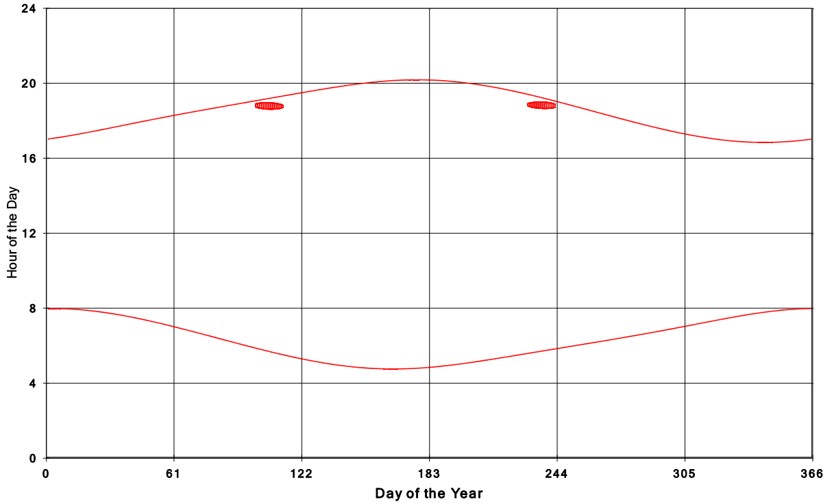
Goshen Wind Energy Centre Shadow Times on House 1001, All Windows from All Turbine
