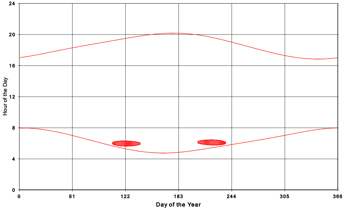
Goshen Wind Energy Centre Shadow Times on House 1023, All Windows from All Turbine
