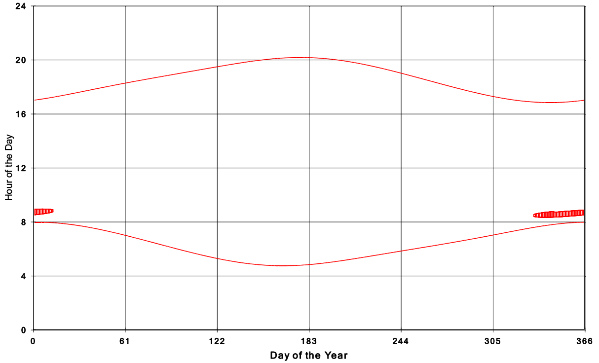
Goshen Wind Energy Centre Shadow Times on House 1121, All Windows from All Turbine
