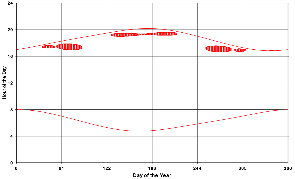
Goshen Wind Energy Centre Shadow Times on House 1014, All Windows from All Turbine
