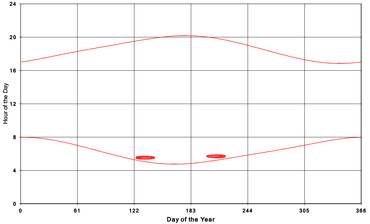
Goshen Wind Energy Centre Shadow Times on House 1124, All Windows from All Turbine
