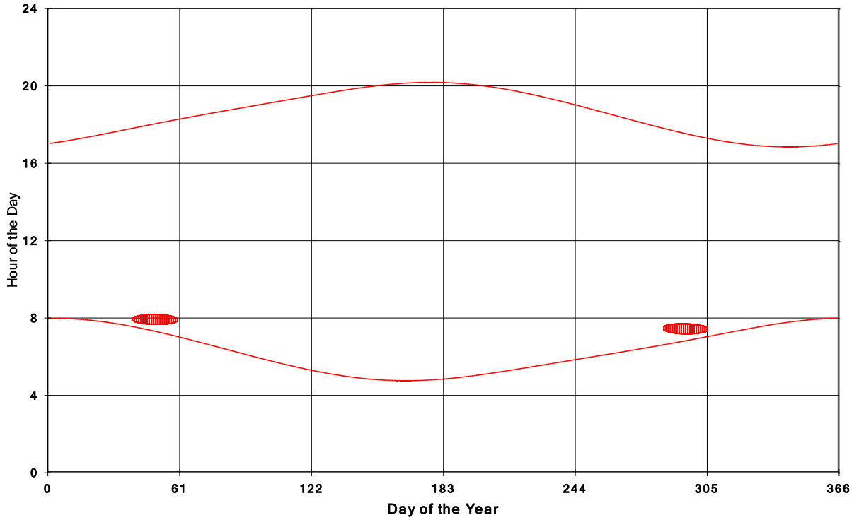
Goshen Wind Energy Centre Shadow Times on House 1123, All Windows from All Turbine
