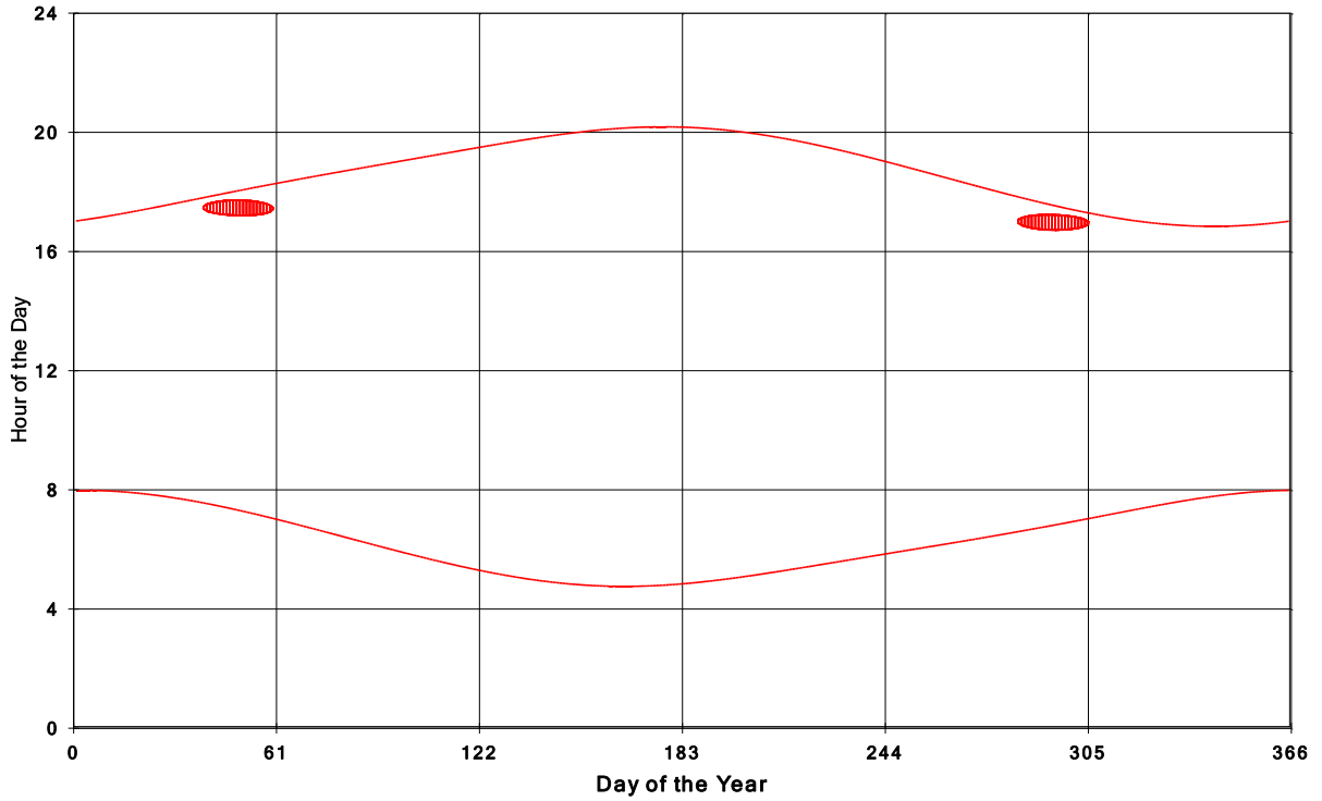
Goshen Wind Energy Centre Shadow Times on House 1036, All Windows from All Turbine
