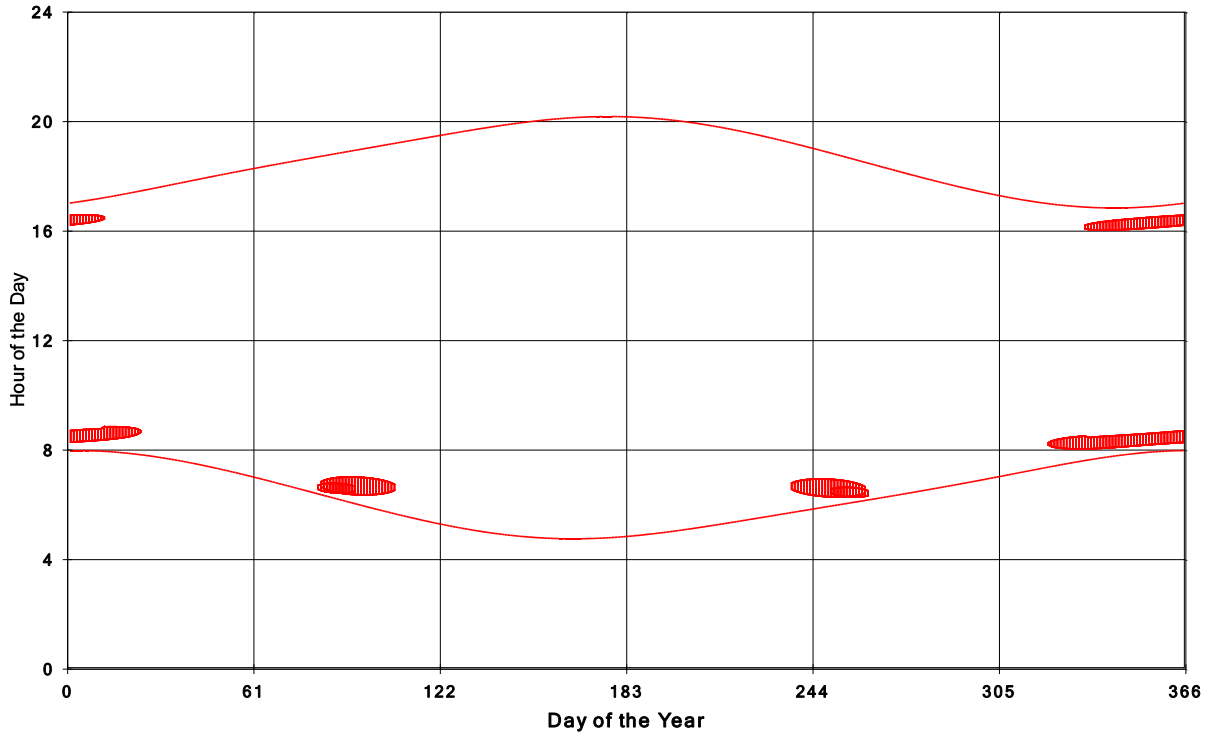
Goshen Wind Energy Centre Shadow Times on House 995, All Windows from All Turbine:
