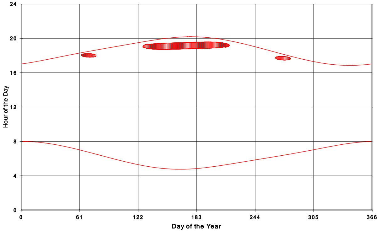
Goshen Wind Energy Centre Shadow Times on House 1002, All Windows from All Turbine
