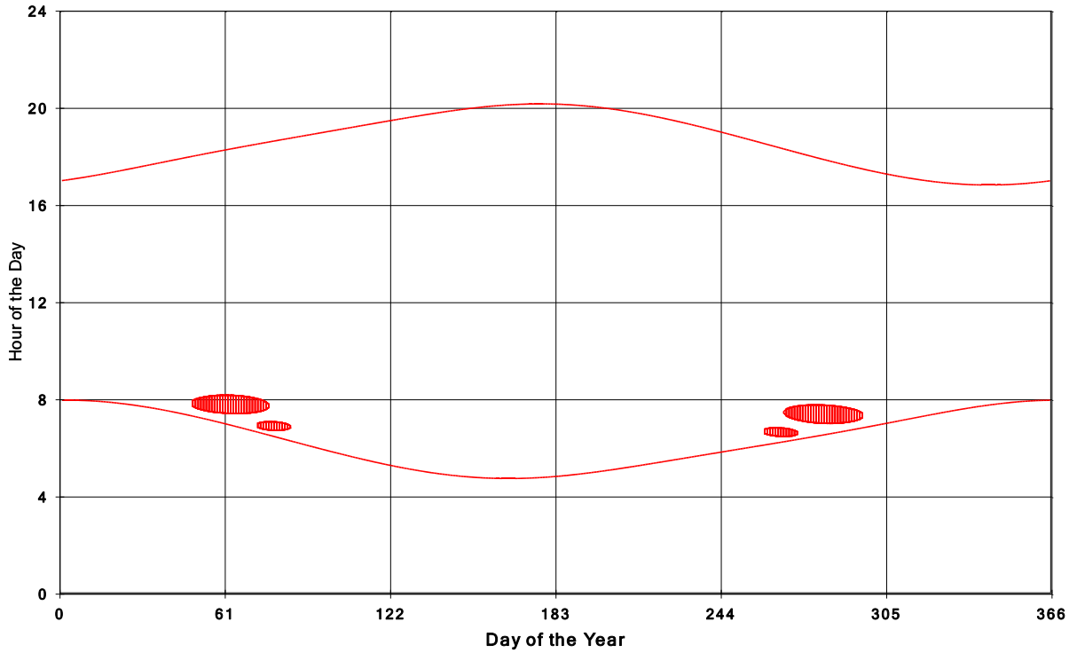
Goshen Wind Energy Centre Shadow Times on House 1051, All Windows from All Turbine
