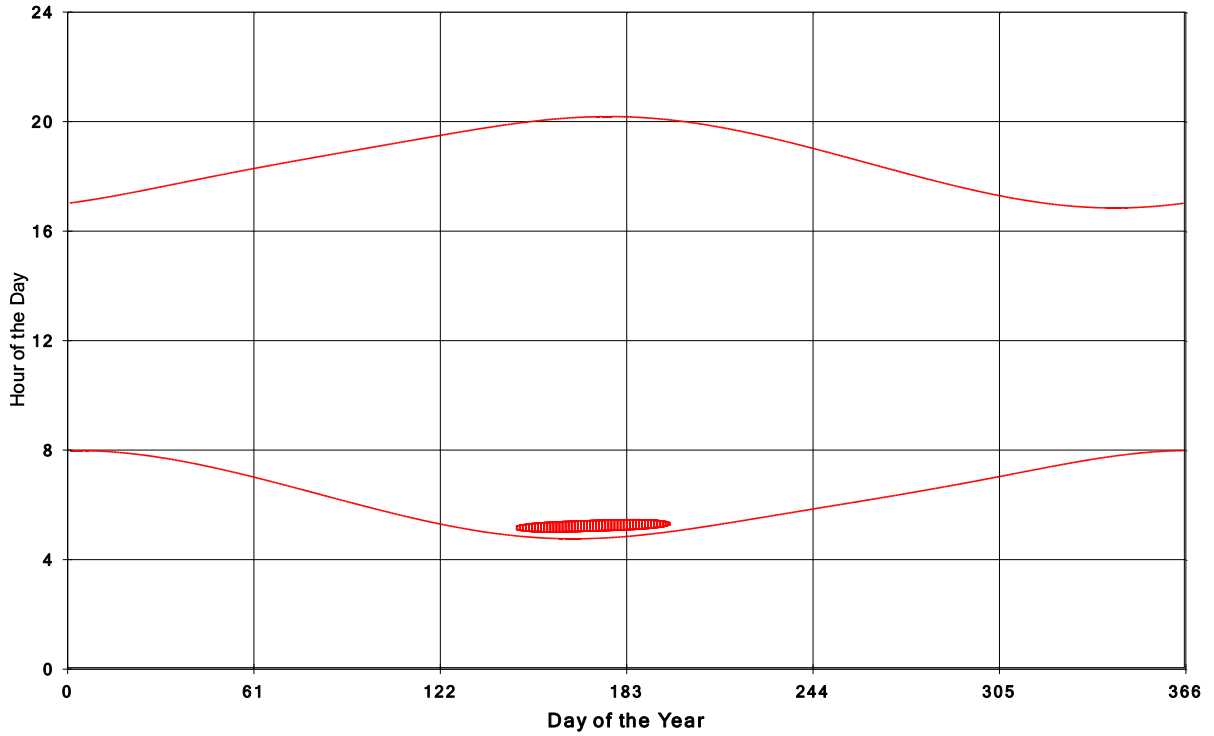
Goshen Wind Energy Centre Shadow Times on House 1054, All Windows from All Turbine
