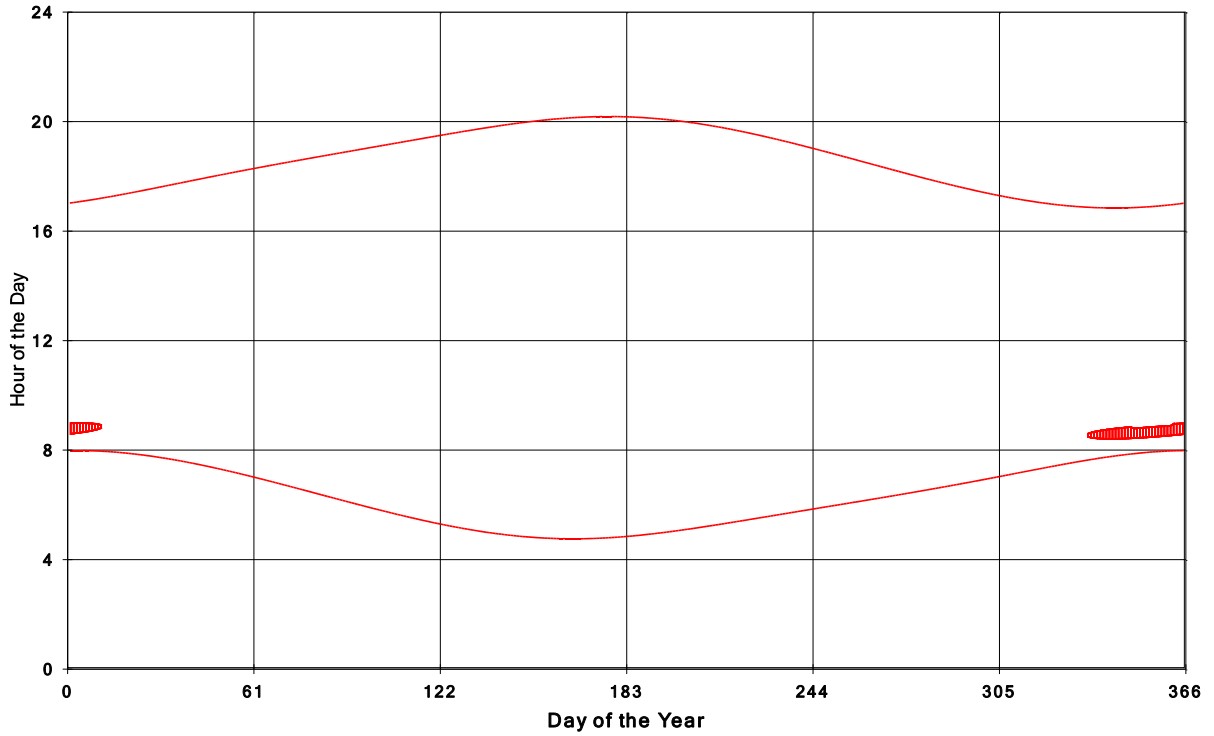
Goshen Wind Energy Centre Shadow Times on House 1140, All Windows from All Turbine
