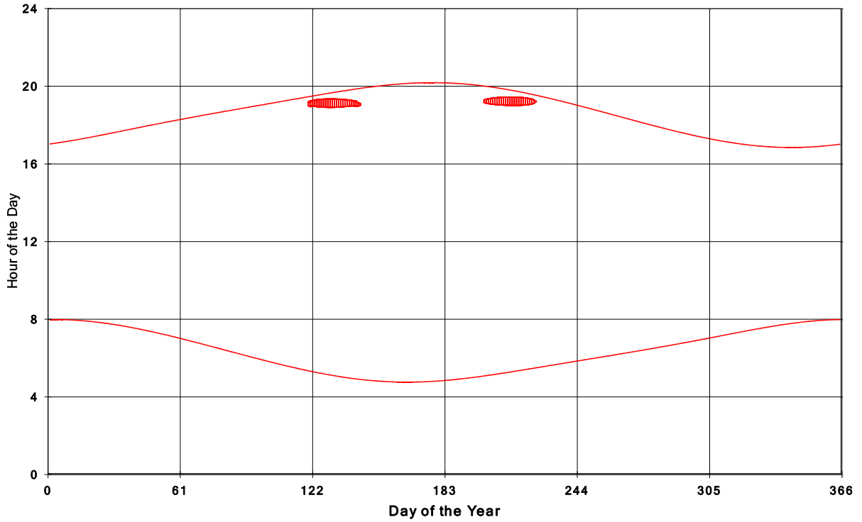
Goshen Wind Energy Centre Shadow Times on House 1038, All Windows from All Turbine
