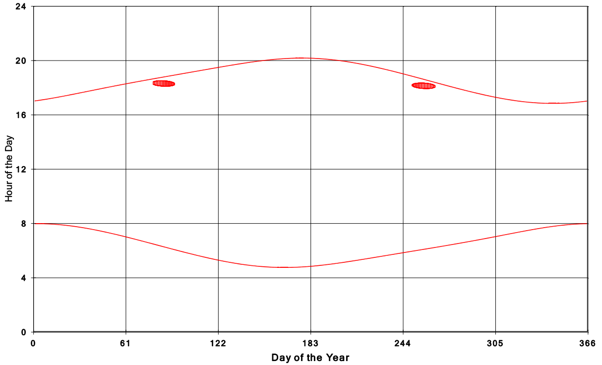
Goshen Wind Energy Centre Shadow Times on House 1139, All Windows from All Turbine
