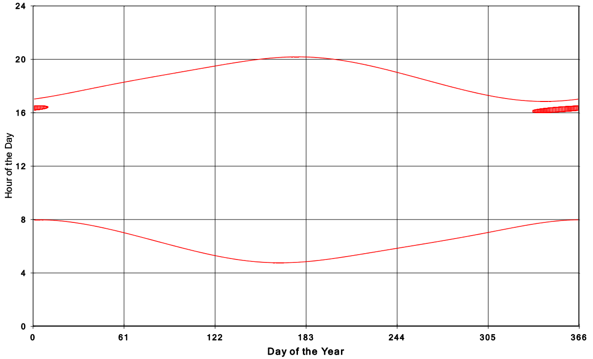
Goshen Wind Energy Centre Shadow Times on House 1046, All Windows from All Turbine
