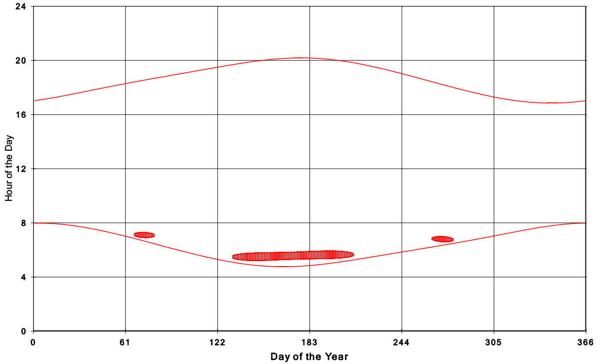
Goshen Wind Energy Centre Shadow Times on House 1132, All Windows from All Turbine
