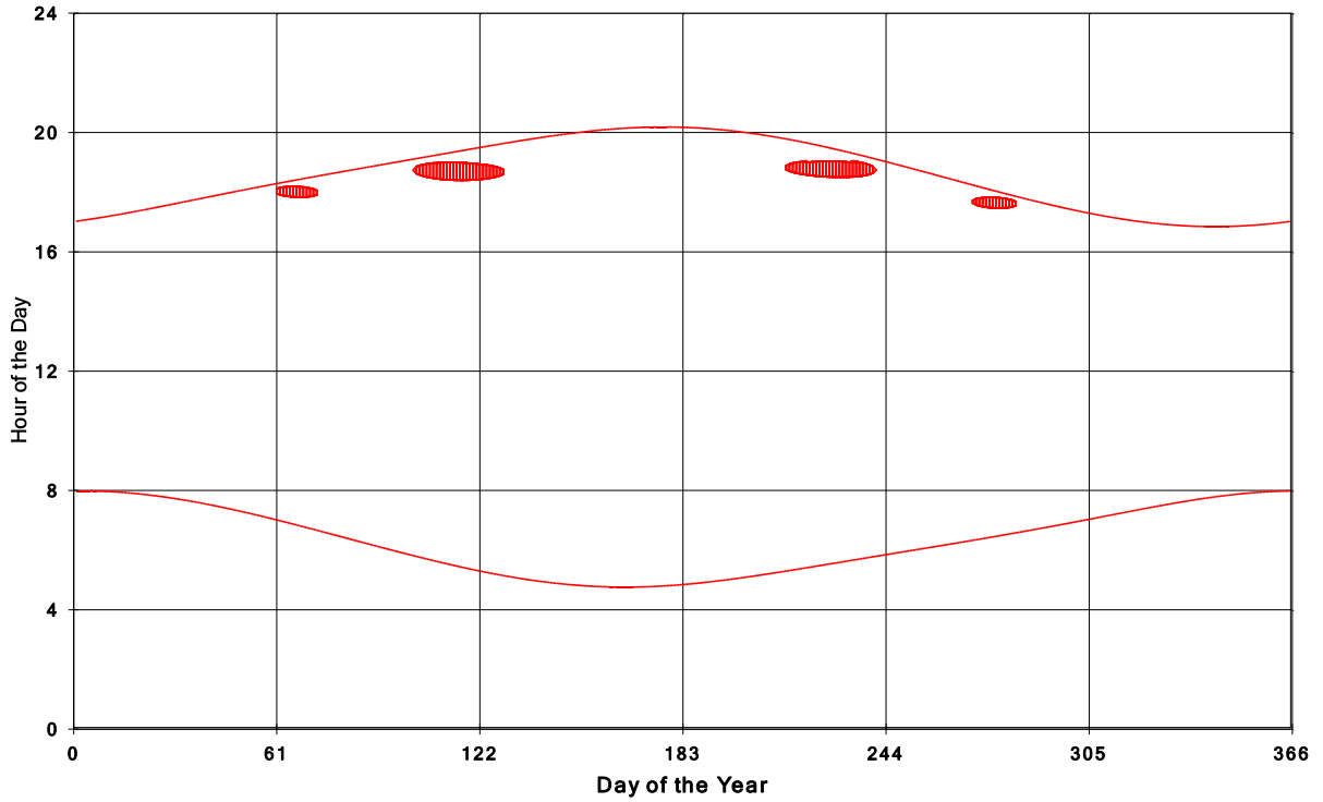
Goshen Wind Energy Centre Shadow Times on House 1003, All Windows from All Turbine
