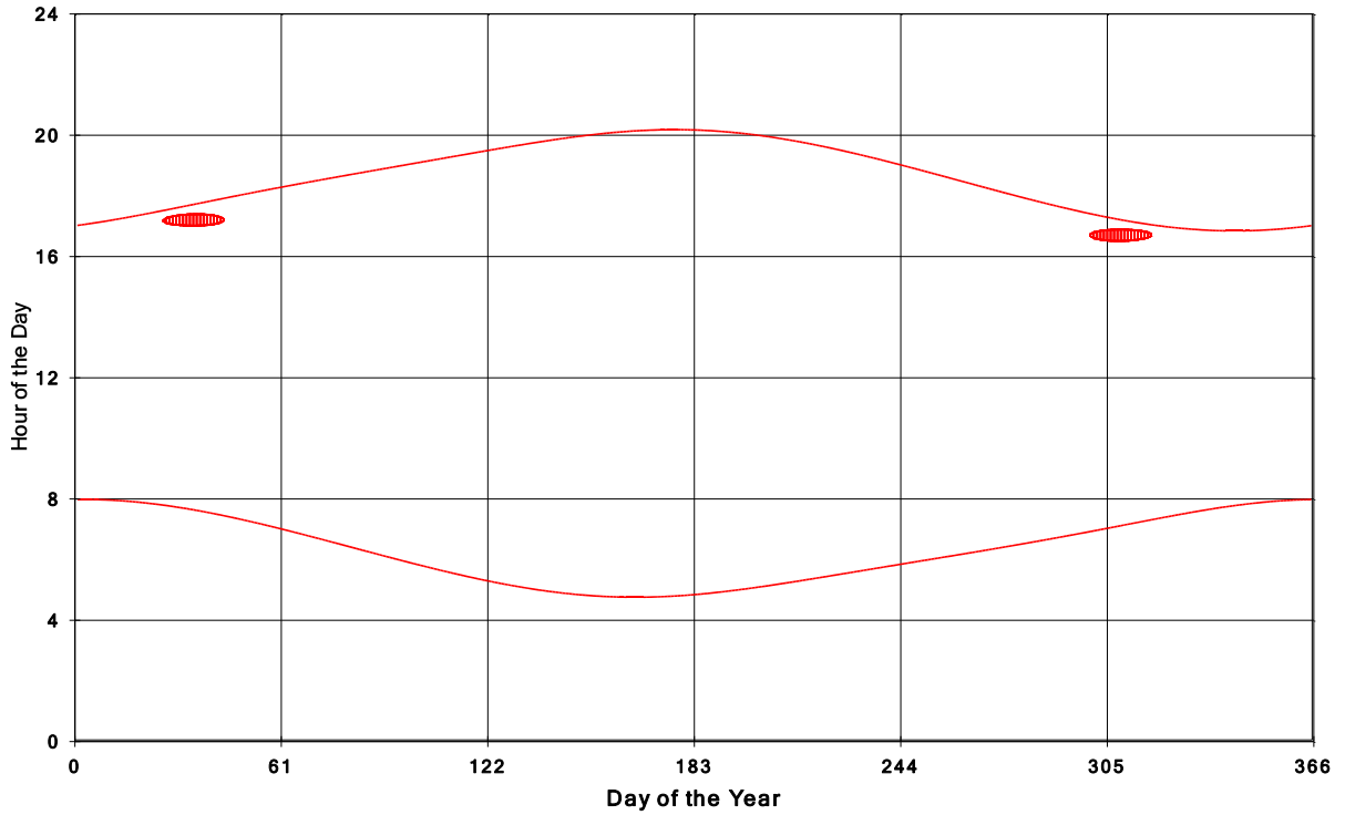
Goshen Wind Energy Centre Shadow Times on House 1134, All Windows from All Turbine
