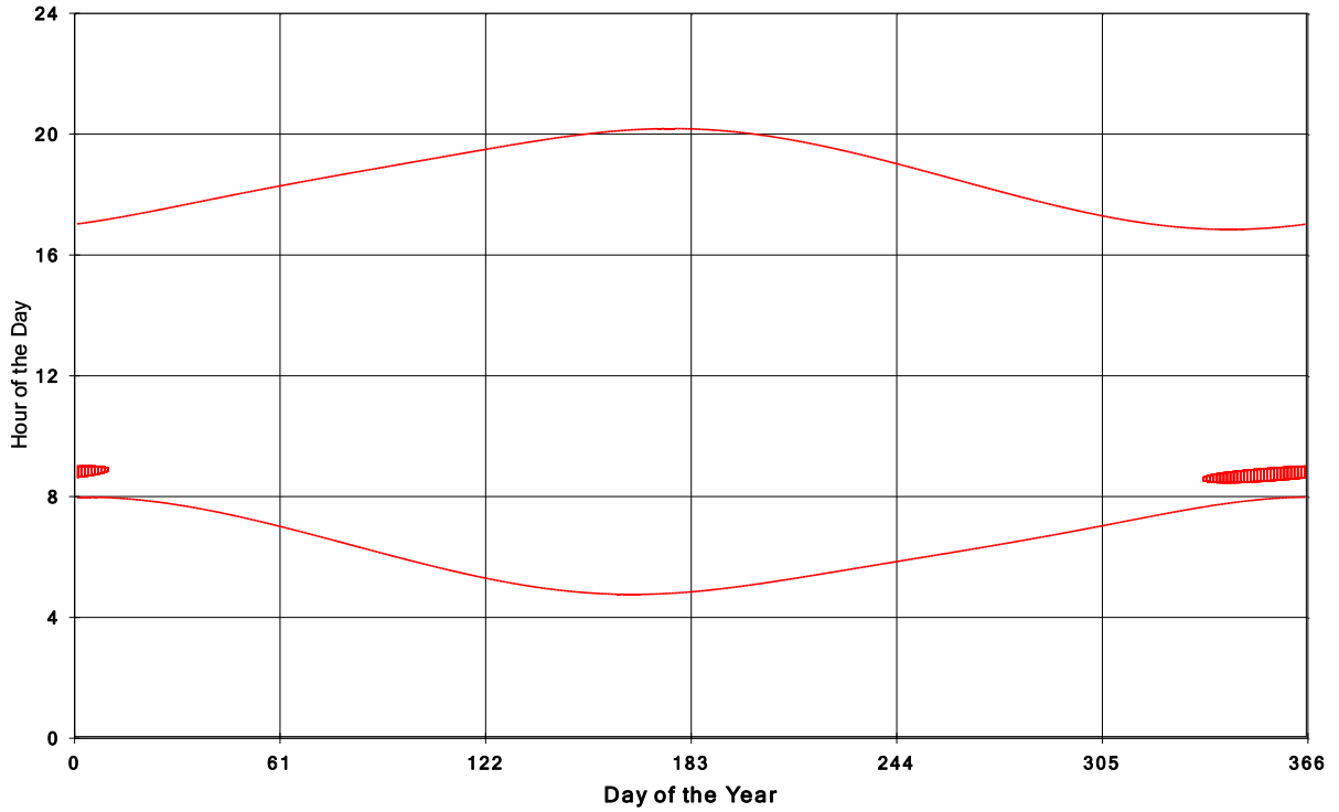
Goshen Wind Energy Centre Shadow Times on House 1150, All Windows from All Turbine
