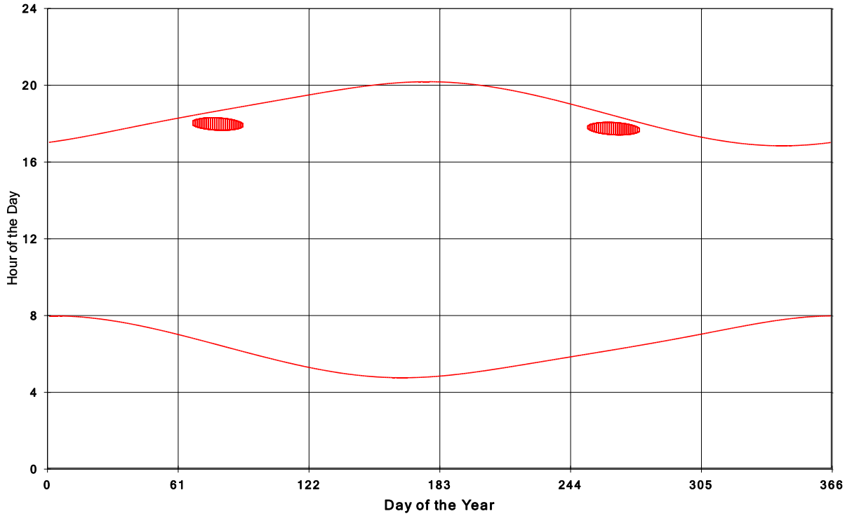
Goshen Wind Energy Centre Shadow Times on House 1160, All Windows from All Turbine
