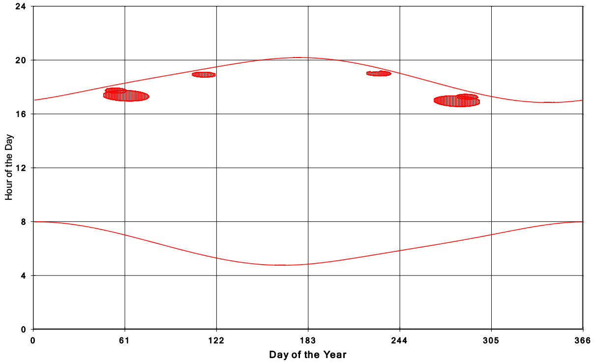
Goshen Wind Energy Centre Shadow Times on House 1016, All Windows from All Turbine
