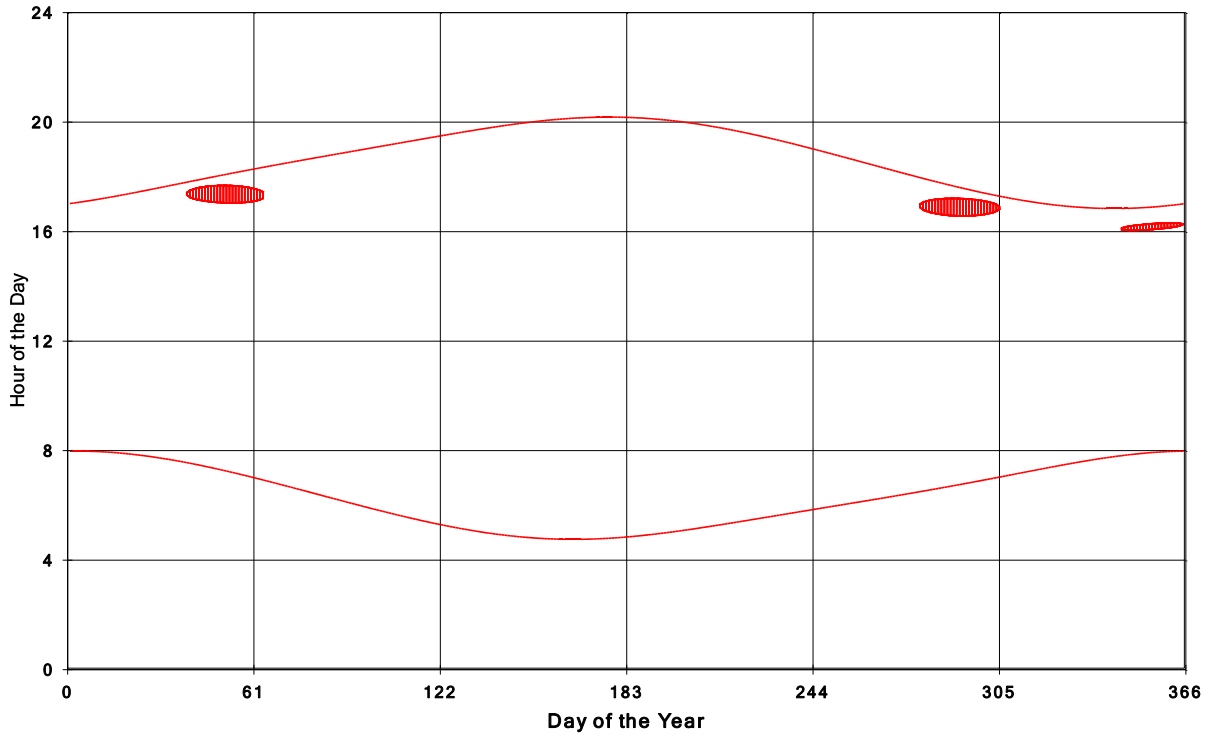
Goshen Wind Energy Centre Shadow Times on House 1031, All Windows from All Turbine
