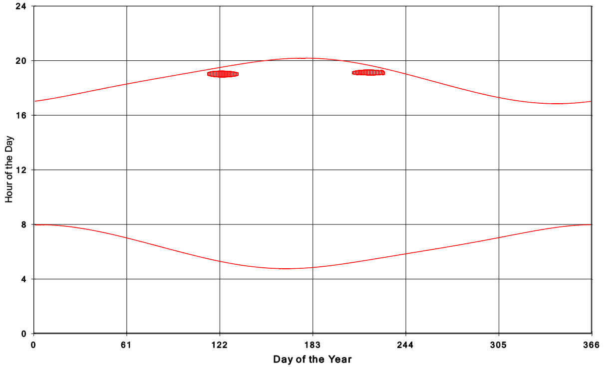
Goshen Wind Energy Centre Shadow Times on House 999, All Windows from All Turbine:
