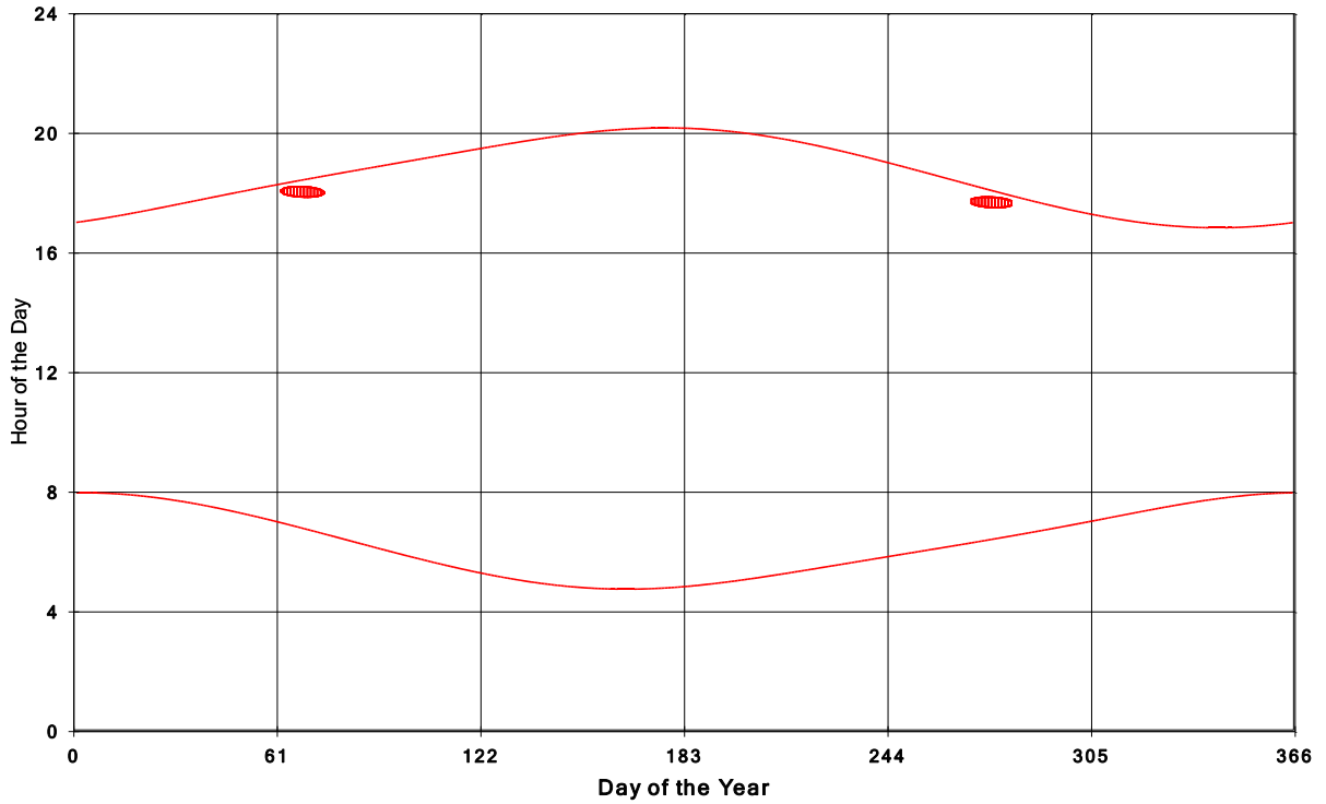
Goshen Wind Energy Centre Shadow Times on House 1096, All Windows from All Turbine
