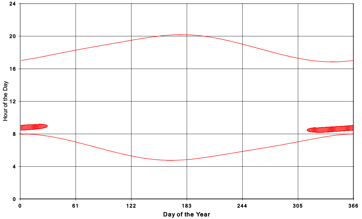
Goshen Wind Energy Centre Shadow Times on House 1135, All Windows from All Turbine
