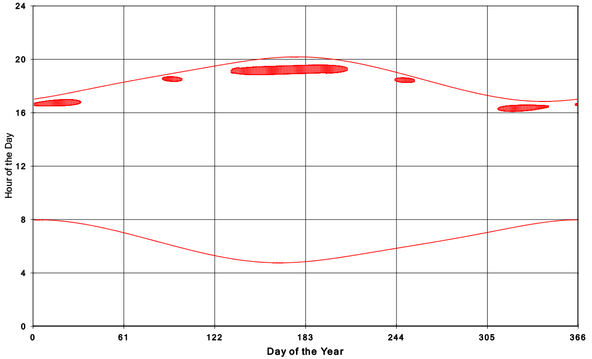
Goshen Wind Energy Centre Shadow Times on House 1017, All Windows from All Turbine
