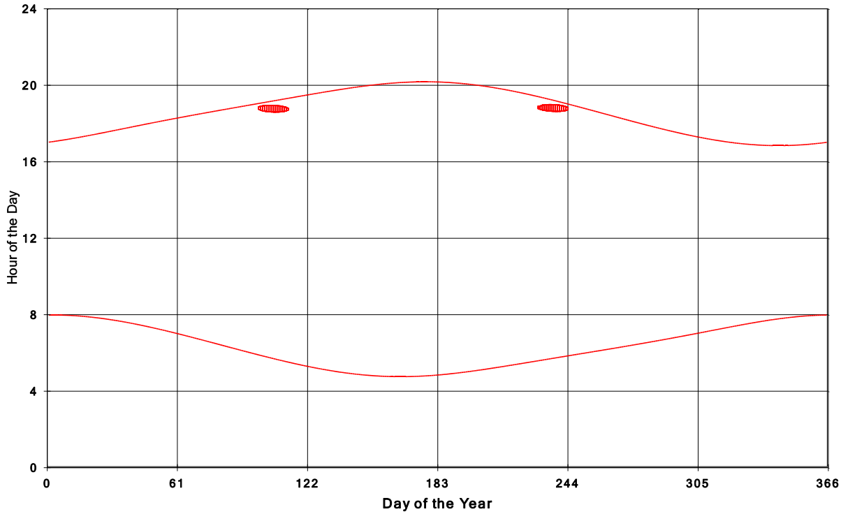
Goshen Wind Energy Centre Shadow Times on House 1000, All Windows from All Turbine:
