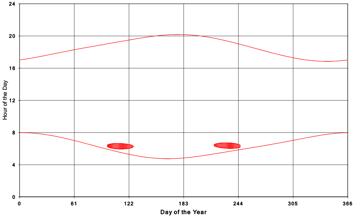
Jericho Wind Energy Centre Shadow Times on House 1141, All Windows from All Turbine
