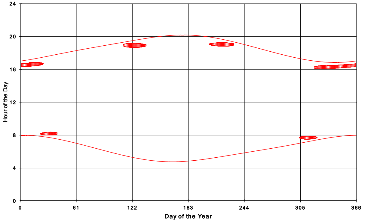
Goshen Wind Energy Centre Shadow Times on House 1131, All Windows from All Turbine
