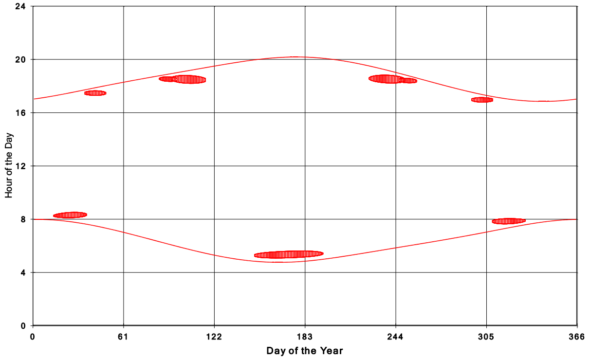
Goshen Wind Energy Centre Shadow Times on House 1034, All Windows from All Turbine
