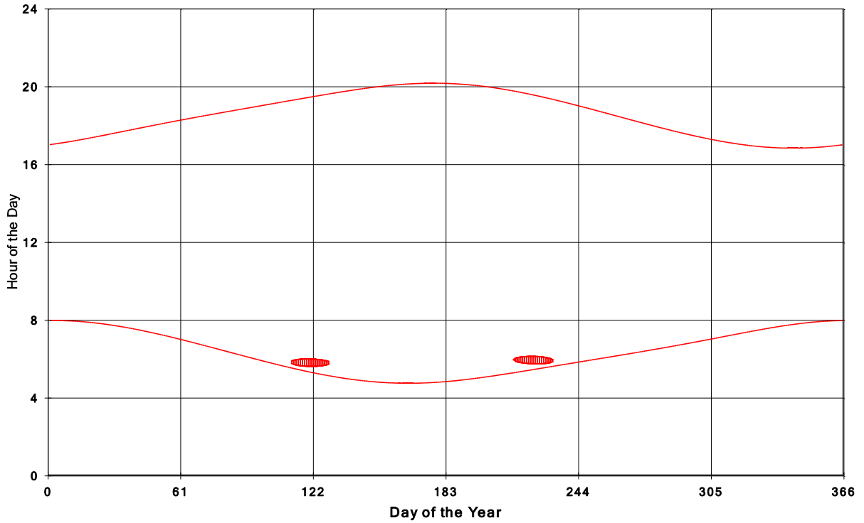
Goshen Wind Energy Centre Shadow Times on House 1159, All Windows from All Turbine
