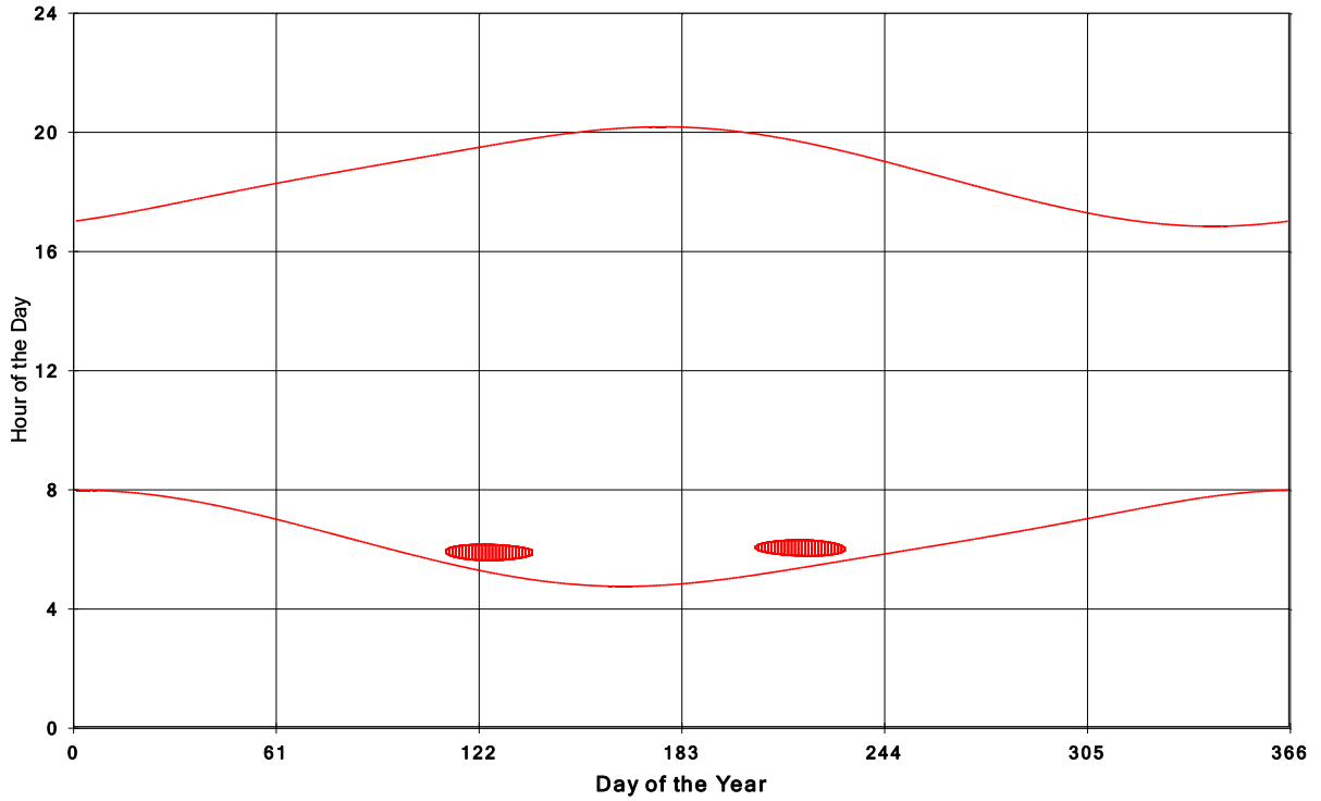
Goshen Wind Energy Centre Shadow Times on House 928, All Windows from All Turbine:
