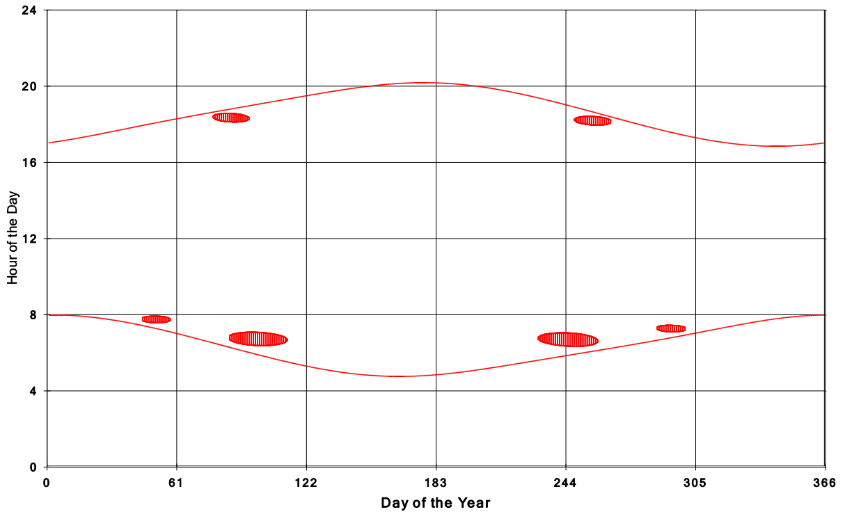
Goshen Wind Energy Centre Shadow Times on House 952, All Windows from All Turbine:
