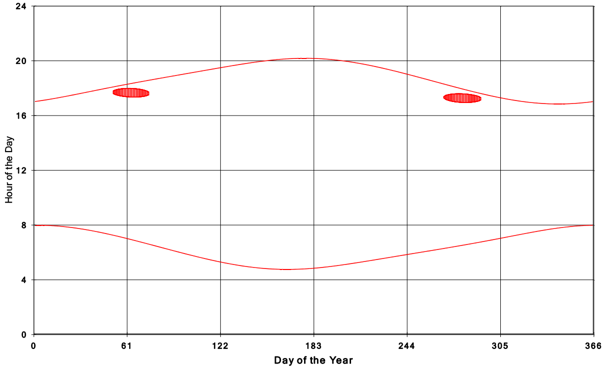
Goshen Wind Energy Centre Shadow Times on House 855, All Windows from All Turbine:
