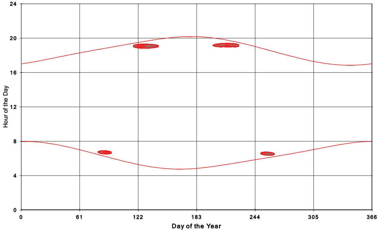
Goshen Wind Energy Centre Shadow Times on House 907, All Windows from All Turbine:
