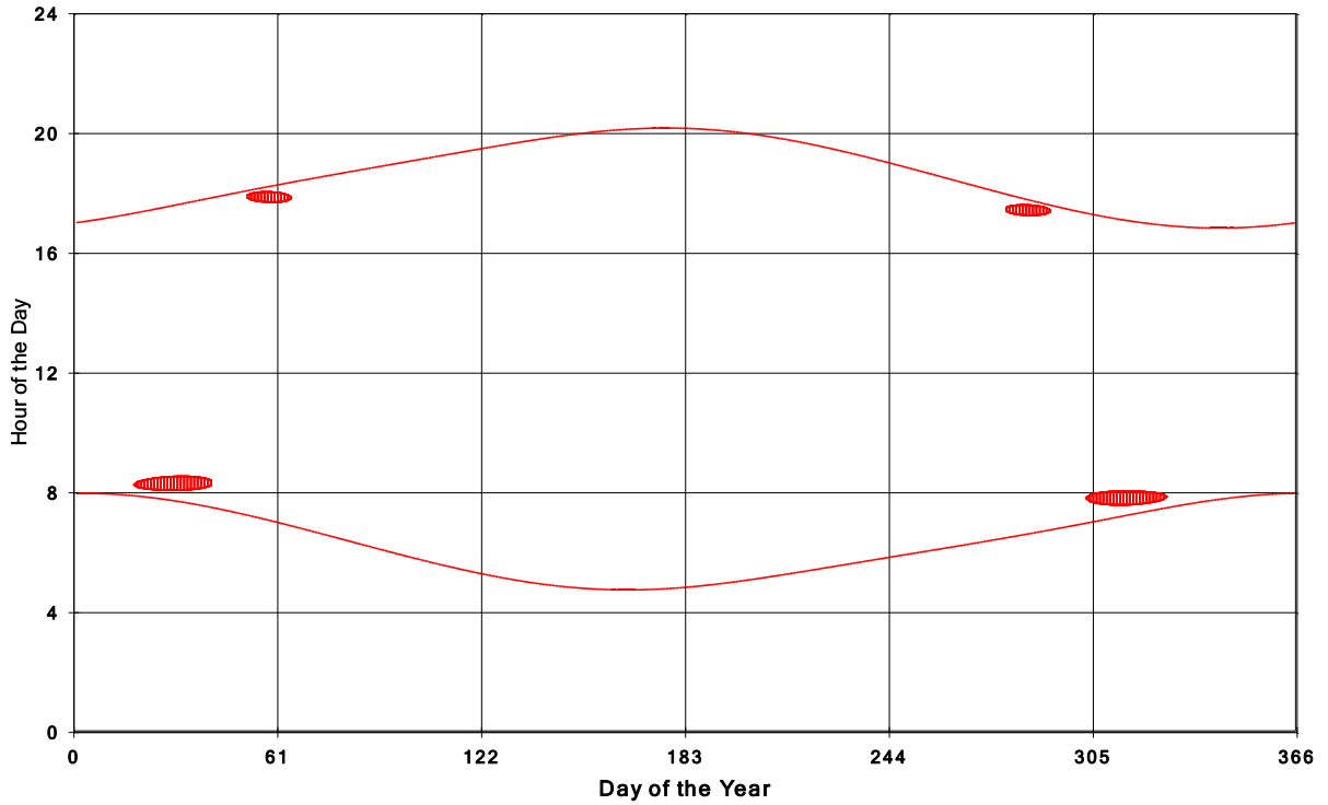
Goshen Wind Energy Centre Shadow Times on House 861, All Windows from All Turbine:
