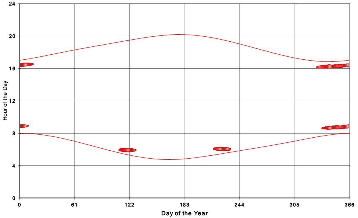
Jericho Wind Energy Centre Shadow Times on House 951, All Windows from All Turbine:
