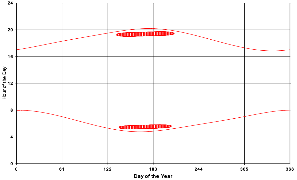
Goshen Wind Energy Centre Shadow Times on House 905, All Windows from All Turbine:
