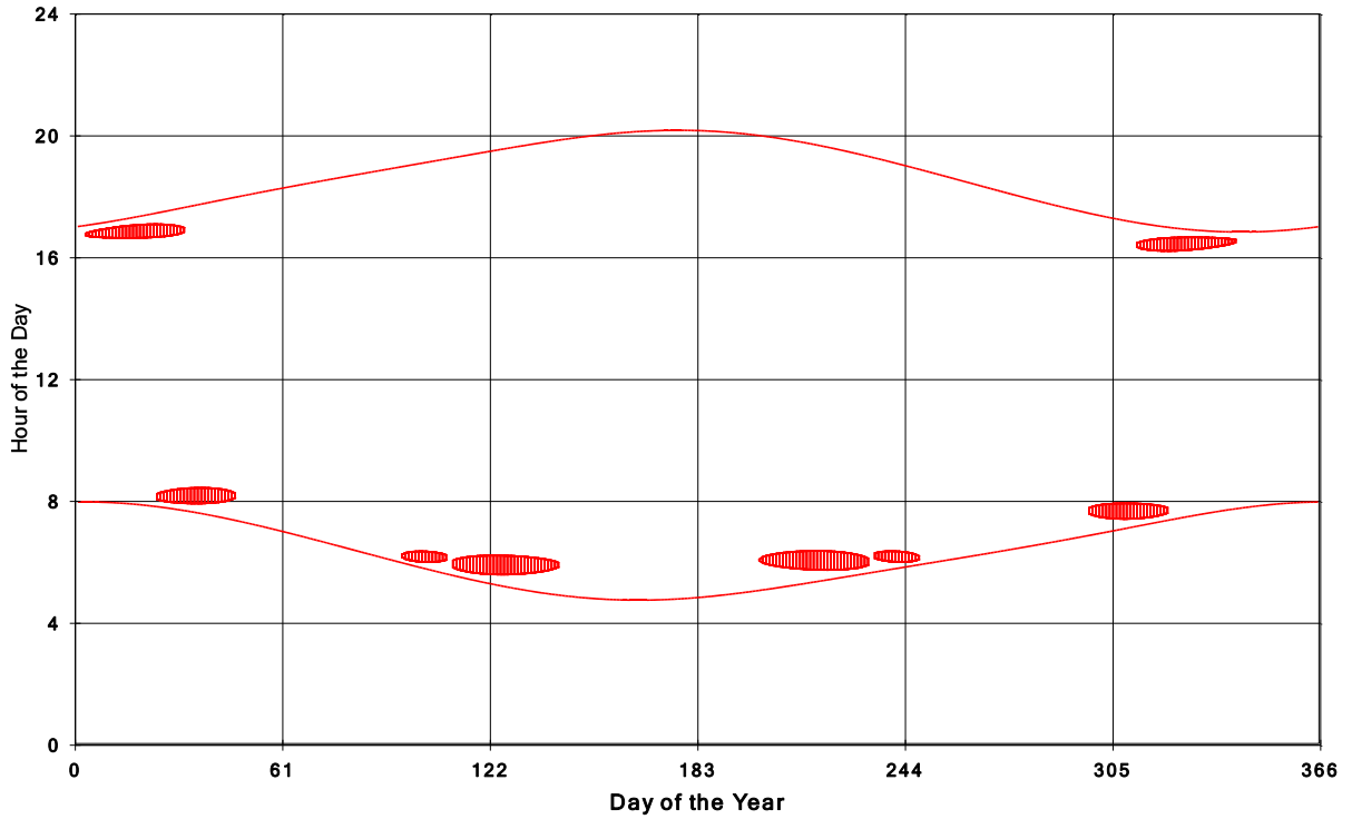
Goshen Wind Energy Centre Shadow Times on House 872, All Windows from All Turbine:
