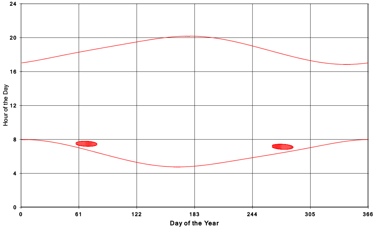
Goshen Wind Energy Centre Shadow Times on House 924, All Windows from All Turbine:
