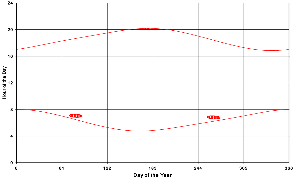
Goshen Wind Energy Centre Shadow Times on House 959, All Windows from All Turbine:
