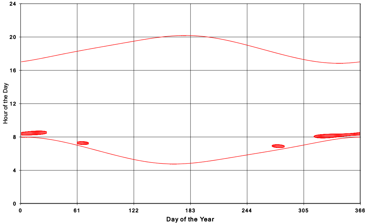
Goshen Wind Energy Centre Shadow Times on House 880, All Windows from All Turbine:
