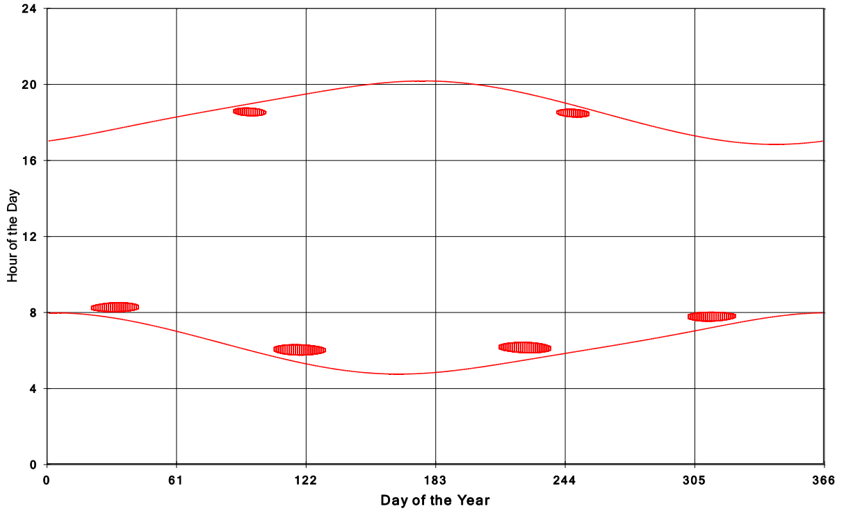
Goshen Wind Energy Centre Shadow Times on House 842, All Windows from All Turbine:
