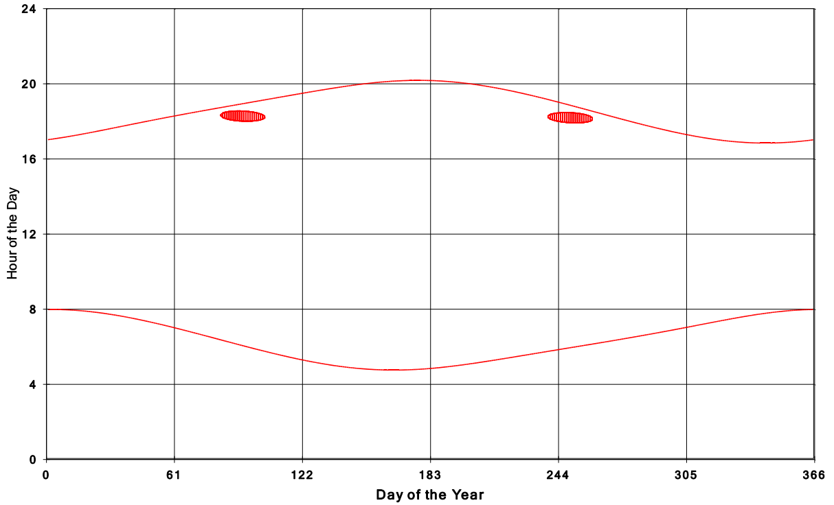
Goshen Wind Energy Centre Shadow Times on House 835, All Windows from All Turbine:
