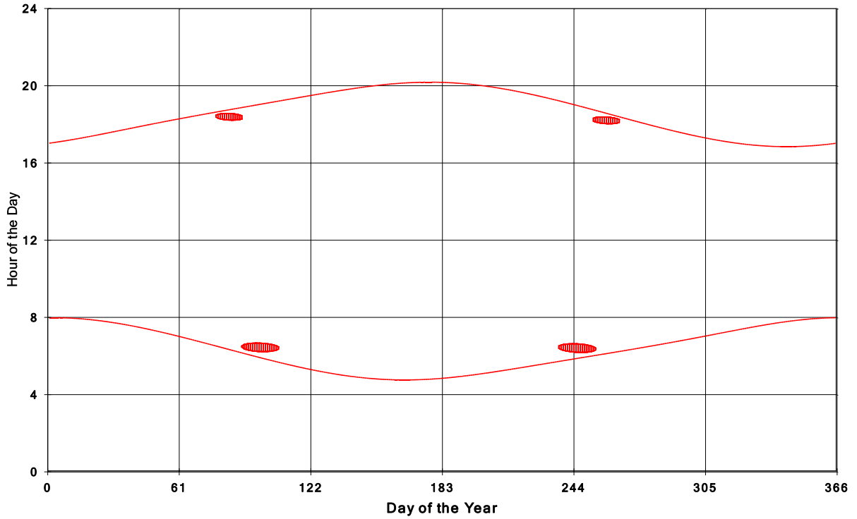
Goshen Wind Energy Centre Shadow Times on House 985, All Windows from All Turbine:
