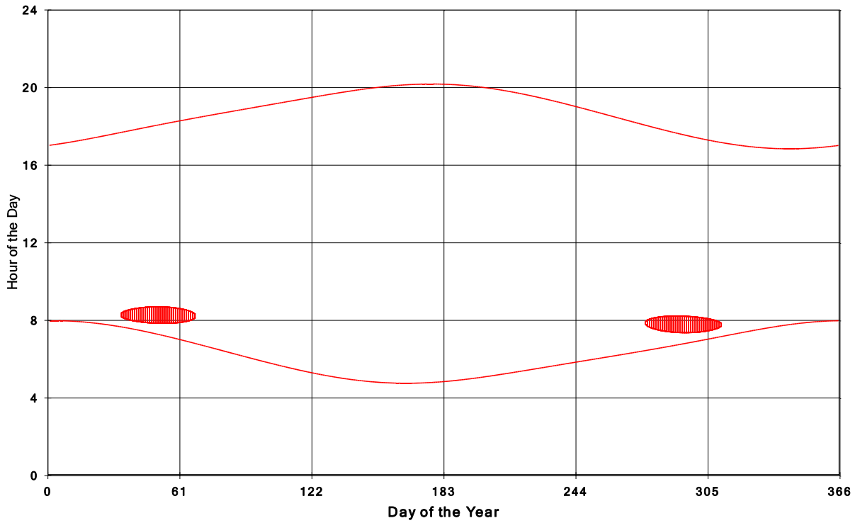
Goshen Wind Energy Centre Shadow Times on House 957, All Windows from All Turbine:
