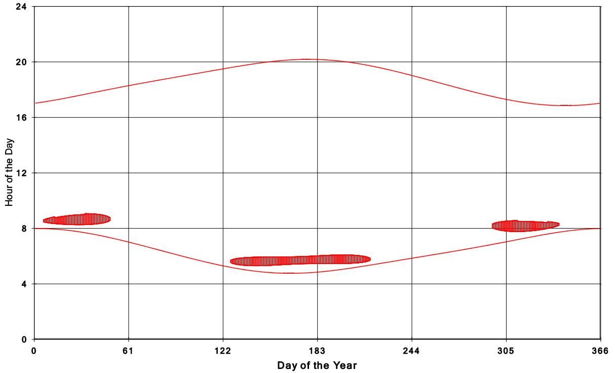
Goshen Wind Energy Centre Shadow Times on House 914, All Windows from All Turbine:
