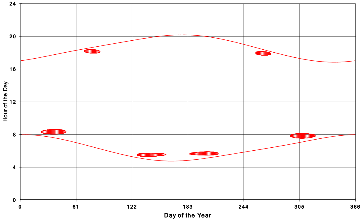
Goshen Wind Energy Centre Shadow Times on House 852, All Windows from All Turbine:
