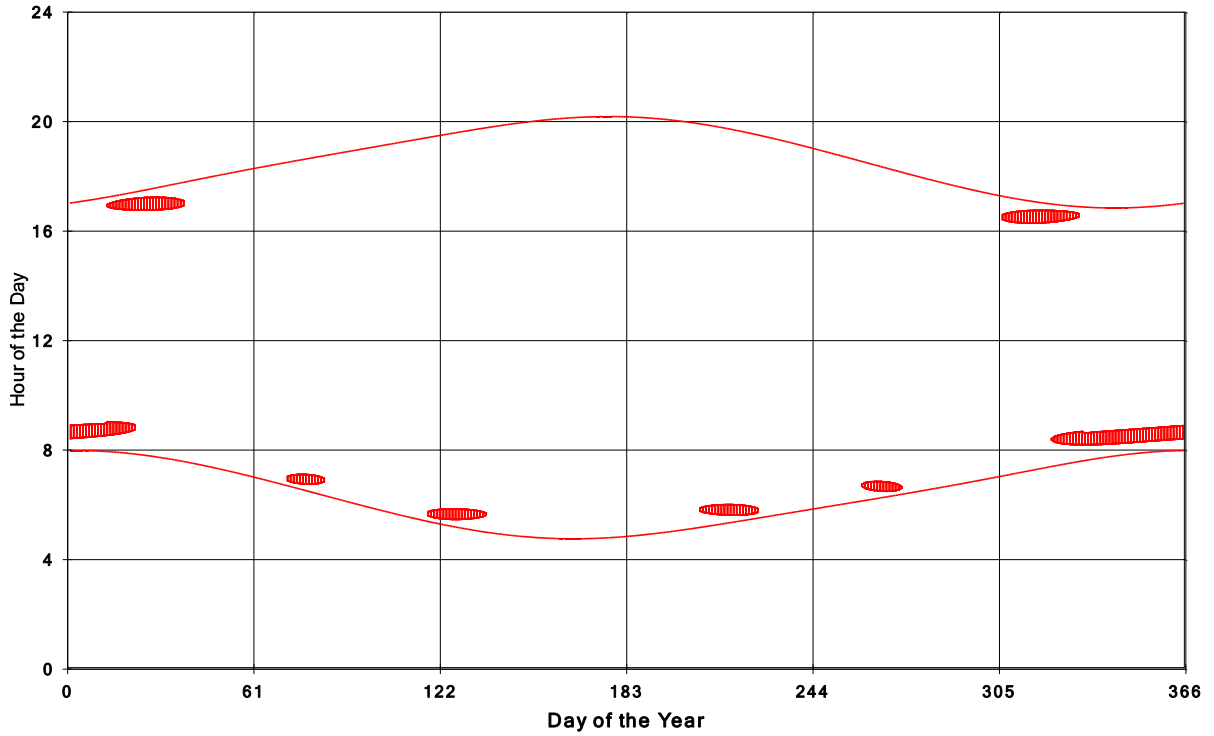
Goshen Wind Energy Centre Shadow Times on House 922, All Windows from All Turbine:
