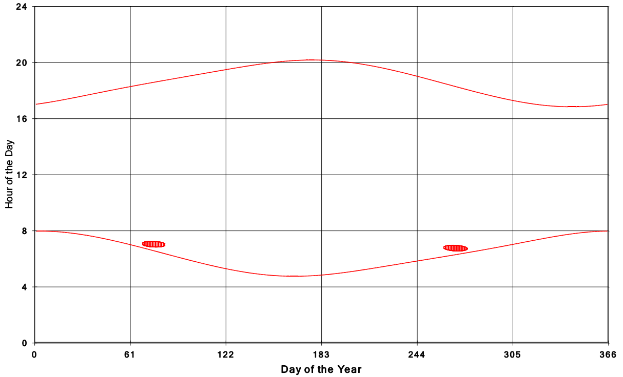
Goshen Wind Energy Centre Shadow Times on House 879, All Windows from All Turbine:
