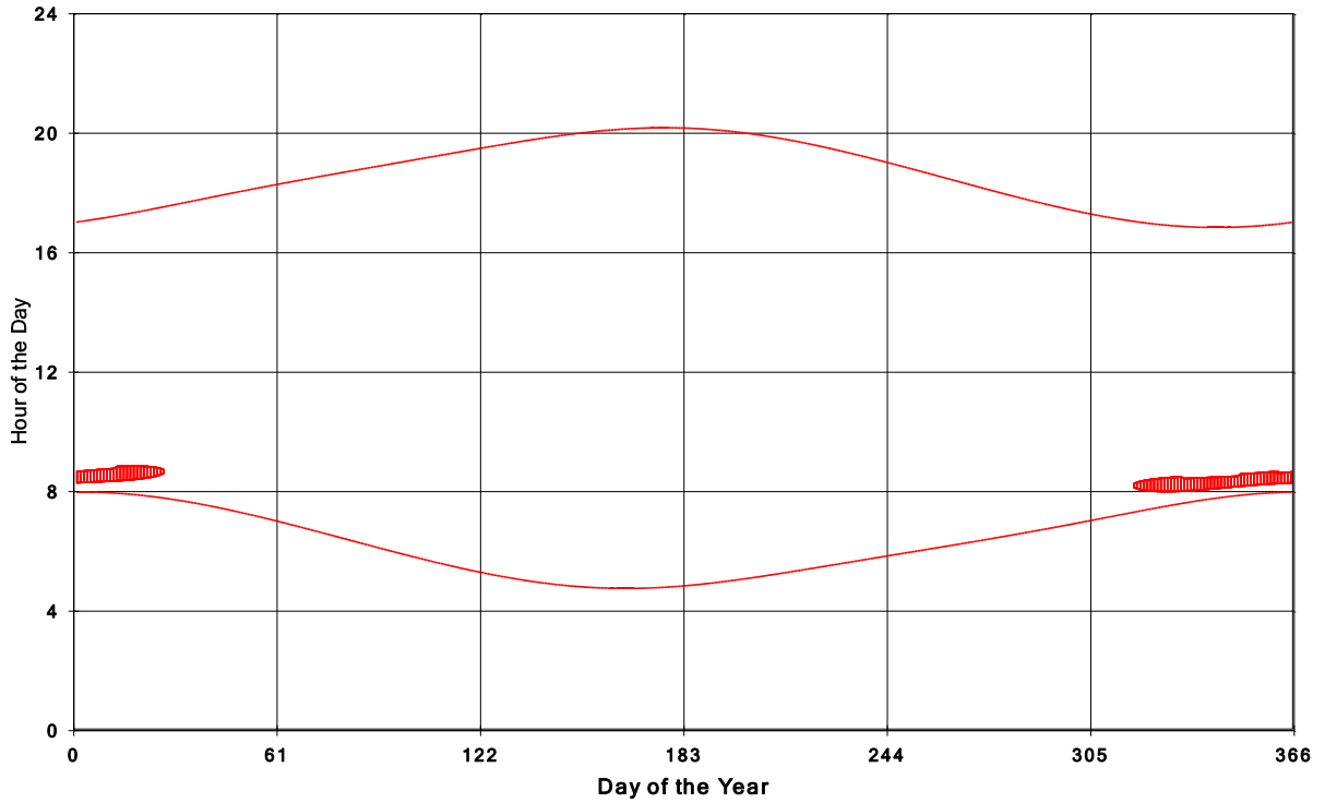
Goshen Wind Energy Centre Shadow Times on House 866, All Windows from All Turbine:
