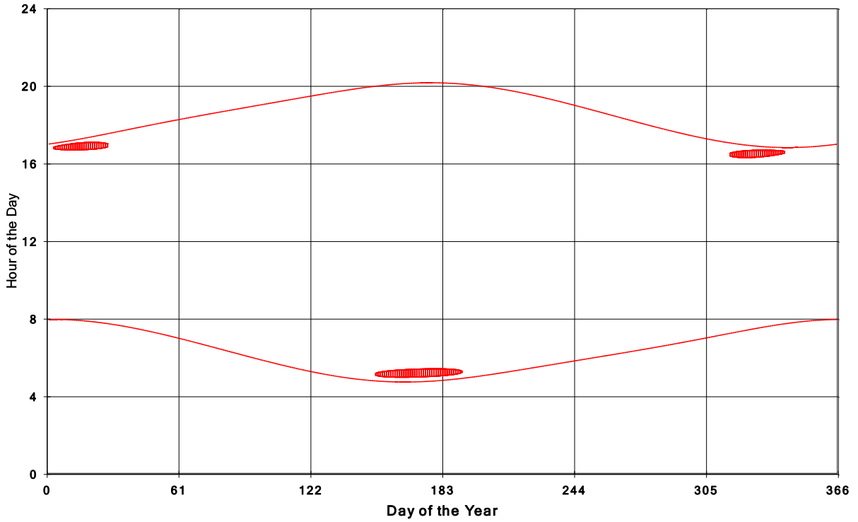
Jericho Wind Energy Centre Shadow Times on House 896, All Windows from All Turbine:
