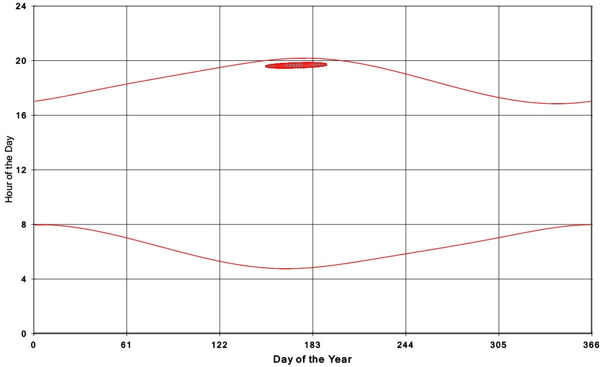
Goshen Wind Energy Centre Shadow Times on House 833, All Windows from All Turbine:
