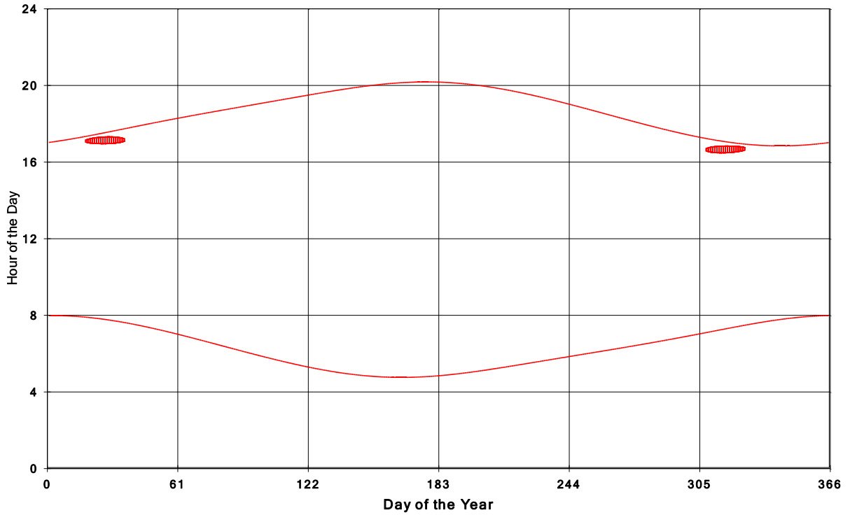
Goshen Wind Energy Centre Shadow Times on House 906, All Windows from All Turbine:
