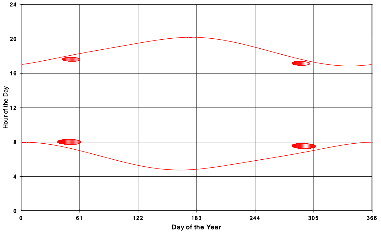
Goshen Wind Energy Centre Shadow Times on House 953, All Windows from All Turbine:
