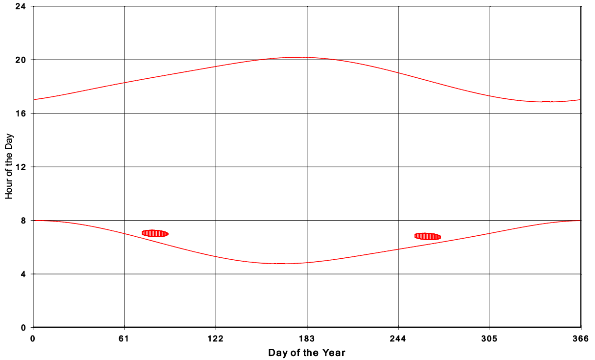
Goshen Wind Energy Centre Shadow Times on House 960, All Windows from All Turbine:
