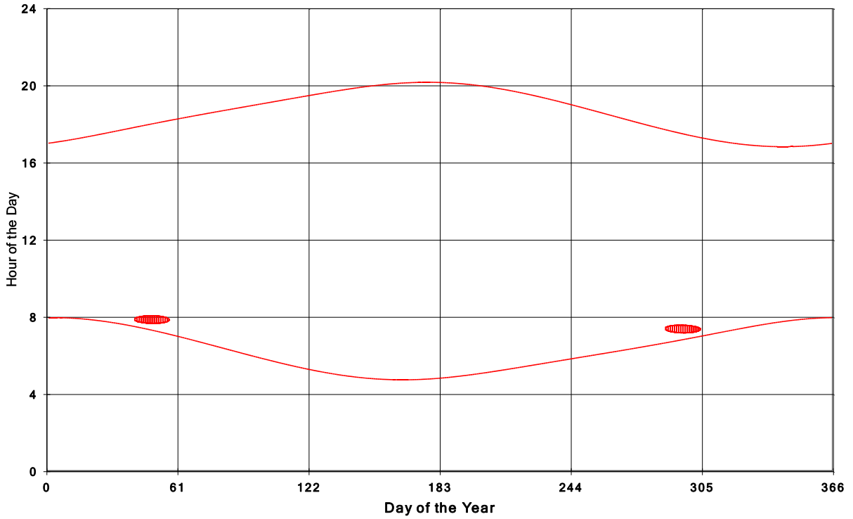
Jericho Wind Energy Centre Shadow Times on House 949, All Windows from All Turbine:
