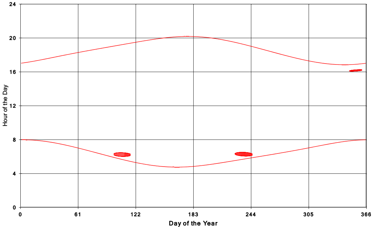
Jericho Wind Energy Centre Shadow Times on House 950, All Windows from All Turbine:
