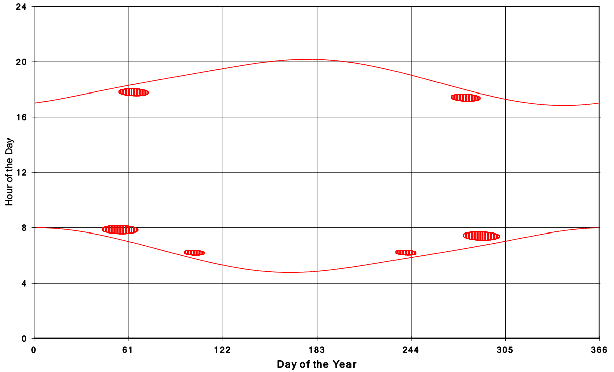
Goshen Wind Energy Centre Shadow Times on House 921, All Windows from All Turbine:
