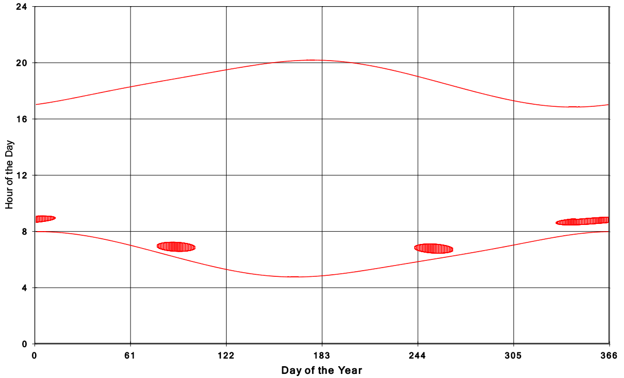
Goshen Wind Energy Centre Shadow Times on House 917, All Windows from All Turbine:
