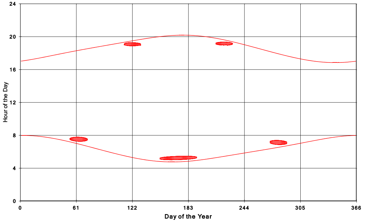
Goshen Wind Energy Centre Shadow Times on House 843, All Windows from All Turbine:
