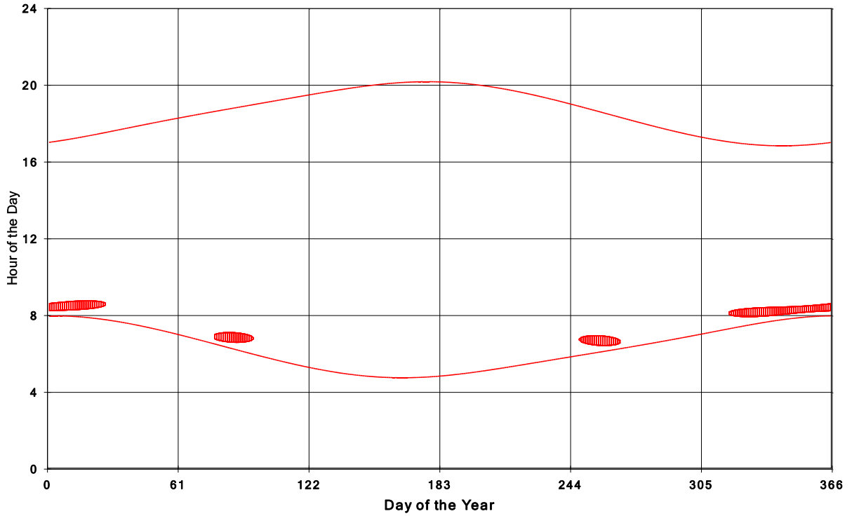
Goshen Wind Energy Centre Shadow Times on House 918, All Windows from All Turbine:
