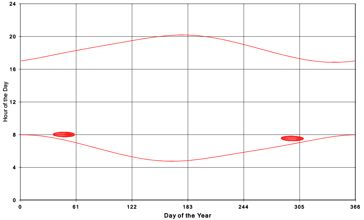
Goshen Wind Energy Centre Shadow Times on House 984, All Windows from All Turbine:
