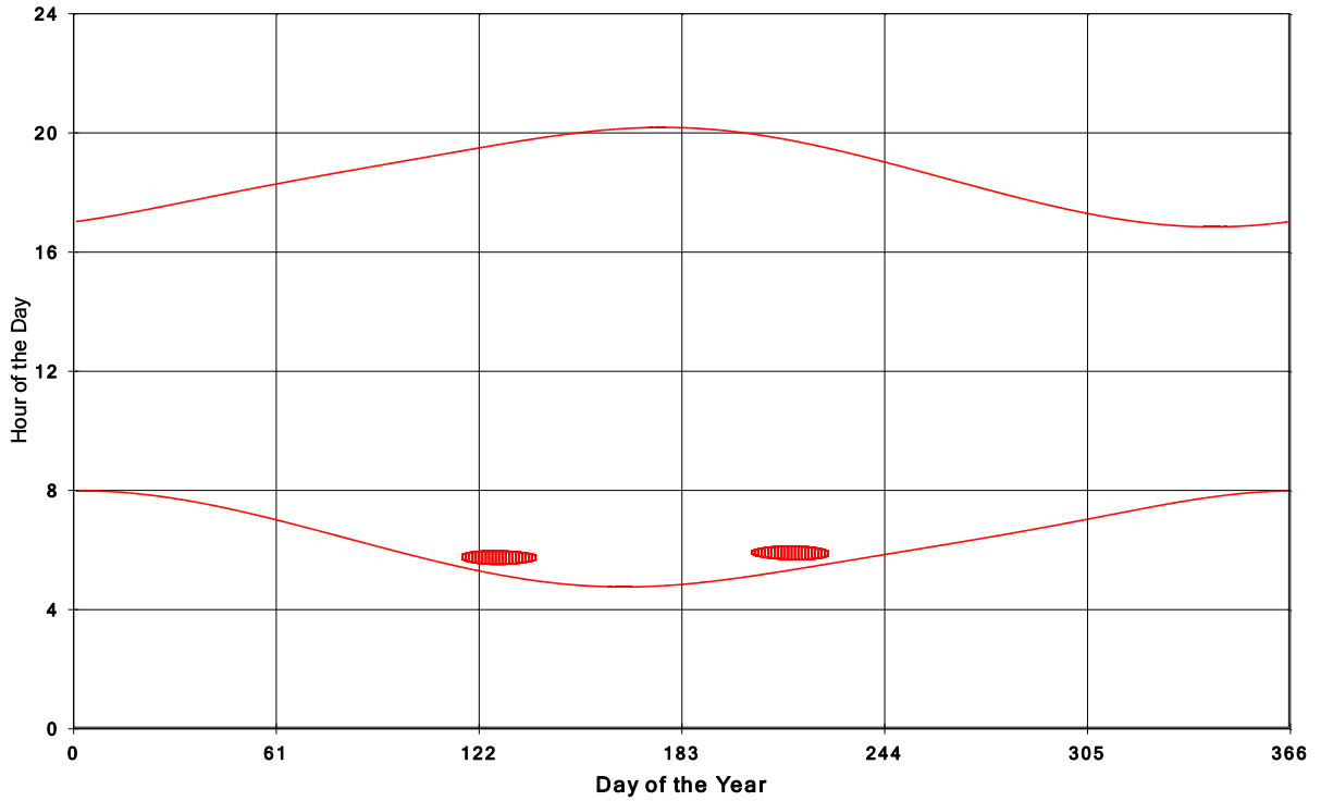
Goshen Wind Energy Centre Shadow Times on House 945, All Windows from All Turbine:
