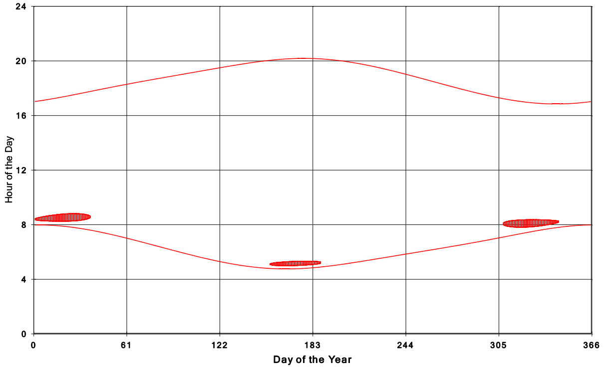
Goshen Wind Energy Centre Shadow Times on House 839, All Windows from All Turbine:
