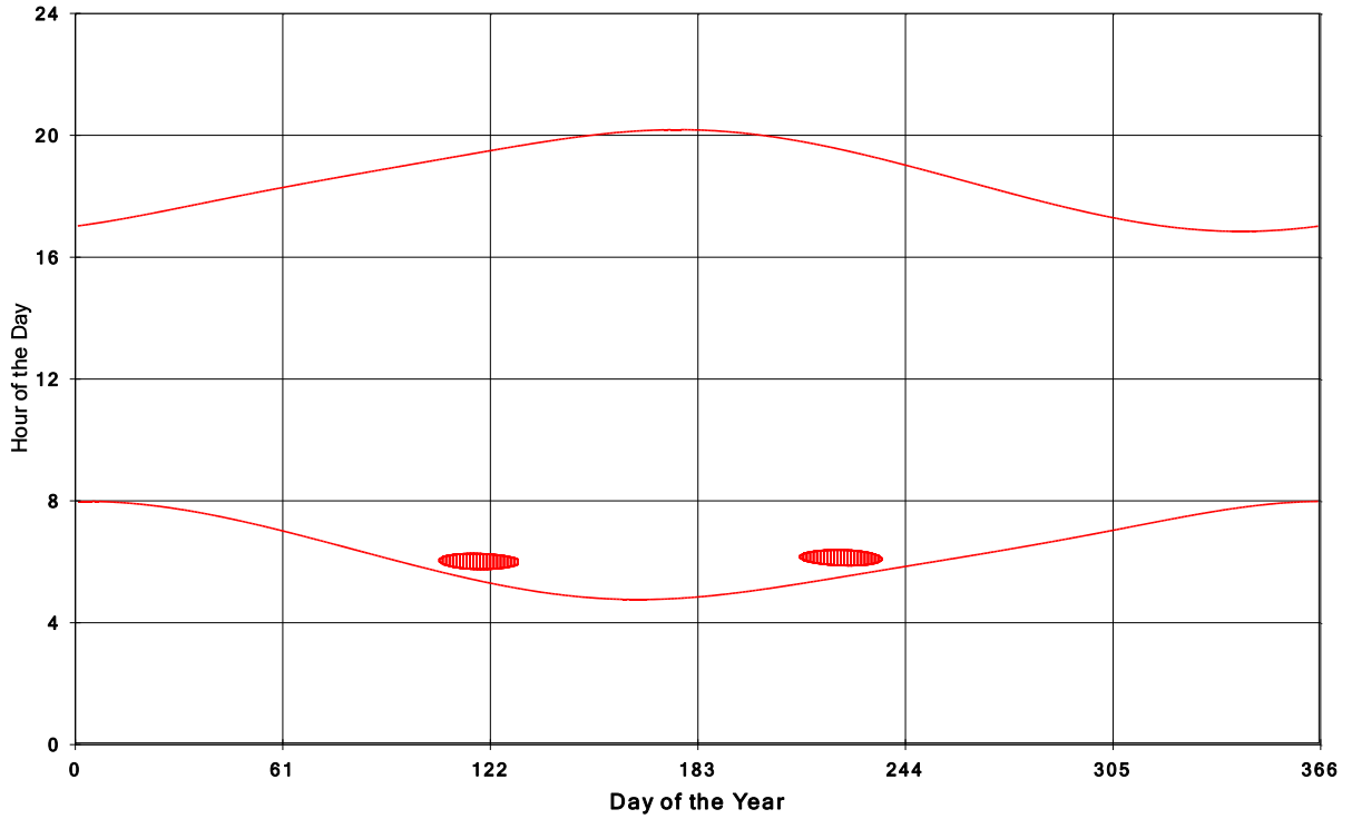
Goshen Wind Energy Centre Shadow Times on House 944, All Windows from All Turbine:
