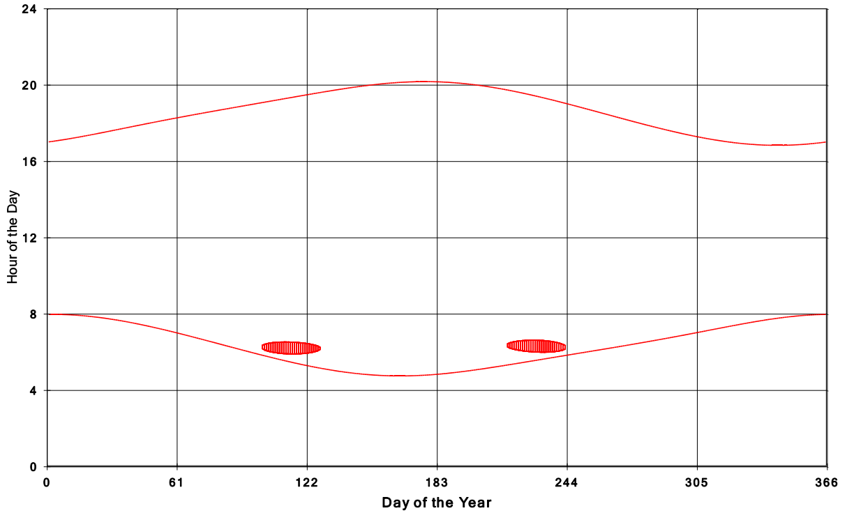
Goshen Wind Energy Centre Shadow Times on House 986, All Windows from All Turbine:
