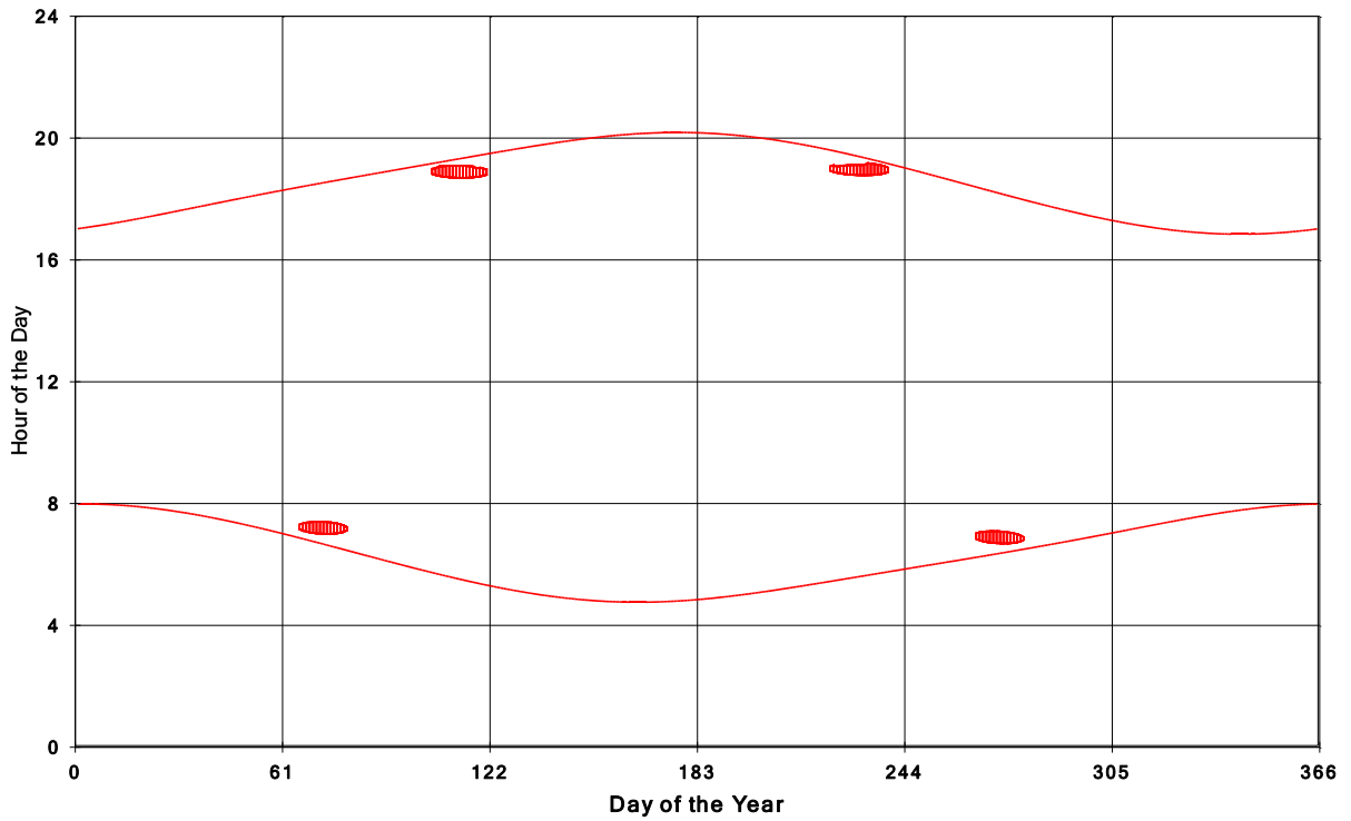
Goshen Wind Energy Centre Shadow Times on House 954, All Windows from All Turbine:
