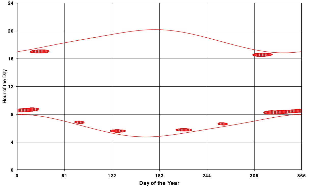
Goshen Wind Energy Centre Shadow Times on House 972, All Windows from All Turbine:
