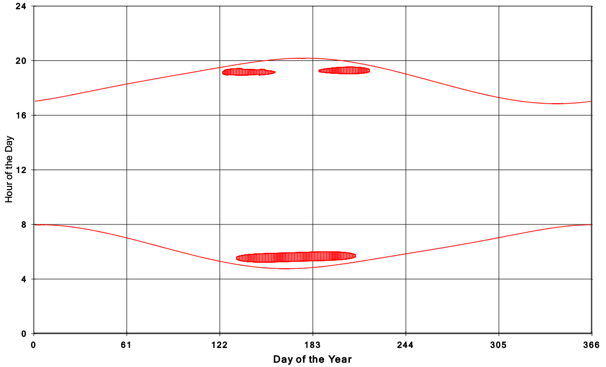
Goshen Wind Energy Centre Shadow Times on House 920, All Windows from All Turbine:
