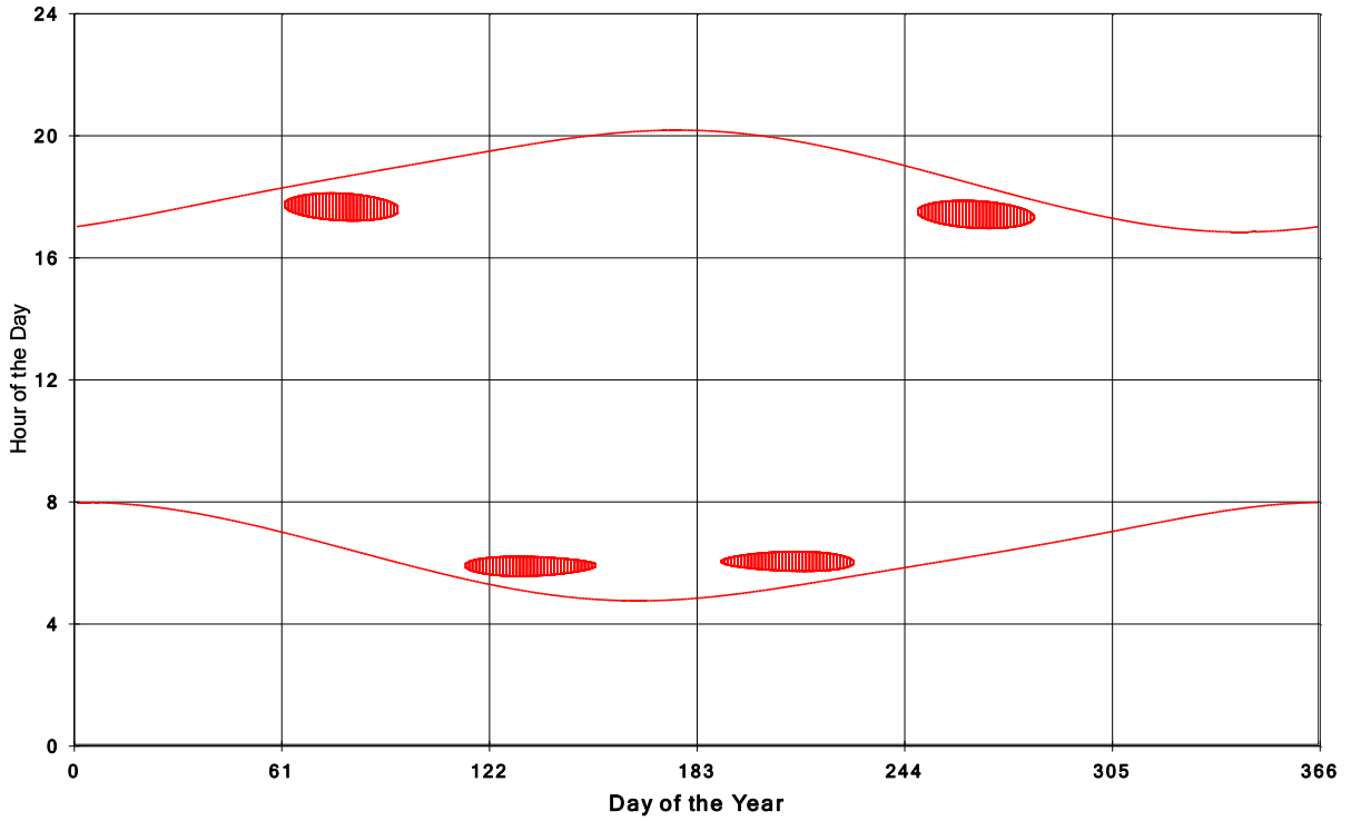
Jericho Wind Energy Centre Shadow Times on House 867, All Windows from All Turbine:
