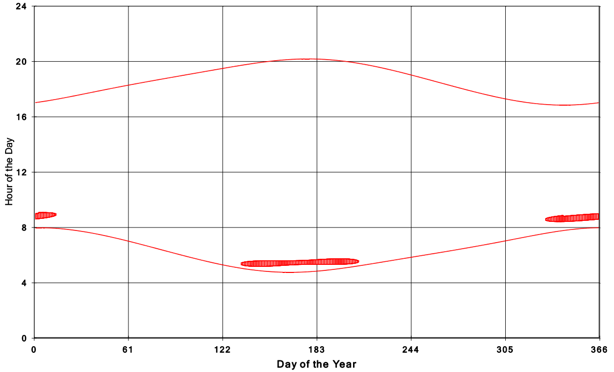
Goshen Wind Energy Centre Shadow Times on House 873, All Windows from All Turbine:
