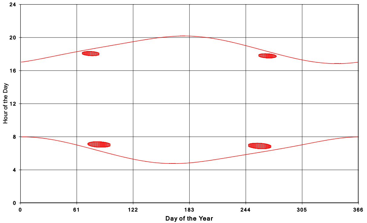
Goshen Wind Energy Centre Shadow Times on House 904, All Windows from All Turbine:
