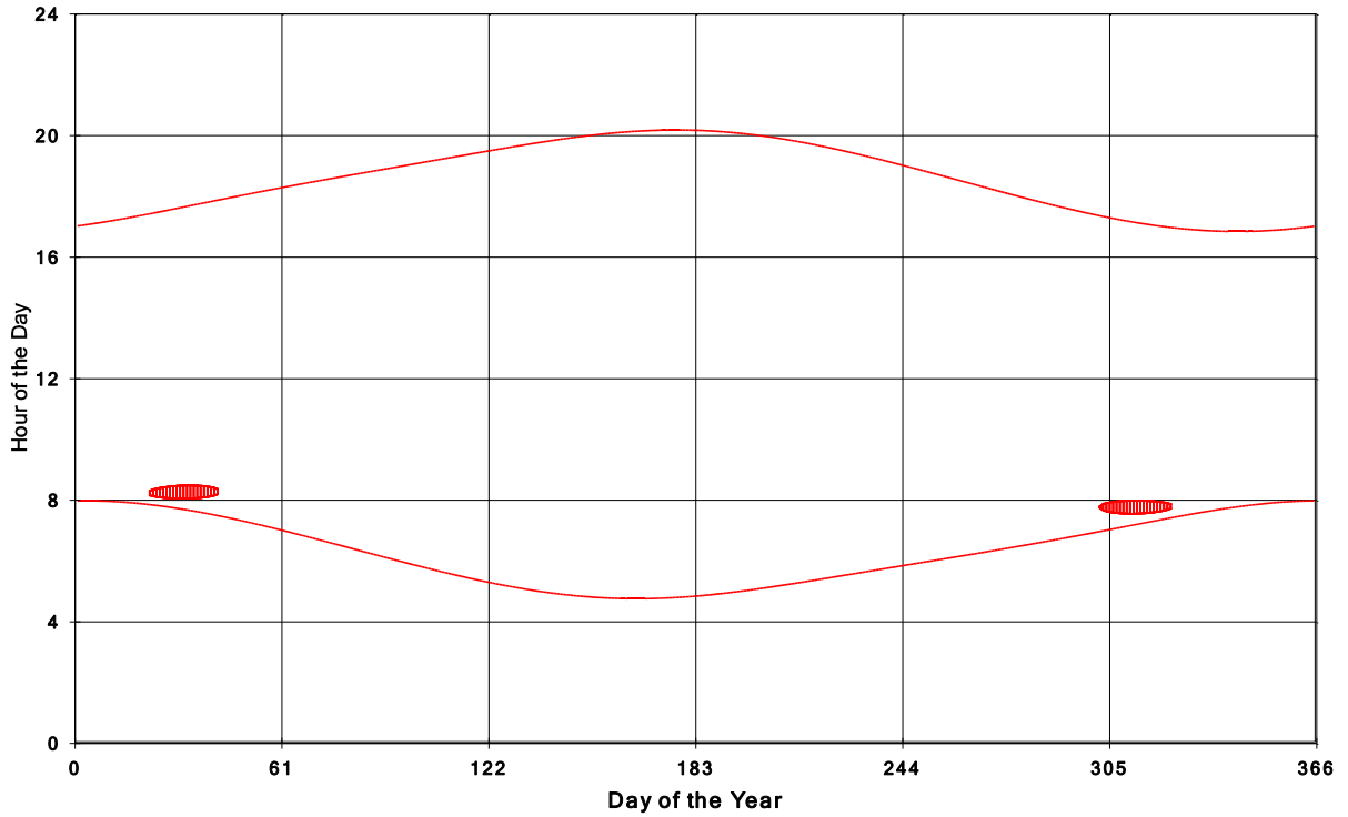
Goshen Wind Energy Centre Shadow Times on House 848, All Windows from All Turbine:
