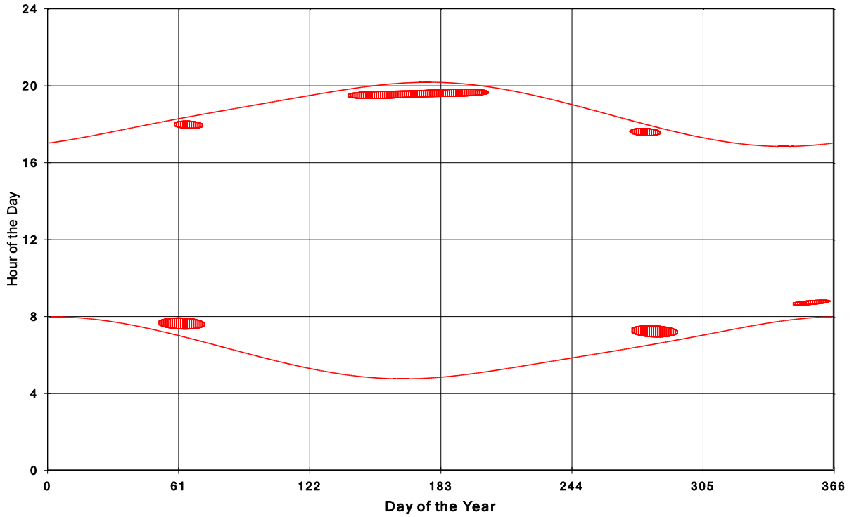
Goshen Wind Energy Centre Shadow Times on House 923, All Windows from All Turbine:
