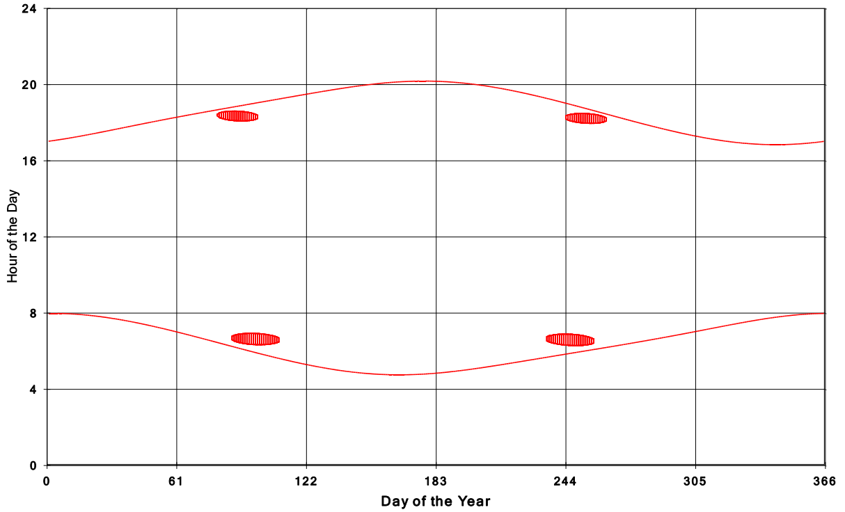
Goshen Wind Energy Centre Shadow Times on House 862, All Windows from All Turbine:
