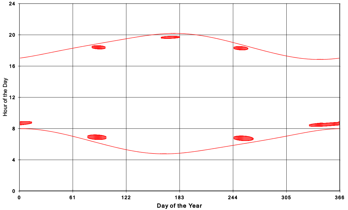
Goshen Wind Energy Centre Shadow Times on House 831, All Windows from All Turbine:
