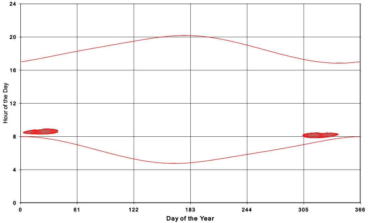
Goshen Wind Energy Centre Shadow Times on House 974, All Windows from All Turbine:
