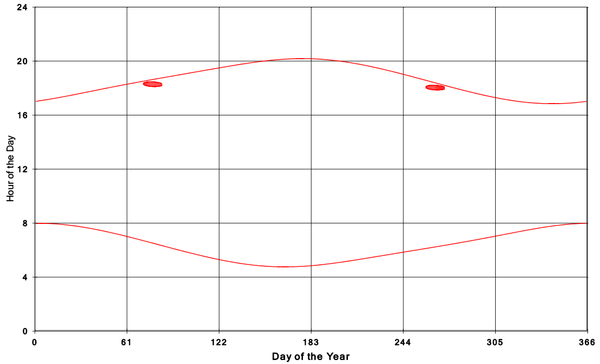
Goshen Wind Energy Centre Shadow Times on House 868, All Windows from All Turbine:
