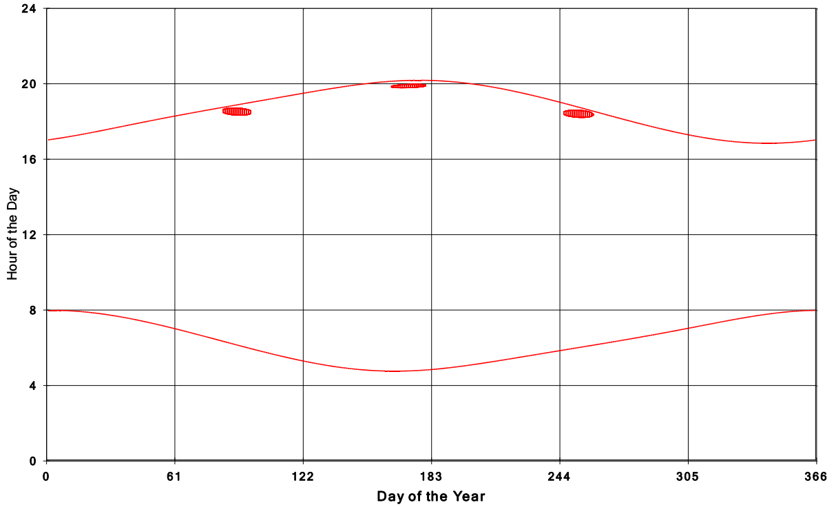
Goshen Wind Energy Centre Shadow Times on House 844, All Windows from All Turbine:
