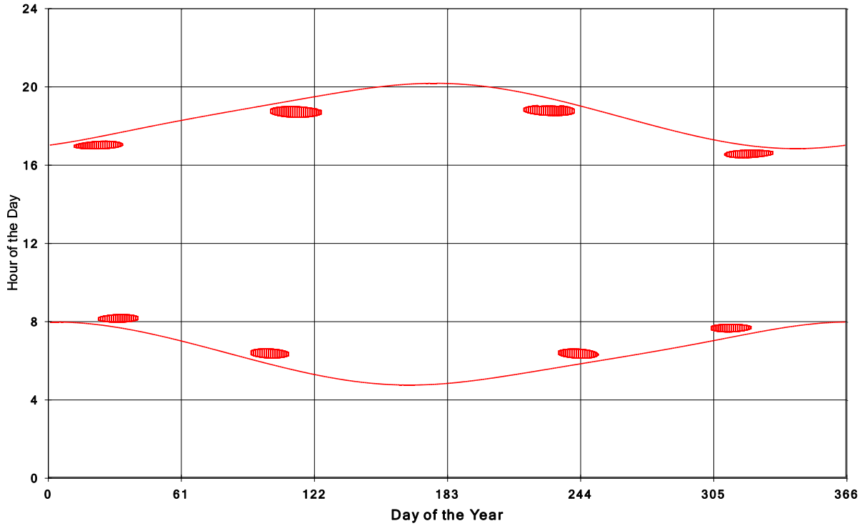
Goshen Wind Energy Centre Shadow Times on House 830, All Windows from All Turbine:
