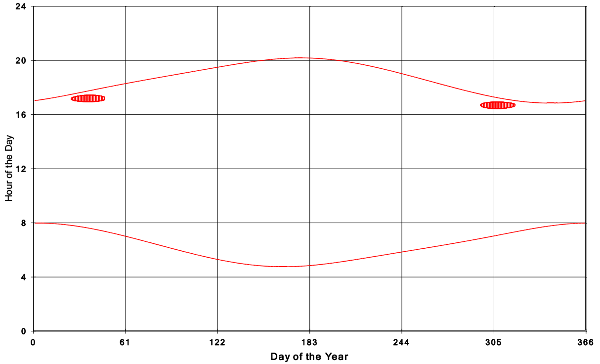
Goshen Wind Energy Centre Shadow Times on House 837, All Windows from All Turbine:
