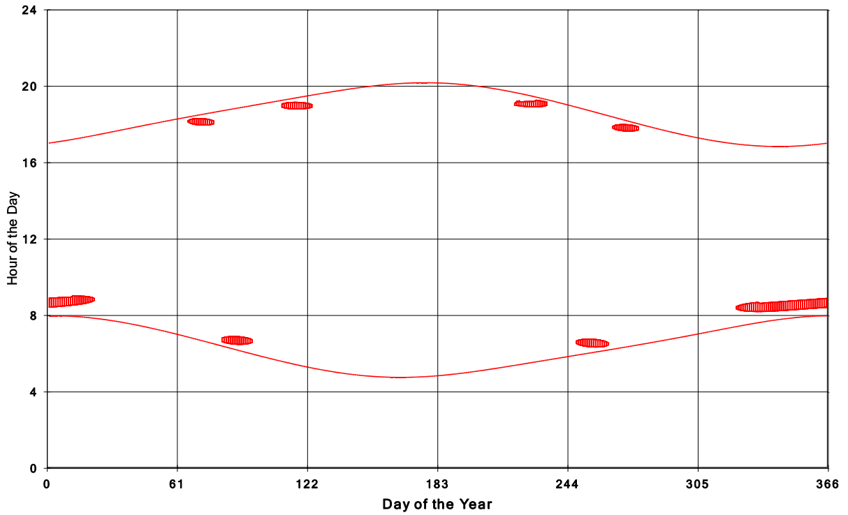
Goshen Wind Energy Centre Shadow Times on House 894, All Windows from All Turbine:
