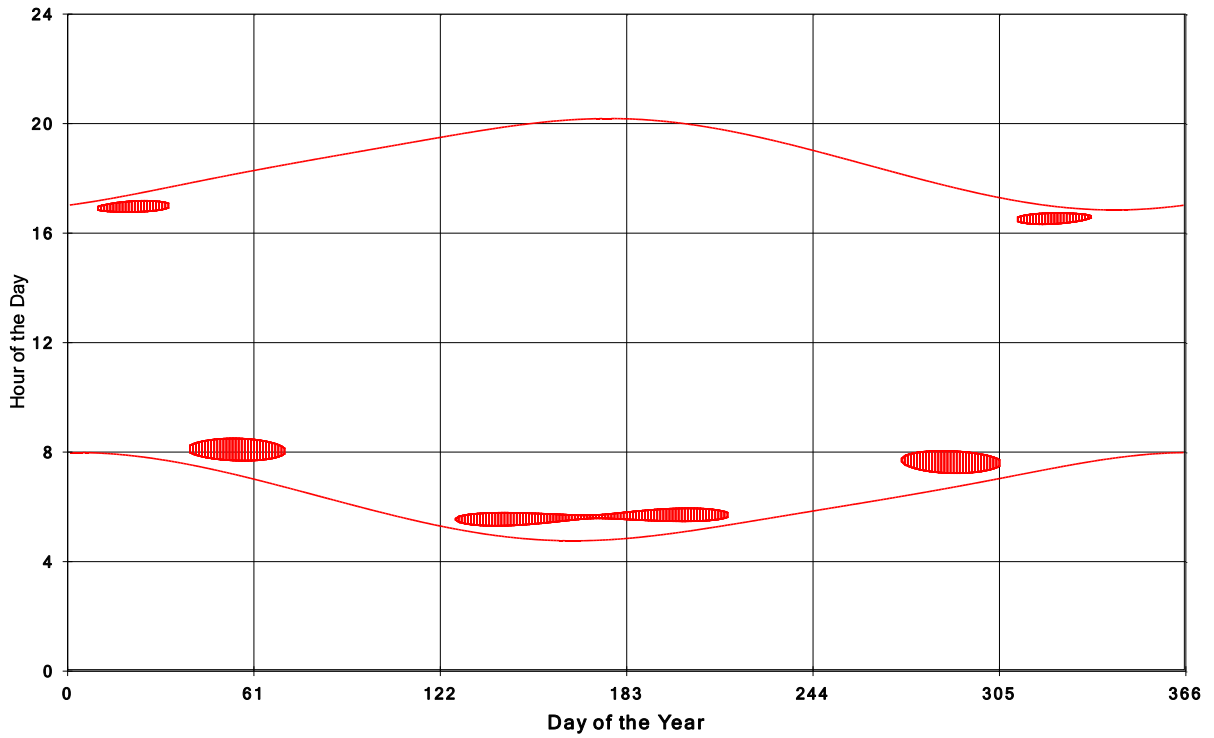
Goshen Wind Energy Centre Shadow Times on House 903, All Windows from All Turbine:
