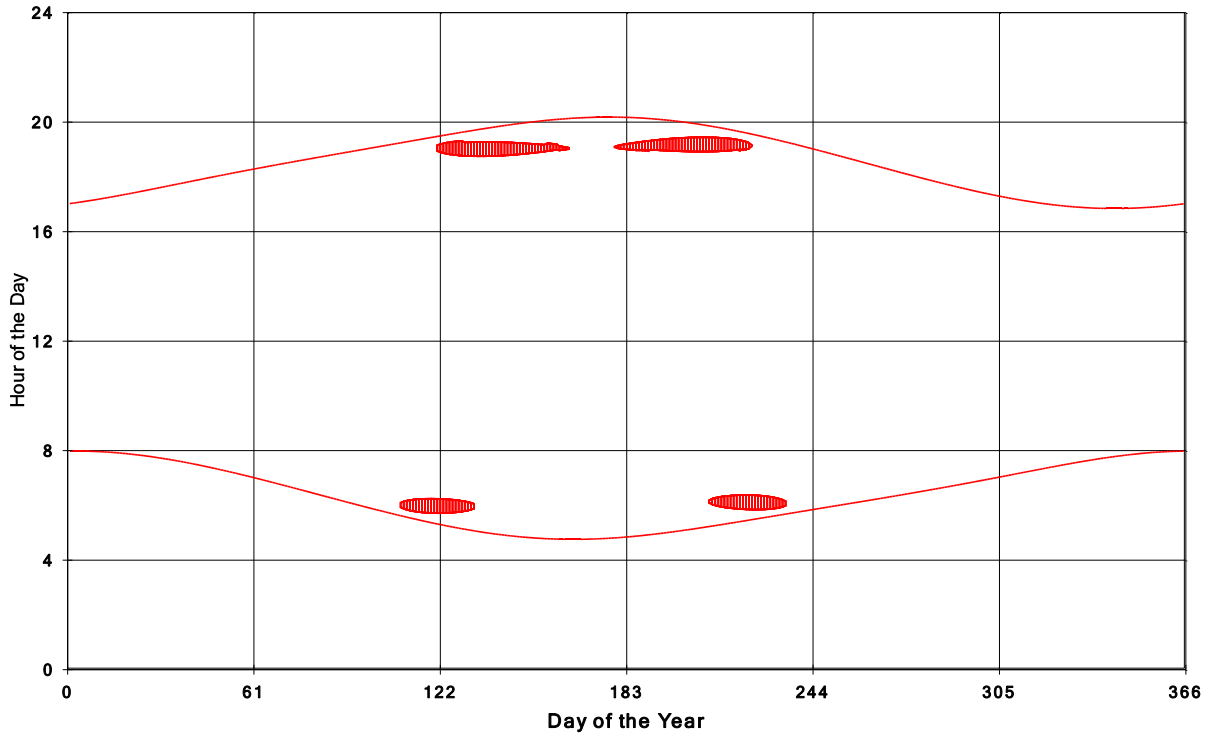
Goshen Wind Energy Centre Shadow Times on House 919, All Windows from All Turbine:
