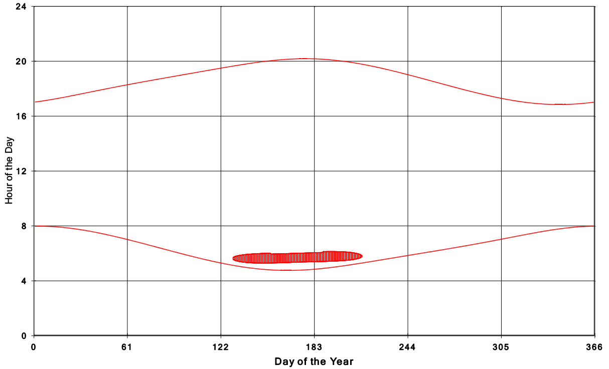
Goshen Wind Energy Centre Shadow Times on House 925, All Windows from All Turbine:
