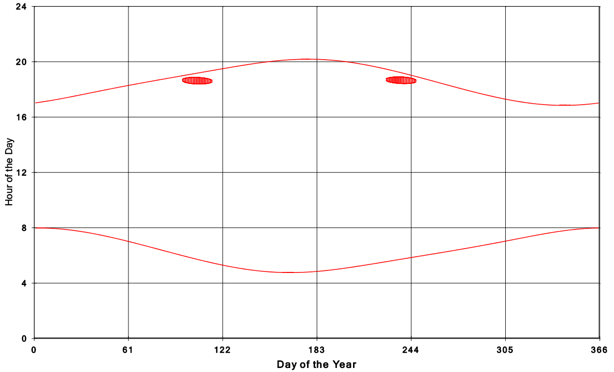
Goshen Wind Energy Centre Shadow Times on House 853, All Windows from All Turbine:
