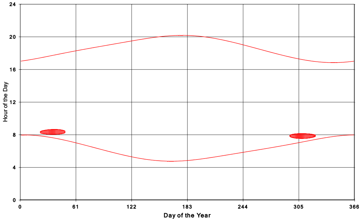
Goshen Wind Energy Centre Shadow Times on House 682, All Windows from All Turbine:
