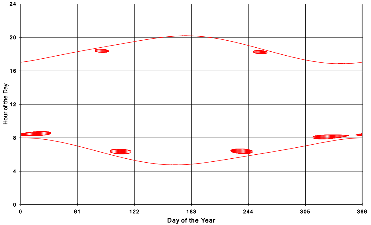
Goshen Wind Energy Centre Shadow Times on House 720, All Windows from All Turbine:
