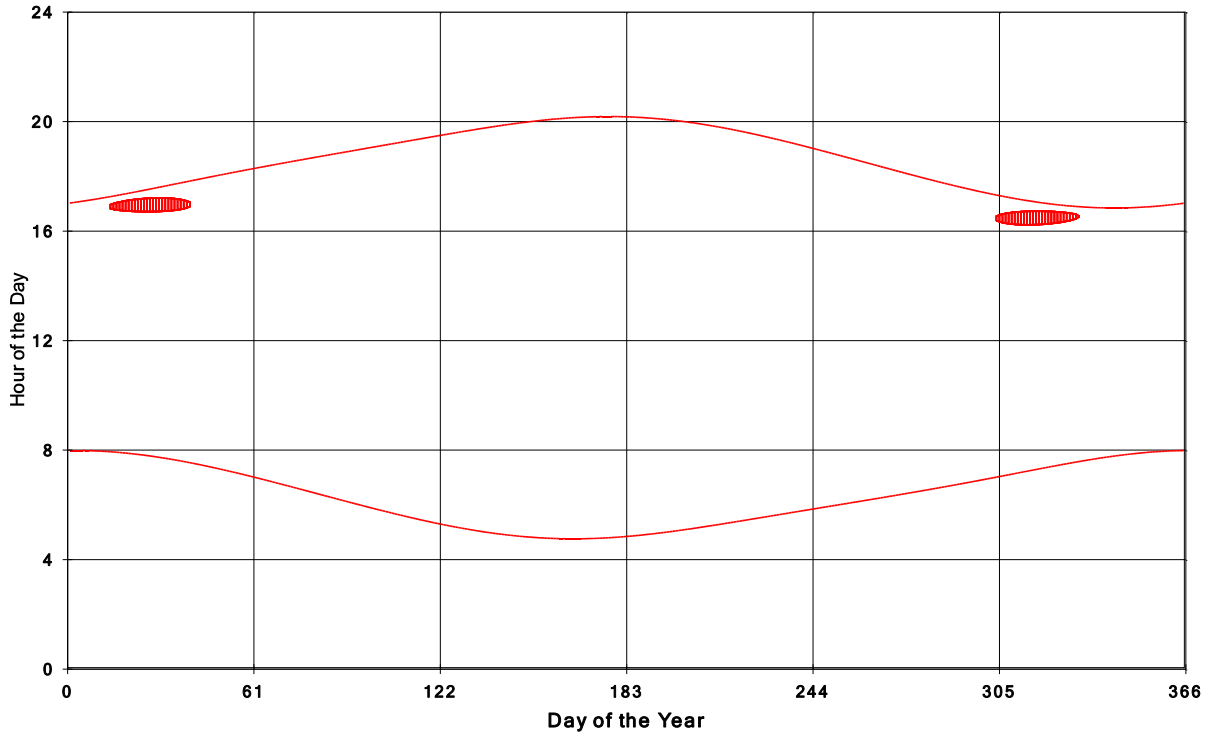
Goshen Wind Energy Centre Shadow Times on House 750, All Windows from All Turbine:
