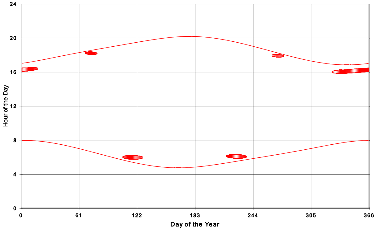
Goshen Wind Energy Centre Shadow Times on House 717, All Windows from All Turbine:
