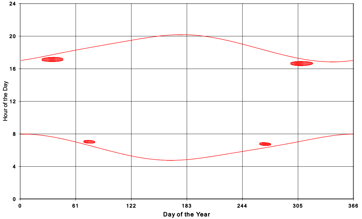
Goshen Wind Energy Centre Shadow Times on House 764, All Windows from All Turbine:
