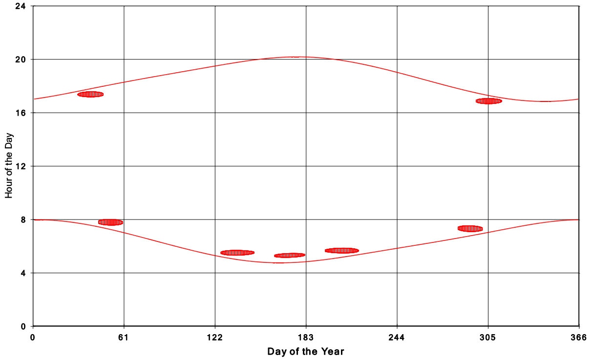
Goshen Wind Energy Centre Shadow Times on House 718, All Windows from All Turbine:
