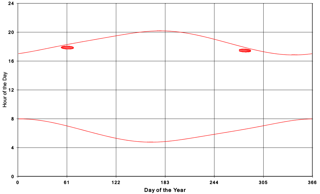
Goshen Wind Energy Centre Shadow Times on House 699, All Windows from All Turbine:
