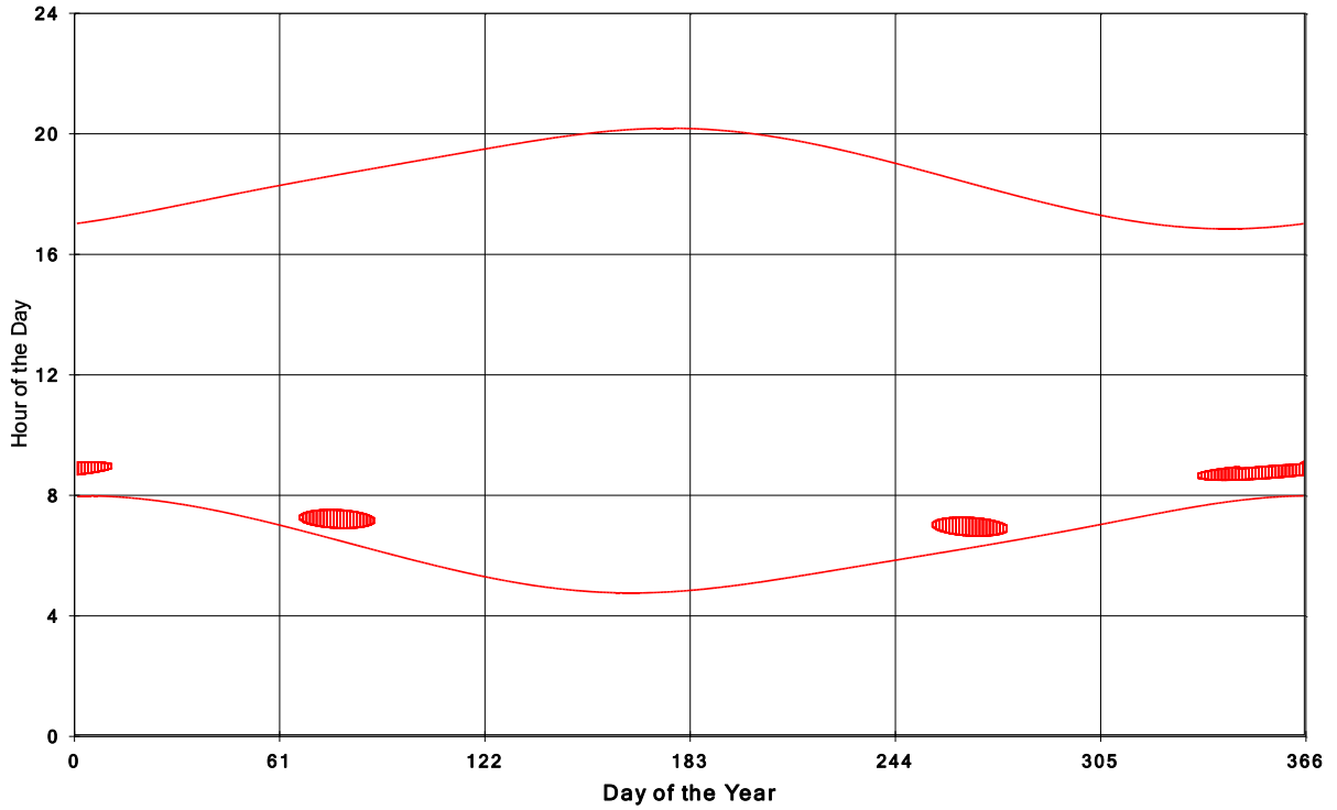
Goshen Wind Energy Centre Shadow Times on House 649, All Windows from All Turbine:
