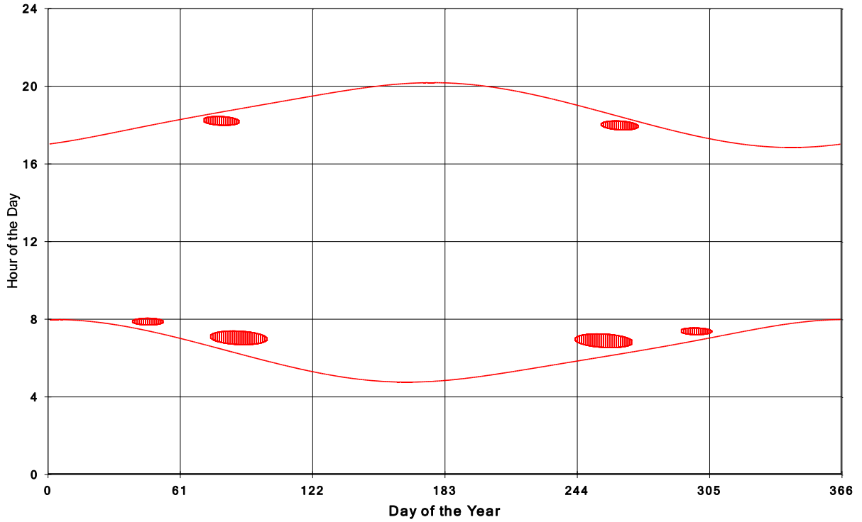
Goshen Wind Energy Centre Shadow Times on House 678, All Windows from All Turbine:
