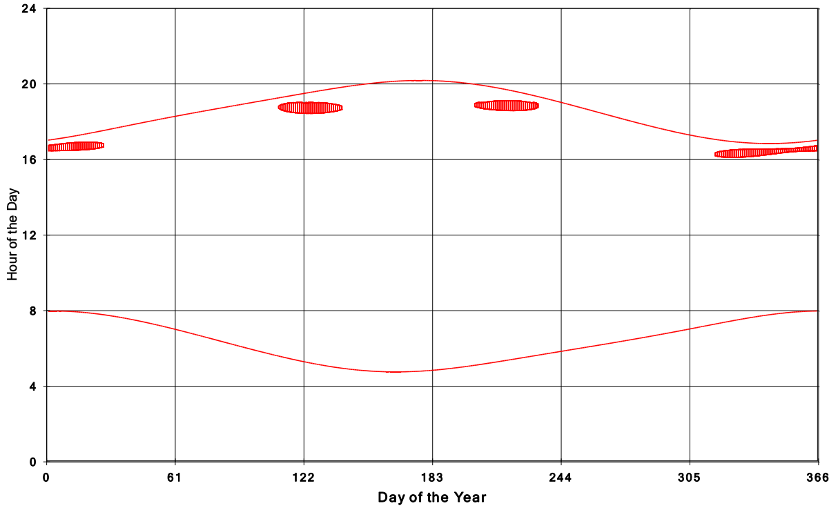
Goshen Wind Energy Centre Shadow Times on House 761, All Windows from All Turbine:
