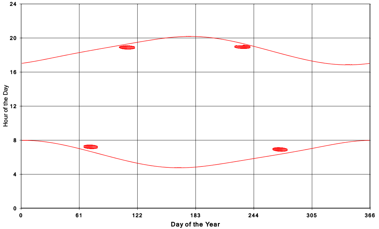
Goshen Wind Energy Centre Shadow Times on House 679, All Windows from All Turbine:
