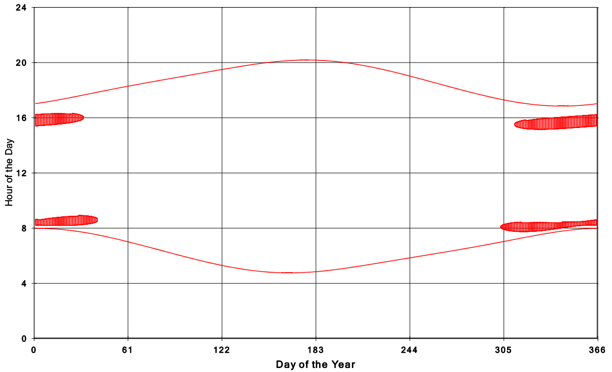
Goshen Wind Energy Centre Shadow Times on House 736, All Windows from All Turbine:
