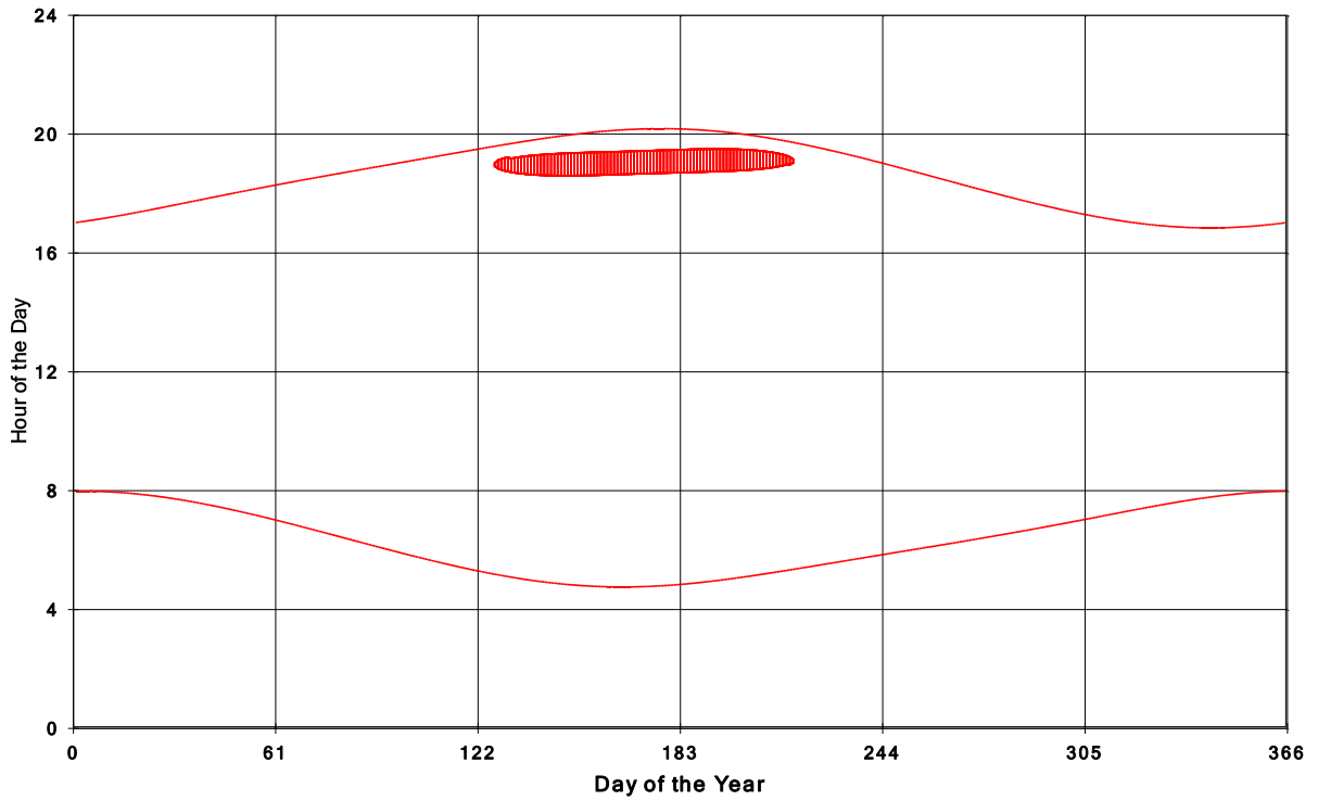
Goshen Wind Energy Centre Shadow Times on House 755, All Windows from All Turbine:
