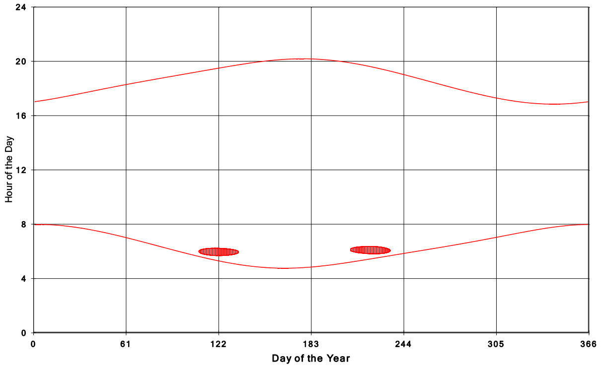
Goshen Wind Energy Centre Shadow Times on House 652, All Windows from All Turbine:
