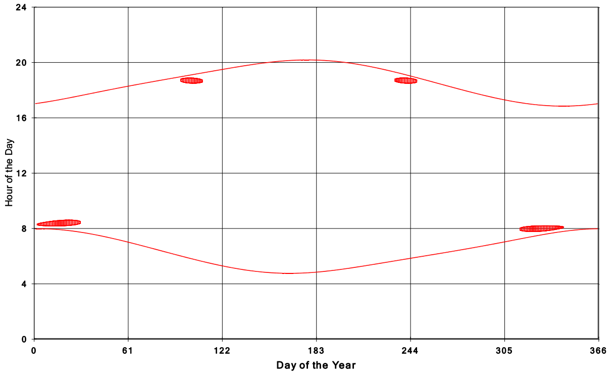
Goshen Wind Energy Centre Shadow Times on House 824, All Windows from All Turbine:
