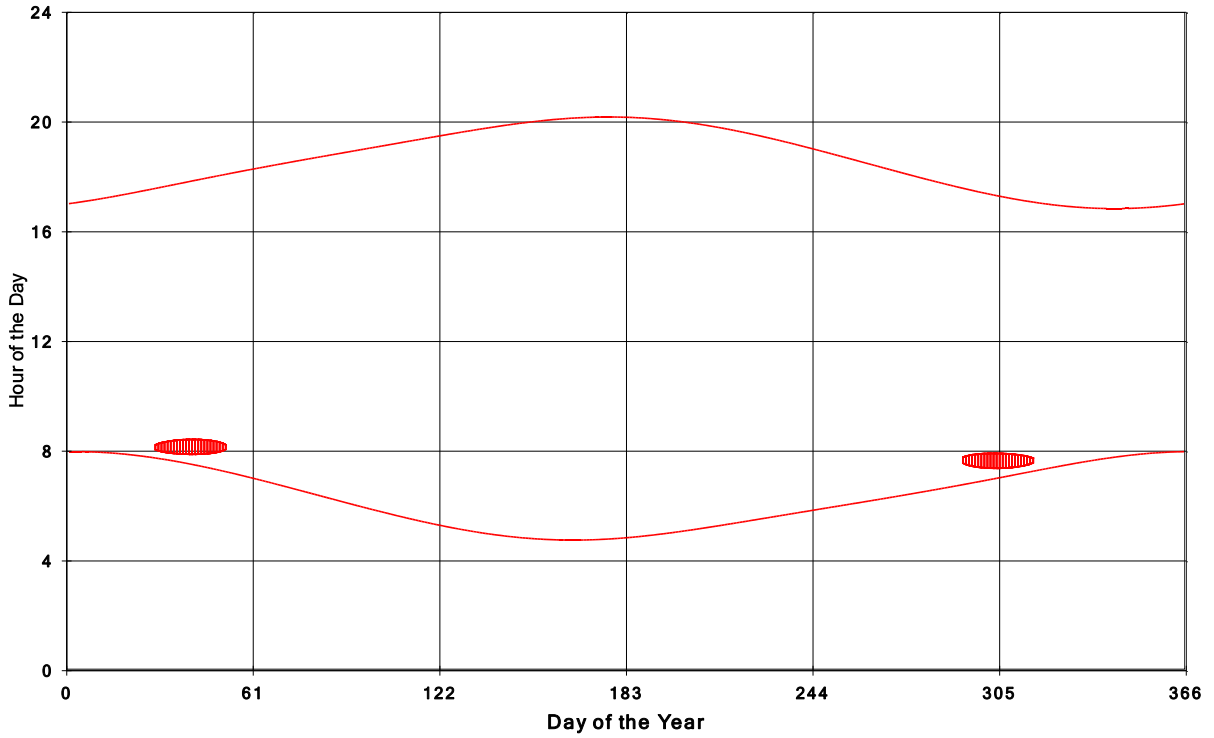
Jericho Wind Energy Centre Shadow Times on House 661, All Windows from All Turbine:
