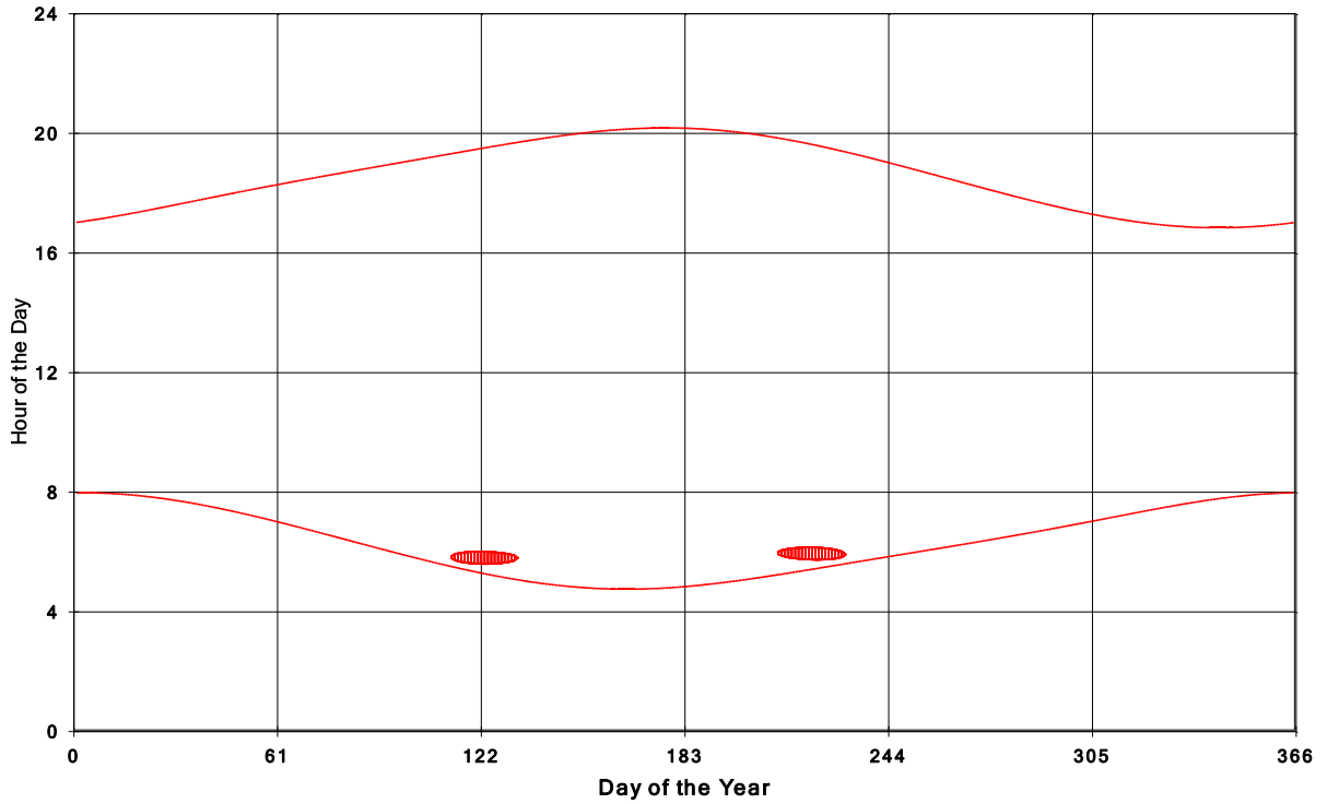
Goshen Wind Energy Centre Shadow Times on House 676, All Windows from All Turbine:
