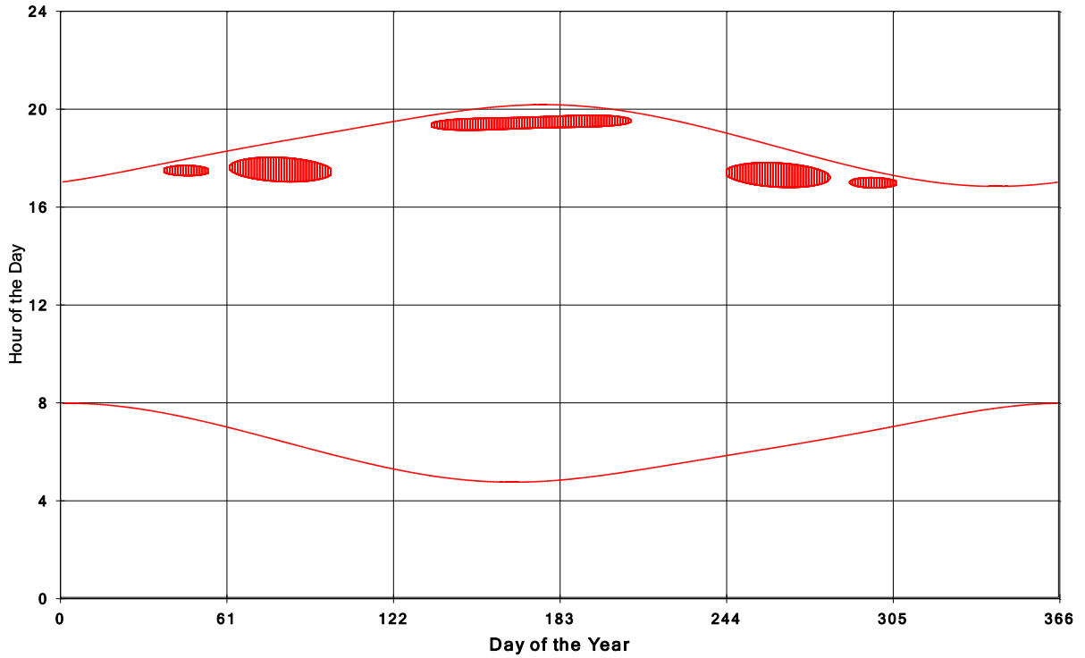
Goshen Wind Energy Centre Shadow Times on House 725, All Windows from All Turbine:
