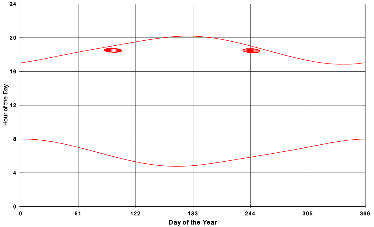
Goshen Wind Energy Centre Shadow Times on House 747, All Windows from All Turbine:
