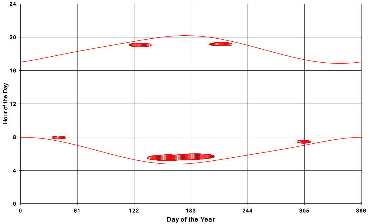
Goshen Wind Energy Centre Shadow Times on House 647, All Windows from All Turbine:
