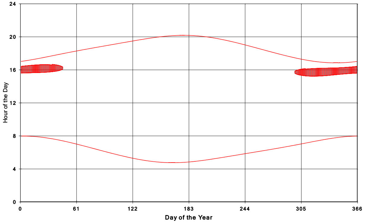
Goshen Wind Energy Centre Shadow Times on House 738, All Windows from All Turbine:
