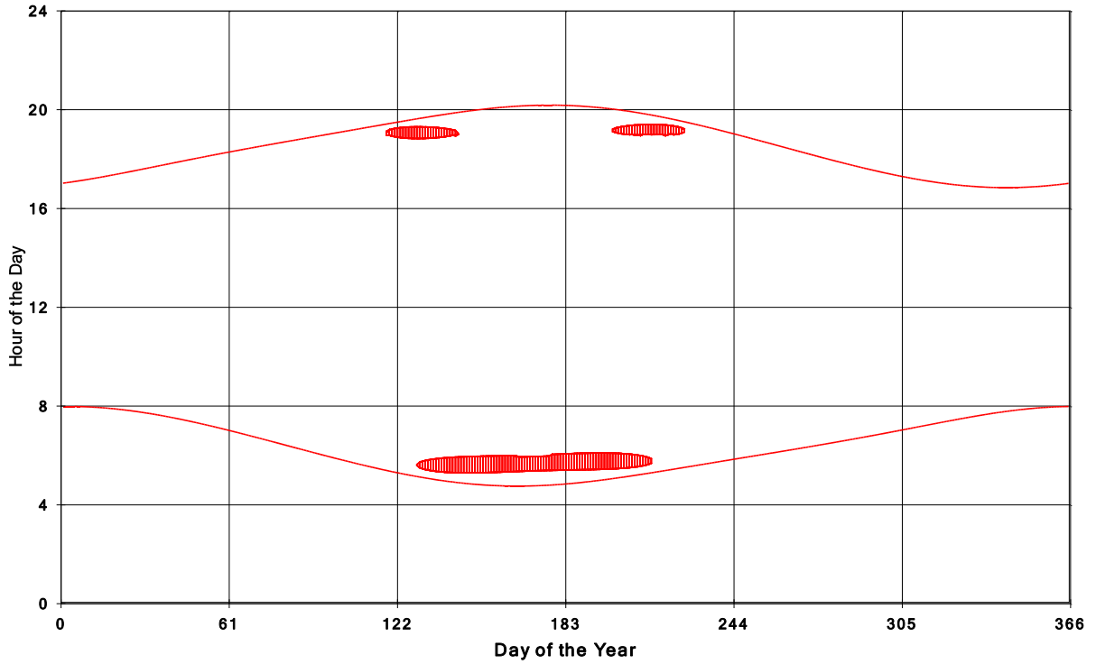
Goshen Wind Energy Centre Shadow Times on House 646, All Windows from All Turbine:
