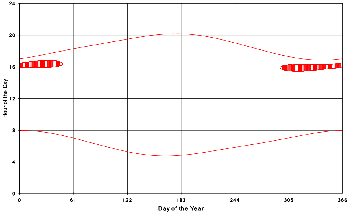
Goshen Wind Energy Centre Shadow Times on House 739, All Windows from All Turbine:
