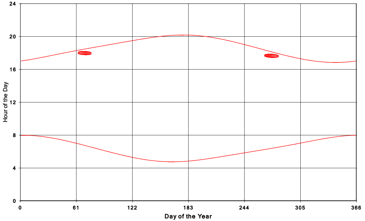
Goshen Wind Energy Centre Shadow Times on House 724, All Windows from All Turbine:
