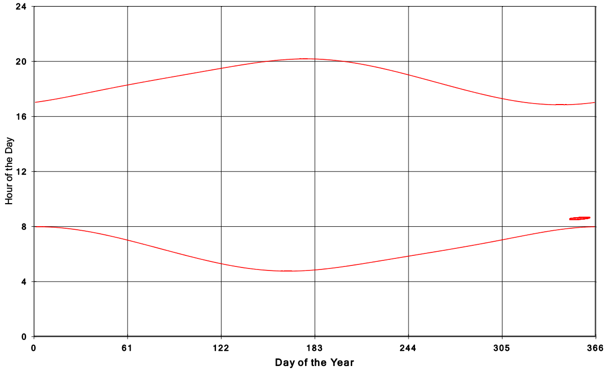
Goshen Wind Energy Centre Shadow Times on House 731, All Windows from All Turbine:
