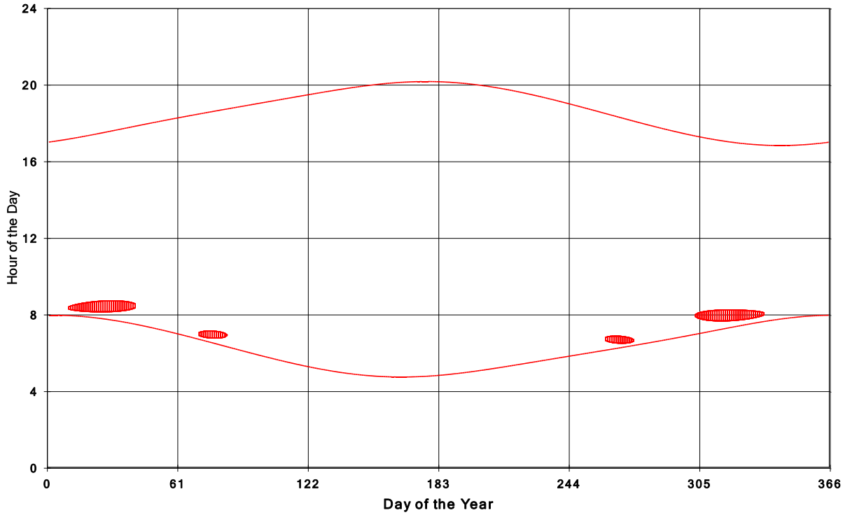
Goshen Wind Energy Centre Shadow Times on House 828, All Windows from All Turbine:
