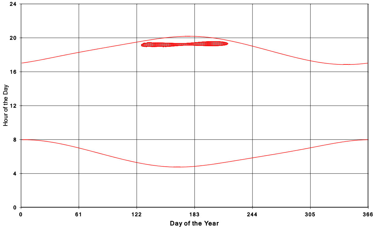
Goshen Wind Energy Centre Shadow Times on House 749, All Windows from All Turbine:
