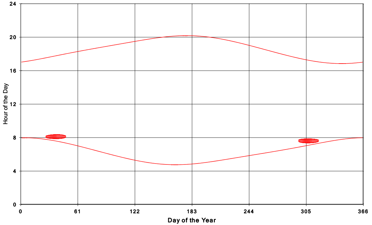
Goshen Wind Energy Centre Shadow Times on House 715, All Windows from All Turbine:
