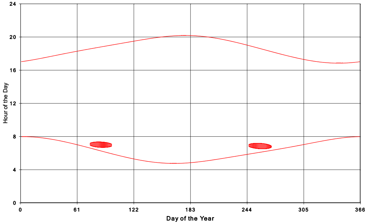
Goshen Wind Energy Centre Shadow Times on House 765, All Windows from All Turbine:
