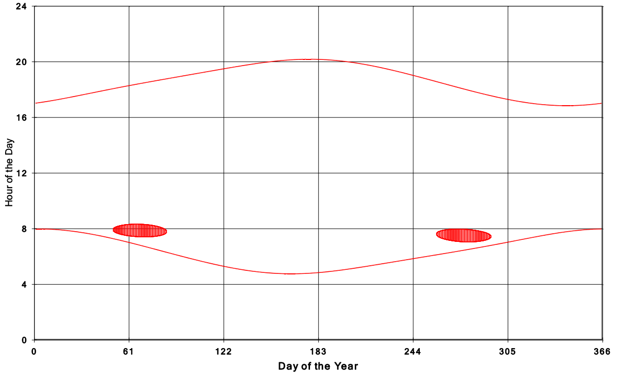
Goshen Wind Energy Centre Shadow Times on House 684, All Windows from All Turbine:
