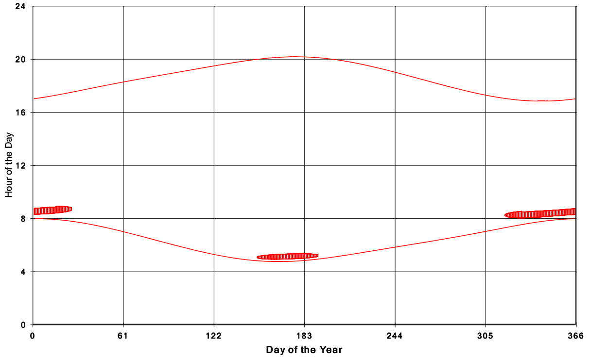
Goshen Wind Energy Centre Shadow Times on House 734, All Windows from All Turbine:
