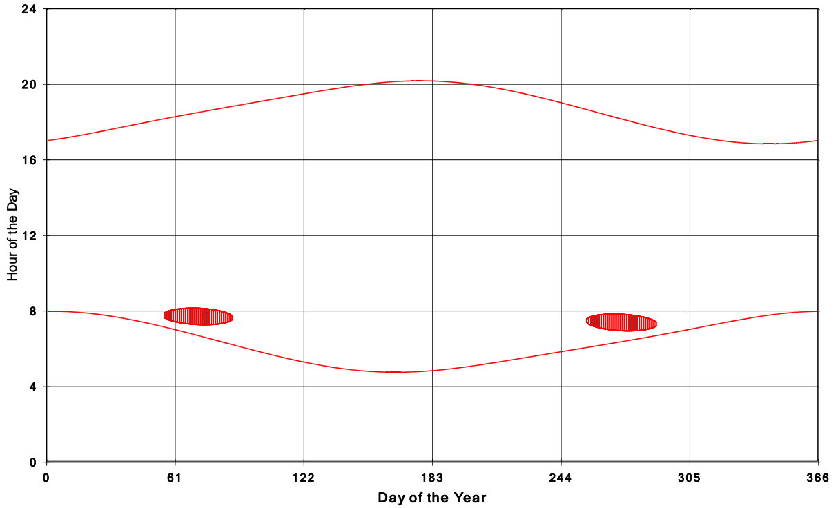
Goshen Wind Energy Centre Shadow Times on House 685, All Windows from All Turbine:
