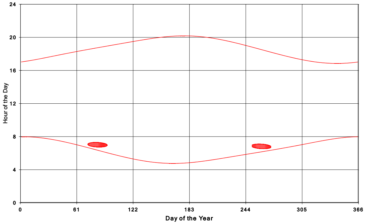
Goshen Wind Energy Centre Shadow Times on House 686, All Windows from All Turbine:
