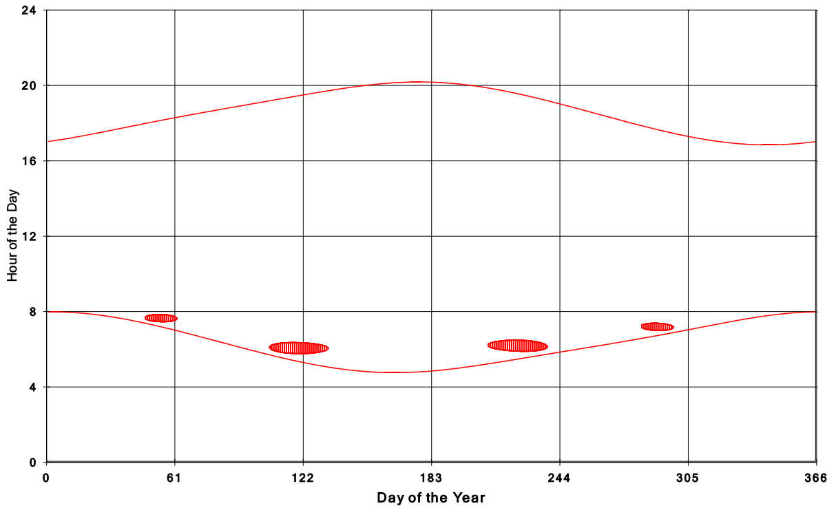
Goshen Wind Energy Centre Shadow Times on House 827, All Windows from All Turbine:
