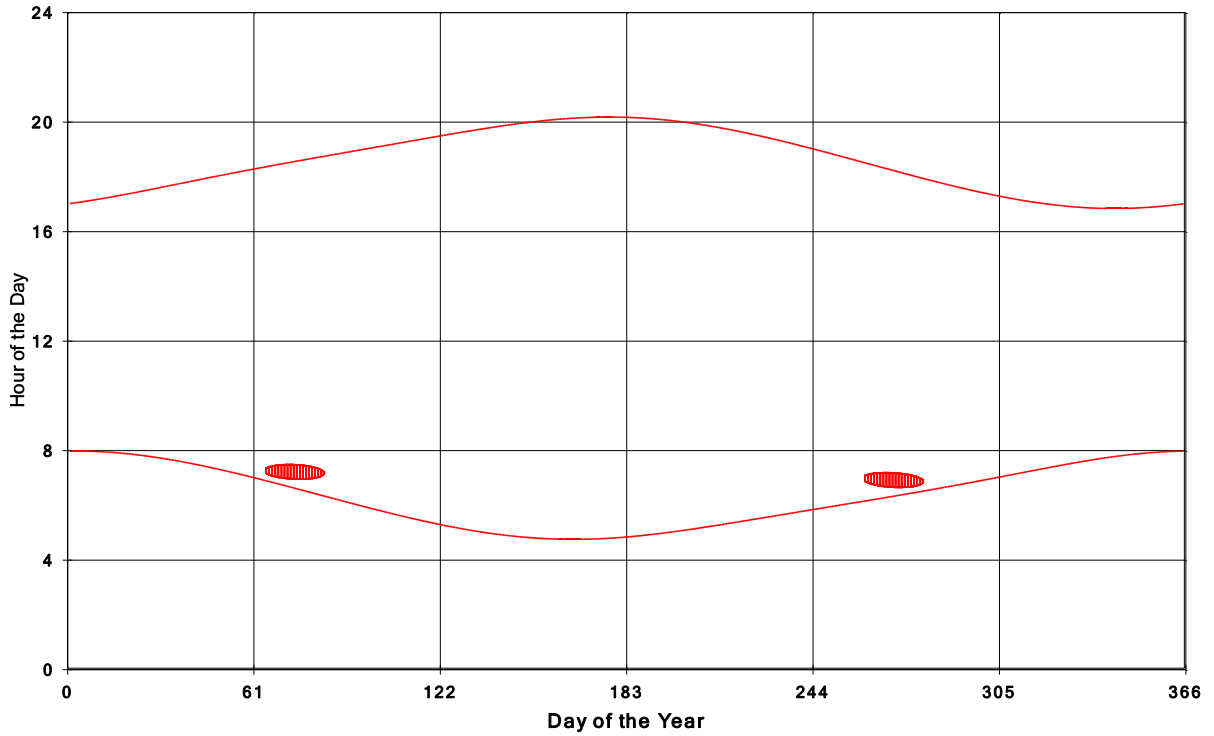
Goshen Wind Energy Centre Shadow Times on House 763, All Windows from All Turbine:
