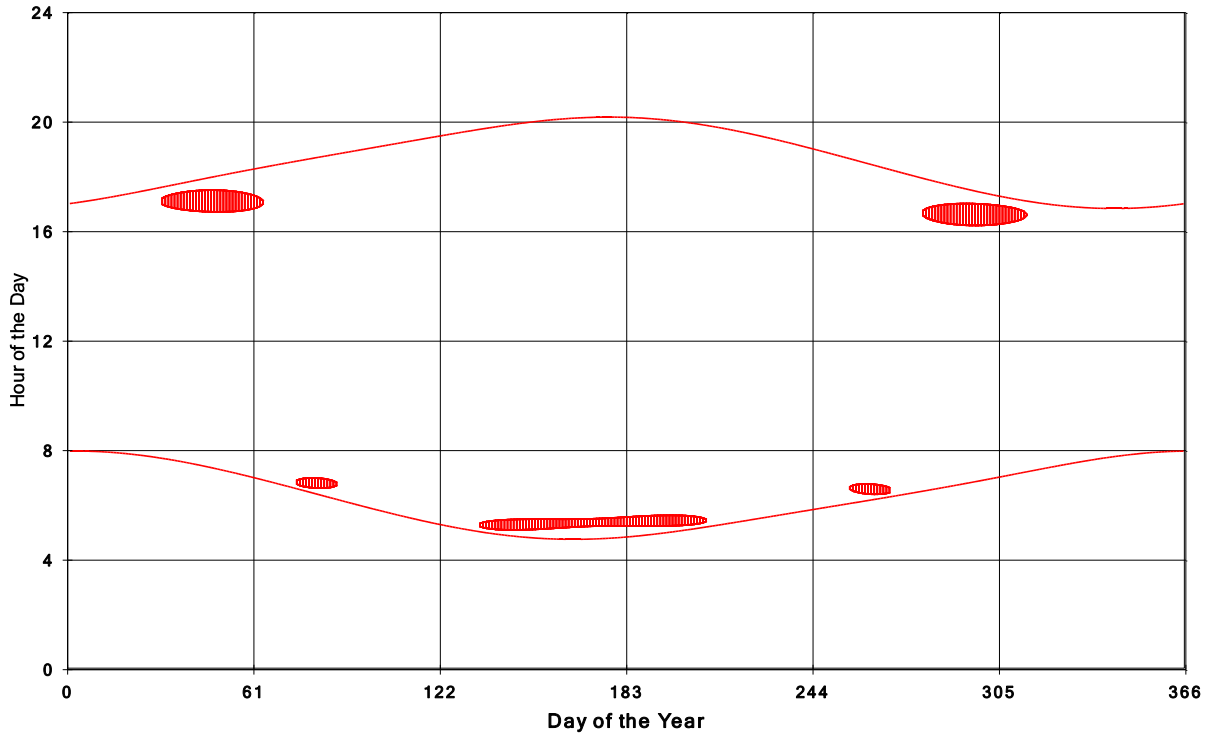
Goshen Wind Energy Centre Shadow Times on House 714, All Windows from All Turbine:
