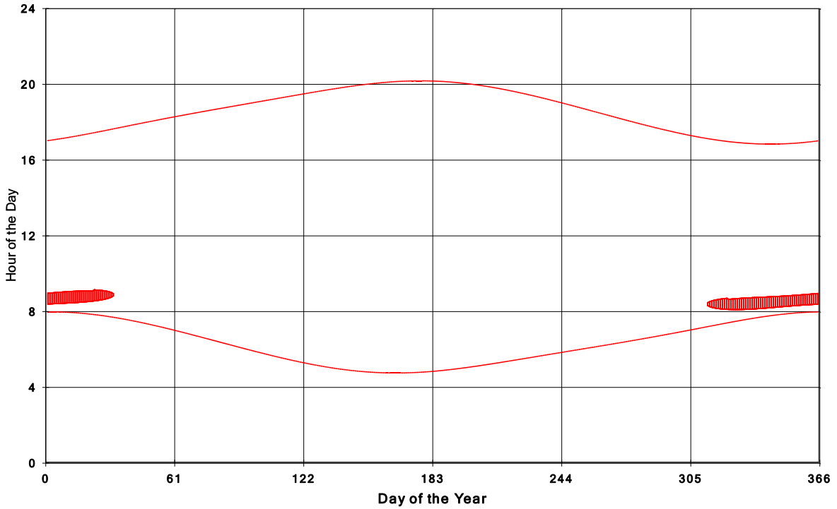
Jericho Wind Energy Centre Shadow Times on House 662, All Windows from All Turbine:
