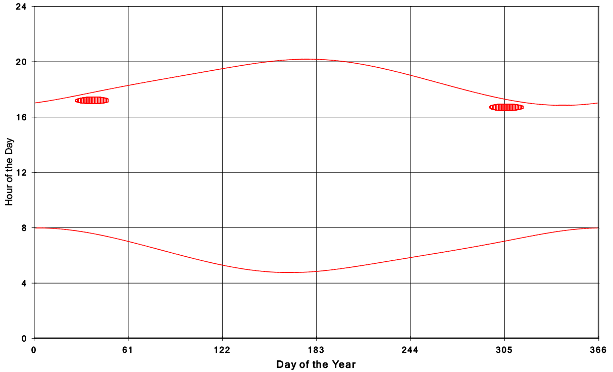
Goshen Wind Energy Centre Shadow Times on House 751, All Windows from All Turbine:
