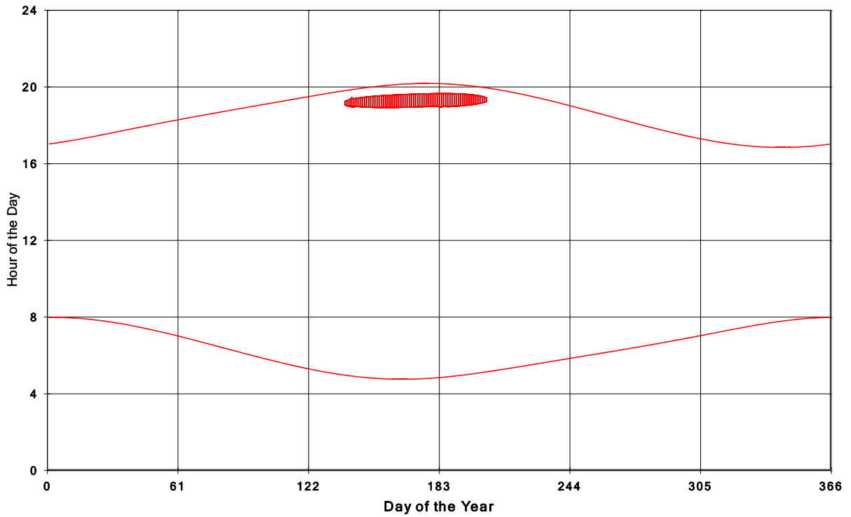
Goshen Wind Energy Centre Shadow Times on House 756, All Windows from All Turbine:
