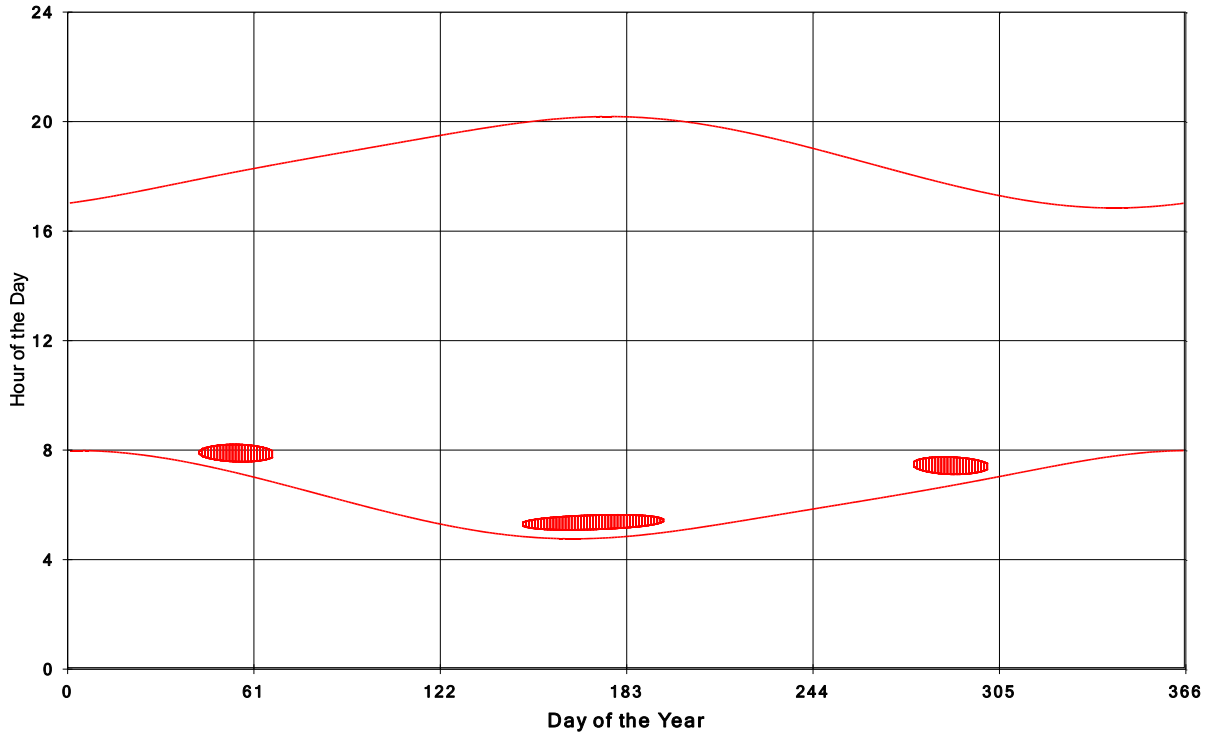
Goshen Wind Energy Centre Shadow Times on House 757, All Windows from All Turbine:
