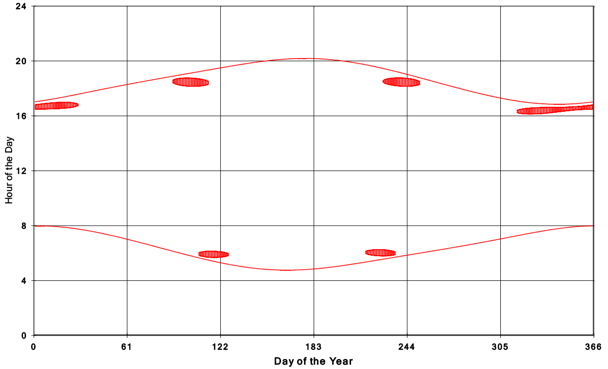
Goshen Wind Energy Centre Shadow Times on House 713, All Windows from All Turbine:
