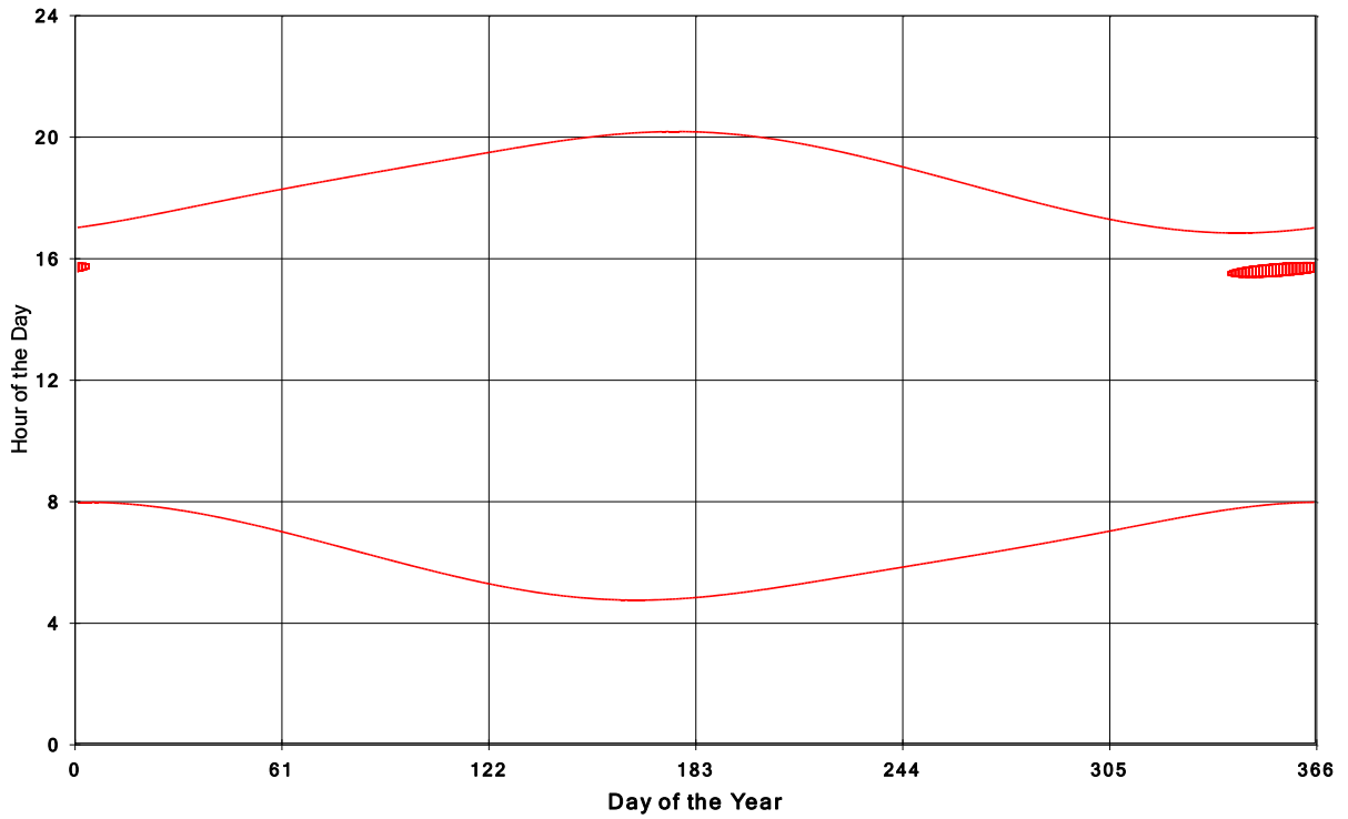
Goshen Wind Energy Centre Shadow Times on House 735, All Windows from All Turbine:
