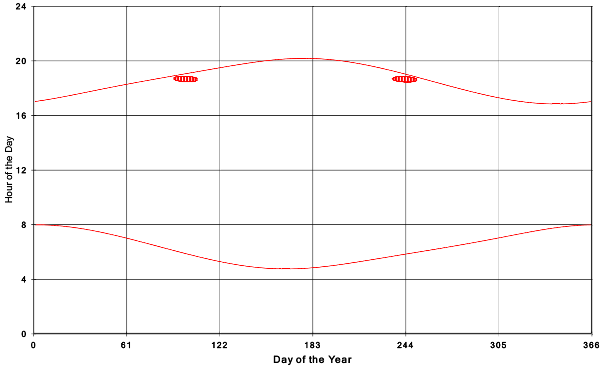
Goshen Wind Energy Centre Shadow Times on House 759, All Windows from All Turbine:
