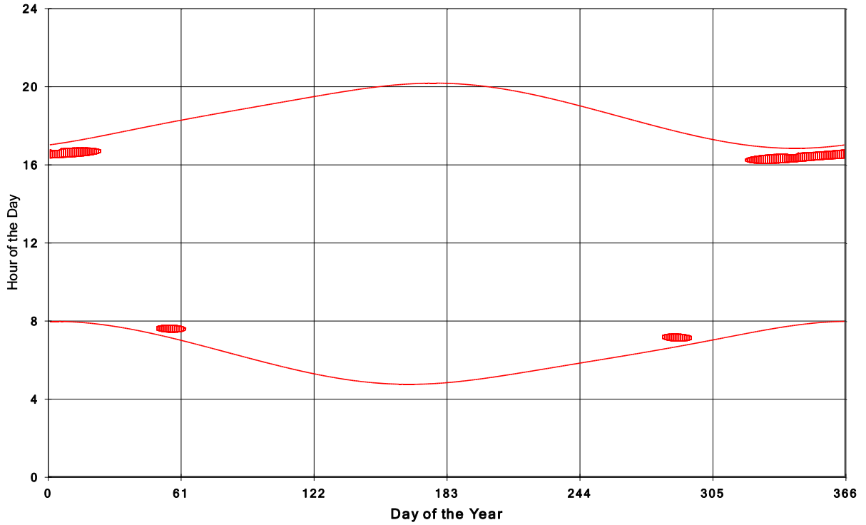
Goshen Wind Energy Centre Shadow Times on House 703, All Windows from All Turbine:
