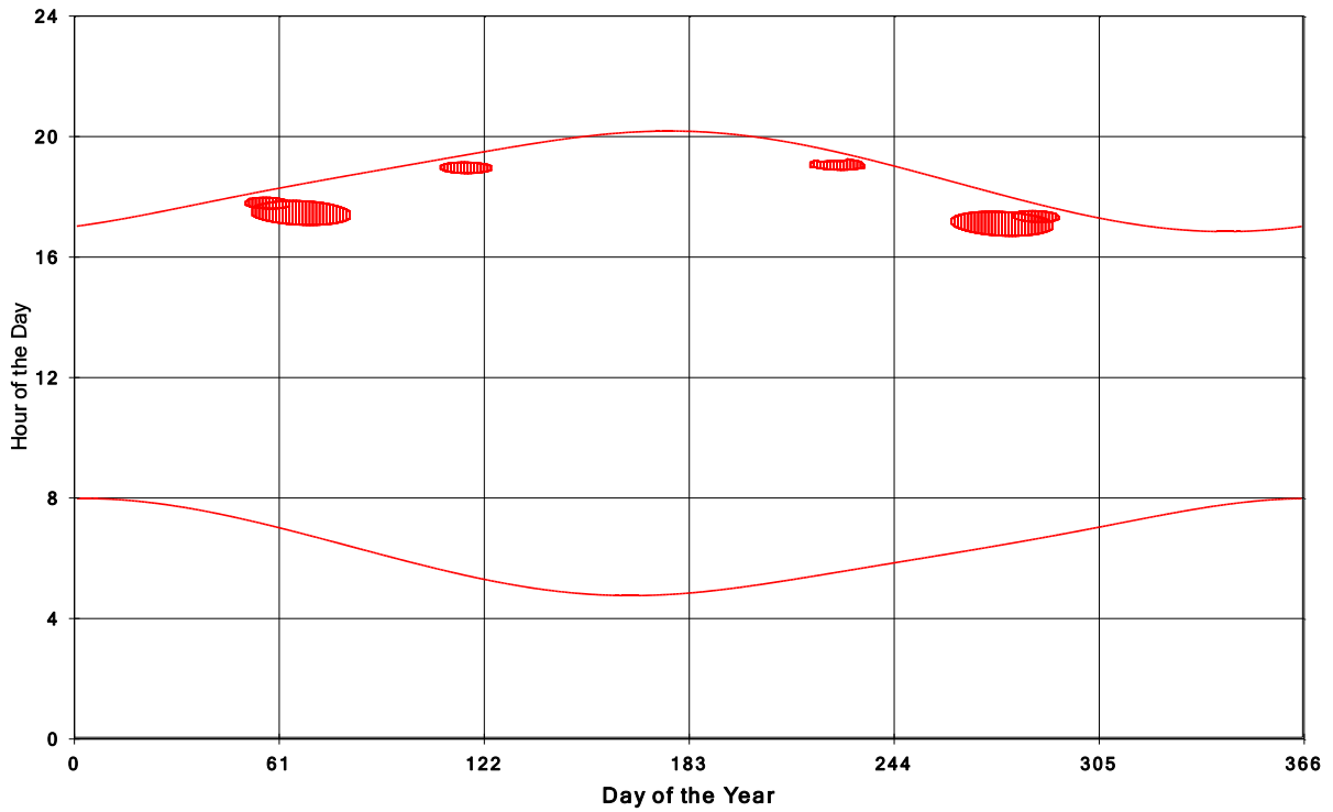
Goshen Wind Energy Centre Shadow Times on House 727, All Windows from All Turbine:
