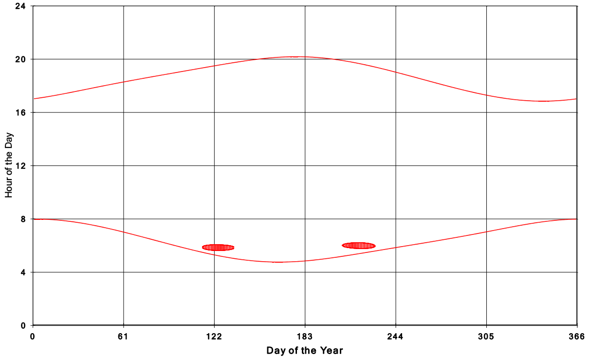
Goshen Wind Energy Centre Shadow Times on House 680, All Windows from All Turbine:
