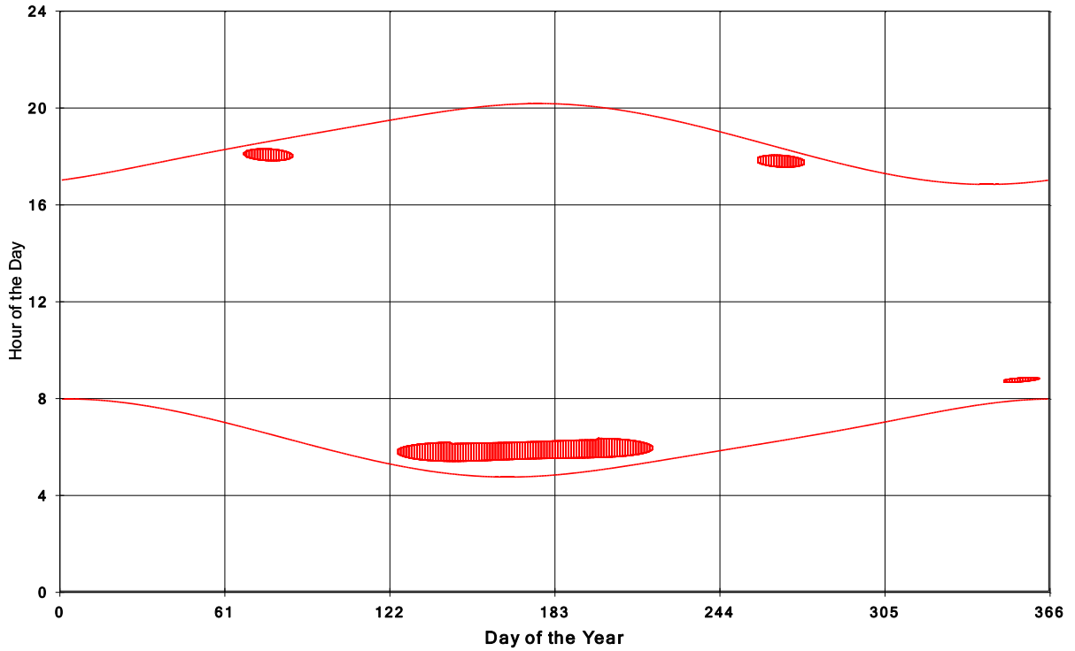
Goshen Wind Energy Centre Shadow Times on House 744, All Windows from All Turbine:
