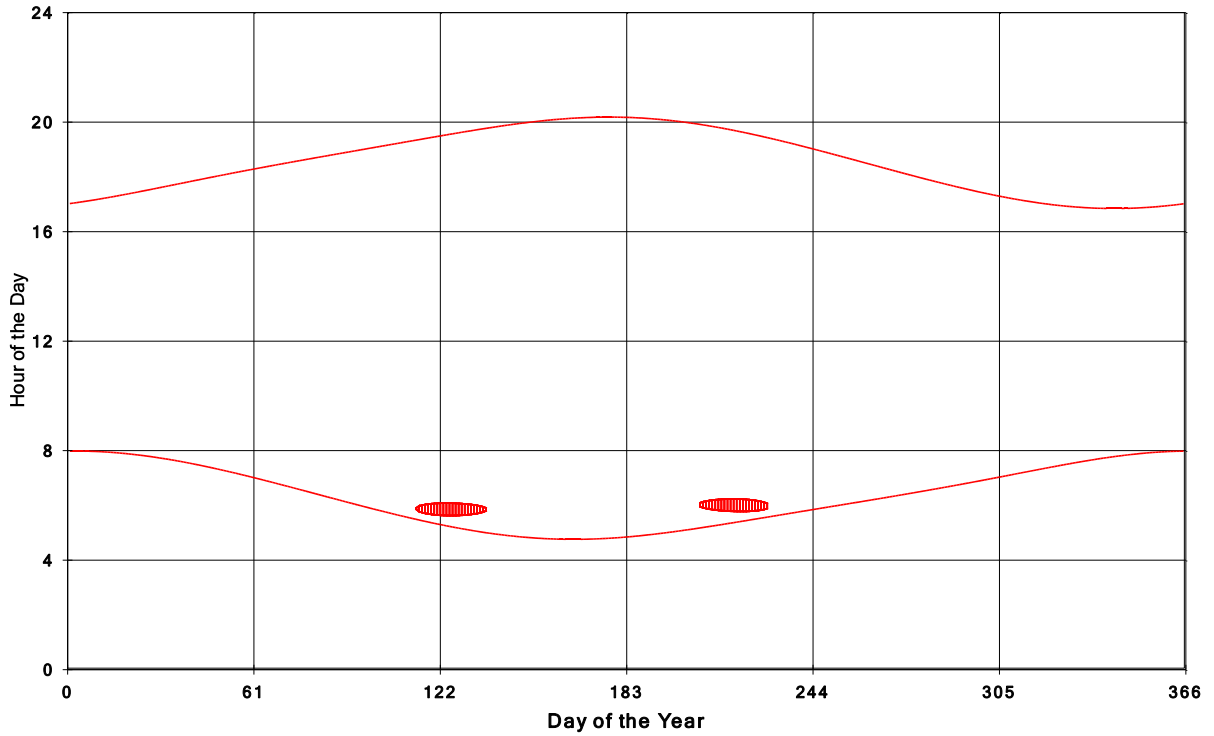
Goshen Wind Energy Centre Shadow Times on House 681, All Windows from All Turbine:
