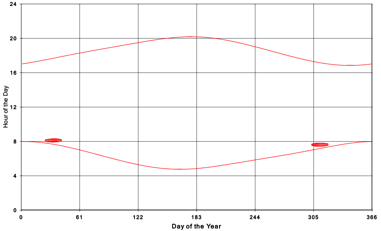
Goshen Wind Energy Centre Shadow Times on House 829, All Windows from All Turbine:
