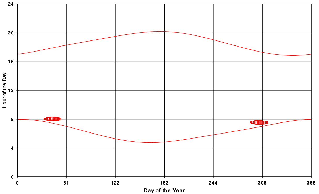
Jericho Wind Energy Centre Shadow Times on House 660, All Windows from All Turbine:
