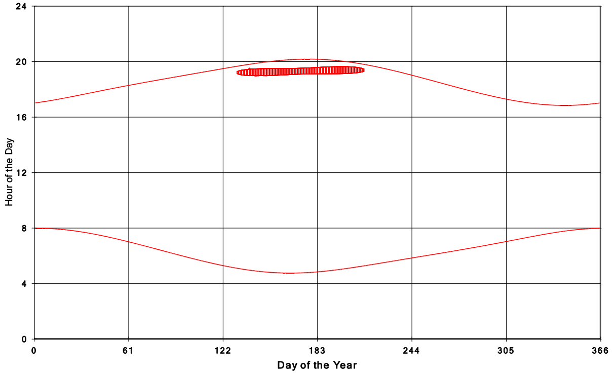
Goshen Wind Energy Centre Shadow Times on House 748, All Windows from All Turbine:
