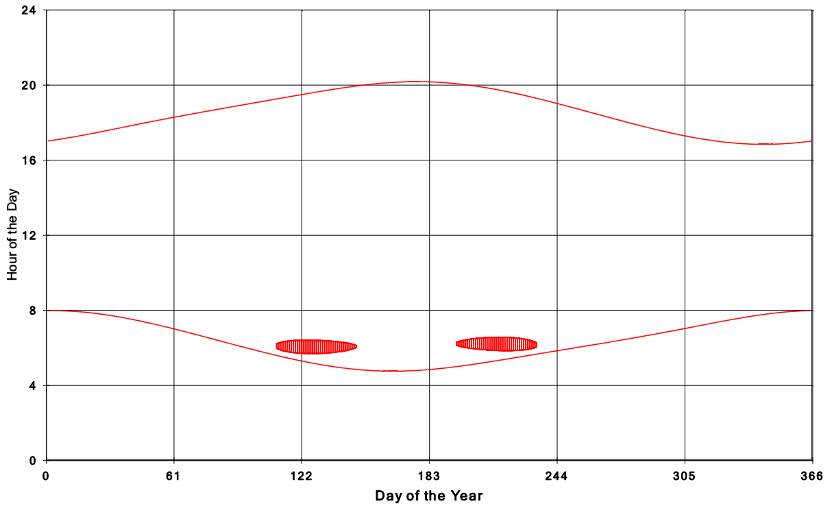
Goshen Wind Energy Centre Shadow Times on House 689, All Windows from All Turbine:
