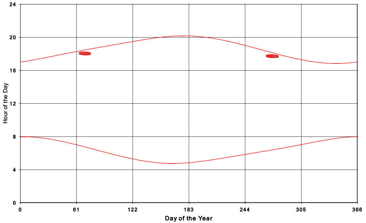
Goshen Wind Energy Centre Shadow Times on House 805, All Windows from All Turbine:
