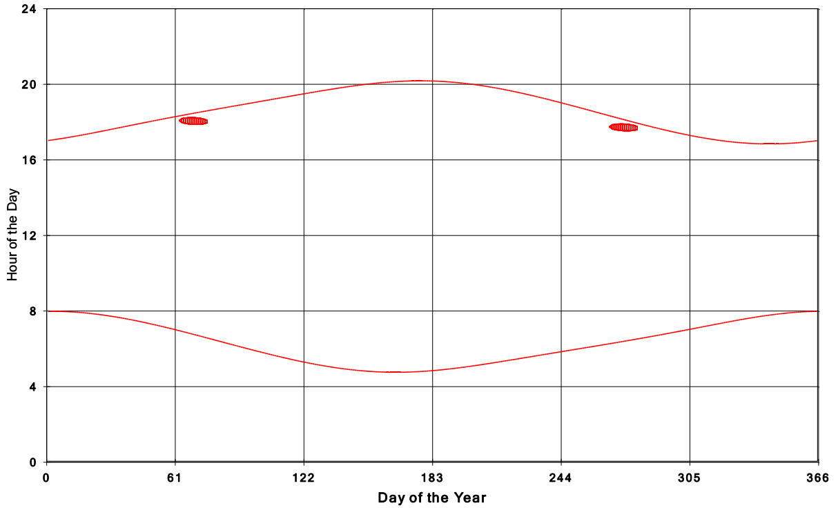
Goshen Wind Energy Centre Shadow Times on House 804, All Windows from All Turbine:
