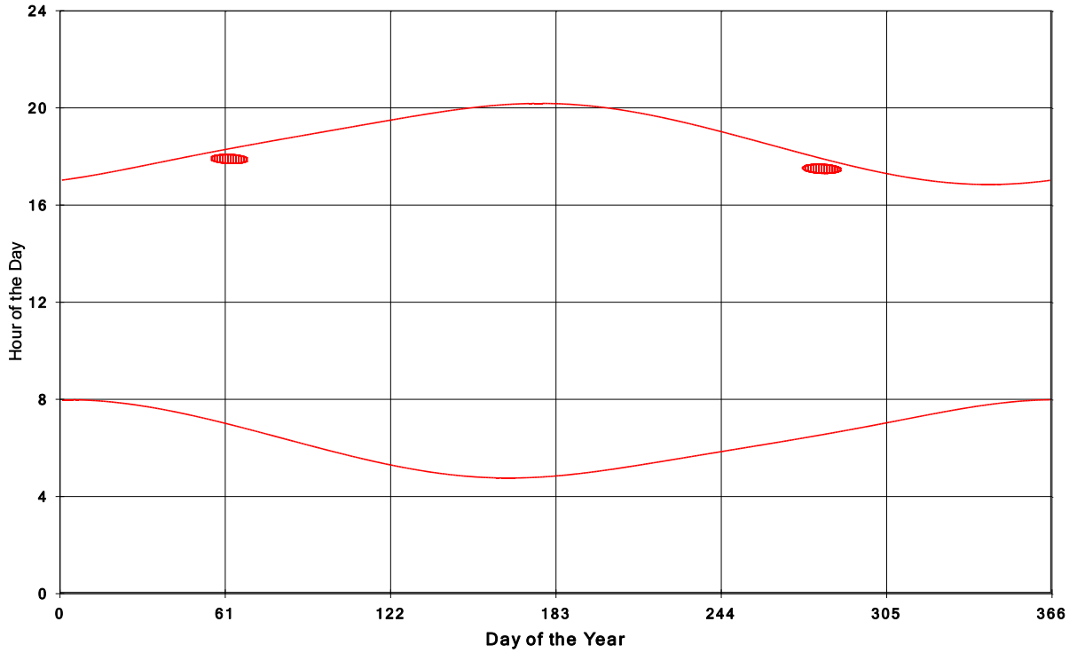
Goshen Wind Energy Centre Shadow Times on House 803, All Windows from All Turbine:
