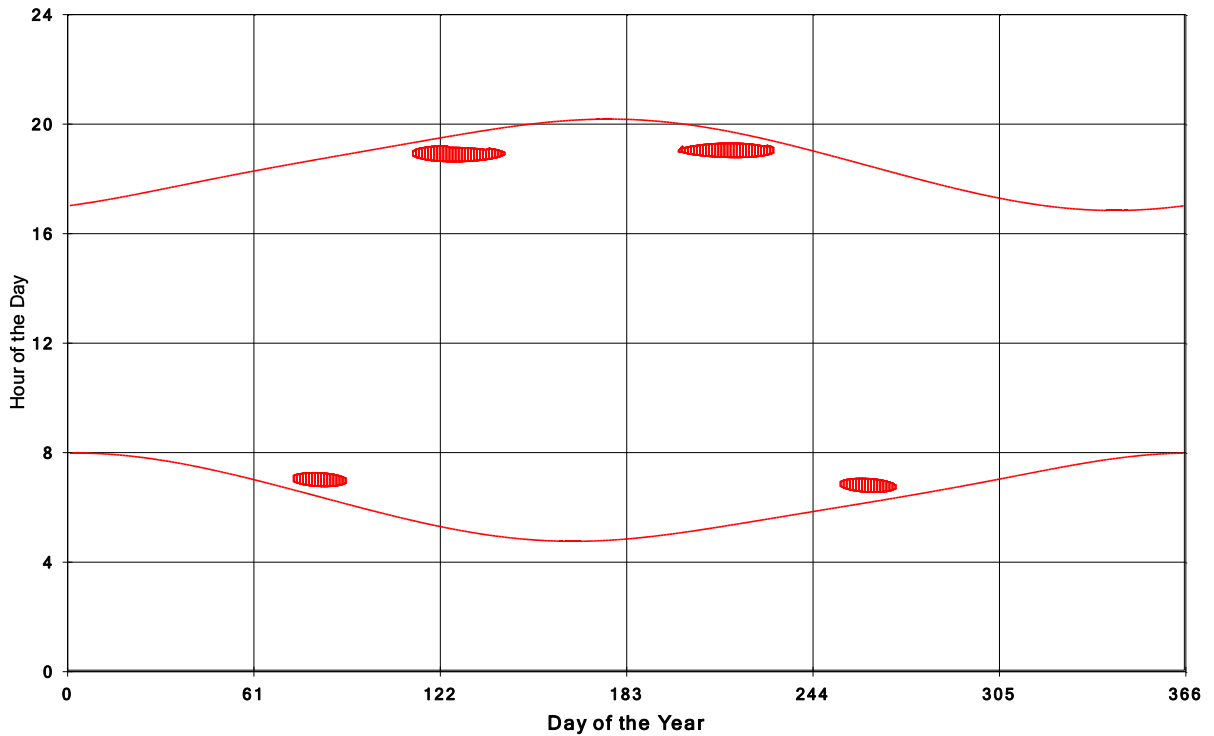
Goshen Wind Energy Centre Shadow Times on House 704, All Windows from All Turbine:
