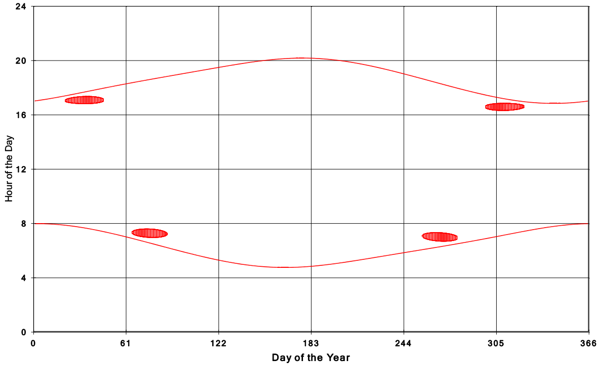
Goshen Wind Energy Centre Shadow Times on House 742, All Windows from All Turbine:
