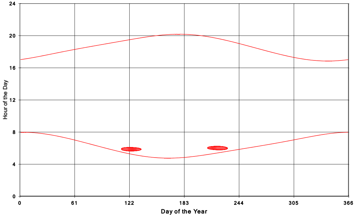
Goshen Wind Energy Centre Shadow Times on House 705, All Windows from All Turbine:
