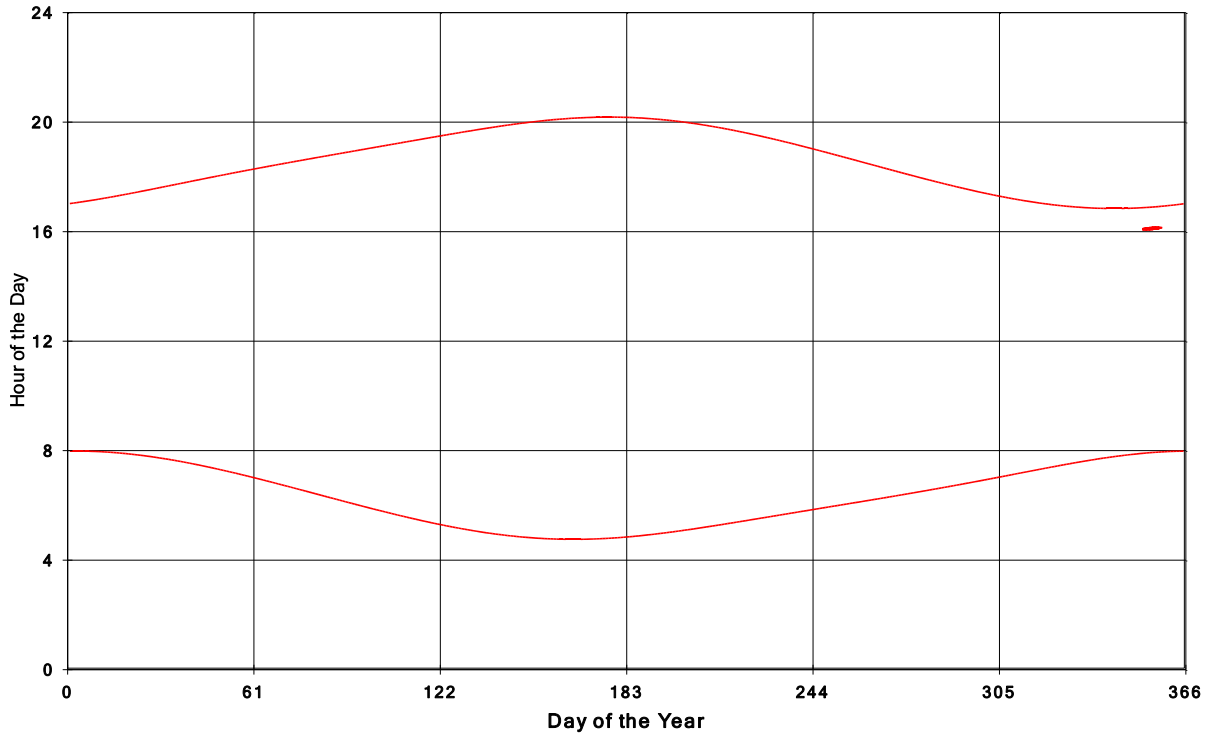
Goshen Wind Energy Centre Shadow Times on House 813, All Windows from All Turbine:
