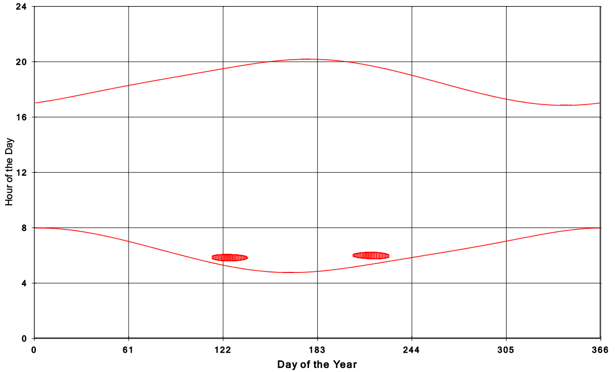
Goshen Wind Energy Centre Shadow Times on House 706, All Windows from All Turbine:
