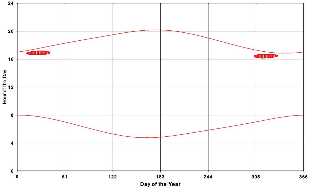
Goshen Wind Energy Centre Shadow Times on House 489, All Windows from All Turbine:
