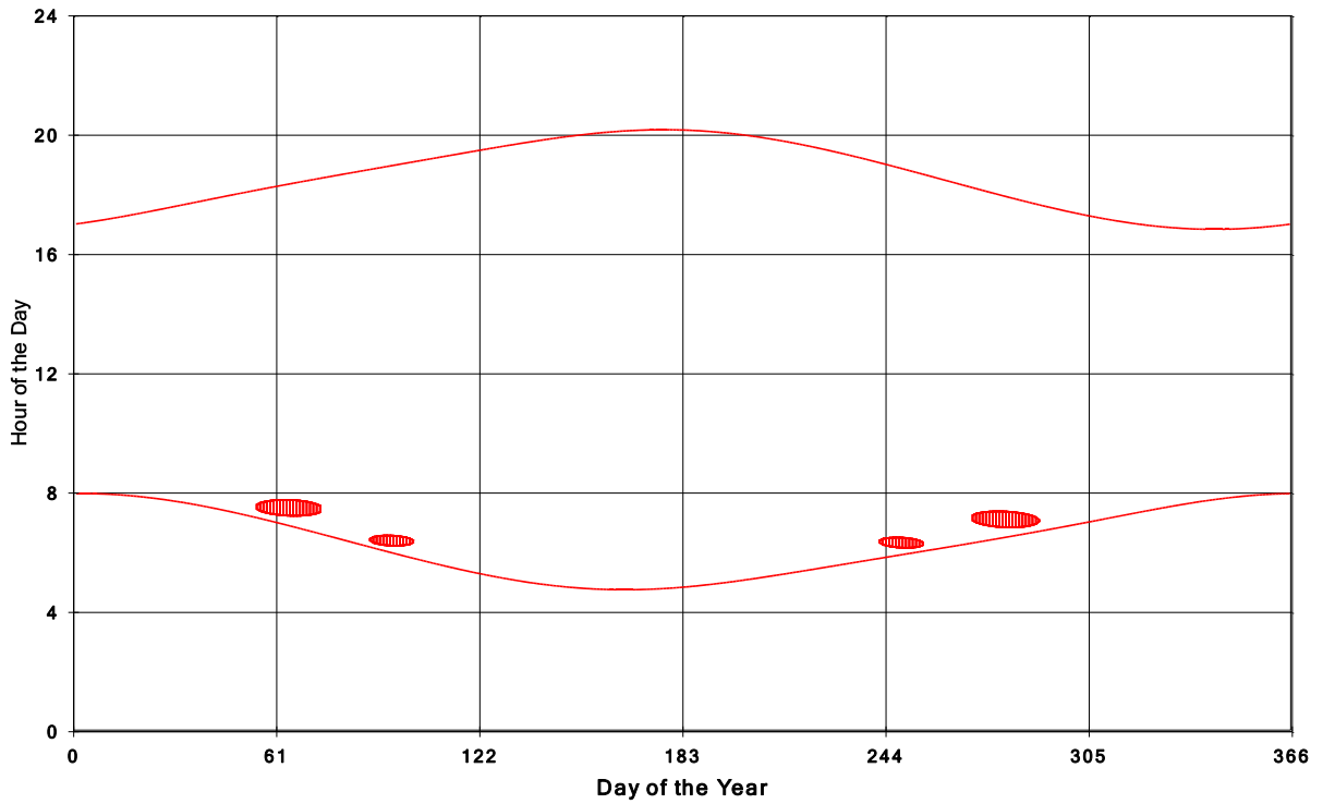
Goshen Wind Energy Centre Shadow Times on House 602, All Windows from All Turbine:
