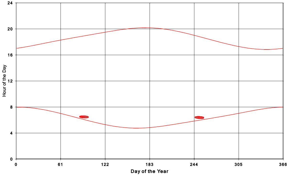
Goshen Wind Energy Centre Shadow Times on House 552, All Windows from All Turbine:
