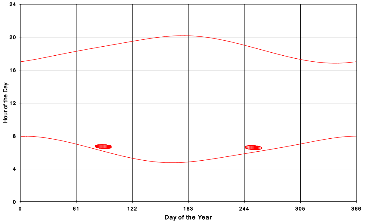
Goshen Wind Energy Centre Shadow Times on House 463, All Windows from All Turbine:
