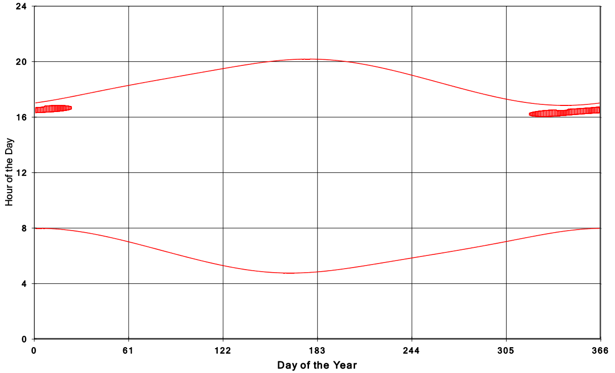
Goshen Wind Energy Centre Shadow Times on House 471, All Windows from All Turbine:
