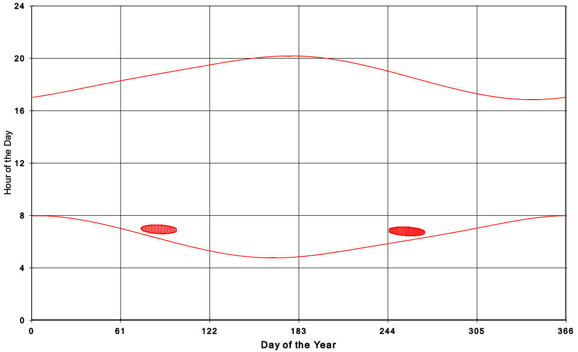
Jericho Wind Energy Centre Shadow Times on House 618, All Windows from All Turbine:
