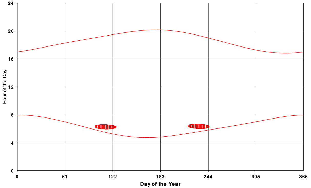
Goshen Wind Energy Centre Shadow Times on House 633, All Windows from All Turbine:
