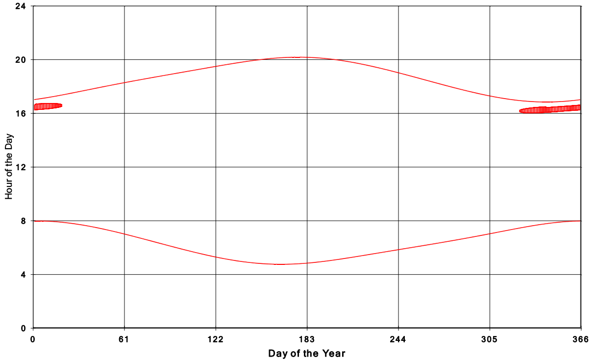
Goshen Wind Energy Centre Shadow Times on House 473, All Windows from All Turbine:
