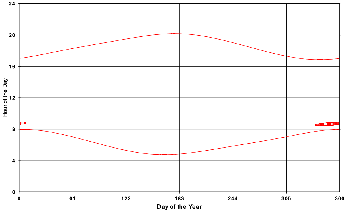
Goshen Wind Energy Centre Shadow Times on House 615, All Windows from All Turbine:
