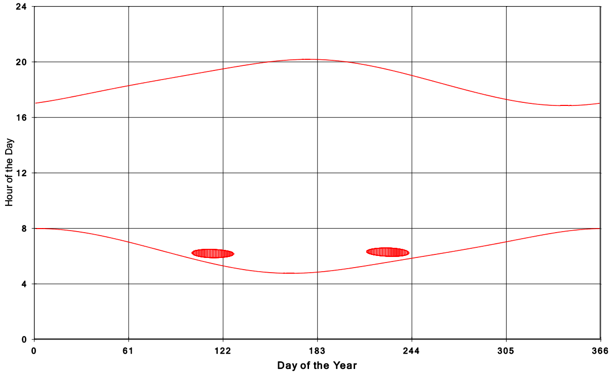
Goshen Wind Energy Centre Shadow Times on House 583, All Windows from All Turbine:
