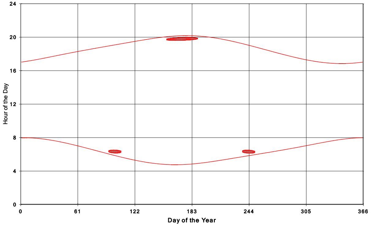
Goshen Wind Energy Centre Shadow Times on House 570, All Windows from All Turbine:
