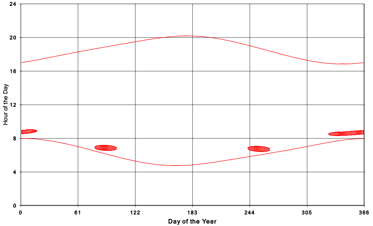
Goshen Wind Energy Centre Shadow Times on House 643, All Windows from All Turbine:
