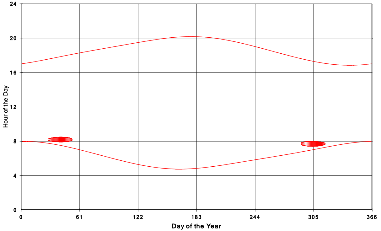
Goshen Wind Energy Centre Shadow Times on House 488, All Windows from All Turbine:
