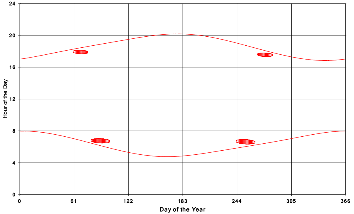
Goshen Wind Energy Centre Shadow Times on House 565, All Windows from All Turbine:
