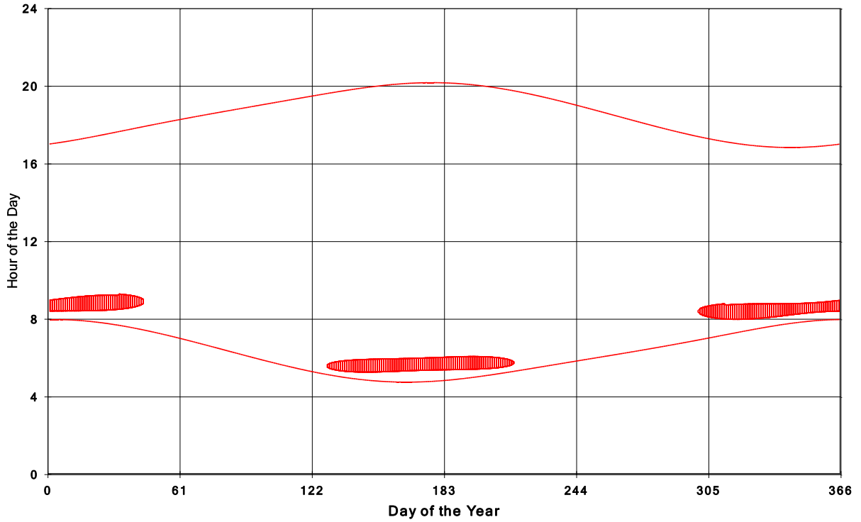
Goshen Wind Energy Centre Shadow Times on House 642, All Windows from All Turbine:
