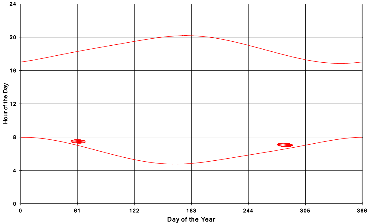
Goshen Wind Energy Centre Shadow Times on House 604, All Windows from All Turbine:
