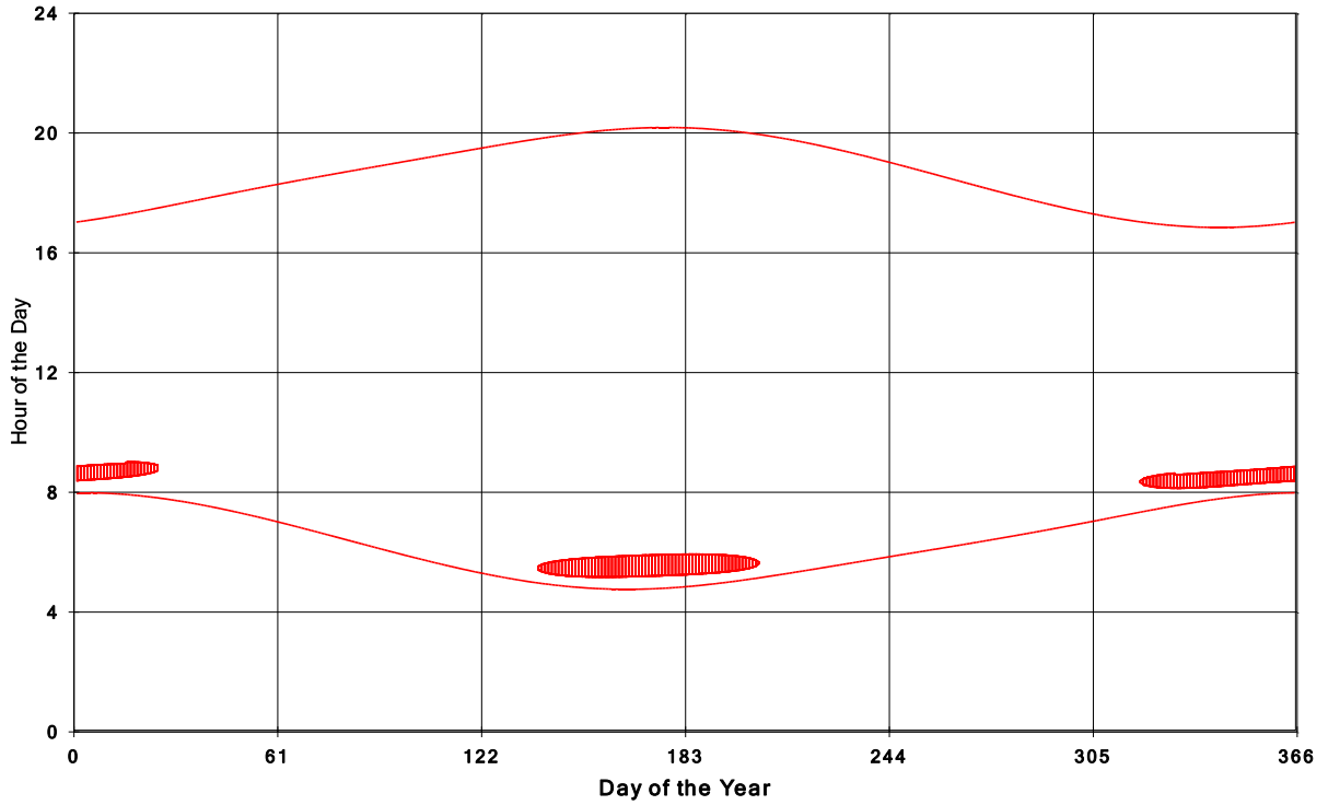
Goshen Wind Energy Centre Shadow Times on House 479, All Windows from All Turbine:
