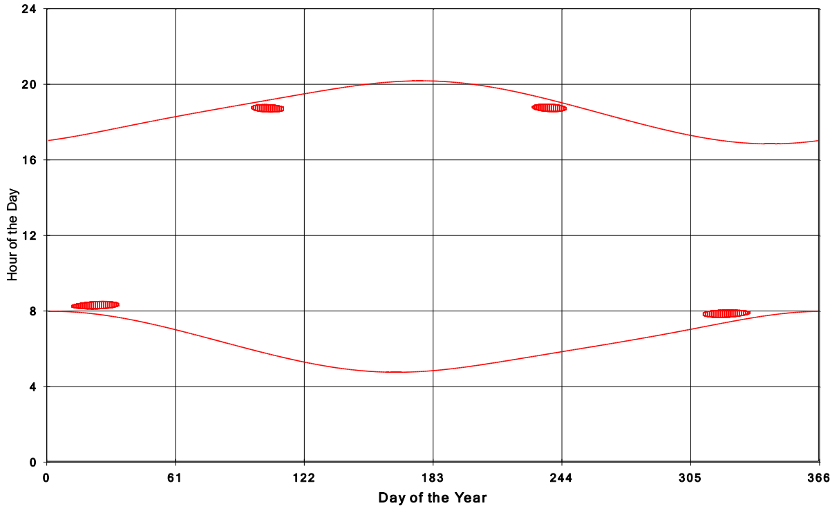
Goshen Wind Energy Centre Shadow Times on House 593, All Windows from All Turbine:
