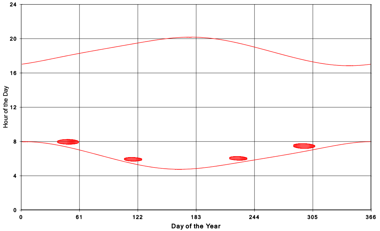
Goshen Wind Energy Centre Shadow Times on House 601, All Windows from All Turbine:
