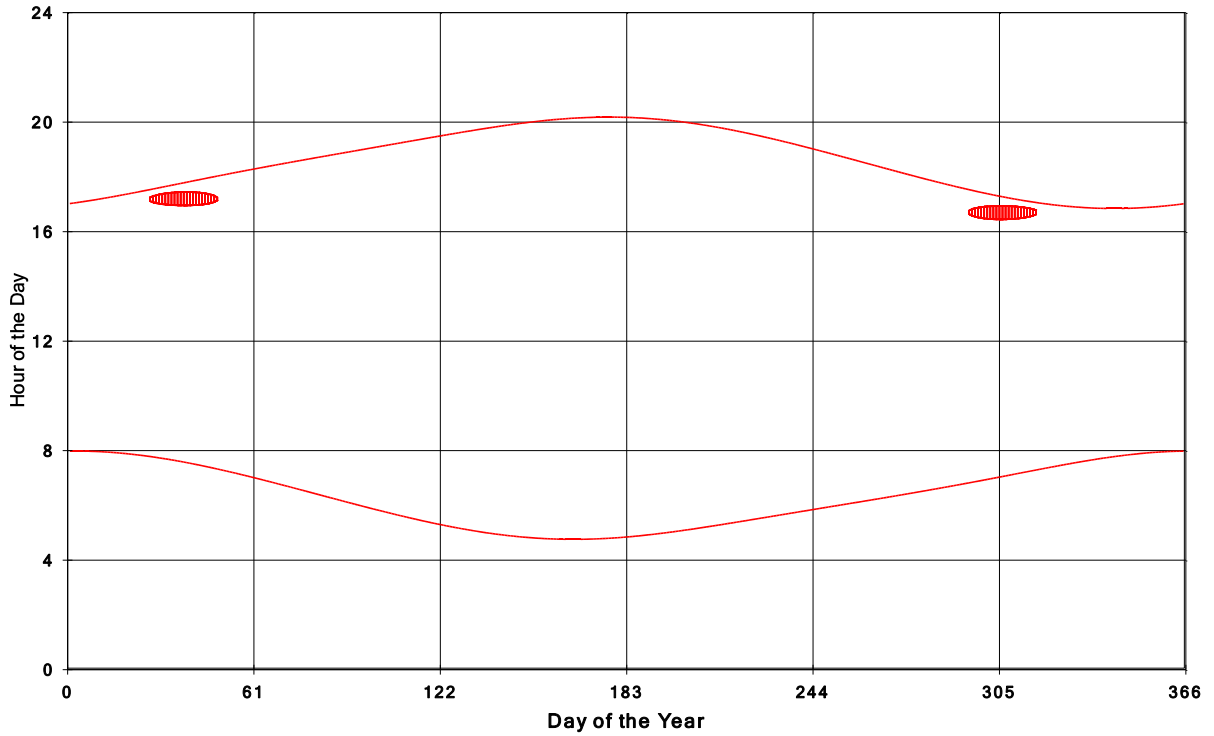
Goshen Wind Energy Centre Shadow Times on House 470, All Windows from All Turbine:
