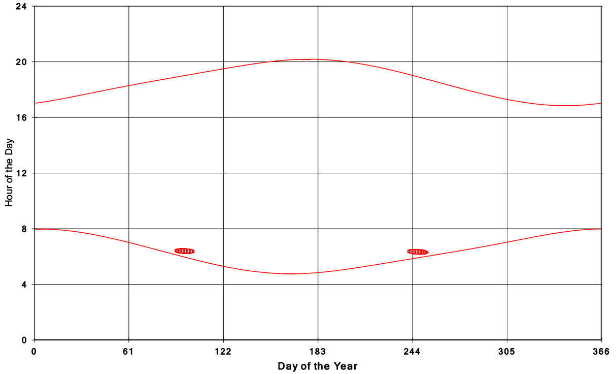
Goshen Wind Energy Centre Shadow Times on House 587, All Windows from All Turbine:
