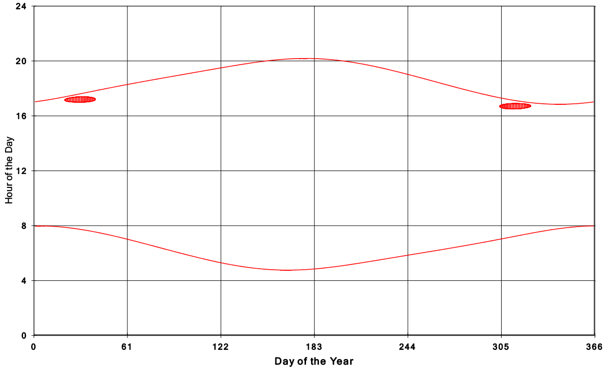
Goshen Wind Energy Centre Shadow Times on House 629, All Windows from All Turbine:
