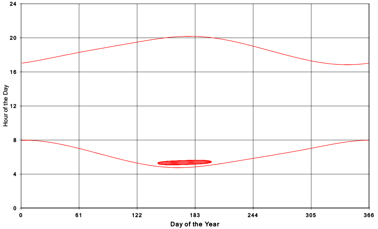
Goshen Wind Energy Centre Shadow Times on House 516, All Windows from All Turbine:
