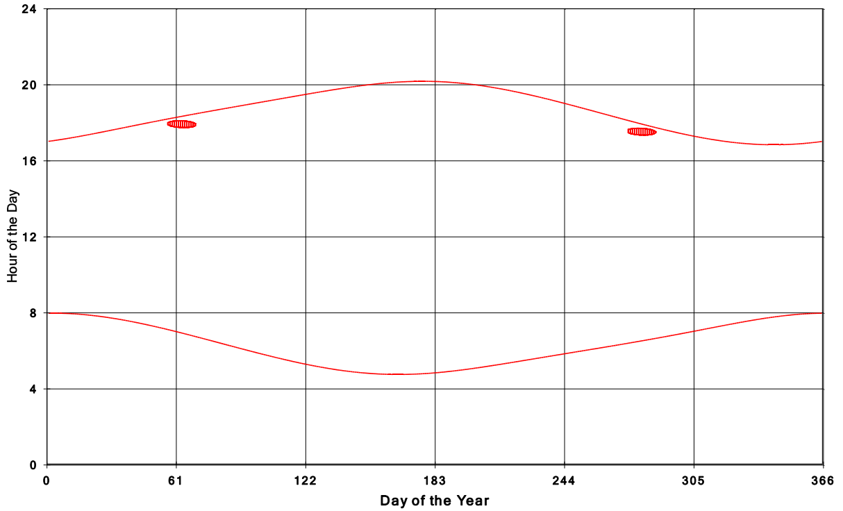
Goshen Wind Energy Centre Shadow Times on House 521, All Windows from All Turbine:
