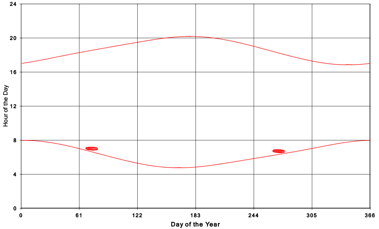
Goshen Wind Energy Centre Shadow Times on House 566, All Windows from All Turbine:
