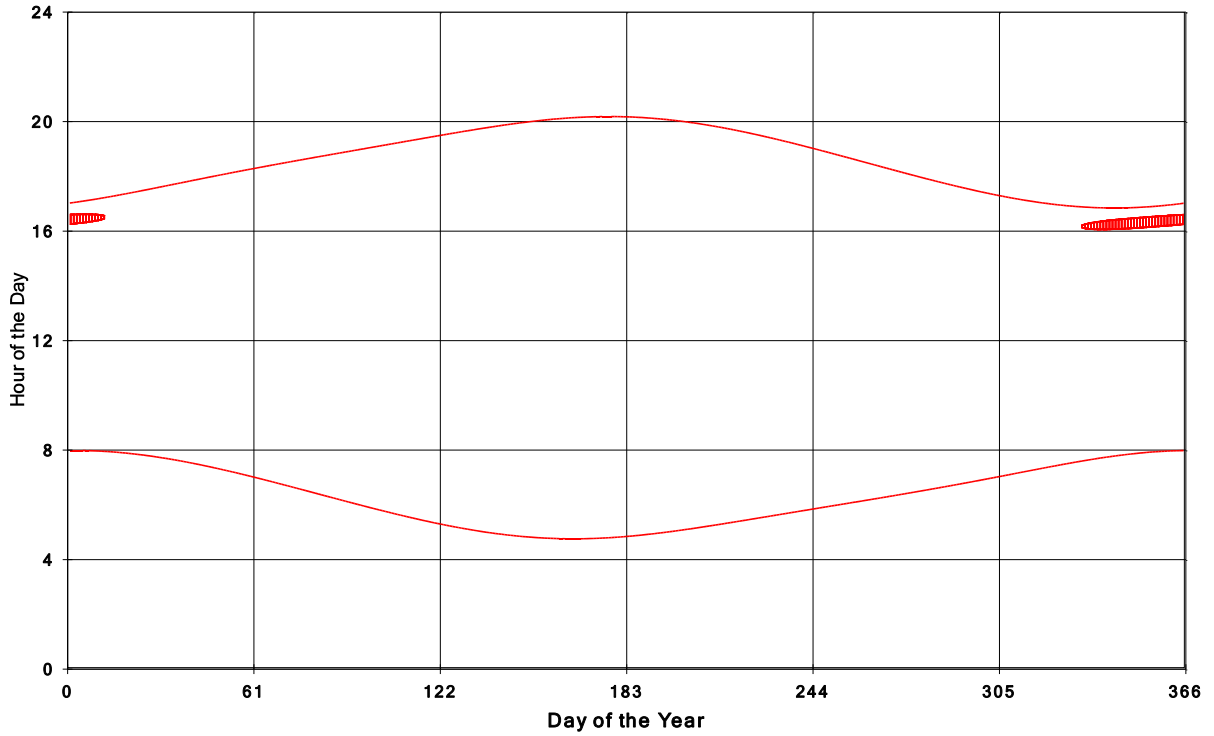
Goshen Wind Energy Centre Shadow Times on House 534, All Windows from All Turbine:
