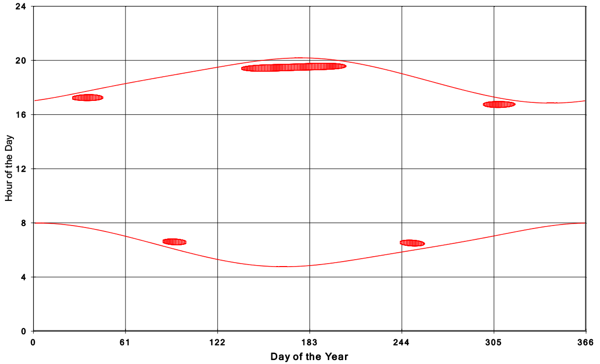
Goshen Wind Energy Centre Shadow Times on House 483, All Windows from All Turbine:
