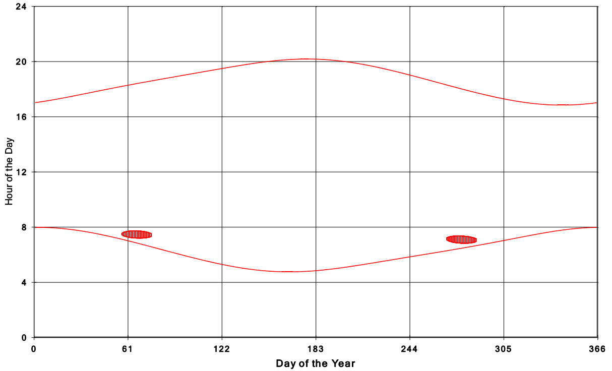
Goshen Wind Energy Centre Shadow Times on House 575, All Windows from All Turbine:
