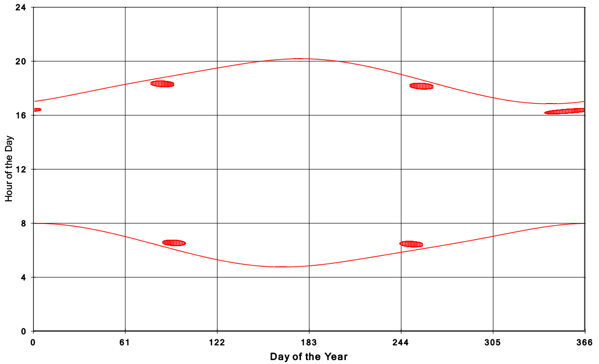
Goshen Wind Energy Centre Shadow Times on House 599, All Windows from All Turbine:
