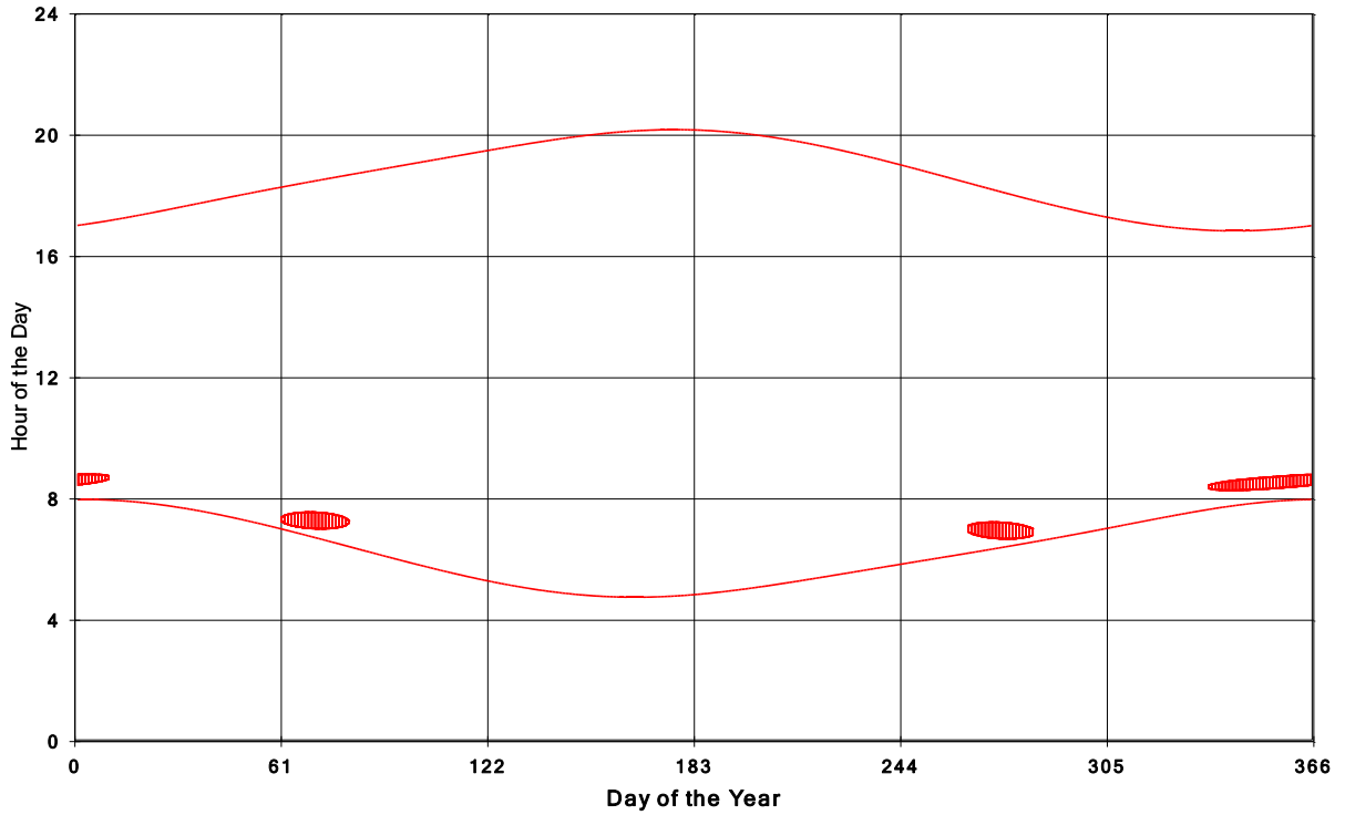
Goshen Wind Energy Centre Shadow Times on House 437, All Windows from All Turbine:
