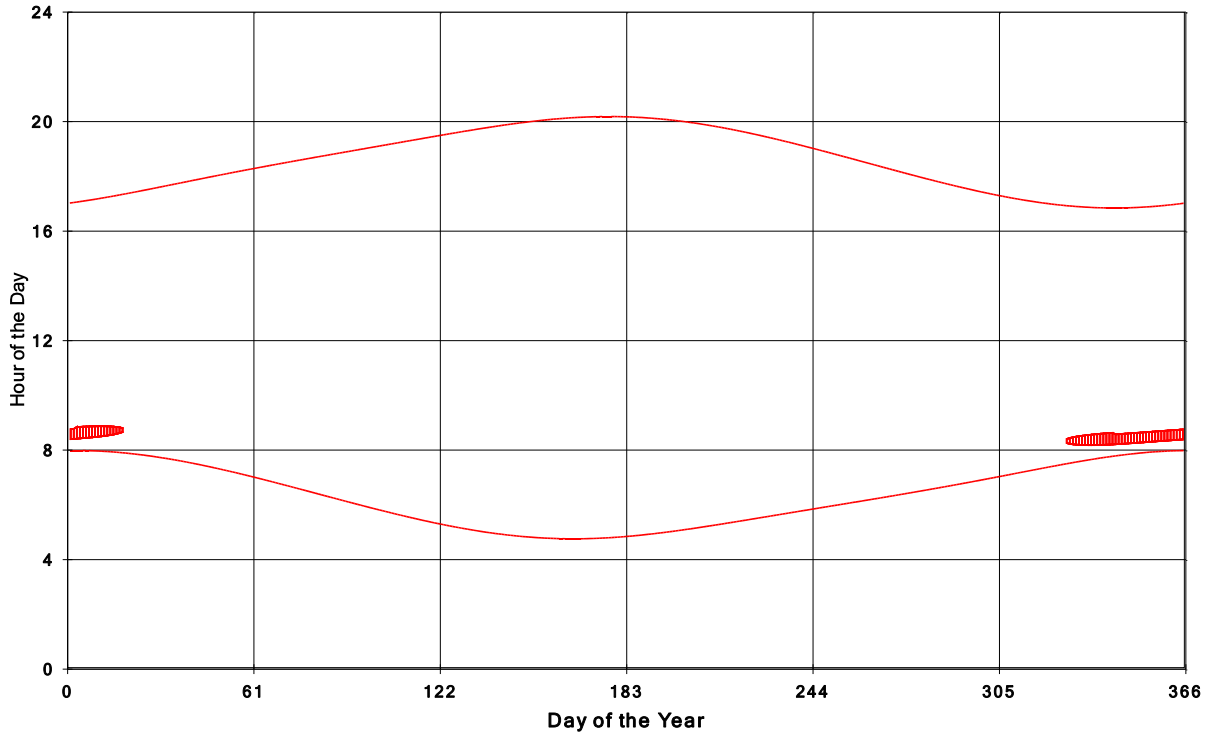
Goshen Wind Energy Centre Shadow Times on House 405, All Windows from All Turbine:
