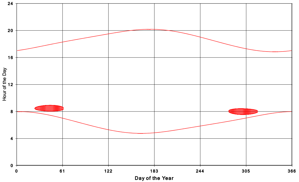
Goshen Wind Energy Centre Shadow Times on House 407, All Windows from All Turbine:
