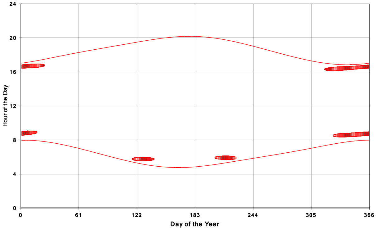
Jericho Wind Energy Centre Shadow Times on House 401, All Windows from All Turbine:
