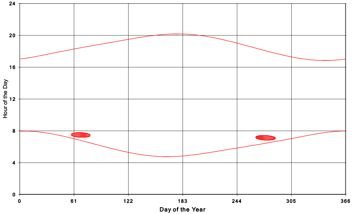
Goshen Wind Energy Centre Shadow Times on House 409, All Windows from All Turbine:
