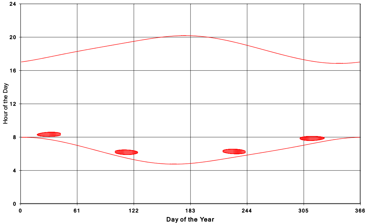
Goshen Wind Energy Centre Shadow Times on House 363, All Windows from All Turbine:
