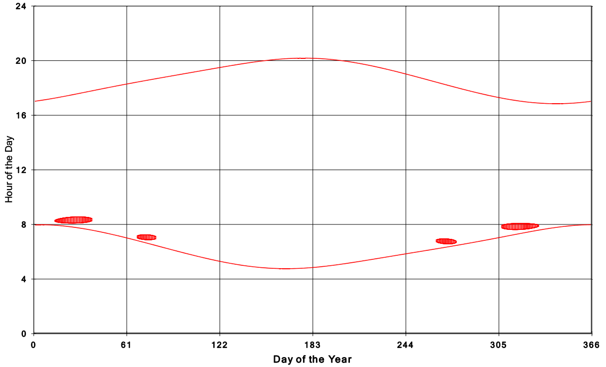
Goshen Wind Energy Centre Shadow Times on House 329, All Windows from All Turbine:
