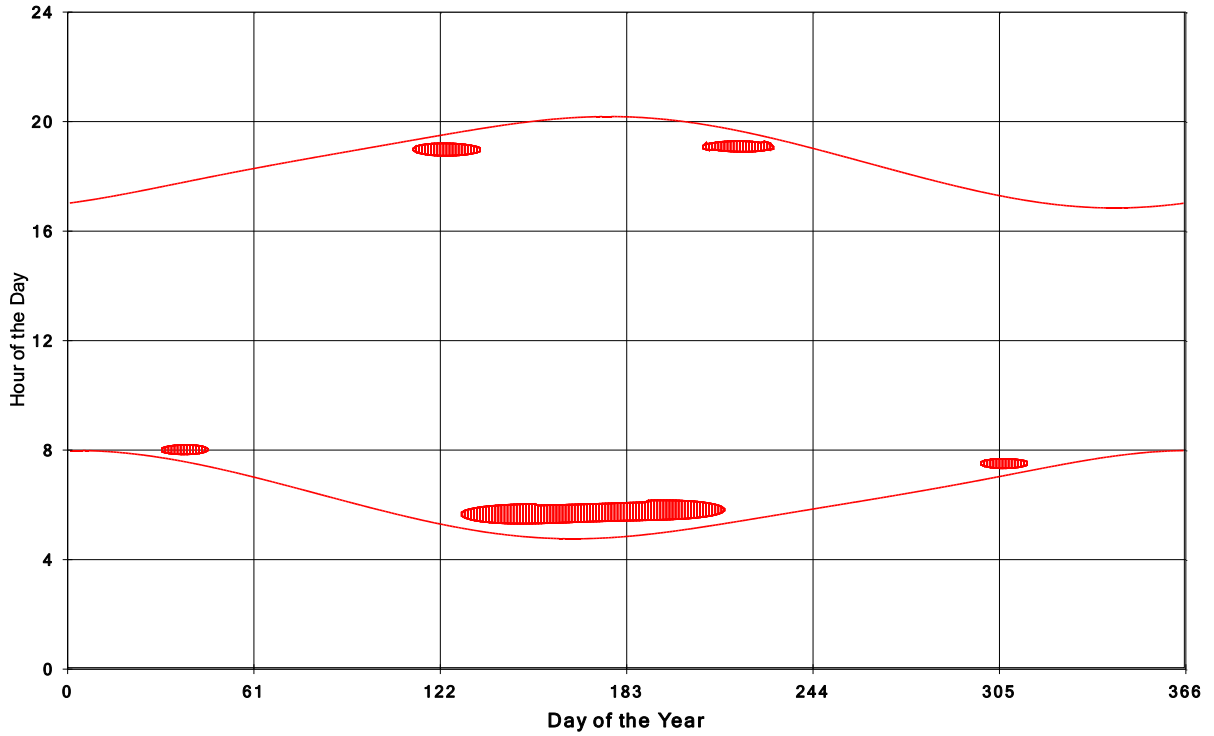
Goshen Wind Energy Centre Shadow Times on House 366, All Windows from All Turbine:
