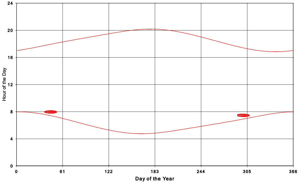
Jericho Wind Energy Centre Shadow Times on House 398, All Windows from All Turbine:
