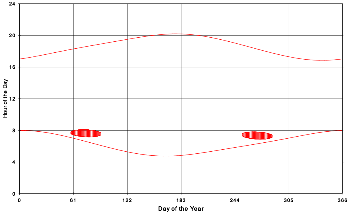
Goshen Wind Energy Centre Shadow Times on House 373, All Windows from All Turbine:
