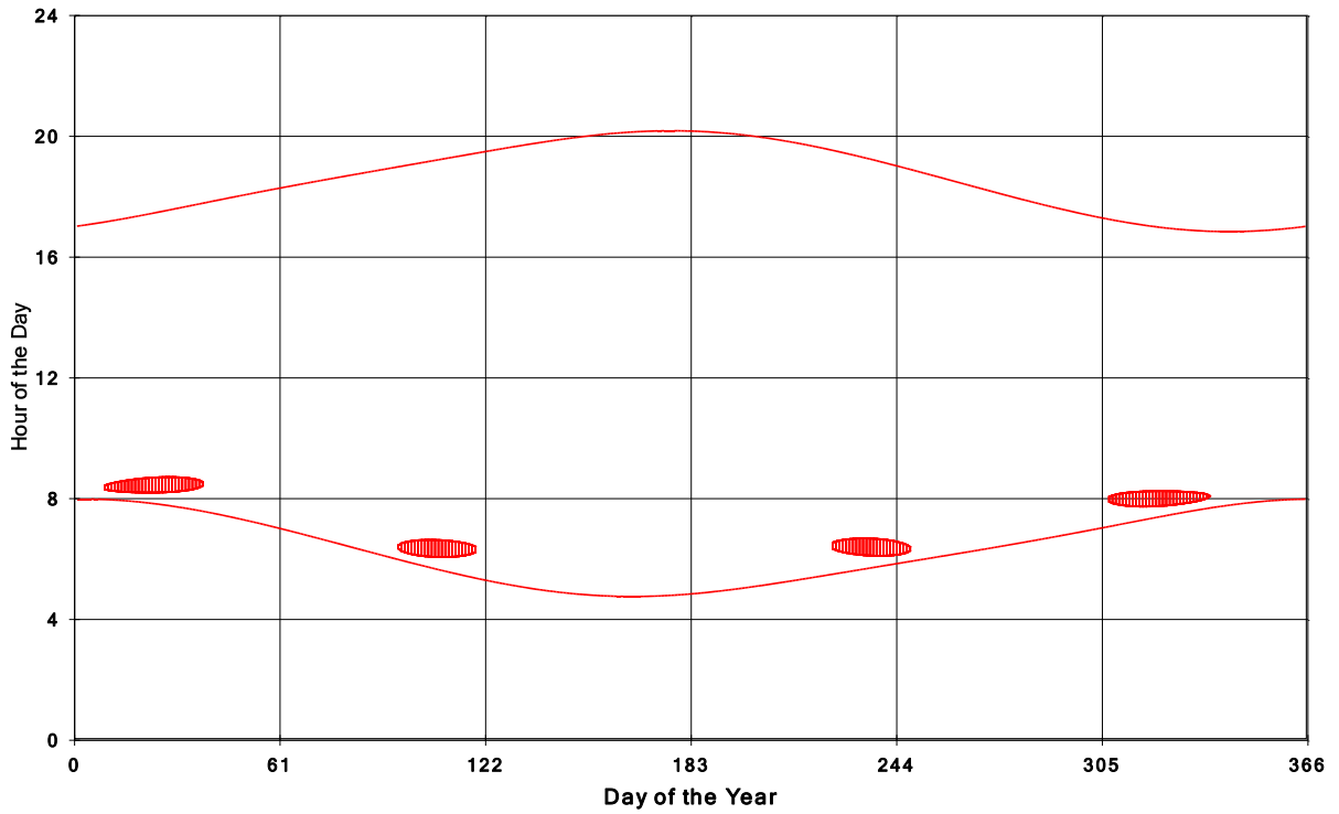
Goshen Wind Energy Centre Shadow Times on House 364, All Windows from All Turbine:
