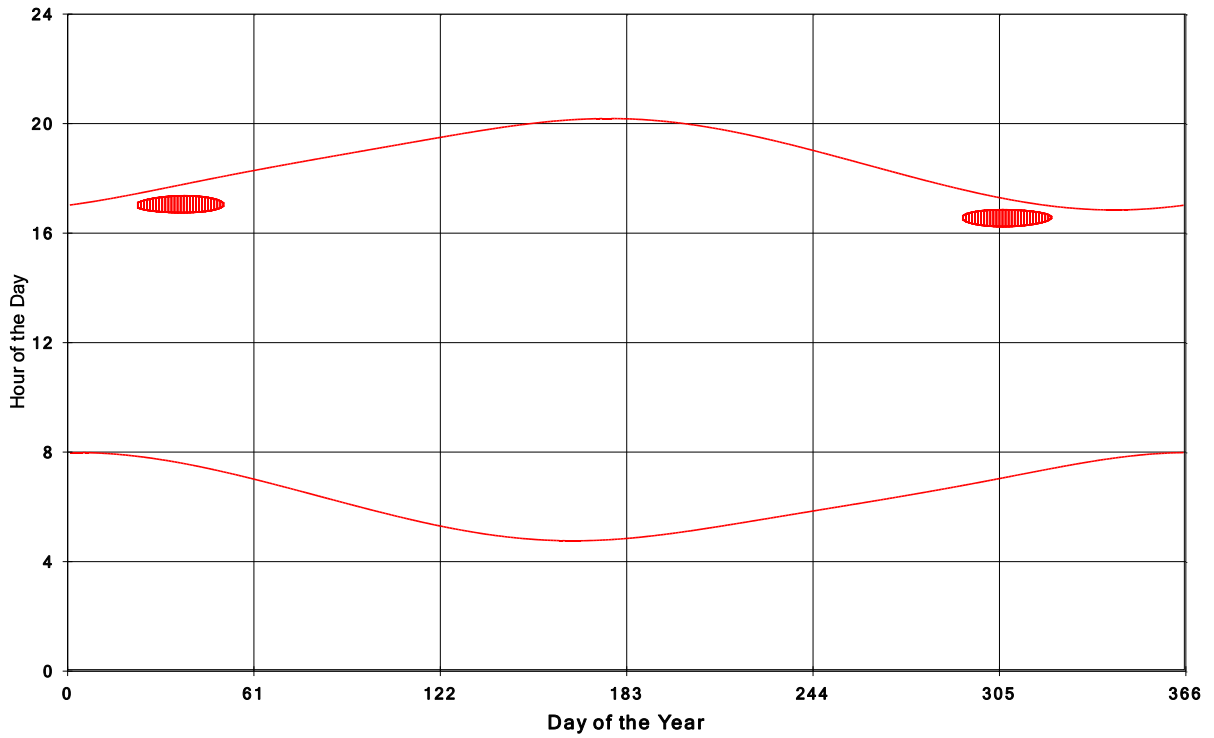
Goshen Wind Energy Centre Shadow Times on House 452, All Windows from All Turbine:
