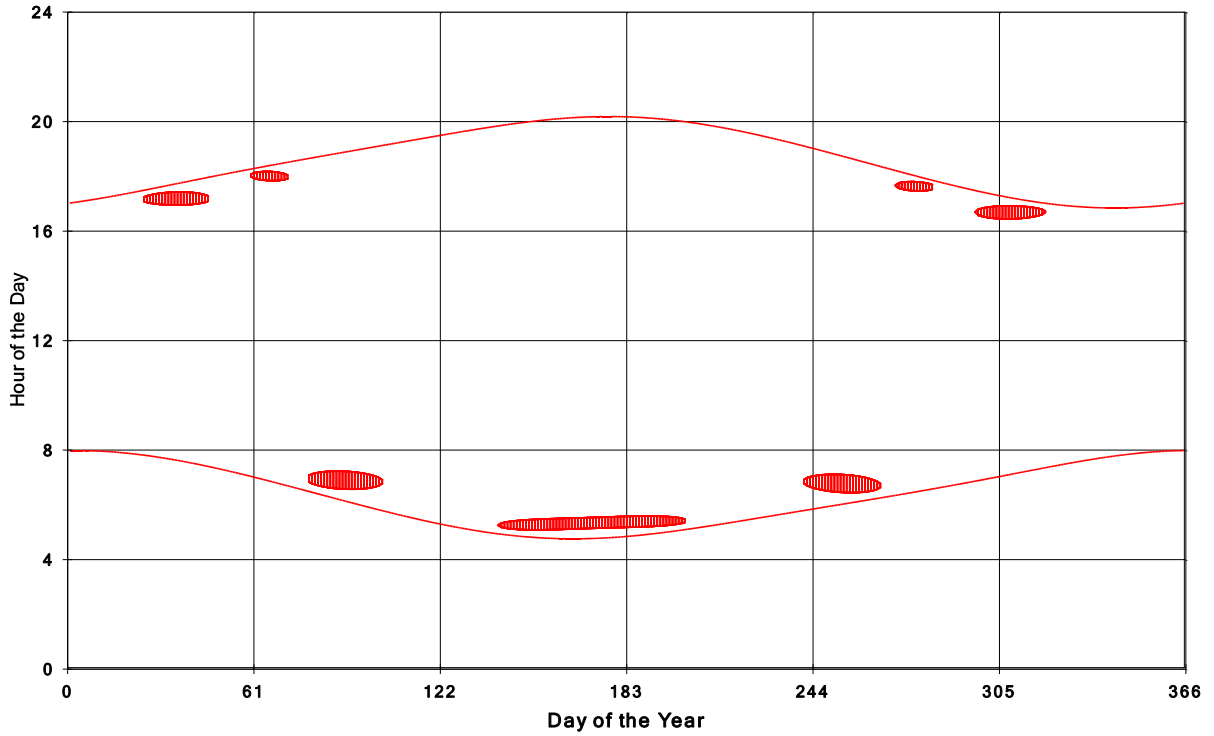
Goshen Wind Energy Centre Shadow Times on House 362, All Windows from All Turbine:
