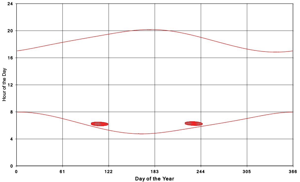
Jericho Wind Energy Centre Shadow Times on House 355, All Windows from All Turbine:
