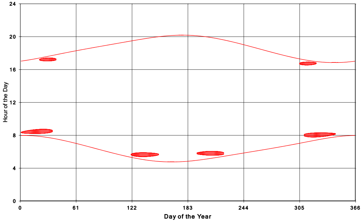
Goshen Wind Energy Centre Shadow Times on House 439, All Windows from All Turbine:
