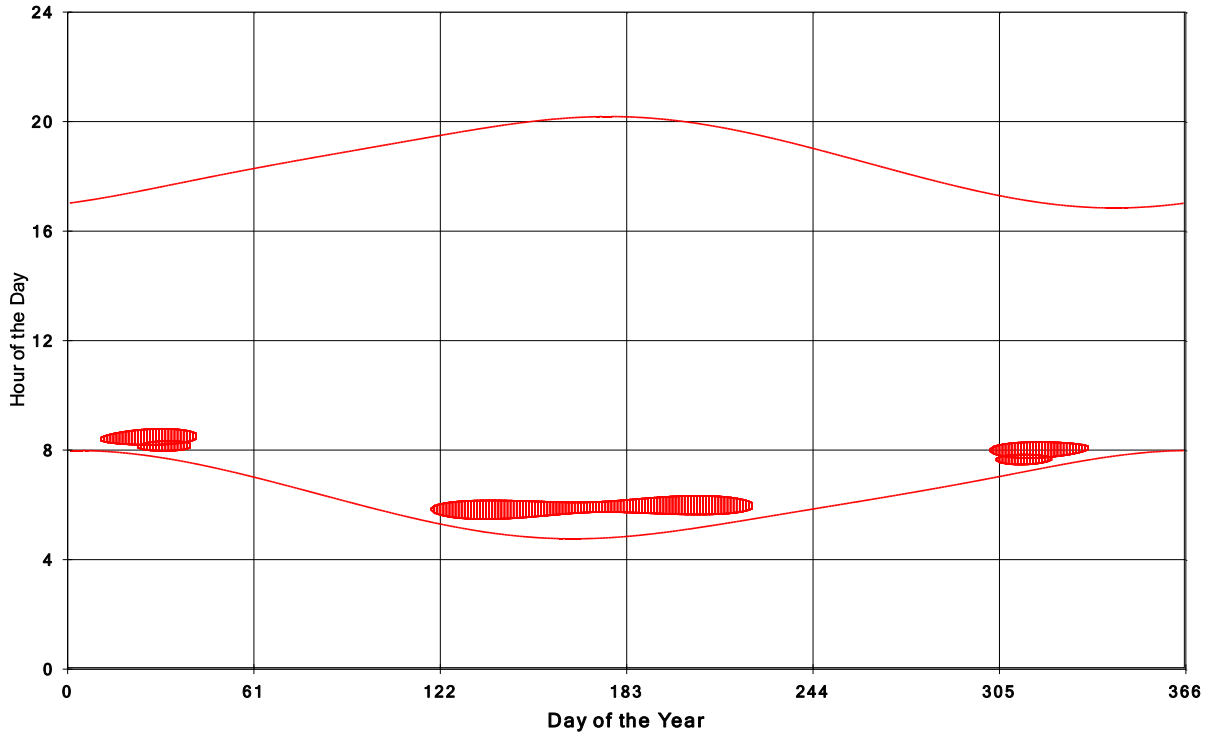
Goshen Wind Energy Centre Shadow Times on House 368, All Windows from All Turbine:
