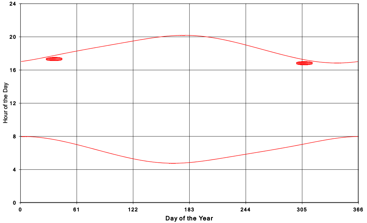
Goshen Wind Energy Centre Shadow Times on House 360, All Windows from All Turbine:
