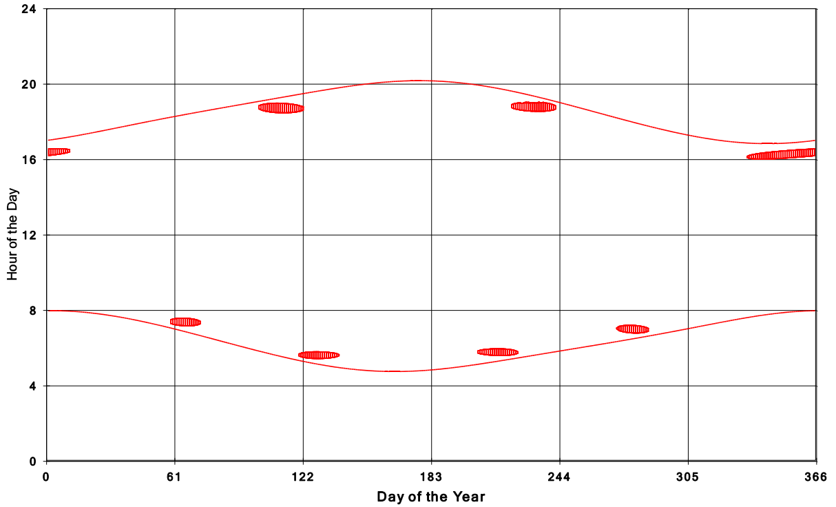
Goshen Wind Energy Centre Shadow Times on House 426, All Windows from All Turbine:
