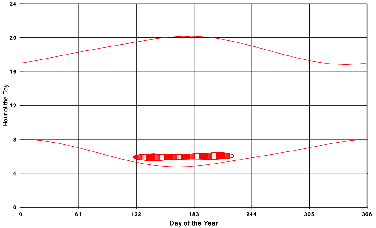
Goshen Wind Energy Centre Shadow Times on House 458, All Windows from All Turbine:
