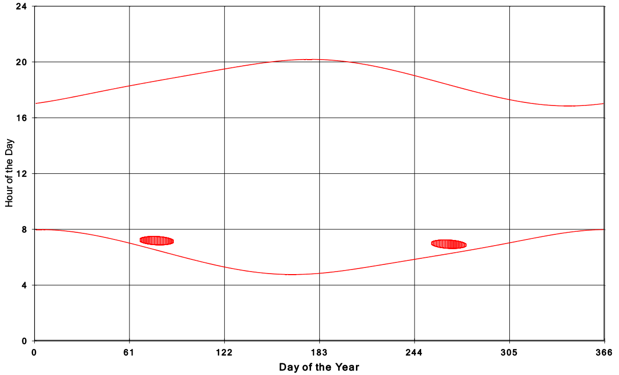
Goshen Wind Energy Centre Shadow Times on House 382, All Windows from All Turbine:
