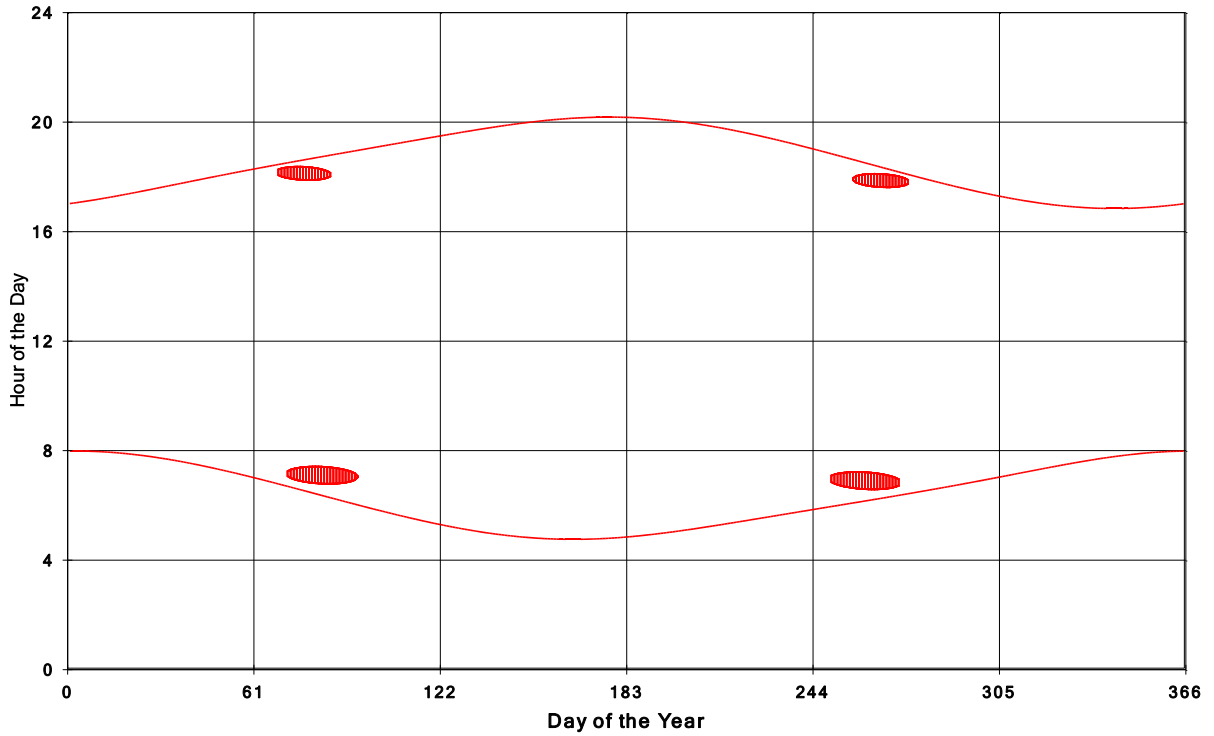
Goshen Wind Energy Centre Shadow Times on House 404, All Windows from All Turbine:
