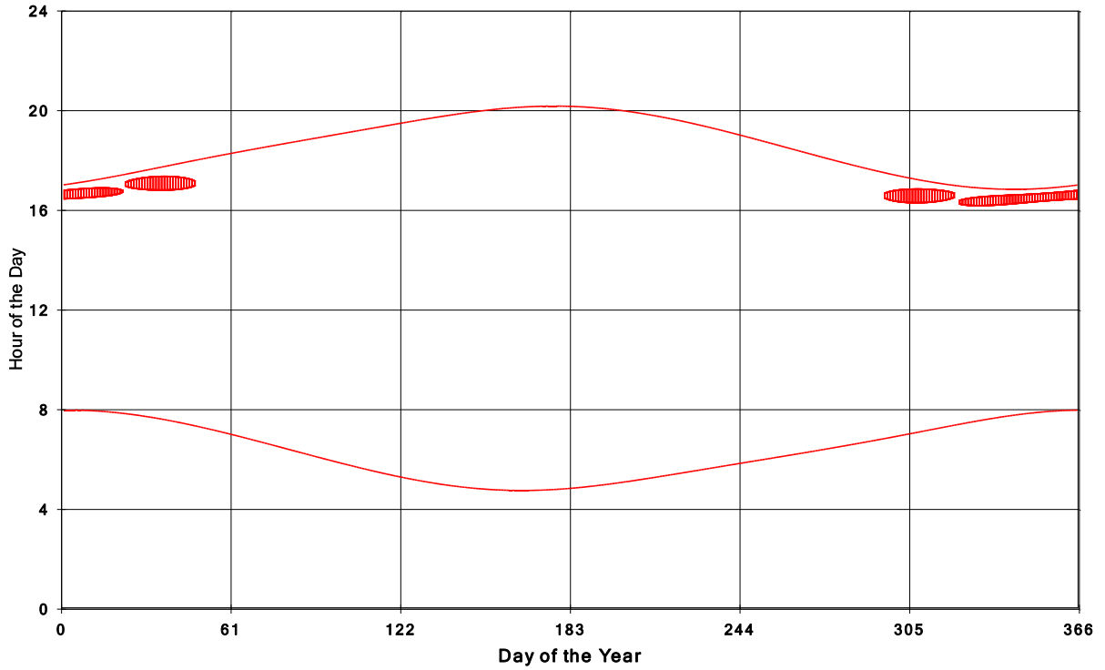
Goshen Wind Energy Centre Shadow Times on House 374, All Windows from All Turbine:
