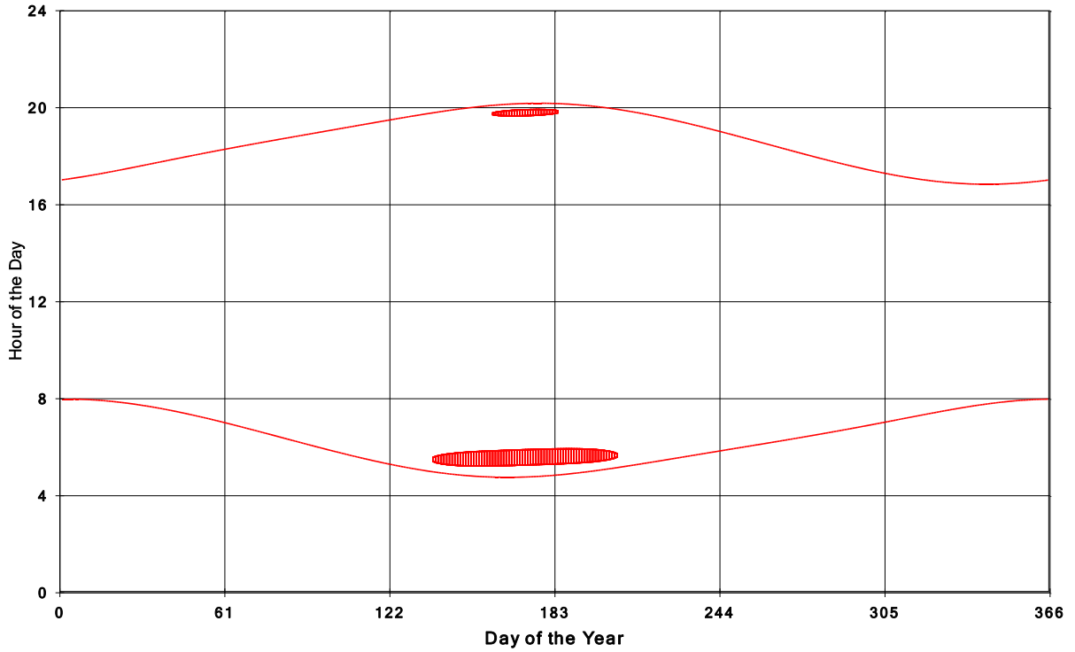
Goshen Wind Energy Centre Shadow Times on House 431, All Windows from All Turbine:
