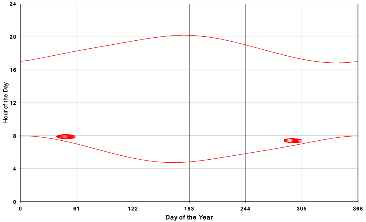
Jericho Wind Energy Centre Shadow Times on House 380, All Windows from All Turbine:
