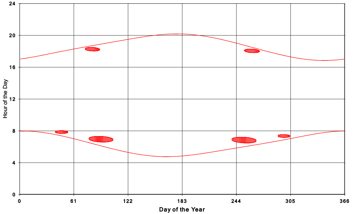
Goshen Wind Energy Centre Shadow Times on House 403, All Windows from All Turbine:
