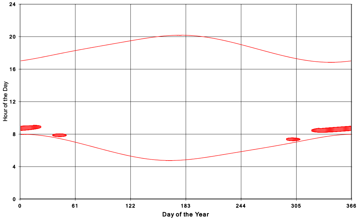
Goshen Wind Energy Centre Shadow Times on House 353, All Windows from All Turbine:
