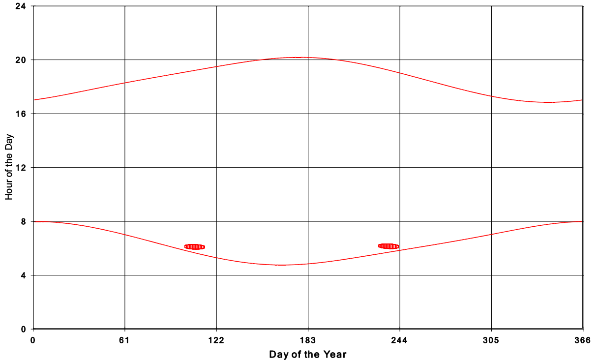
Goshen Wind Energy Centre Shadow Times on House 396, All Windows from All Turbine:
