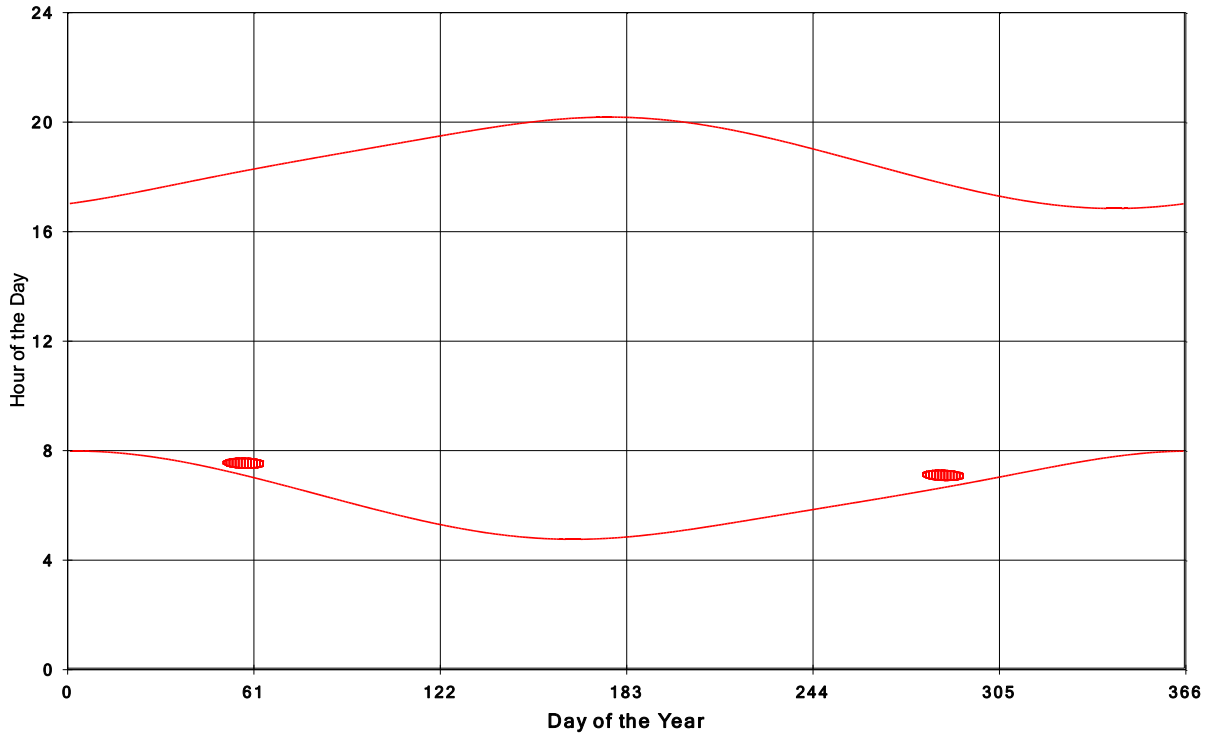
Goshen Wind Energy Centre Shadow Times on House 449, All Windows from All Turbine:
