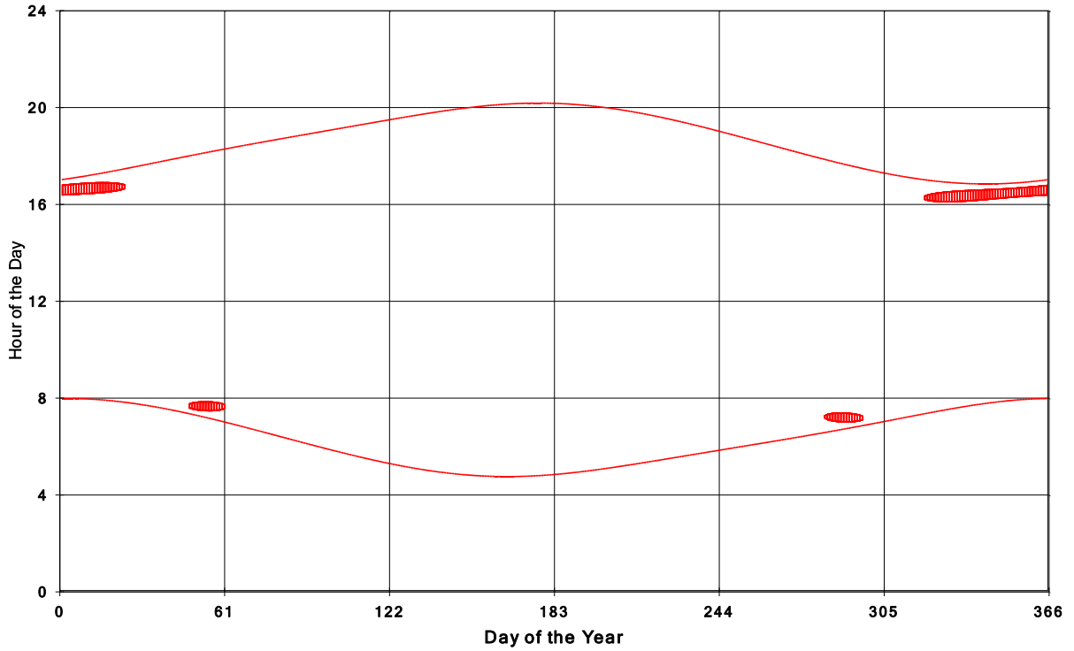
Goshen Wind Energy Centre Shadow Times on House 423, All Windows from All Turbine:
