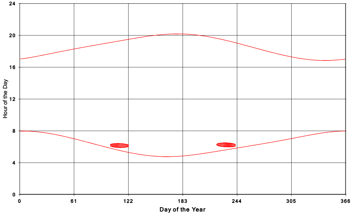
Goshen Wind Energy Centre Shadow Times on House 393, All Windows from All Turbine:
