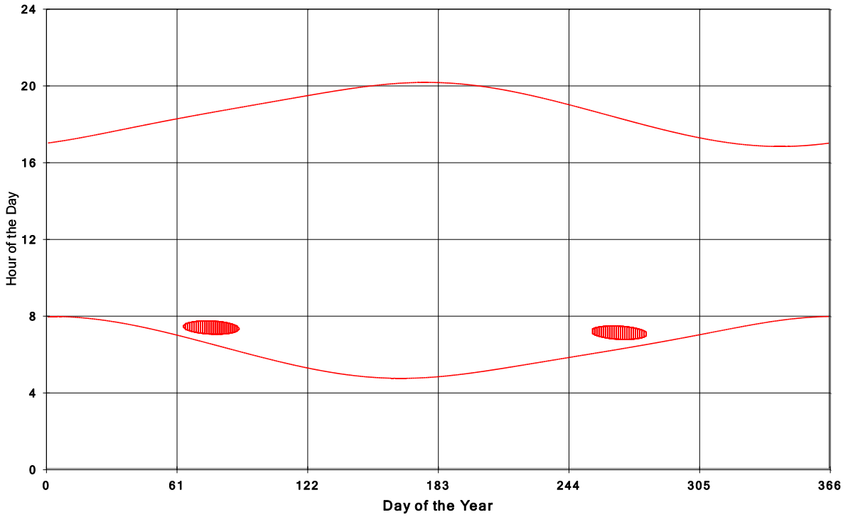
Jericho Wind Energy Centre Shadow Times on House 400, All Windows from All Turbine:
