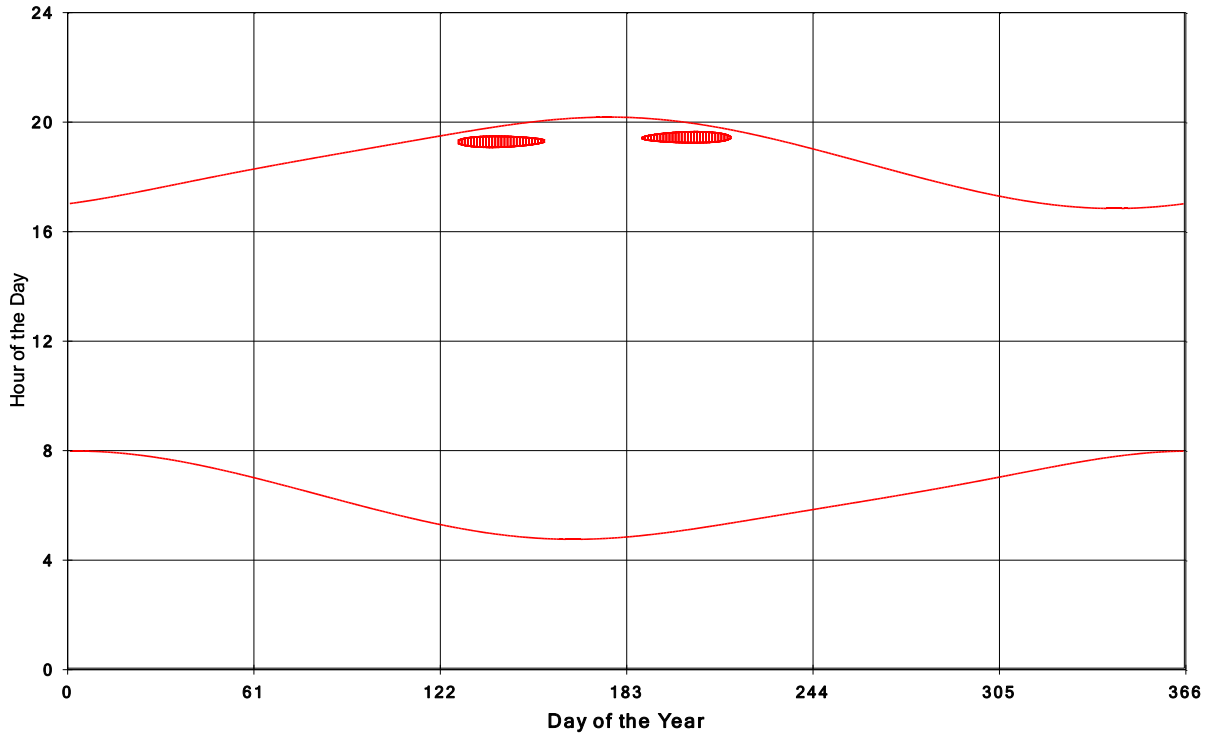
Goshen Wind Energy Centre Shadow Times on House 420, All Windows from All Turbine:
