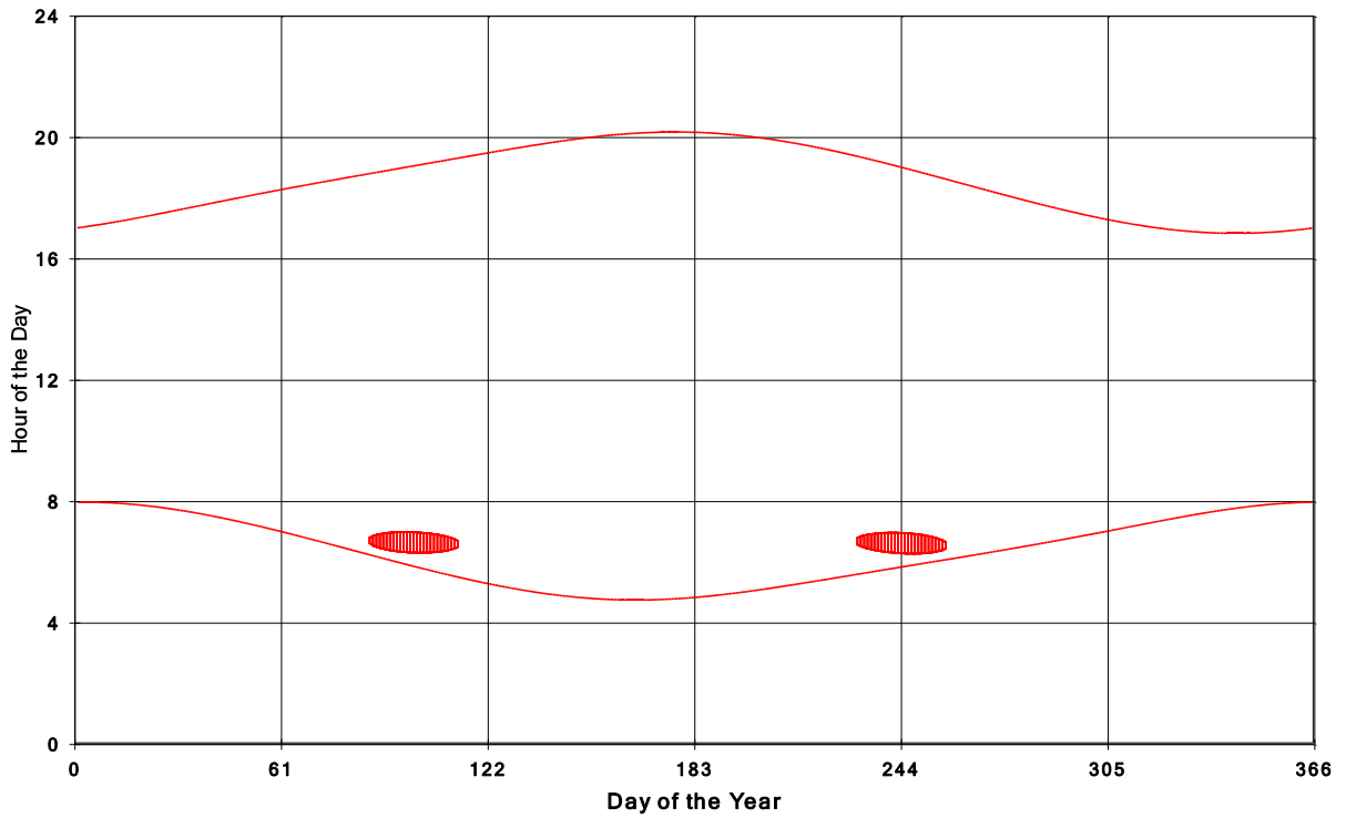
Goshen Wind Energy Centre Shadow Times on House 408, All Windows from All Turbine:
