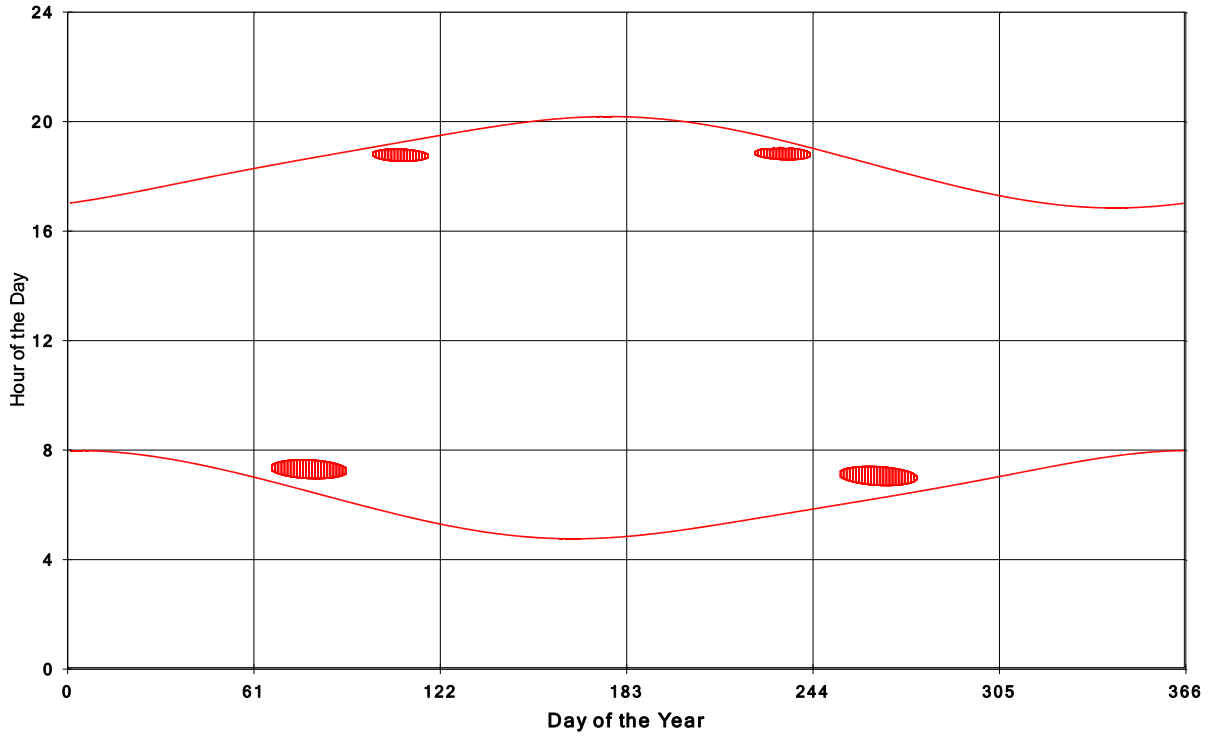
Goshen Wind Energy Centre Shadow Times on House 429, All Windows from All Turbine:
