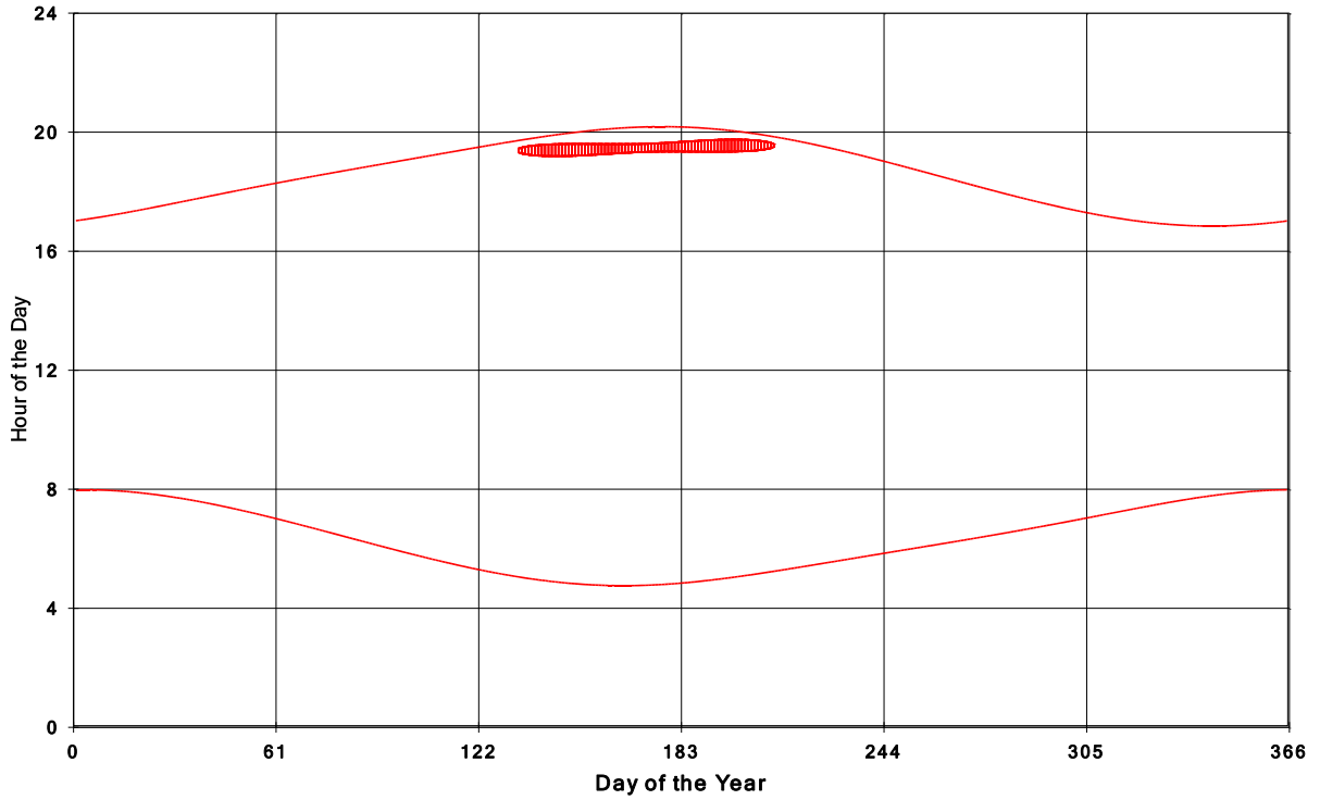
Goshen Wind Energy Centre Shadow Times on House 419, All Windows from All Turbine:
