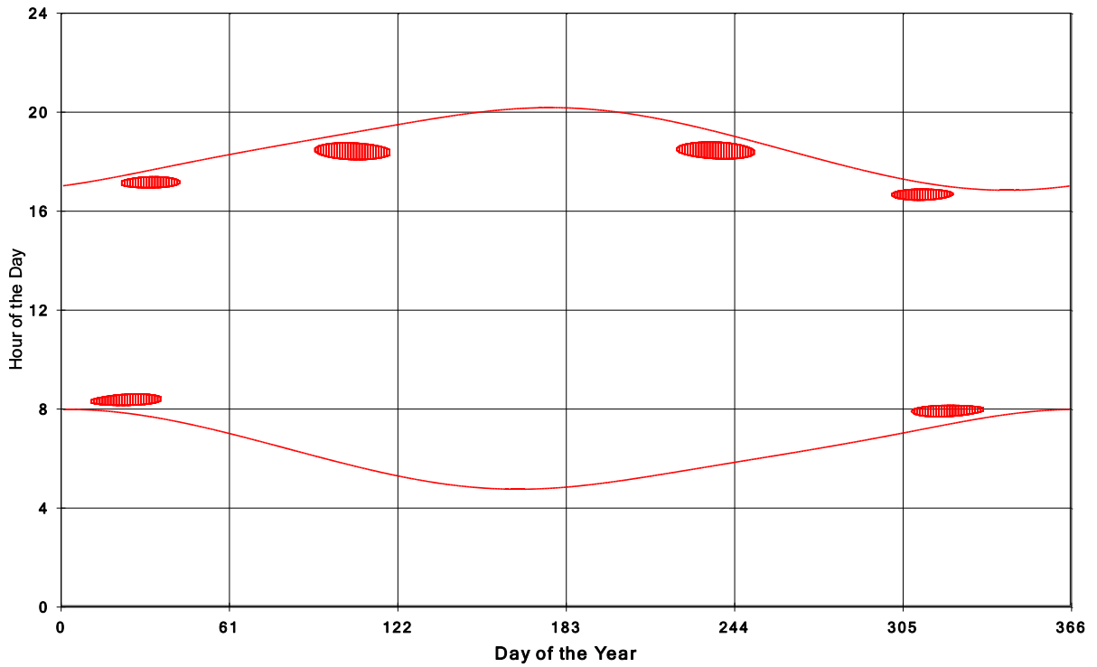
Goshen Wind Energy Centre Shadow Times on House 453, All Windows from All Turbine:
