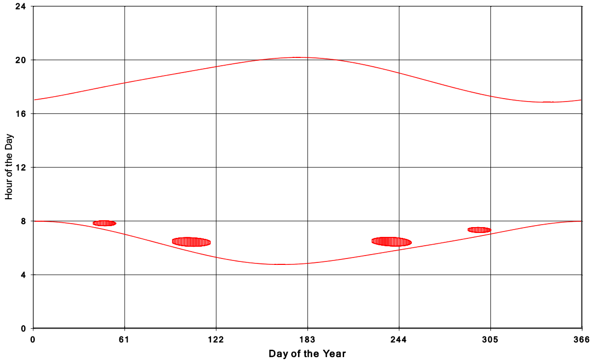
Goshen Wind Energy Centre Shadow Times on House 441, All Windows from All Turbine:
