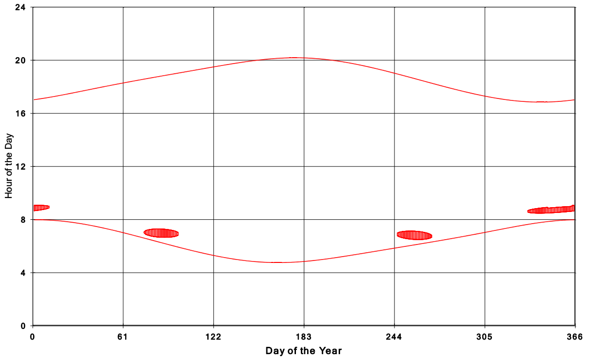
Goshen Wind Energy Centre Shadow Times on House 365, All Windows from All Turbine:
