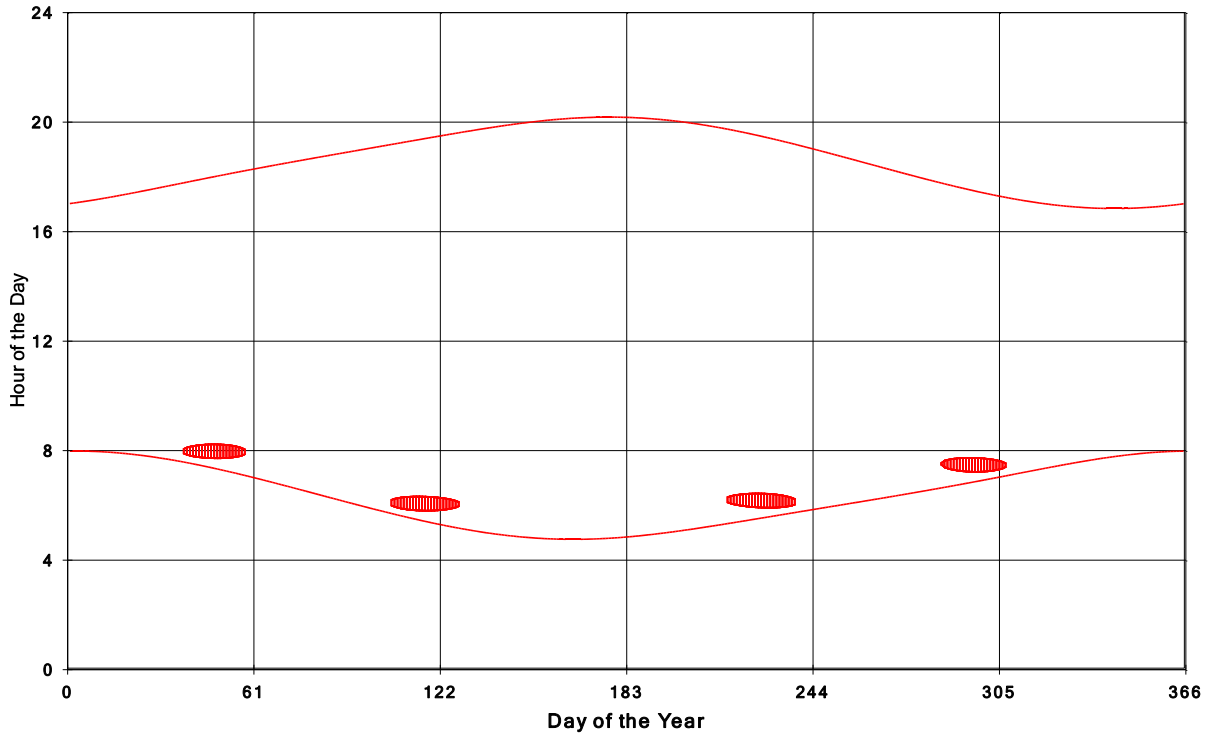
Goshen Wind Energy Centre Shadow Times on House 369, All Windows from All Turbine:
