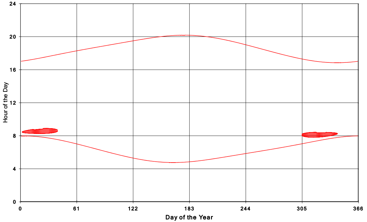
Goshen Wind Energy Centre Shadow Times on House 370, All Windows from All Turbine:
