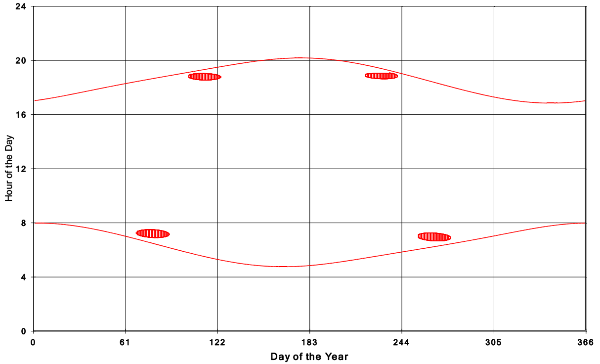
Goshen Wind Energy Centre Shadow Times on House 428, All Windows from All Turbine:
