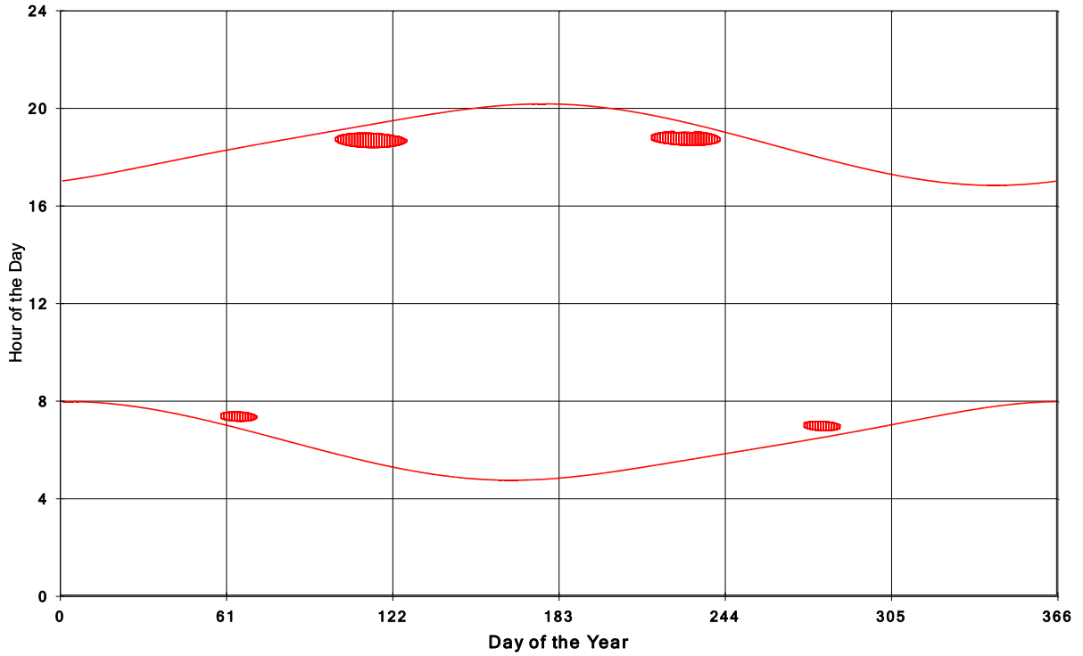
Goshen Wind Energy Centre Shadow Times on House 425, All Windows from All Turbine:
