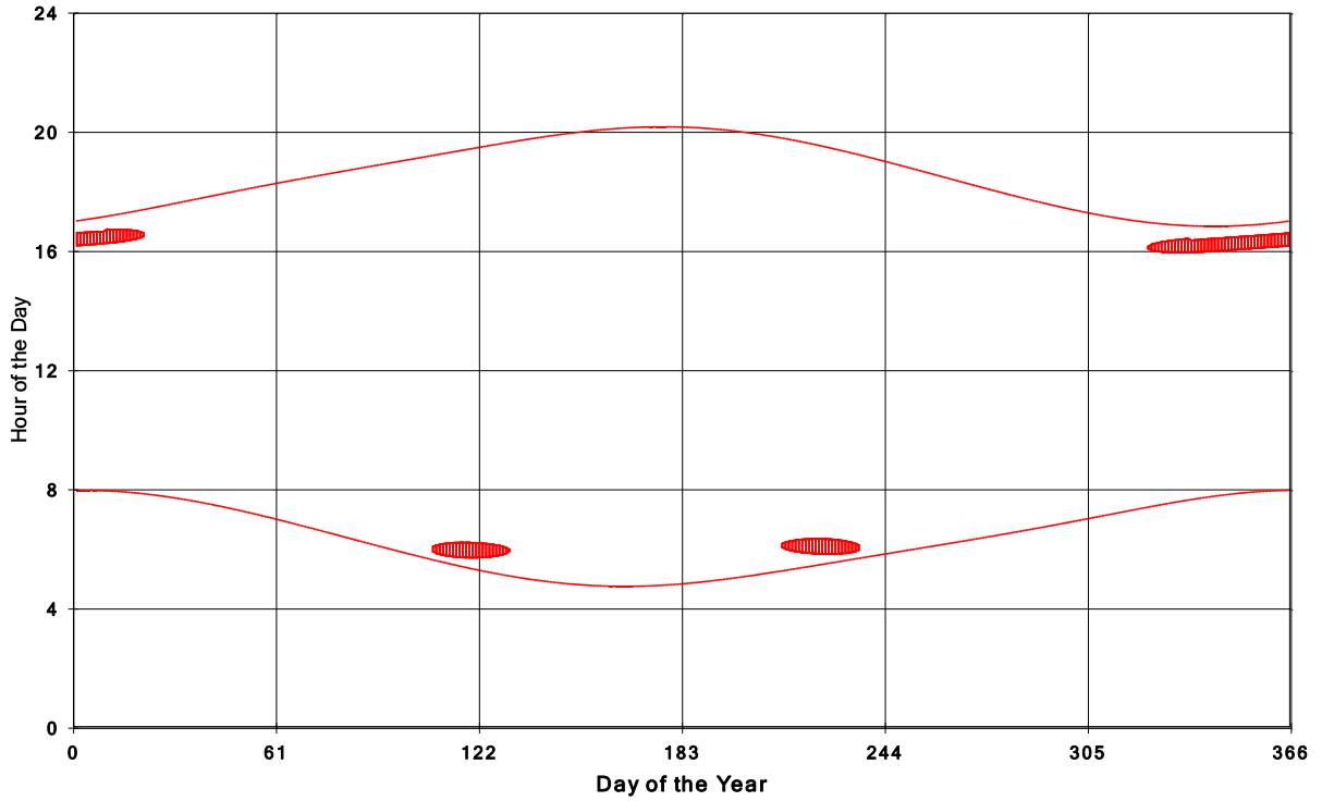
Goshen Wind Energy Centre Shadow Times on House 438, All Windows from All Turbine:
