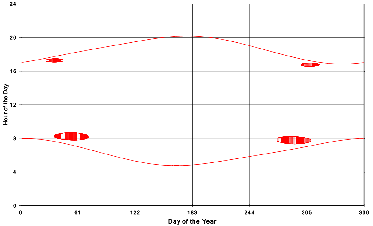
Goshen Wind Energy Centre Shadow Times on House 460, All Windows from All Turbine:
