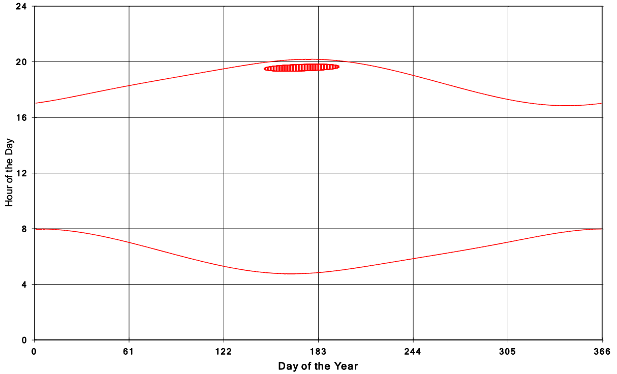
Goshen Wind Energy Centre Shadow Times on House 444, All Windows from All Turbine:
