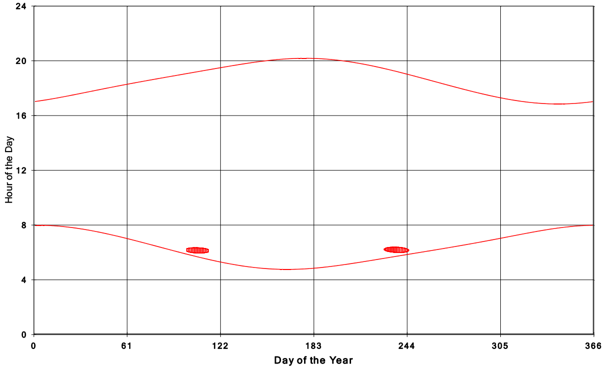
Goshen Wind Energy Centre Shadow Times on House 389, All Windows from All Turbine:
