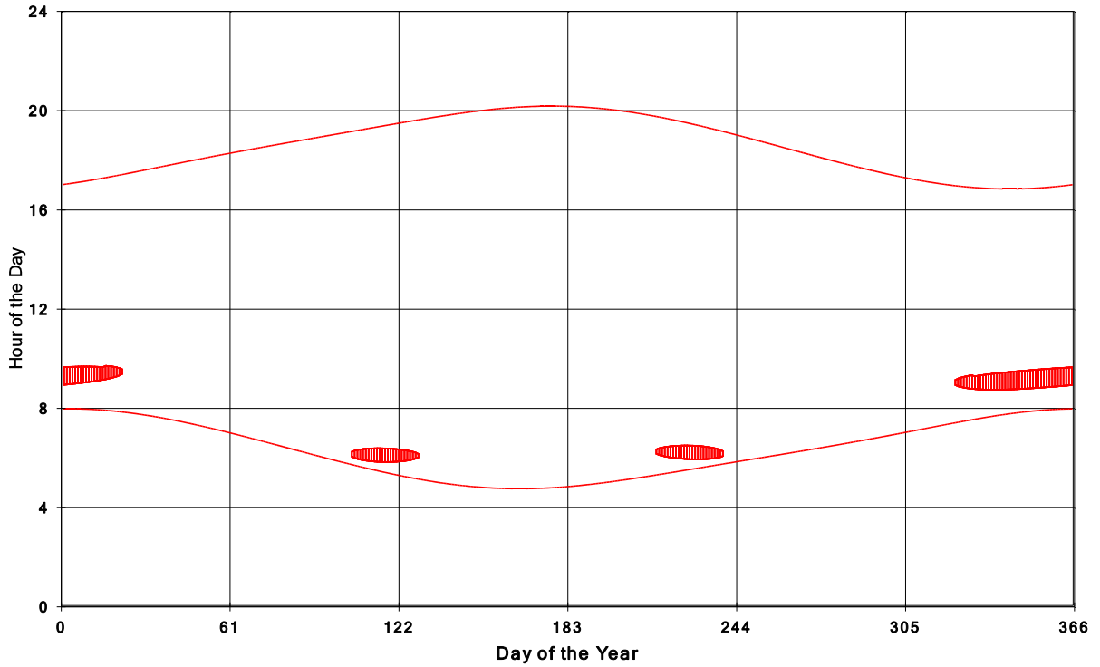
Goshen Wind Energy Centre Shadow Times on House 361, All Windows from All Turbine:
