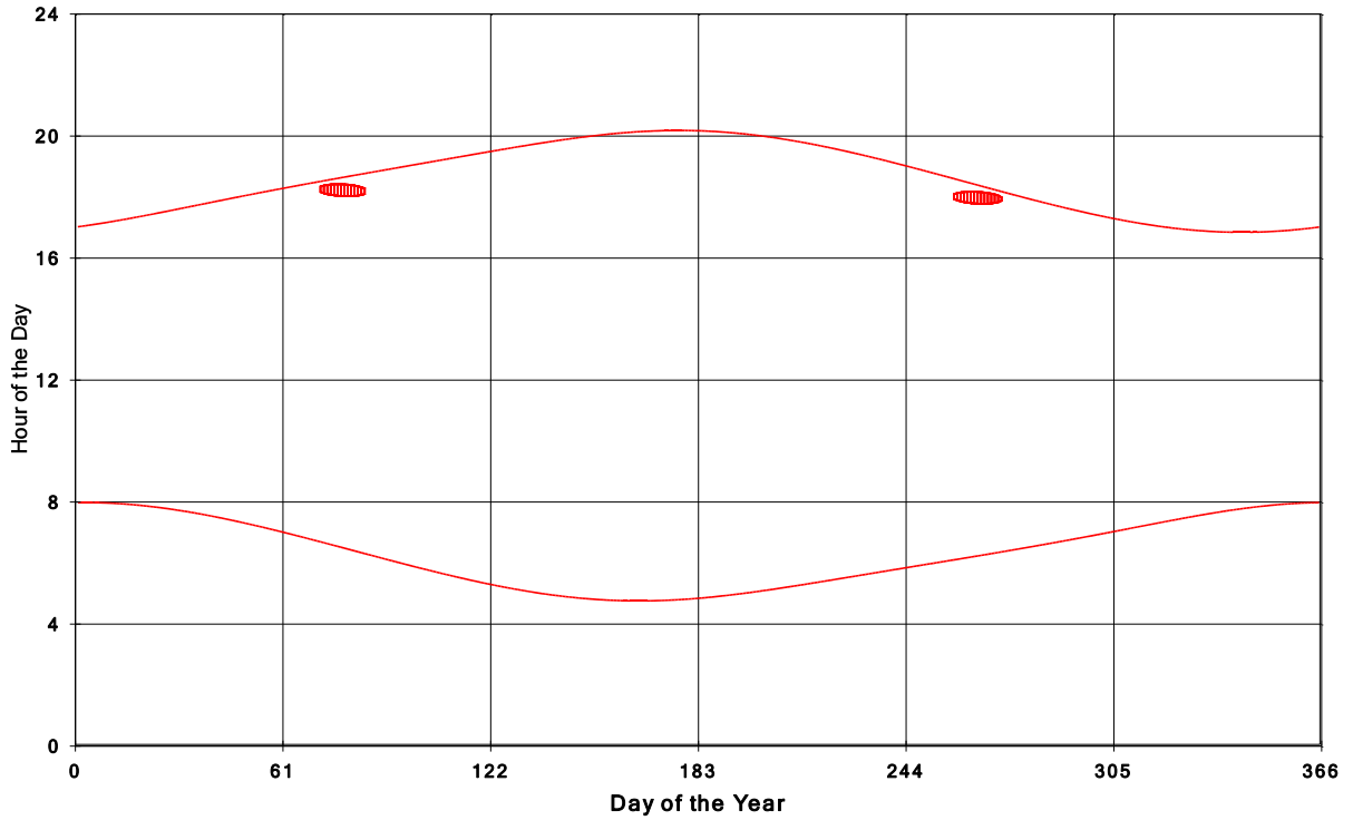
Goshen Wind Energy Centre Shadow Times on House 451, All Windows from All Turbine:
