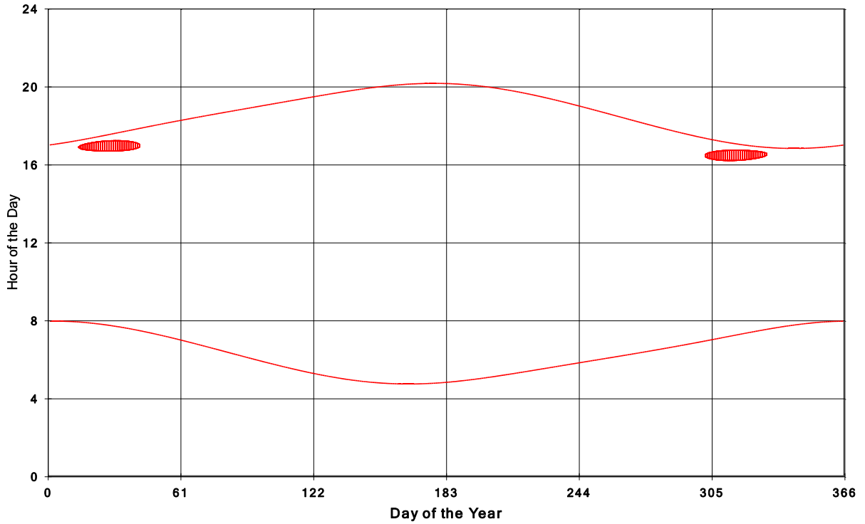
Goshen Wind Energy Centre Shadow Times on House 424, All Windows from All Turbine:
