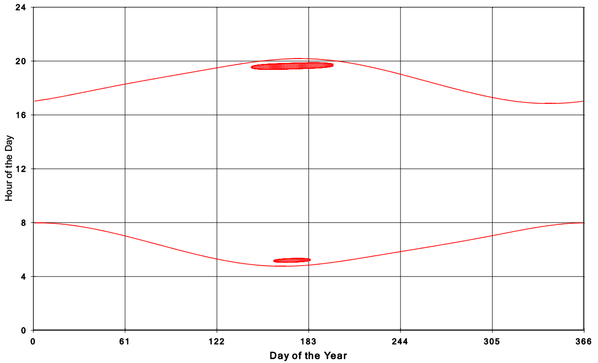
Goshen Wind Energy Centre Shadow Times on House 457, All Windows from All Turbine:
