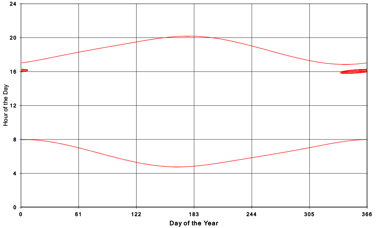
Goshen Wind Energy Centre Shadow Times on House 261, All Windows from All Turbine:
