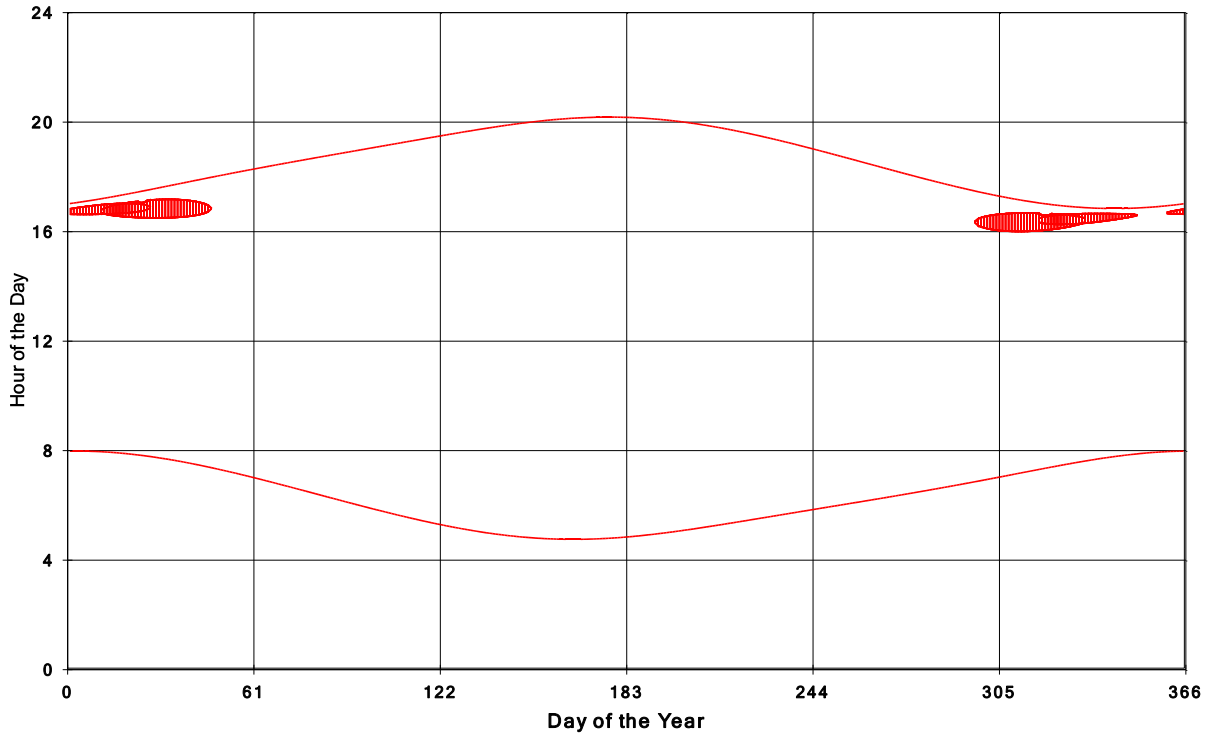
Goshen Wind Energy Centre Shadow Times on House 202, All Windows from All Turbine:
