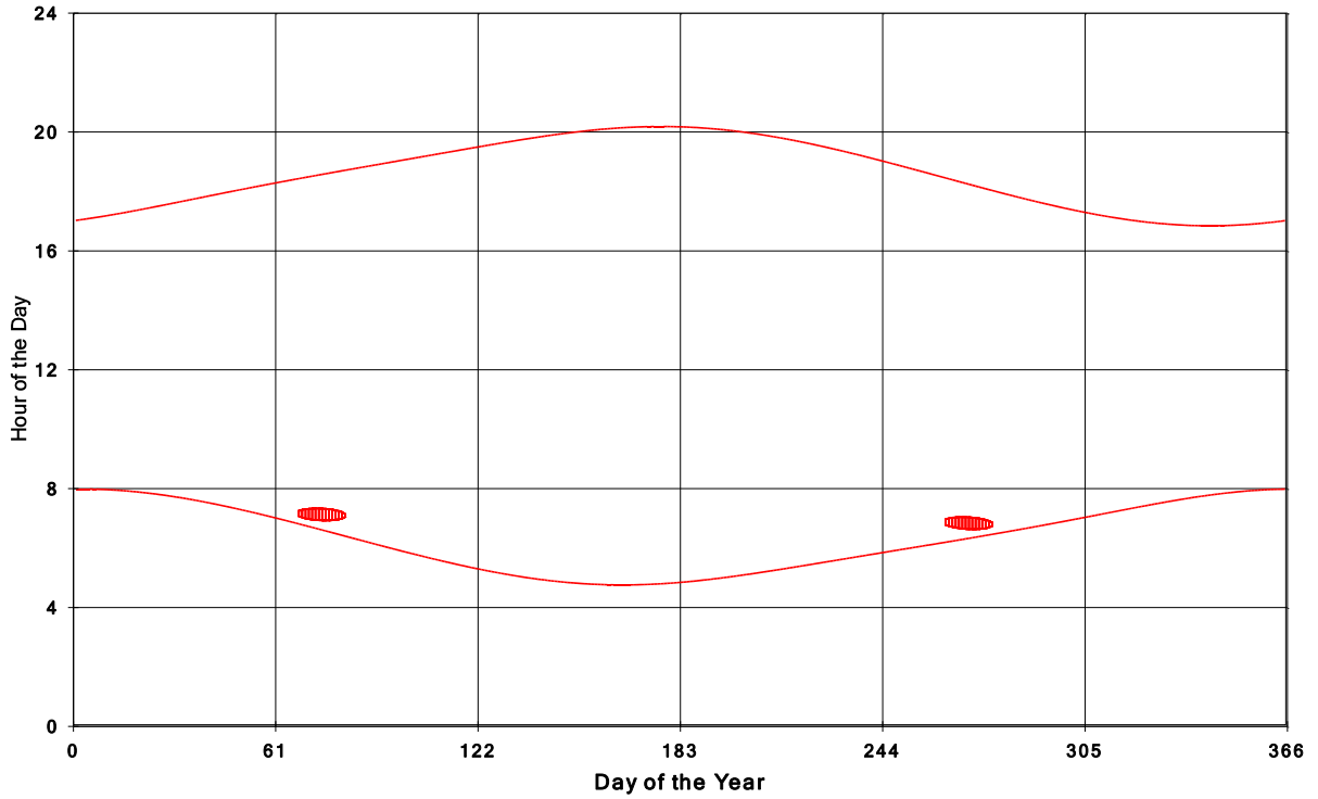
Goshen Wind Energy Centre Shadow Times on House 143, All Windows from All Turbine:
