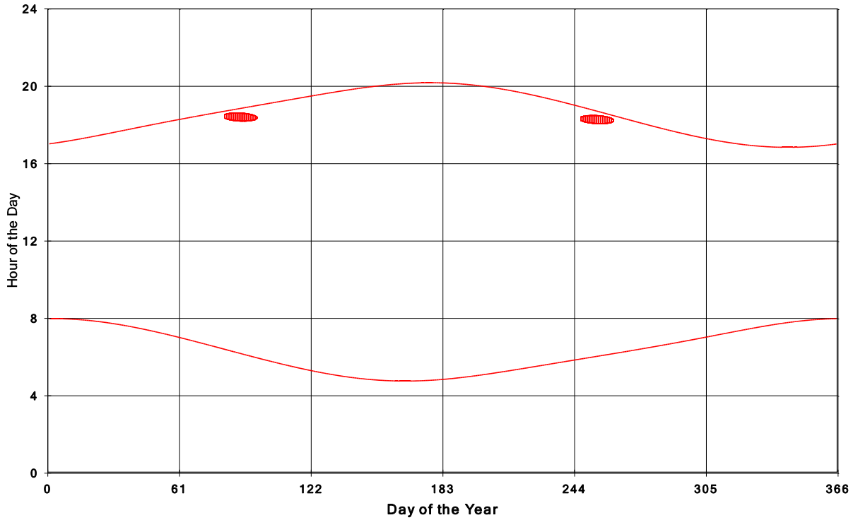
Goshen Wind Energy Centre Shadow Times on House 151, All Windows from All Turbine:
