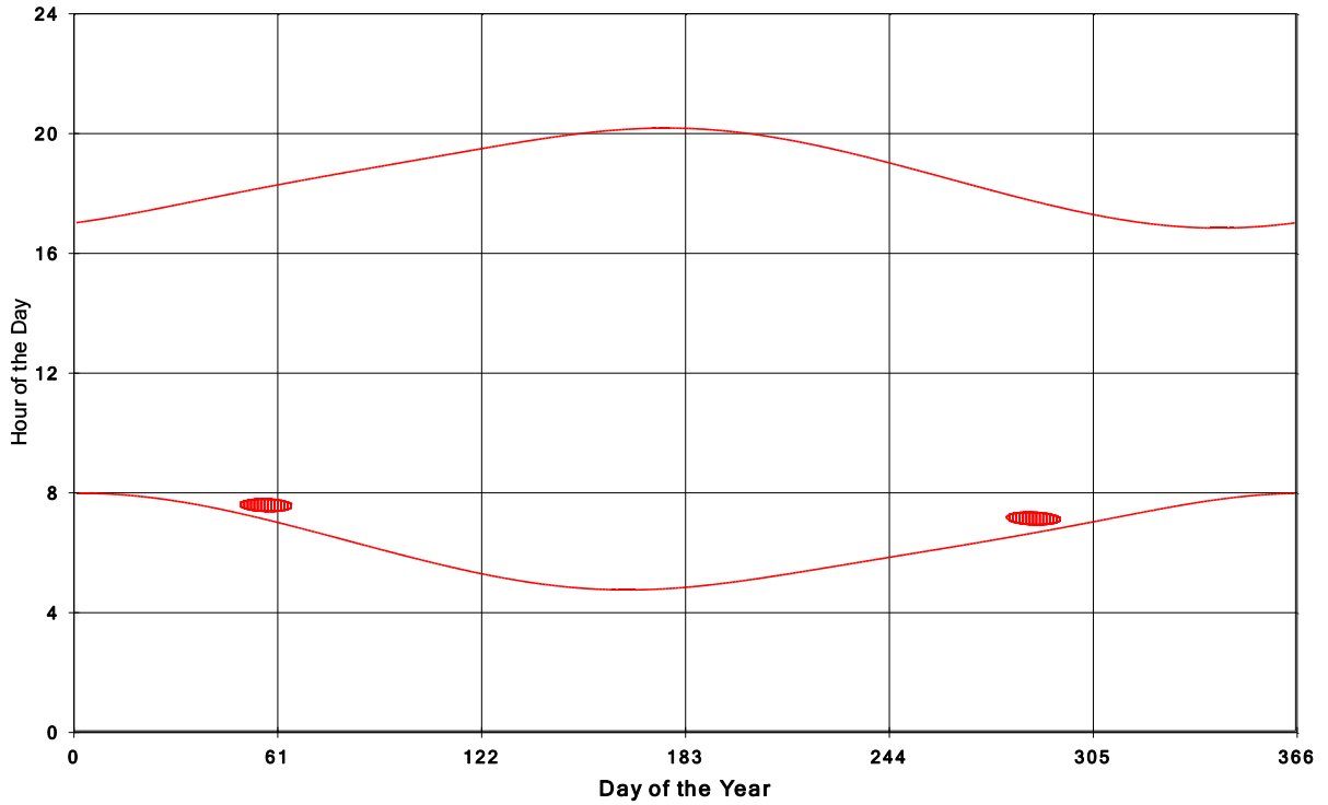
Goshen Wind Energy Centre Shadow Times on House 328, All Windows from All Turbine:
