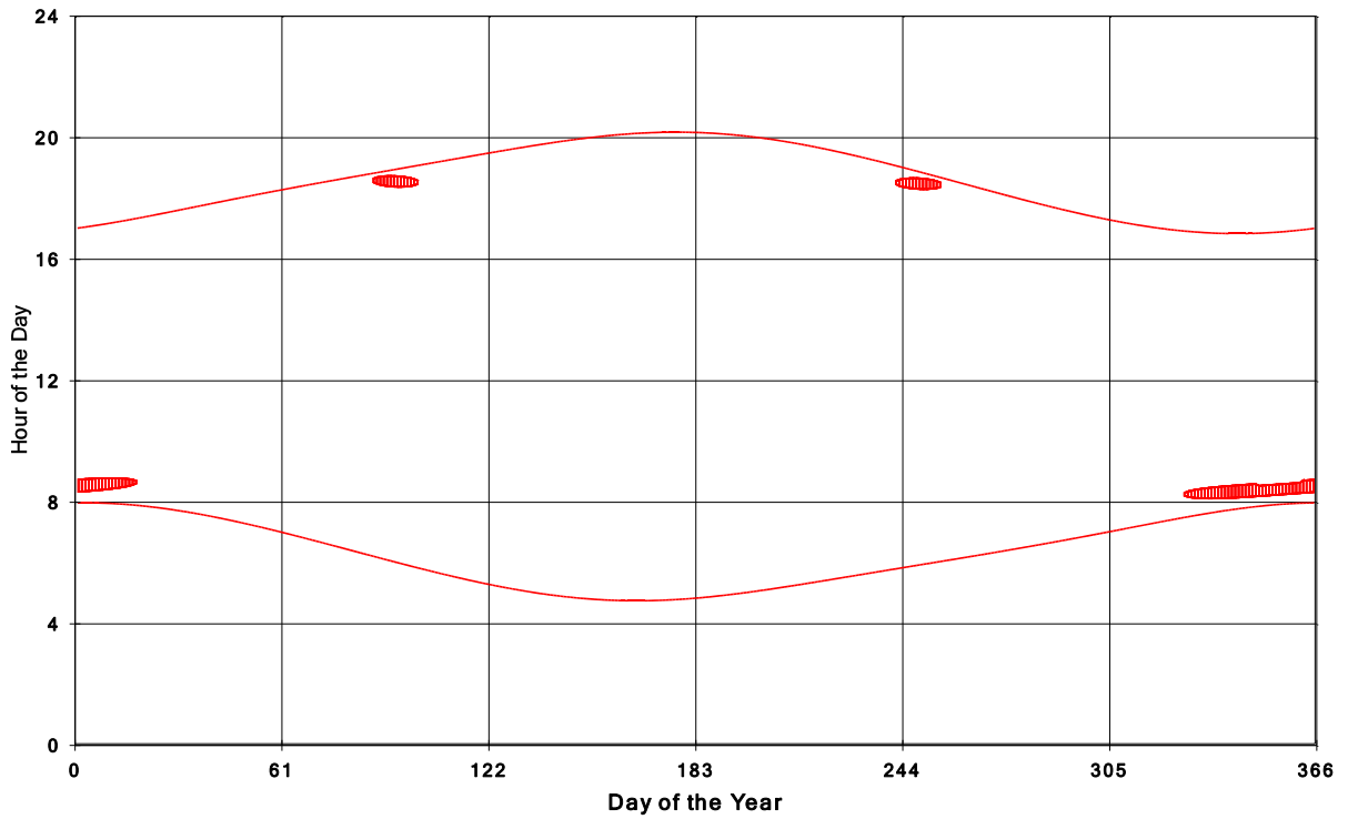
Goshen Wind Energy Centre Shadow Times on House 278, All Windows from All Turbine:
