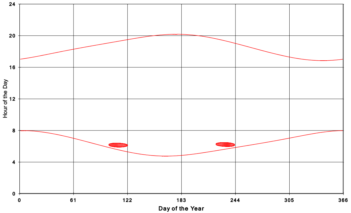
Goshen Wind Energy Centre Shadow Times on House 291, All Windows from All Turbine:
