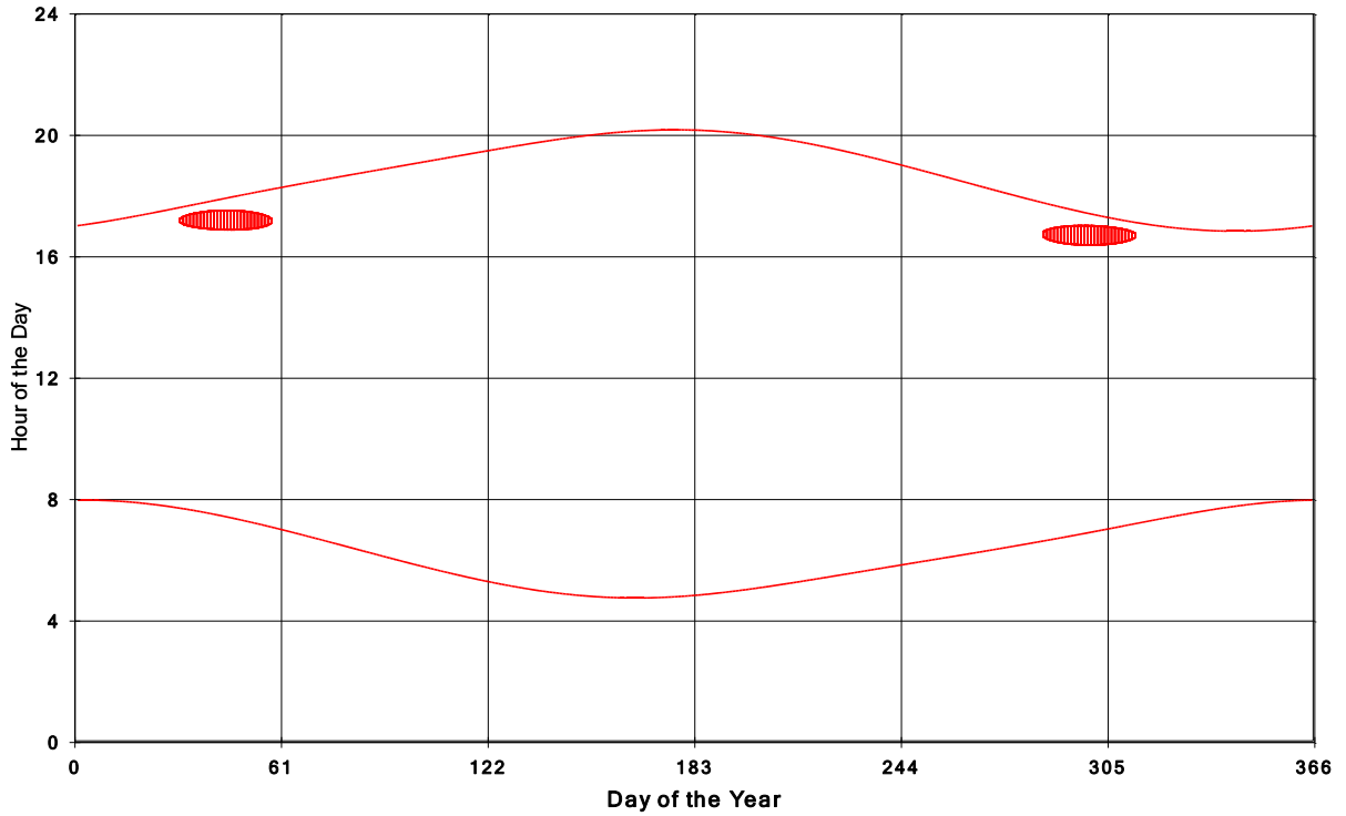
Goshen Wind Energy Centre Shadow Times on House 290, All Windows from All Turbine:
