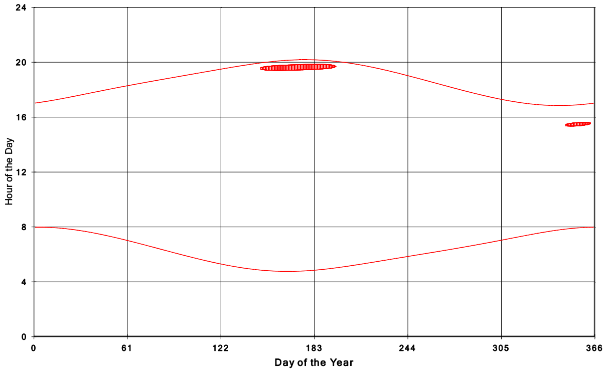
Goshen Wind Energy Centre Shadow Times on House 209, All Windows from All Turbine:
