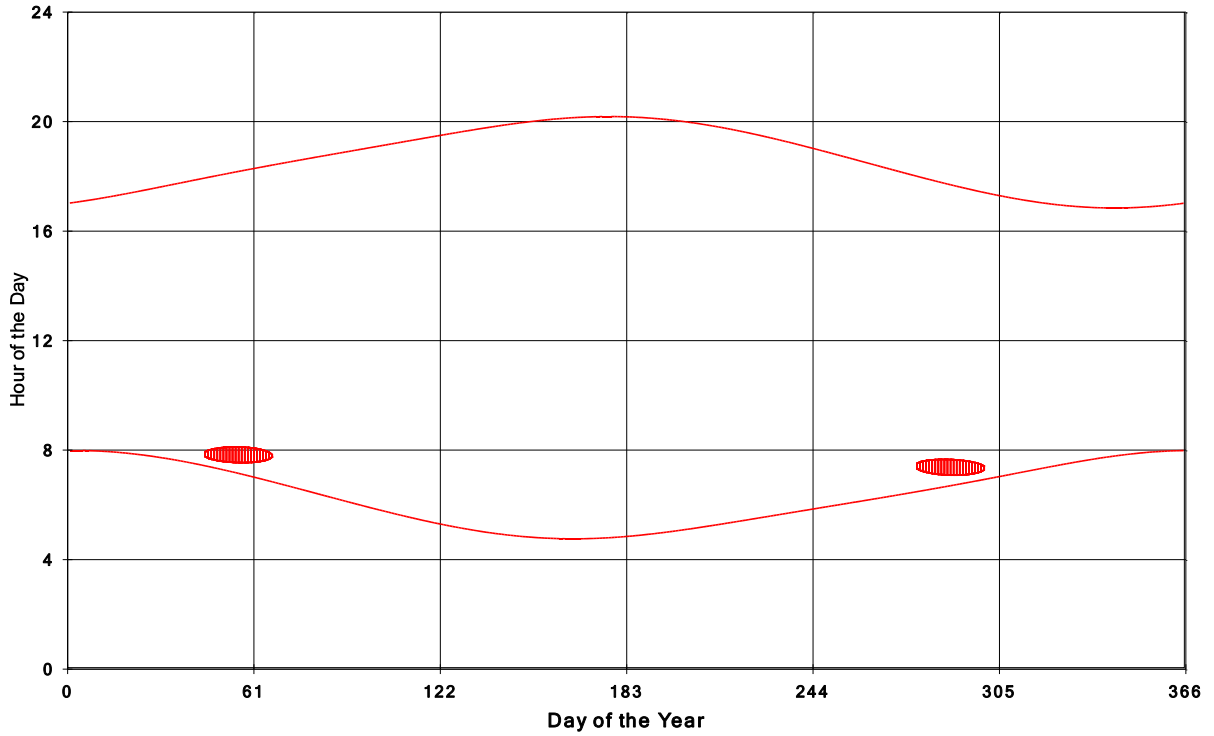
Goshen Wind Energy Centre Shadow Times on House 312, All Windows from All Turbine:
