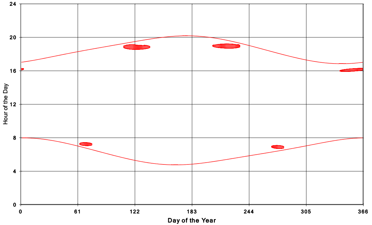
Goshen Wind Energy Centre Shadow Times on House 162, All Windows from All Turbine:
