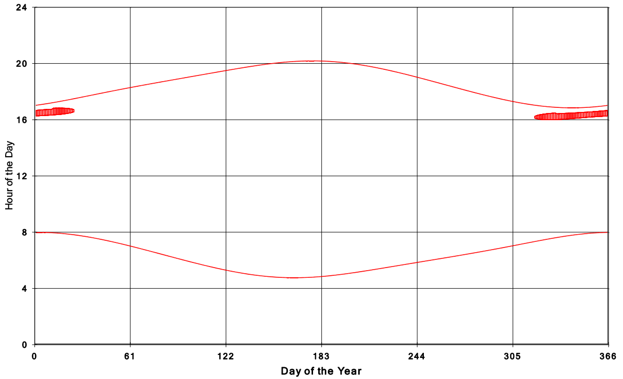
Goshen Wind Energy Centre Shadow Times on House 215, All Windows from All Turbine:
