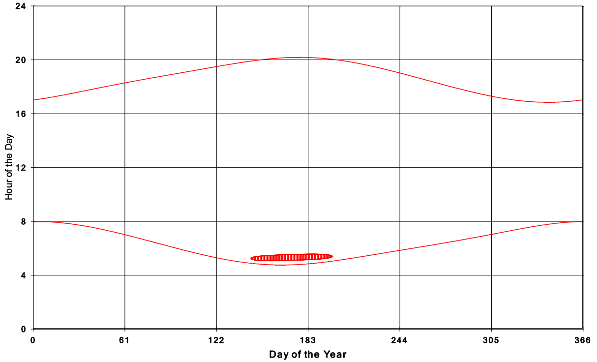
Goshen Wind Energy Centre Shadow Times on House 249, All Windows from All Turbine:
