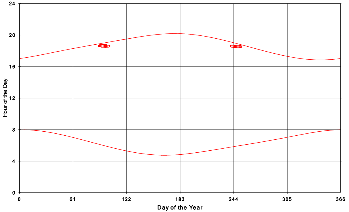
Goshen Wind Energy Centre Shadow Times on House 152, All Windows from All Turbine:
