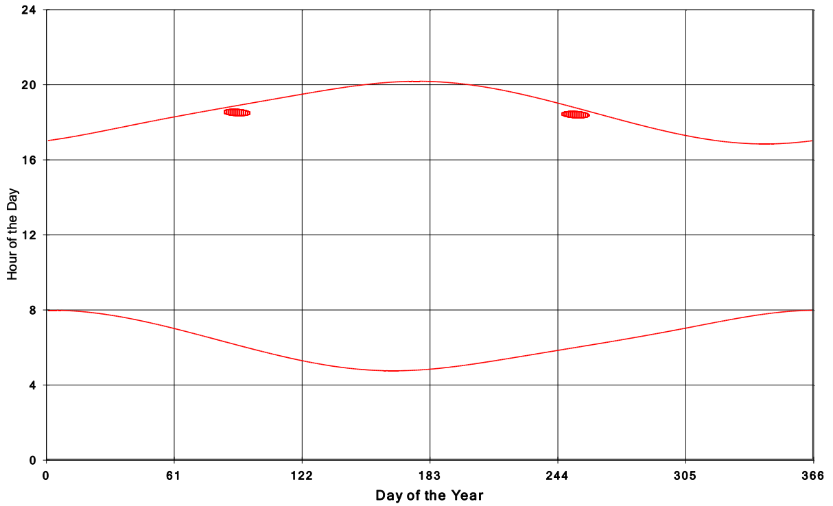
Goshen Wind Energy Centre Shadow Times on House 317, All Windows from All Turbine:
