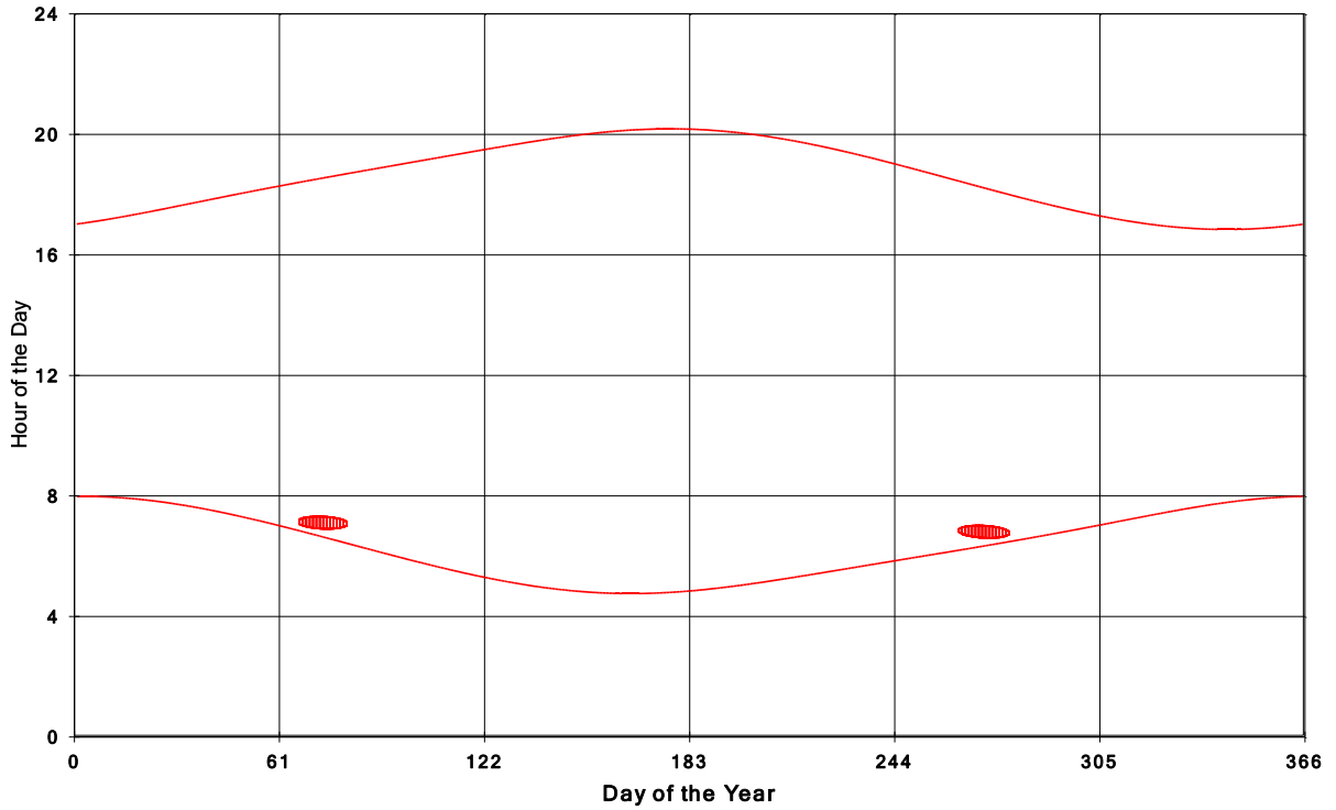
Goshen Wind Energy Centre Shadow Times on House 220, All Windows from All Turbine:
