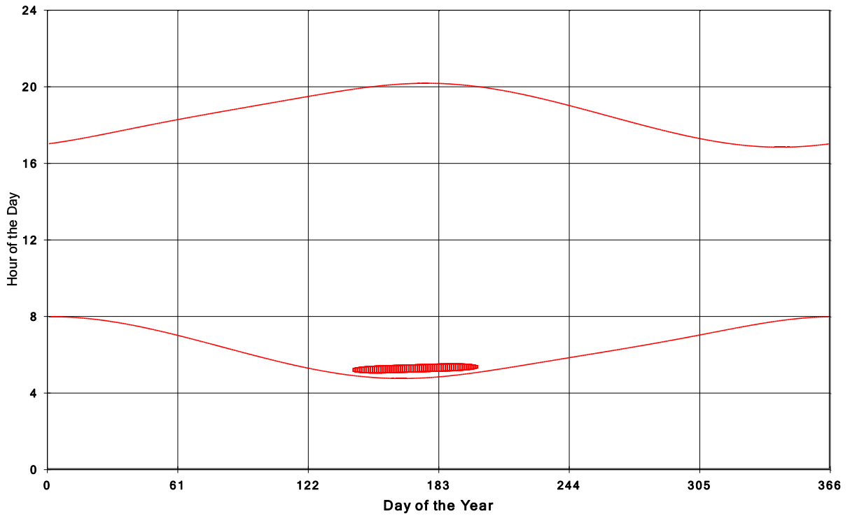
Goshen Wind Energy Centre Shadow Times on House 320, All Windows from All Turbine:
