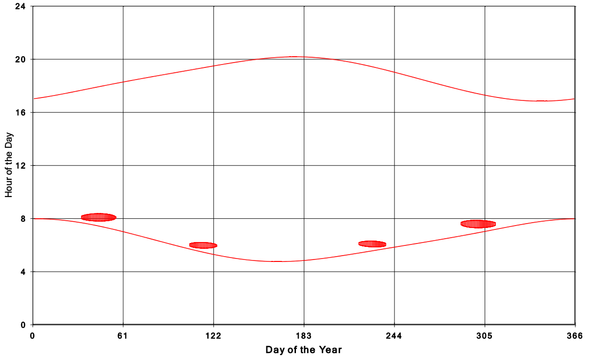
Goshen Wind Energy Centre Shadow Times on House 322, All Windows from All Turbine:
