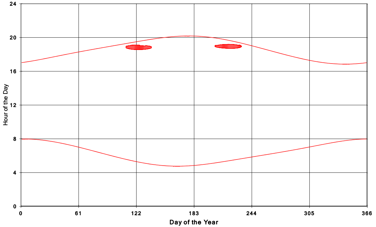
Goshen Wind Energy Centre Shadow Times on House 289, All Windows from All Turbine:
