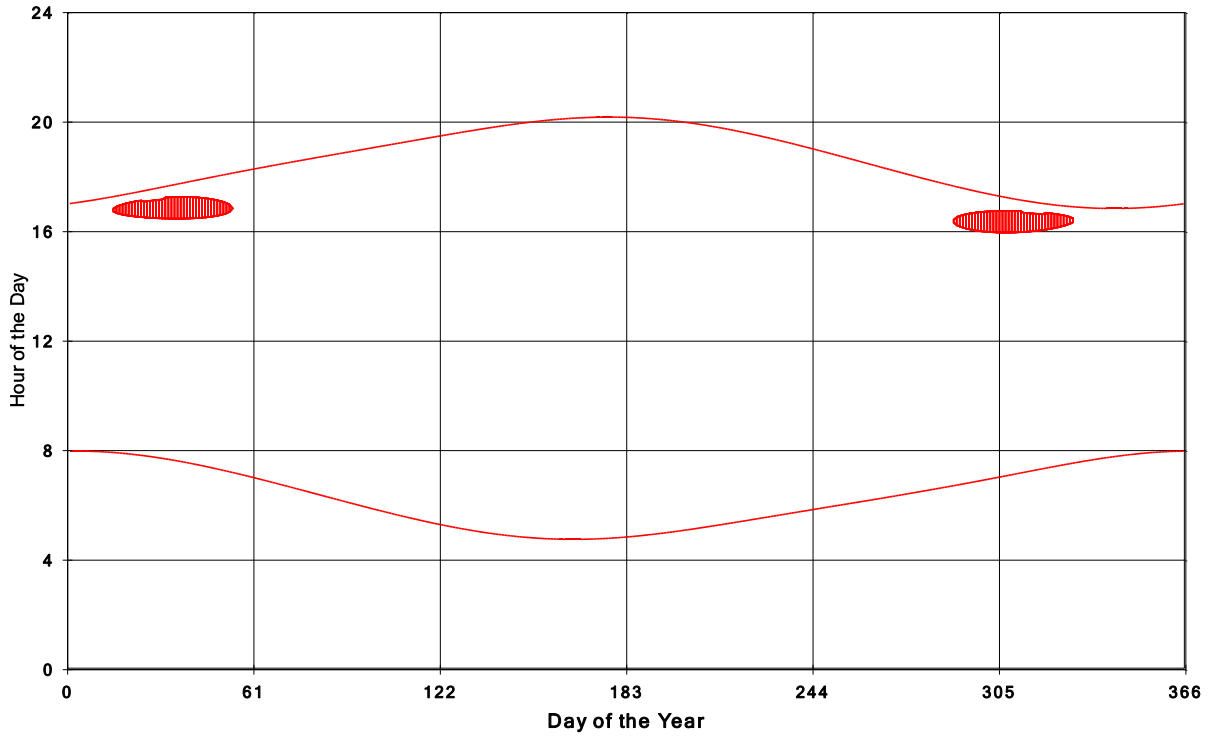
Goshen Wind Energy Centre Shadow Times on House 186, All Windows from All Turbine:
