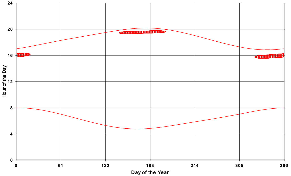
Goshen Wind Energy Centre Shadow Times on House 211, All Windows from All Turbine:
