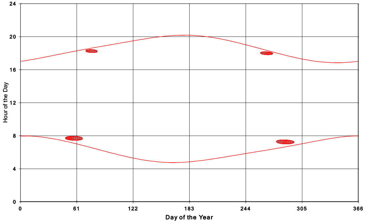
Goshen Wind Energy Centre Shadow Times on House 303, All Windows from All Turbine:
