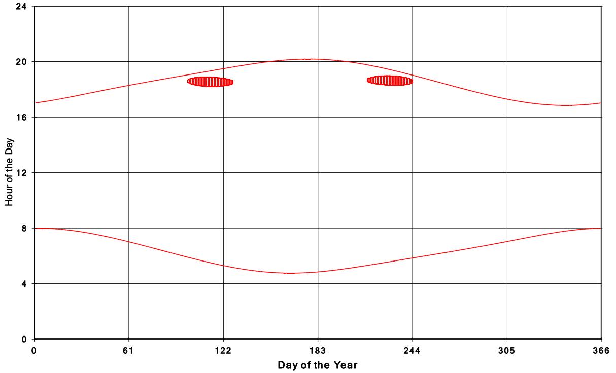
Goshen Wind Energy Centre Shadow Times on House 293, All Windows from All Turbine:
