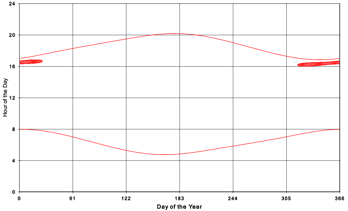
Goshen Wind Energy Centre Shadow Times on House 316, All Windows from All Turbine:
