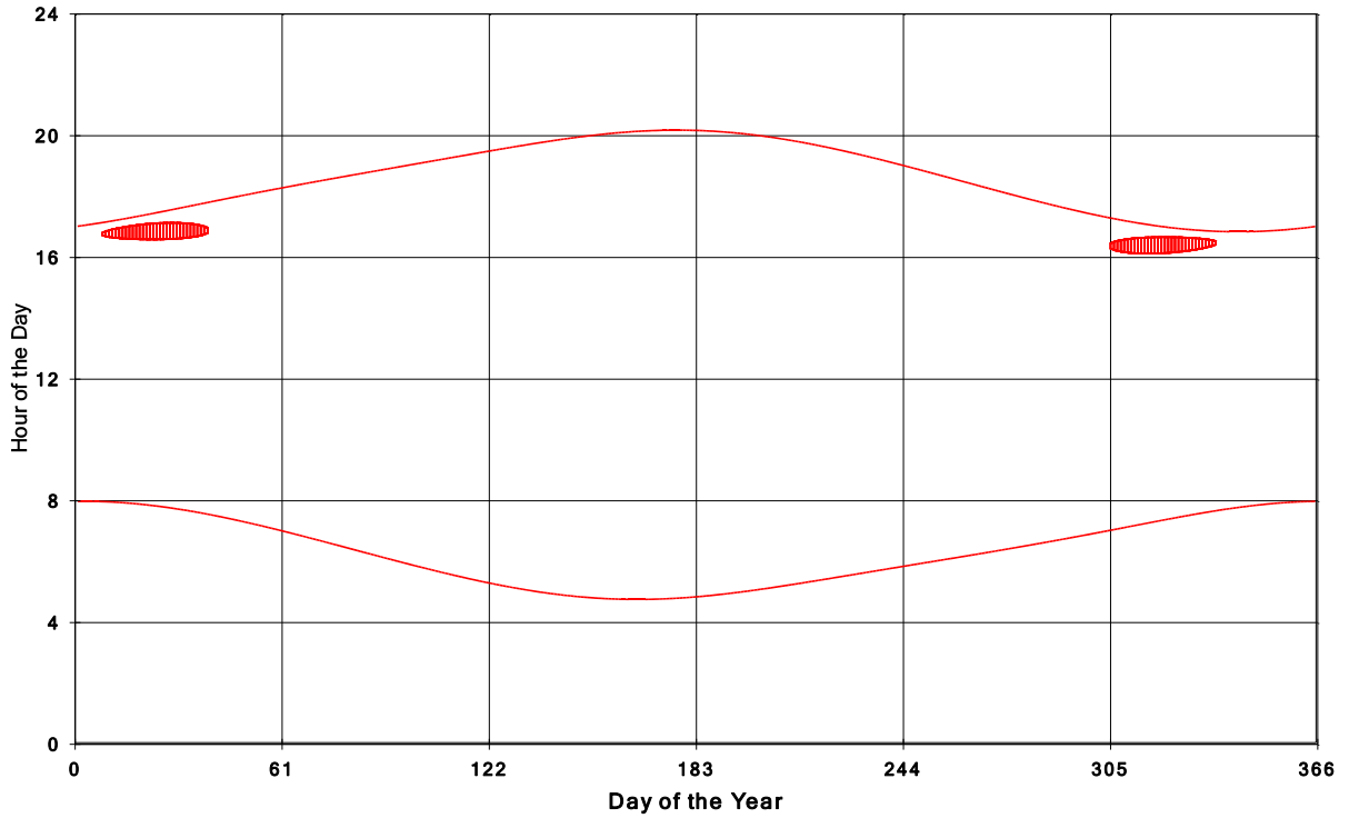
Goshen Wind Energy Centre Shadow Times on House 170, All Windows from All Turbine:
