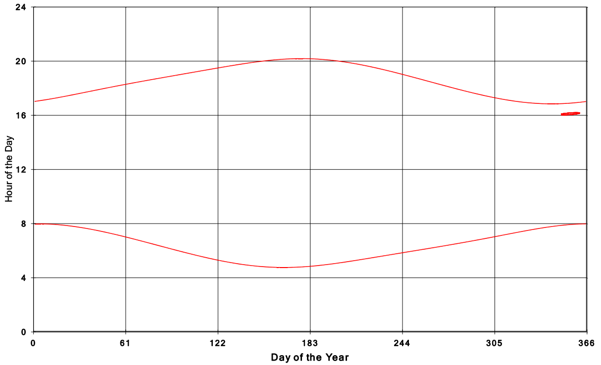
Goshen Wind Energy Centre Shadow Times on House 207, All Windows from All Turbine:
