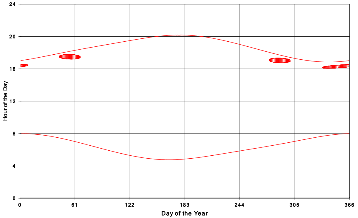
Goshen Wind Energy Centre Shadow Times on House 189, All Windows from All Turbine:
