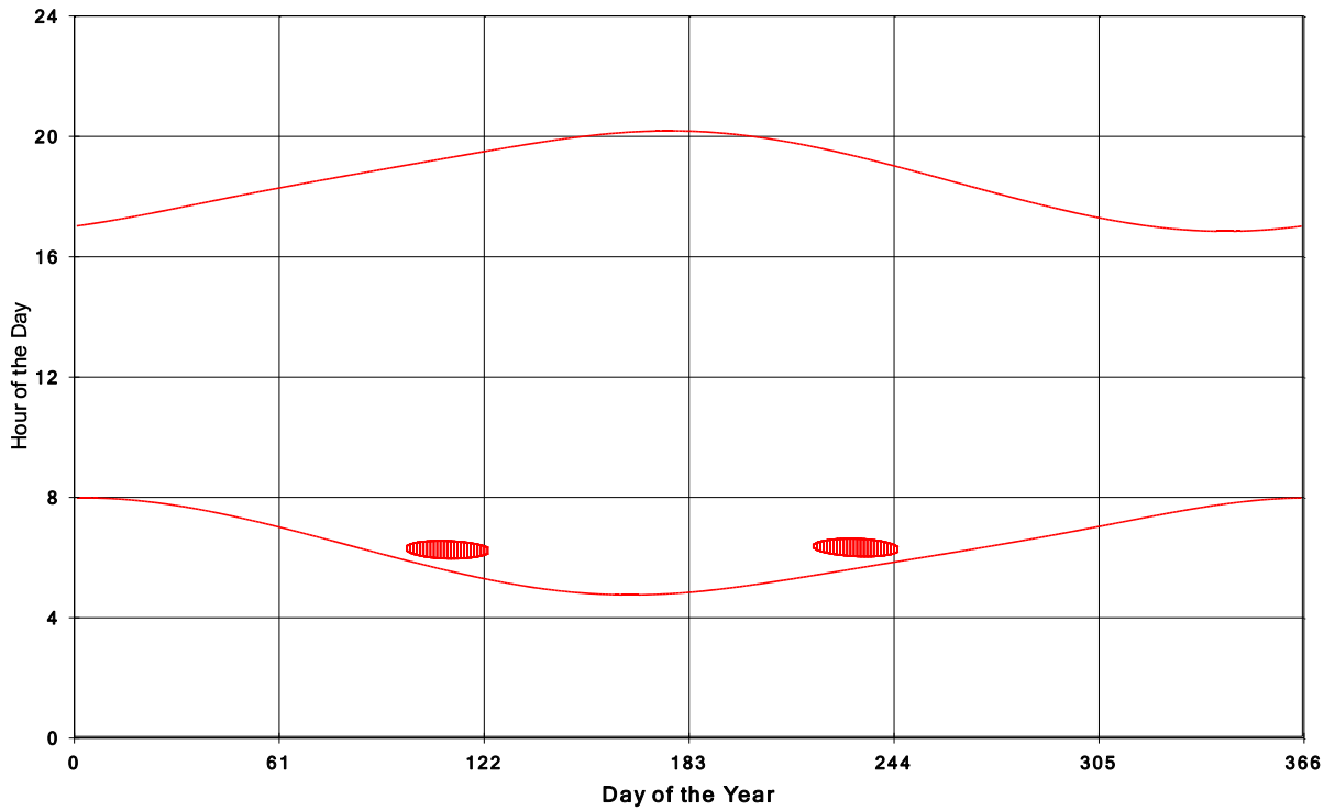
Goshen Wind Energy Centre Shadow Times on House 156, All Windows from All Turbine:
