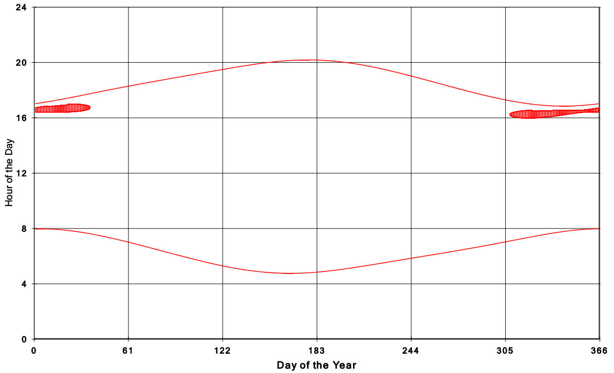
Goshen Wind Energy Centre Shadow Times on House 204, All Windows from All Turbine:
