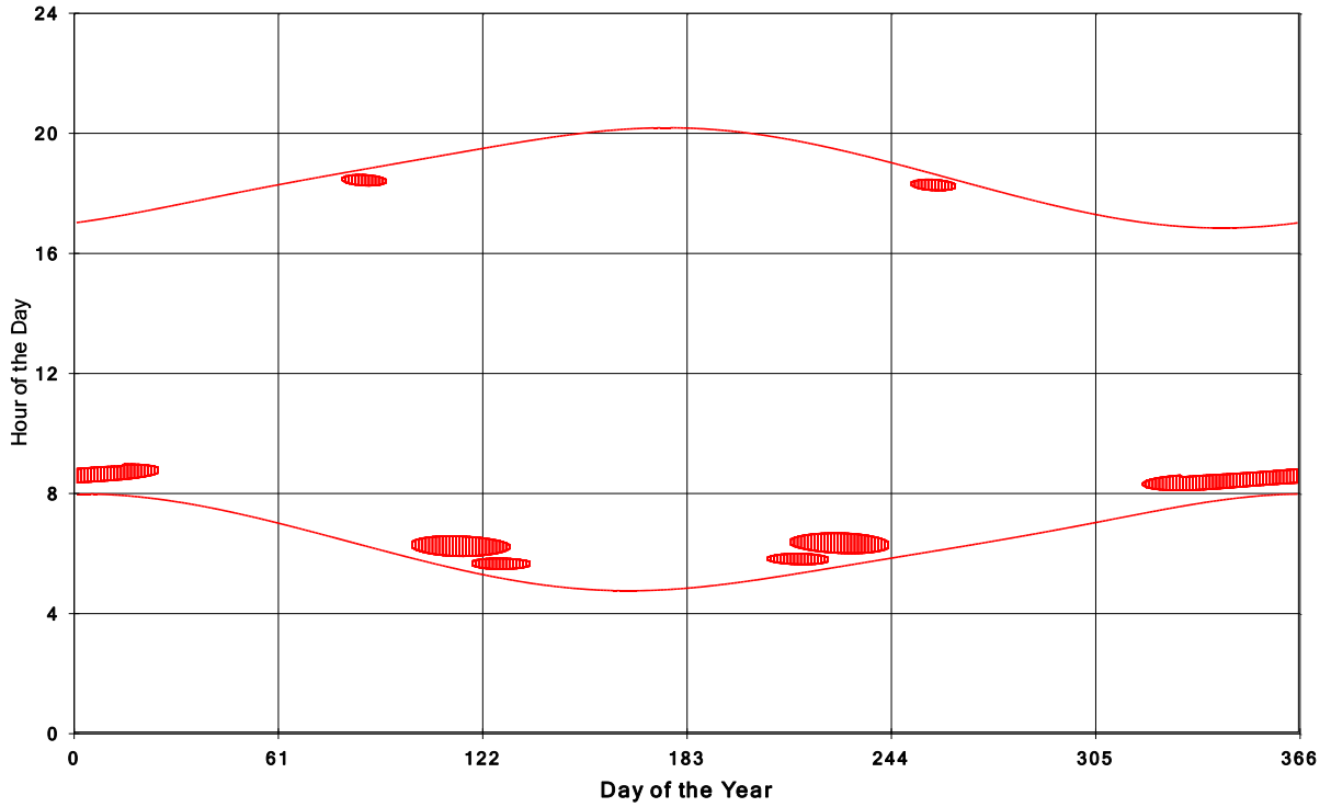
Goshen Wind Energy Centre Shadow Times on House 171, All Windows from All Turbine:
