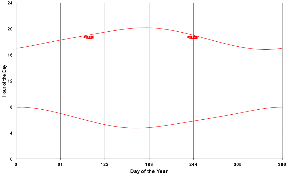
Goshen Wind Energy Centre Shadow Times on House 217, All Windows from All Turbine:
