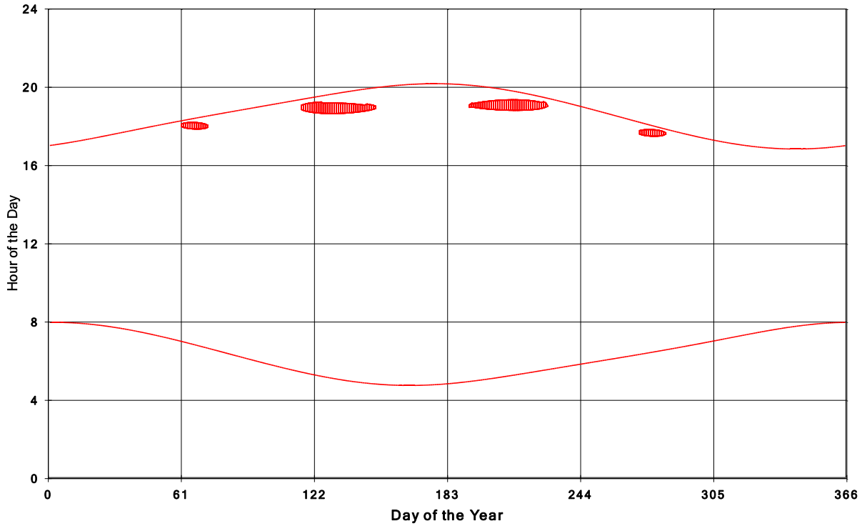
Goshen Wind Energy Centre Shadow Times on House 306, All Windows from All Turbine:
