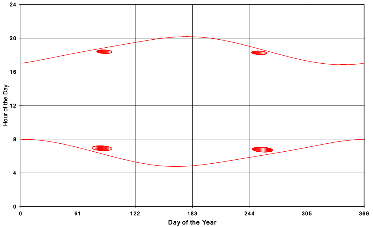
Goshen Wind Energy Centre Shadow Times on House 190, All Windows from All Turbine:
