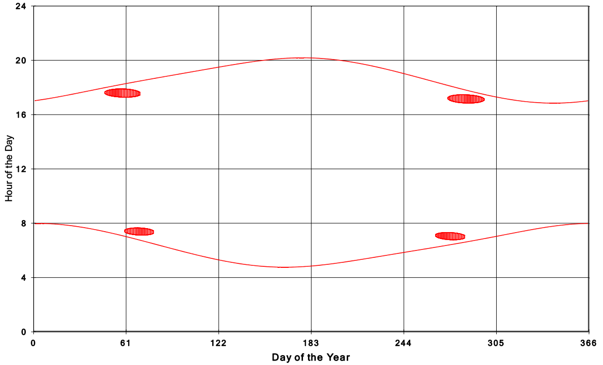
Goshen Wind Energy Centre Shadow Times on House 307, All Windows from All Turbine:
