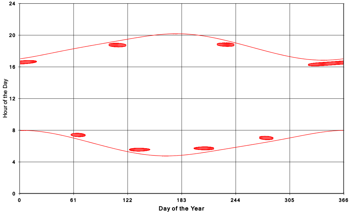
Goshen Wind Energy Centre Shadow Times on House 163, All Windows from All Turbine:
