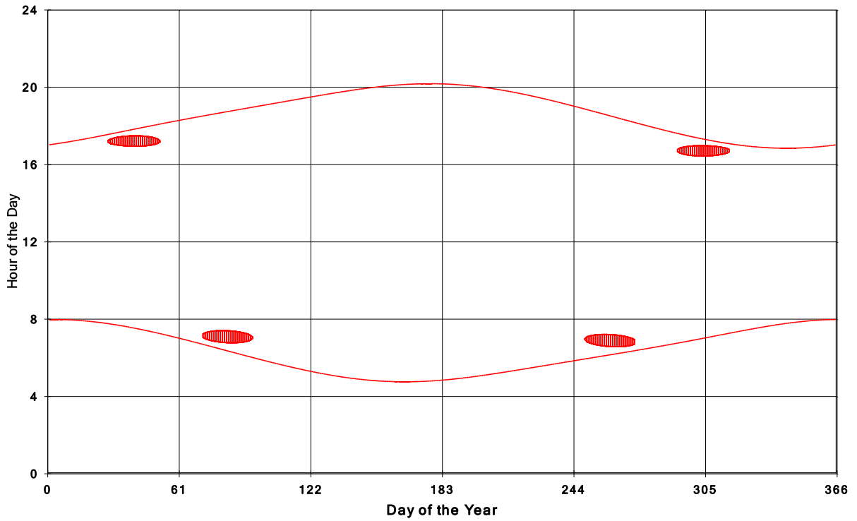
Goshen Wind Energy Centre Shadow Times on House 192, All Windows from All Turbine:
