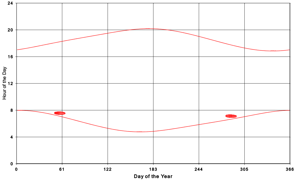
Goshen Wind Energy Centre Shadow Times on House 326, All Windows from All Turbine:
