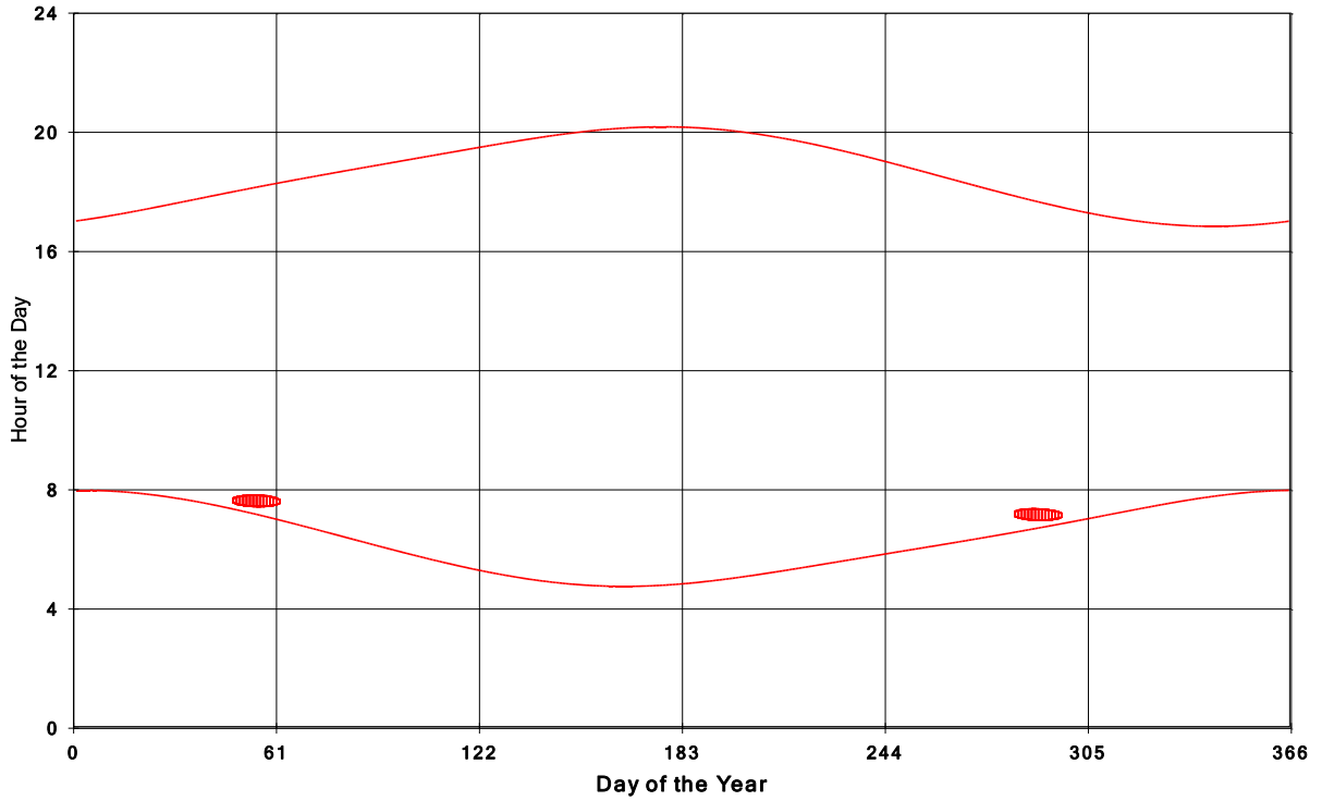
Goshen Wind Energy Centre Shadow Times on House 325, All Windows from All Turbine:
