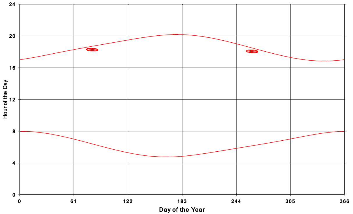
Goshen Wind Energy Centre Shadow Times on House 206, All Windows from All Turbine:
