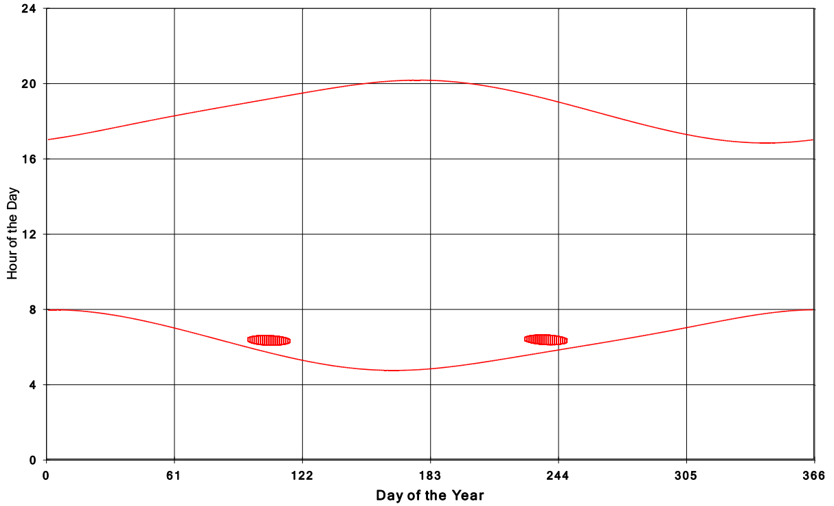
Goshen Wind Energy Centre Shadow Times on House 314, All Windows from All Turbine:
