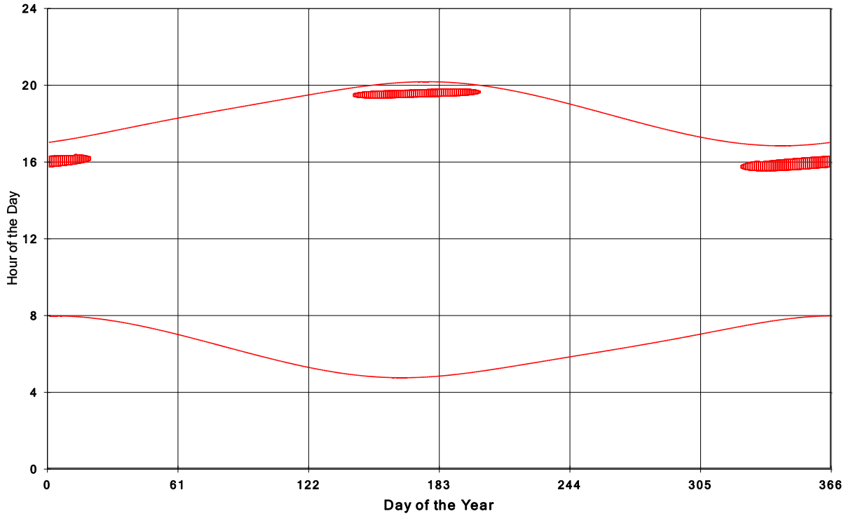
Goshen Wind Energy Centre Shadow Times on House 210, All Windows from All Turbine:
