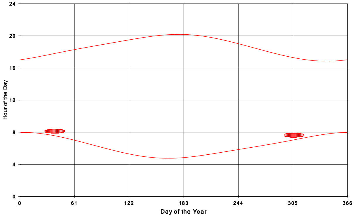
Goshen Wind Energy Centre Shadow Times on House 174, All Windows from All Turbine:
