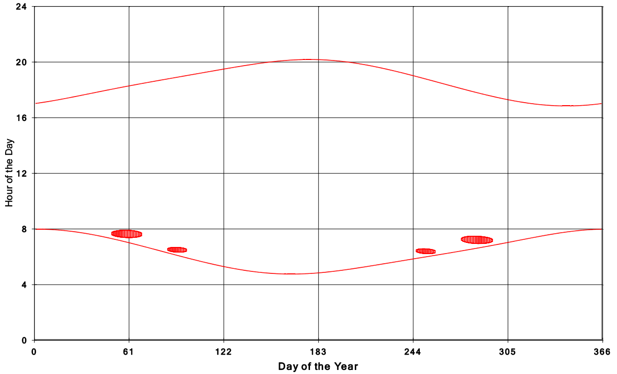
Goshen Wind Energy Centre Shadow Times on House 324, All Windows from All Turbine:
