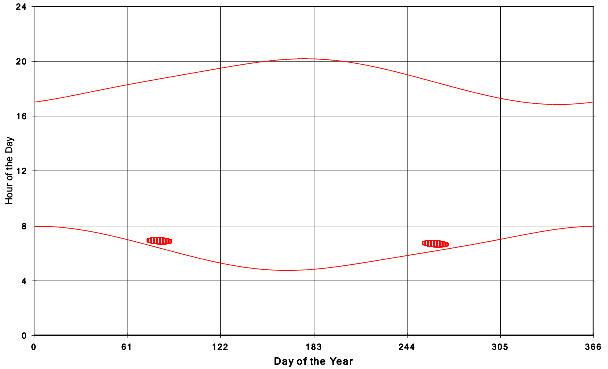
Goshen Wind Energy Centre Shadow Times on House 172, All Windows from All Turbine:
