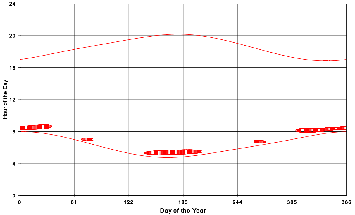
Goshen Wind Energy Centre Shadow Times on House 295, All Windows from All Turbine:
