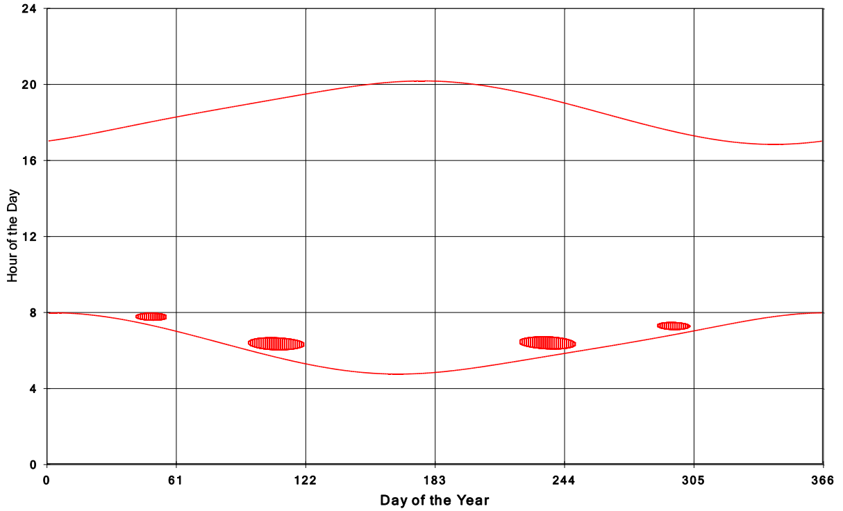
Goshen Wind Energy Centre Shadow Times on House 173, All Windows from All Turbine:
