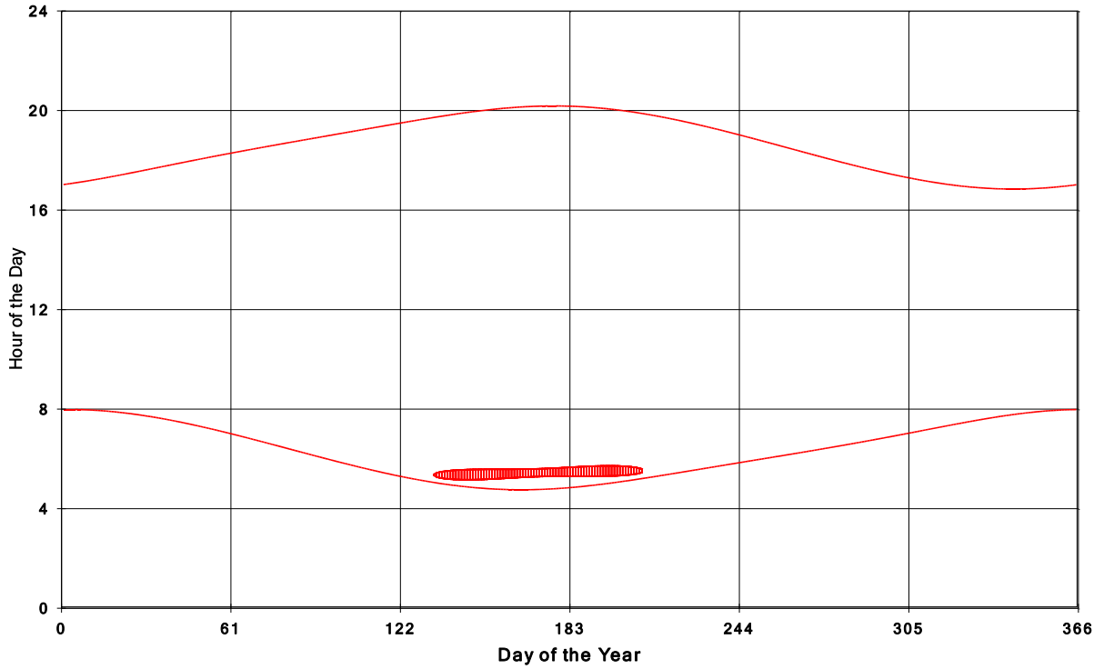
Goshen Wind Energy Centre Shadow Times on House 321, All Windows from All Turbine:
