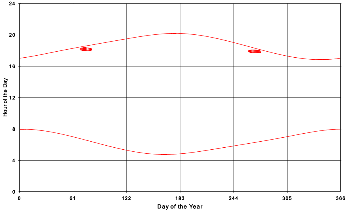
Goshen Wind Energy Centre Shadow Times on House 187, All Windows from All Turbine:
