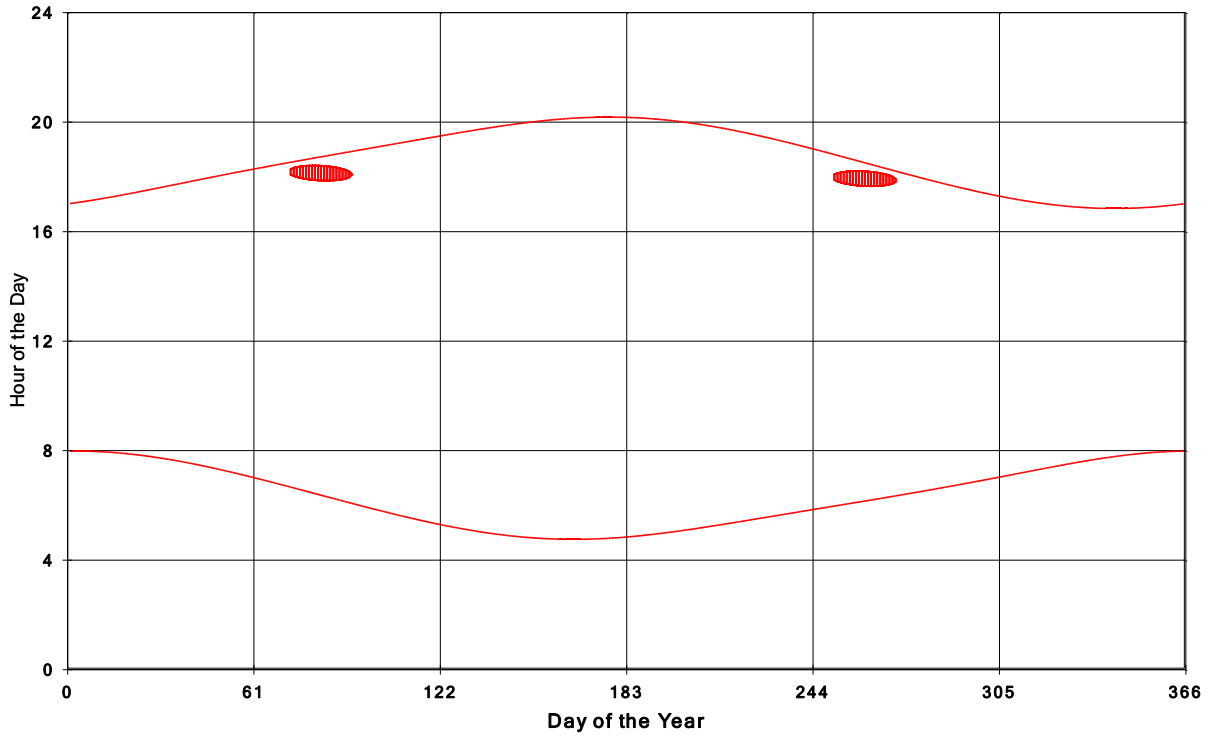
Goshen Wind Energy Centre Shadow Times on House 180, All Windows from All Turbine:
