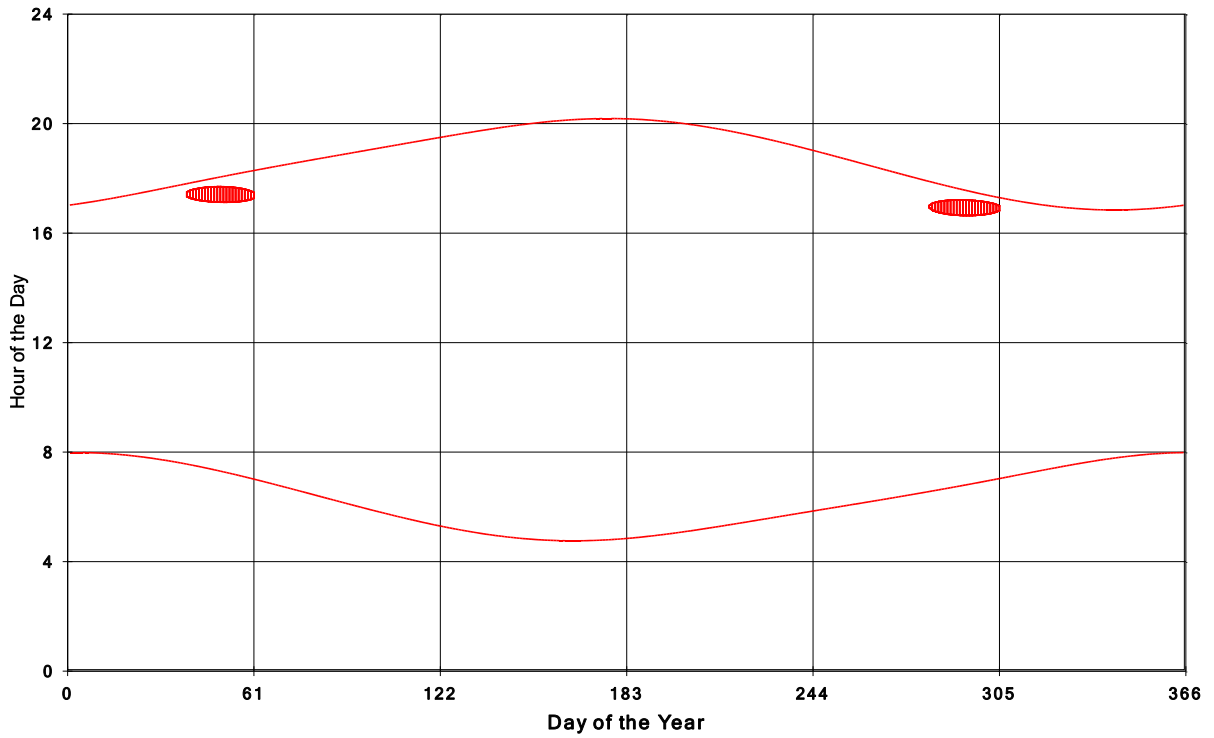
Goshen Wind Energy Centre Shadow Times on House 269, All Windows from All Turbine:
