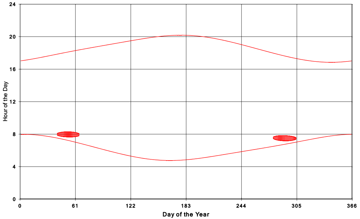
Goshen Wind Energy Centre Shadow Times on House 310, All Windows from All Turbine:
