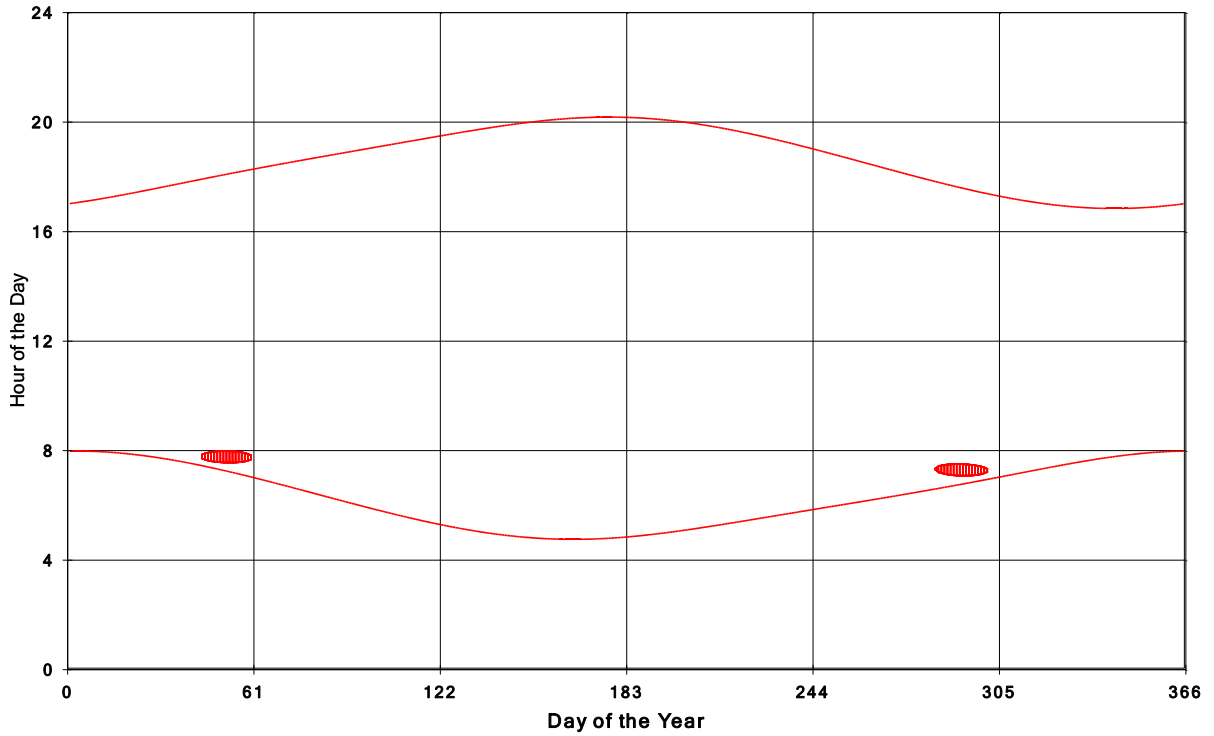
Goshen Wind Energy Centre Shadow Times on House 154, All Windows from All Turbine:
