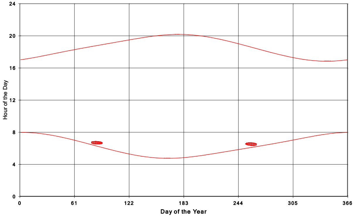
Goshen Wind Energy Centre Shadow Times on House 308, All Windows from All Turbine:
