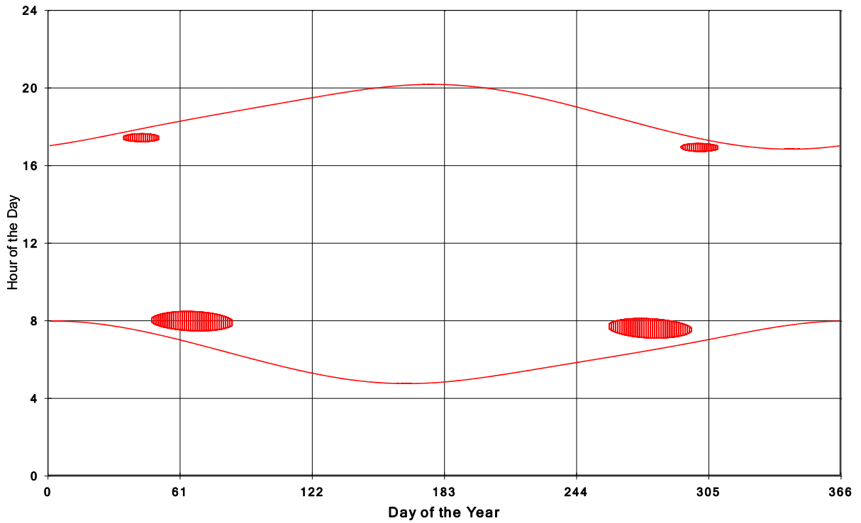
Goshen Wind Energy Centre Shadow Times on House 193, All Windows from All Turbine:
