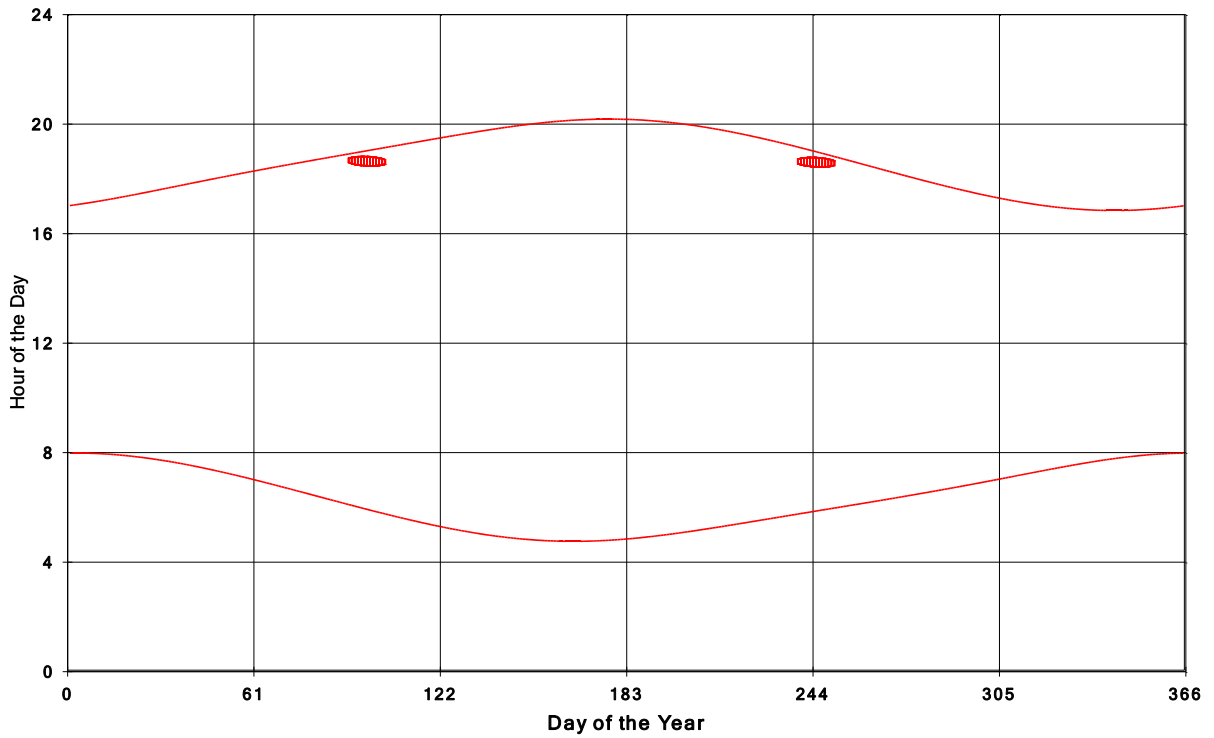
Goshen Wind Energy Centre Shadow Times on House 216, All Windows from All Turbine:
