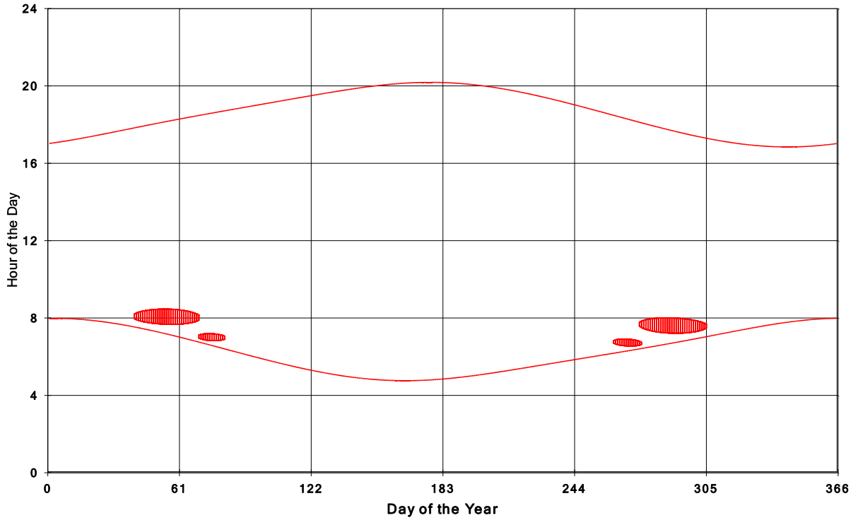
Goshen Wind Energy Centre Shadow Times on House 212, All Windows from All Turbine:
