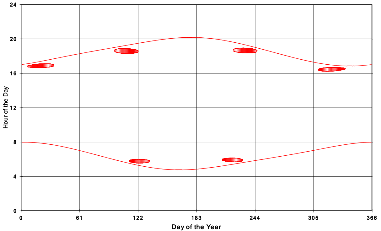
Goshen Wind Energy Centre Shadow Times on House 167, All Windows from All Turbine:
