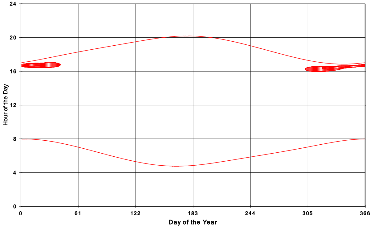
Goshen Wind Energy Centre Shadow Times on House 201, All Windows from All Turbine:
