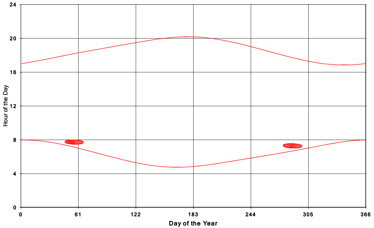
Goshen Wind Energy Centre Shadow Times on House 311, All Windows from All Turbine:
