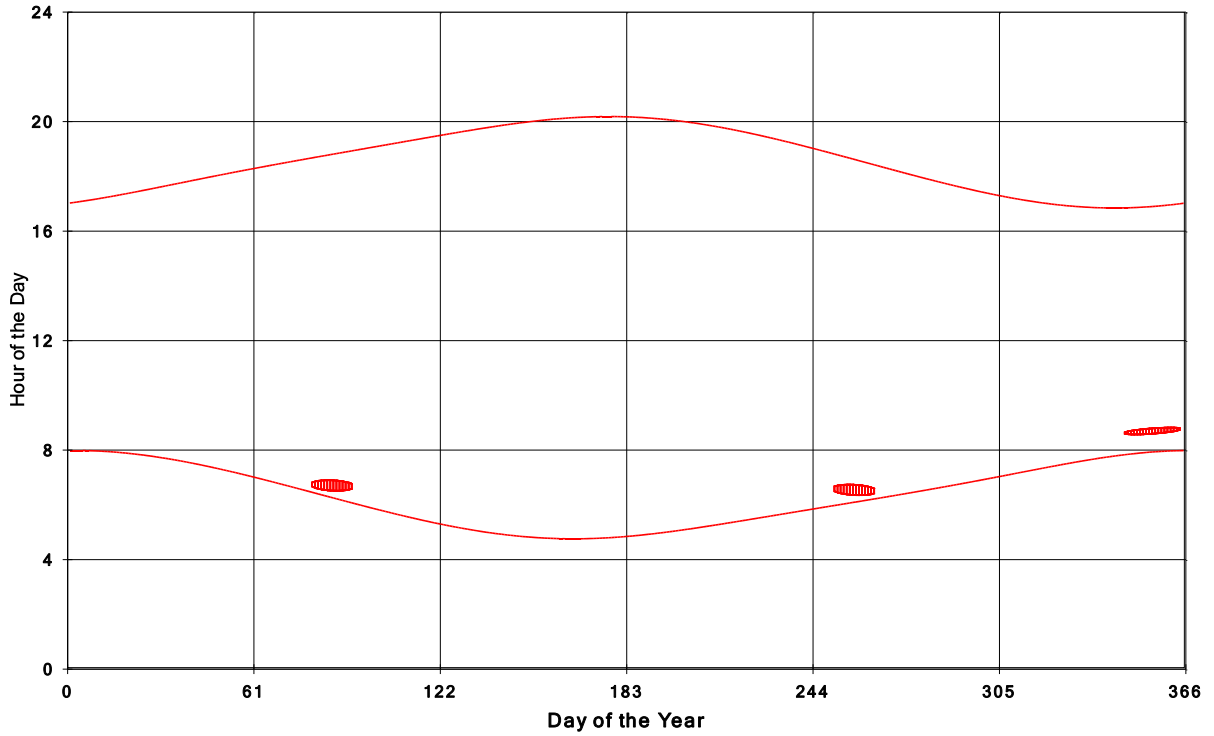
Goshen Wind Energy Centre Shadow Times on House 327, All Windows from All Turbine:
