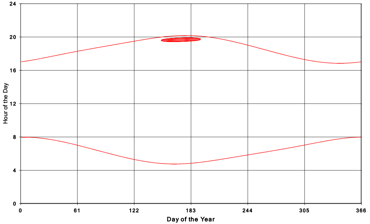
Goshen Wind Energy Centre Shadow Times on House 157, All Windows from All Turbine:
