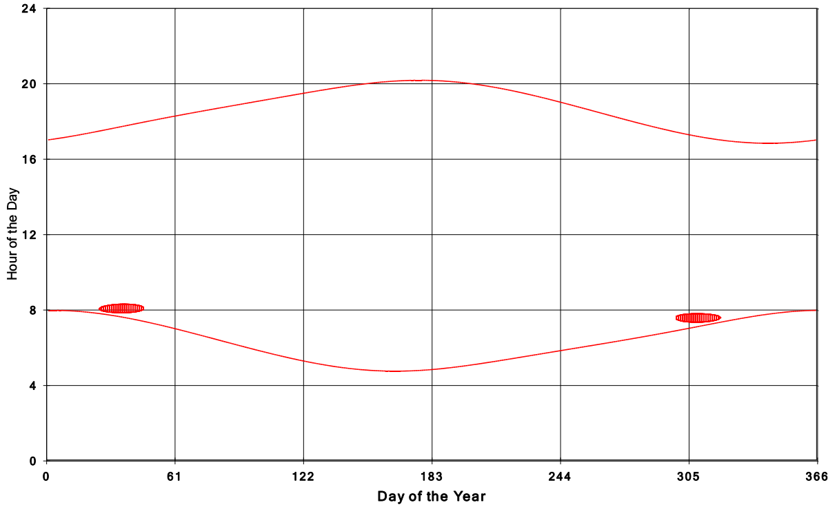
Goshen Wind Energy Centre Shadow Times on House 183, All Windows from All Turbine:
