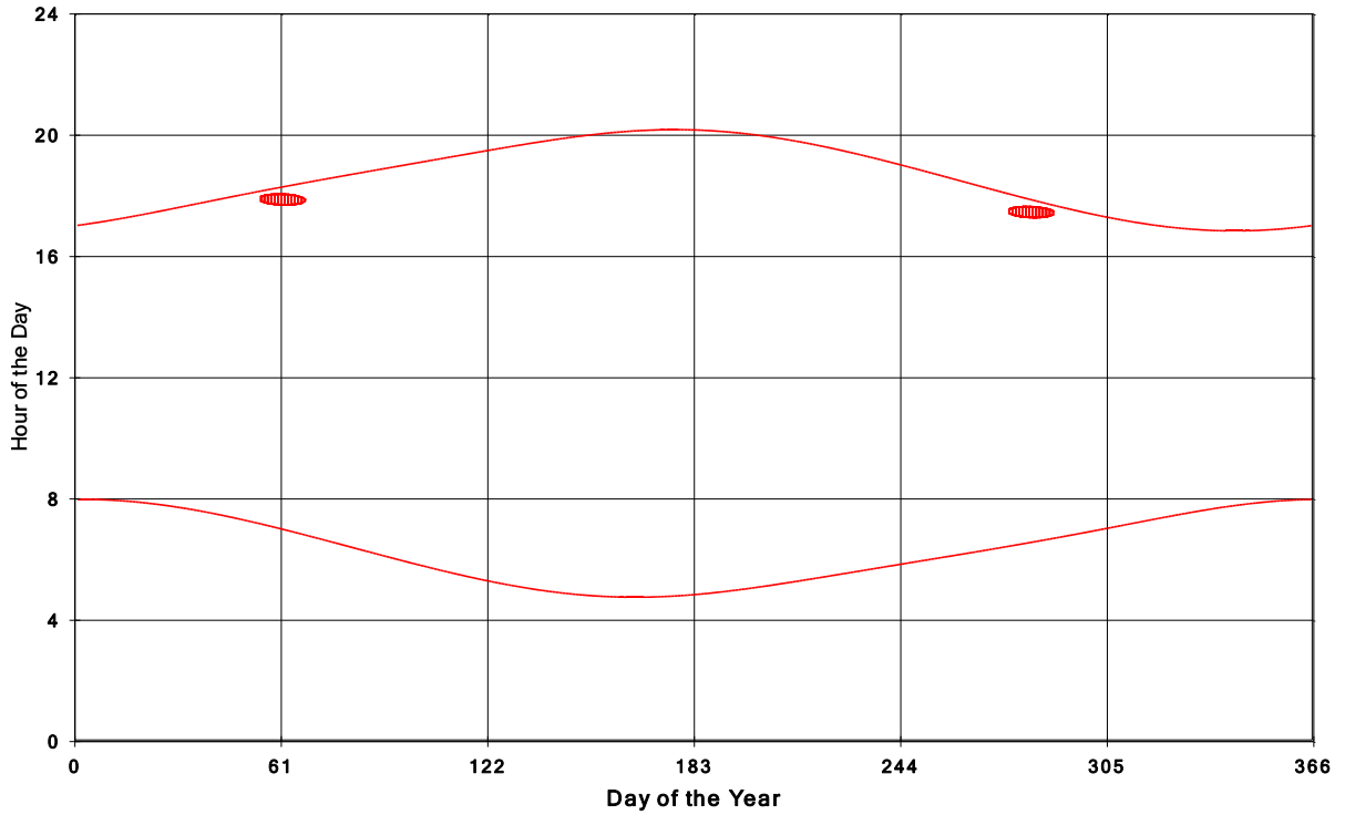
Goshen Wind Energy Centre Shadow Times on House 253, All Windows from All Turbine:
