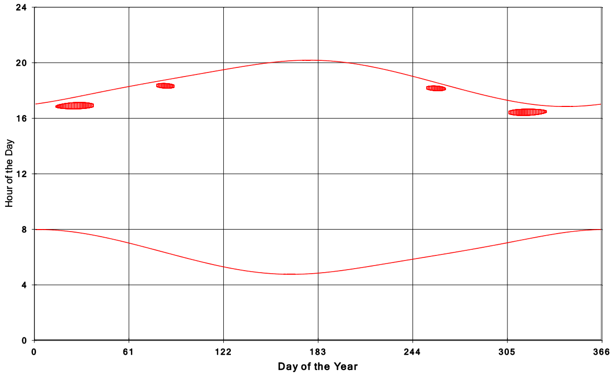
Goshen Wind Energy Centre Shadow Times on House 7, All Windows from All Turbines:
