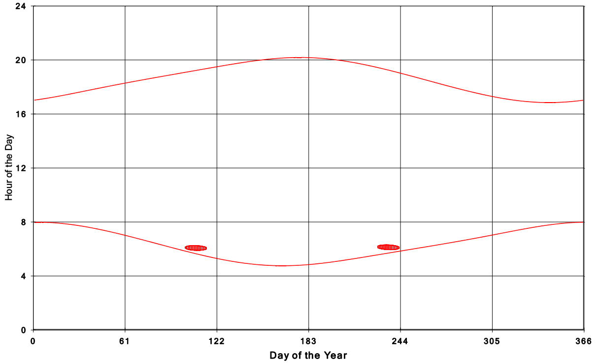
Goshen Wind Energy Centre Shadow Times on House 107, All Windows from All Turbine:
