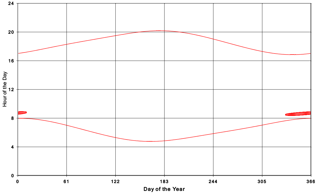
Goshen Wind Energy Centre Shadow Times on House 71, All Windows from All Turbine:
