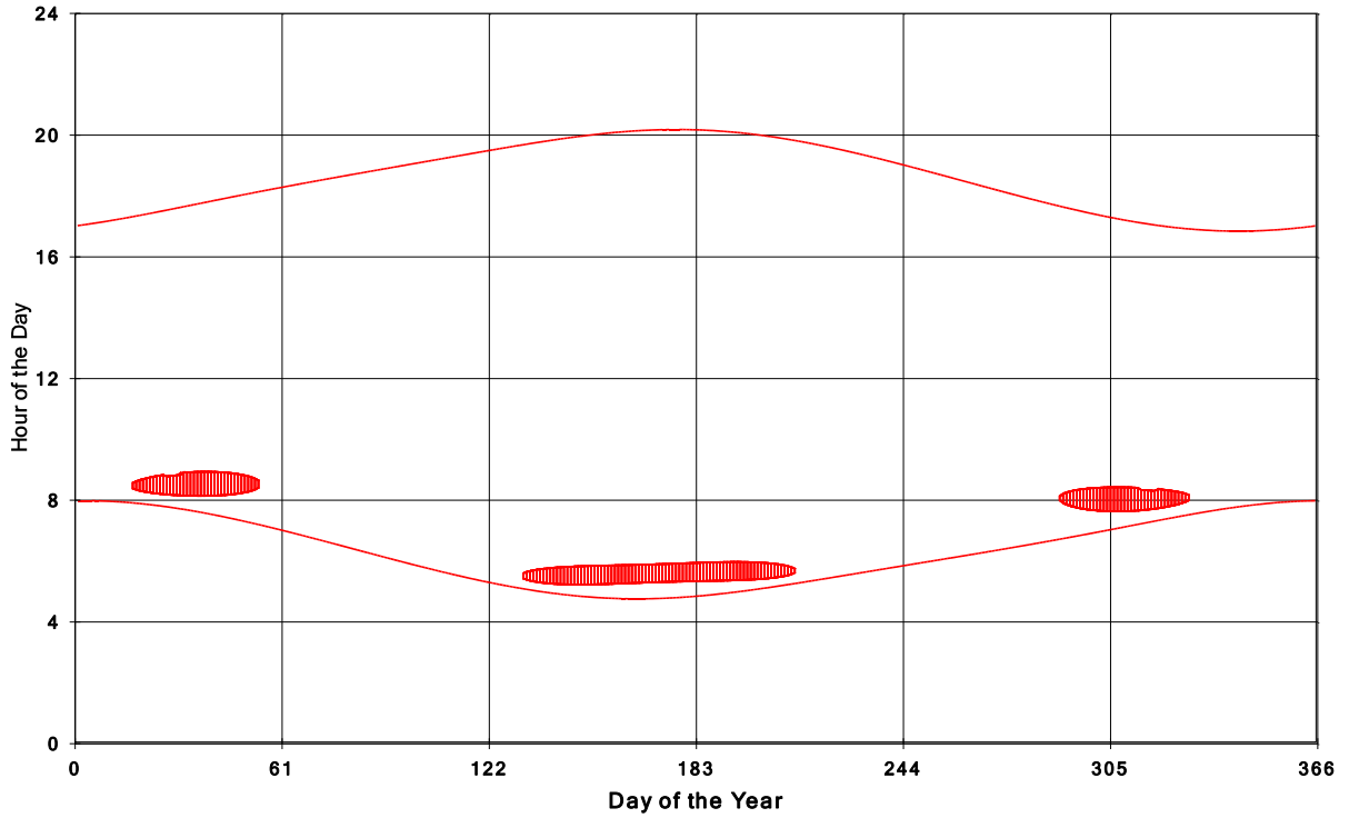
Goshen Wind Energy Centre Shadow Times on House 100, All Windows from All Turbine:
