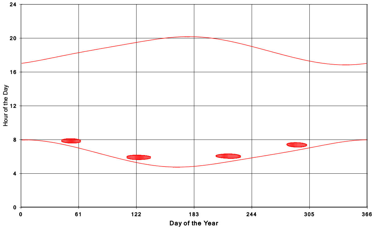
Goshen Wind Energy Centre Shadow Times on House 113, All Windows from All Turbine:
