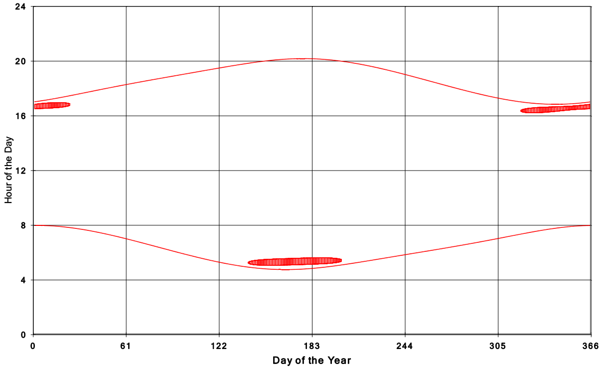
Jericho Wind Energy Centre Shadow Times on House 73, All Windows from All Turbine:
