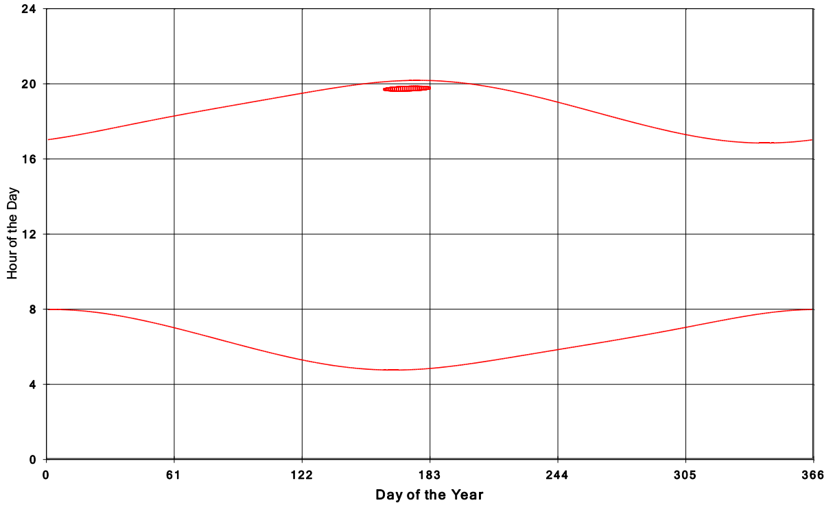
Goshen Wind Energy Centre Shadow Times on House 127, All Windows from All Turbine:
