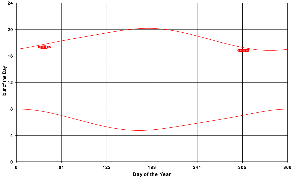
Goshen Wind Energy Centre Shadow Times on House 81, All Windows from All Turbine:
