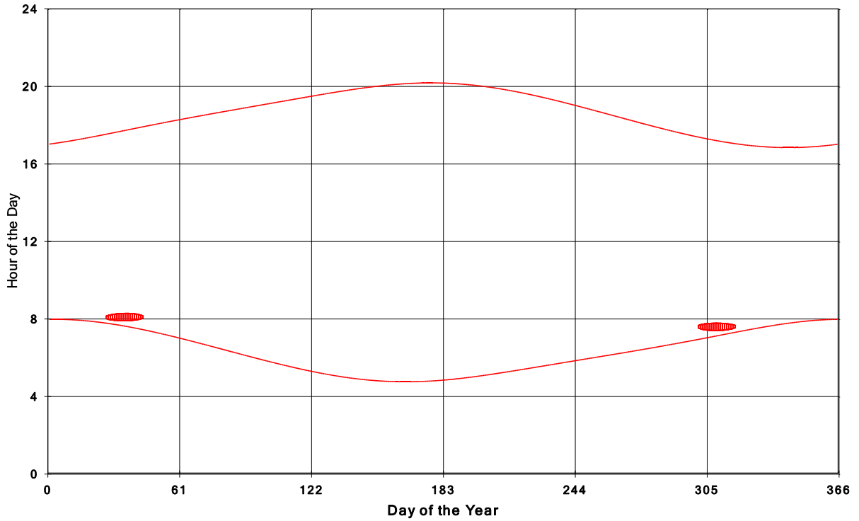
Goshen Wind Energy Centre Shadow Times on House 47, All Windows from All Turbine:
