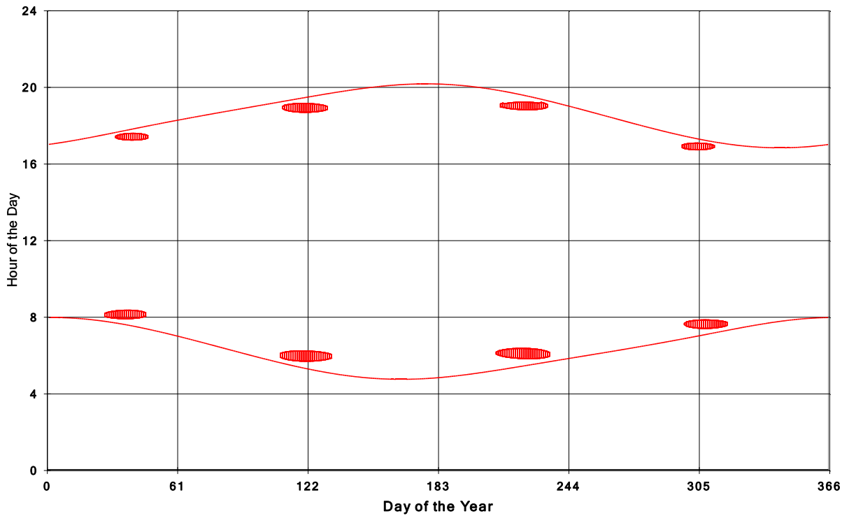
Goshen Wind Energy Centre Shadow Times on House 4, All Windows from All Turbines:
