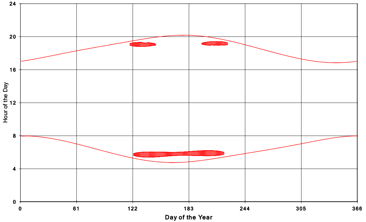
Goshen Wind Energy Centre Shadow Times on House 110, All Windows from All Turbine:
