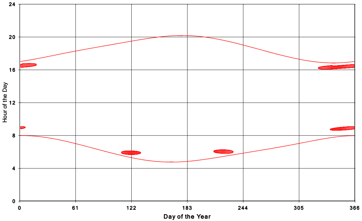
Jericho Wind Energy Centre Shadow Times on House 136, All Windows from All Turbine:
