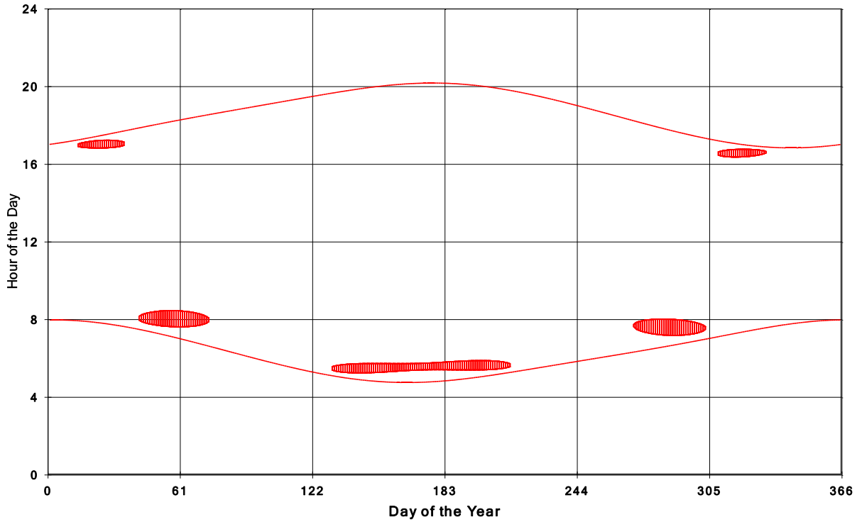
Goshen Wind Energy Centre Shadow Times on House 83, All Windows from All Turbine:
