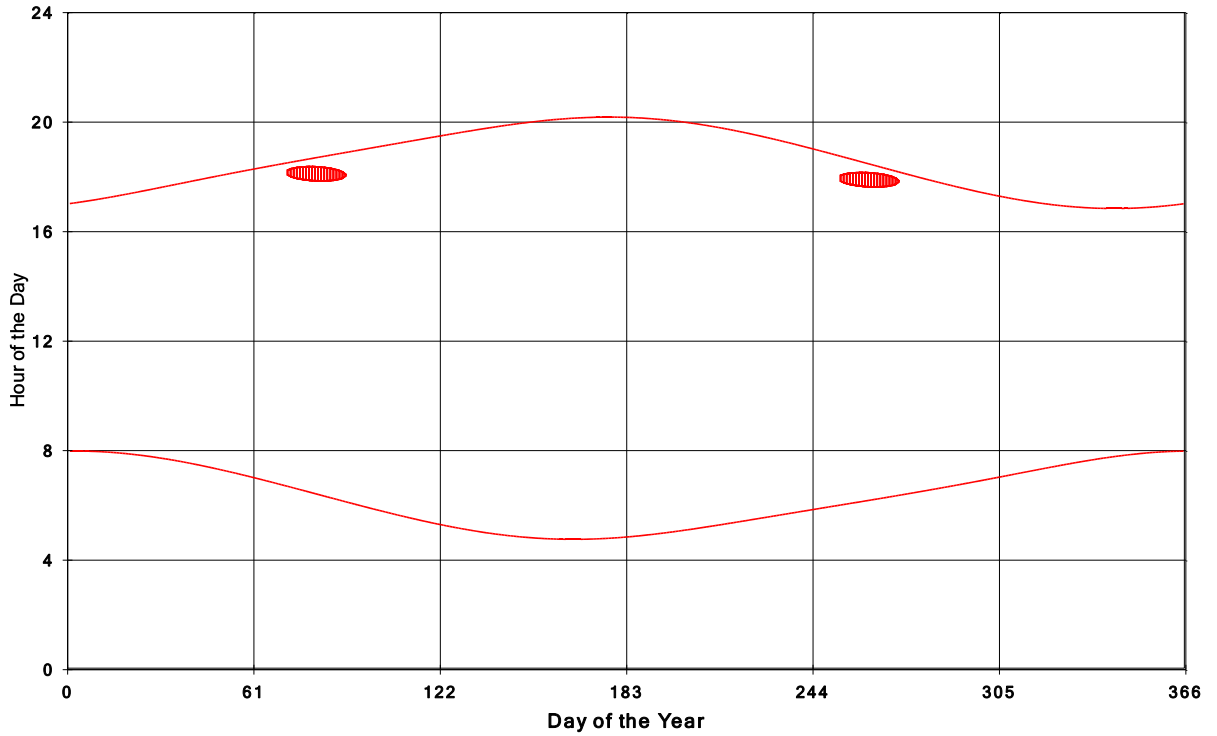
Goshen Wind Energy Centre Shadow Times on House 11, All Windows from All Turbine:
