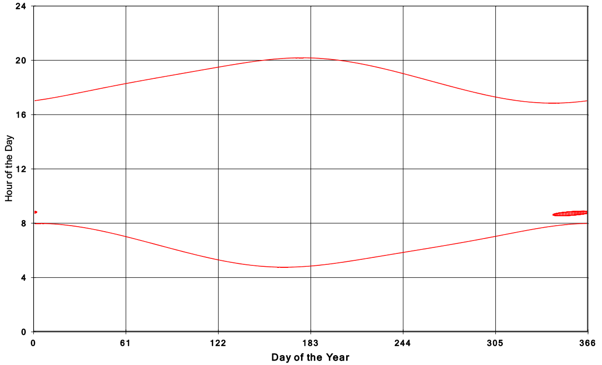
Goshen Wind Energy Centre Shadow Times on House 72, All Windows from All Turbine:
