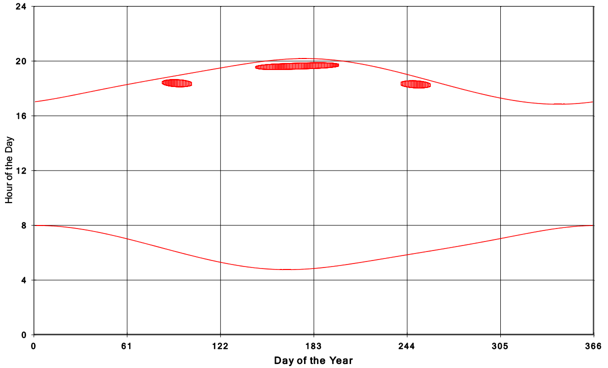
Goshen Wind Energy Centre Shadow Times on House 27, All Windows from All Turbine:
