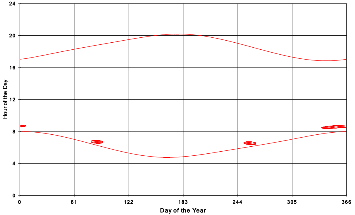
Goshen Wind Energy Centre Shadow Times on House 46, All Windows from All Turbine:
