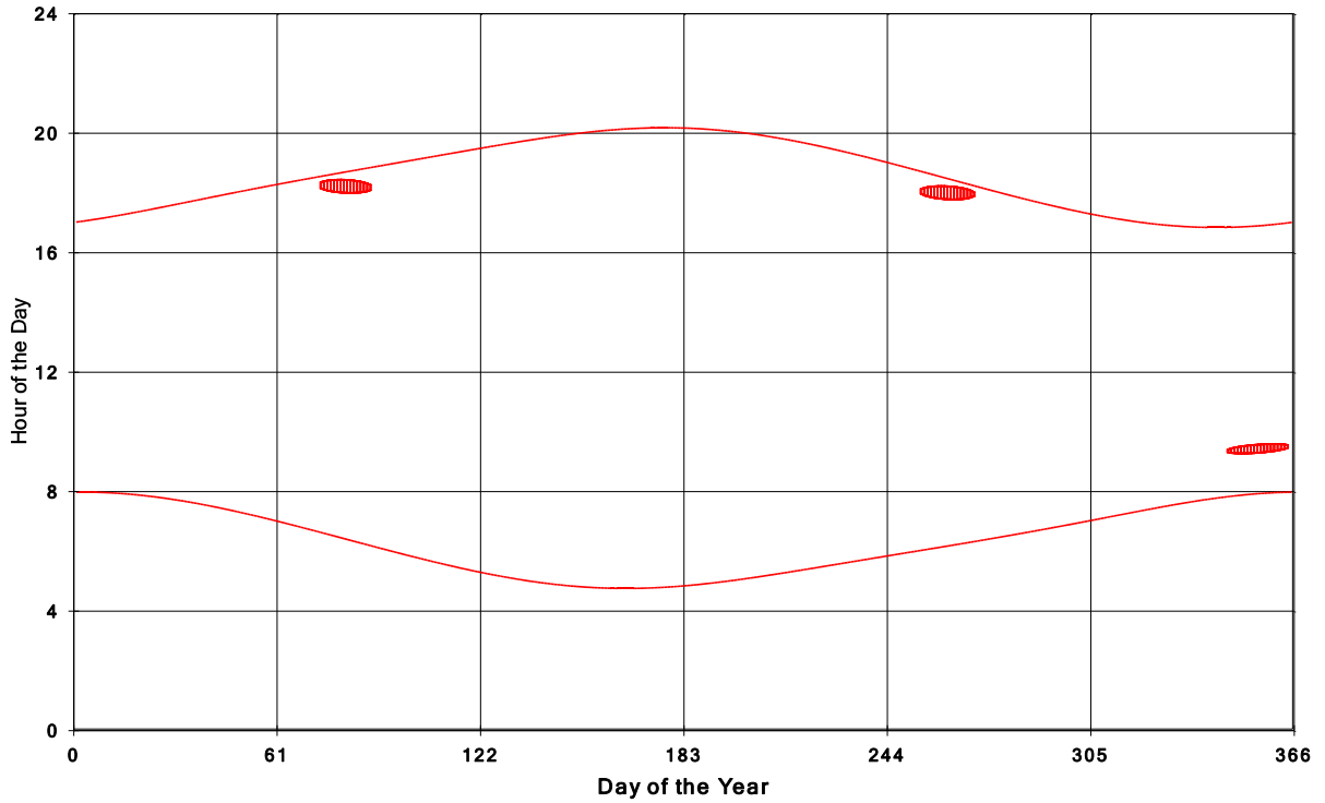
Goshen Wind Energy Centre Shadow Times on House 121, All Windows from All Turbine:
