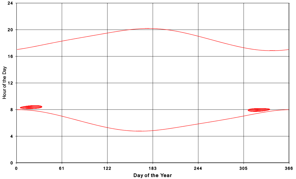
Goshen Wind Energy Centre Shadow Times on House 13, All Windows from All Turbine:
