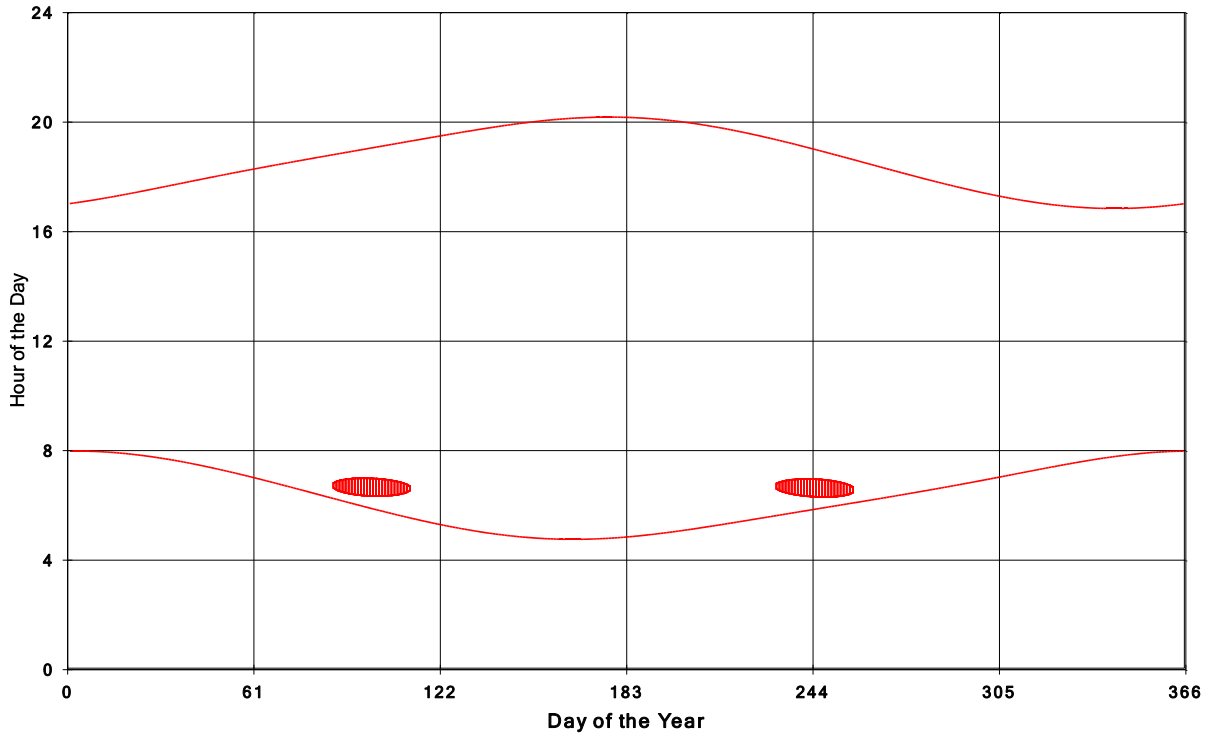
Goshen Wind Energy Centre Shadow Times on House 138, All Windows from All Turbine:
