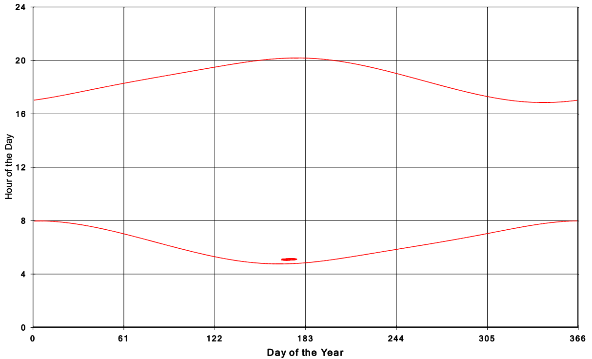
Goshen Wind Energy Centre Shadow Times on House 34, All Windows from All Turbine:
