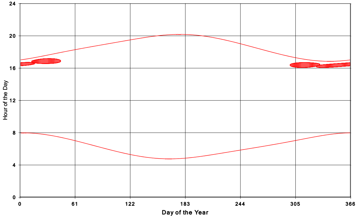
Goshen Wind Energy Centre Shadow Times on House 120, All Windows from All Turbine:
