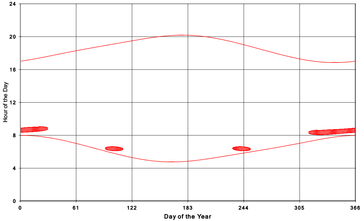
Goshen Wind Energy Centre Shadow Times on House 45, All Windows from All Turbine:
