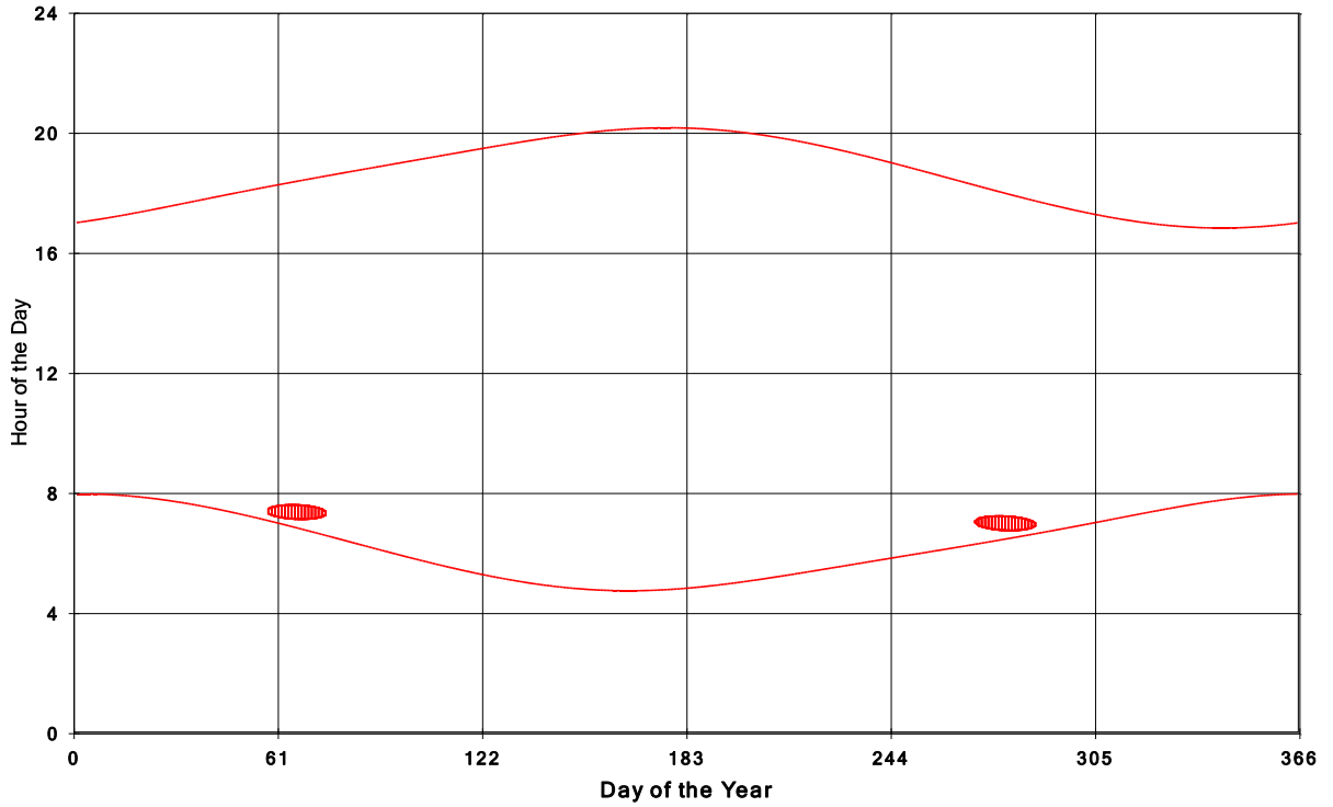
Goshen Wind Energy Centre Shadow Times on House 14, All Windows from All Turbine:
