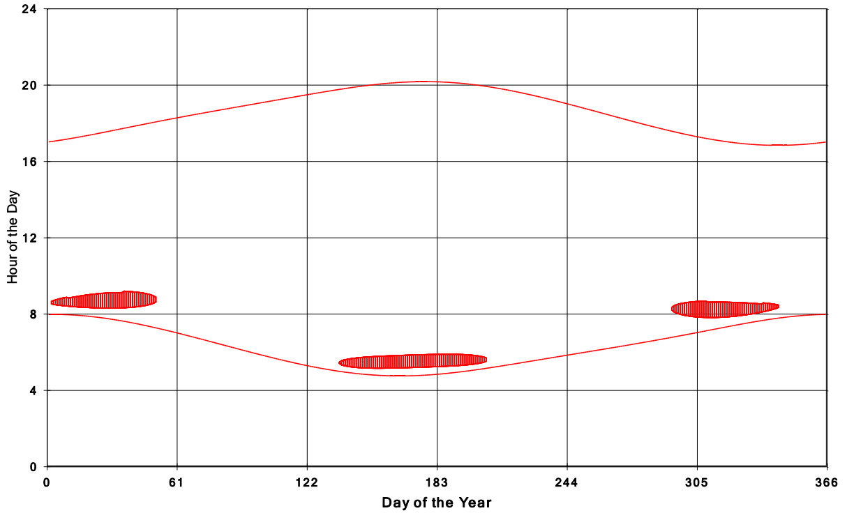
Goshen Wind Energy Centre Shadow Times on House 101, All Windows from All Turbine:
