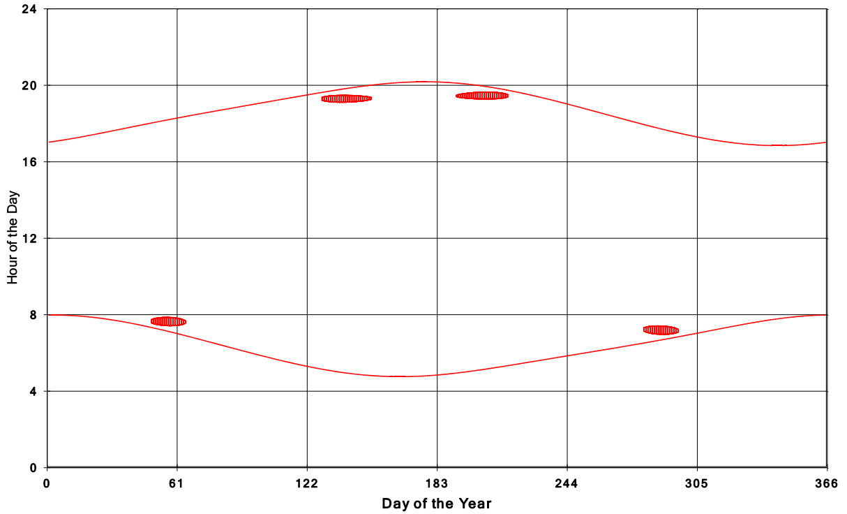
Goshen Wind Energy Centre Shadow Times on House 36, All Windows from All Turbine:
