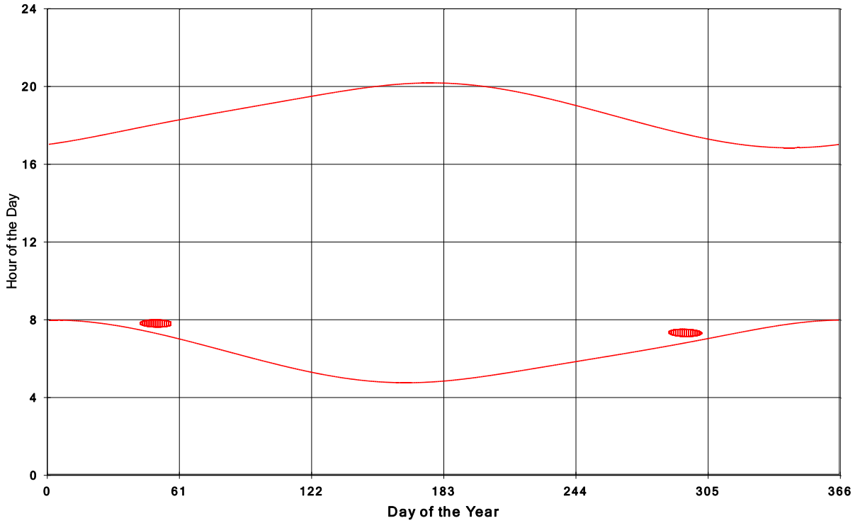
Jericho Wind Energy Centre Shadow Times on House 135, All Windows from All Turbine:
