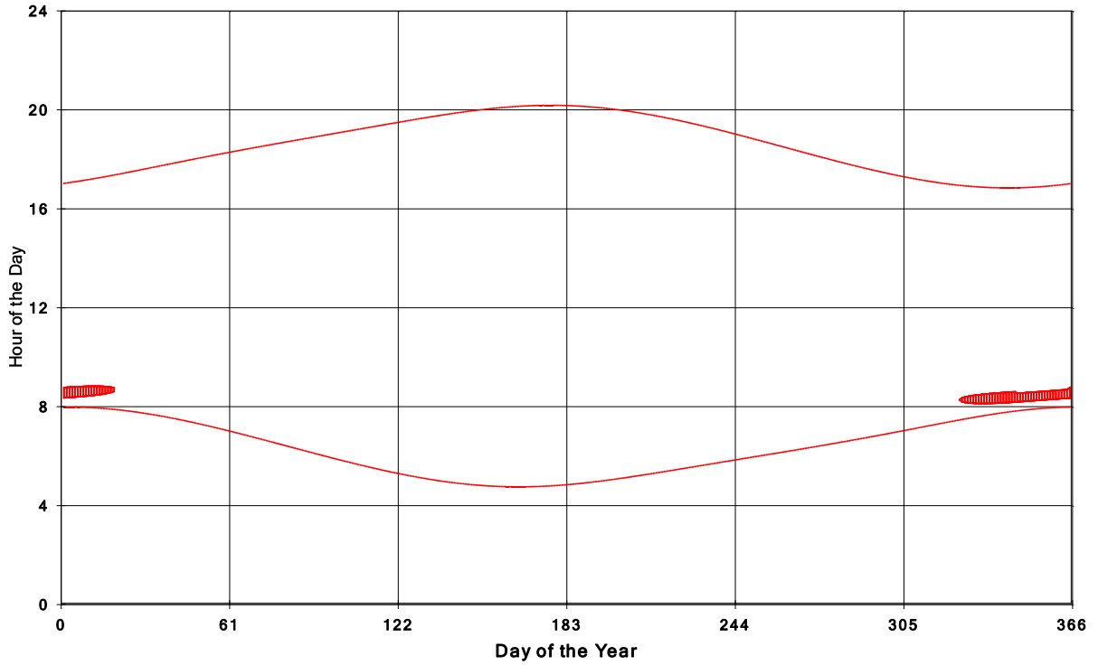
Goshen Wind Energy Centre Shadow Times on House 137, All Windows from All Turbine:
