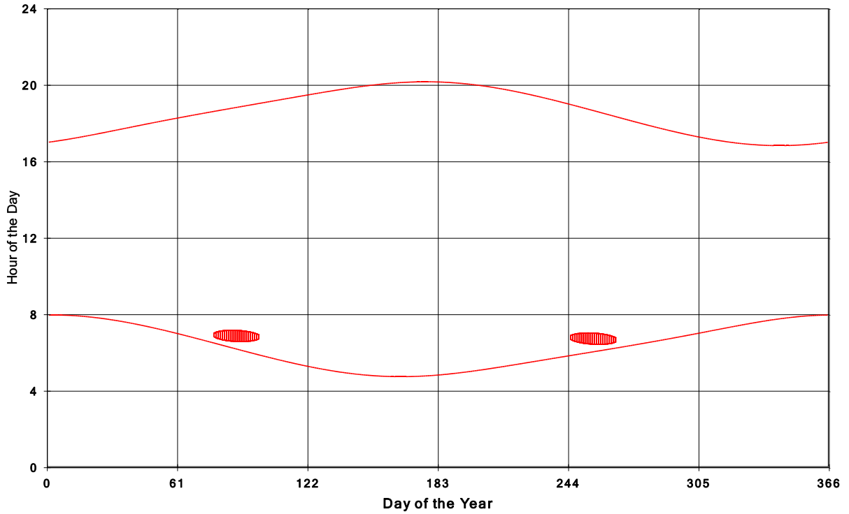
Goshen Wind Energy Centre Shadow Times on House 140, All Windows from All Turbine:
