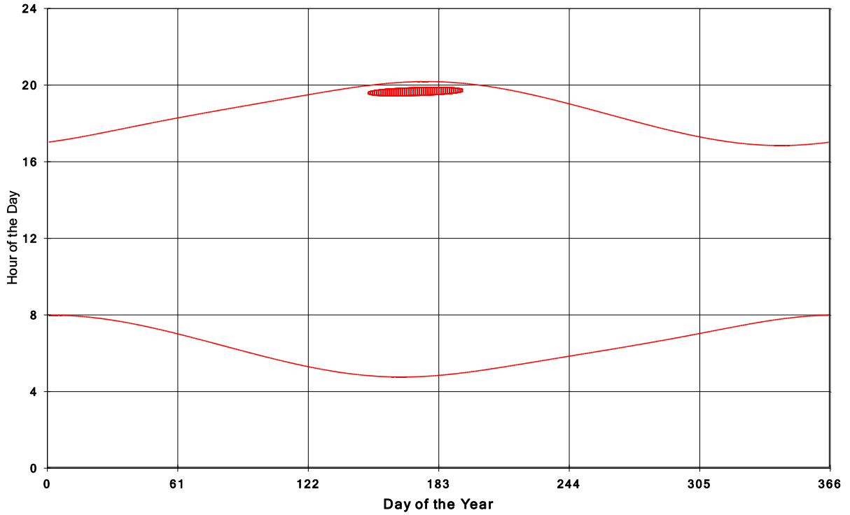
Goshen Wind Energy Centre Shadow Times on House 128, All Windows from All Turbine:
