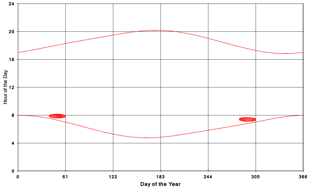
Goshen Wind Energy Centre Shadow Times on House 75, All Windows from All Turbine:
