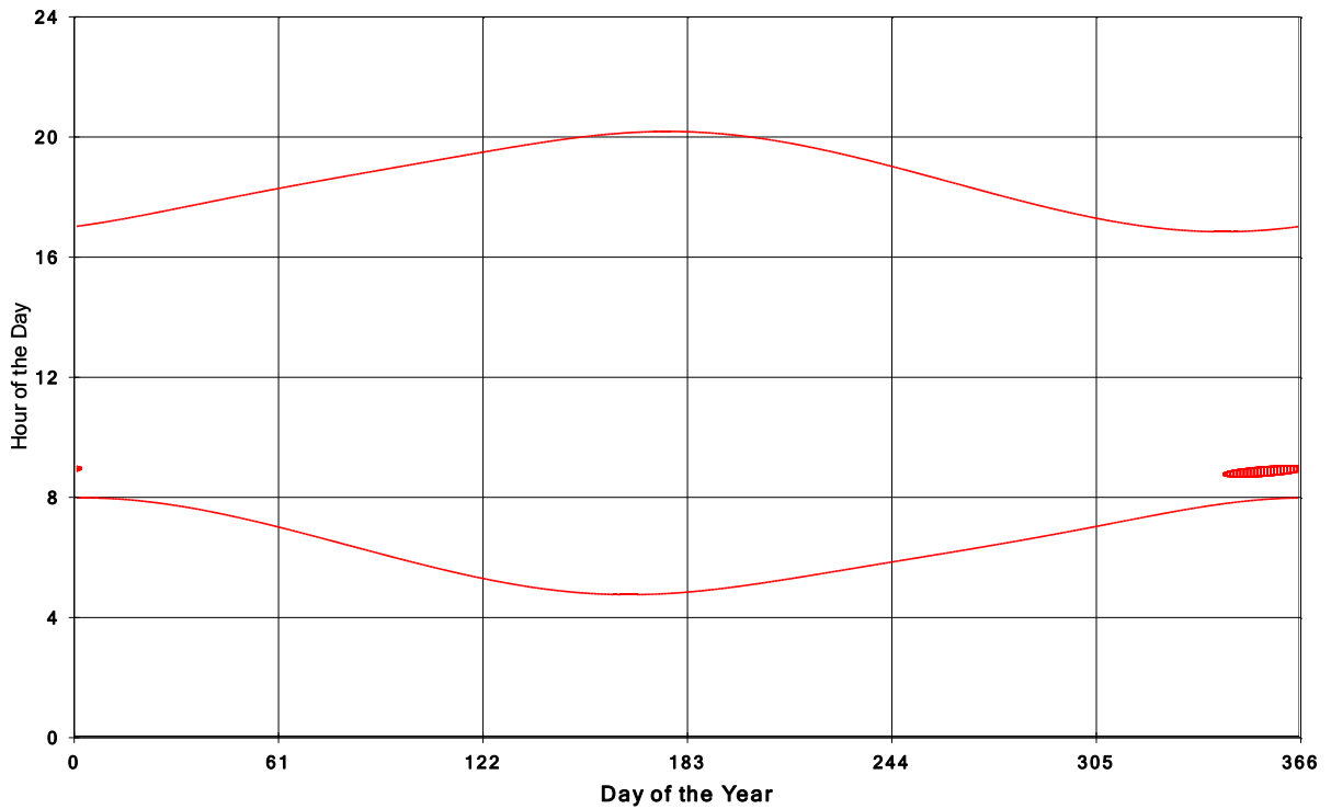
Goshen Wind Energy Centre Shadow Times on House 8, All Windows from All Turbines:
