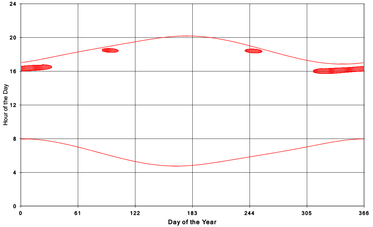
Goshen Wind Energy Centre Shadow Times on House 1, All Windows from All Turbines
