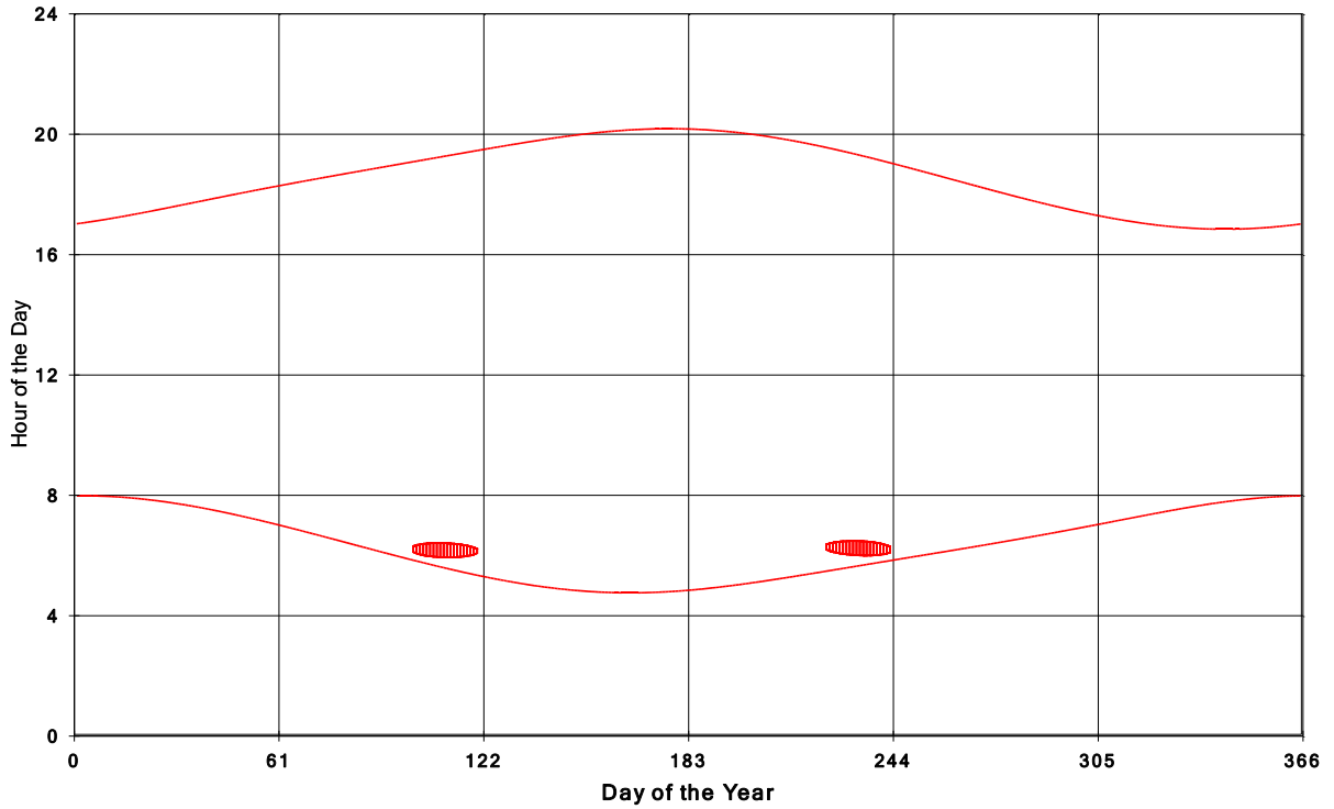
Goshen Wind Energy Centre Shadow Times on House 134, All Windows from All Turbine:
