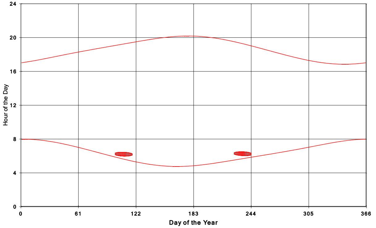
Goshen Wind Energy Centre Shadow Times on House 18, All Windows from All Turbine:
