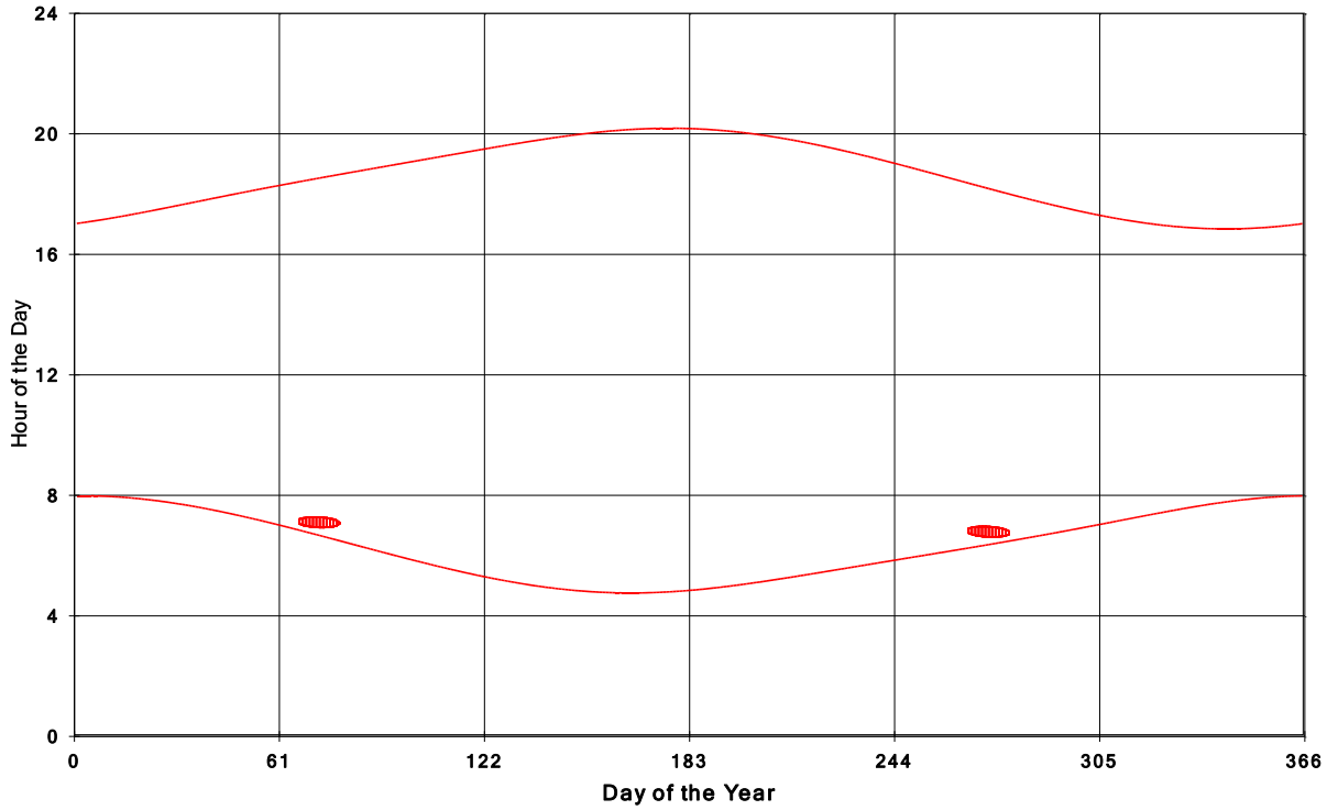
Goshen Wind Energy Centre Shadow Times on House 56, All Windows from All Turbine:
