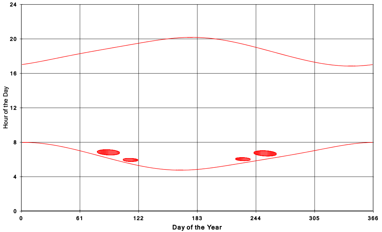
Goshen Wind Energy Centre Shadow Times on House 3, All Windows from All Turbines:
