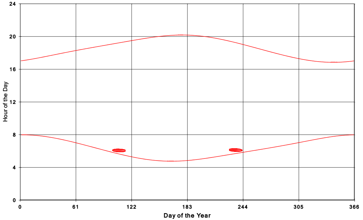
Goshen Wind Energy Centre Shadow Times on House 108, All Windows from All Turbine:
