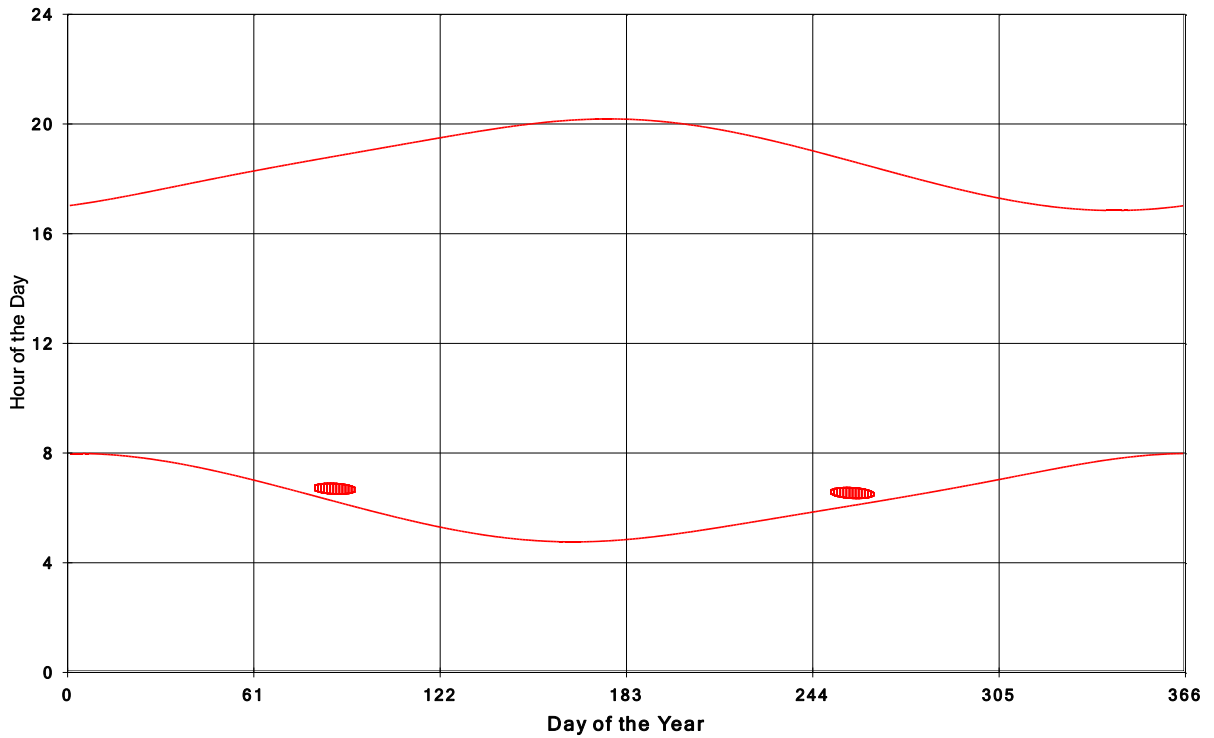
Goshen Wind Energy Centre Shadow Times on House 2, All Windows from All Turbines
