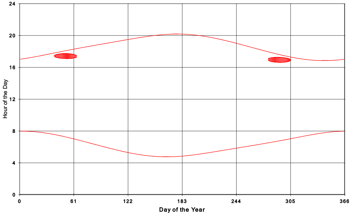
Goshen Wind Energy Centre Shadow Times on House 87, All Windows from All Turbine:
