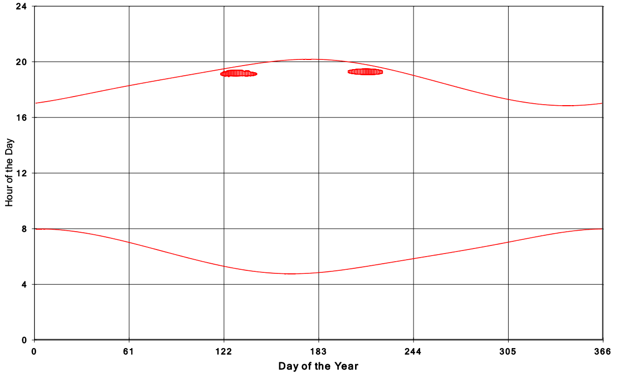
Goshen Wind Energy Centre Shadow Times on House 28, All Windows from All Turbine:
