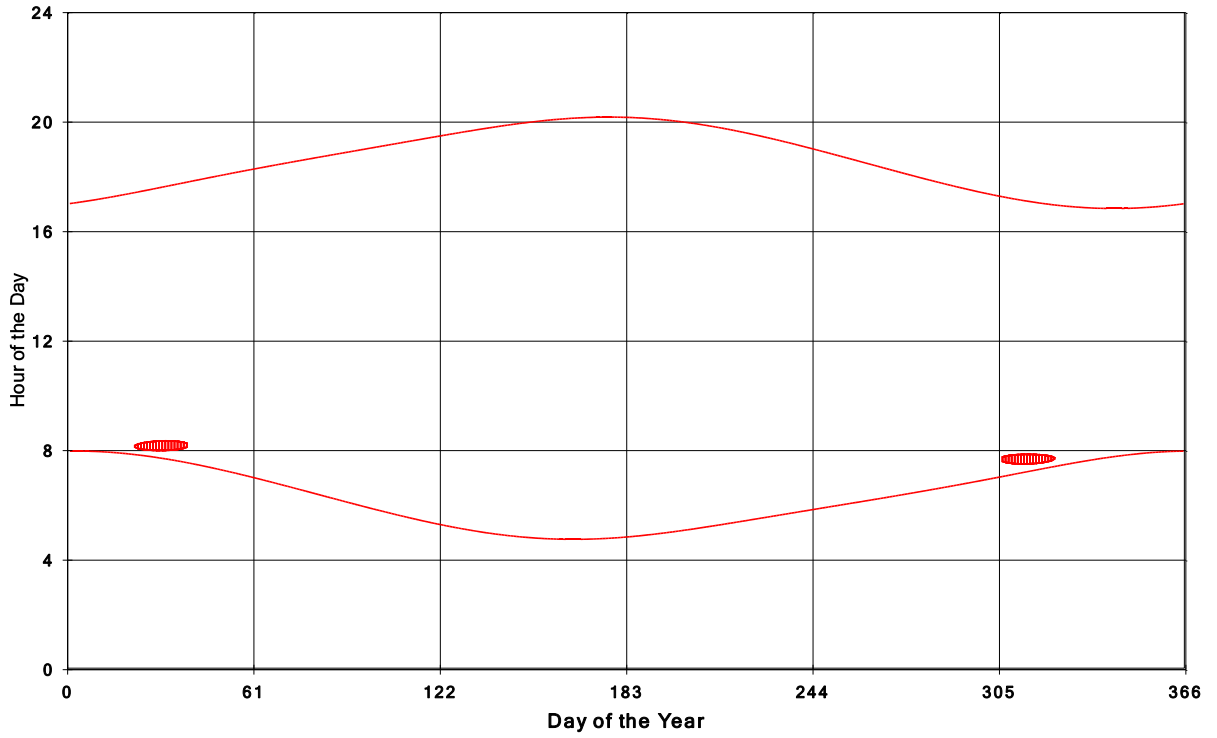
Goshen Wind Energy Centre Shadow Times on House 24, All Windows from All Turbine:
