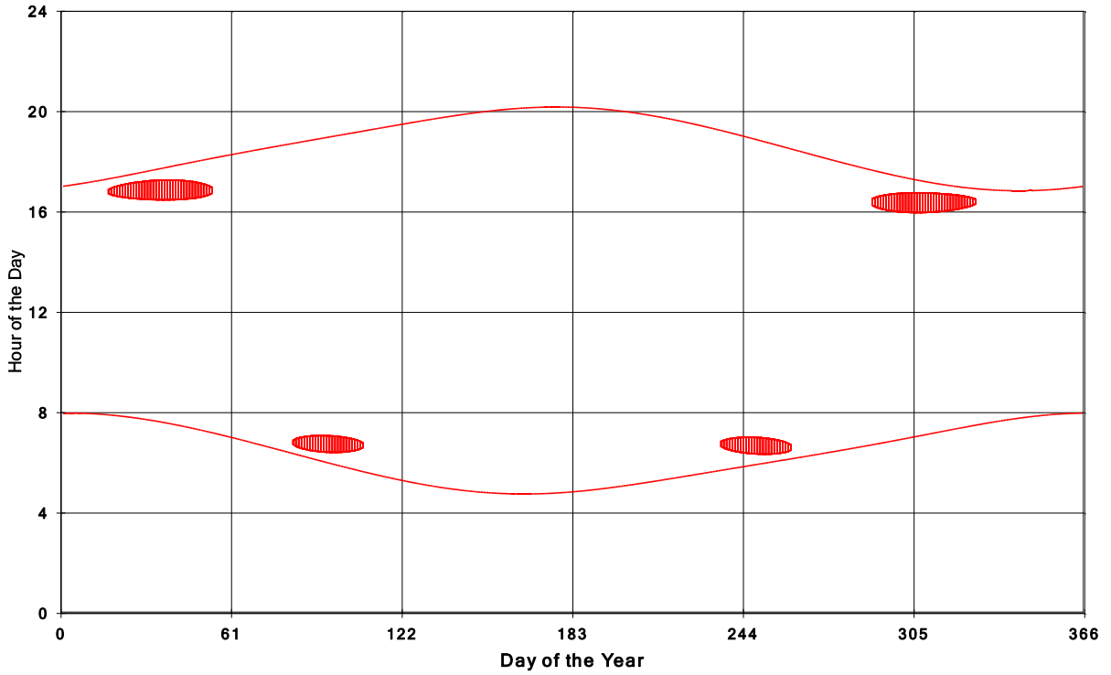
Jericho Wind Energy Centre Shadow Times on House 33, All Windows from All Turbine:
