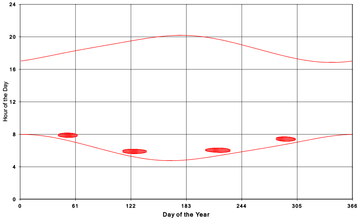
Goshen Wind Energy Centre Shadow Times on House 114, All Windows from All Turbine:
