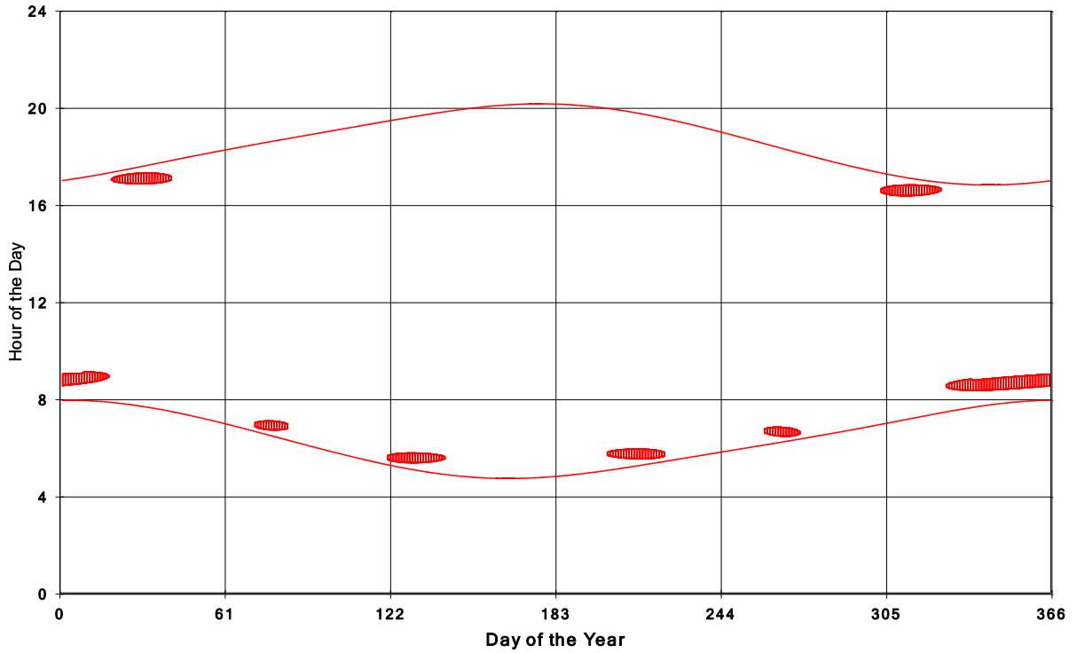
Goshen Wind Energy Centre Shadow Times on House 112, All Windows from All Turbine:
