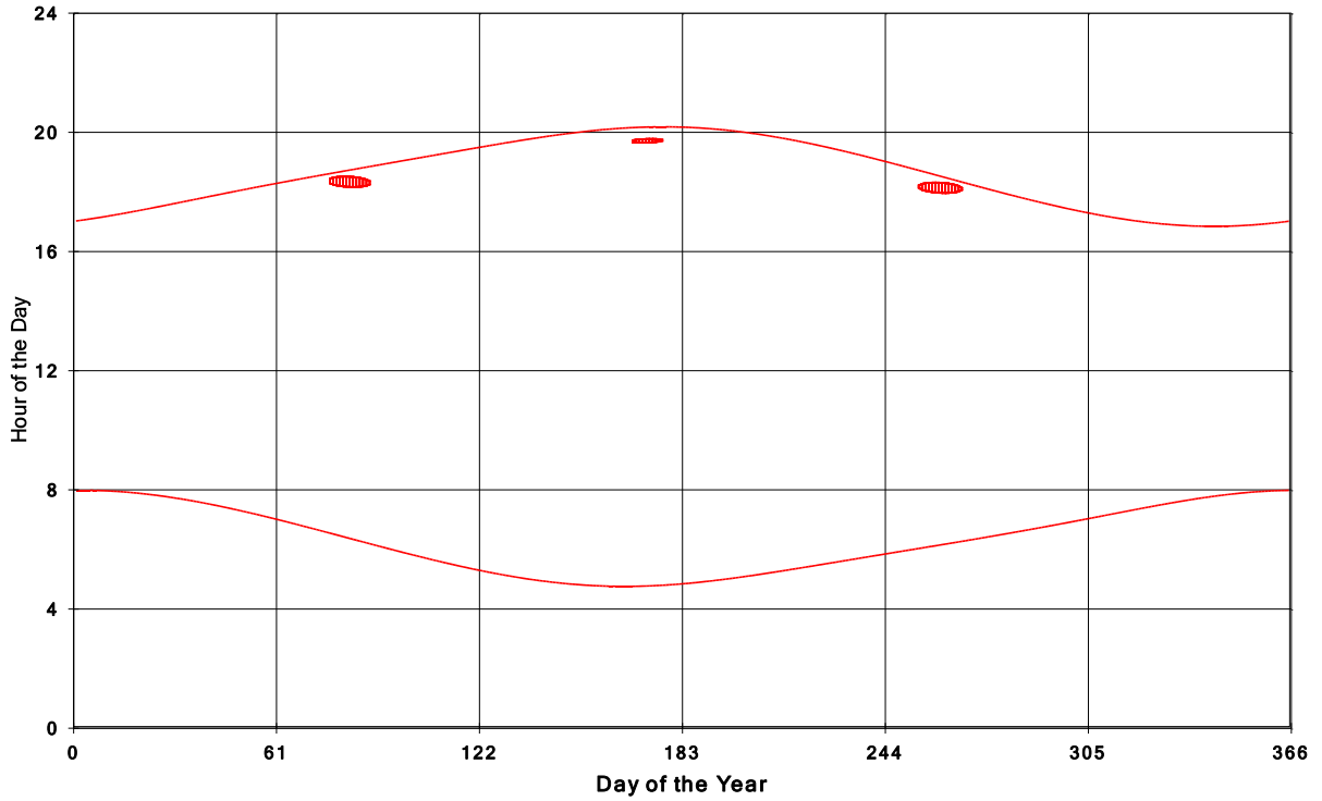
Goshen Wind Energy Centre Shadow Times on House 84, All Windows from All Turbine:
