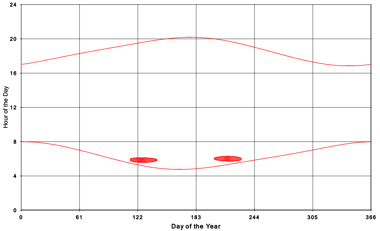
Goshen Wind Energy Centre Shadow Times on House 116, All Windows from All Turbine:
