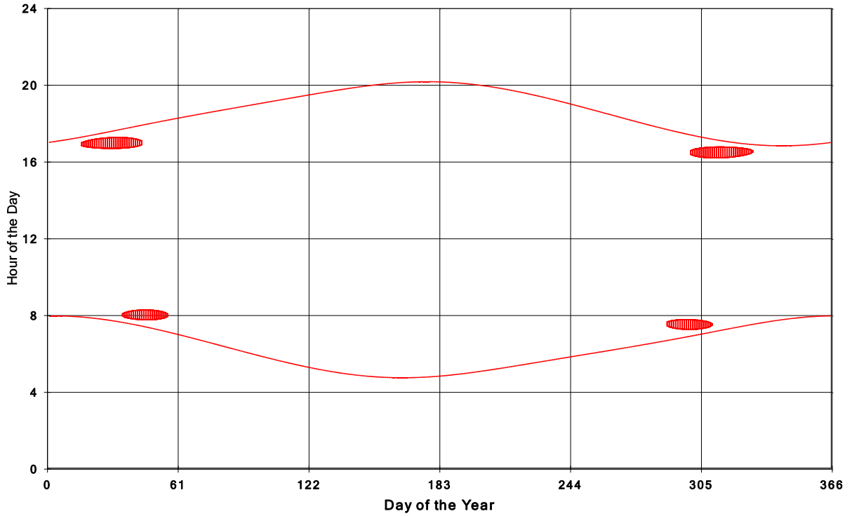
Goshen Wind Energy Centre Shadow Times on House 86, All Windows from All Turbine:
