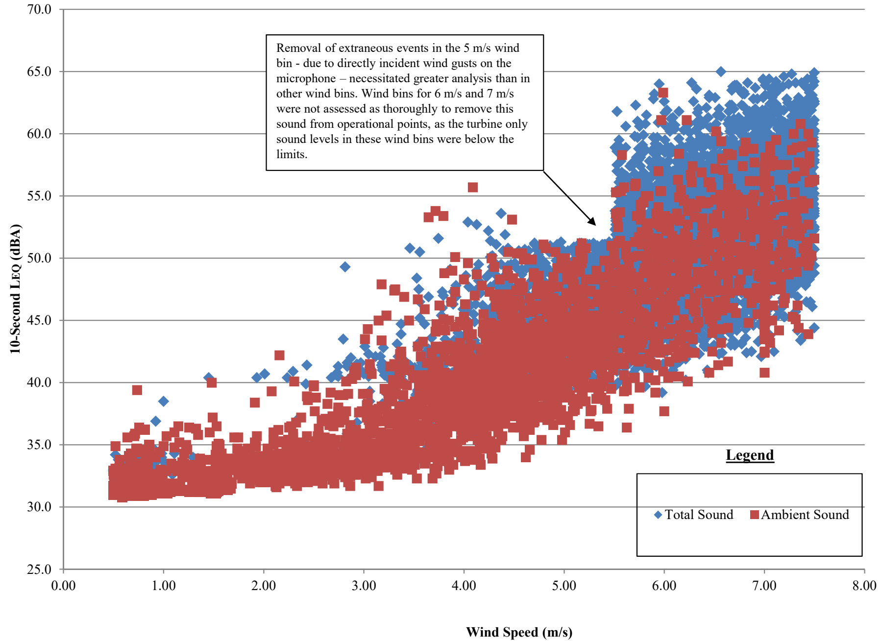
Figure 2 - Valid L_{EQ} Data - Monitor B
